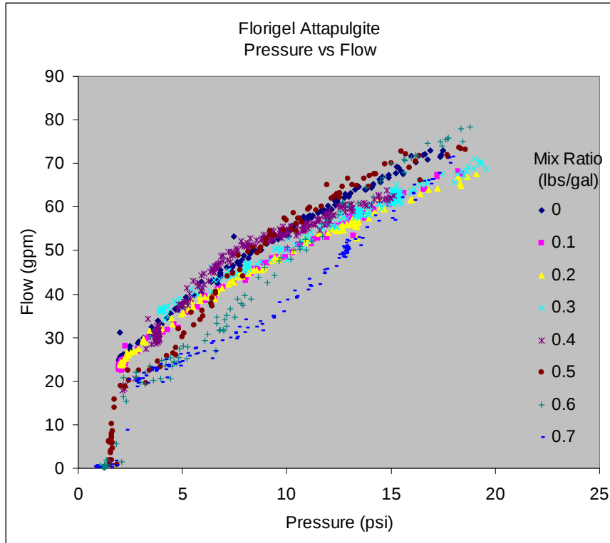
Figure 3.19. Florigel Attapulgate pressure versus flow testing results.
