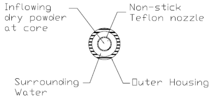
Figure 2.15. Cross-section of eductor showing powder / water interface (mixing zone).
