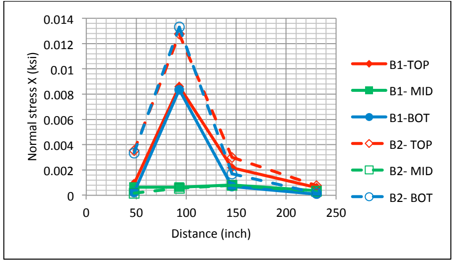
Figure 3.23: Comparison of Normal Stress in X Direction for Cases B1 and B2
