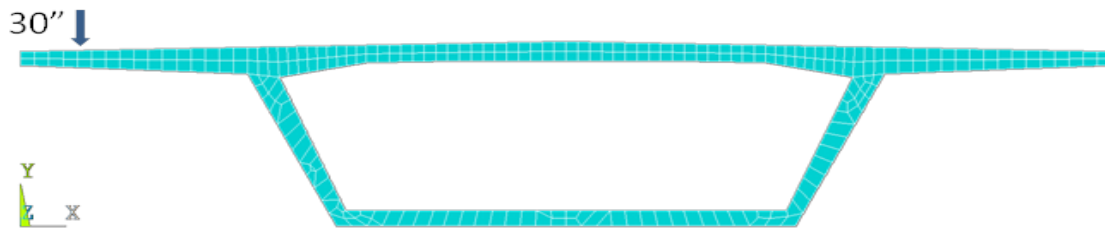
Figure 3.27: Load Positions on Wing 30 Inches from Edge of Wing Slab
