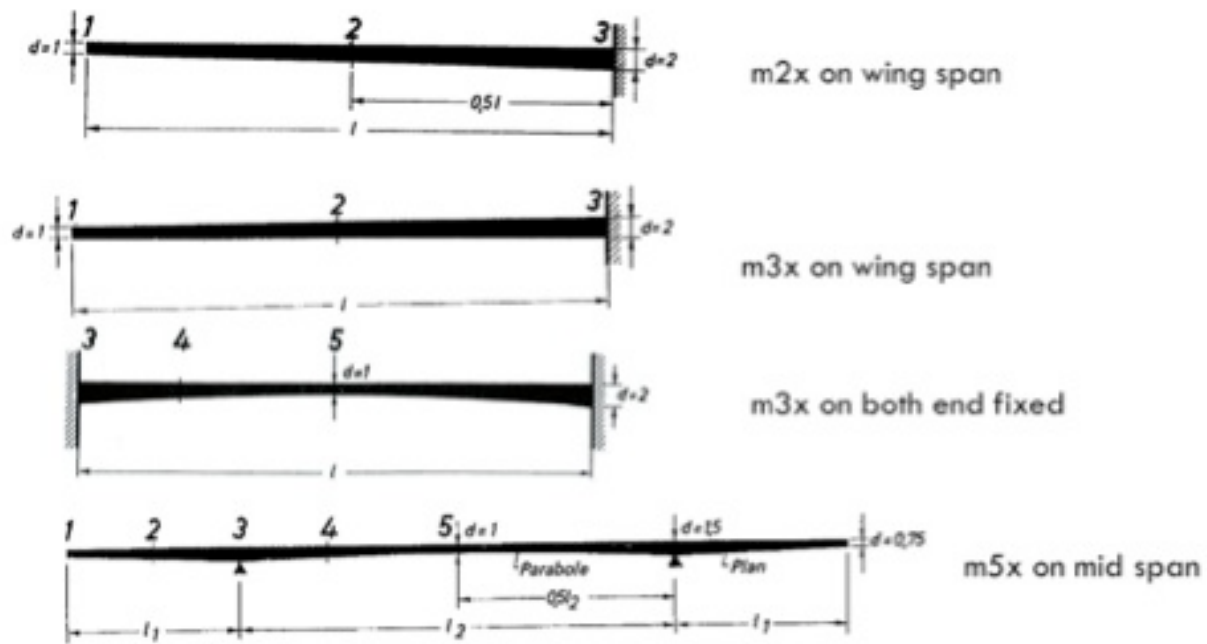
Figure 4.2: Moment Reading Locations for Various Boundary Conditions (from Homberg Charts)
