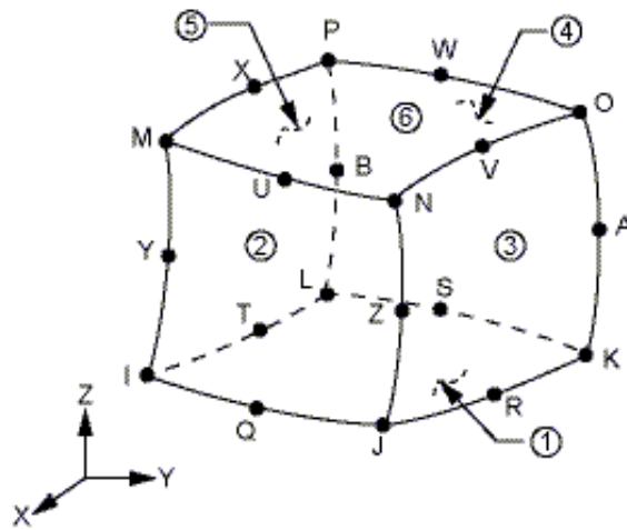
Figure 2.3: SOLID186 Element Geometry (ANSYS 2010)
