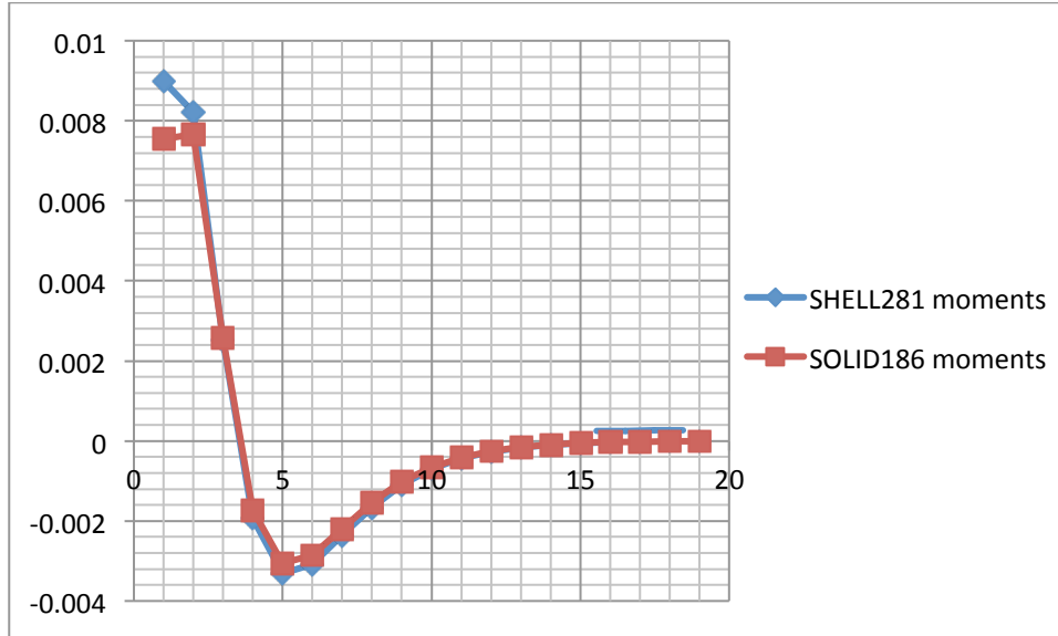
Figure 4.4: Comparison of Moment Function for SHELL281 vs. SOLID186 Element Models
