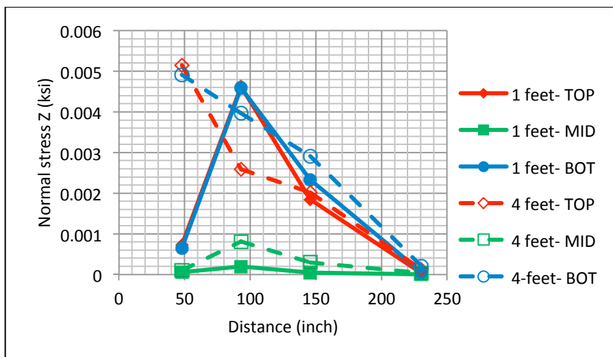
Figure 3.14: Comparison of Normal Stress in Z Direction for Cases A3-A and A3-B
