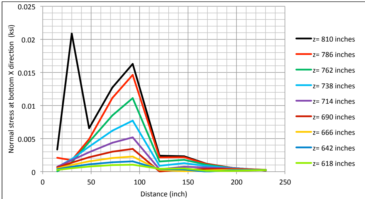
Figure 3.32: Normal Stress X Direction at Bottom Surface
