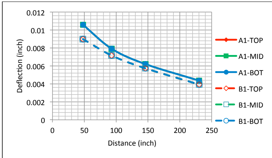
Figure 3.17: Comparison of Deflection for Cases A1 and B1
