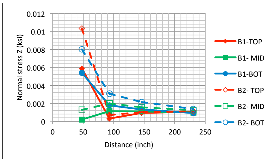
Figure 3.22: Comparison of Normal Stress in Z Direction for Cases B1 and B2
