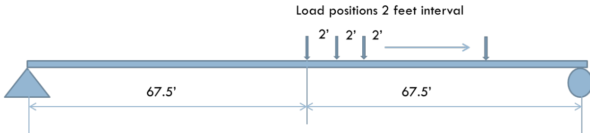
Figure 3.28: Load Positions at 2-foot Intervals up to 16 Feet from Mid Span (Not to Scale)
