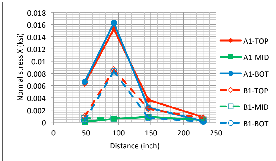
Figure 3.19: Comparison of Normal Stress in X Direction for Cases A1 and B1
