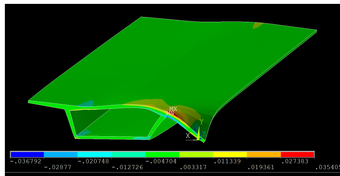
Figure 3.11: Exaggerated Deflected Shape for Case A3-A
