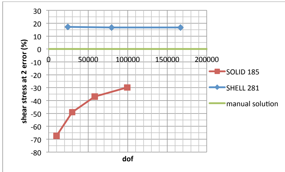
Figure 2.13: Shear Stress at Location 2 with Increasing Degrees of Freedom
