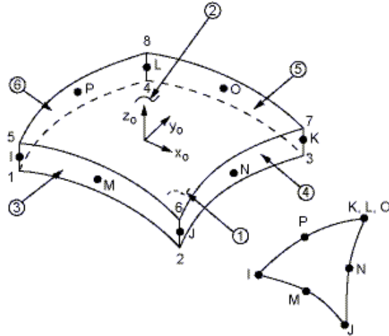
Figure 2.2: SHELL281 Element Geometry (ANSYS 2010)
