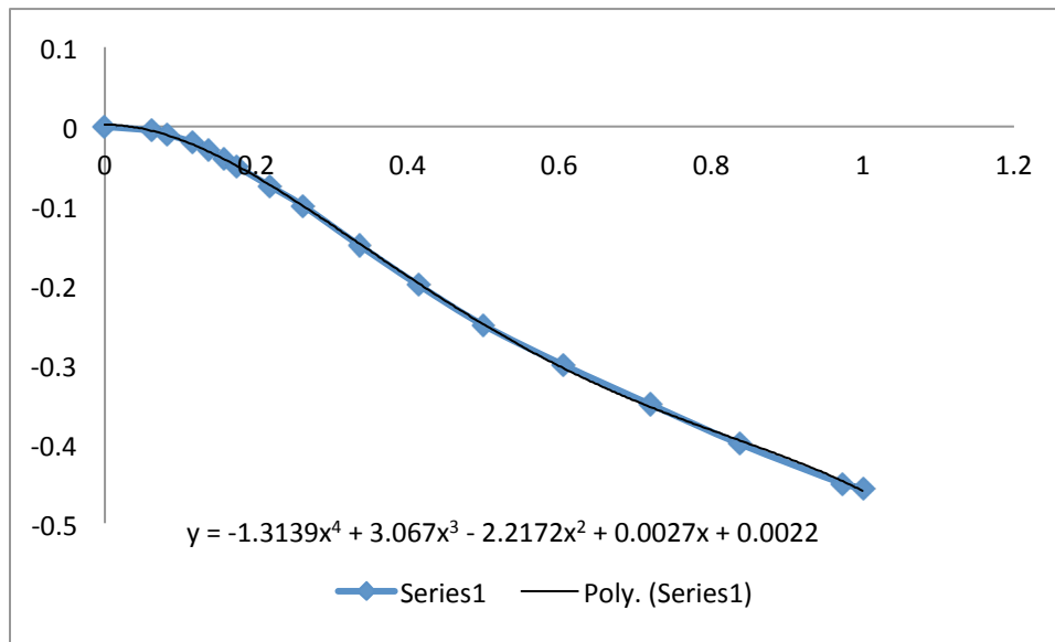
Figure 5.15: Moment Function for y = 0.4 Grid Line for m3x Wing Span
