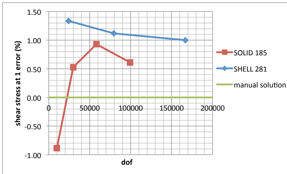
Figure 2.12: Shear Stress at Location 1 with Increasing Degrees of Freedom
