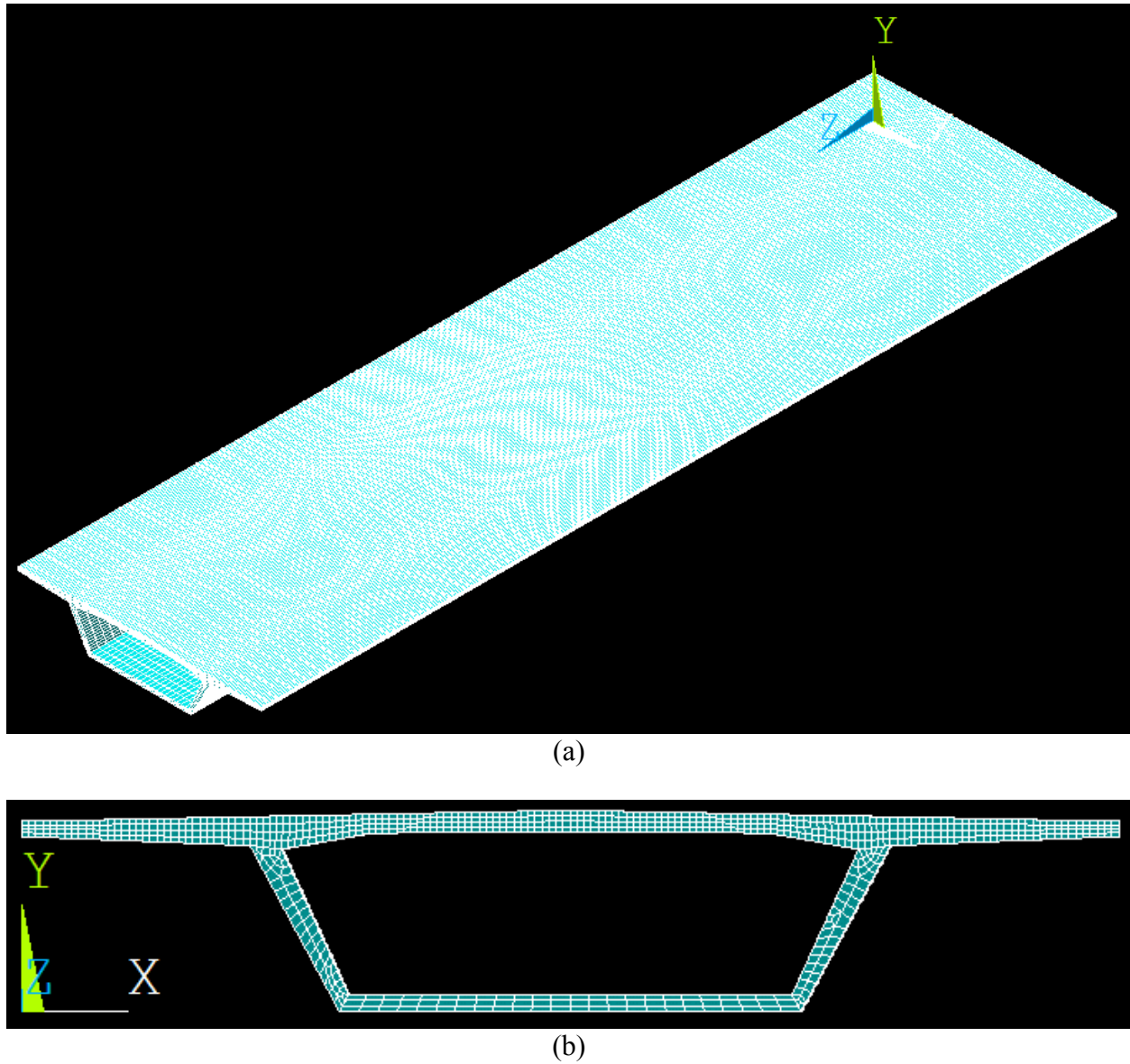
Figure 3.2: FE Bridge Model: (a) Oblique View (b) Sectional View
