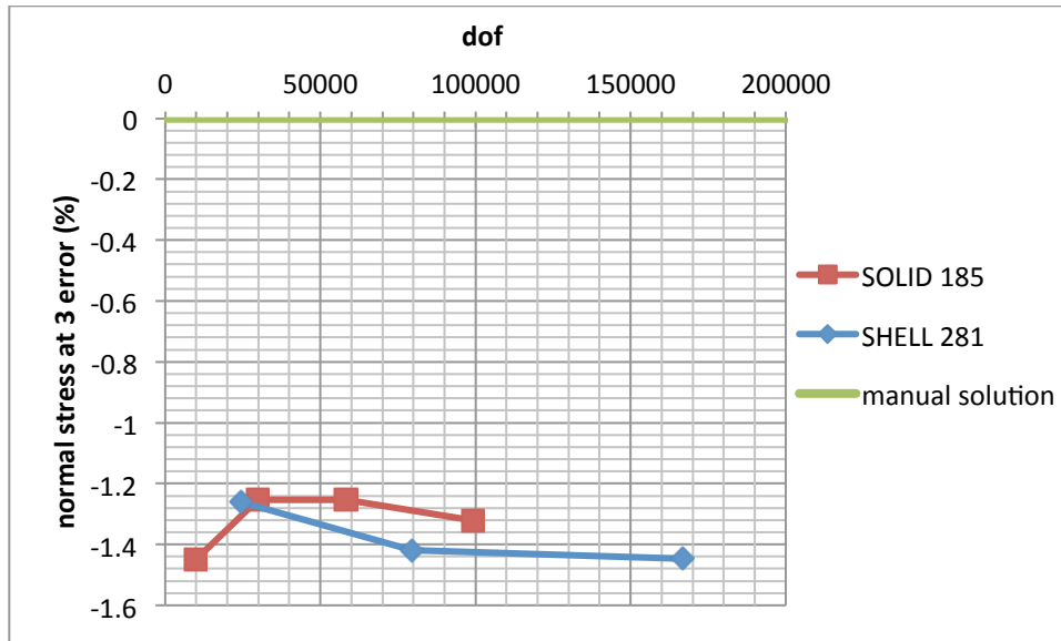
Figure 2.11: Normal Stress at Location 3 with Increasing Degrees of Freedom
