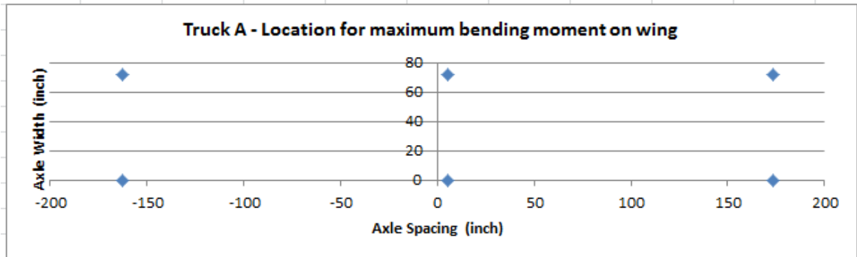
Figure 5.6: Sample Wheel Location for Maximum Moment
