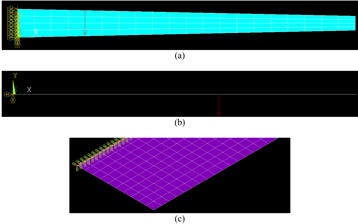
Figure 4.3: ANSYS Cantilever Plate (a) SOLID186 Element Model Cross-sectional View (b) SHELL281 Model Cross-sectional View (c) Oblique View of Plate Model
