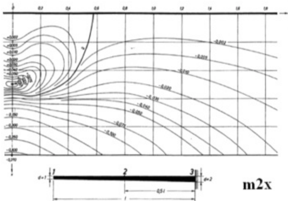
Figure 4.1: Influence Surface Moment Coefficients at Location 2 ( m_{2x} )
