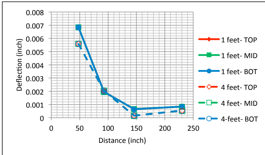
Figure 3.13: Comparison of Deflection for Cases A3-A and A3-B
