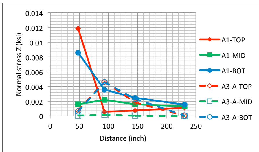
Figure 3.9: Comparison of Normal Stress Z Direction for Cases A1 and A3-A
