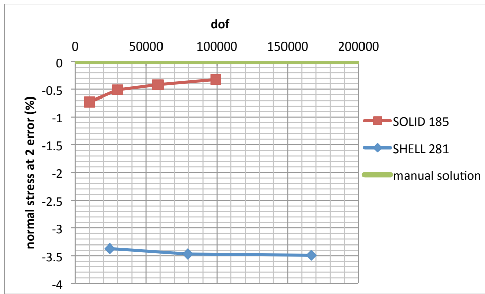
Figure 2.10: Normal Stress at Location 2 with Increasing Degrees of Freedom
