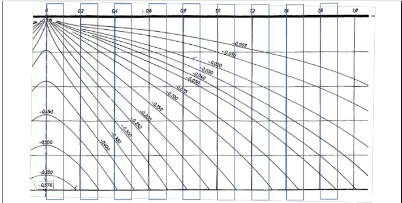
Figure 5.14: Homberg Chart for m3x Wing Span with Additional Grid at 0.1 Interval
