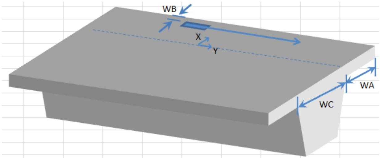
Figure 5.2: Schematic Representation of Required Data for Tool
