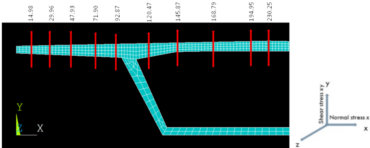
Figure 3.29: Reading Locations across the Width of Bridge, in Inches
