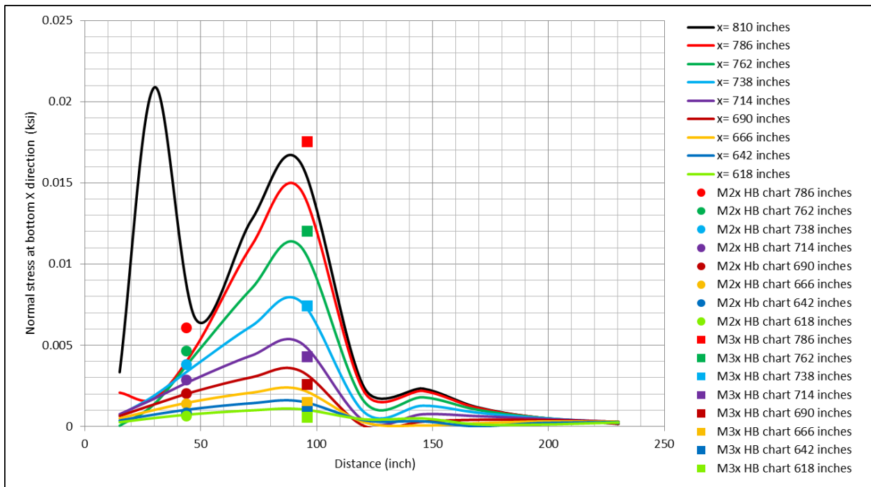
Figure 3.34: Comparison of Normal Stress in X Direction for FEM Results and Homberg Chart (Stress from Bottom Surface)
