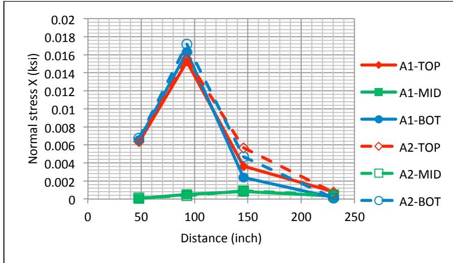
Figure 3.6: Normal Stress X Direction for Cases A1 and A2
