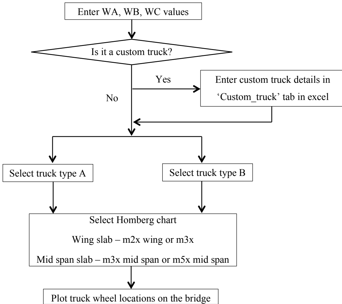
Figure 5.9: Flow Chart of the Tool
