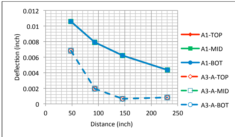
Figure 3.8: Comparison of Deflections for Cases A1 and A3-A
