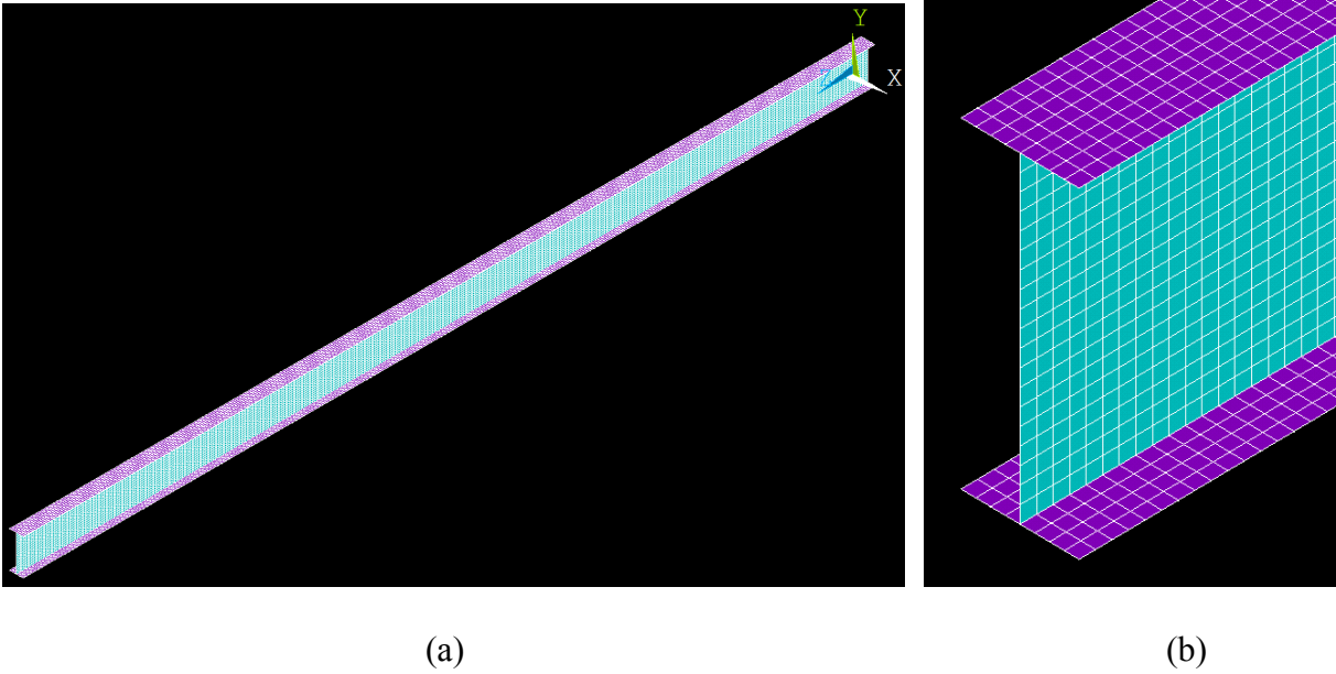
Figure 2.4: Beam Model with SHELL281 Elements: (a) Complete Beam (b) Enlarged Section
