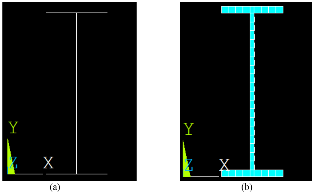
Figure 2.1: Sample I-shaped Beam for (a) SHELL281 Model and (b) SOLID186 Model
