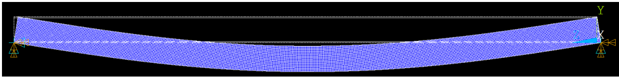
Figure 2.6: Deflected Shape of Beam under Pressure Load (Deflection Exaggerated)
