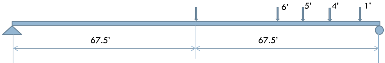
Figure 3.24: Load Positions with No Diaphragm Modeled at Support
