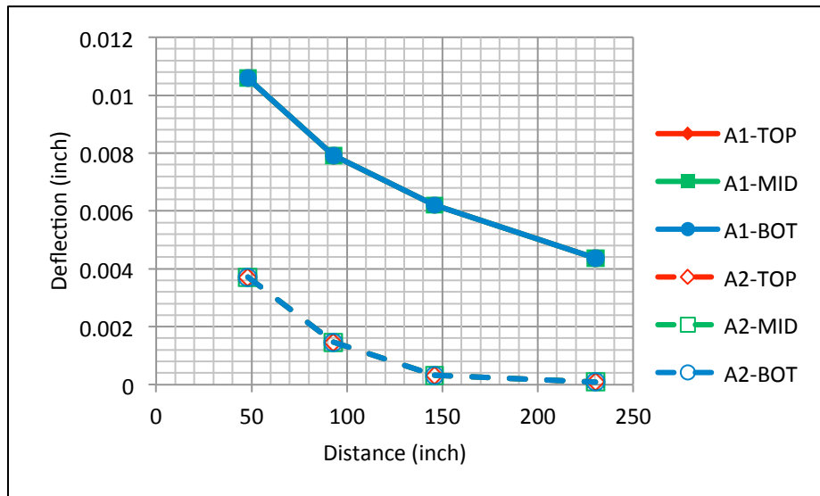
Figure 3.5: Deflection for Cases A1 and A2
