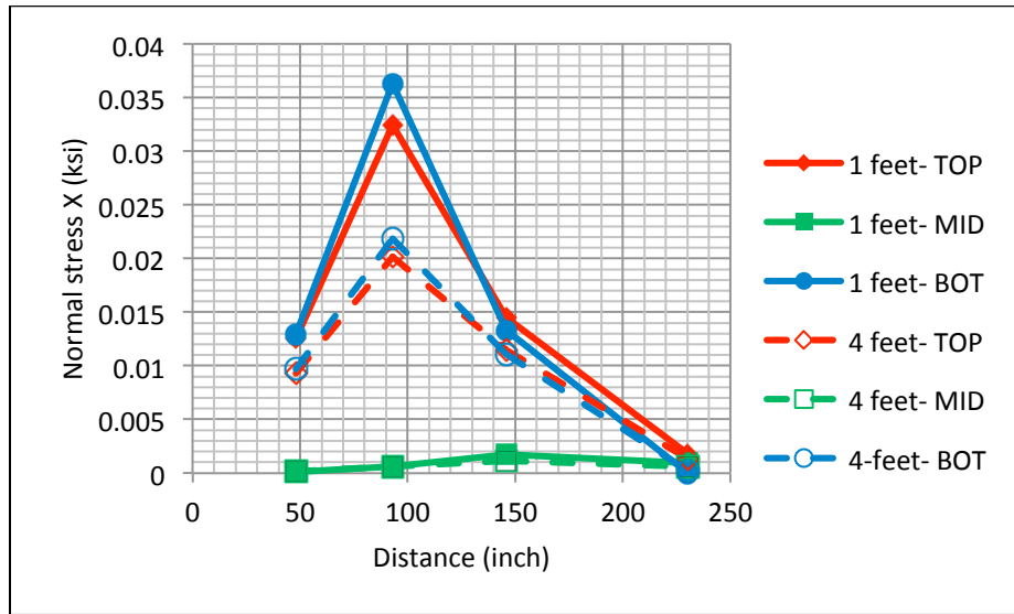
Figure 3.15: Comparison of Normal Stress in X Direction for Cases A3-A and A3-B
