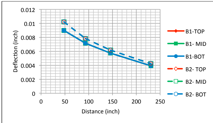
Figure 3.21: Comparison of Deflection for Cases B1 and B2
