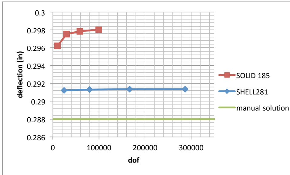
Figure 2.7: Comparison of SHELL281, SOLID186 and Manual (Analytical) Solutions
