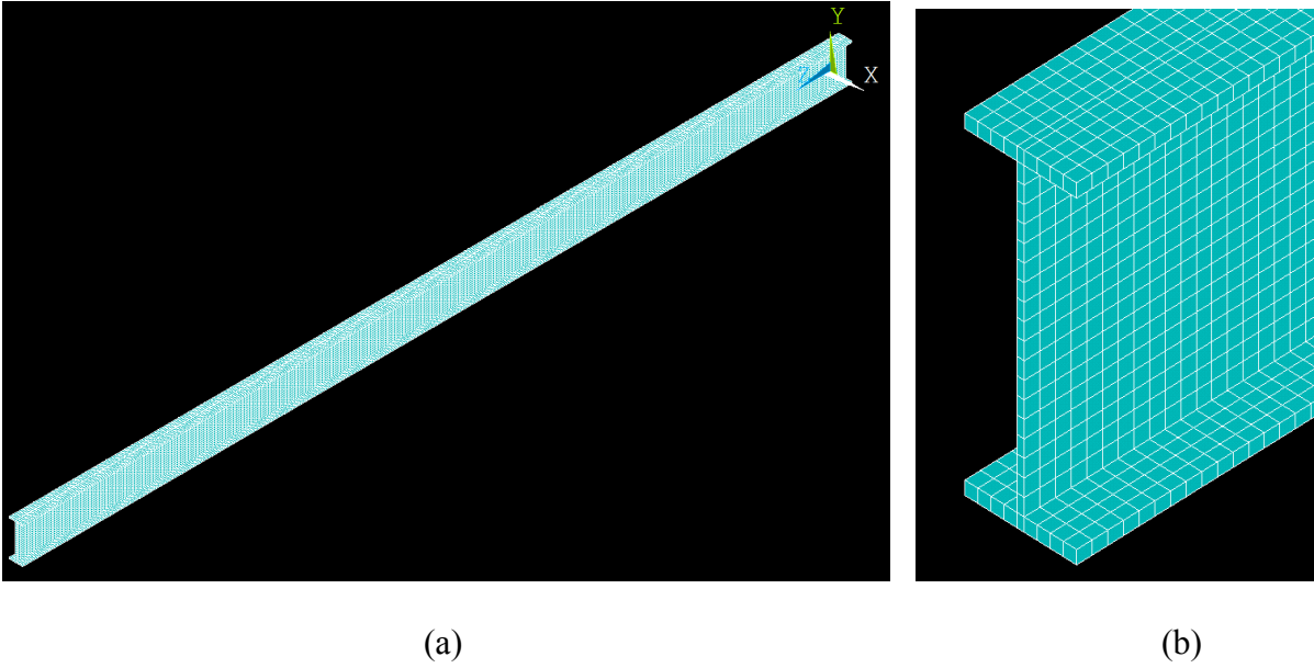
Figure 2.5: Beam Model with SOLID186 Elements: (a) Complete Beam (b) Enlarged Section
