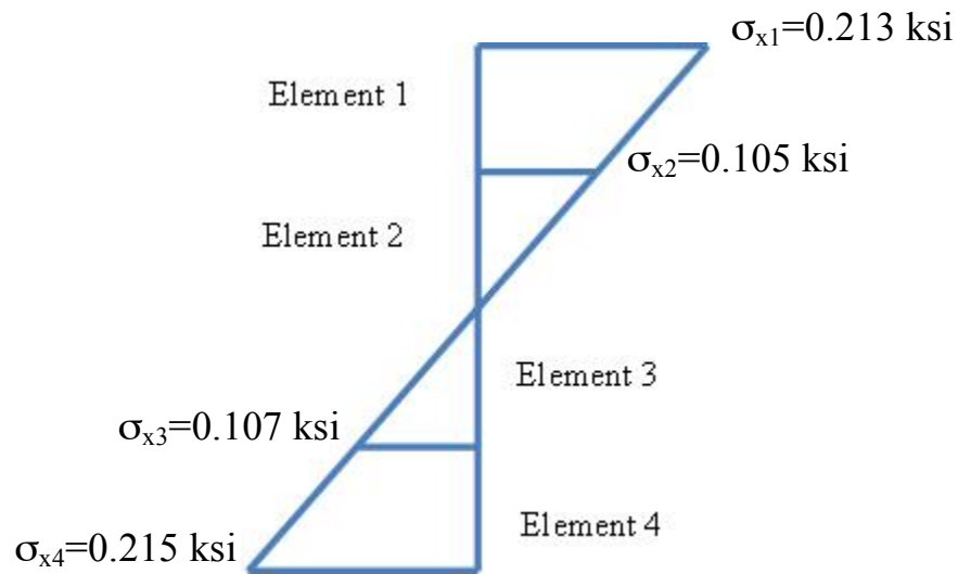
Figure 4.9: Schematic Representation of Stress Envelope (Sample Stresses in X Direction for TTT#3 Truck)
