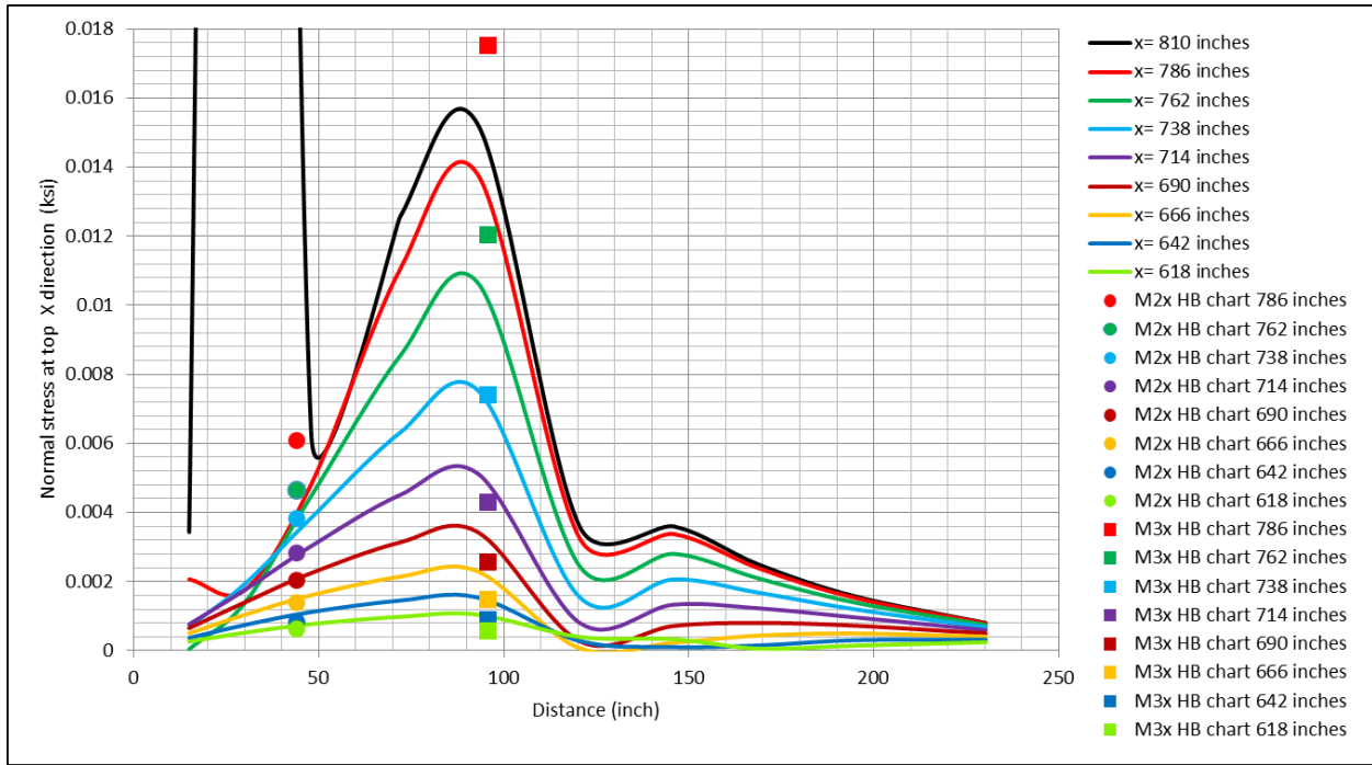
Figure 3.33: Comparison of Normal Stress in X Direction for FEM Results and Homberg Chart (Stress from Top Surface)
