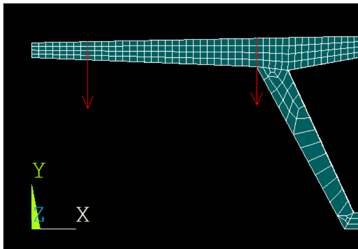
Figure 4.14: Bridge Section Showing m2x Wing with Applied HS20 Truck Load
