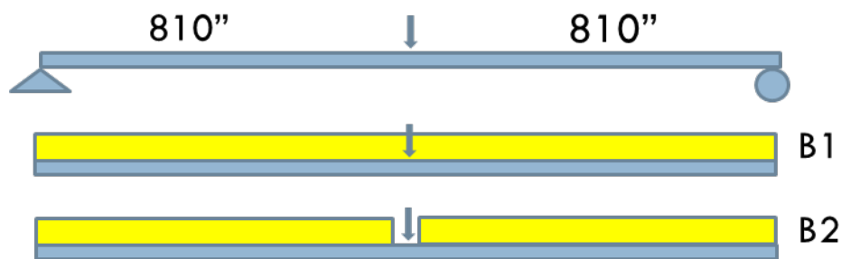
Figure 3.20: Loading Condition for Cases B1 and B2
