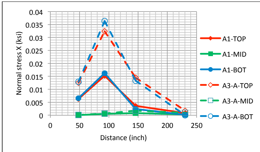
Figure 3.10: Comparison of Normal Stress X Direction for Cases A1 and A3-A
