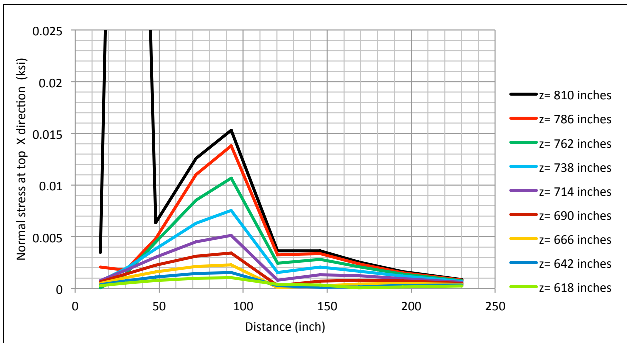
Figure 3.30: Normal Stress X Direction at Top Surface
