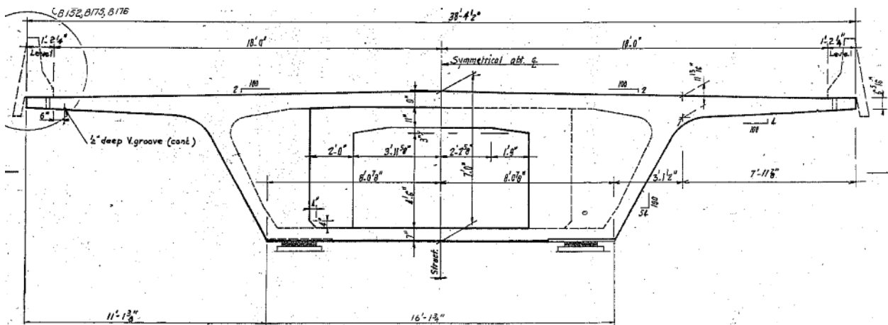
Figure 3.1: Channel Five Bridge Cross Section
