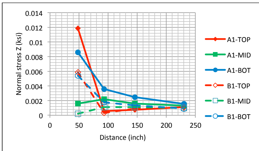
Figure 3.18: Comparison of Normal Stress in Z Direction for Cases A1 and B1
