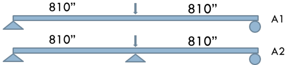
Figure 3.4: Loading Conditions for Cases A1 and A2
