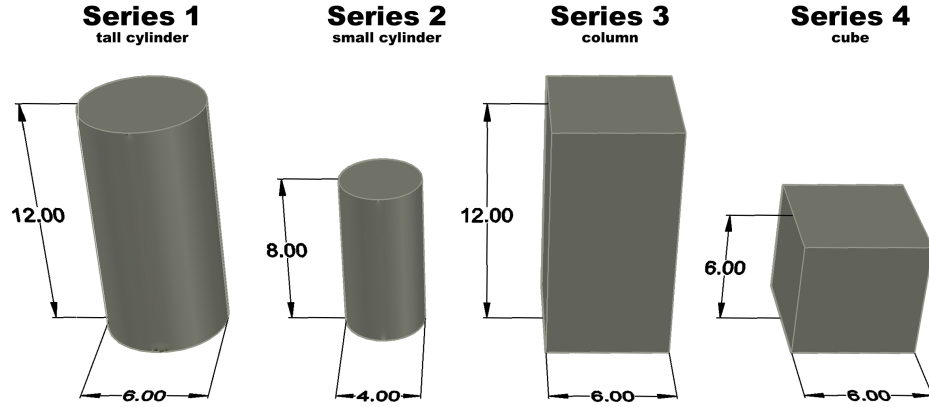
Figure 3.2: Test series (dimensions in inches)
