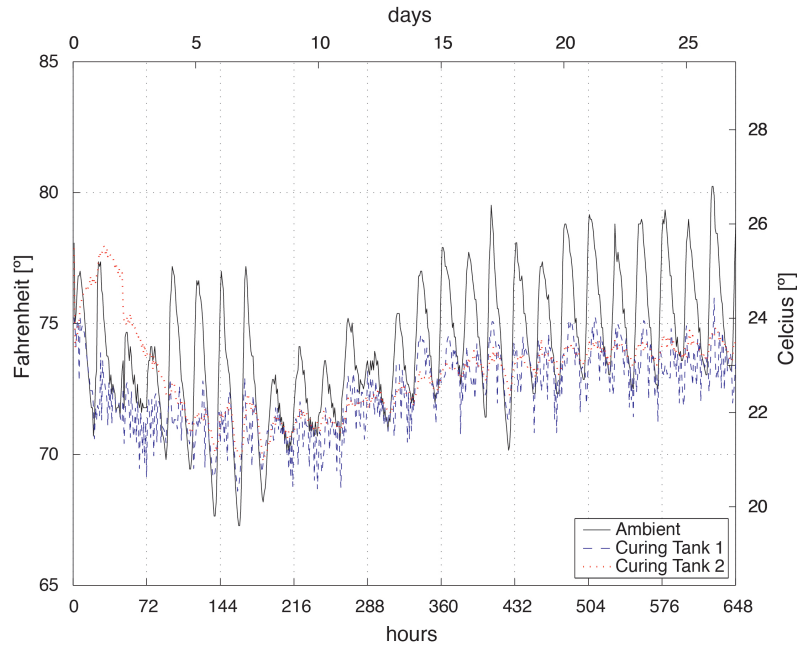
Figure 3.5: Curing temperature throughout curing period
