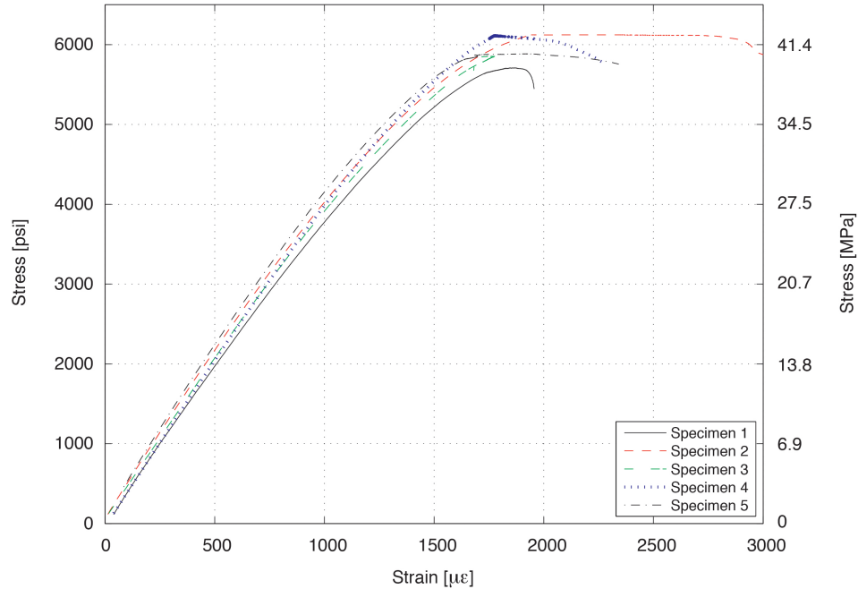
Figure 4.4: Relationship between compressive stress and longitudinal strain under conventional friction (load sustained at 90% of the measured control group strength)
