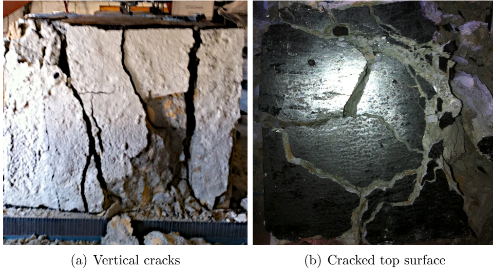
Figure 4.13: Fracture pattern of test group cubes (reduced friction)
