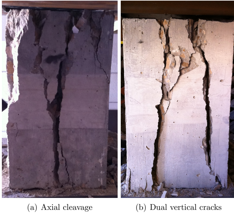
Figure 4.12: Fracture pattern of test group columns (reduced friction)
