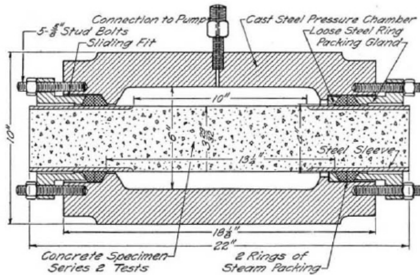
Figure 2.1: Hydraulic pressure chamber according to Richart et al. (1928)
