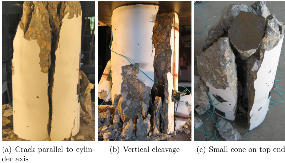
Figure 4.11: Fracture pattern of test group cylinders (reduced friction)
