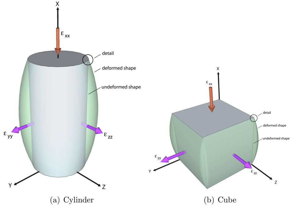
Figure 5.6: Deformed and undeformed specimen shapes (global behavior)
