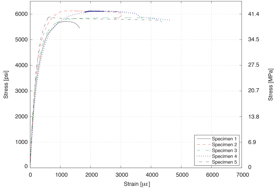
Figure 4.5: Relationship between compressive stress and transverse strain under conventional friction (load sustained at 90% of the measured control group strength)
