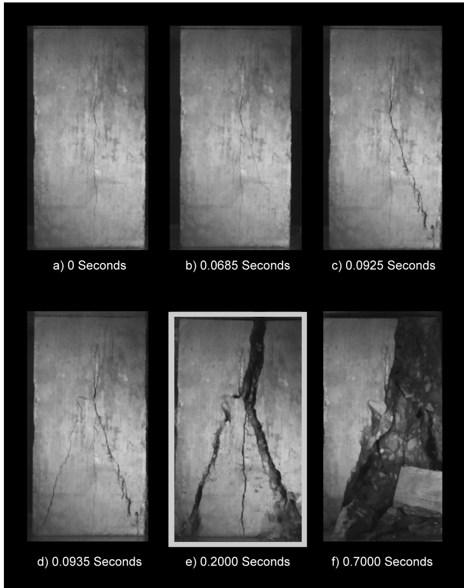
Figure 4.15: Column failure under regular friction
