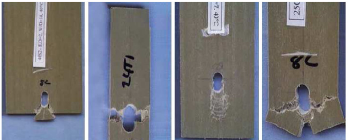
Figure 9 Typical Failure Modes of Mechanical Connections (Potyrała, 2011).
