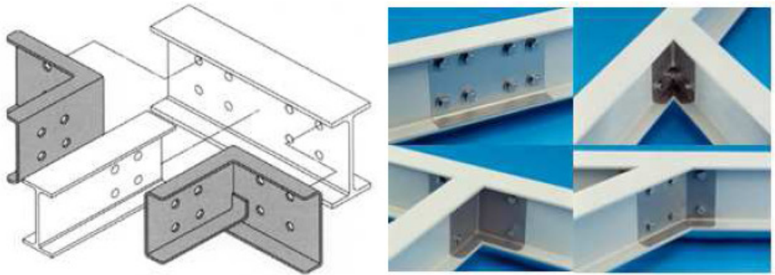
Figure 7 Mechanical Connections for Structural FRP Shapes (Potyrała, 2011).
