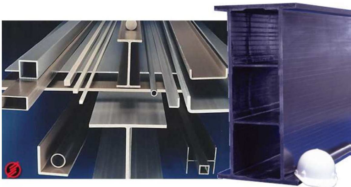
Figure 5 The Range of Composite Profiles Reinforced with Glass and Carbon Fibers, as Produced by Strongwell (Potyrała, 2011).
