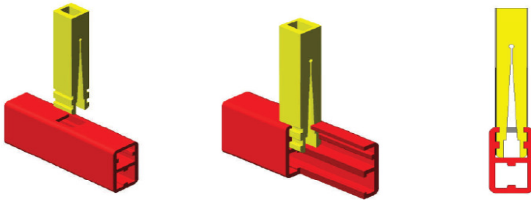
Figure 6 Composite Support & Solutions, Inc. “Snaplock” Connection, (Caltrans, 2008).
