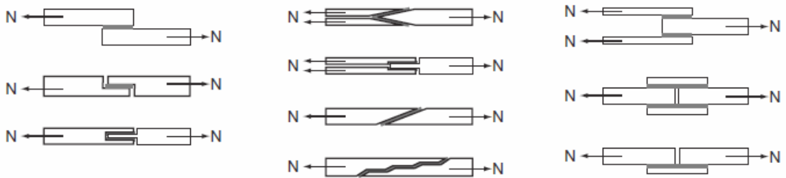
Figure 8 Various Bonded FRP Connection Configurations (Potyrała, 2011).
