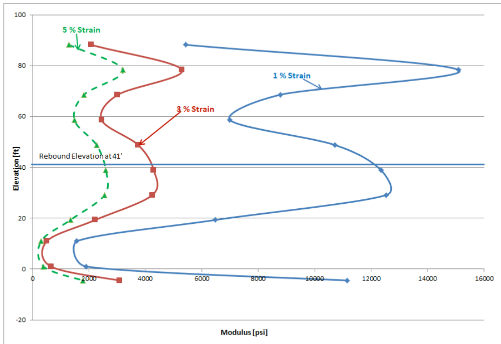
Figure 4.34 John Young Average PPMT Elastic Modulus versus Elevation
