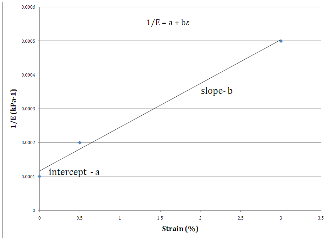
Figure 4.33 Typical 1/E versus strain plot based on the Kondner (1963) model
