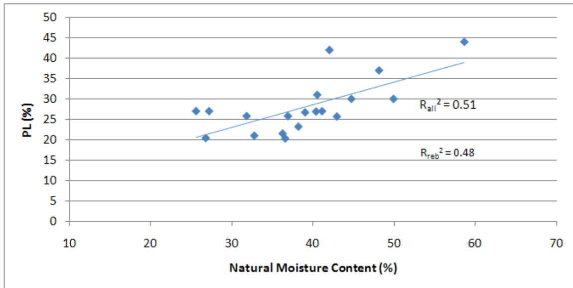
Figure 4.11 Research Phase Moisture Content versus Plastic Limit with Regression Coefficients for all Soils and Rebound Soils
