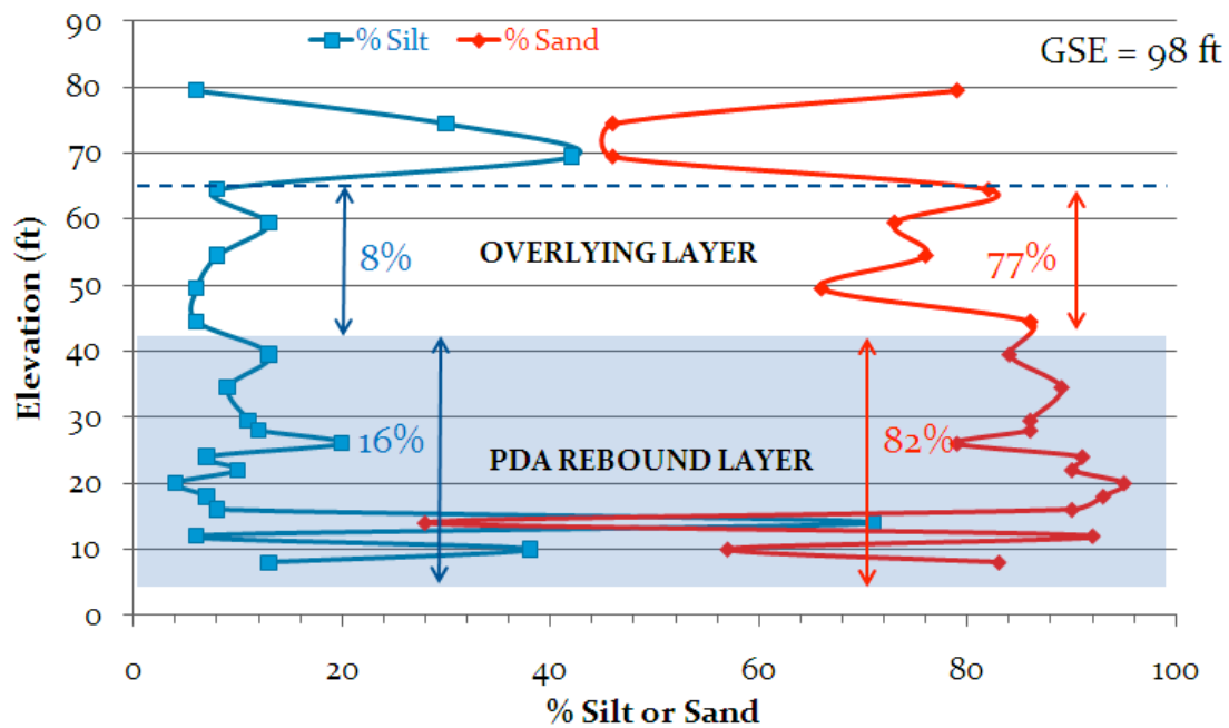
Figure 4.5 Anderson Street Overpass Elevation versus Sand Content and Silt Content
