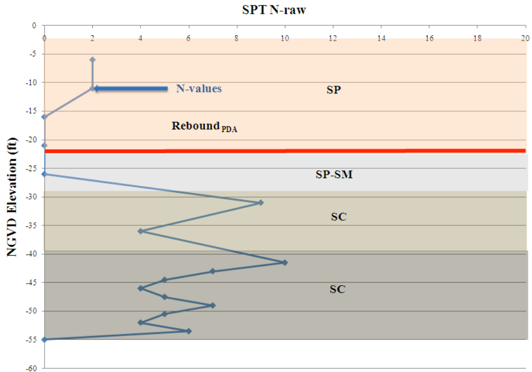
Figure 2.14 Generalized Ramsey Branch Bridge Soil Profile from Borings near End Bent 1
