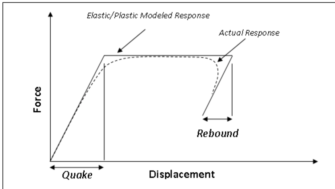
Figure 2.2 Simplified Force Displacement Model with Quake and Rebound
