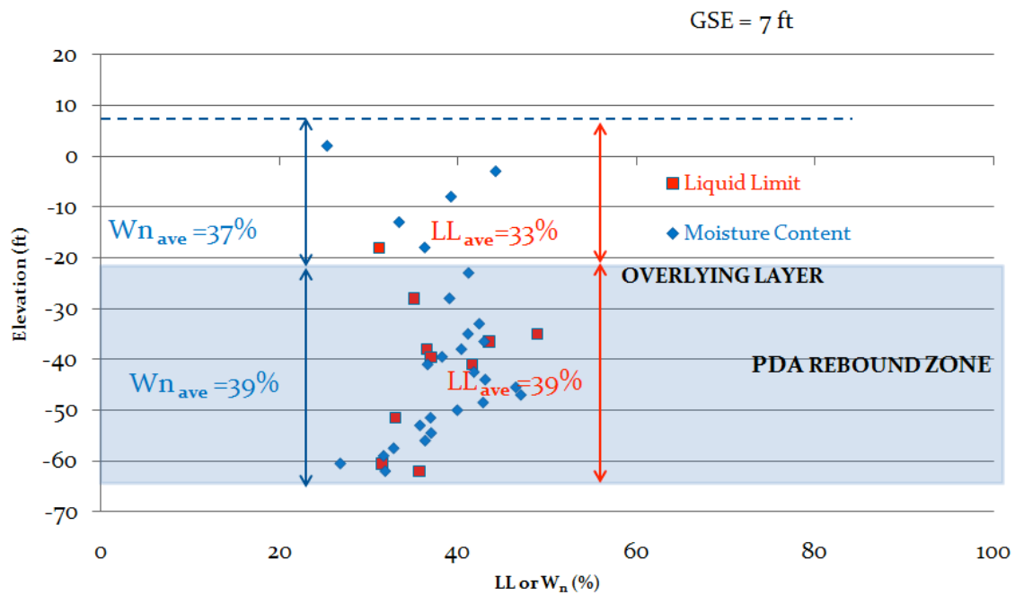
Figure 4.14 Research Phase Ramsey Branch Bridge Elevation versus Liquid Limit and Moisture Content
