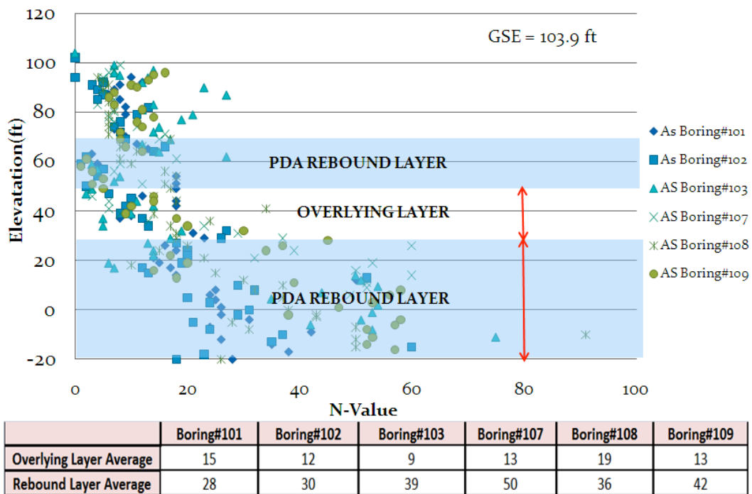
Figure 4.15 Design phase: Anderson Street Overpass Elevation versus N-values with Tabular Averages
