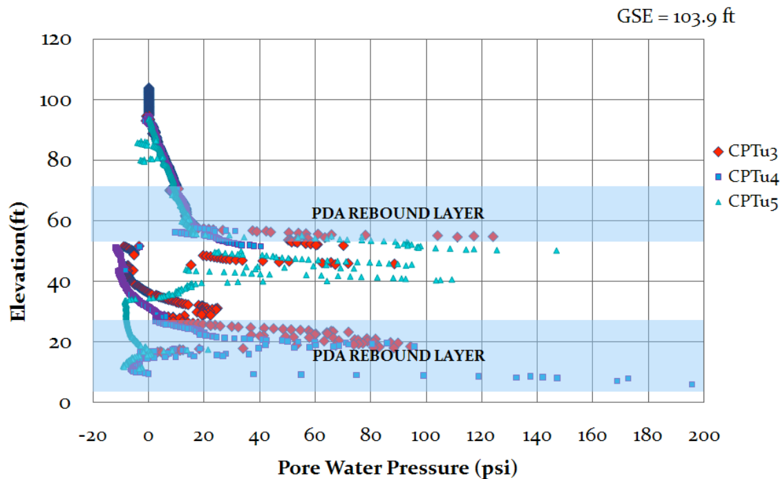
Figure 4.30 Research Phase: Anderson Street Overpass CPTu Pore Water Pressure versus Elevation
