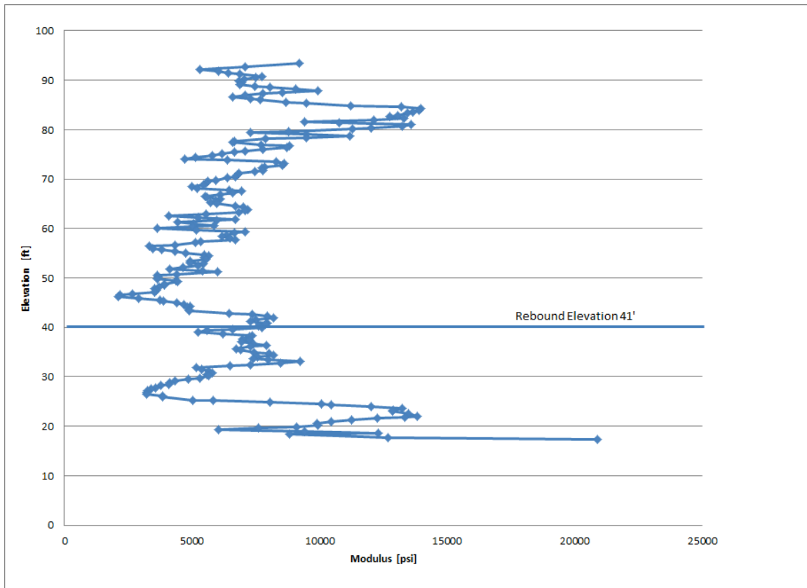
Figure 4.37 John Young Average DMT Elastic Modulus versus Elevation
