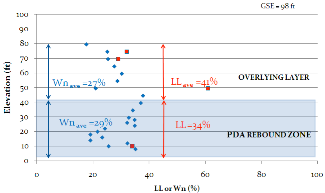
Figure 4.12 Research Phase Anderson Street Overpass Elevation versus Liquid Limit and Moisture Content
