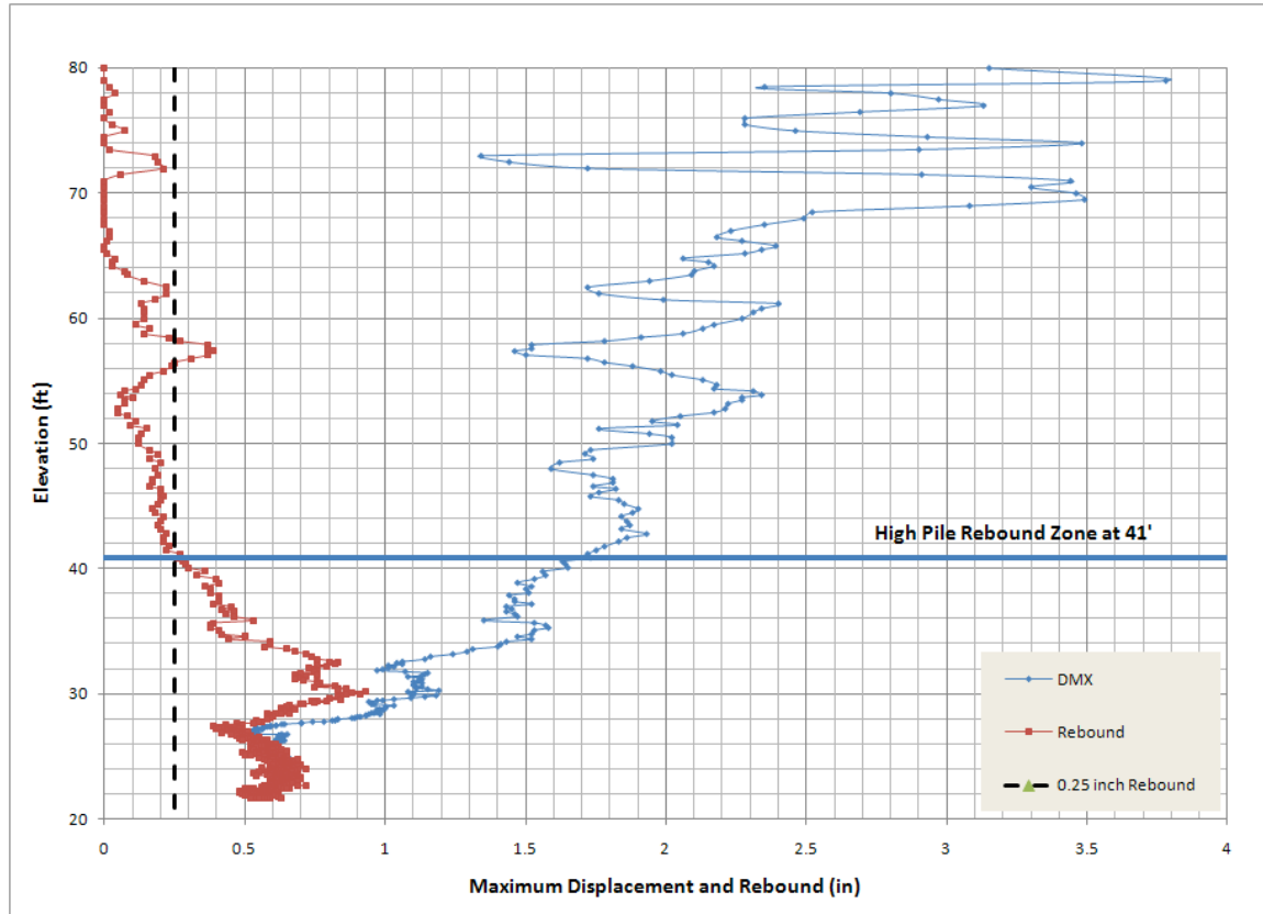
Figure 4.2 PDA Rebound and Maximum Displacement versus Elevation for John Young Pile #6 in End Bent 2 Westbound
