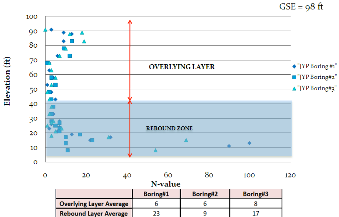
Figure 4.18 Research Phase: John Young Elevation versus N-values with Tabular Averages
