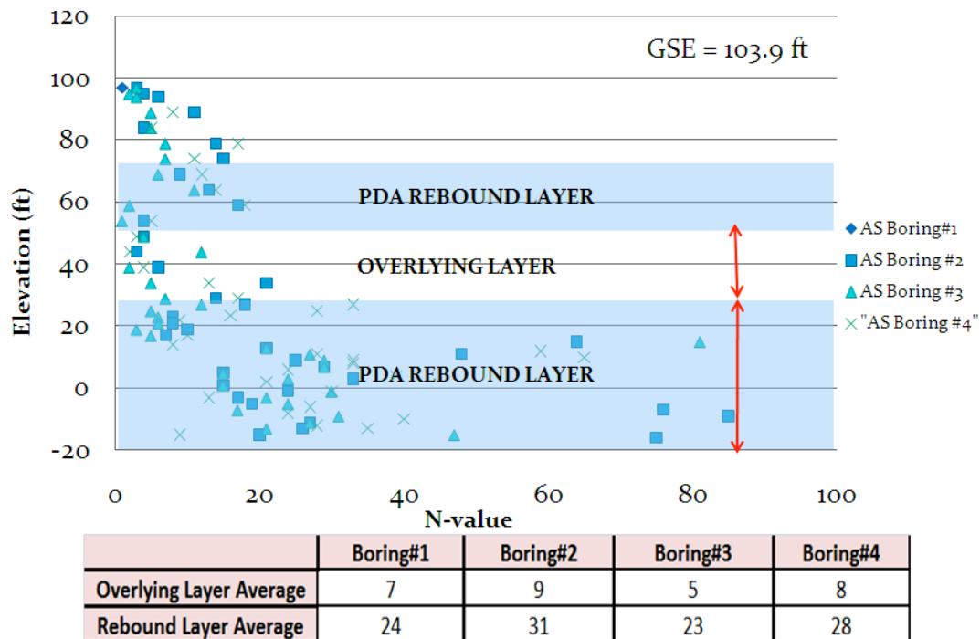
Figure 4.15 Design phase: Anderson Street Overpass Elevation versus N-values with Tabular Averages
