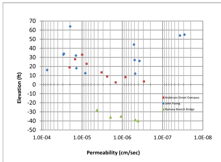
Figure 4.42 Permeability from CU Triaxial Testing versus Elevation
