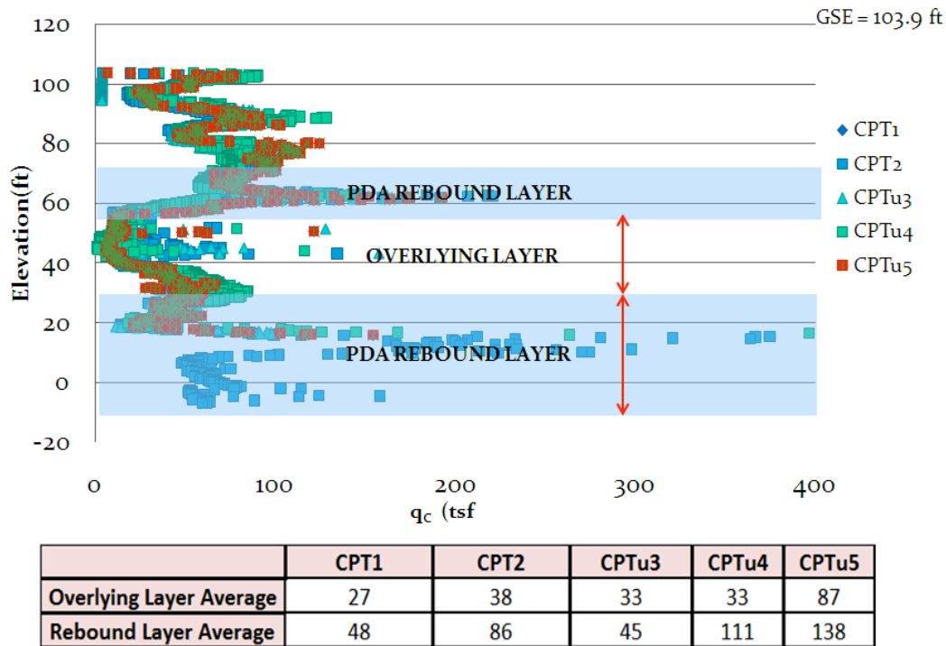
Figure 4.24 Retesting Phase Anderson Street Overpass CPT q_c versus Elevation with Tabular Averages
