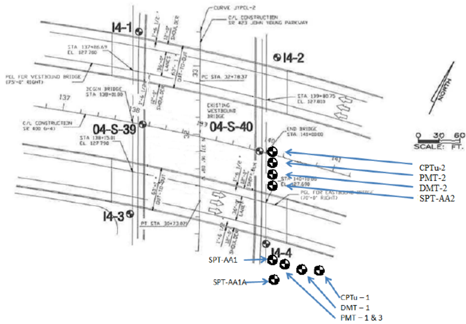
Figure 2.16 Field Retesting Boring Locations for John Young near Pile #6 in End Bent 2 Westbound
