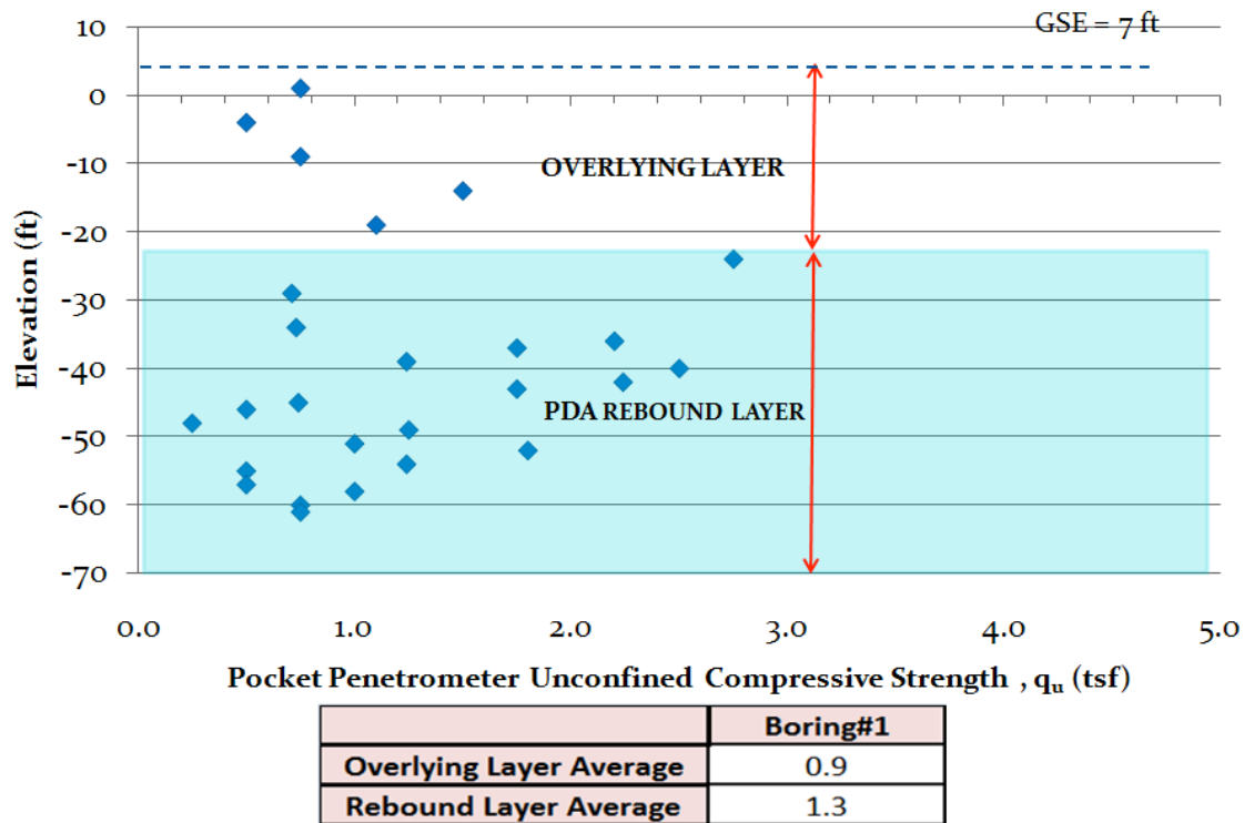
Figure 4.23 Pocket Penetrometer q_u versus Elevation for Ramsey Branch Bridge with Tabular Averages
