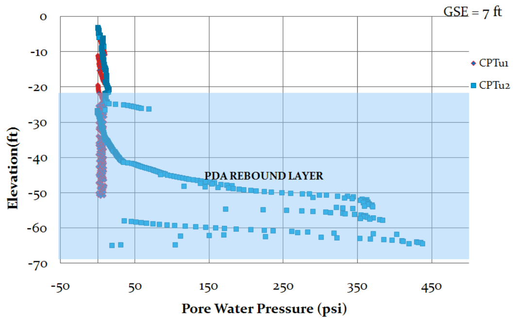
Figure 4.31 Research Phase: John Young CPTu Pore Water Pressure versus Elevation
