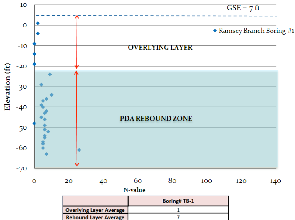
Figure 4.20 Research Phase: Ramsey Branch Bridge Elevation versus N-values with Tabular Averages
