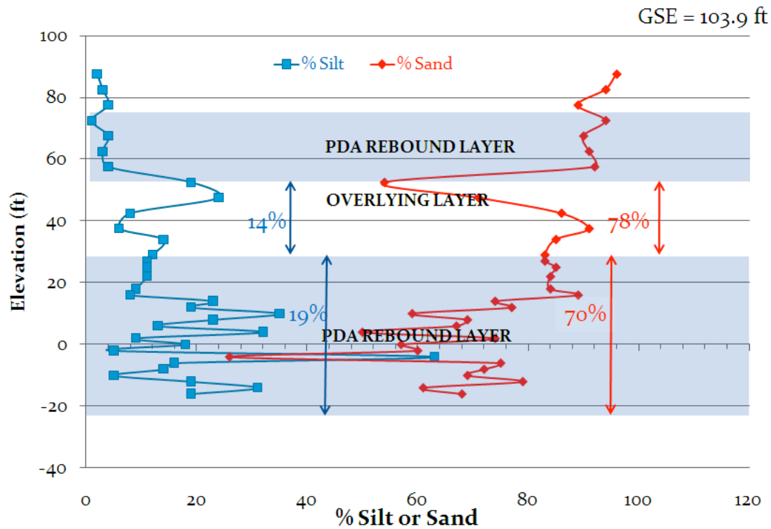
Figure 4.5 Anderson Street Overpass Elevation versus Sand Content and Silt Content
