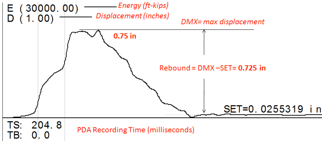
Figure 2.3 PDA Energy (ft-K) Displacement (in) versus Time (ms) Results Showing High Rebound
