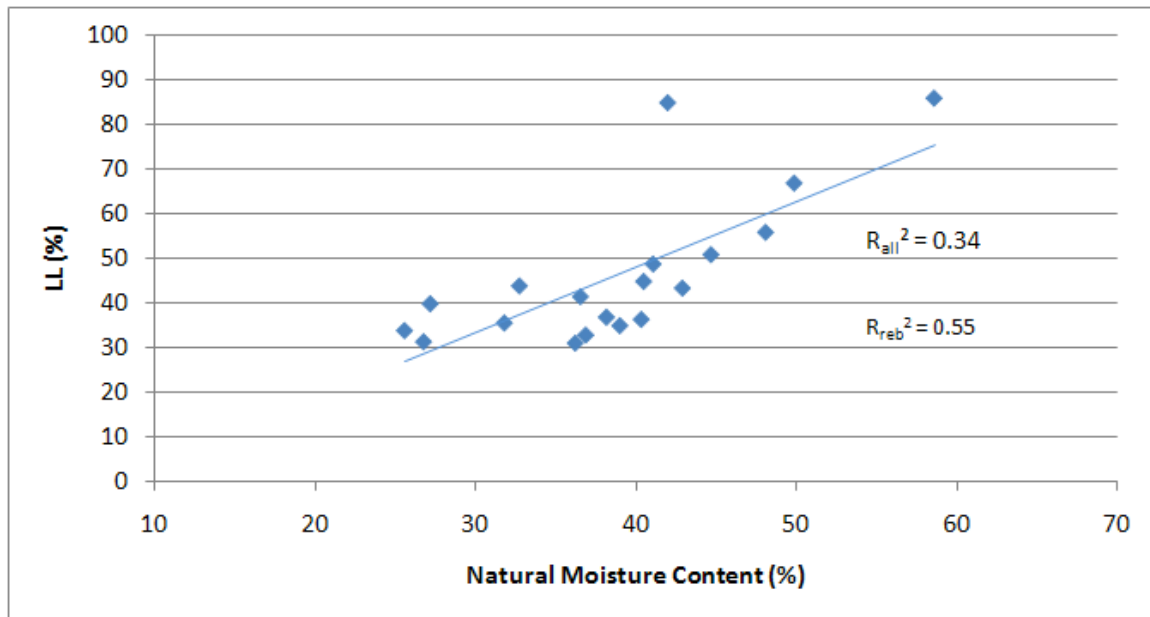
Figure 4.10 Research Phase Moisture Content versus Liquid Limit with Regression Coefficients for all Soils and Rebound Soils
