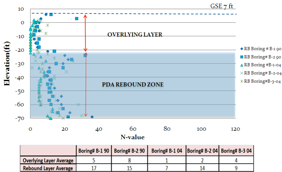
Figure 4.19 Design Phase: Ramsey Branch Bridge Elevation versus N-values with Tabular Averages
