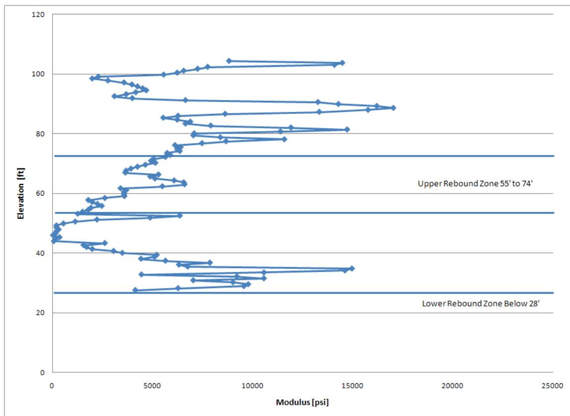
Figure 4.36 Anderson Street Overpass Average DMT Elastic Modulus versus Elevation
