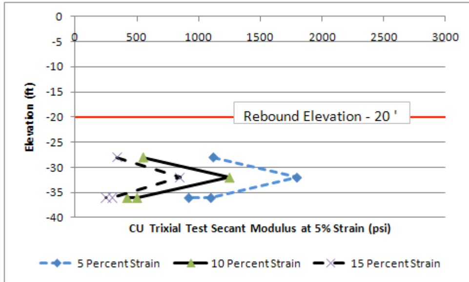
Figure 4.41 Ramsey Branch Bridge CU Triaxial 5, 10 and 15 percent Secant Modulus versus Elevation
