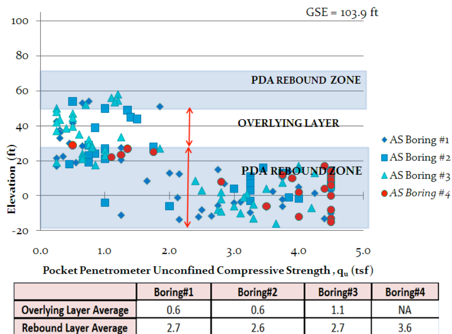
Figure 4.21 Pocket Penetrometer q_u versus Elevation for Anderson Street Overpass with Tabular Averages
