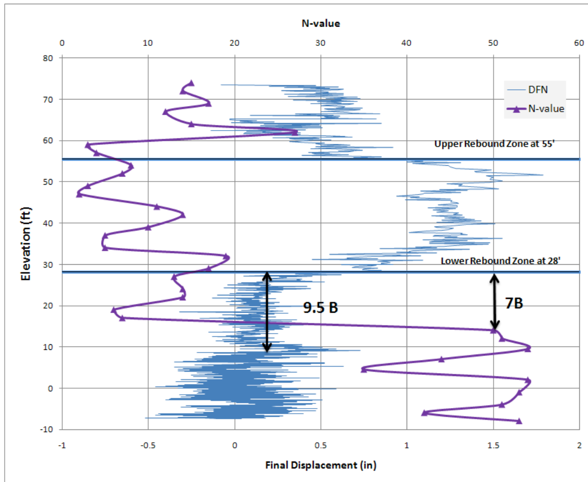
Figure 4.3 PDA Final Displacement and AS-103 N-values versus Elevation for Anderson Street Pile #6 in Pier 6
