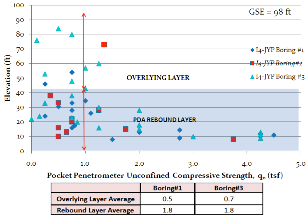
Figure 4.22 Pocket Penetrometer q_u versus Elevation for John Young with Tabular Averages
