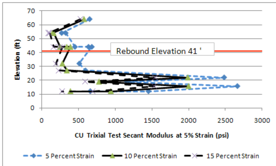
Figure 4.40 John Young CU Triaxial 5, 10 and 15 percent Secant Modulus versus Elevation
