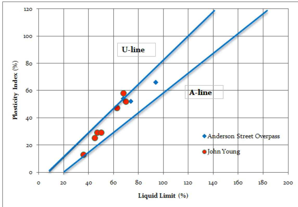
Figure 4.8 Design Phase Plasticity Chart for Anderson Street Overpass and John Young Data from No Rebound Zones
