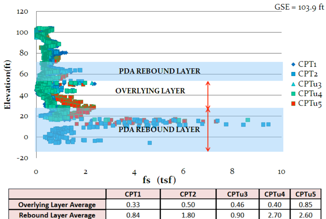
Figure 4.27 Retesting Phase Anderson Street Overpass CPT Friction versus Elevation with Tabular Averages
