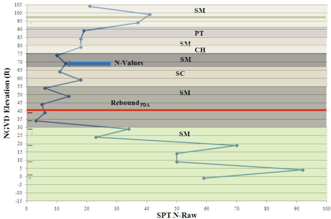
Figure 2.12 Generalized John Young Soil Profile from Borings near End Bent 2 Westbound
