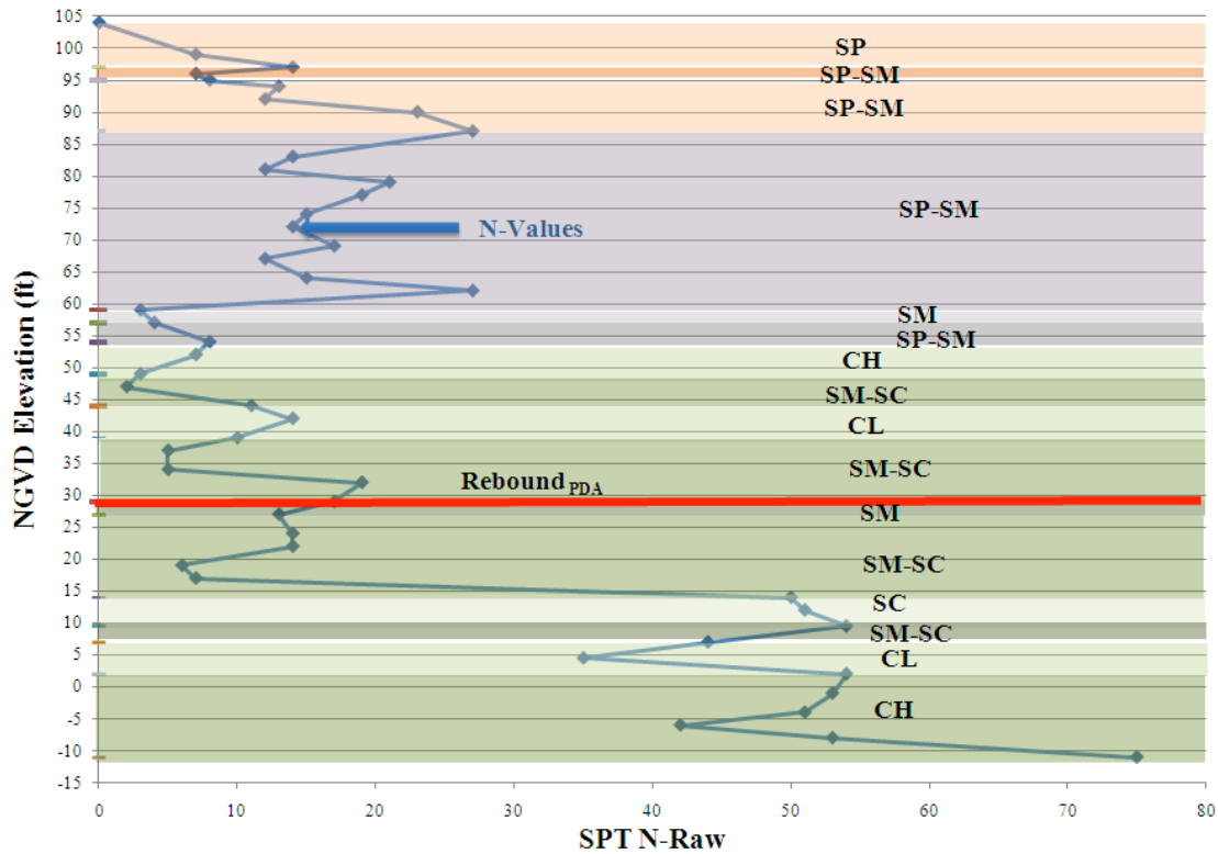
Figure 2.10 Anderson Street Overpass Soil Generalized Profile at Pier 6
