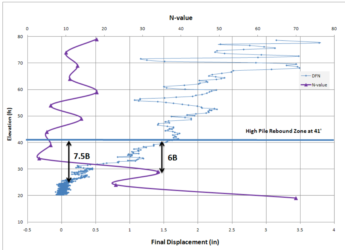
Figure 4.4 PDA Final Displacement and Boring 04-S-49 N-values versus Elevation for John Young Pile #6 in End Bent 2 Westbound
