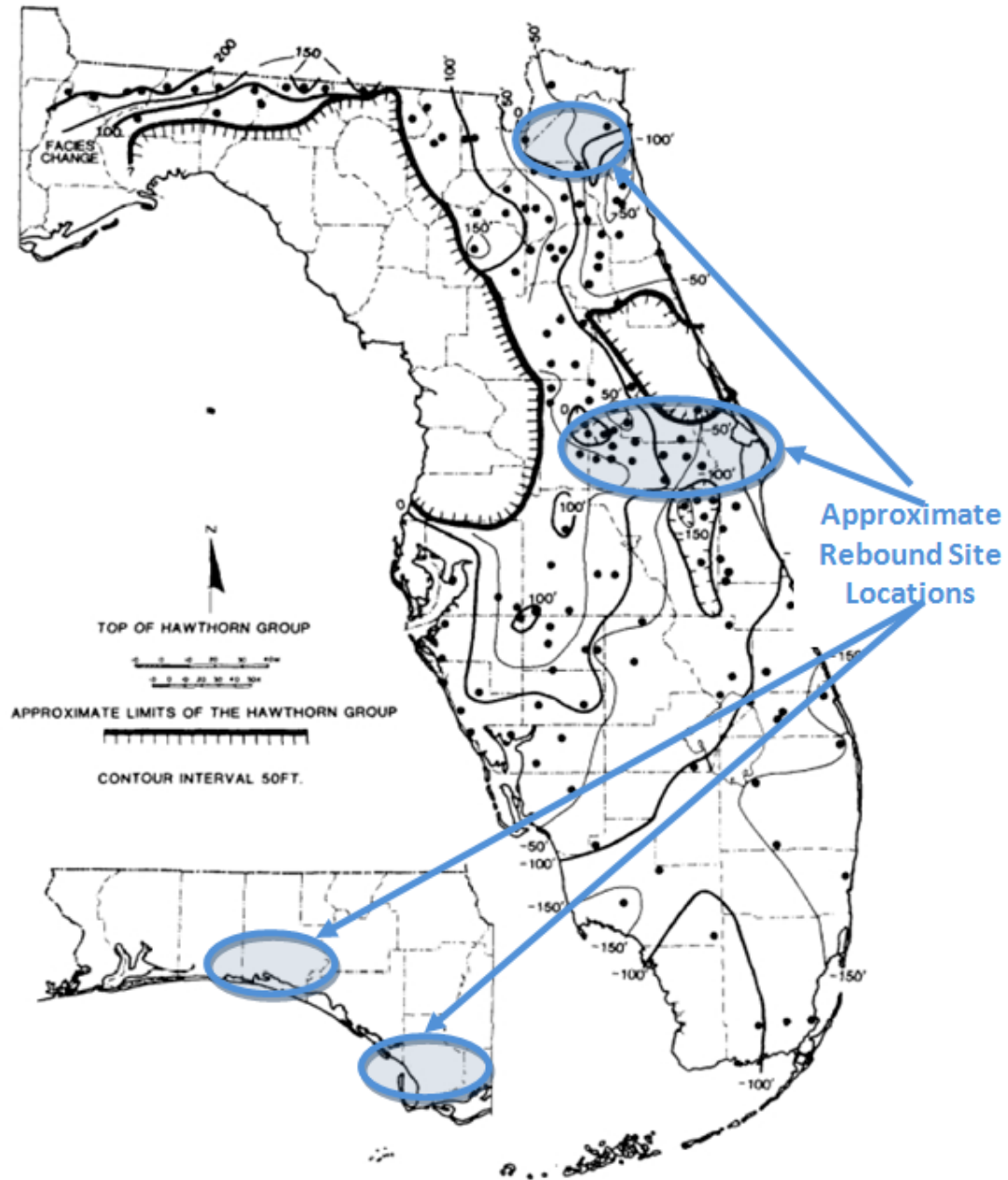
Figure 2.4 Top Elevation Contours of the Hawthorn Group with Approximate High Pile Rebound Site Locations [after (Scott, 1990)]
