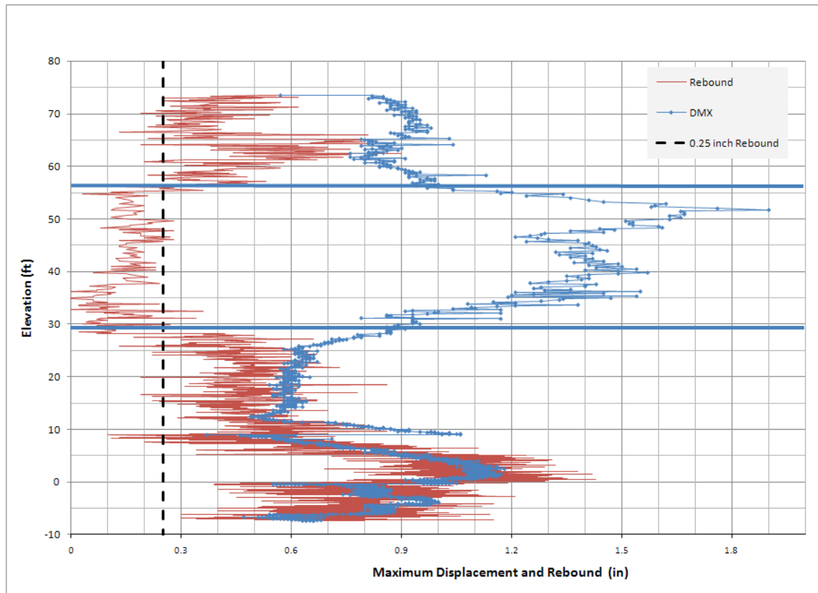
Figure 4.1 PDA Rebound and Maximum Displacement versus Elevation for Anderson Street Pile #6 in Pier 6
