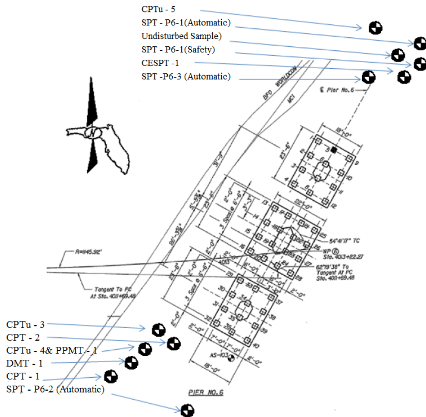
Figure 2.15 Field Retesting Boring Locations for Anderson Street Overpass near Pile #6 Pier 6
