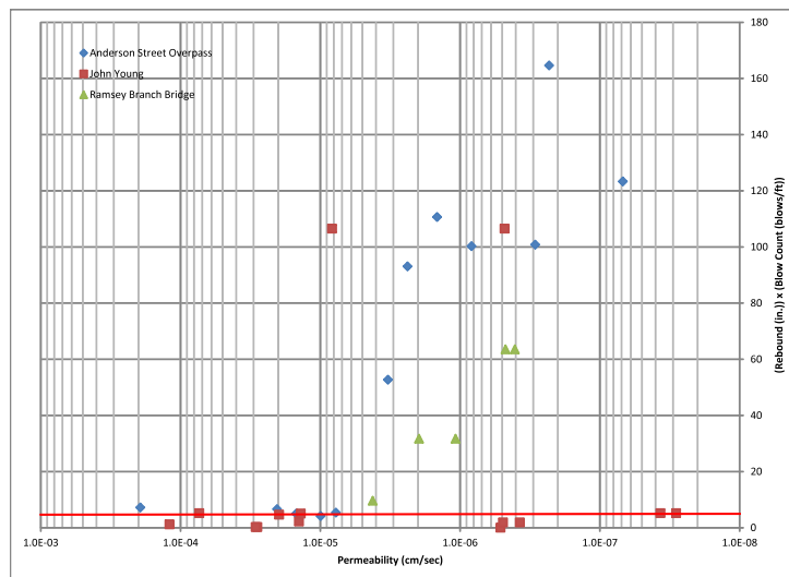
Figure 4.43 CU Triaxial Permeability versus Rebound times the Pile Driving Hammer Blow Count
