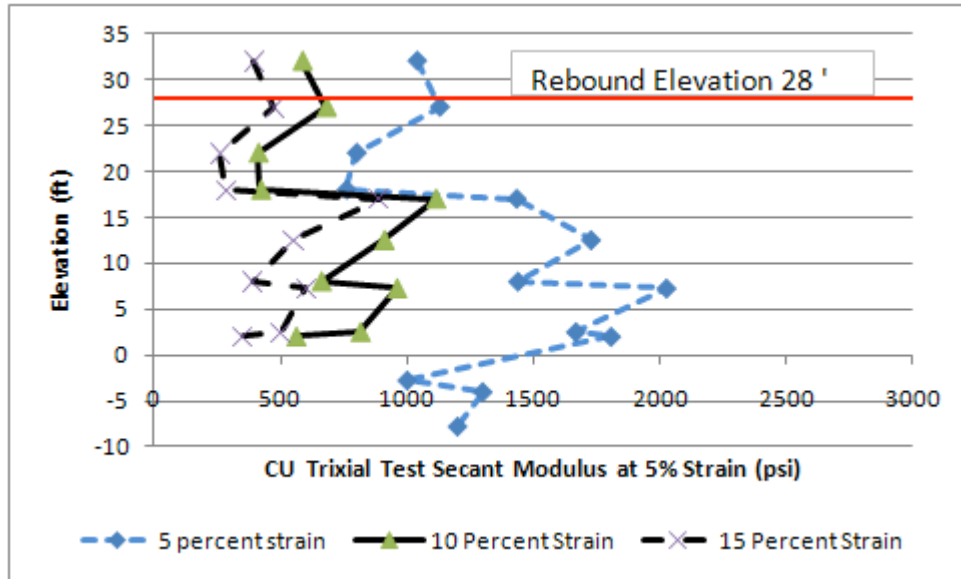
Figure 4.39 Anderson Street Overpass CU Triaxial 5, 10 and 15 percent Secant Modulus versus Elevation
