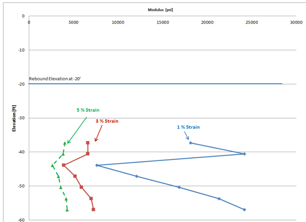
Figure 4.35 Ramsey Branch Bridge PPMT Elastic Modulus versus Elevation
