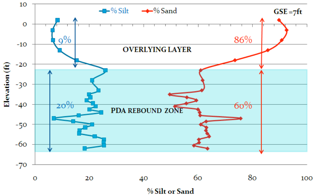
Figure 4.7 Ramsey Branch Bridge Elevation versus Sand Content and Silt Content
