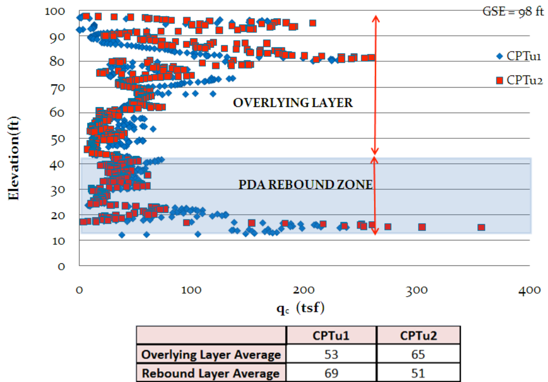
Figure 4.25 Retesting Phase John Young CPT q_c versus Elevation with Tabular Averages
