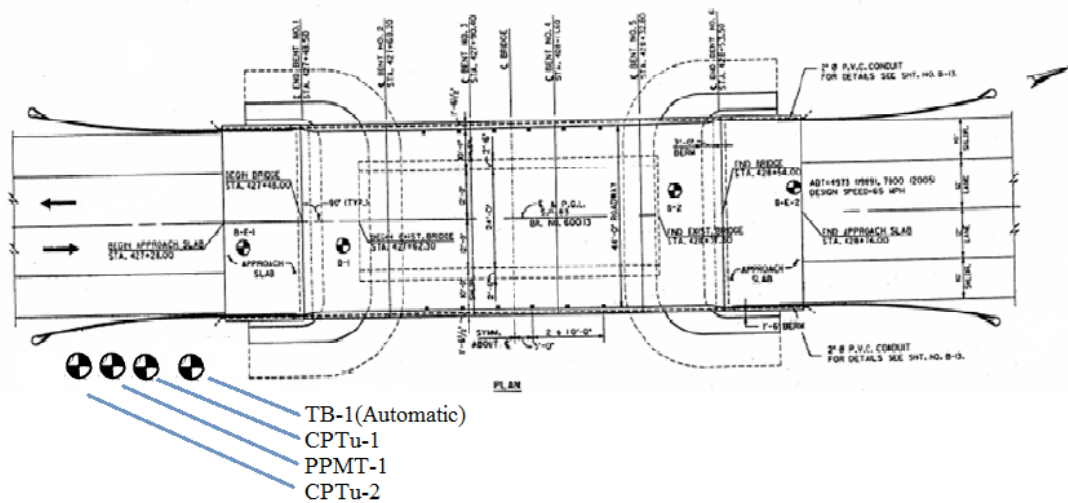
Figure 2.17 Field Retesting Boring Locations for Ramsey Branch Bridge near End Bent 1
