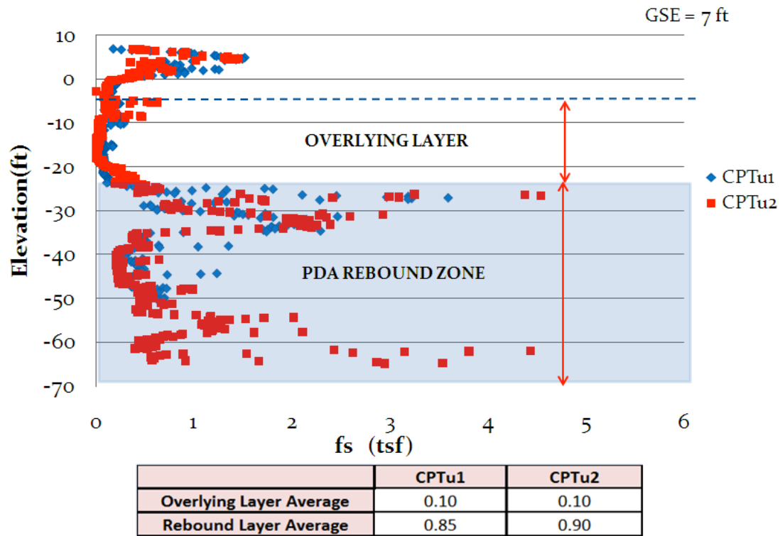
Figure 4.29 Retesting Phase Ramsey Branch Bridge CPT Friction versus Elevation with Tabular Averages
