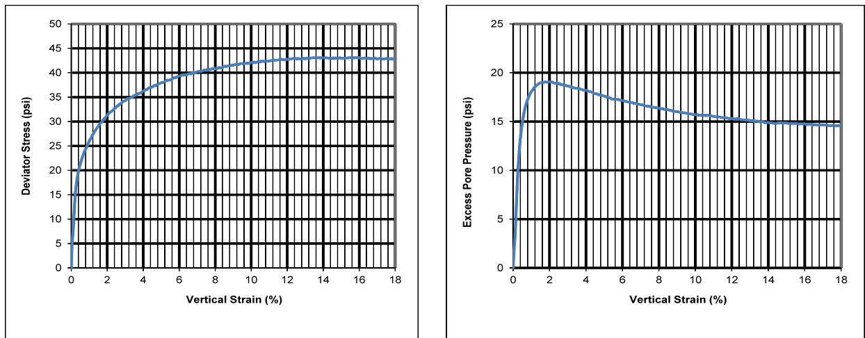
Figure 4.38 Typical CU Triaxial Results with Deviator Stress and Excess Pore Pressure versus Strain
