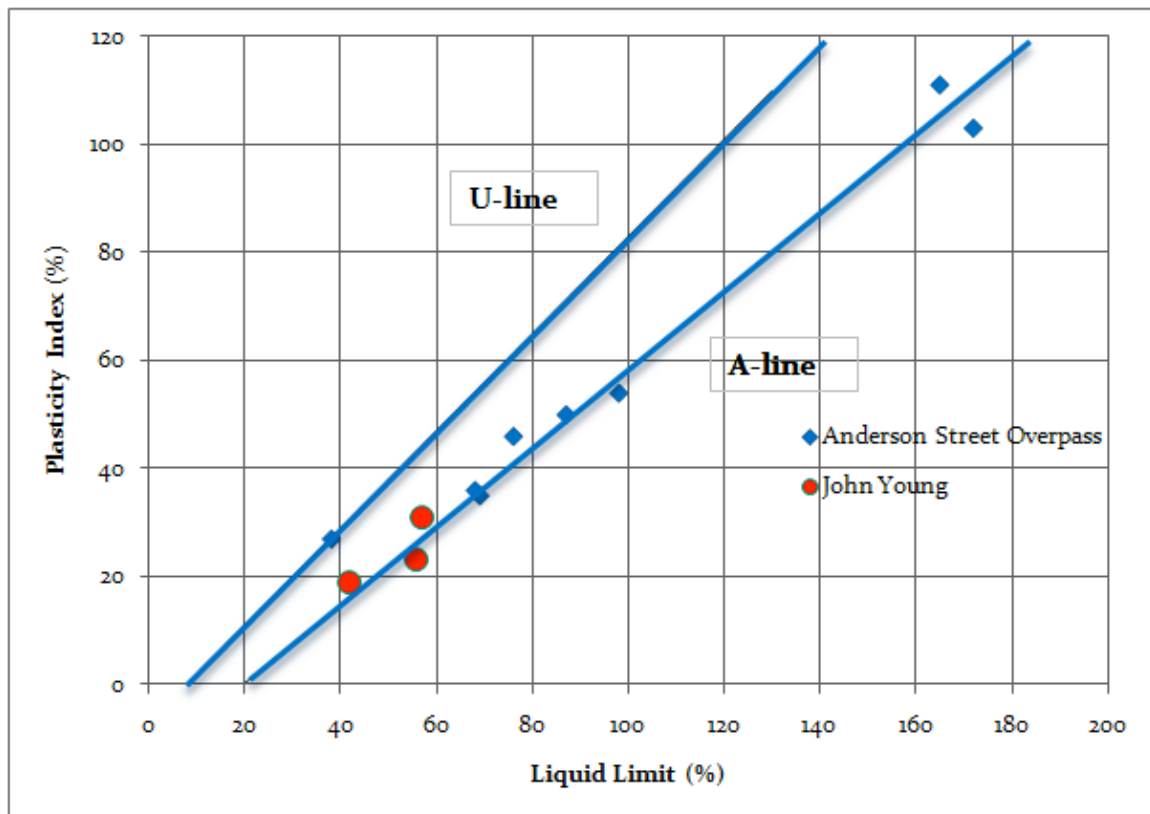
Figure 4.9 Design Phase Plasticity Chart for Anderson Street Overpass and John Young Data from Rebound Zones
