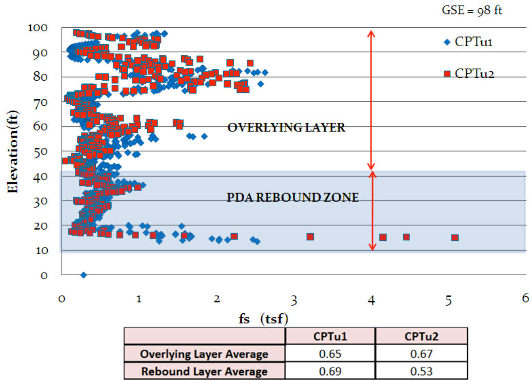
Figure 4.28 Retesting Phase John Young CPT Friction versus Elevation with Tabular Averages
