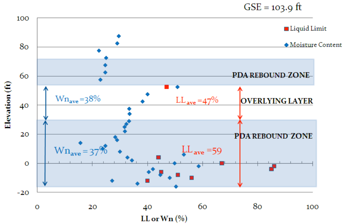
Figure 4.12 Research Phase Anderson Street Overpass Elevation versus Liquid Limit and Moisture Content
