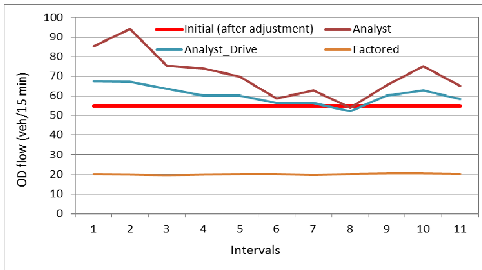
Figure 6-1 Temporal profile of initial, Analyst, and Analyst Drive OD
