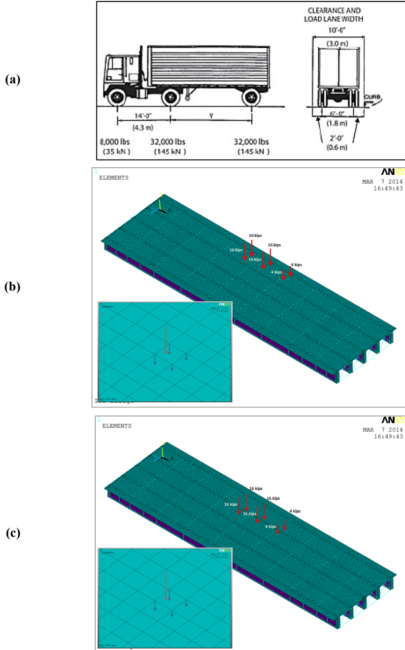
Figure 3-2. Truck portion of the HL-93 Design Load (a); Placing single truck load in two different transverse locations (b) and (c)
