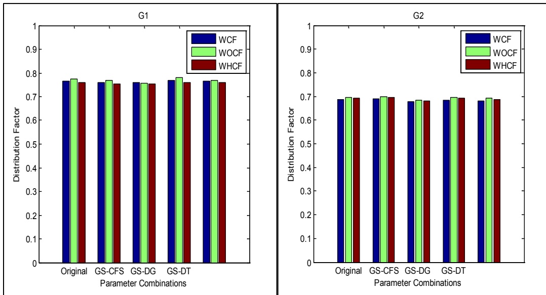
Figure A-33. Distribution factor for girders G1 and G2 related to different Parameter combinations for bridge I-95 over SR-421
