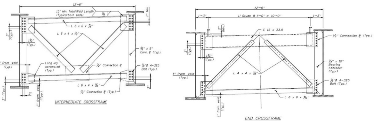
Figure 4-3. Cross-frame details of the I-95 Bridge over SR-421
