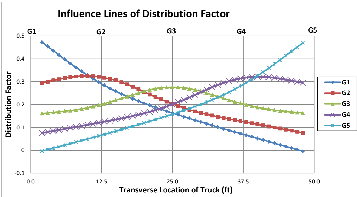
Figure 3-3. Influence lines of distribution factors for all girders, I-95 Bridge over SR-421
