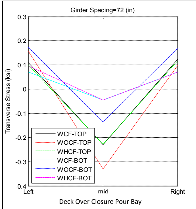
Figure 4-13. Deck stresses in 6 points including top and bottom of deck in two side and middle point for a single parameter Girder Spacing =72 in
