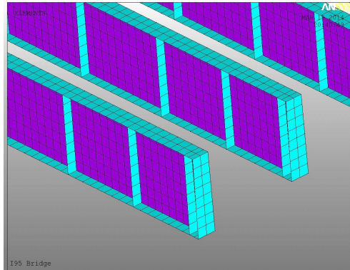
Stiffeners added
