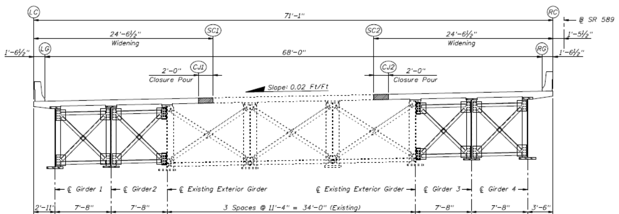
Figure 4-5. Cross-section of the bridge SR-589 over Waters Avenue
