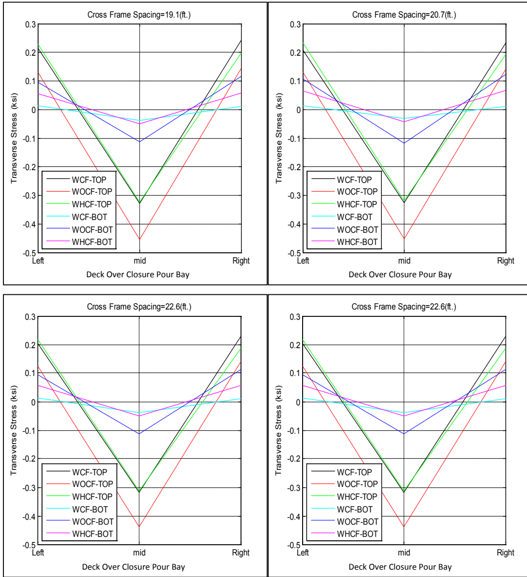
Figure A-55. Transverse stress at closure pour related to different cross-frame spacing for SR-589 over Waters Avenue
