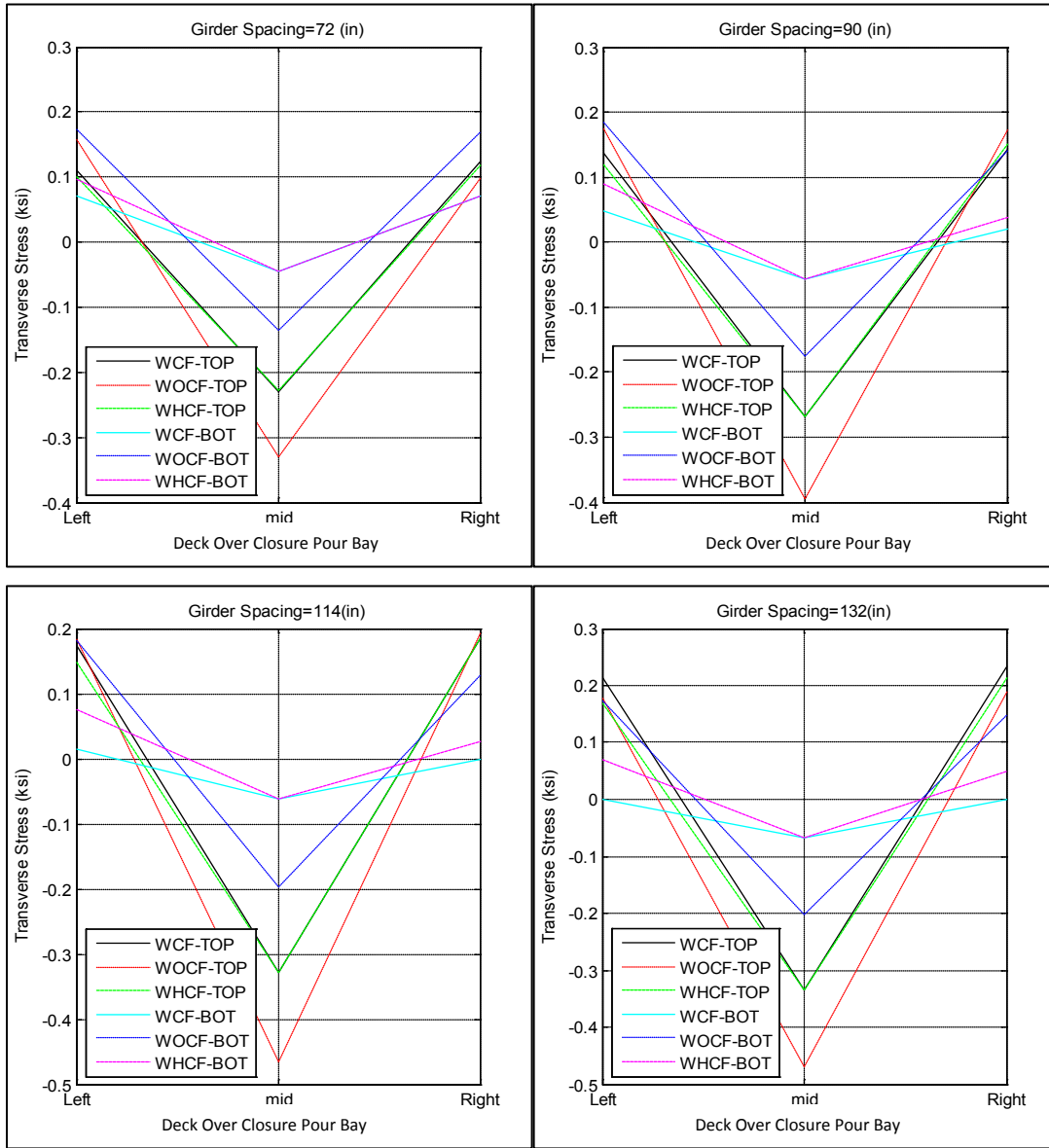
Figure A-3. Transverse stress at closure pour related to different girder spacing; 72, 90, 114, 132 inches for bridge I-95 over SR-421
