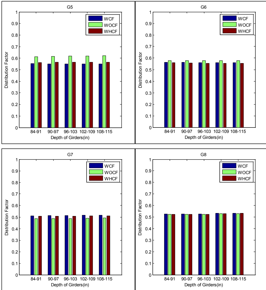
Figure A-49. Distribution factor for girders G5, G6, G7 and G8 related to different depth of girders for bridge SR-589 over Waters Avenue
