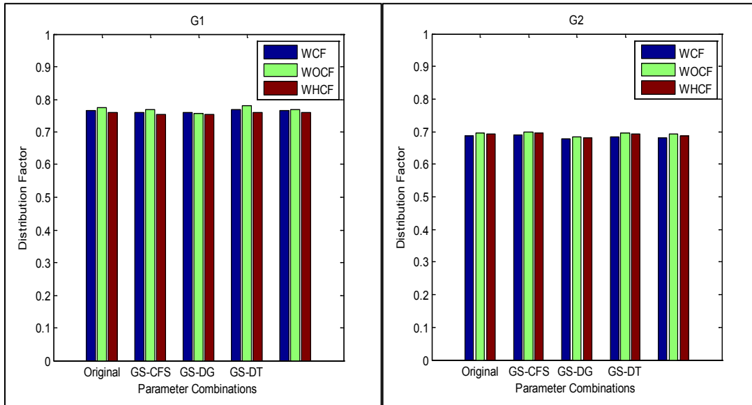
Figure A-65. Distribution factor for girders G1 and G2 related to different parameter combinations for bridge SR-589 over Waters Avenue
