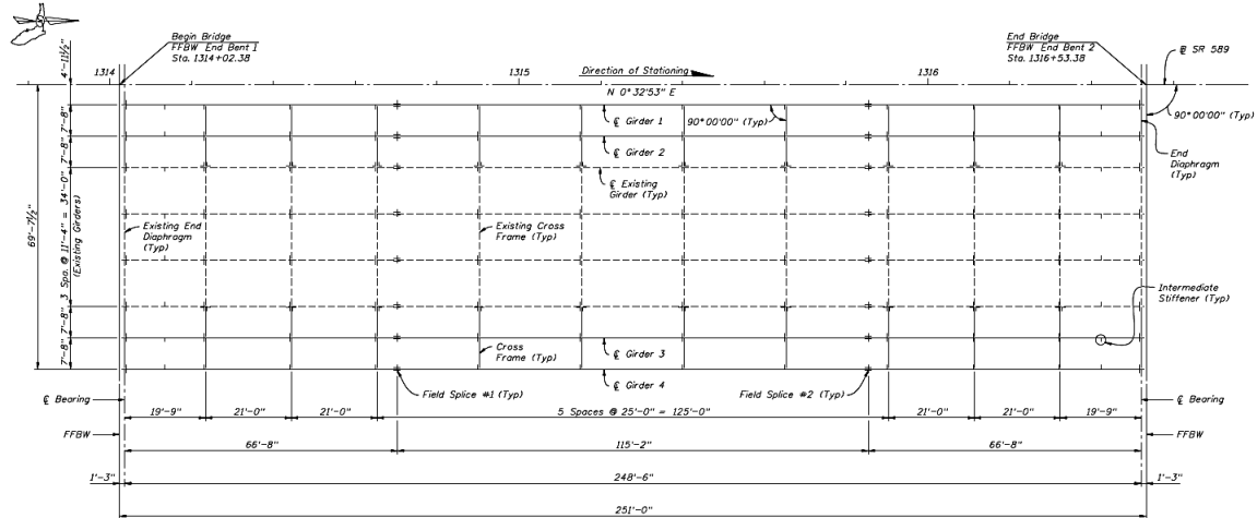
Figure 4-6. Framing plan of the bridge SR-589 over Waters Avenue
