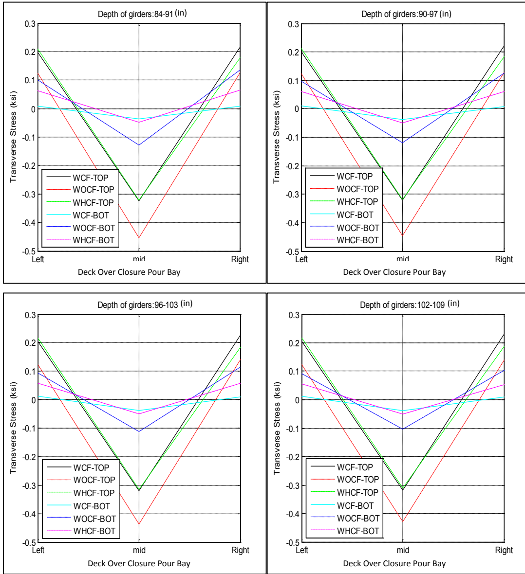
Figure A-50. Transverse stress at closure pour related to different depth of girders for SR-589 over Waters Avenue
