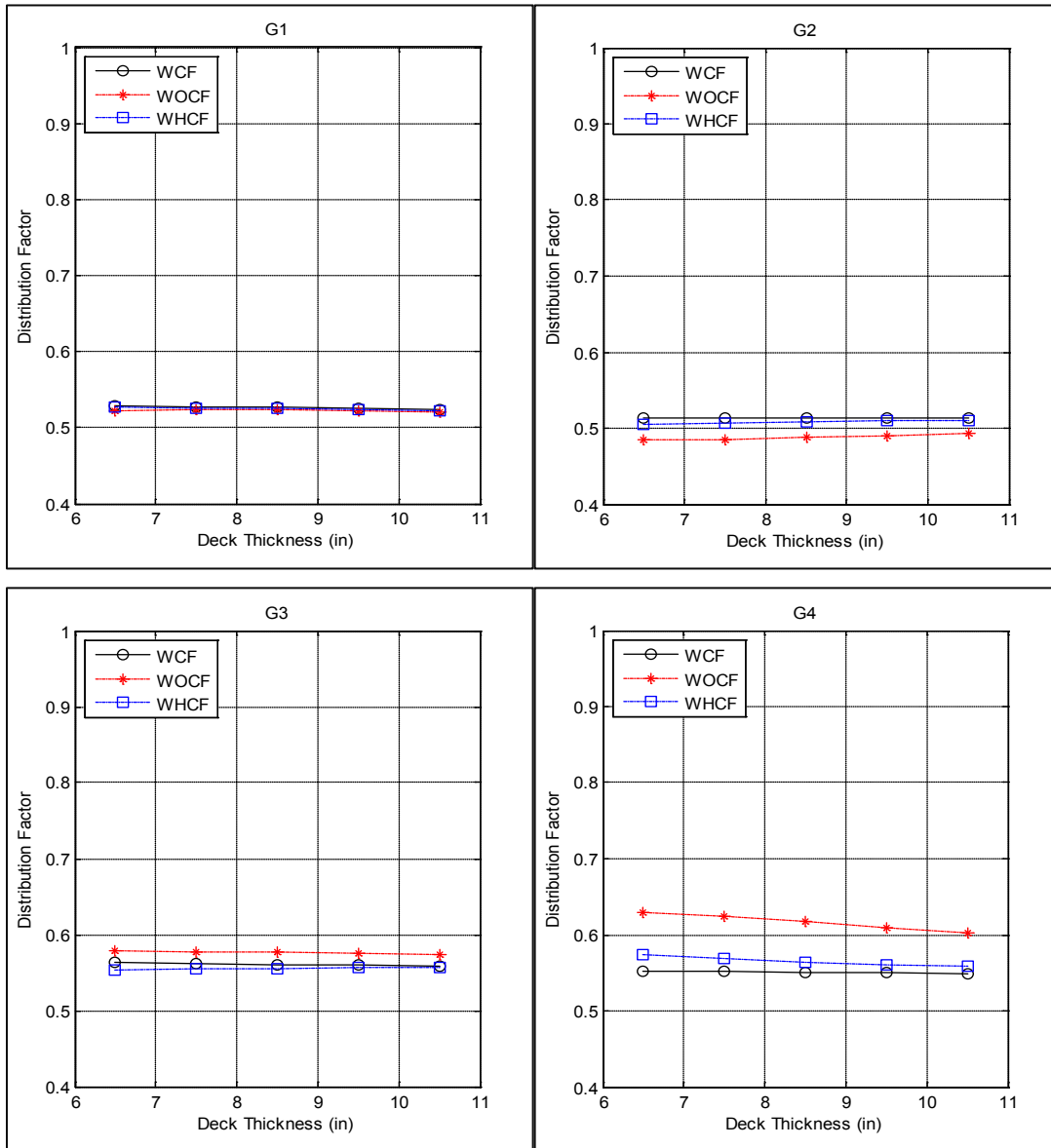
Figure A-43. Distribution factor for girders G1, G2, G3 and G4 related to different deck thicknesses for bridge SR-589 over Waters Avenue
