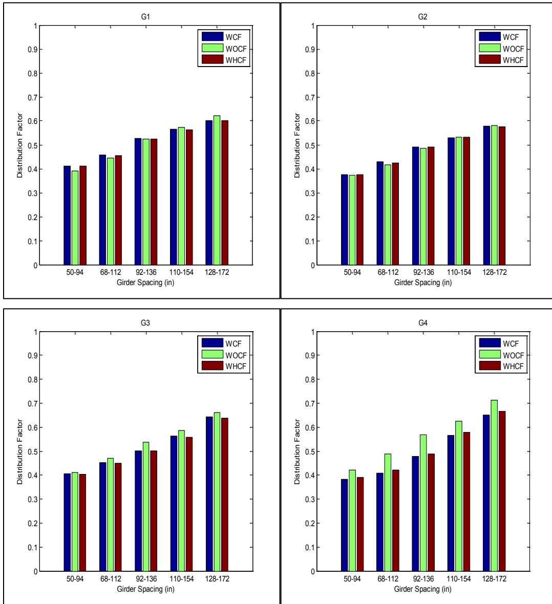
Figure A-38. Distribution factor for girders G1, G2, G3 and G4 related to different girder spacing for bridge SR-589 over Waters Avenue
