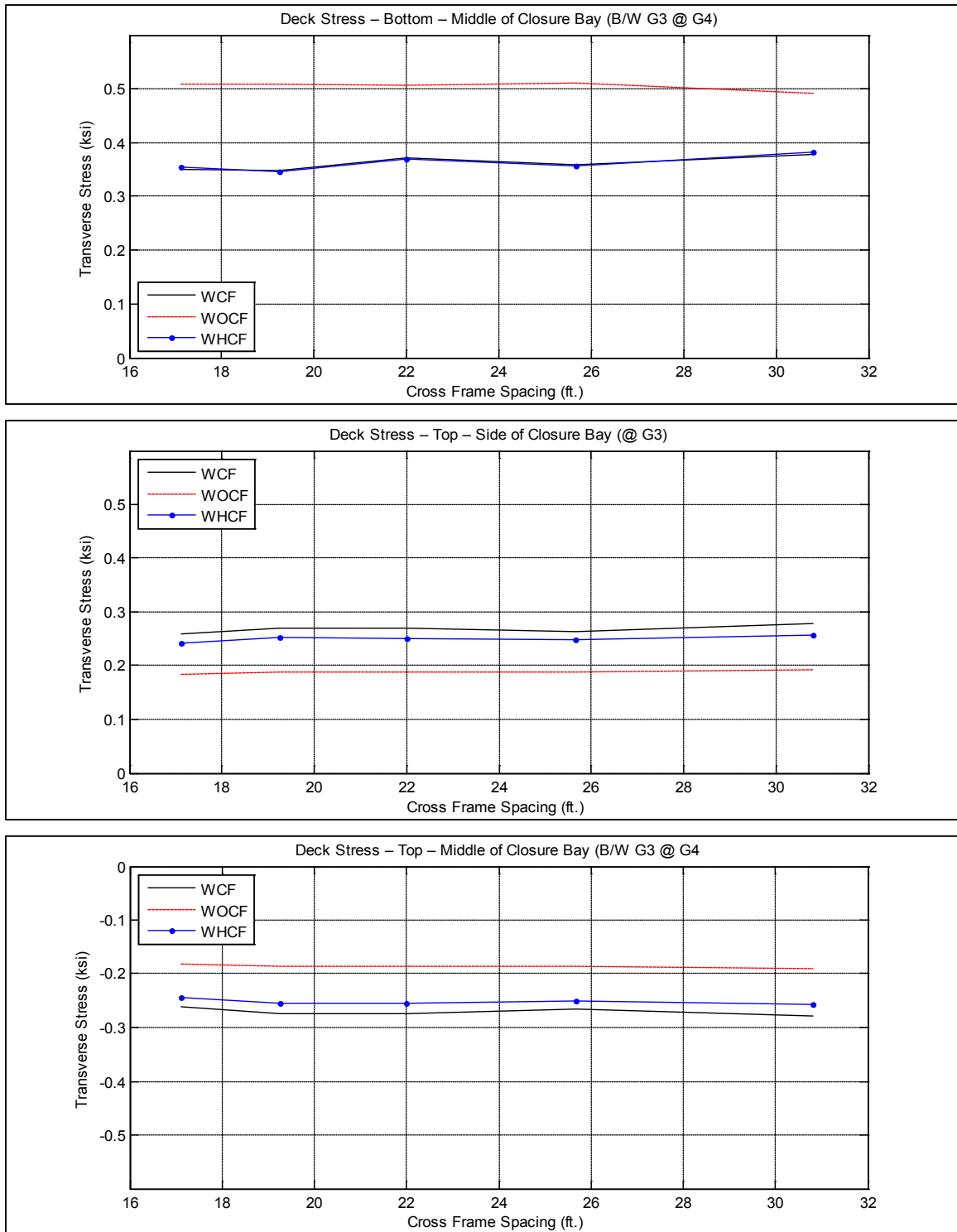
Figure A-23. Transverse deck stresses at middle and side of closure pour vs. cross-frame spacing for bridge I-95 over SR-421
