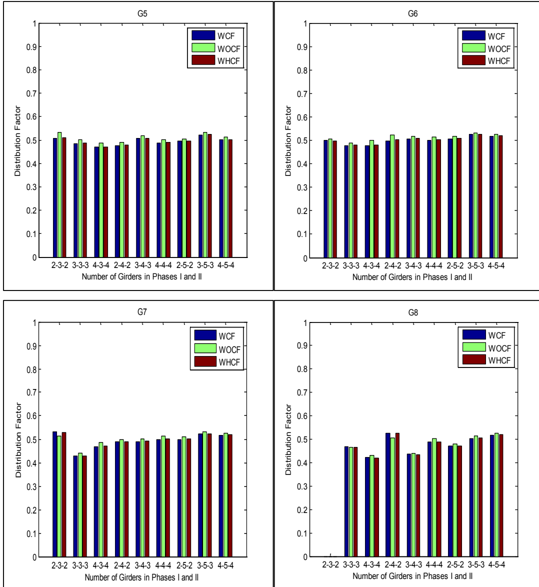
Figure A-59. Distribution factor for girders G5, G6, G7 and G8 related to different configuration of phases for bridge SR-589 over Waters Avenue
