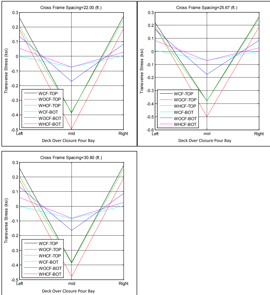
Figure A-22. Transverse stress at closure pour related to different cross frame spacing; 22.0, 25.67 and 30.8 ft. for bridge I-95 over SR-421
