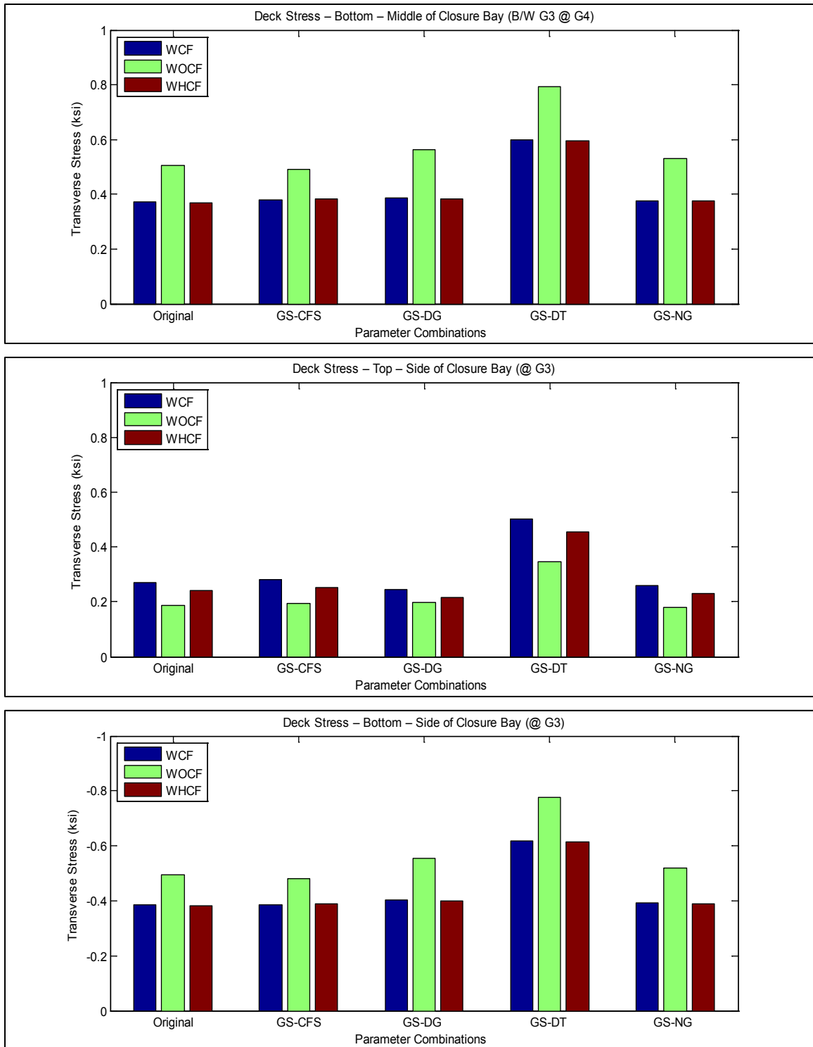
Figure A-36. Transverse deck stresses at middle and side of closure pour vs. parameter combinations for bridge I-95 over SR-421
