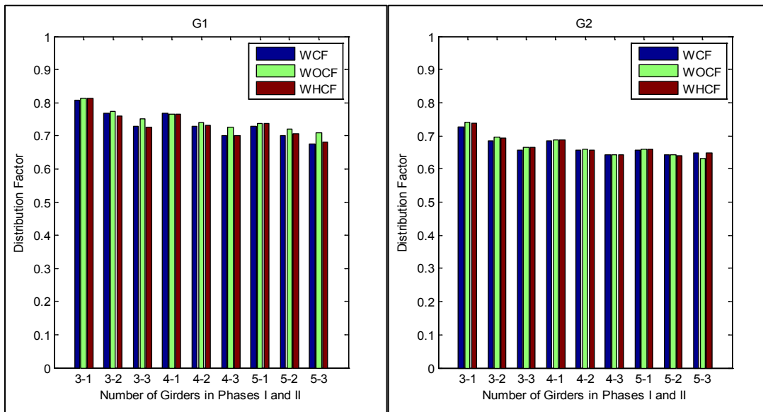
Figure A-25. Distribution factor for girders G1 and G2 related to different phase I and II configurations for bridge I-95 over SR-421
