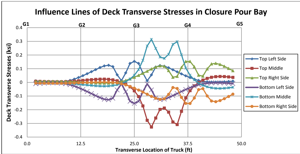
Figure 3-6. Influence lines – Transverse deck stress
