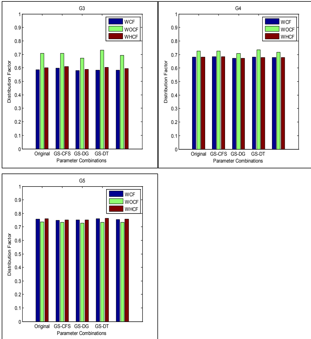
Figure A-66. Distribution factor for girders G3, G4 and G5 related to different parameter combinations for bridge SR-589 over Waters Avenue
