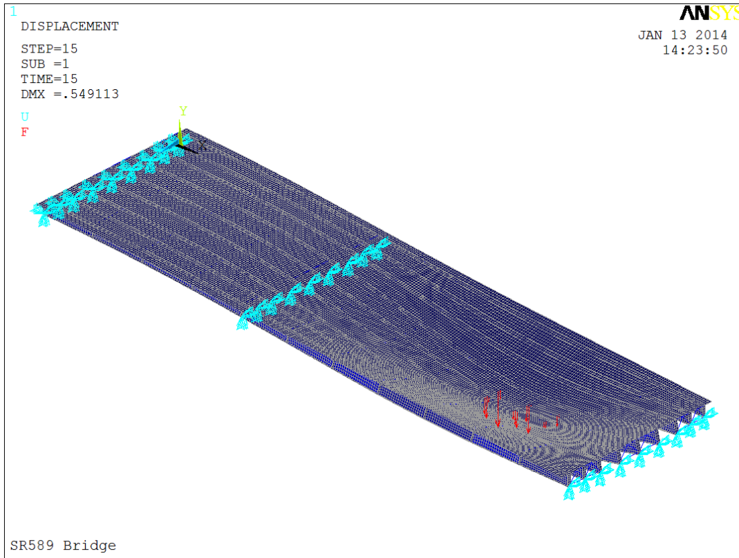
Figure 6-6. SR-589 Bridge over Hillsborough Avenue under truck loading located at critical longitudinal location.
