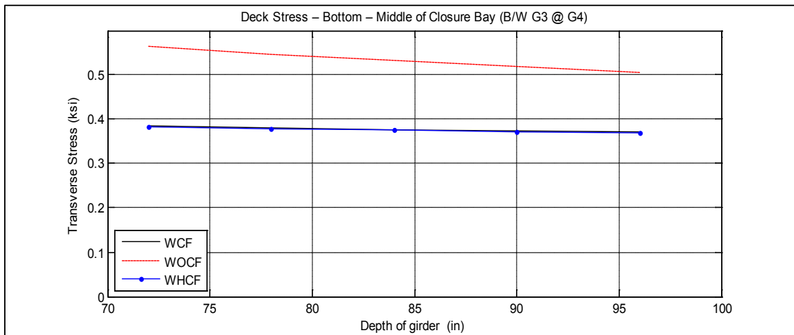
Figure A-17. Transverse deck stresses at Bottom -middle of closure pour vs. depth of girders for bridge I-95 over SR-421
