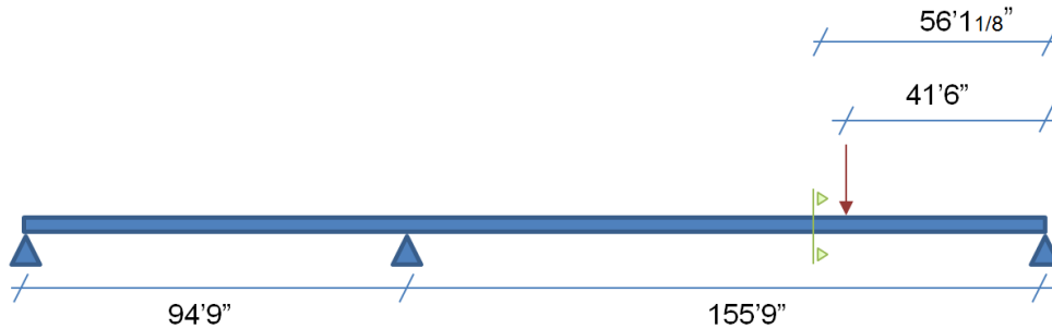
Figure 6-5. Critical longitudinal loading location and corresponding maximum response cross-section for the SR-589 Bridge over Hillsborough Avenue
