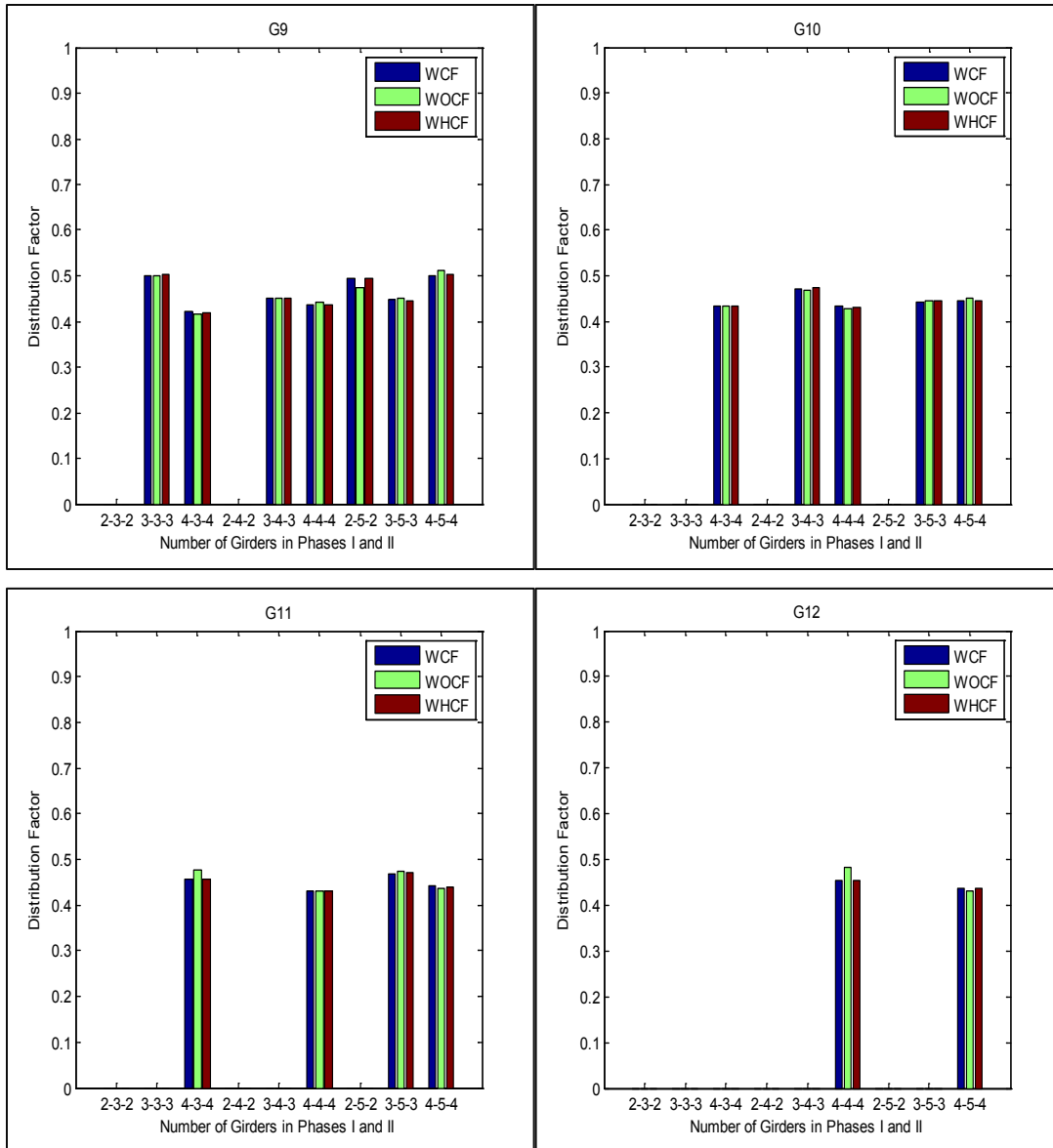
Figure A-60. Distribution factor for girders G9, G10, G11 and G12 related to different configuration of phases for bridge SR-589 over Waters Avenue
