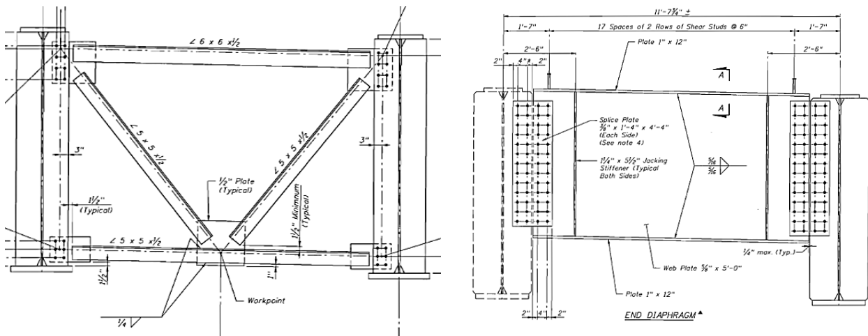
Figure 6-9. Cross-frame details of the SR-589 Bridge over Hillsborough Avenue
