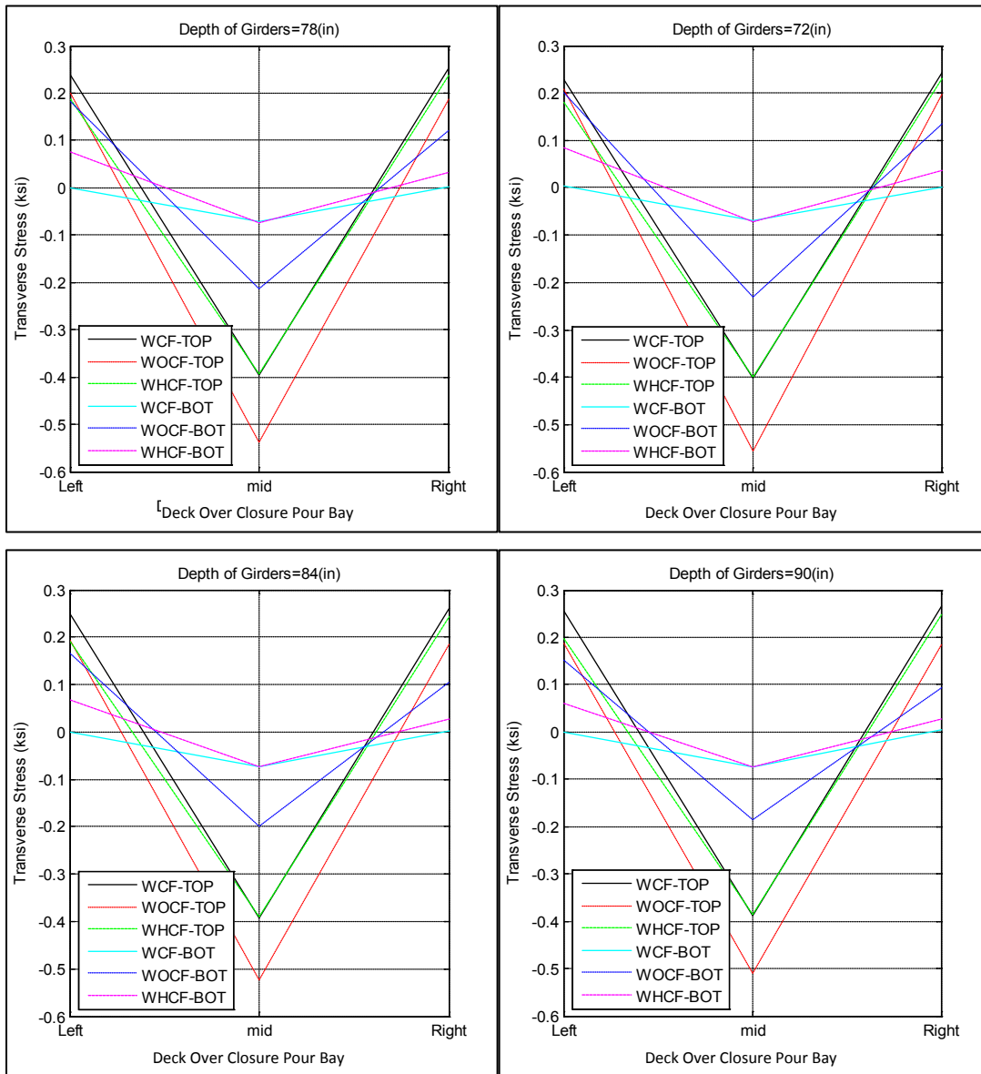
Figure A-15. Transverse stress at closure pour related to different depth of girders; 72, 78, 84 and 90 inches for bridge I-95 over SR-421
