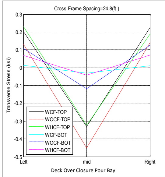
Figure A-55. Transverse stress at closure pour related to different cross-frame spacing for SR-589 over Waters Avenue – Cont'd
