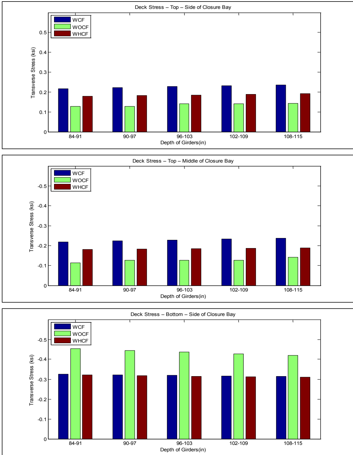
Figure A-52. Transverse deck stresses at middle and side of closure pour vs. depth of girders for bridge SR-589 over Waters Avenue
