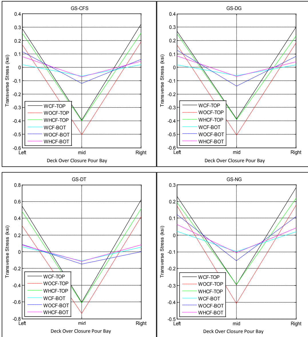
Figure A-67. Transverse stress at closure pour related to different parameter combinations for SR-589 over Waters Avenue
