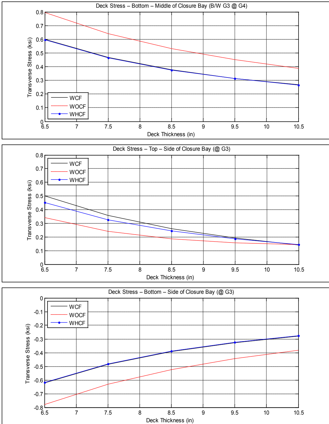
Figure A-11. Transverse deck stresses at middle and side of closure pour vs. deck thickness for bridge I-95 over SR-421
