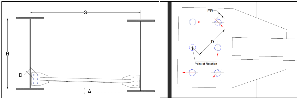
Figure 5-4. Proposed connection detail to accommodate relative vertical displacement
