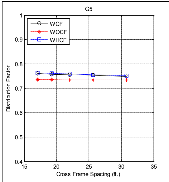
Figure A-20. Distribution factor for girder G5 related to different cross frame spacing for bridge I-95 over SR-421
