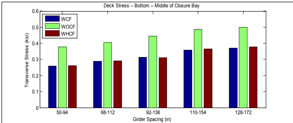
Figure A-41. Transverse deck stresses at Bottom -middle of closure pour vs. girder spacing for bridge SR-589 over Waters Avenue
