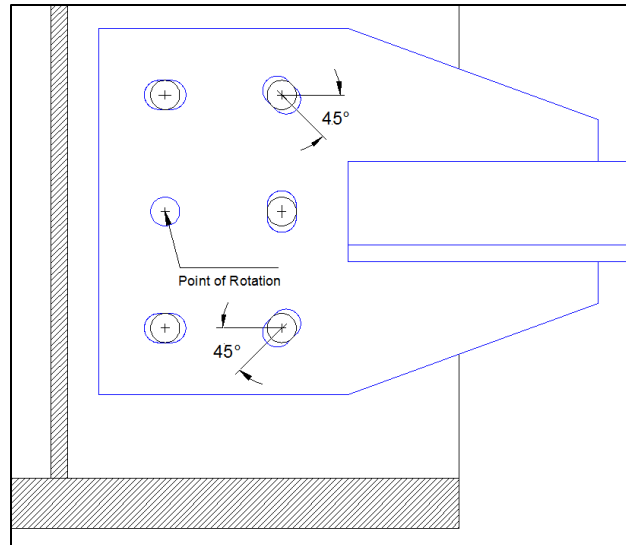
Figure 5-5. Radial slotted hole connection to accommodate large movement
