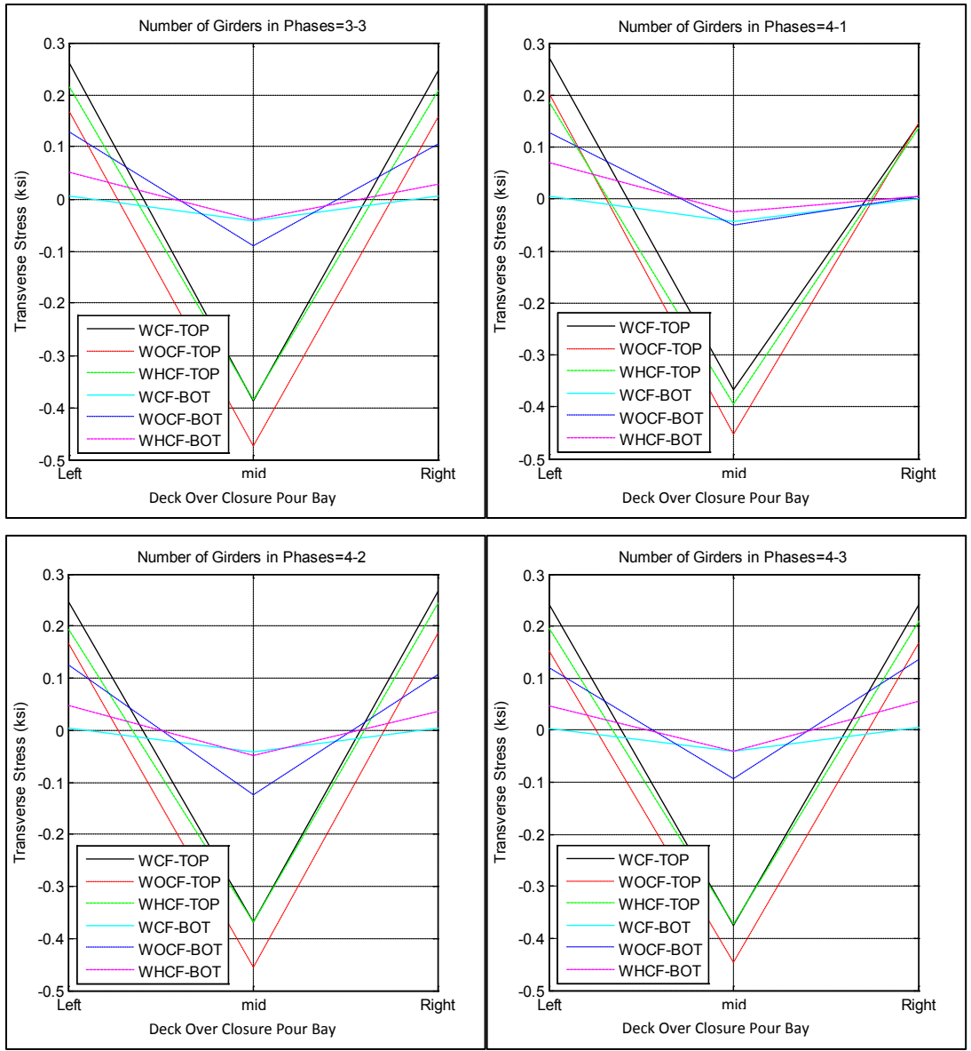
Figure A-29. Transverse stress at closure pour related to different number of girders in phase I and II; 3-3, 4-1, 4-2 and 4-3 for bridge I-95 over SR-421
