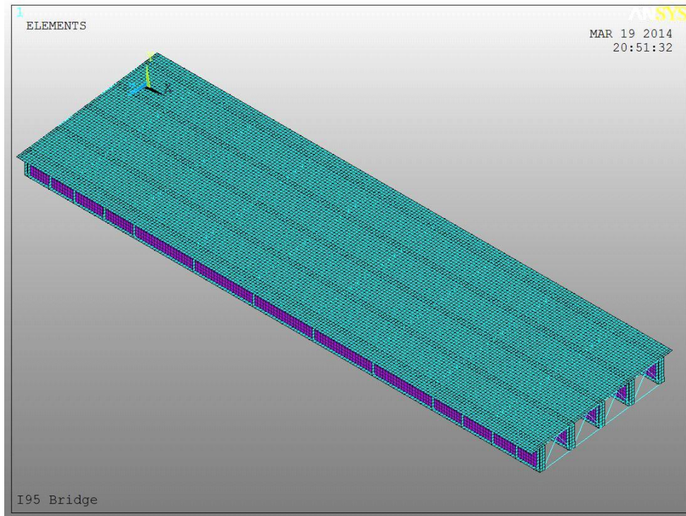
Full Structure
