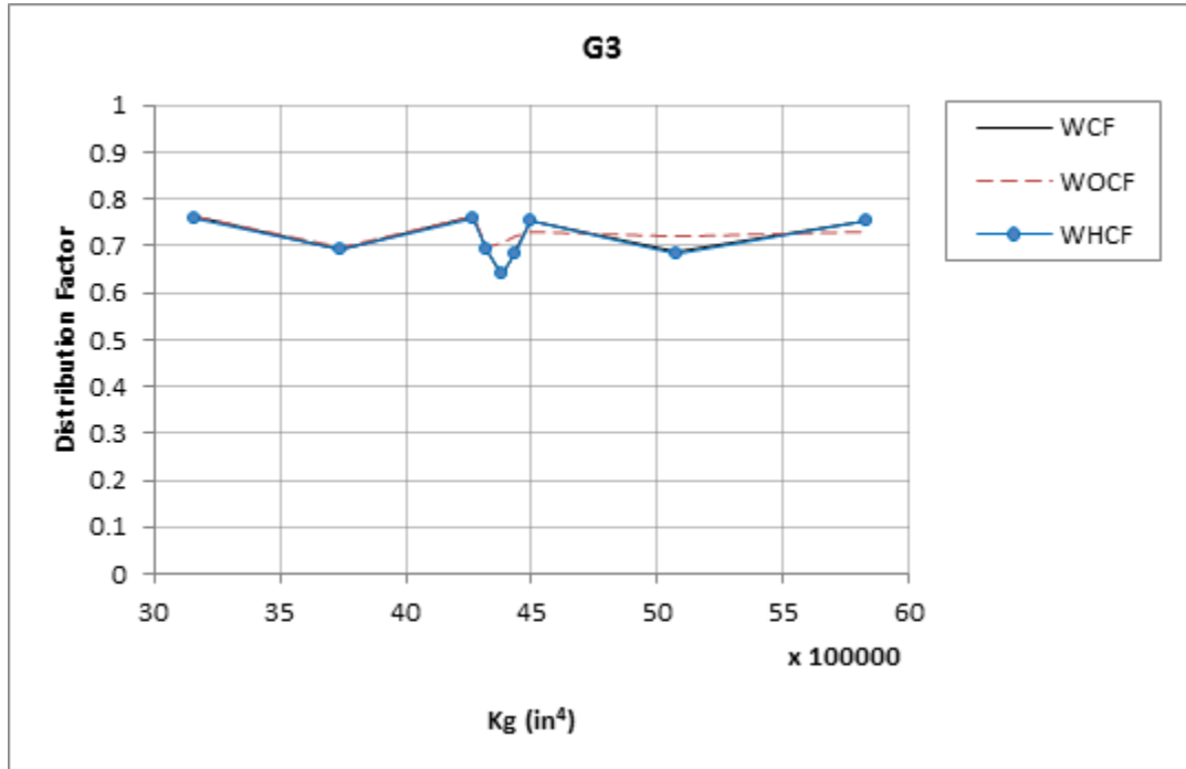
Figure 4-16. Distribution Factor vs. K_g for G3bridge I-95 over SR-421
