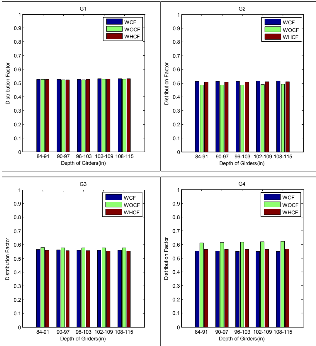
Figure A-48. Distribution factor for girders G1, G2, G3 and G4 related to different depth of girders for bridge SR-589 over Waters Avenue
