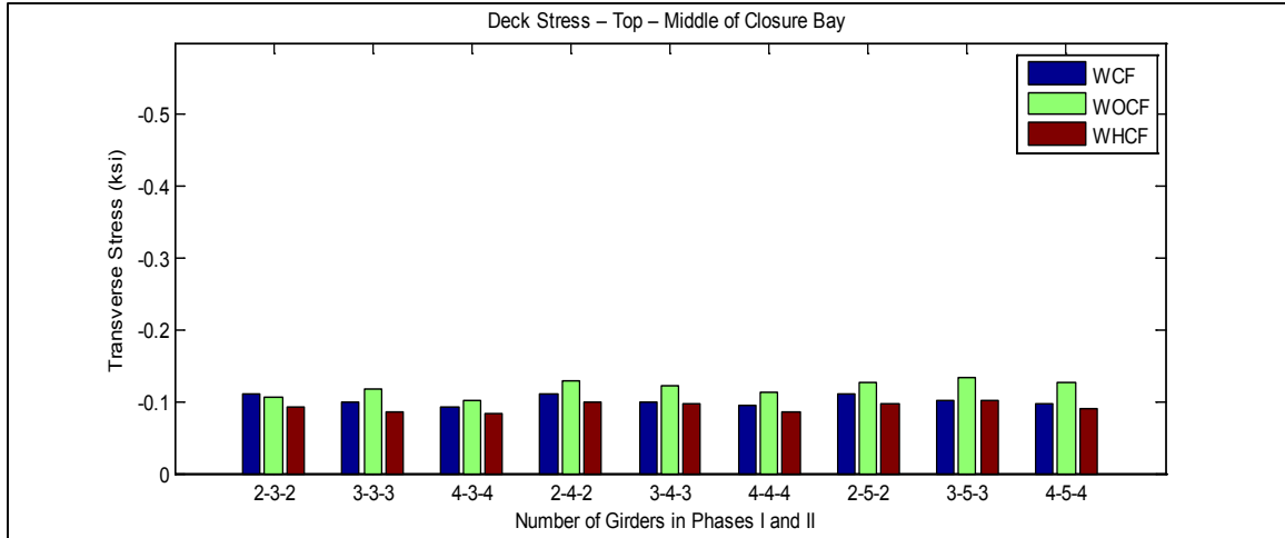
Figure A-64. Transverse deck stresses at top -middle of closure pour vs. number of girders in phases for bridge SR-589 over Waters Avenue
