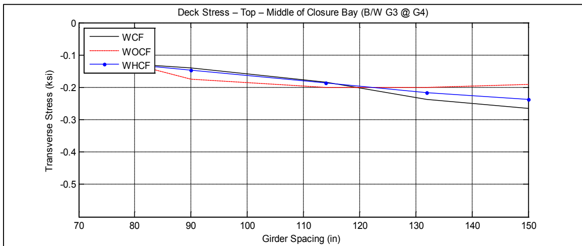
Figure A-6. Transverse deck stresses at middle and side of closure pour vs. girder spacing for bridge I-95 over SR-421
