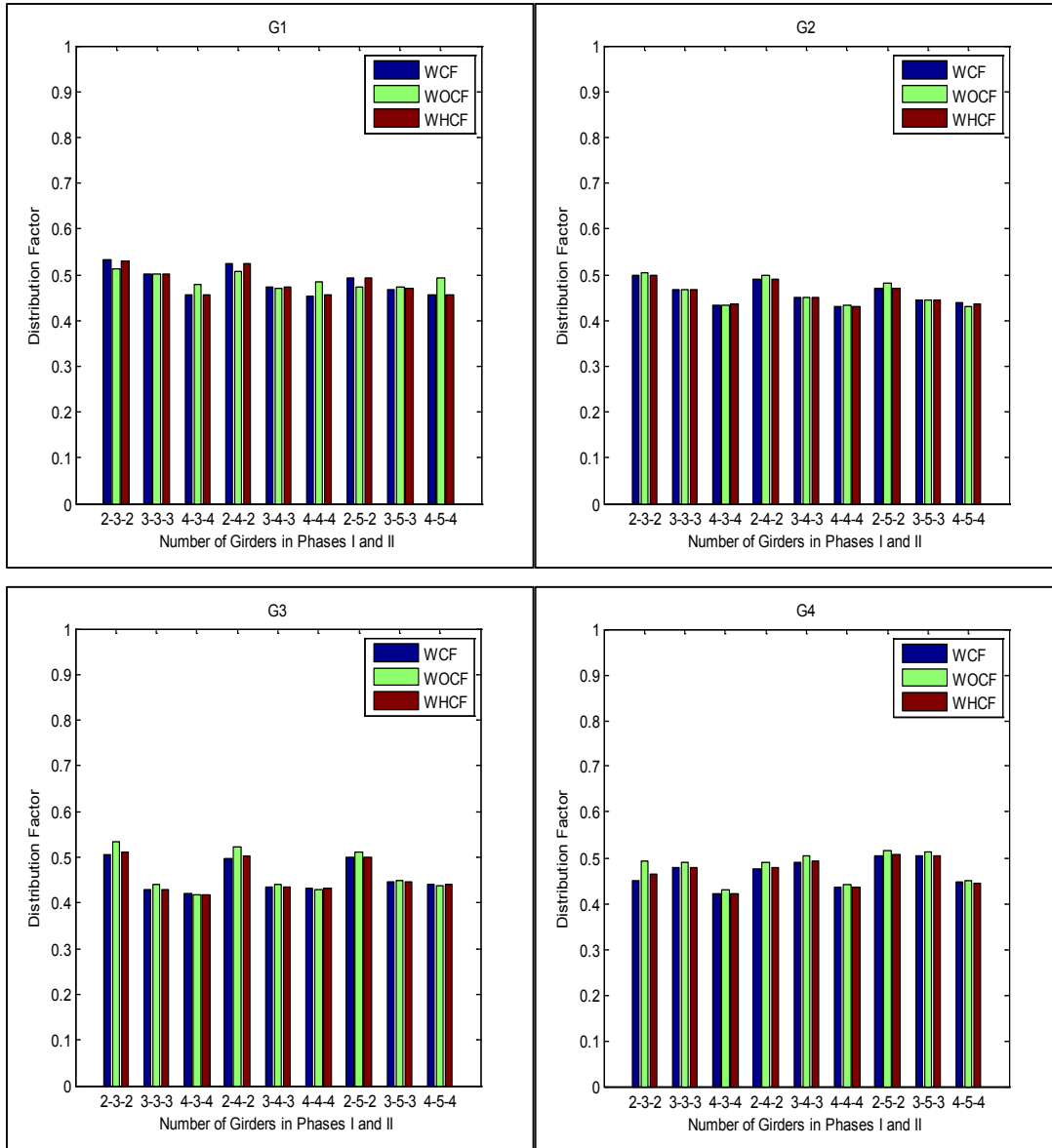
Figure A-58. Distribution factor for girders G1, G2, G3 and G4 related to different configuration of phases for bridge SR-589 over Waters Avenue
