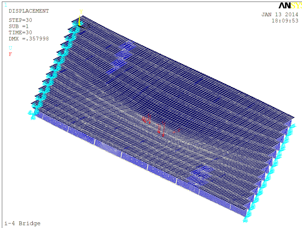
Figure 6-11. Deformed shape of bridge I-4 over SR46 under truck loading located at mid-width and mid-span
