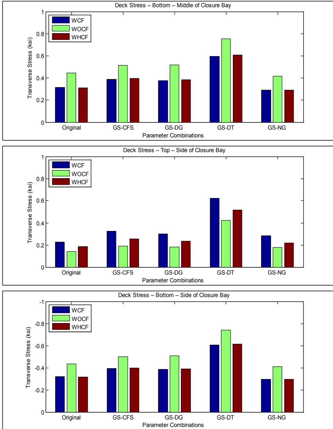
Figure A-68. Transverse deck stresses at middle and side of closure pour vs. parameter combinations for bridge SR-589 over Waters Avenue
