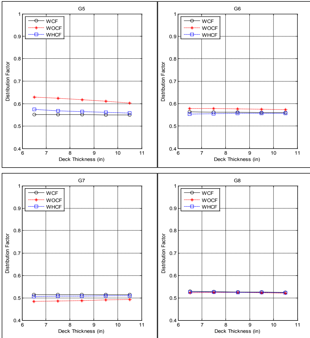
Figure A-44. Distribution factor for girders G5, G6, G7 and G8 related to different deck thicknesses for bridge SR-589 over Waters Avenue
