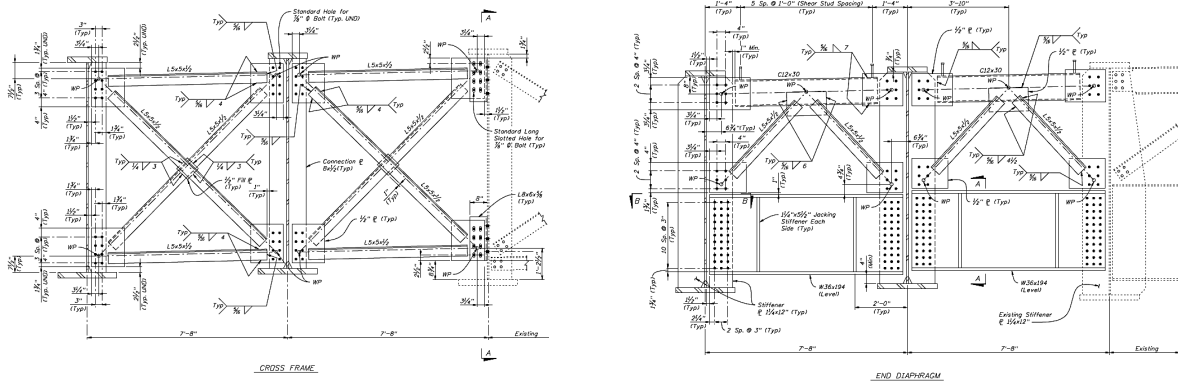
Figure 4-7. Cross-frame details of the bridge SR-589 over Waters Avenue
