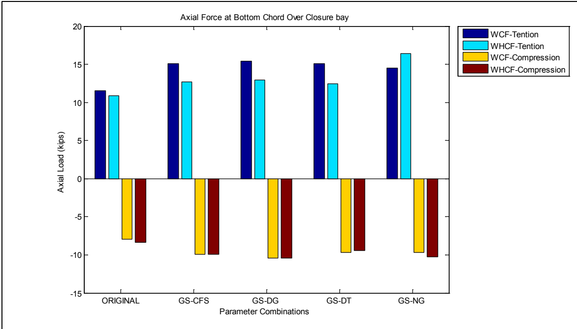
Figure 4-19. Axial force at bottom chord over closure bay in two original and alternative cross-frame cases for bridge SR-589 over Waters Avenue
