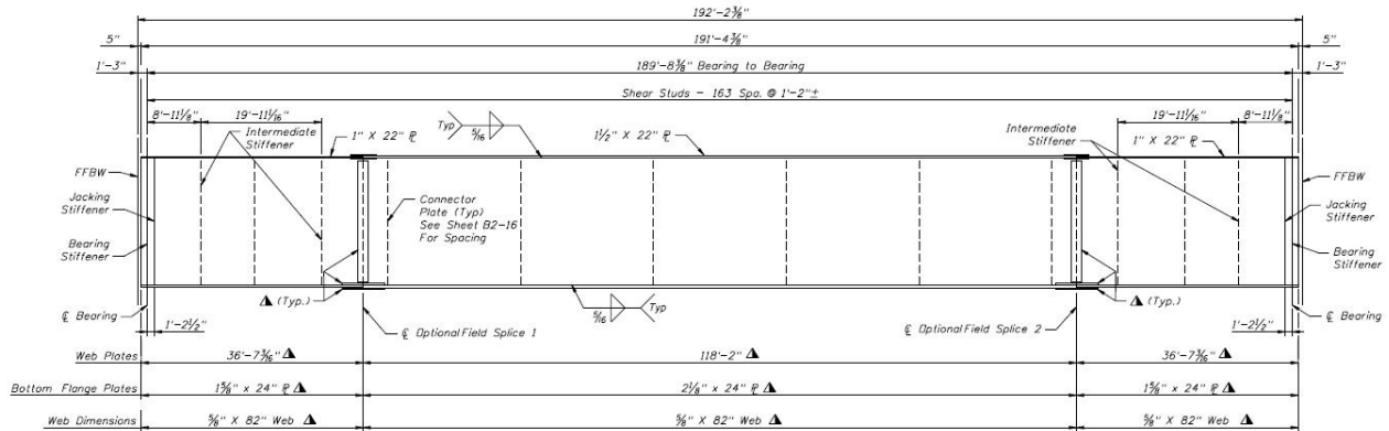
Figure 4-4. Typical details of girders of the I-95 Bridge over SR-421
