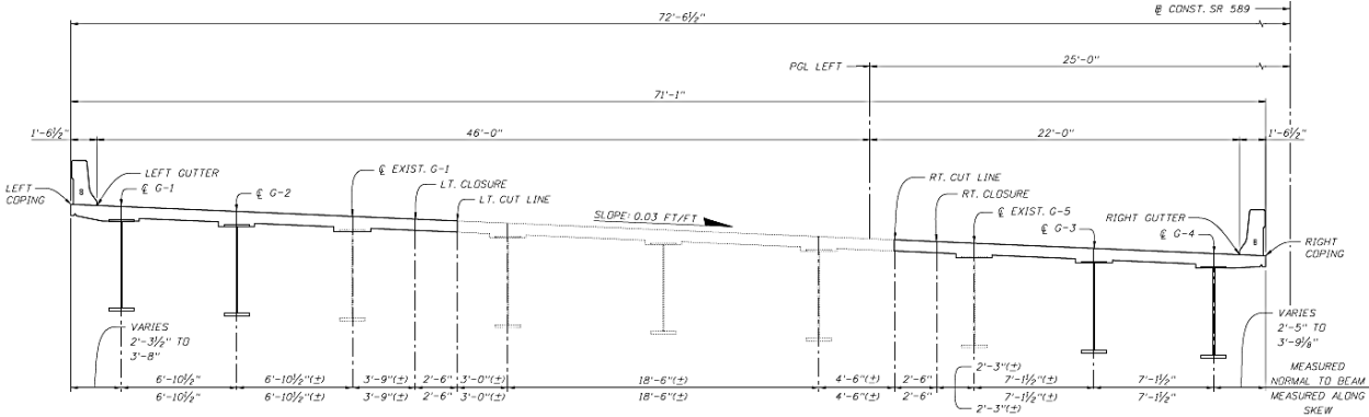
Figure 6-1. Cross-section of the SR-589 Bridge over Hillsborough Avenue
