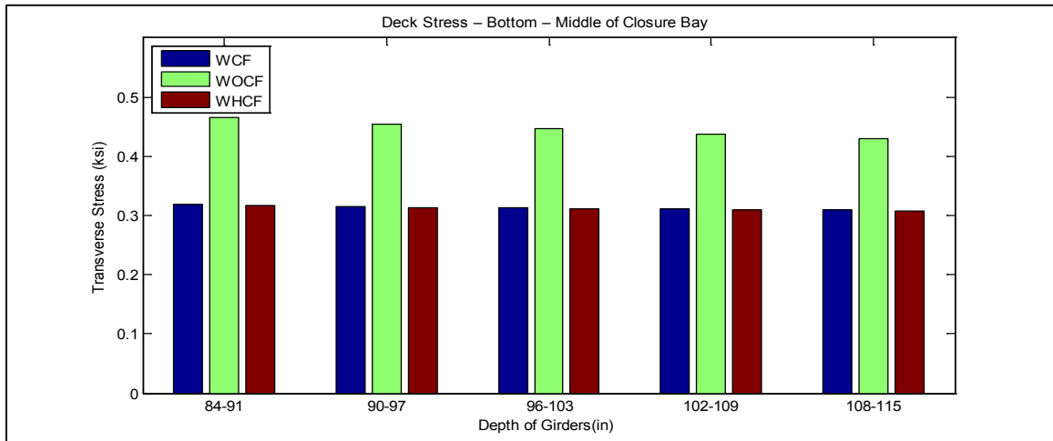
Figure A-51. Transverse deck stresses at Bottom -middle of closure pour vs. depth of girders for bridge SR-589 over Waters Avenue
