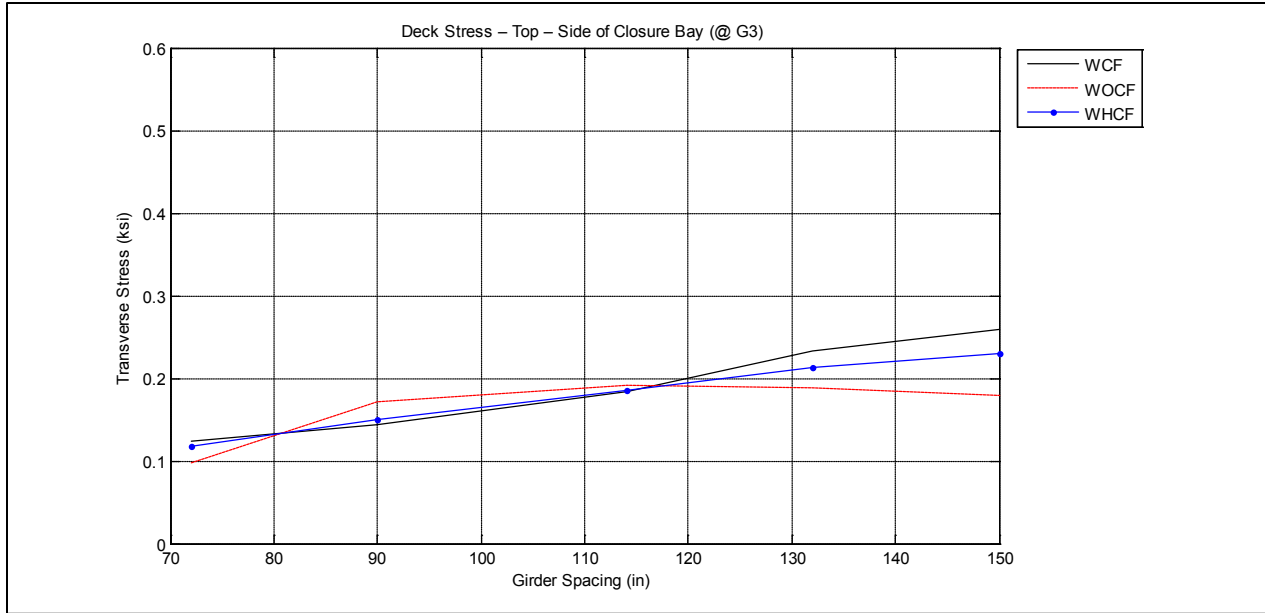
Figure 4-15. Transverse stress of the deck vs. girder spacing at top side
