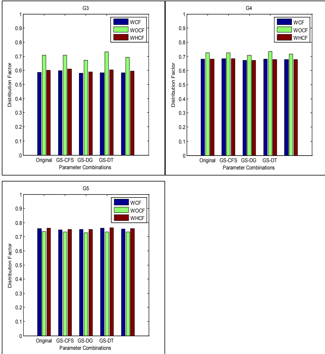
Figure A-34. Distribution factor for girders G3, G4 and G5 related to different Parameter combinations for bridge I-95 over SR-421
