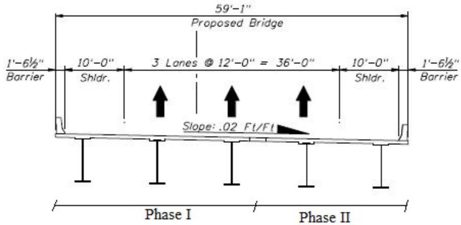
Figure 4-1. Cross-section of the bridge I-95 over SR-421
