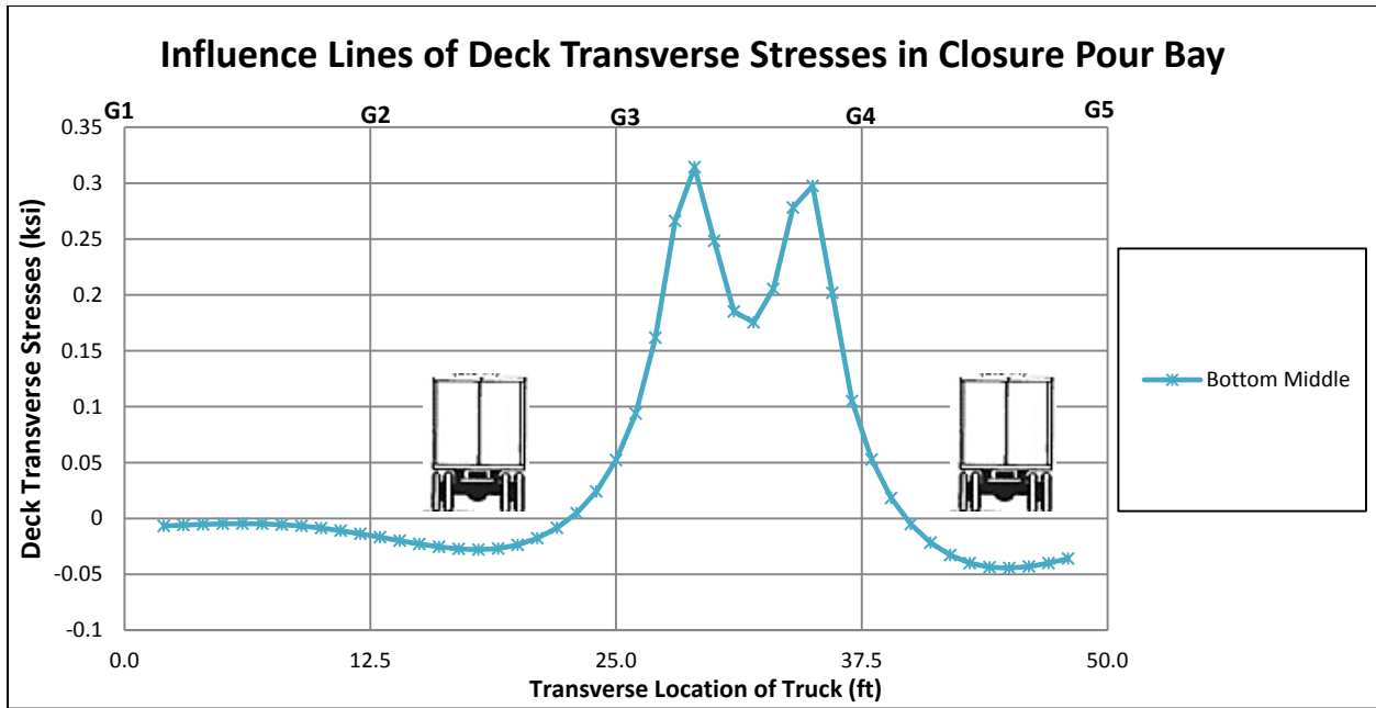
Figure 3-7. Bottom middle isolated and loaded for maximum compressive stress
