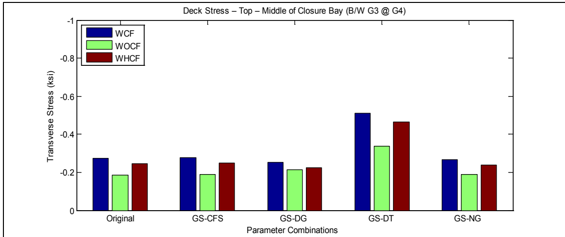
Figure A-37. Transverse deck stresses at top -middle of closure pour vs. parameter combinations for bridge I-95 over SR-421
