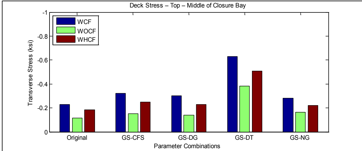
Figure A-69. Transverse deck stresses at top-middle of closure pour vs. parameter combinations for bridge SR-589 over Waters Avenue
