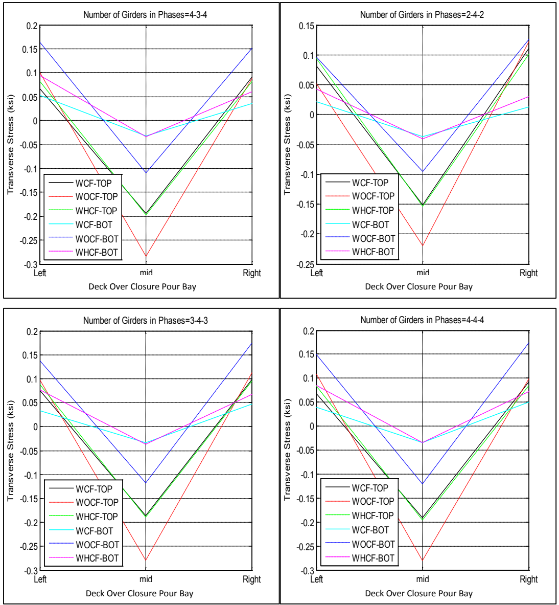
Figure A-62. Transverse stress at closure pour related to different number of girders in phases for SR-589 over Waters Avenue – Cont'd
