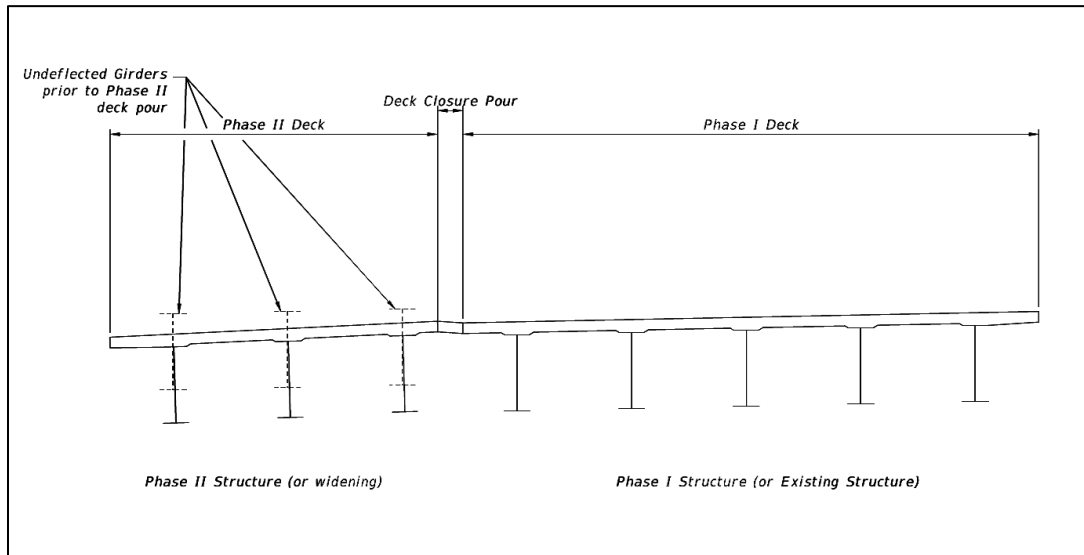
Figure 1-7. Twisting of one phase.
