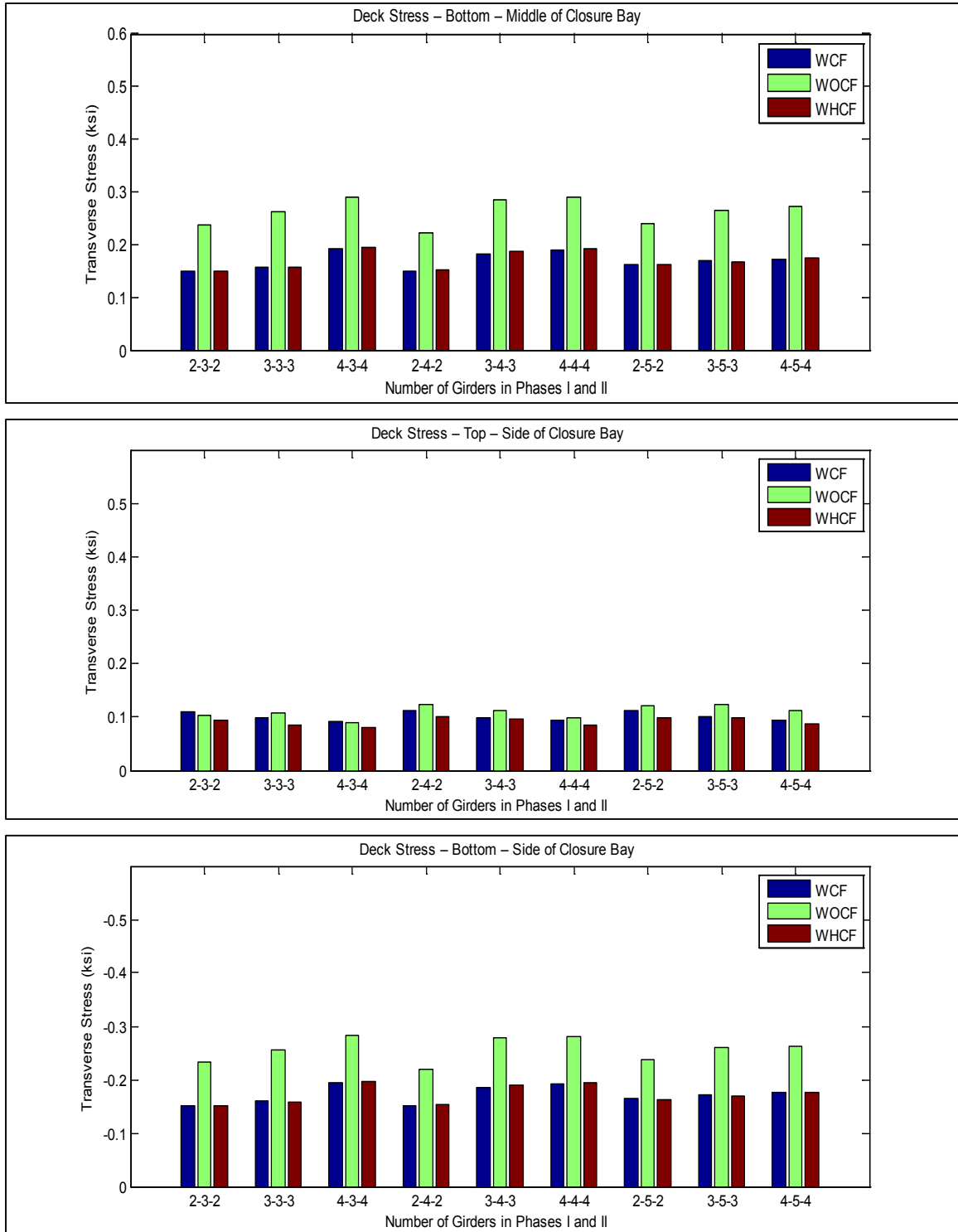
Figure A-63. Transverse deck stresses at middle and side of closure pour vs. number of girders in phases for bridge SR-589 over Waters Avenue
