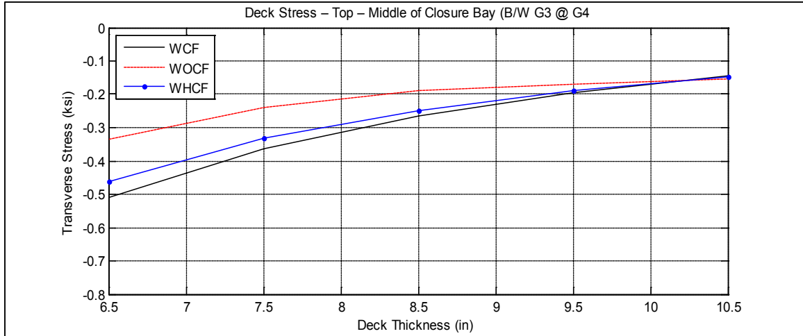
Figure A-12. Transverse deck stresses at top-middle of closure pour vs. deck thickness for bridge I-95 over SR-421
