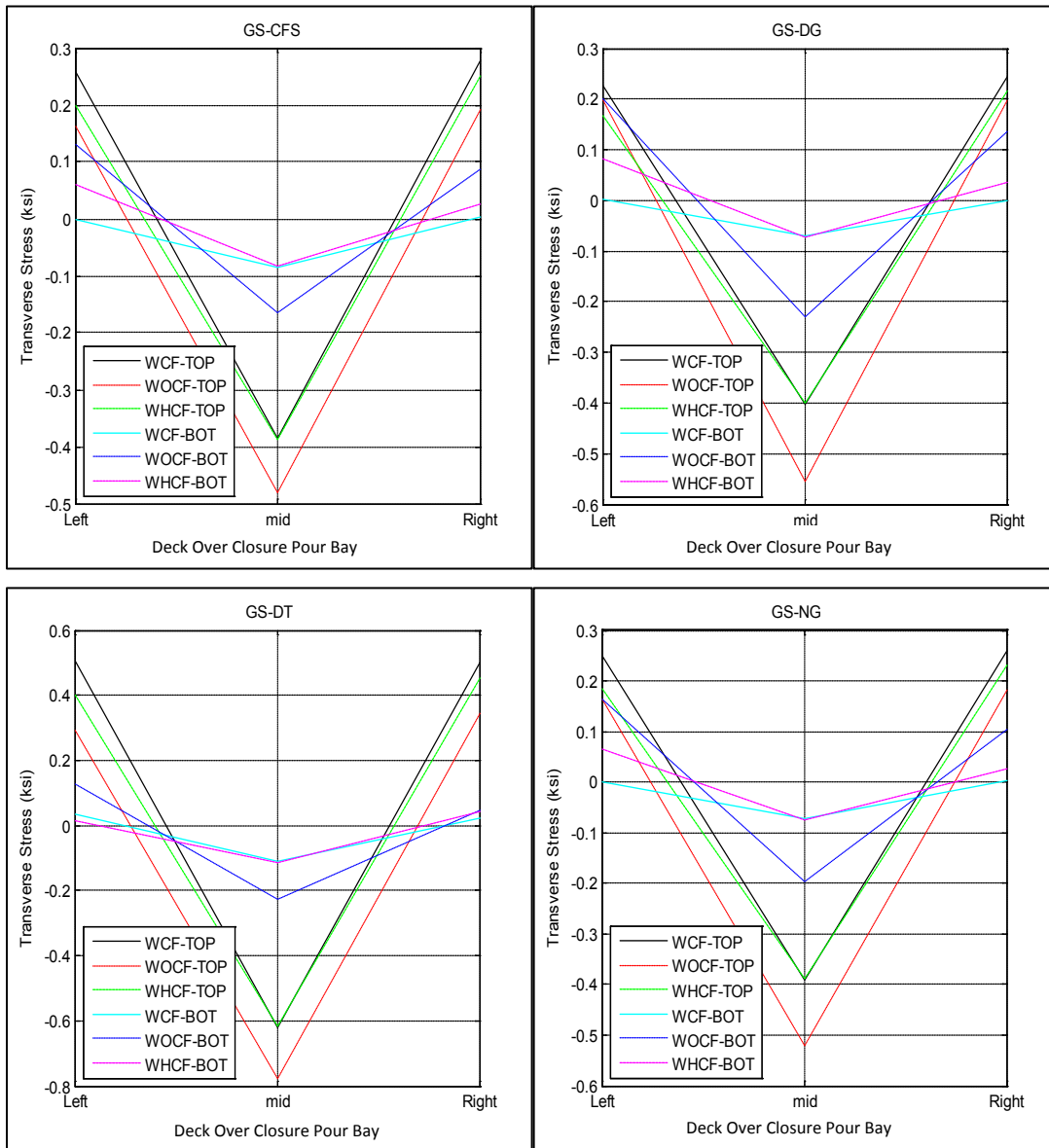
Figure A-35. Transverse stress at closure pour related to different parameter combinations for bridge I-95 over SR-421
