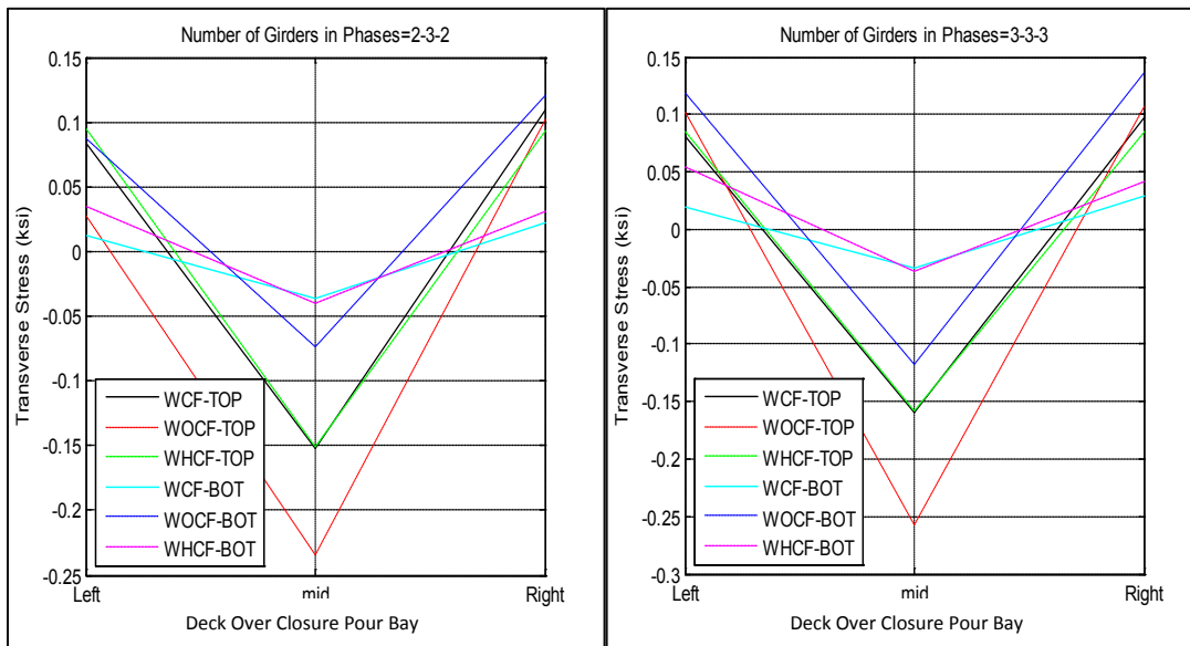
Figure A-62. Transverse stress at closure pour related to different number of girders in phases for SR-589 over Waters Avenue
