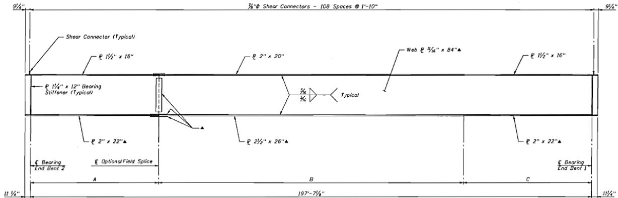
Figure 6-10. Typical details of girders of the SR-589 Bridge over Hillsborough Avenue
