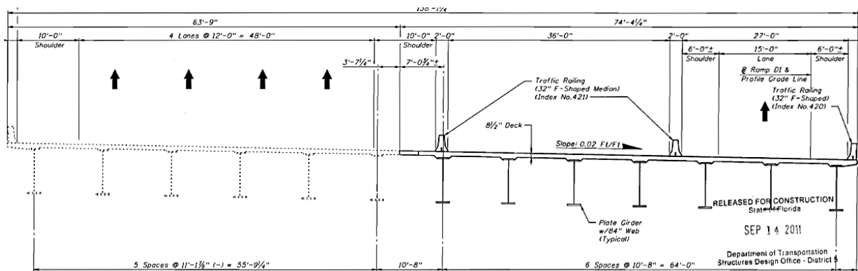
Figure 6-7. Cross-section of the bridge SR-589 over Hillsborough Avenue
