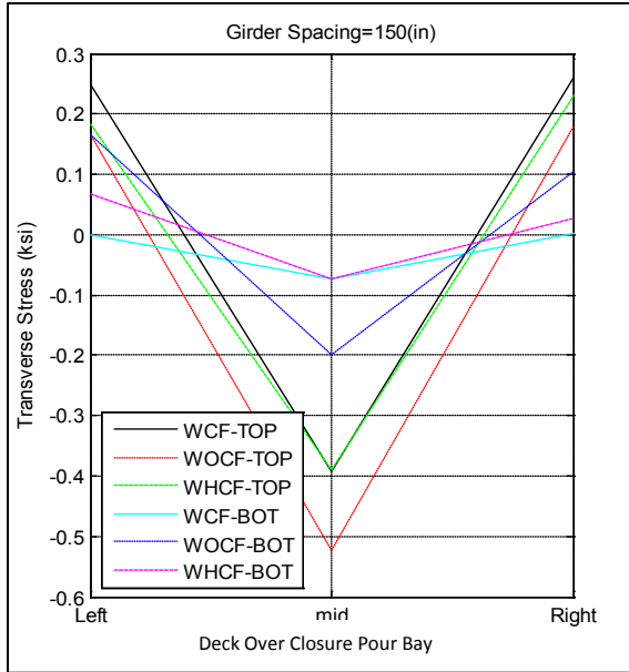
Figure A-4. Transverse stress at closure pour related to girder spacing; 150 in for bridge I-95 over SR-421
