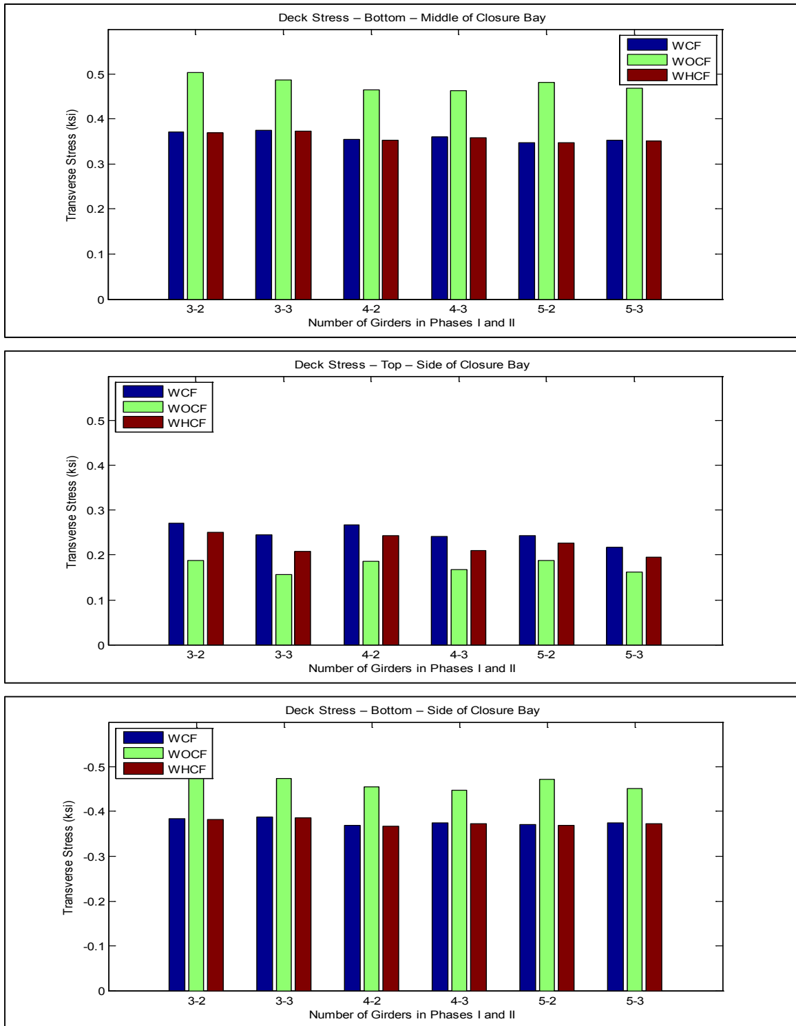
Figure A-31. Transverse deck stresses at middle and side of closure pour vs. number of girders in phases for bridge I-95 over SR-421
