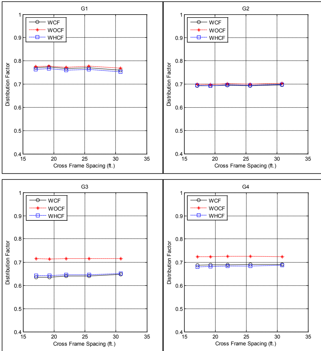
Figure A-19. Distribution factor for girders G1, G2, G3 and G4 related to different cross frame spacing for bridge I-95 over SR-421
