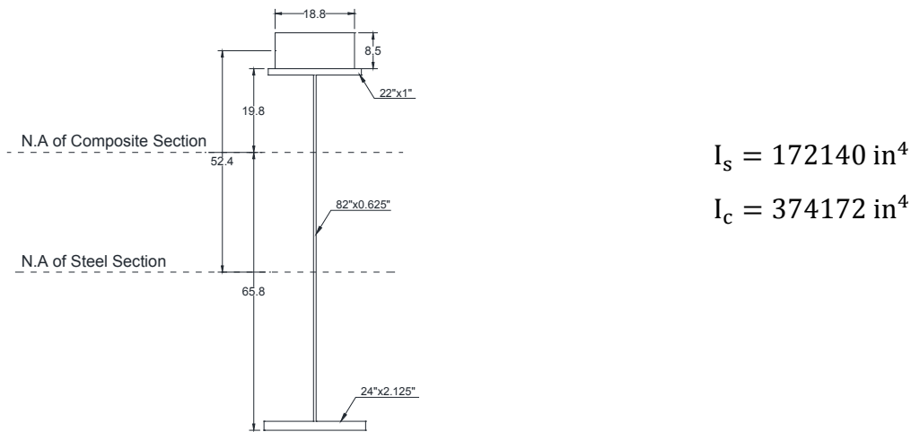
Figure 6-12. Details of steel and composite cross-section
