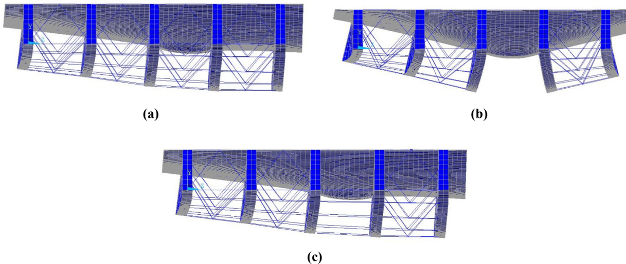
Figure 4-10. Bridge I-95 over SR-421 deformed shape in three different cases: (a) WCF; (b) WOCF; (c) WHCF
