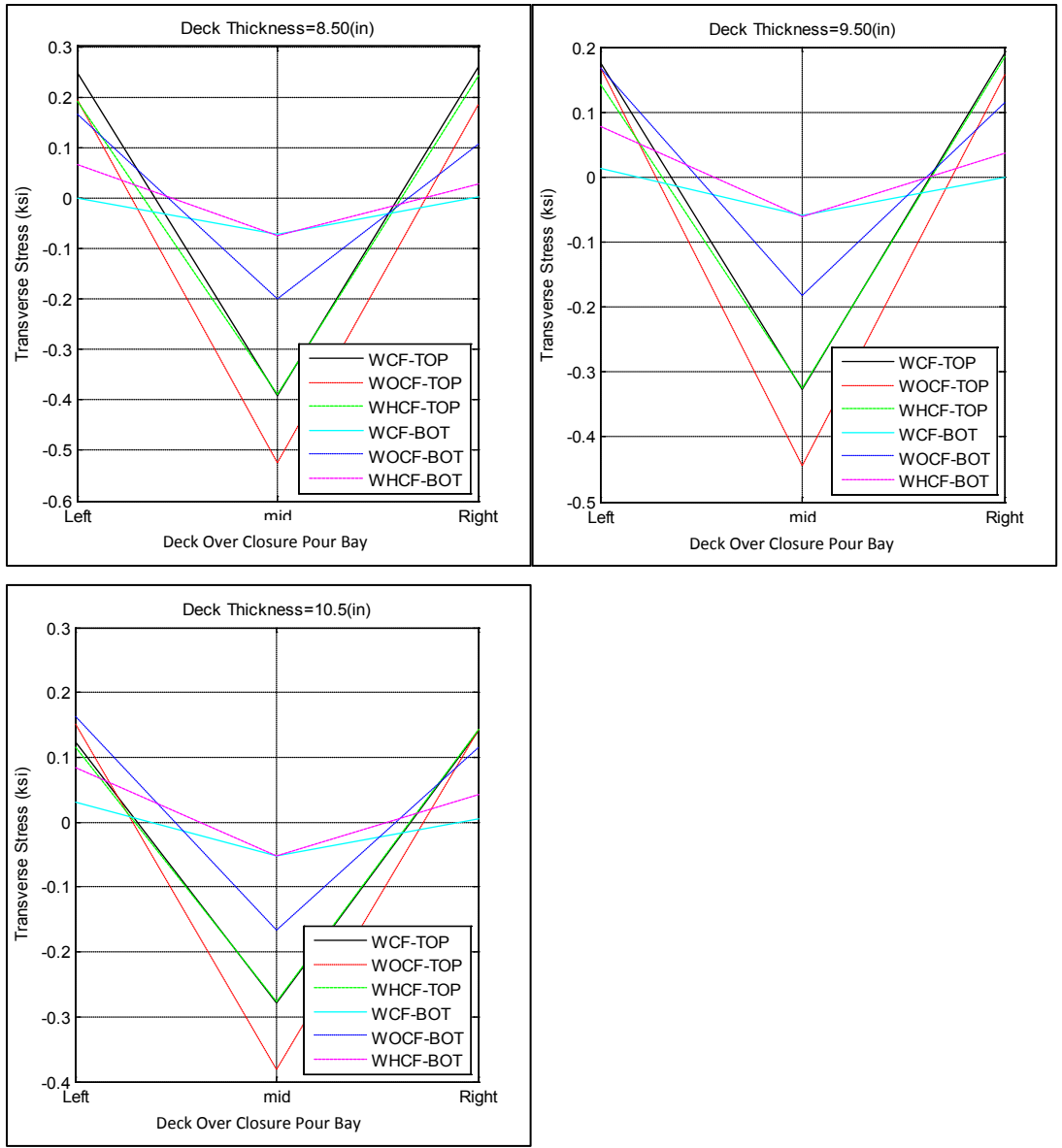
Figure A-10. Transverse stress at closure pour related to deck thicknesses; 8.5, 9.5 and 10.5 inches for bridge I-95 over SR-421
