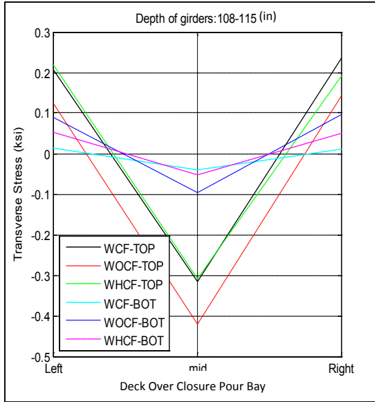
Figure A-50. Transverse stress at closure pour related to different depth of girders for SR-589 over Waters Avenue – Cont'd
