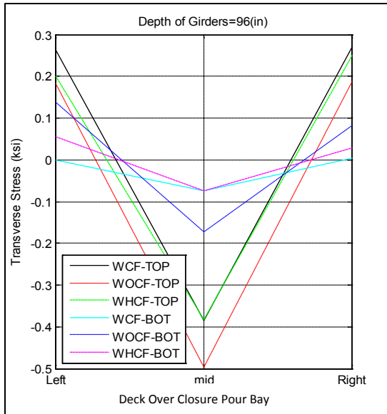
Figure A-16. Transverse stress at closure pour related to depth of girders; 96 inches for bridge I-95 over SR-421
