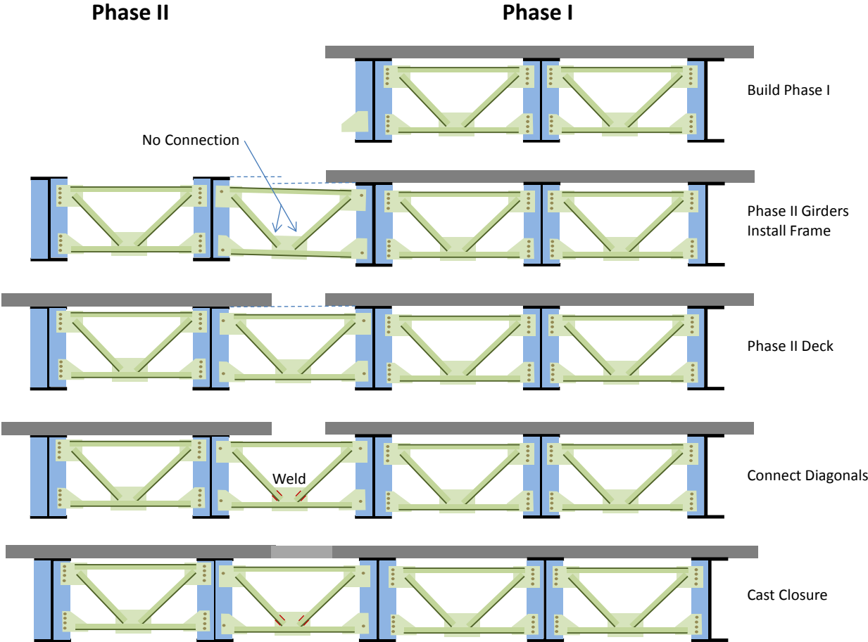
Figure 5-2. Delayed installation of diagonal elements
