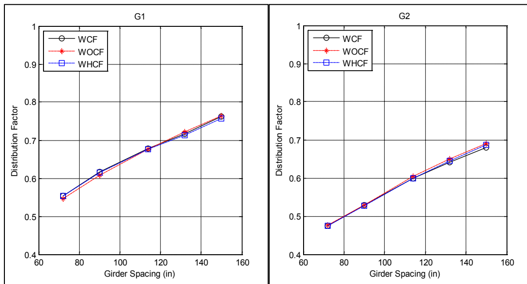
Figure A-1. Distribution factor for girders G1 and G2 related to different girder spacing for bridge I-95 over SR-421
