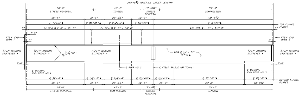
Figure 6-4. Girder elevation for the SR-589 Bridge over Hillsborough Avenue
