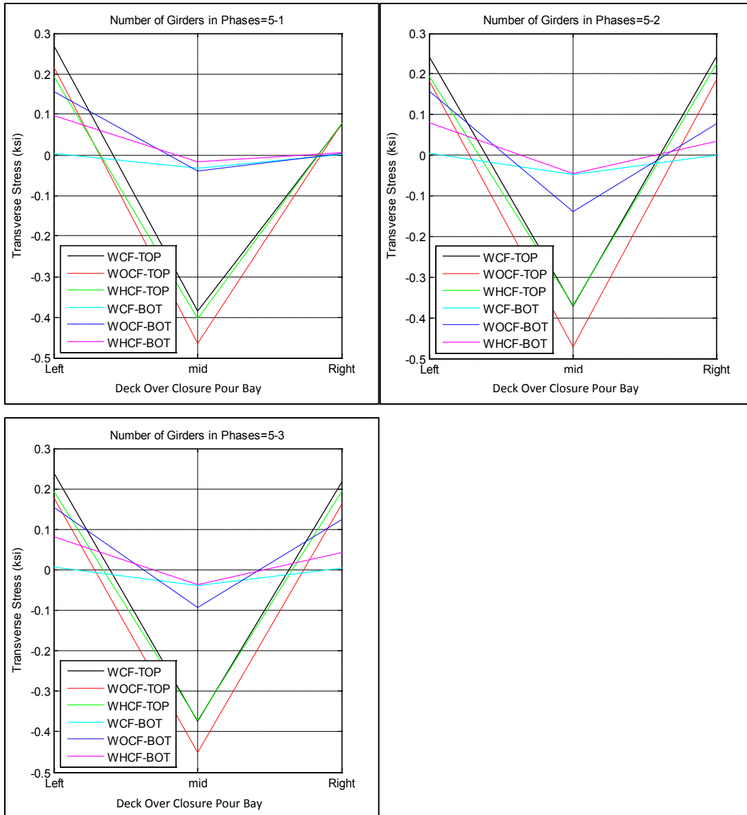
Figure A-30. Transverse stress at closure pour related to different number of girders in phase I and II; 5-1, -5-2 and 5-3 for bridge I-95 over SR-421
