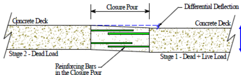
Figure 2-1. Illustration of differential deflection at a closure pours
