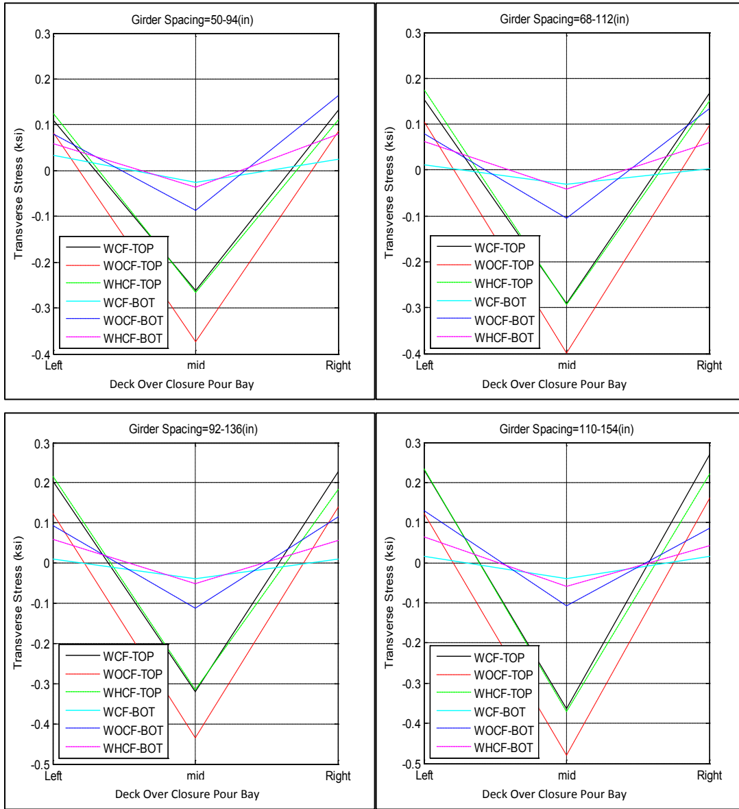
Figure A-40. Transverse stress at closure pour related to different girder spacing for SR-589 over Waters Avenue
