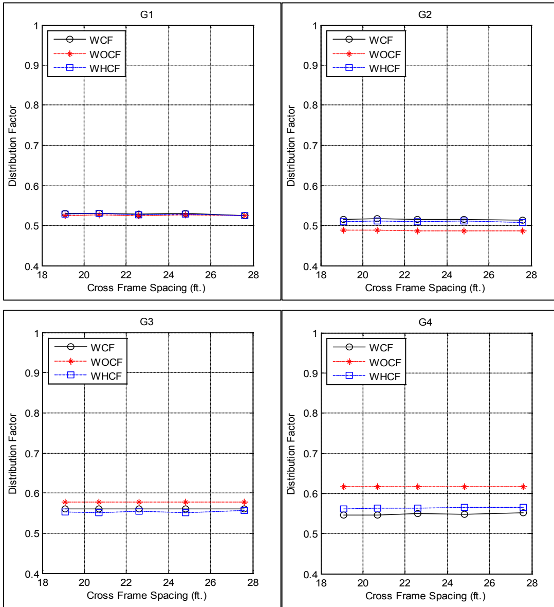
Figure A-53. Distribution factor for girders G1, G2, G3 and G4 related to different cross frame spacing for bridge SR-589 over Waters Avenue
