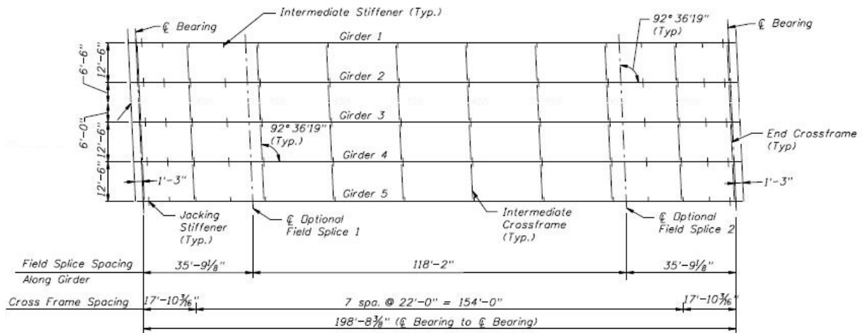
Figure 4-2. Framing plan of the I-95 Bridge over SR-421
