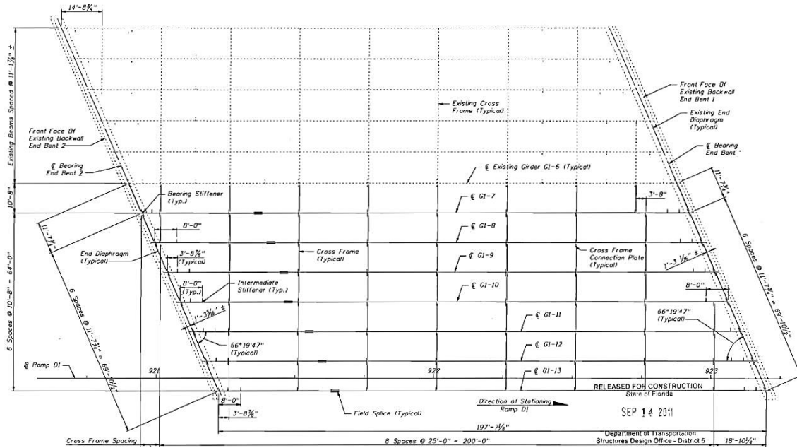
Figure 6-8. Framing plan of the SR-589 Bridge over Hillsborough Avenue
