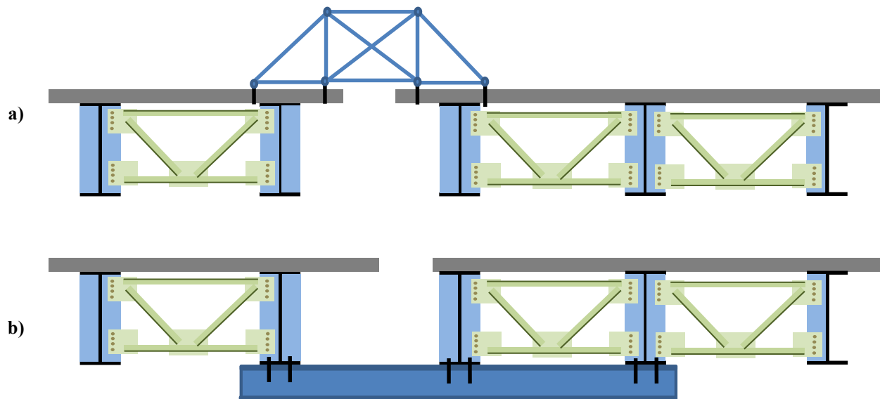
Figure 2-2. Temporary connection between the phases
