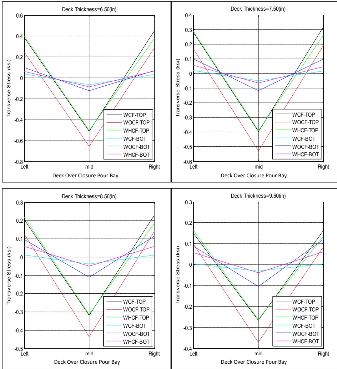
Figure A-45. Transverse stress at closure pour related to different deck thicknesses for SR-589 over Waters Avenue
