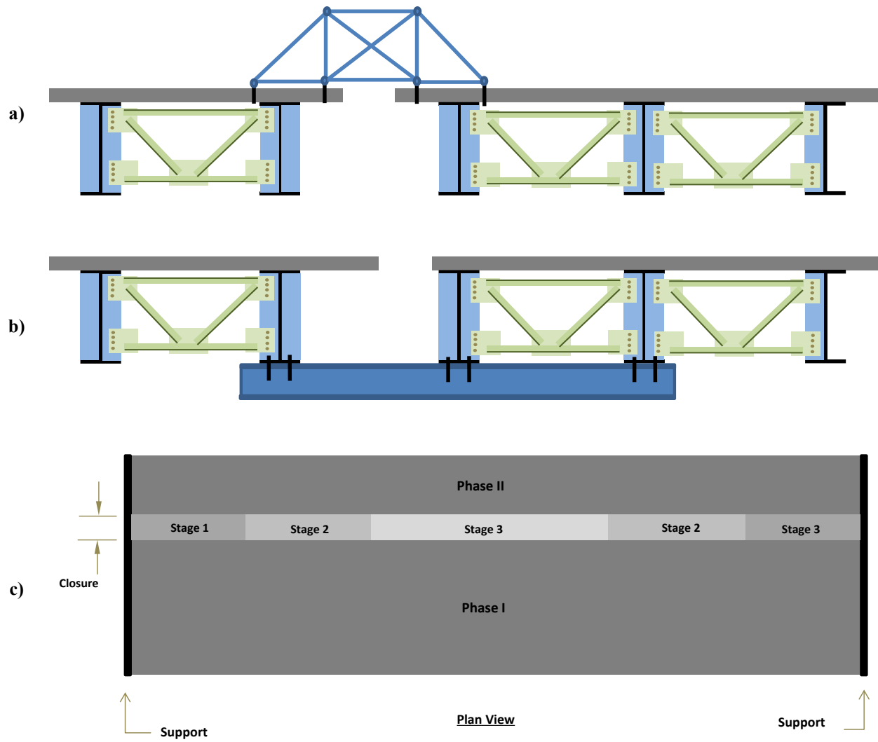
Figure 5-7. Vibration mitigation methods a & b) Temporary connection c) staged casting of closure
