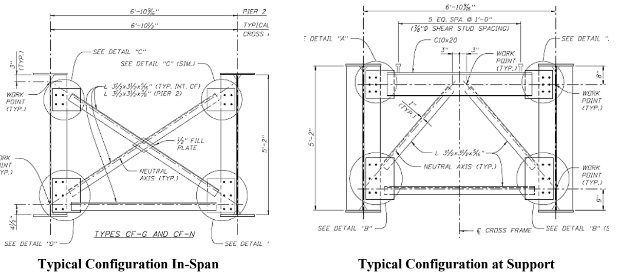
Figure 6-3. Cross-frame details of the SR-589 Bridge over Hillsborough Avenue
