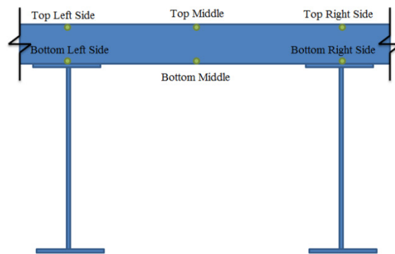
Figure 3-5. Position of the points where the stresses of deck were obtained
