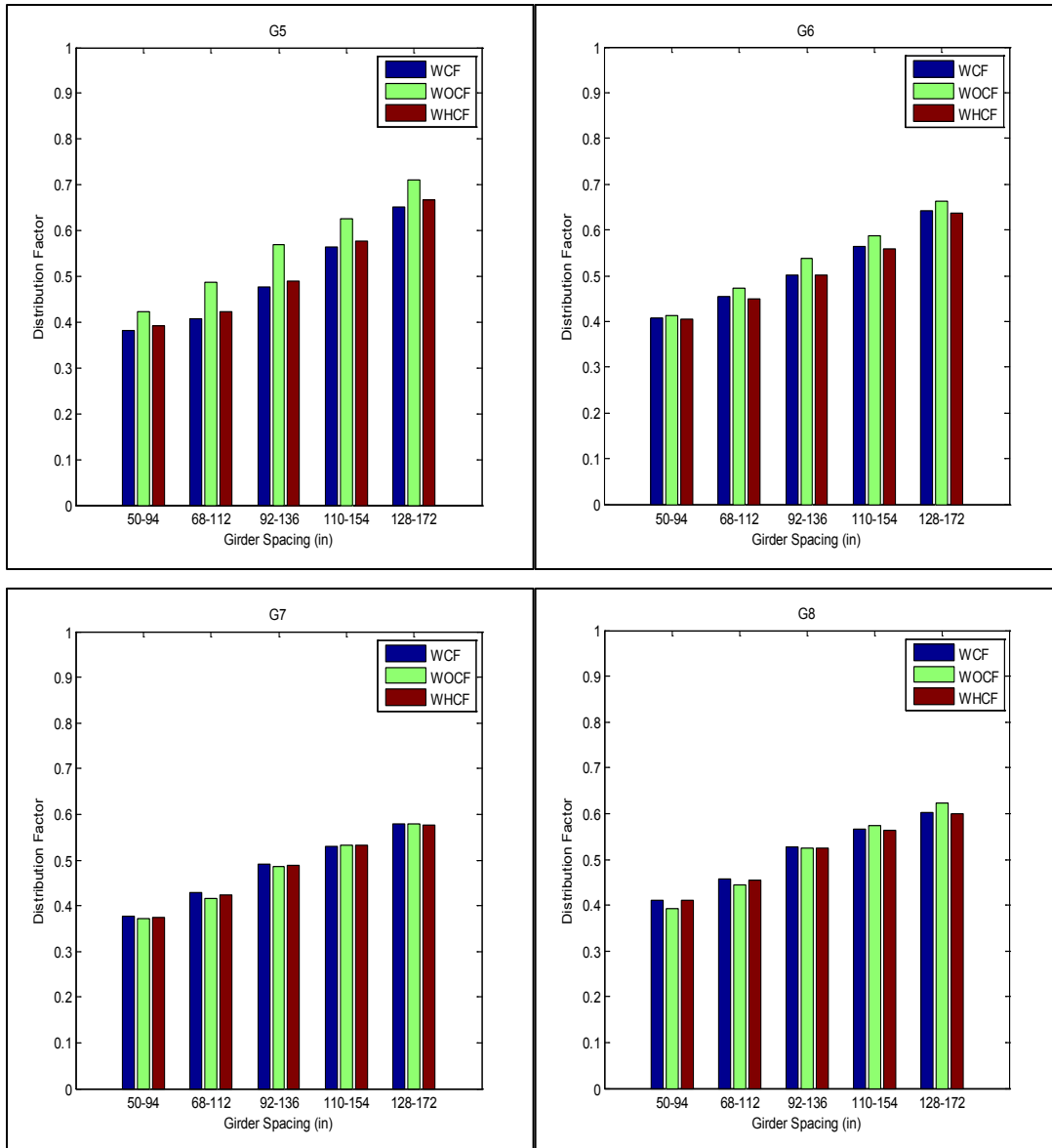
Figure A-39. Distribution factor for girders G5, G6, G7 and G8 related to different girder spacing for bridge SR-589 over Waters Avenue
