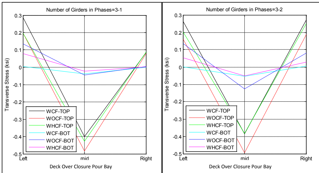
Figure A-28. Transverse stress at closure pour related to different number of girders in phase I and II; 3-1 and 3-2 for bridge I-95 over SR-421
