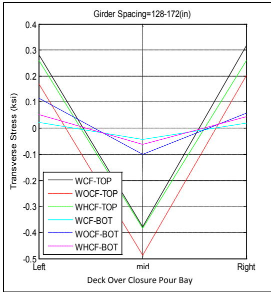
Figure A-40. Transverse stress at closure pour related to different girder spacing for SR-589 over Waters Avenue – Cont'd
