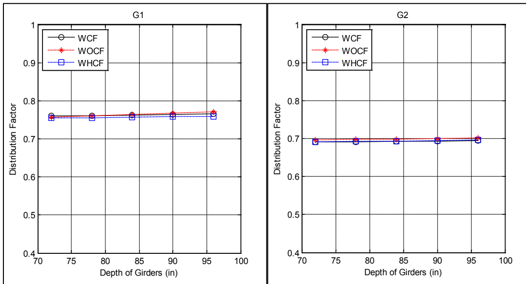
Figure A-13. Distribution factor for girders G1 and G2 related to different depth of girders for bridge I-95 over SR-421
