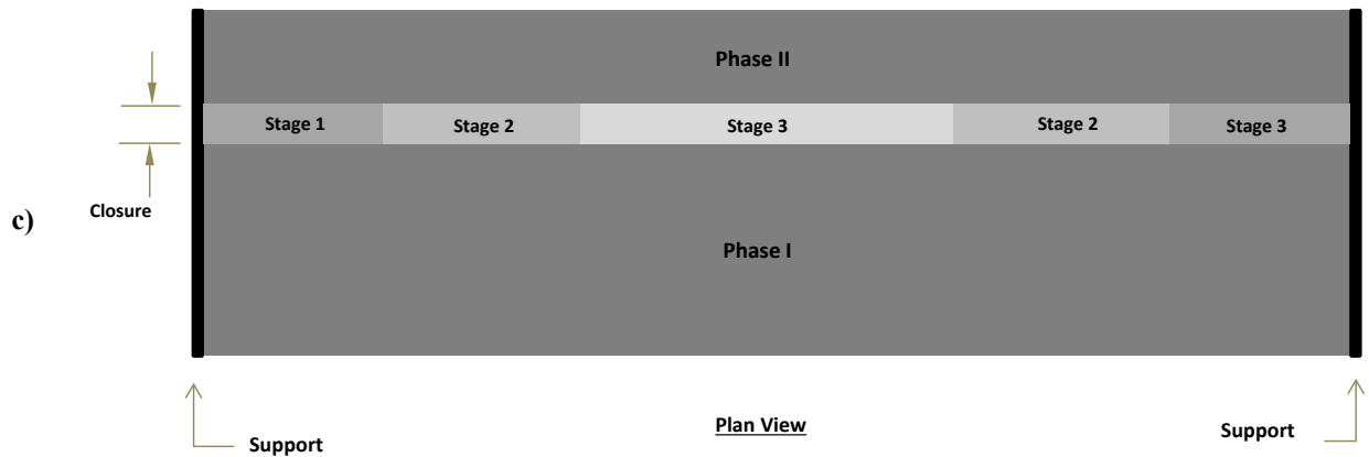
Figure 2-3 Staged casting of closure region
