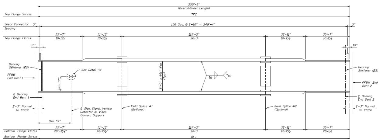
Figure 4-8. Typical Details of Girders of the Bridge SR-589 over Waters Avenue
