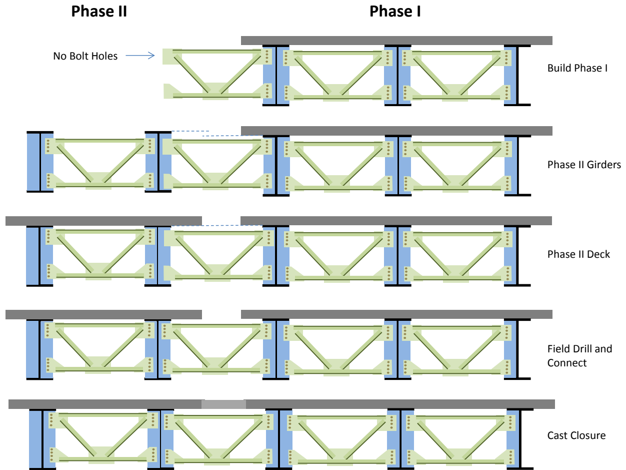
Figure 5-1. Field drilled connection
