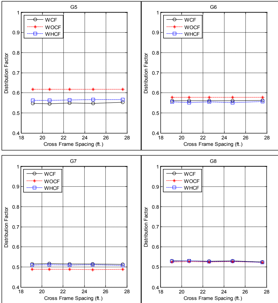
Figure A-54. Distribution factor for girders G5, G6, G7 and G8 related to different cross frame spacing for bridge SR-589 over Waters Avenue
