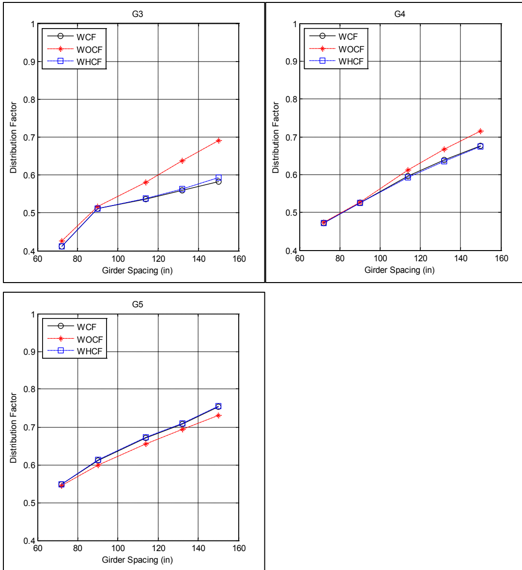
Figure A-2. Distribution factor for girders G3, G4 and G5 related to different girder spacing for bridge I-95 over SR-421
