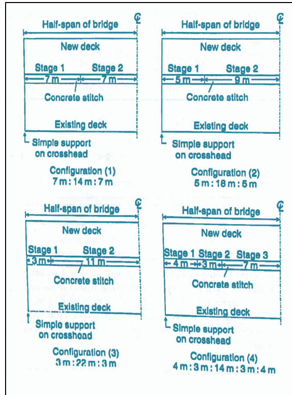
Figure 2-4. Different sequences of casting the closure region (Kwan and Ng, 2006)
