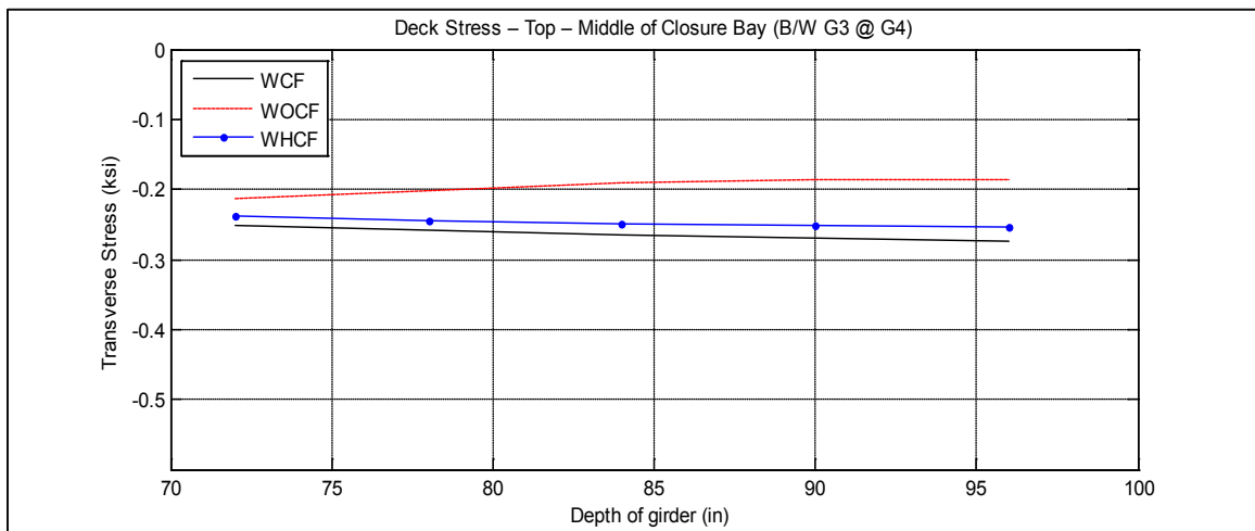
Figure A-18. Transverse deck stresses at middle and side of closure pour vs. depth of girders for bridge I-95 over SR-421
