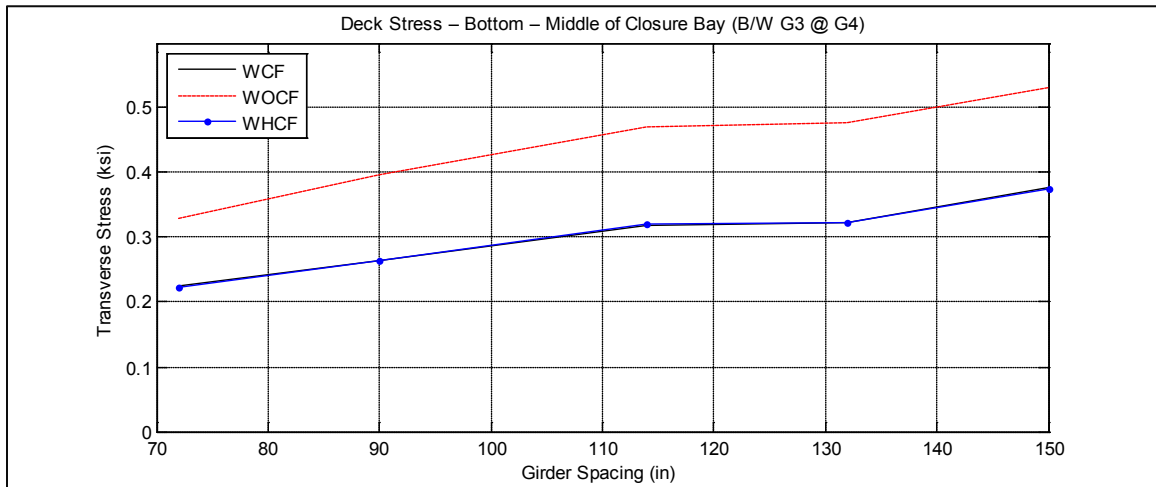
Figure A-5. Transverse deck stresses at Bottom -middle of closure pour vs. girder spacing for bridge I-95 over SR-421
