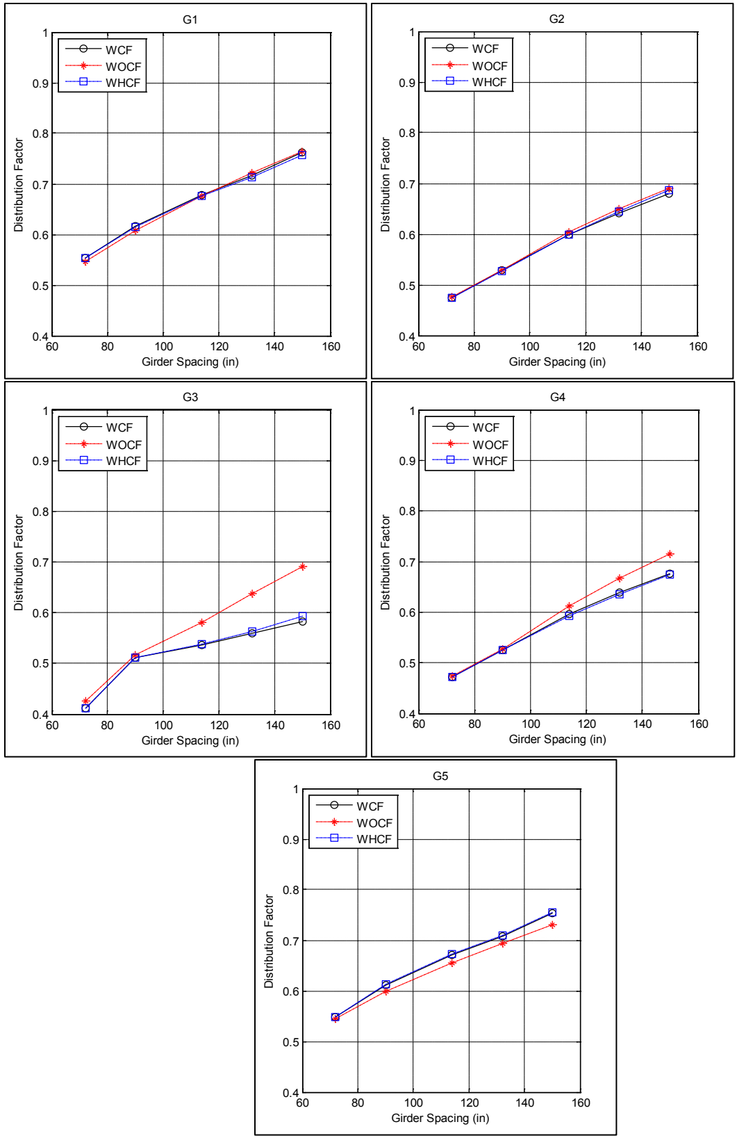
Figure 4-11. Distribution factor vs. girder spacing for all girders of bridge I-95 over SR-421
