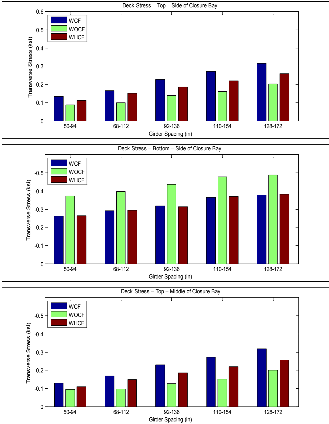
Figure A-42. Transverse deck stresses at middle and side of closure pour vs. girder spacing for bridge SR-589 over Waters Avenue
