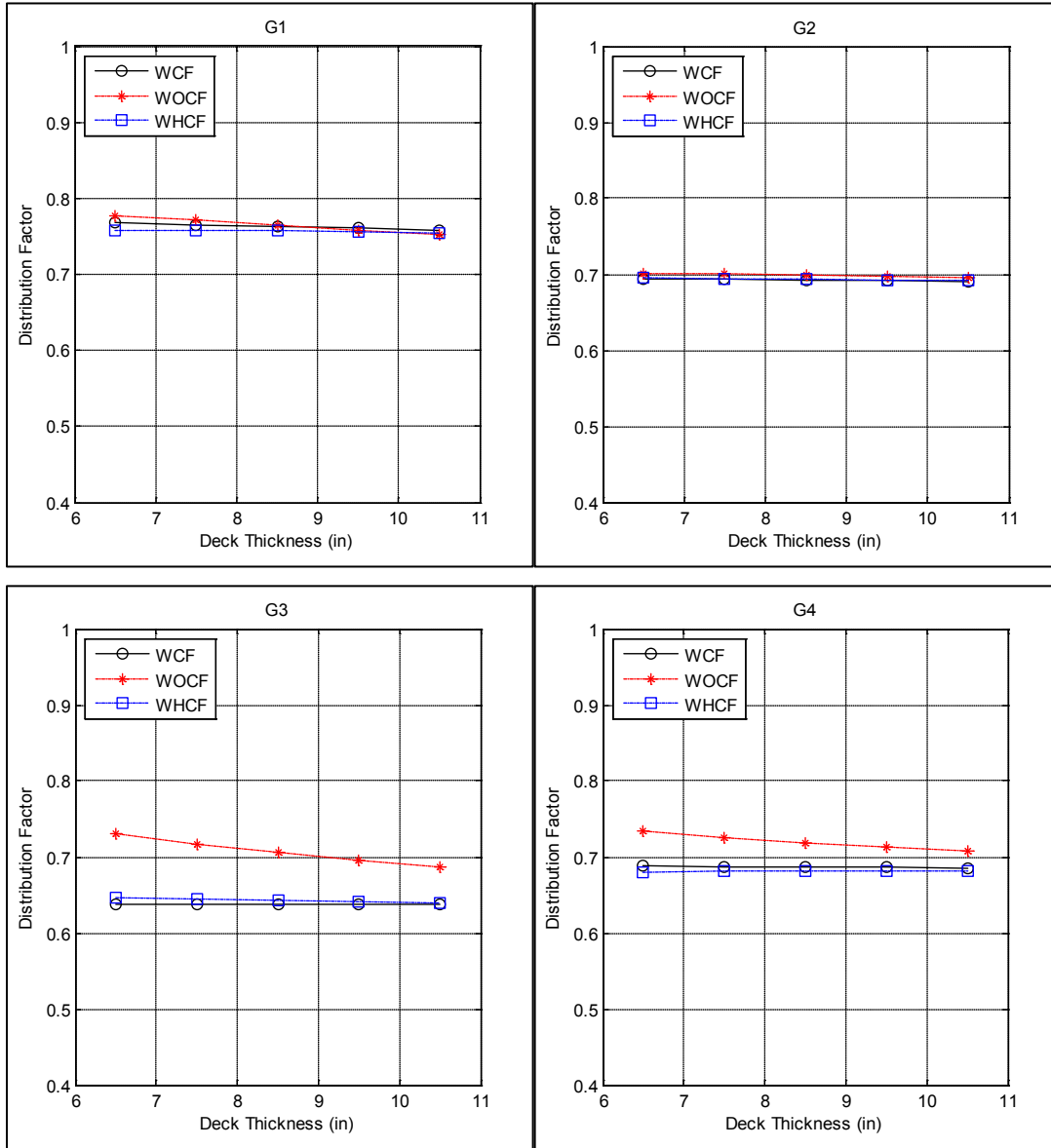
Figure A-7. Distribution factor for girders G1, G2, G3 and G4 related to different deck thicknesses for bridge I-95 over SR-421
