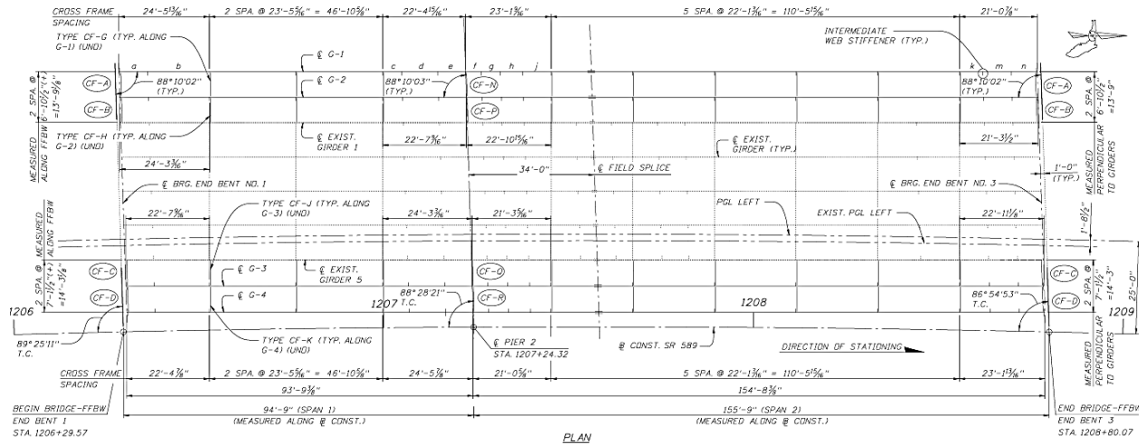
Figure 6-2. Framing plan of the SR-589 Bridge over Hillsborough Avenue
