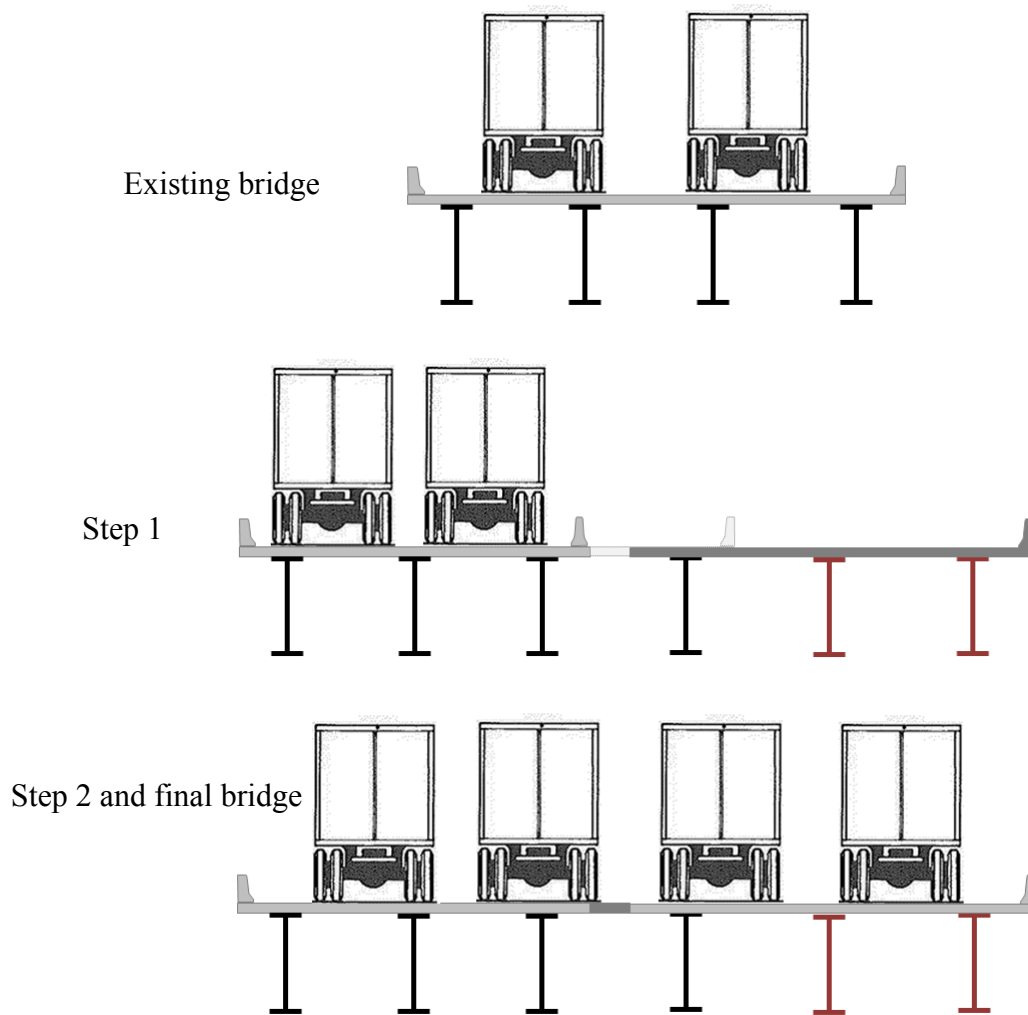
Figure 1-3. Typical construction sequences of a bridge widening using phase construction approach
