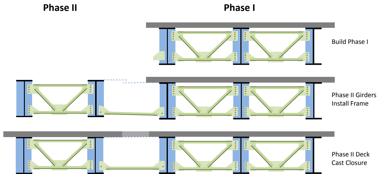
Figure 5-3. Horizontal struts between construction phases
