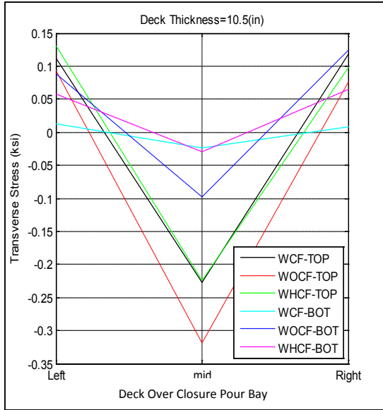
Figure A-45. Transverse stress at closure pour related to different deck thicknesses for SR-589 over Waters Avenue – Cont'd
