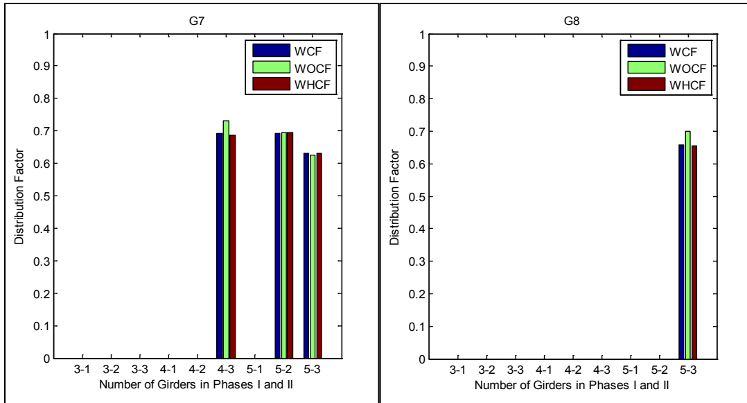
Figure A-27. Distribution factor for girders G7 and G8 related to different phase I and II configurations for bridge I-95 over SR-421
