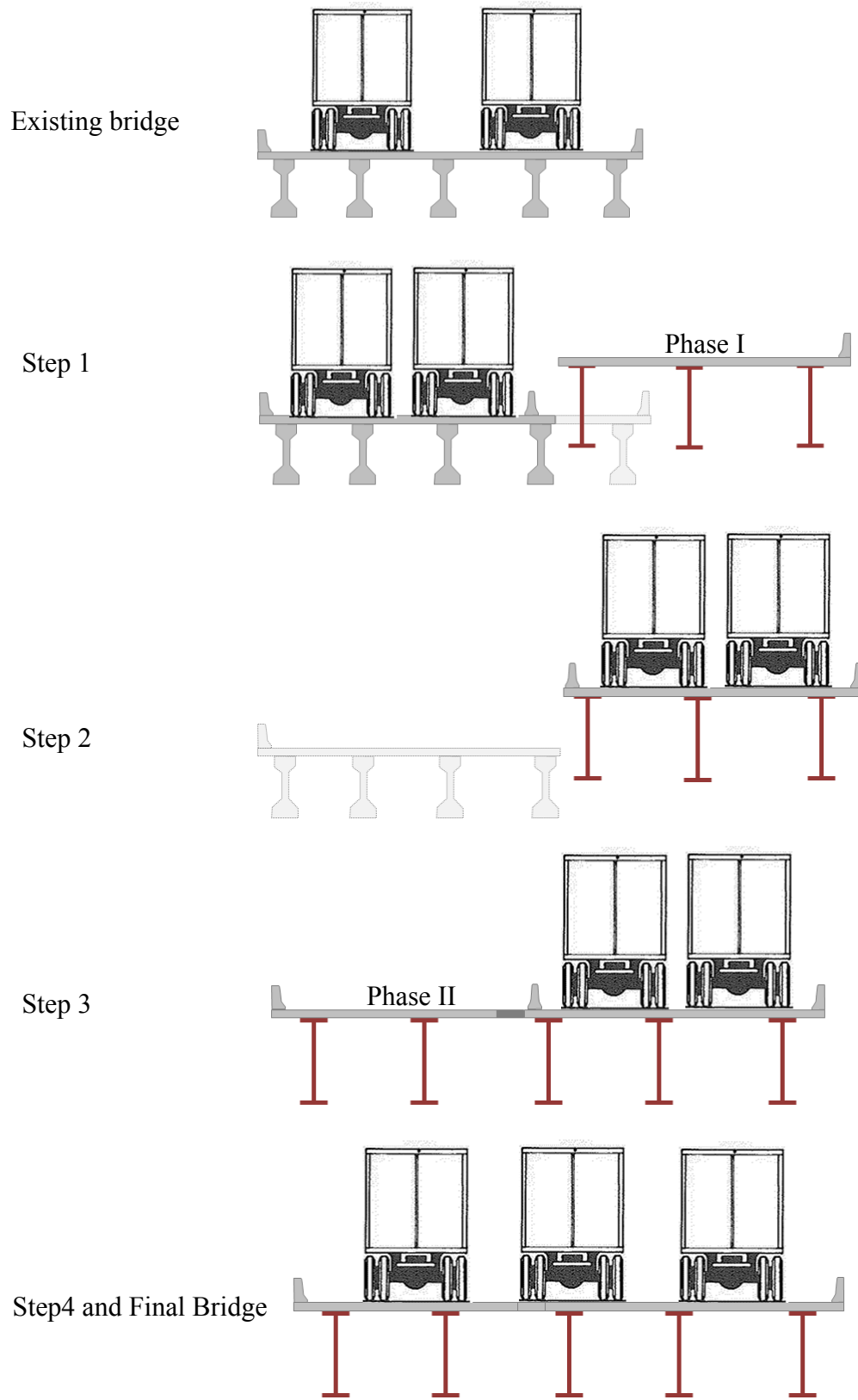
Figure 1-2. Typical construction sequences of a bridge replacement using phase construction approach
