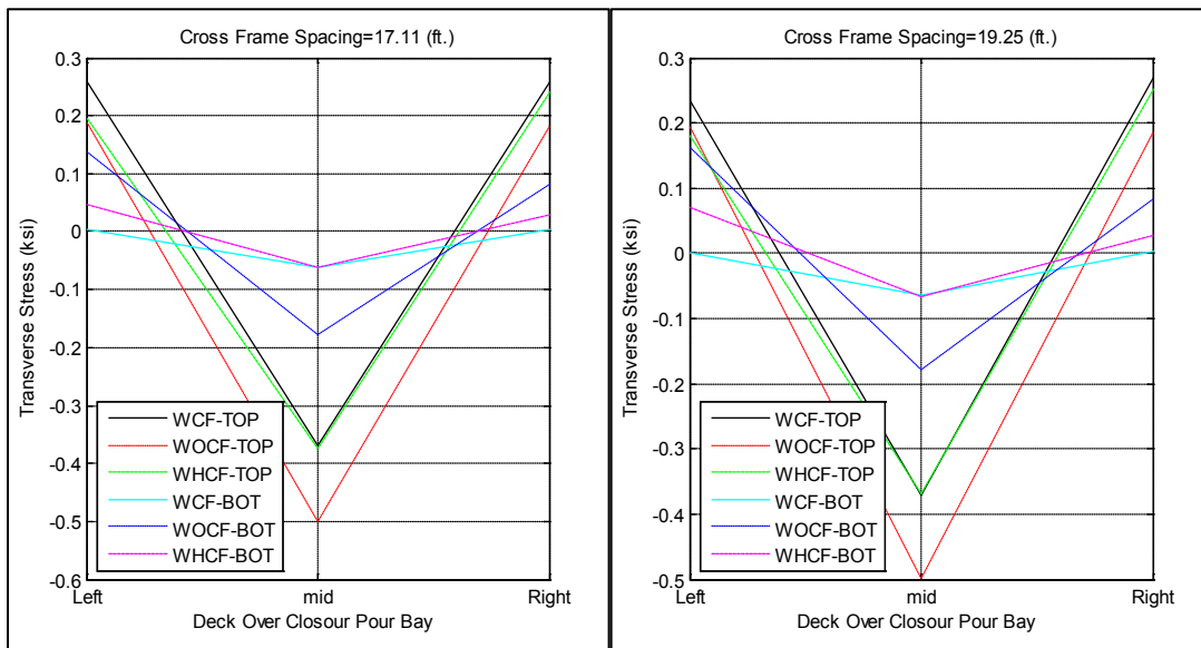
Figure A-21. Transverse stress at closure pour related to different cross frame spacing; 17.11 and 19.25 ft. for bridge I-95 over SR-421
