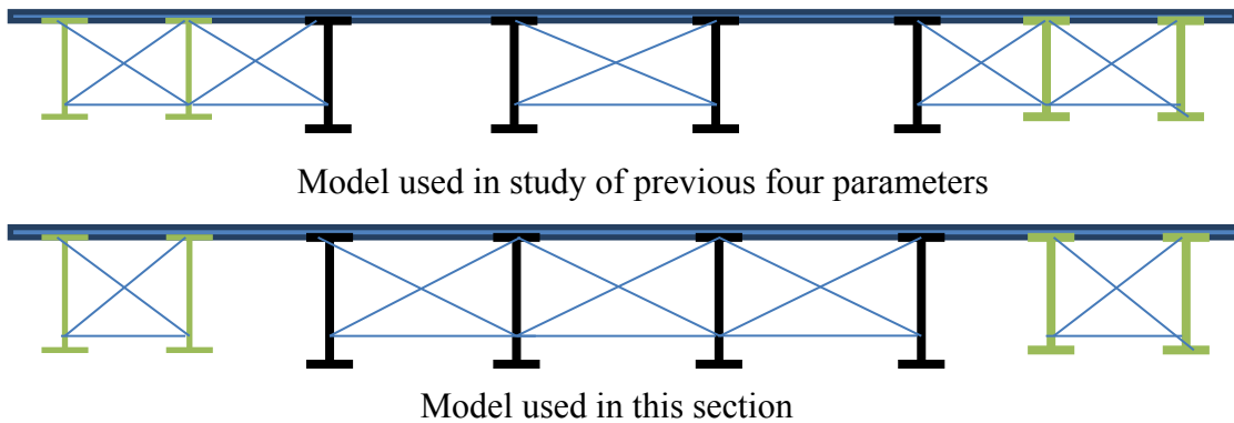
Figure 4-17. Difference between models used for bridge SR-589 over Waters Avenue in this section and previous sections
