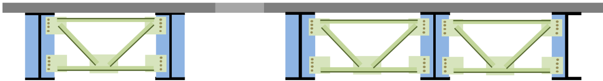
Figure 5-6. Elimination of cross-frames between construction phases
