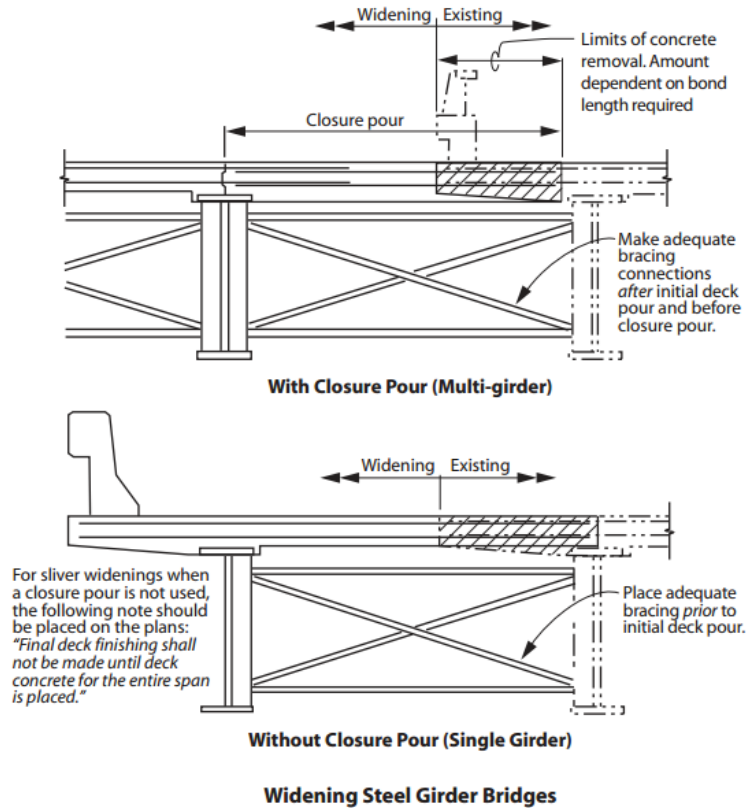
Figure 1-4. Widening steel girder bridges with and without closure pour
