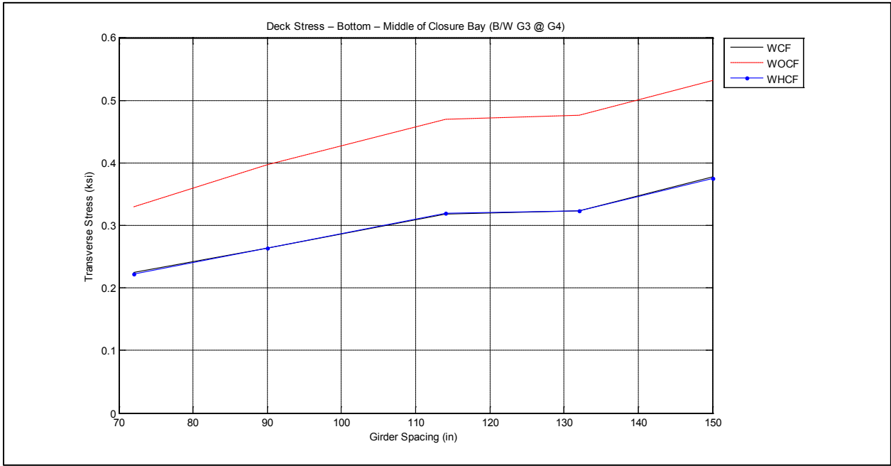
Figure 4-14. Transverse stress of the deck vs. girder spacing at bottom mid-point
