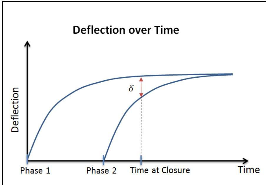
Figure 1-5. Figure displacement of phase I and phase II portion of the bridge
