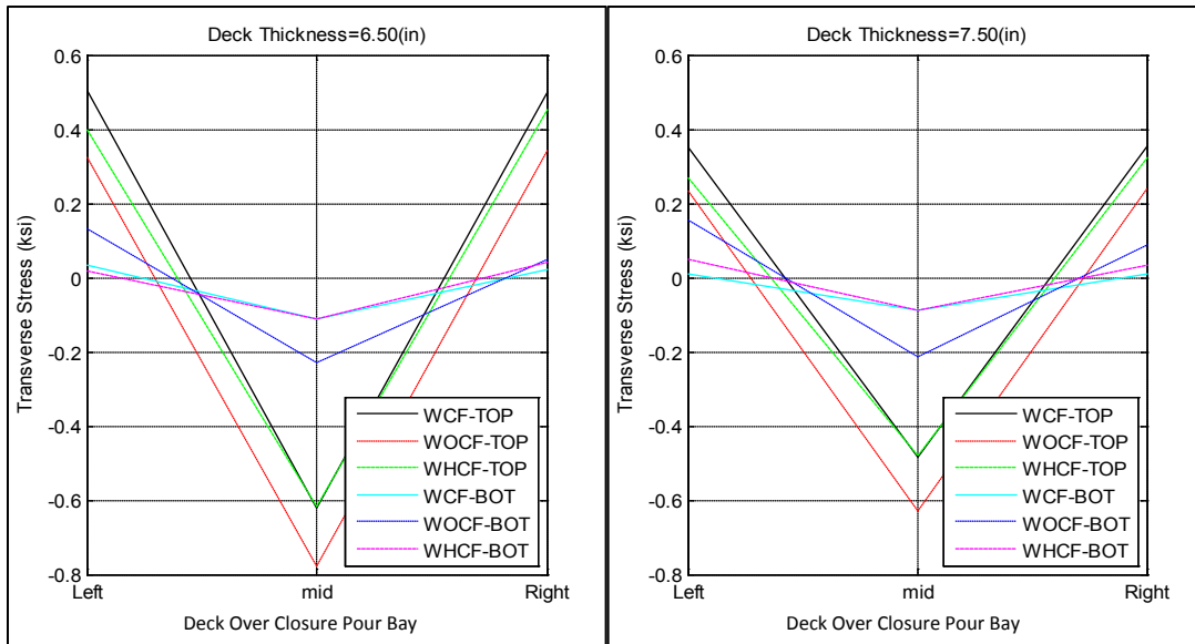
Figure A-9. Transverse stress at closure pour related to deck thicknesses; 6.5 and 7.5 inches for bridge I-95 over SR-421
