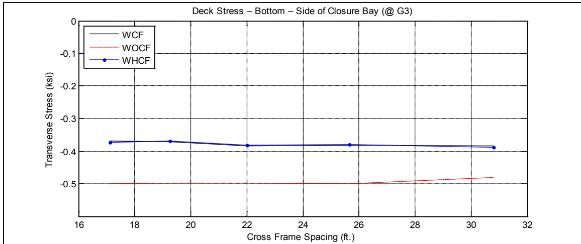
Figure A-24. Transverse deck stresses at Bottom -side of closure pour vs. cross-frame spacing for bridge I-95 over SR-421
