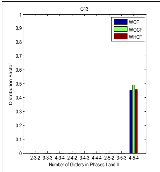
Figure A-61. Distribution factor for girder G13 related to different configuration of phases for bridge SR-589 over Waters Avenue
