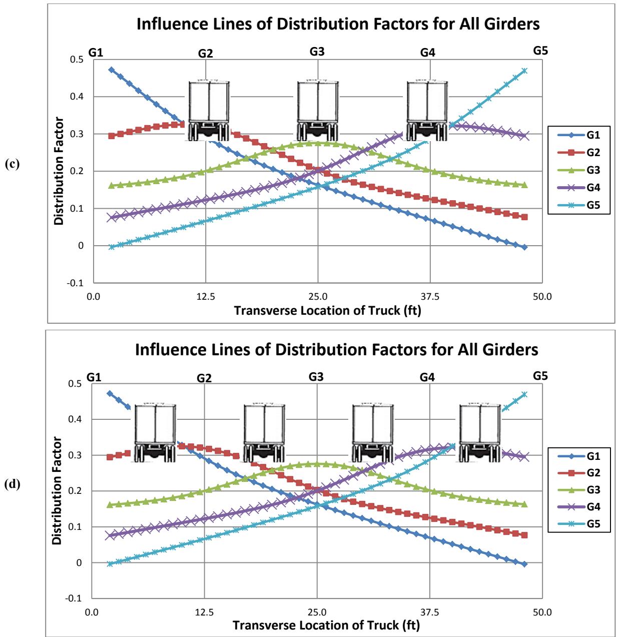
Figure 3-4. The critical positioning for obtaining the distribution factor with: (a) A single truck, (b) Two trucks, (c) Three trucks, (d) Four trucks – Cont'd
