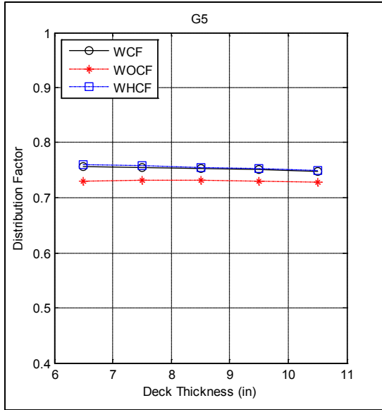
Figure A-8. Distribution factor for girder G5 related to different deck thicknesses for bridge I-95 over SR-421
