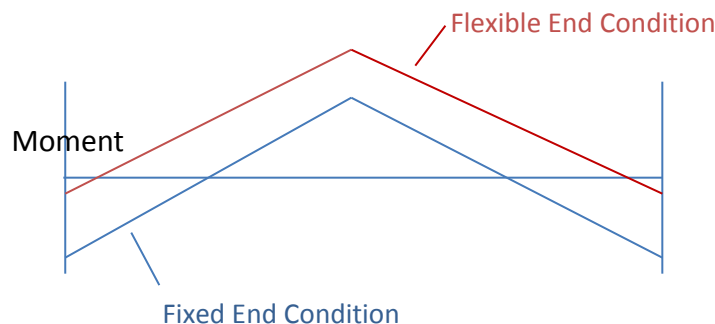
Figure 4-18. Difference moment distribution due to different end flexibility condition.
