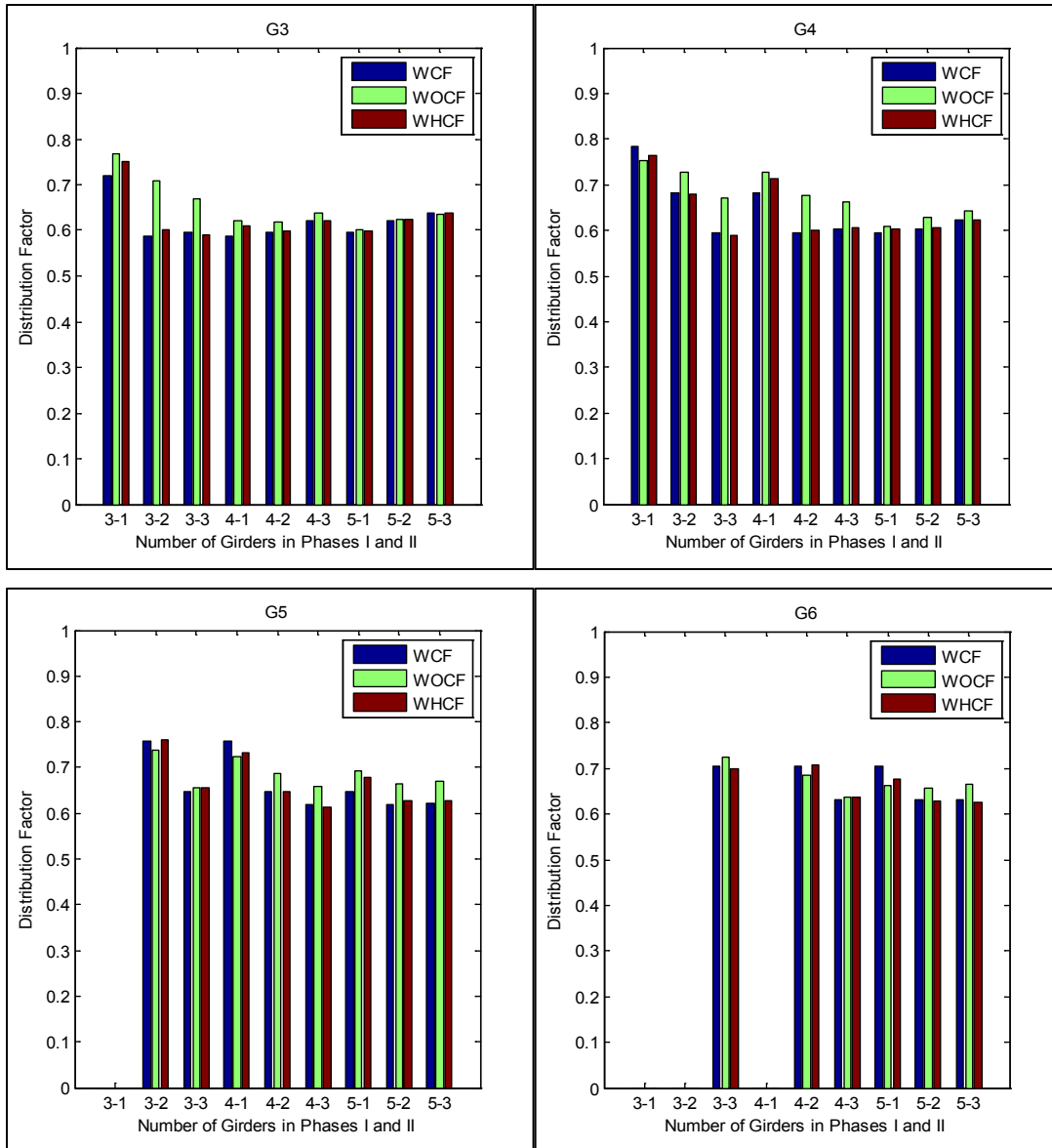
Figure A-26. Distribution factor for girders G3, G4, G5 and G6 related to different phase I and II configurations for bridge I-95 over SR-421
