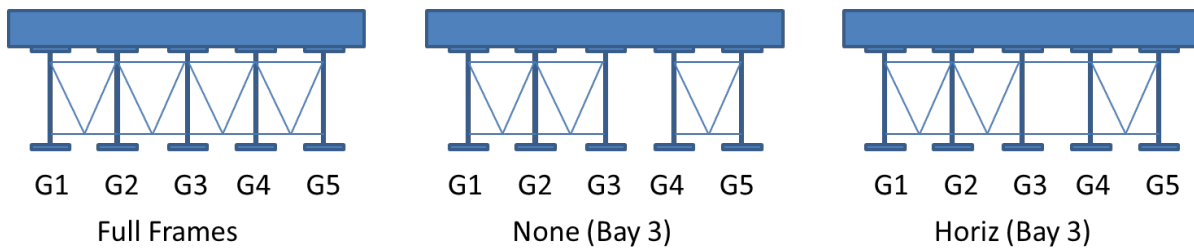
Figure 4-9. Three different investigated cases for bridge I-95 over SR-421
