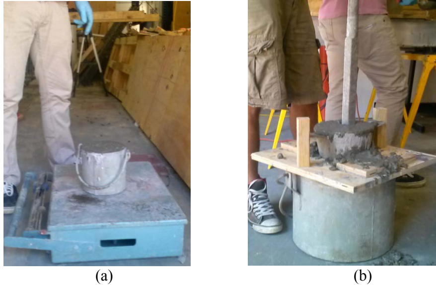
Figure 4.3 - Plastic property measurements (a) unit weight (b) time of flow
