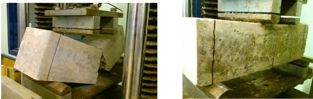
Figure 4.8 - Modes of failure
