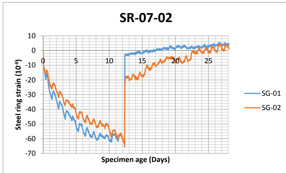
Figure A7. Mix M07: Concrete with 1.5" Polypropylene fibers
