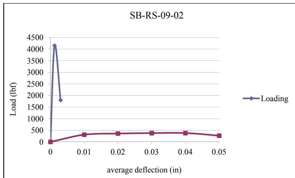
(b) Specimen 2
