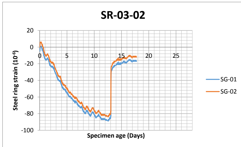
Figure A3. Mix M03: Concrete with steel fibers
