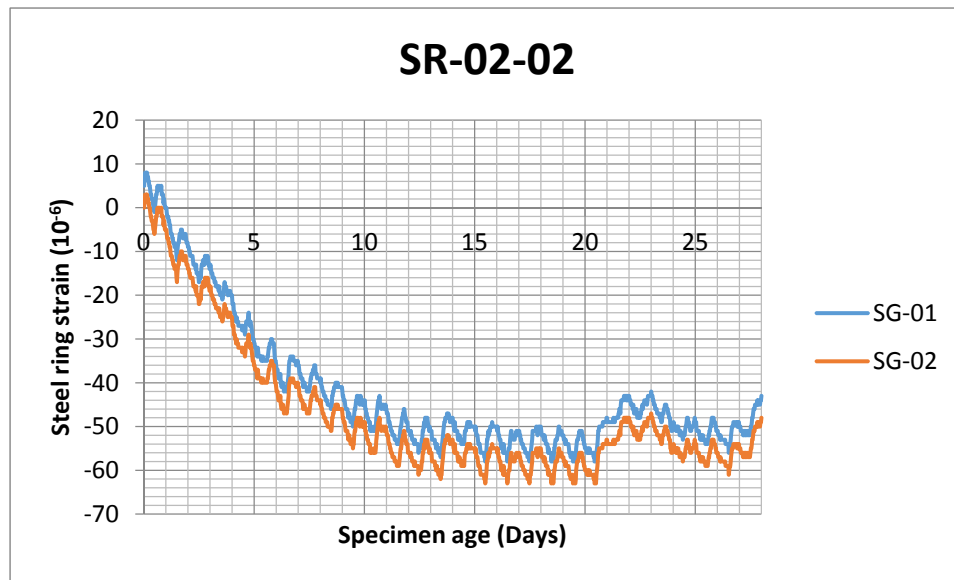
Figure A2. Mix M02: Concrete with 0.5" Polypropylene fibers
