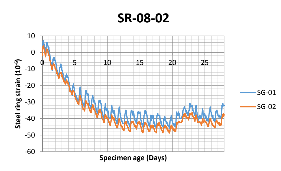
Figure A8. Mix M08: Concrete with 0.75" Polypropylene fibers
