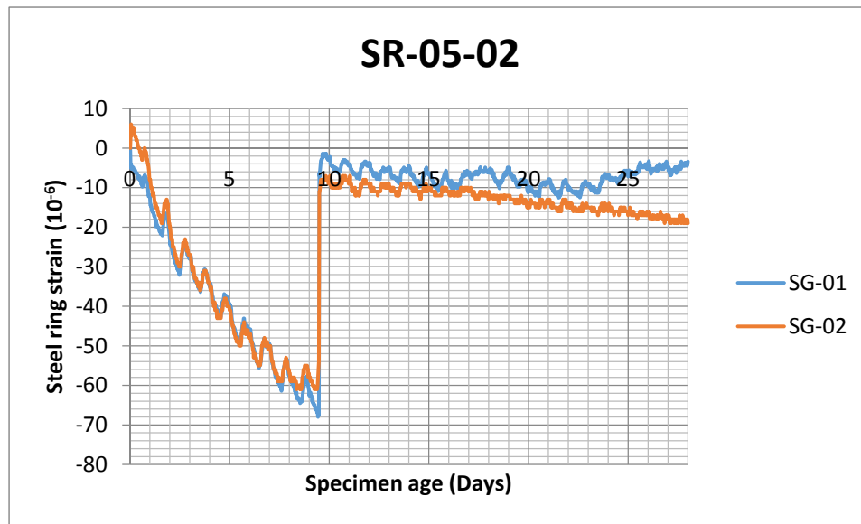
Figure A5. Mix M05: Concrete with Basalt fibers
