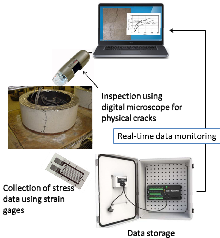
Figure 3.13 - Schematic of restrained shrinkage test
