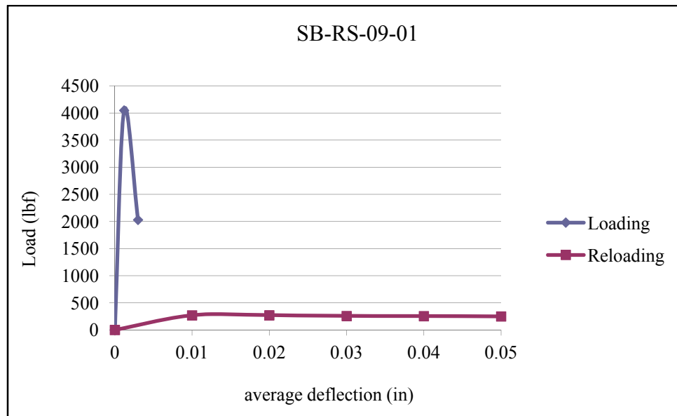
(a) Specimen 1
