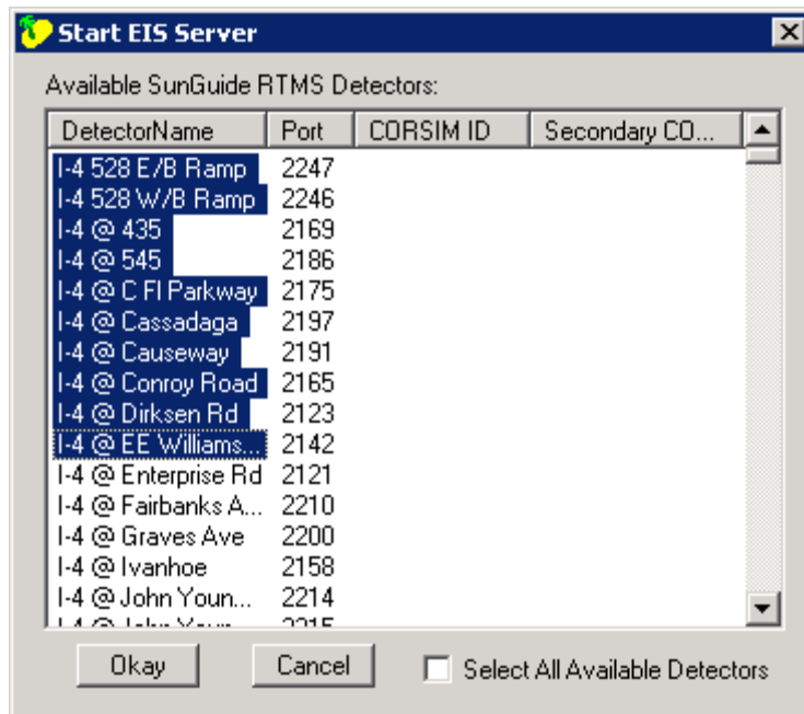
Figure 5-7 RTMS Simulator Interface for Detector Selection
