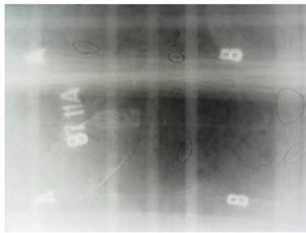
Figure A.13: X-Ray inspection of post-tensioned deck ramp D in Fort Lauderdale: x-ray inspection equipment (left) and example film radiograph (right) (DMJM Harris, 2003)
