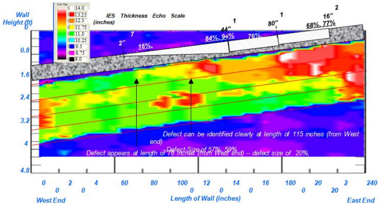
Figure A.18: Image created from impact-echo scan data collected with Olson equipment from the results from the south wall with actual design defects of top duct Orwell bridge. void areas are indicated by (apparent) increased thicknesses as shown in the thickness scale of 1
