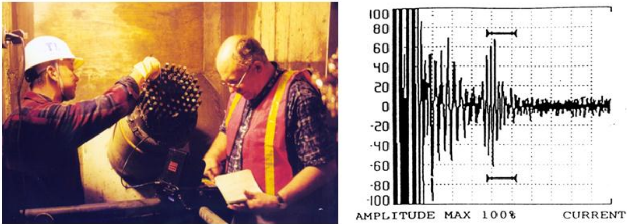
Figure A.14: Ultrasonic guided wave (at 50 khz) testing in progress (left) and a sample signal showing reflection from defect (right)
