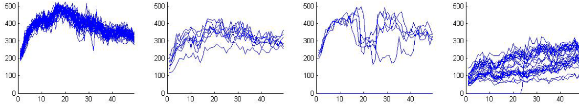
(b) Four clusters. Vertical axis is traffic volume per five minutes and horizontal axis is time in minutes.
