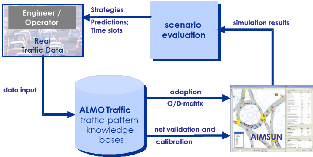
Figure 2-1 Integrated AIMSUN and ALMO Environment
