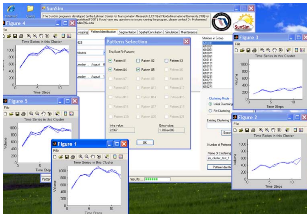
Figure B-8: User Interface for Data Clustering Results
