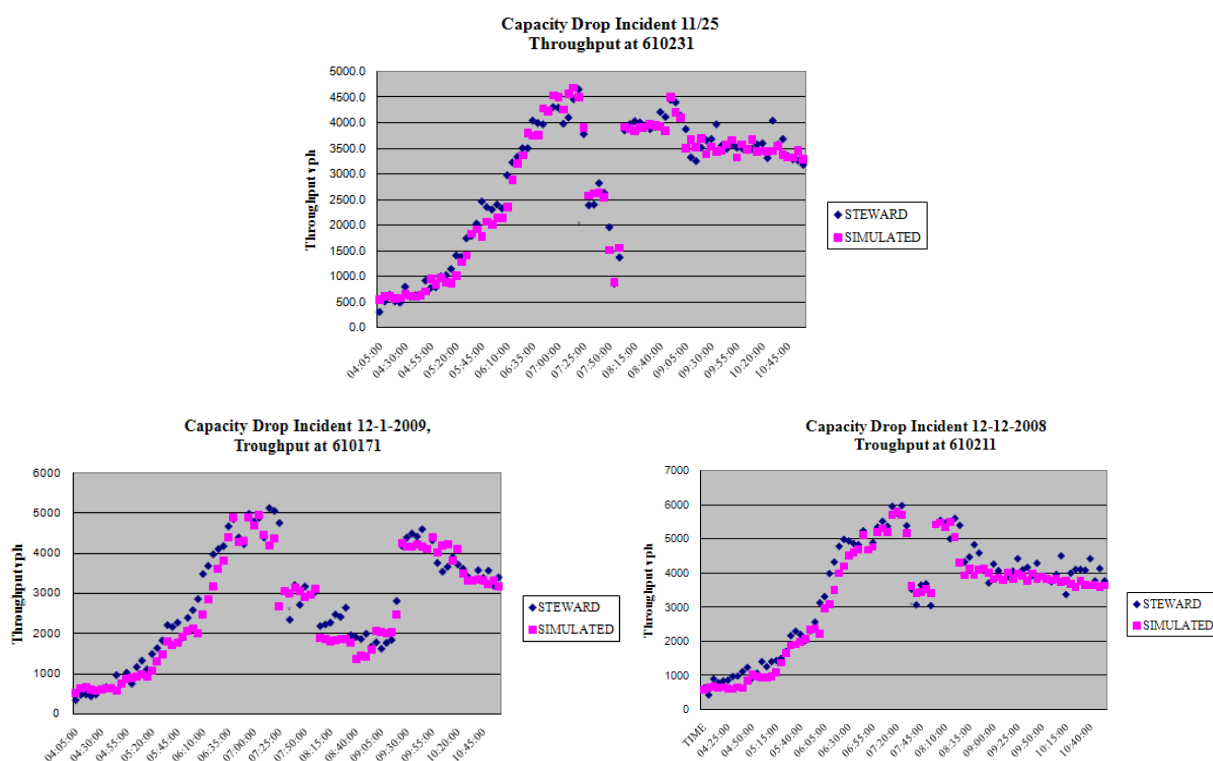
Figure 4-5 Comparison of Capacity Drop based on Detector Measurements and Simulation
