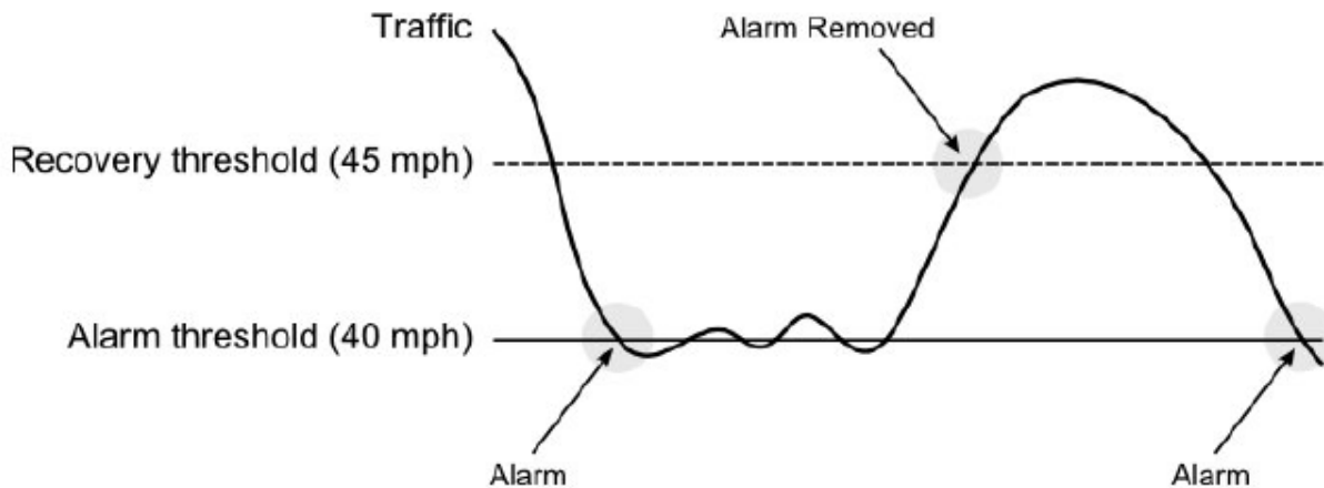
Figure 6-12 TSS Alarm Enhancement in SunGuide R5.0.3
