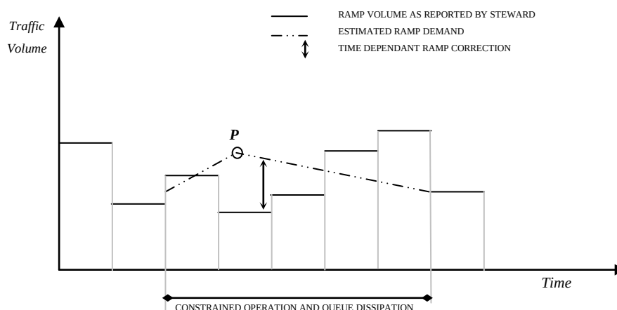
Figure 3-2 Ramp Volume Correction
