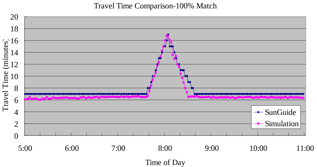
Figure 6-7 Travel Time Comparison for Incident Conditions, 100% Match
