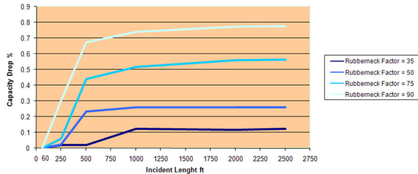
Figure 4-2 Effects of Incident Length and Rubberneck Factor on Capacity Drop
