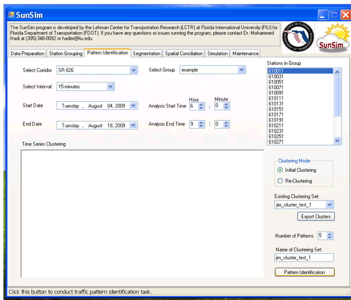
Figure B-6: User Interface for Pattern Identification
