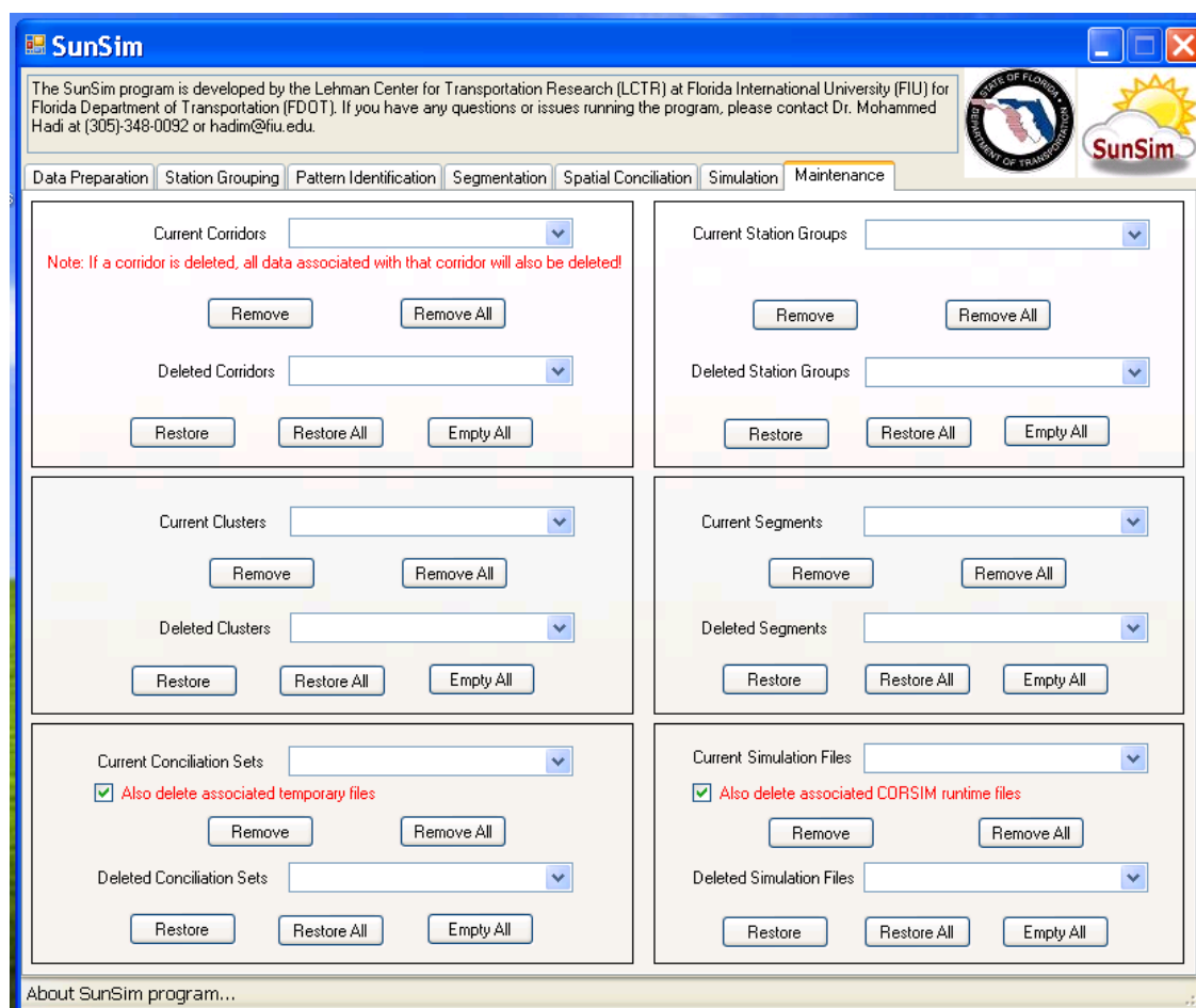
Figure B-15: User Interface for the Maintenance Module
