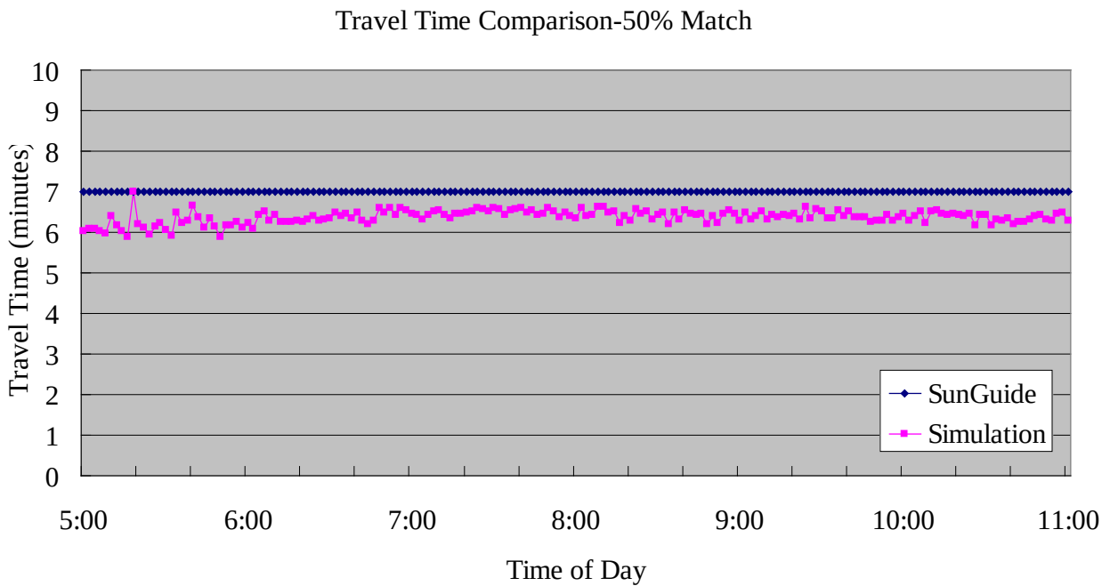
Figure 6-3 Travel Time Comparison for No-incident Conditions, 50% Match
