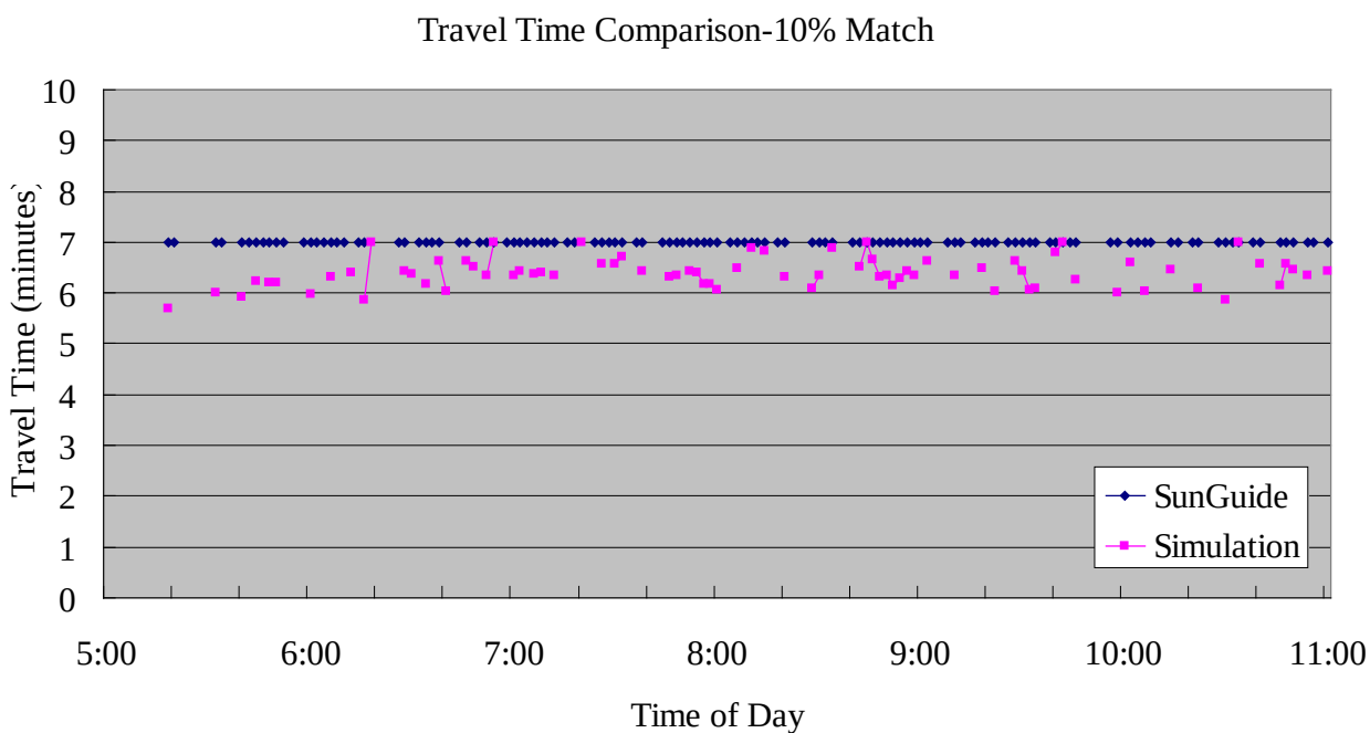
Figure 6-5 Travel Time Comparison for No-incident Conditions, 10% Match
