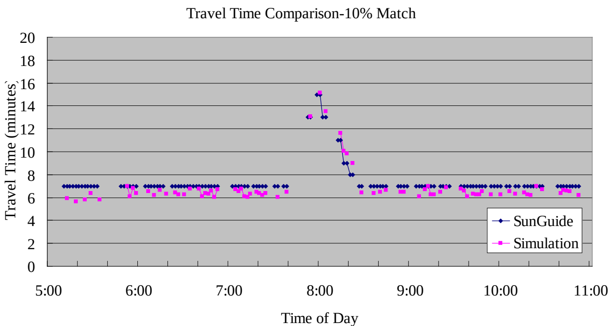
Figure 6-10 Travel Time Comparison for Incident Conditions, 10% Match
