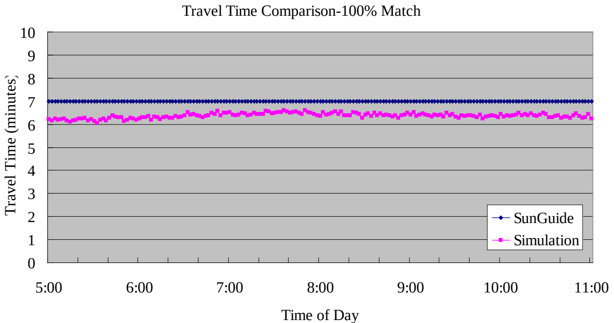
Figure 6-2 Travel Time Comparison for No-incident Conditions, 100% Match
