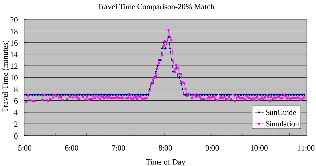
Figure 6-9 Travel Time Comparison for Incident Conditions, 20% Match
