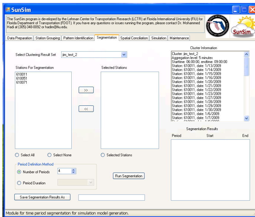
Figure B-10: User Interface for Data Segmentation
