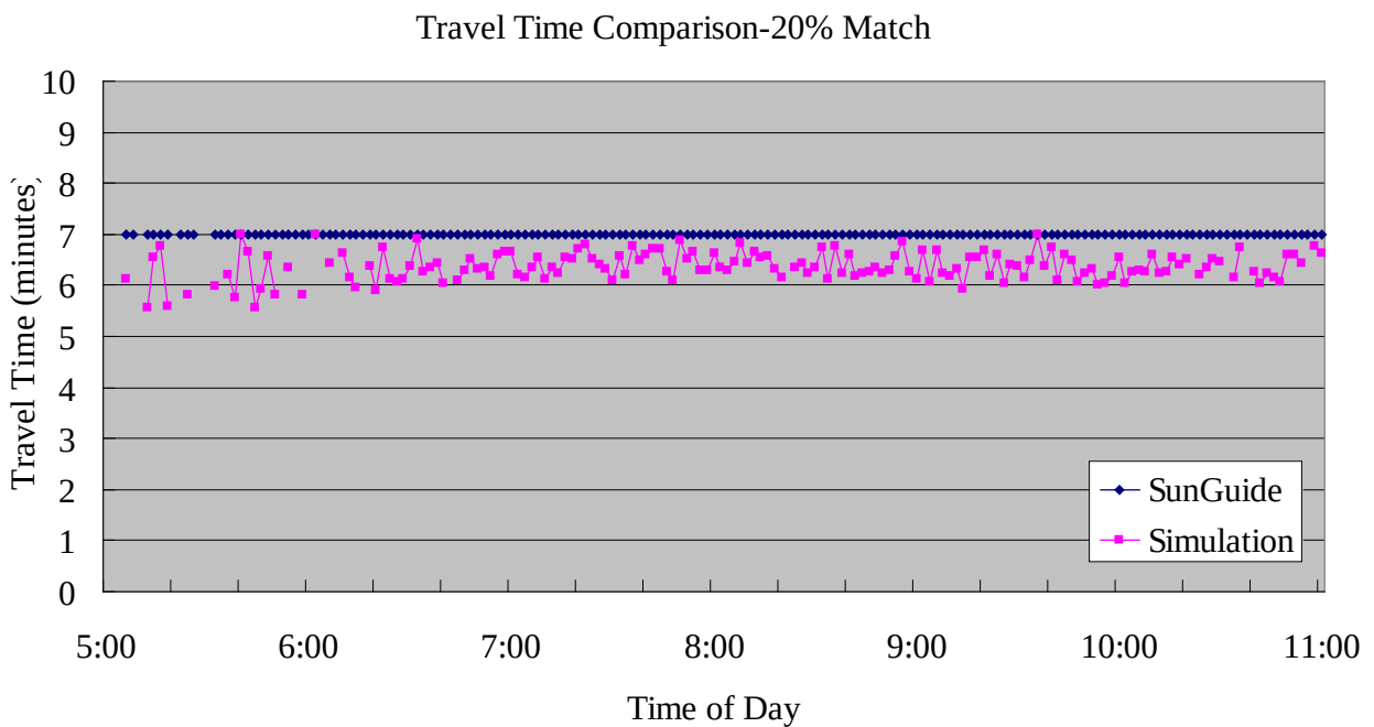
Figure 6-4 Travel Time Comparison for No-incident Conditions, 20% Match
