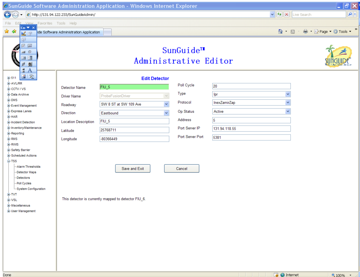
Figure D-11: SunGuide Interface for Coding AVI/LPR Detectors
