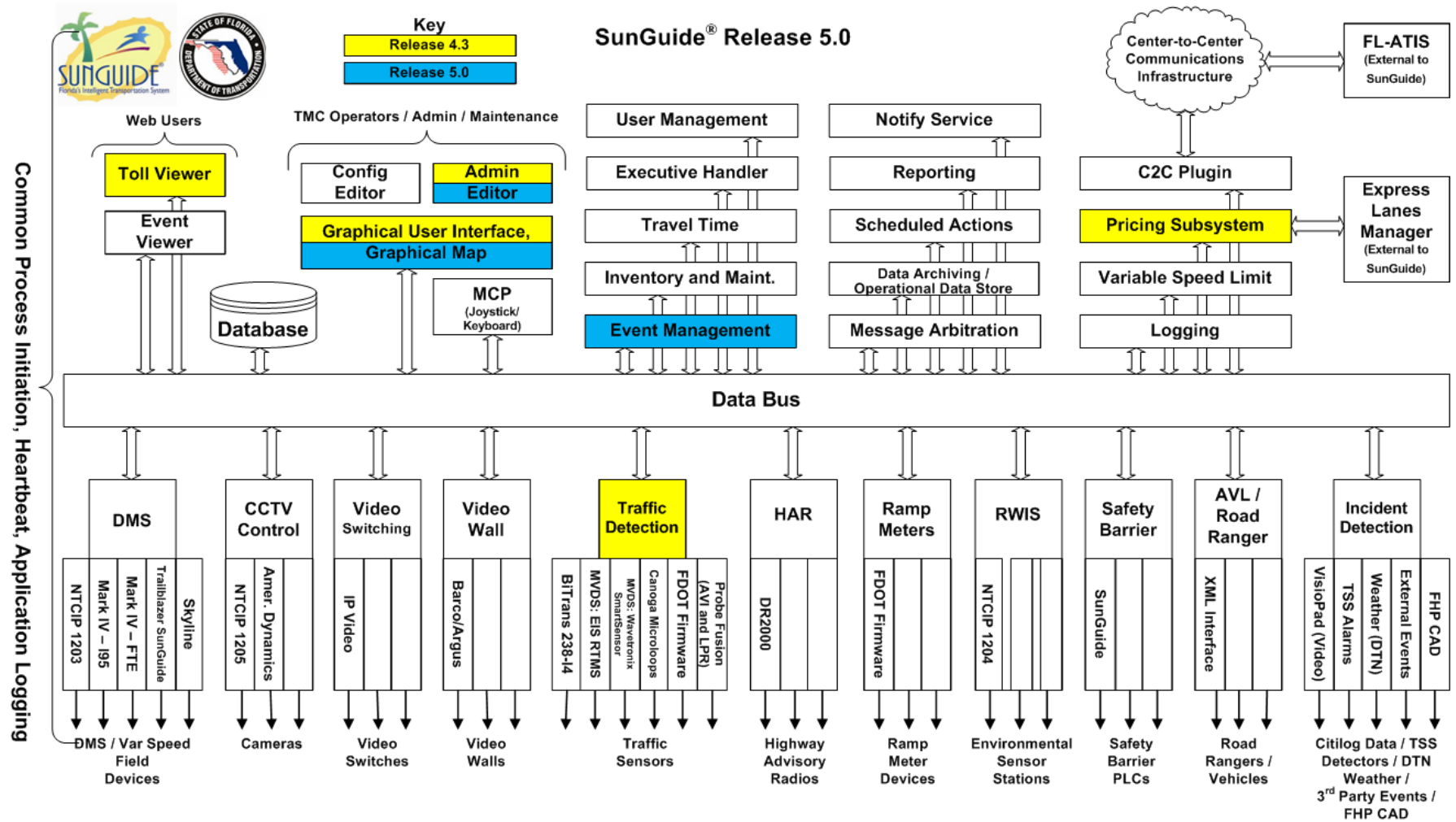
Figure 2-5 GraphicalView of Version 5.0 of the SunGuide Software
