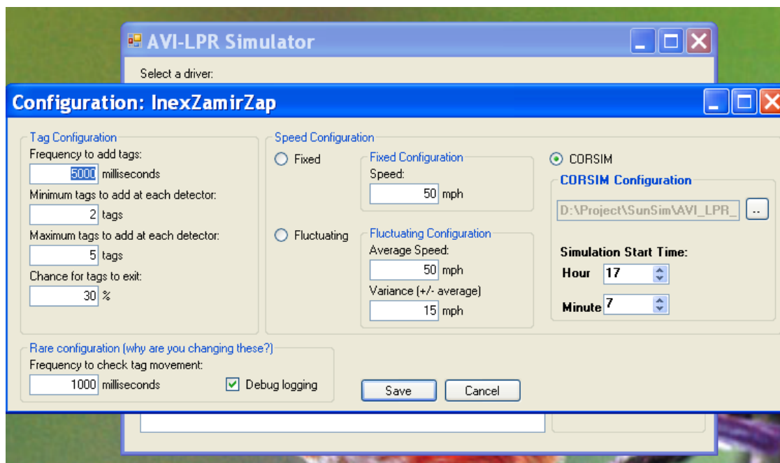
Figure D-14: AVI/LPR Simulator Interface for Configuration Settings
