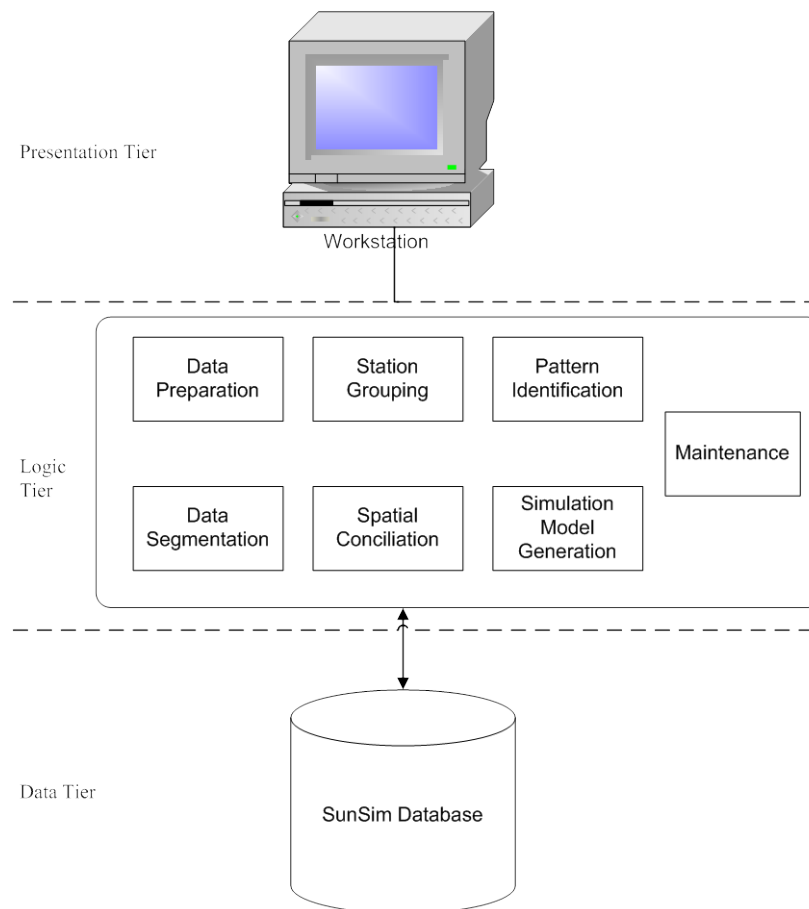
Figure 5-2 SunSim Core Simulation Development System Architecture
