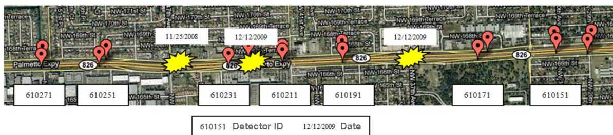
Figure 4-3 Locations of the Selected Incidents and Detector Stations
