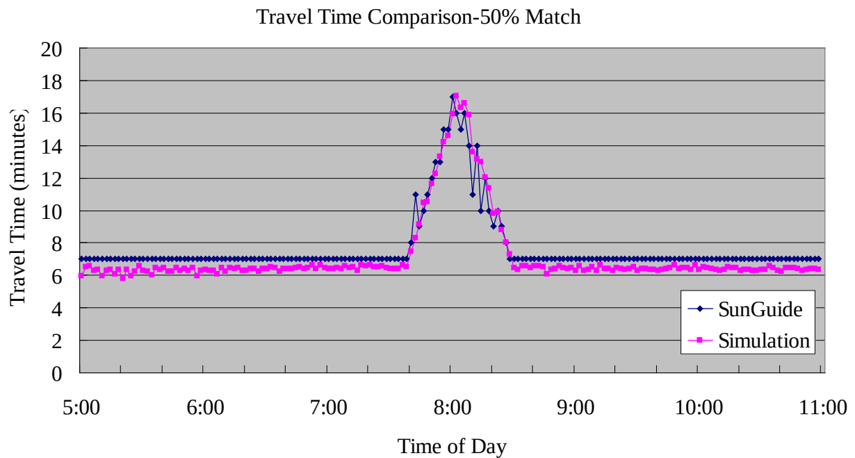
Figure 6-8 Travel Time Comparison for Incident Conditions, 50% Match
