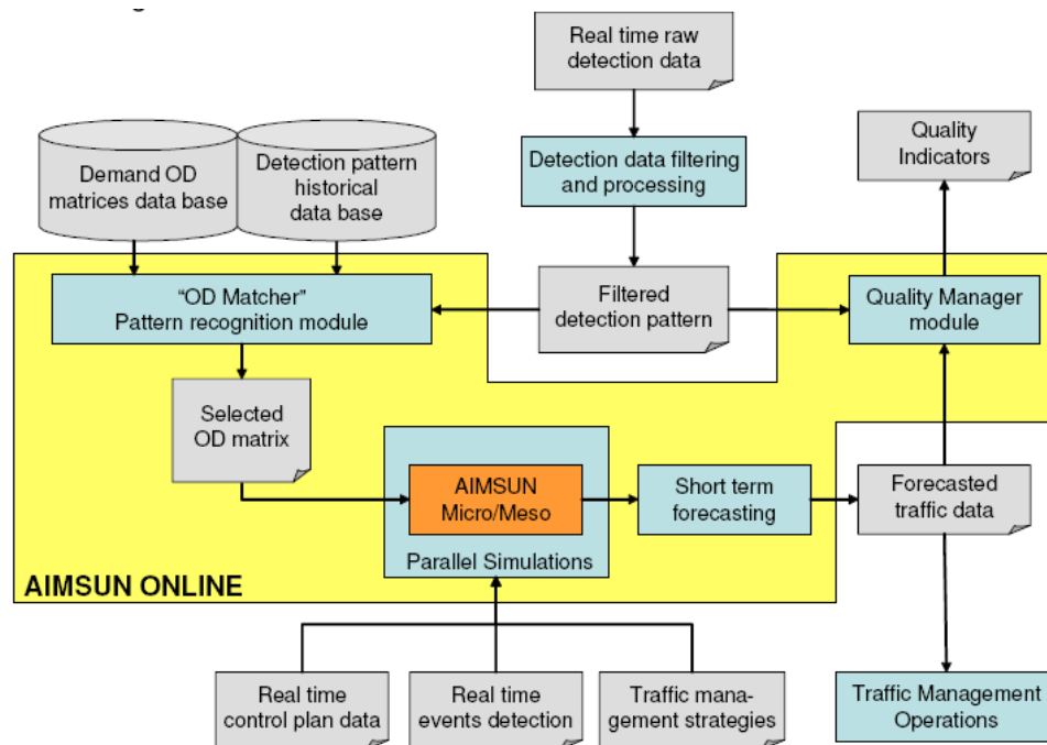
Figure 2-4 Architecture of Online Version of AIMSUN
