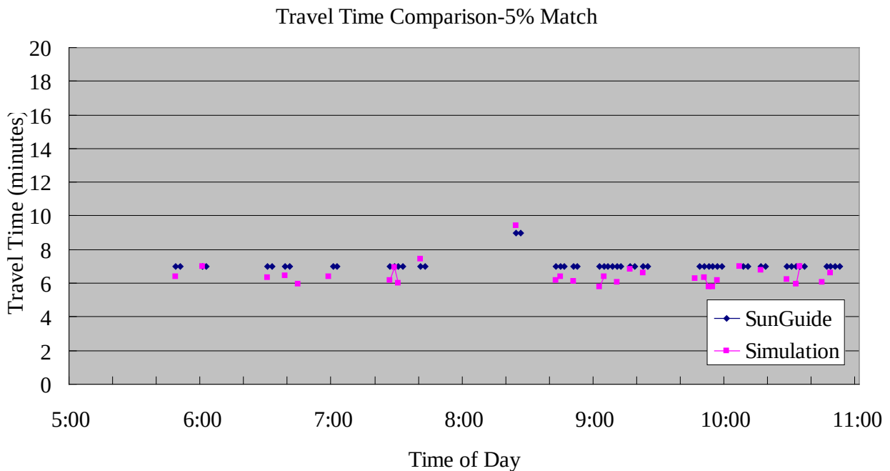
Figure 6-11 Travel Time Comparison for Incident Conditions, 5% Match
