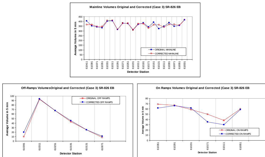
Figure 3-7 Mainline and Ramp Volume Corrections for Case 3
