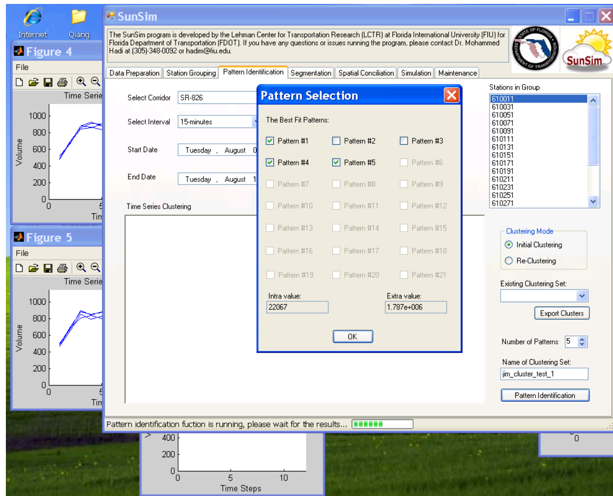
Figure B-7: User Interface for Data Clustering Results
