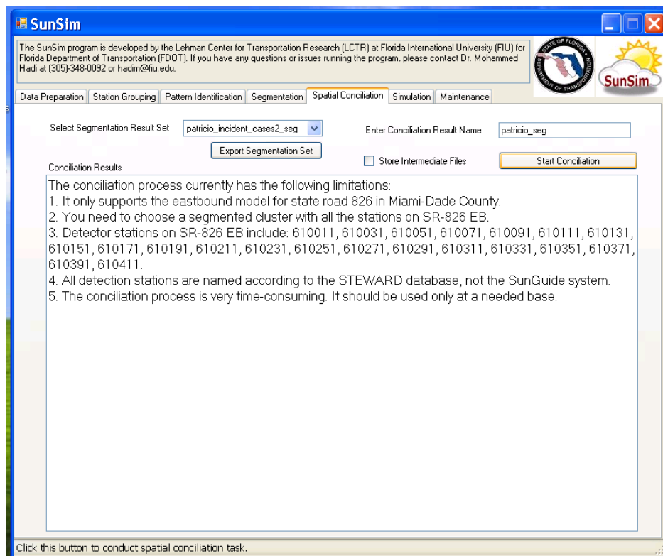
Figure B-12: User Interface for Spatial Conciliation
