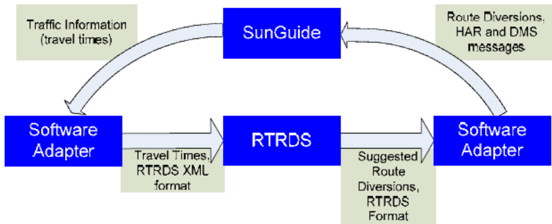
Figure 2-3 Proposed RTRDS Processes (Source: Aved et al., 2007)
