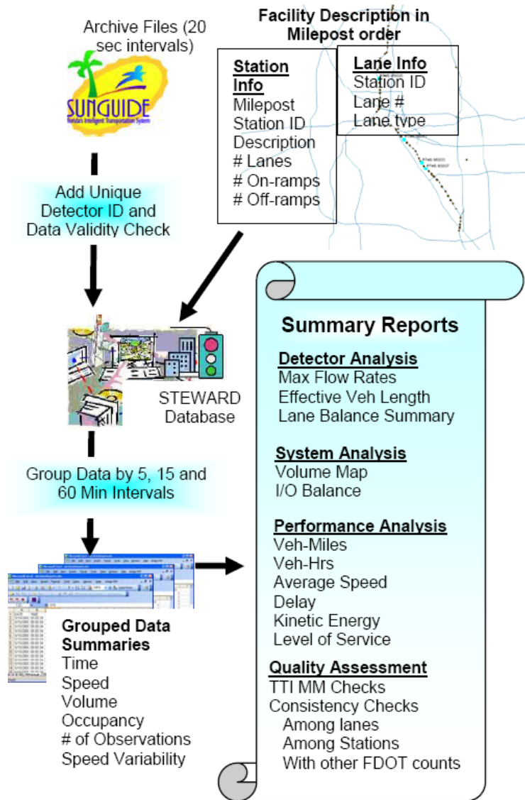
Figure 2-6 STEWARD Archives TSS Flow Chart
