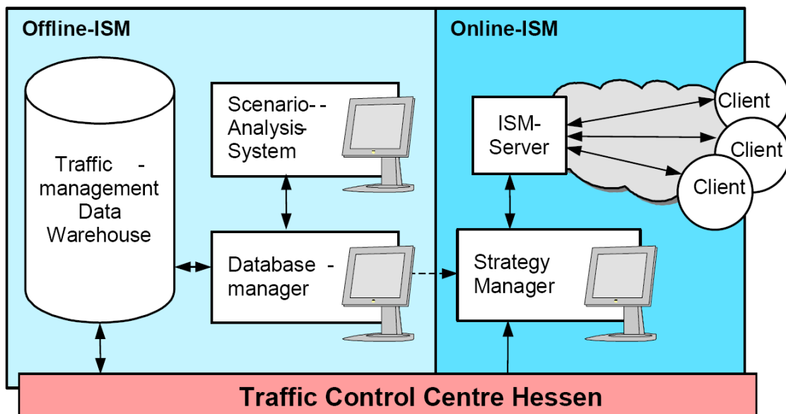
Figure 2-2 Conceptual Architecture of ISM
