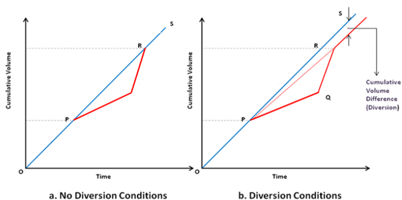
Figure 4-1 Estimation of the Difference between the Demands during Average and Incident Days
