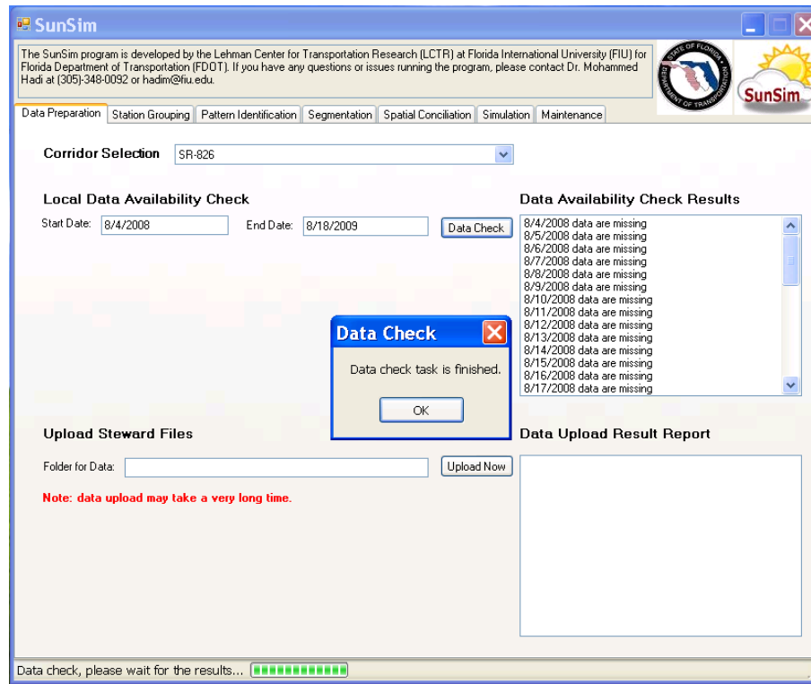
Figure B-2: User Interface for Data Availability Check Results
