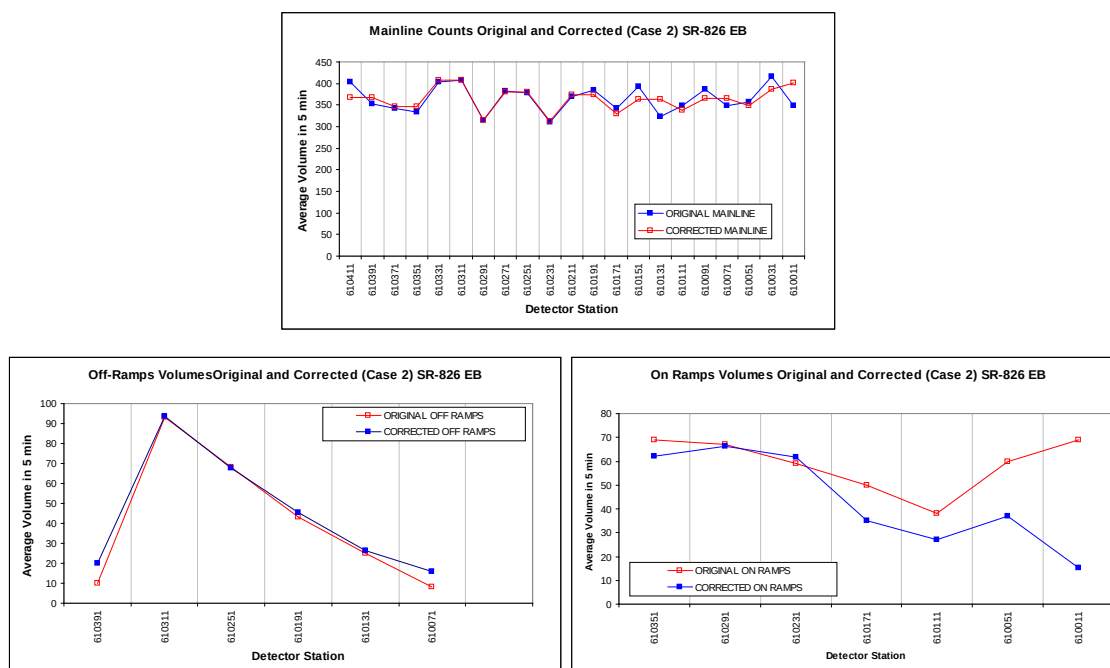
Figure 3-6 Mainline and Ramp Volume Corrections for Case 2
