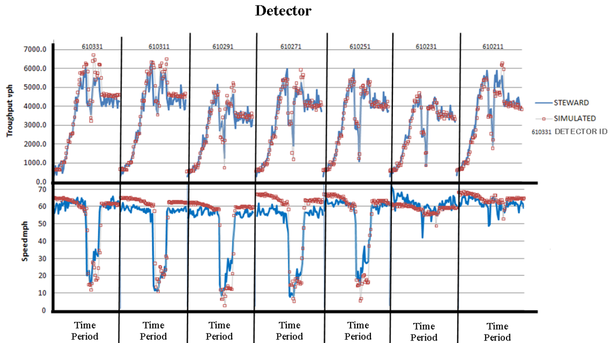
Figure 4-6 Simulation and Real-World Speed and Throughput Measurements for Incident 1
