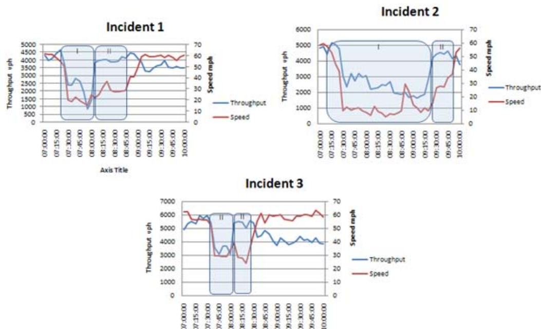
Figure 4-4 Throughput and Speed Measurements for the Three Investigated Incidents
