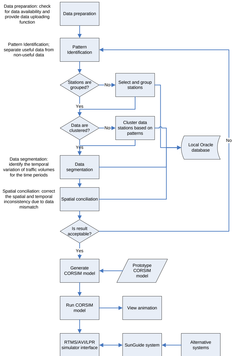
Figure 5-4 SunSim System Flow Chart
