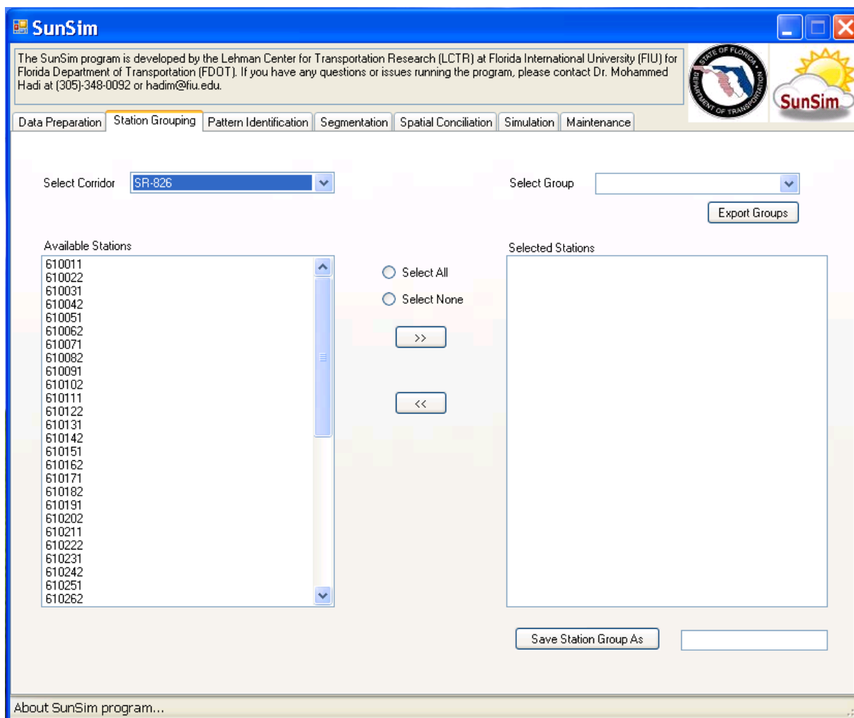
Figure B.4: User Interface for Detection Station Selection (Data Selection Tab)
