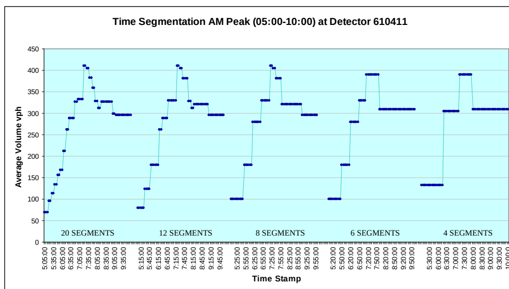
Figure 3-4 Time Segmentation based on Volumes
