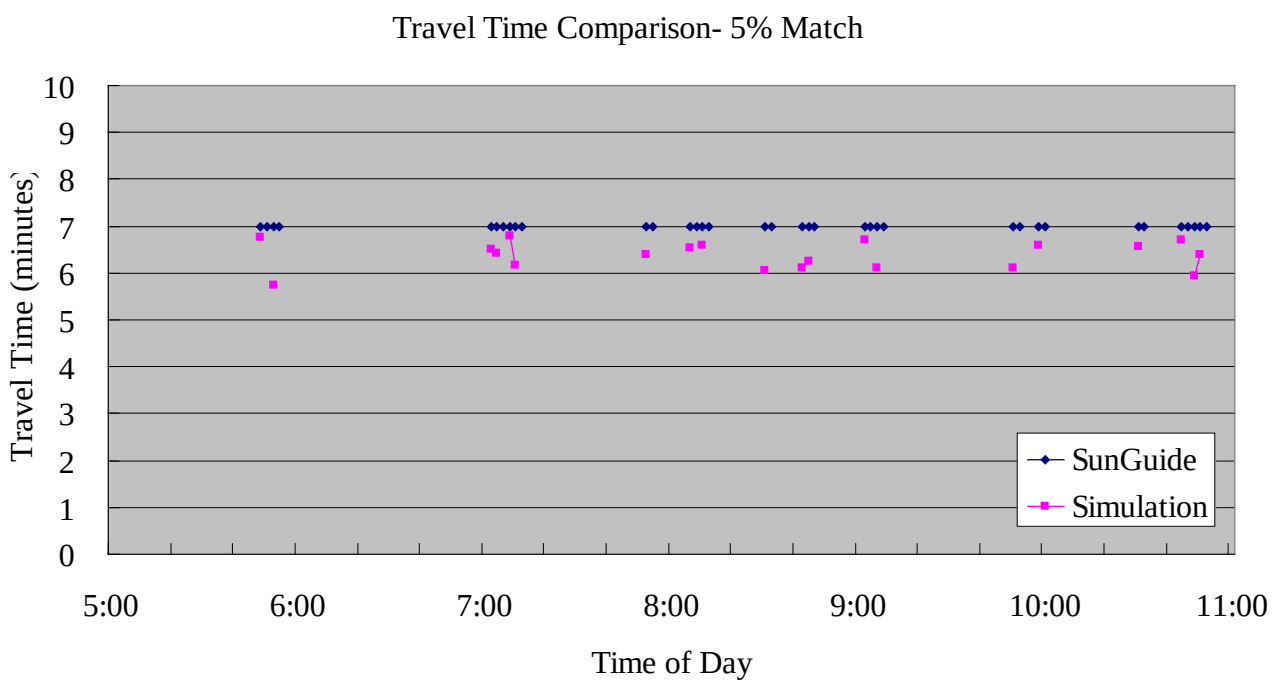
Figure 6-6 Travel Time Comparison for No-incident Conditions, 5% Match
