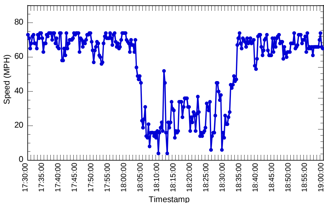
FIGURE 5-4 Speed Data for the Detector in the Opposite Direction
