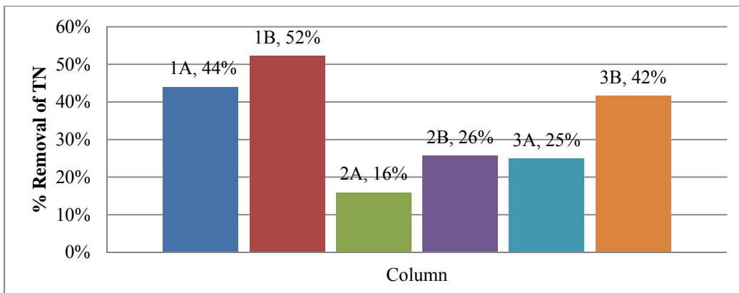
Figure A-2 % Average Removal of TN for each Column – 24 Hour Event; Average EBCT of 234.8 minutes (9/24/2013 – 11/18/2013)
