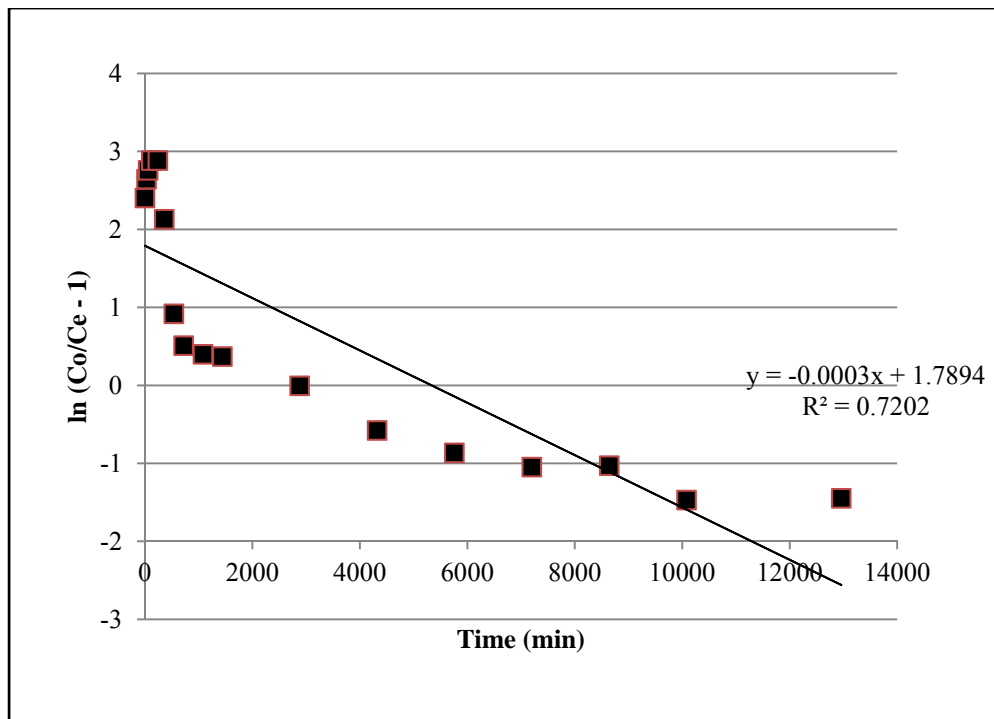
Figure 5-4 Plot of \ln(C_o/C_e - 1) vs. time for BAM Nutrient mix 3-2 using spiked phosphorus pond water with an initial PO_4 concentration of 1.0 \text{ mg}\cdot\text{mL}^{-1} and flow rate of 0.167 \text{ l}\cdot\text{hr}^{-1} used to derive values for the Thomas Model
