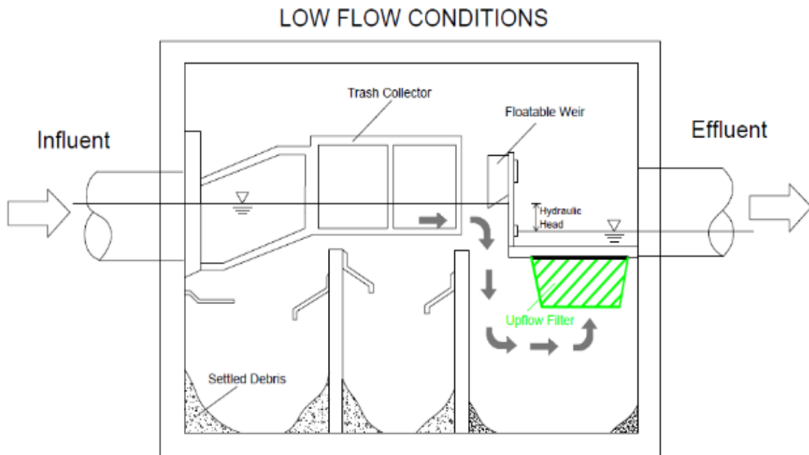
Figure 6-7 Diagram of Up-flow On-Line Sorption Filter during Low Flow
