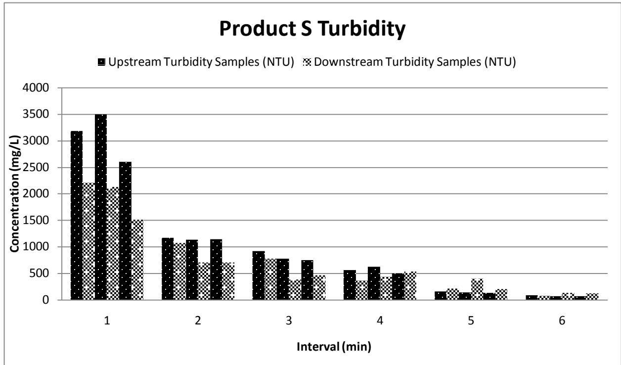
Figure 43: Sample water turbidity for 3 rainfall events on Product S over time
