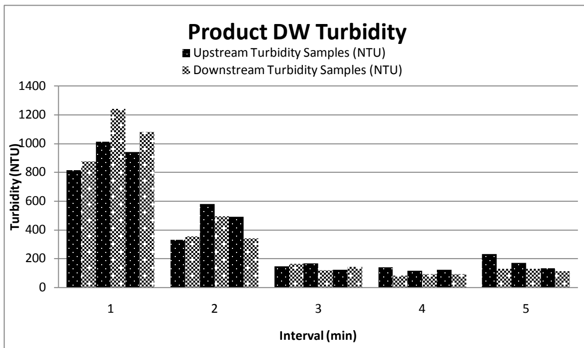
Figure 88: Sample water turbidity for 3 rainfall events on Product DW over time
