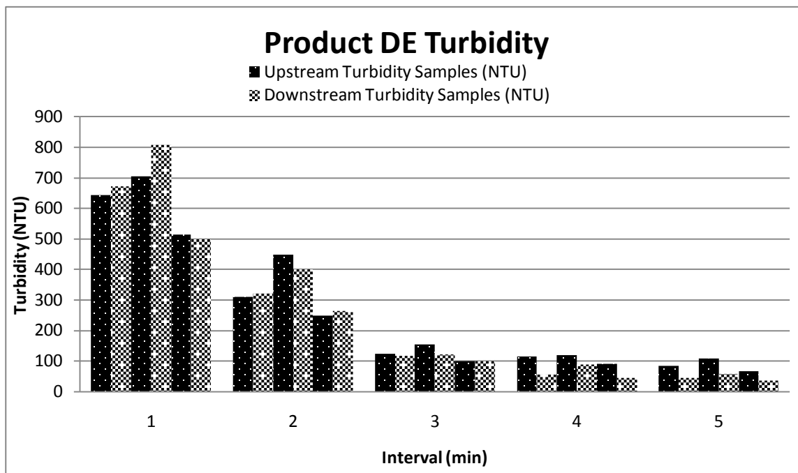
Figure 89: Sample water turbidity for 3 rainfall events on Product DE over time
