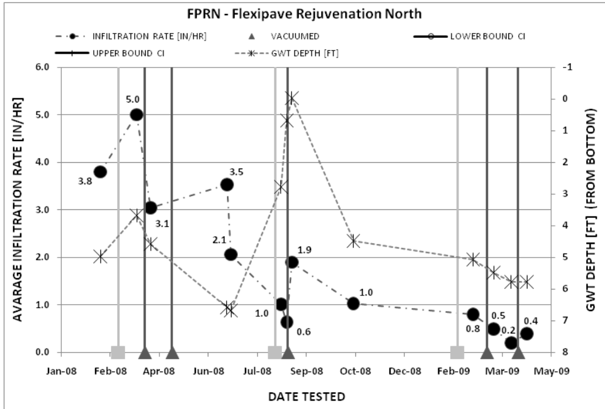
Figure 31: Infiltration Rate results (ERIK) Rejuvenation section's North infiltrmeter
