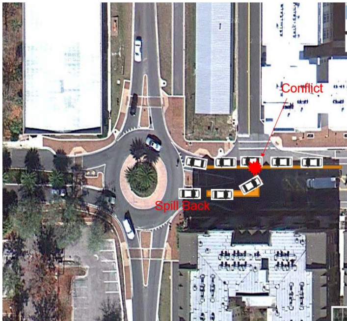
Figure 65. Conflict and Spillback associated with Left-turn Access to Driveway
