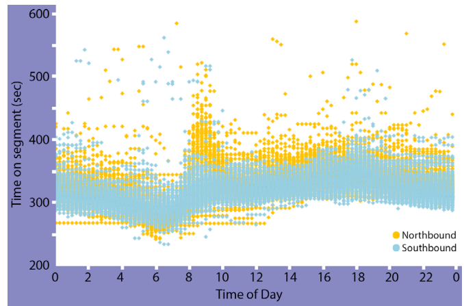
Travel time along an arterial road segment in Jacksonville, Florida. Note the difference between northbound and southbound travel times during peak morning hours.
