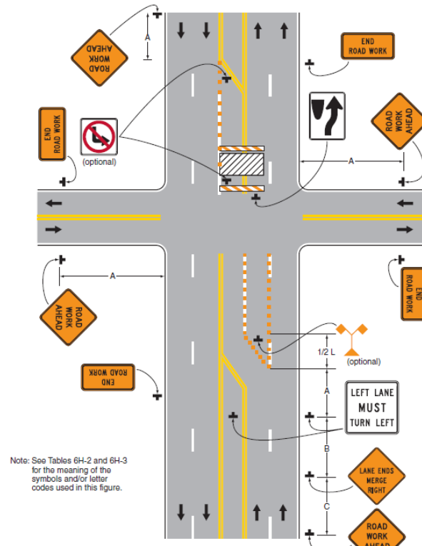
Figure 2.5 Multiple Lane Closures at an Intersection
