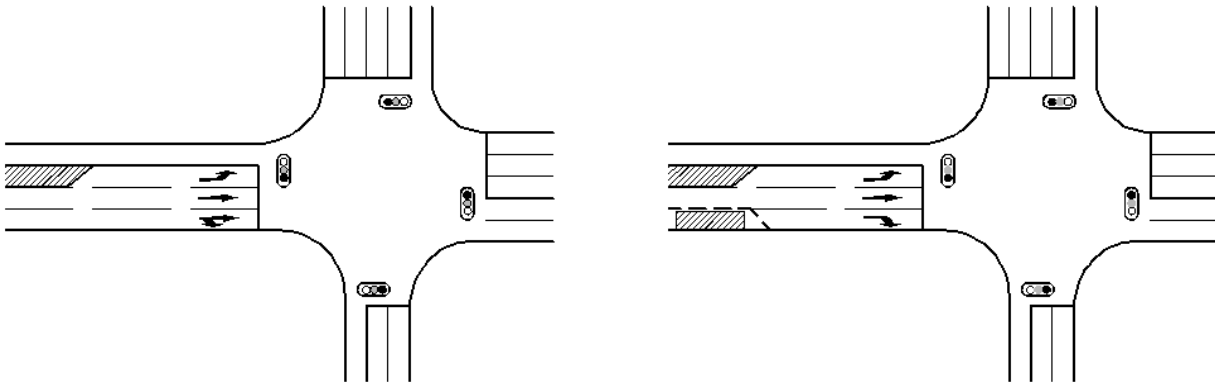
Figure 3.5 Approach Configuration before and after the Lane Closure
