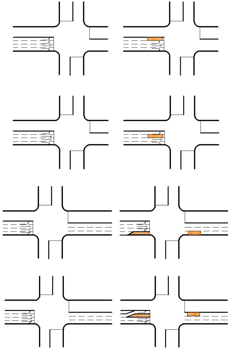
Figure 3.11 Lane Closures at the Stop Bar that Only Cause Reduction in the Number of Lanes
