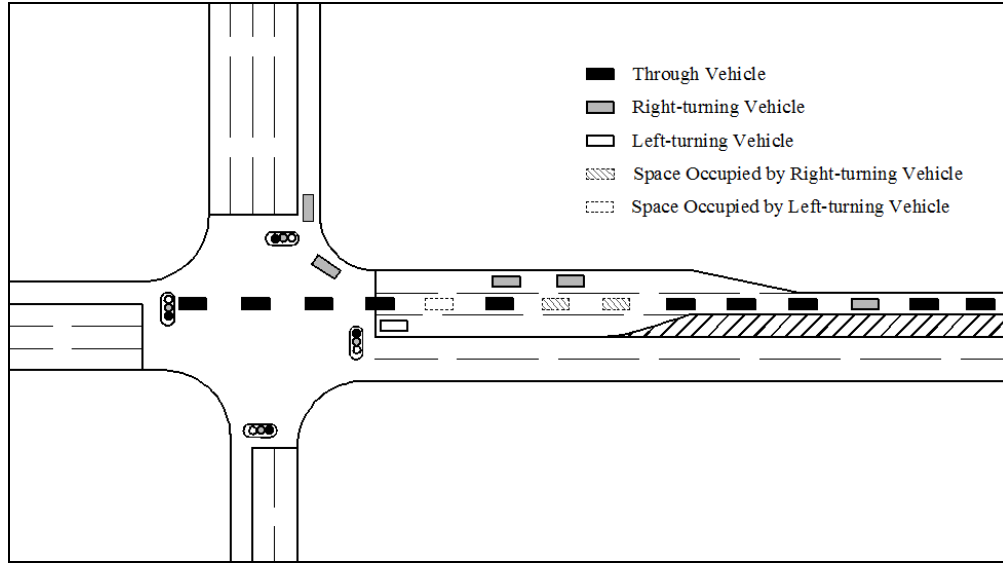
Figure 3.4 Lane Utilization during Queue Discharge (Li and Elefteriadou, 2012)
