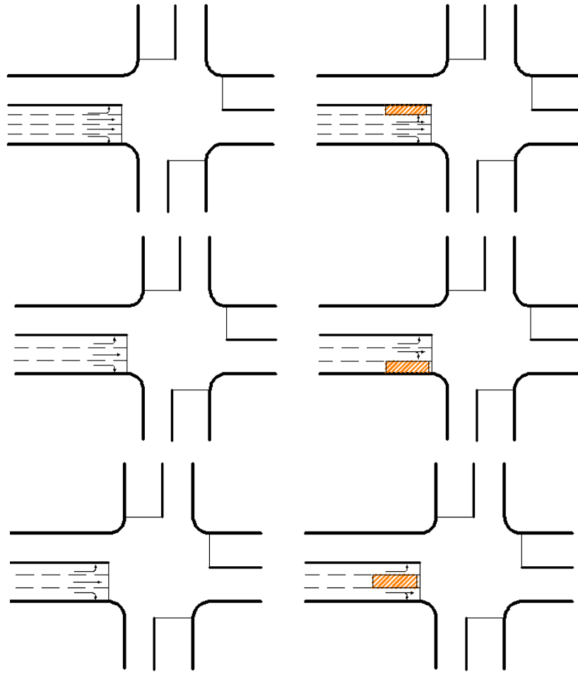
Figure 2.11 Lane Closure Results in the Creation of a Shared Lane
