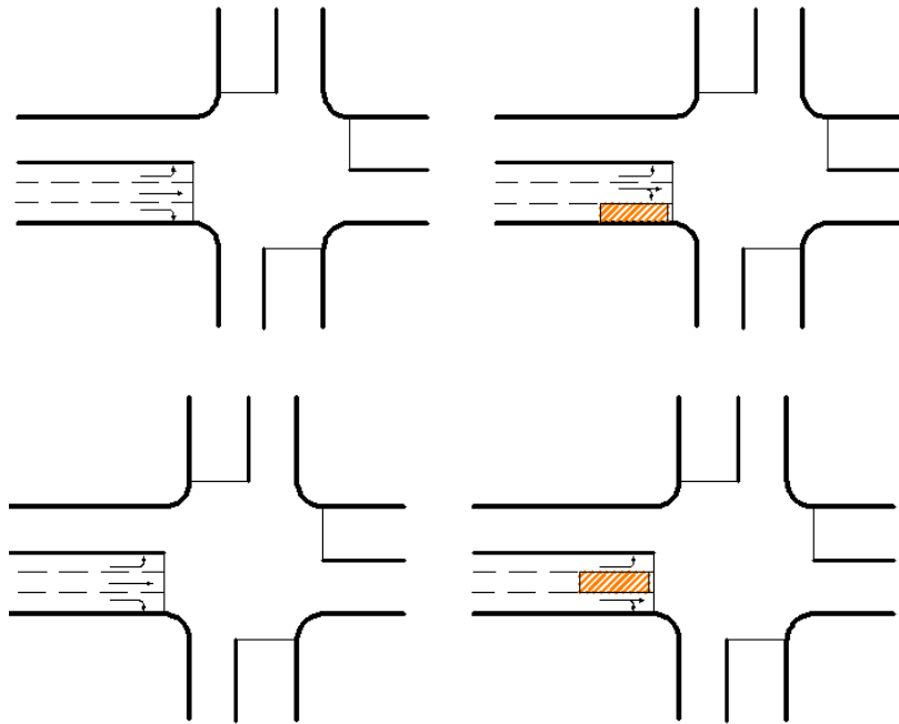
a) Turning Vehicles Have to Share A Lane with Through Vehicles
