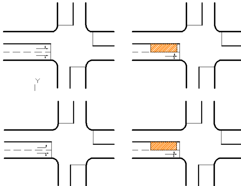
Figure 2.13 Lane Closure Results in the Creation of a One-lane Approach
