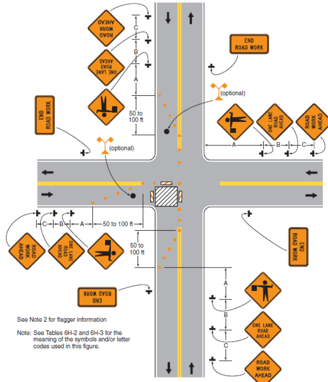
Figure 2.7 Closure at the Side of an Intersection
