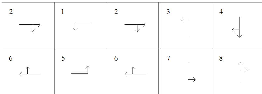
Figure 3.7 Proposed Phasing Diagram of the Study Intersection
