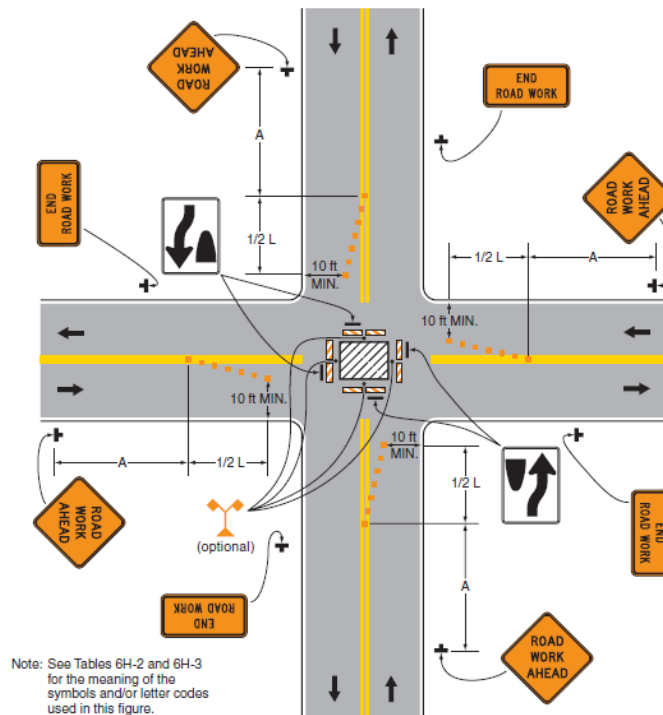
Figure 2.6 Closure in the Center of an Intersection
