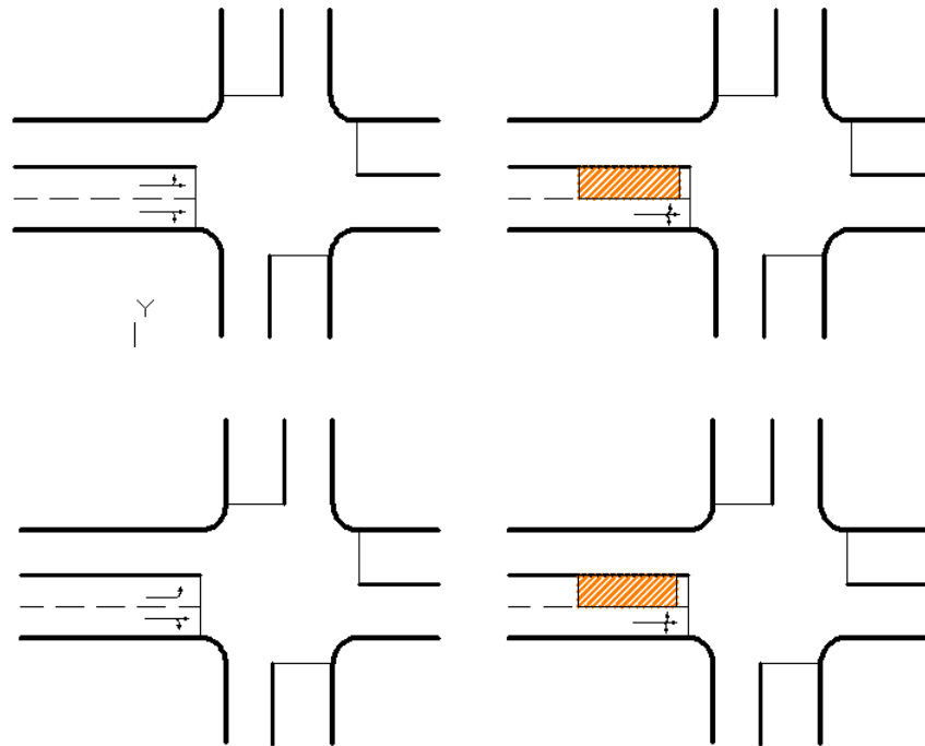
c) Lane Closure for a Two Lane Approach
