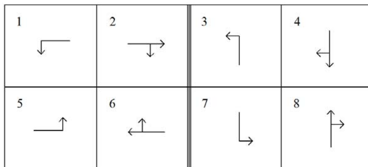
Figure 3.6 Phasing Diagram of the Study Intersection
