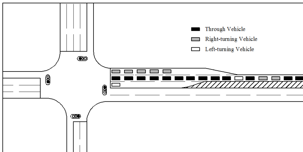
Figure 3.3 Queuing during the Red Interval (Li and Elefteriadou, 2012)
