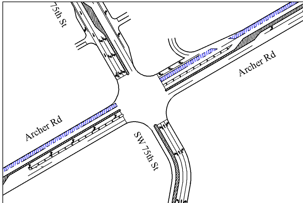
Figure 5.3 Sketch of the Lane Closure in Westbound for the Intersection of Archer Rd and SW 75 th St.
