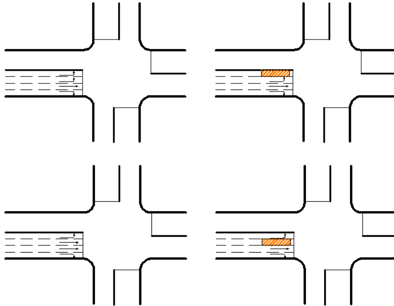
Figure 2.14 Lane Closure on the Near Side of the Intersection
