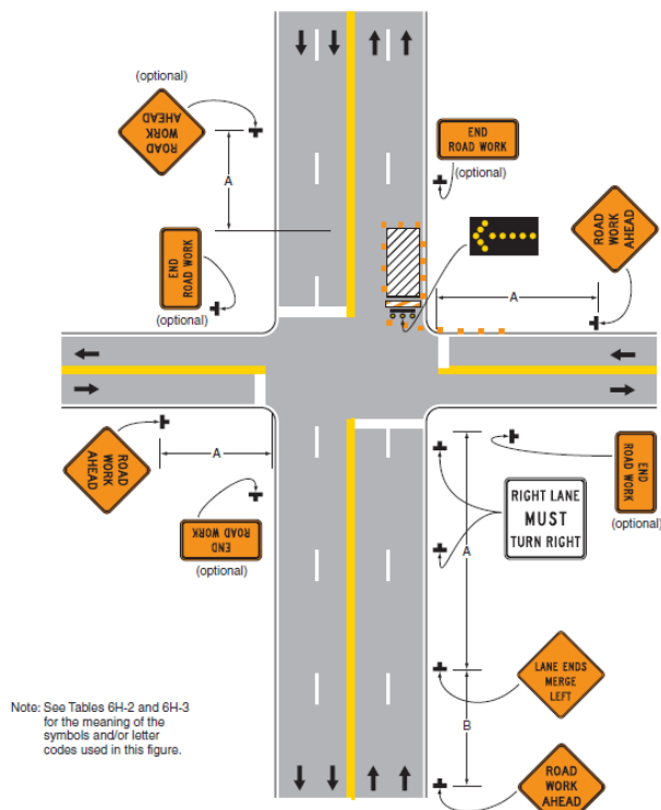
Figure 2.2 Right-Hand Lane Closure on the Far Side of an Intersection
