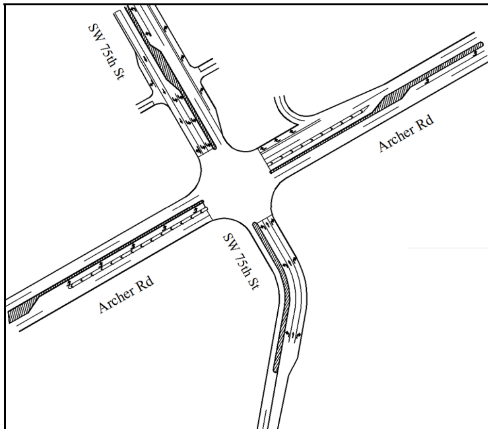
Figure 4.1 Sketch of the Intersection at Archer Rd and SW 75 th St
