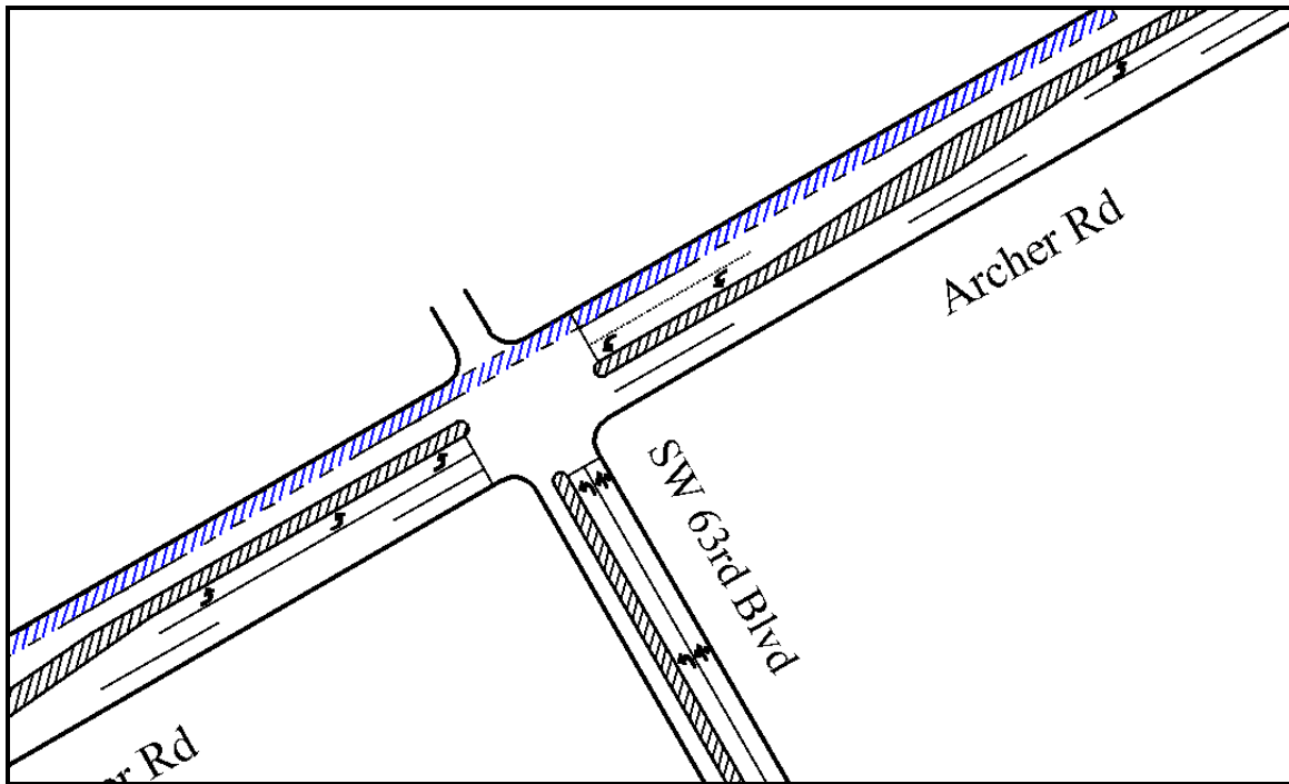
Figure 4.5 Sketch of the Lane Closure in Westbound Archer Rd at the Intersection of Archer Rd and SW 63 rd Blvd
