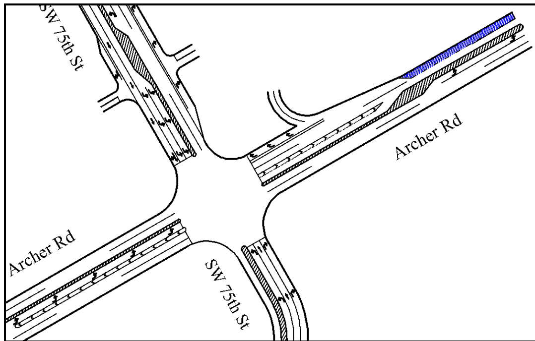
Figure 5.1 Sketch of the Lane Closure in Westbound Archer Rd before the Intersection of Archer Rd and SW 75 th St.
