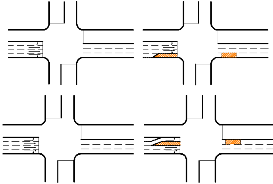
Figure 2.15 Lane Closure on the Far Side of the Intersection
