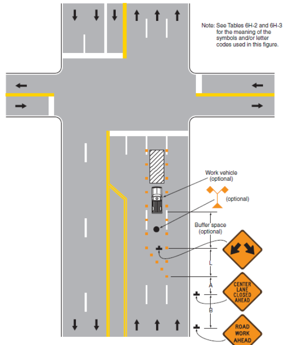
Figure 2.1 Lane Closure on the Near Side of an Intersection
