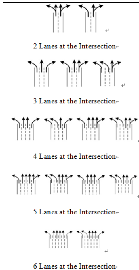
Figure 2.8 Lane Channelization Configurations (Heaslip et al., 2011)
