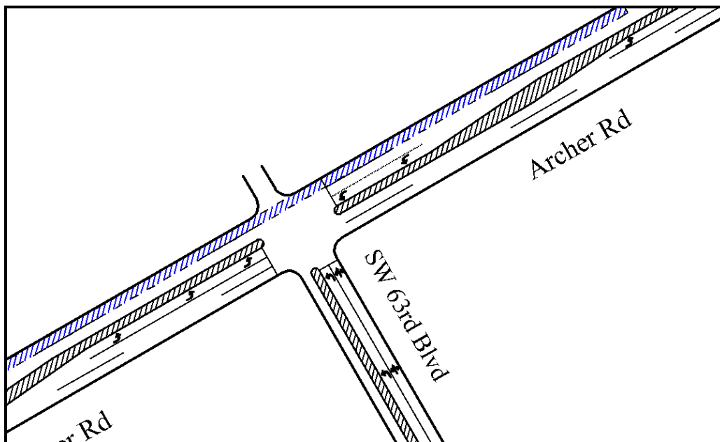
Figure 5.4 Sketch of the Lane Closure in Westbound for the Intersection of Archer Rd and SW 63 rd Blvd
