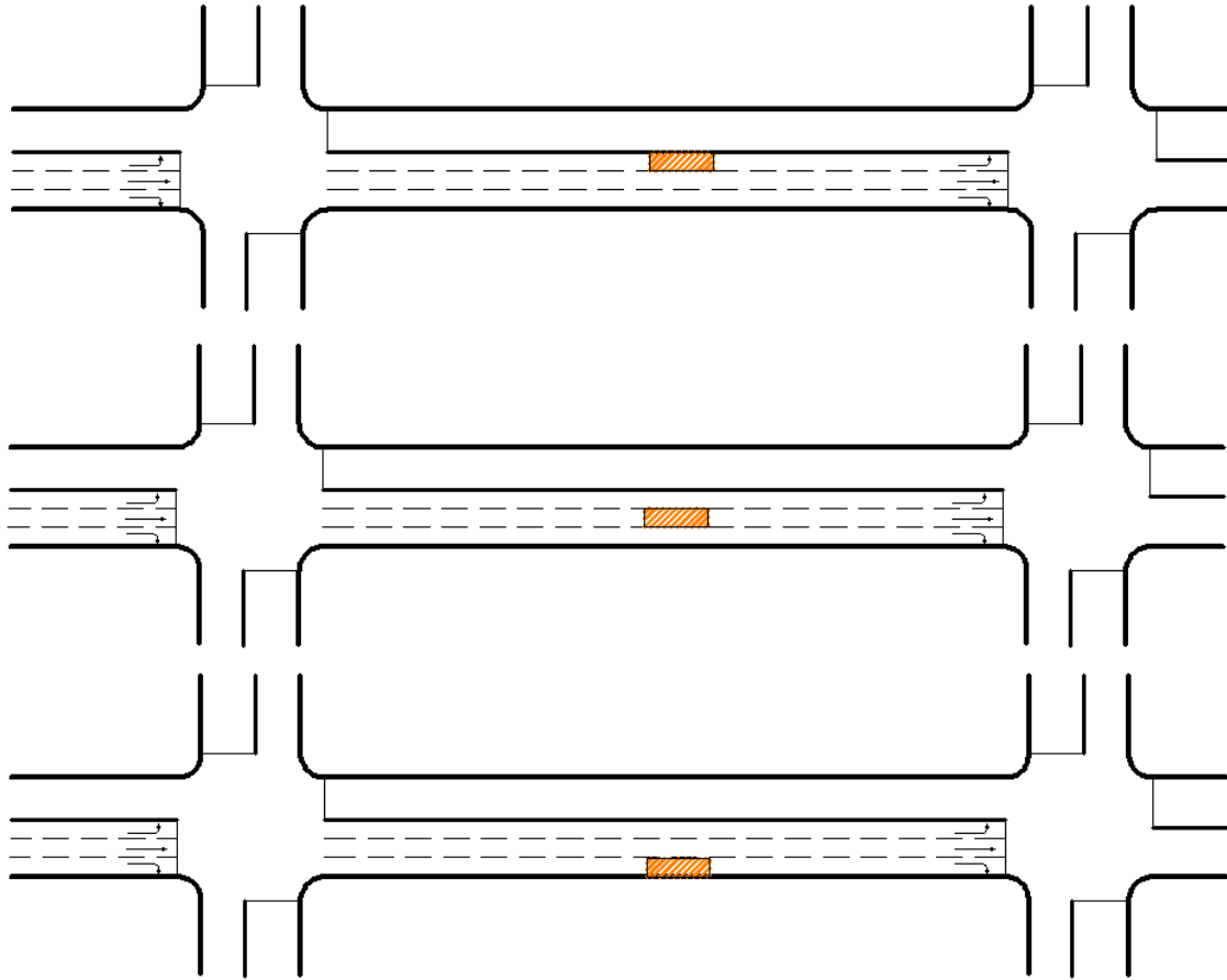
Figure 3.12 Configurations for the Case of Lane Closure between Intersections
