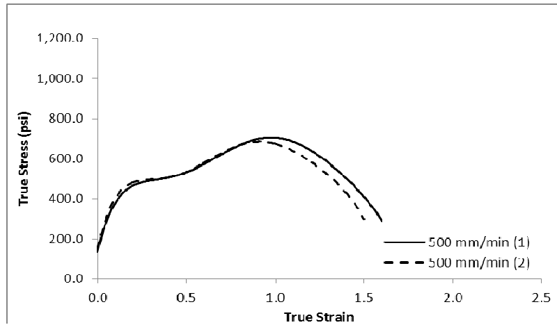
Figure 28 Binder-G, RTFO-plus-PAV, true stress-true strain
