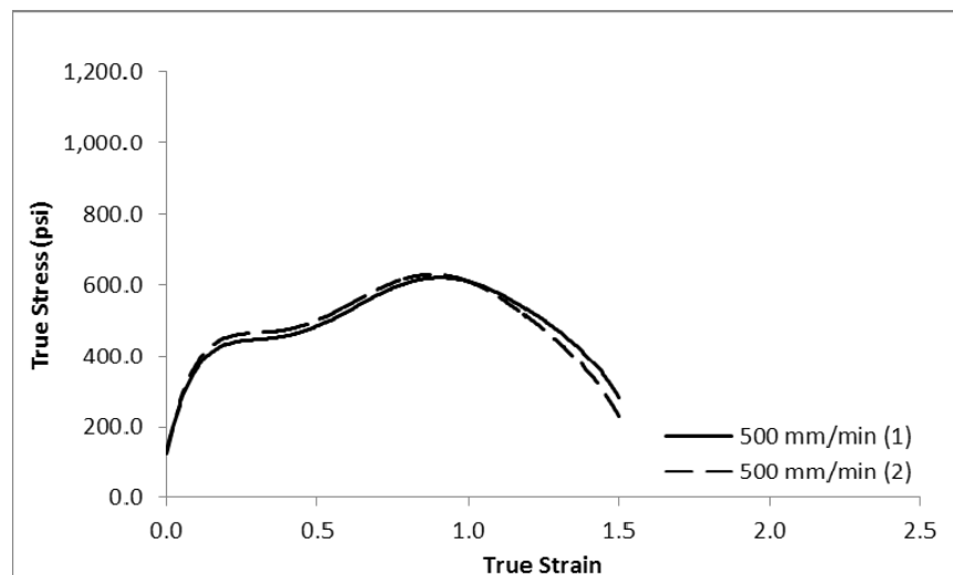
Figure 27 Binder-B, RTFO-plus-PAV, true stress-true strain
