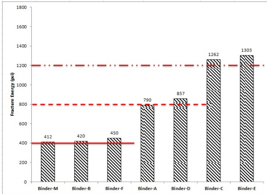
Figure 23 Average fracture energy densities for all PAV residue binders
