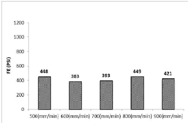
Figure 12 Binder-B, fracture energy vs. loading rates
