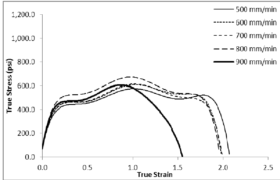
Figure 9 Binder-A, true stress-true strain
