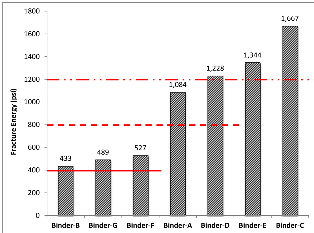
Figure 32 Fracture energy densities for all RTFO-plus-PAV Specimens
