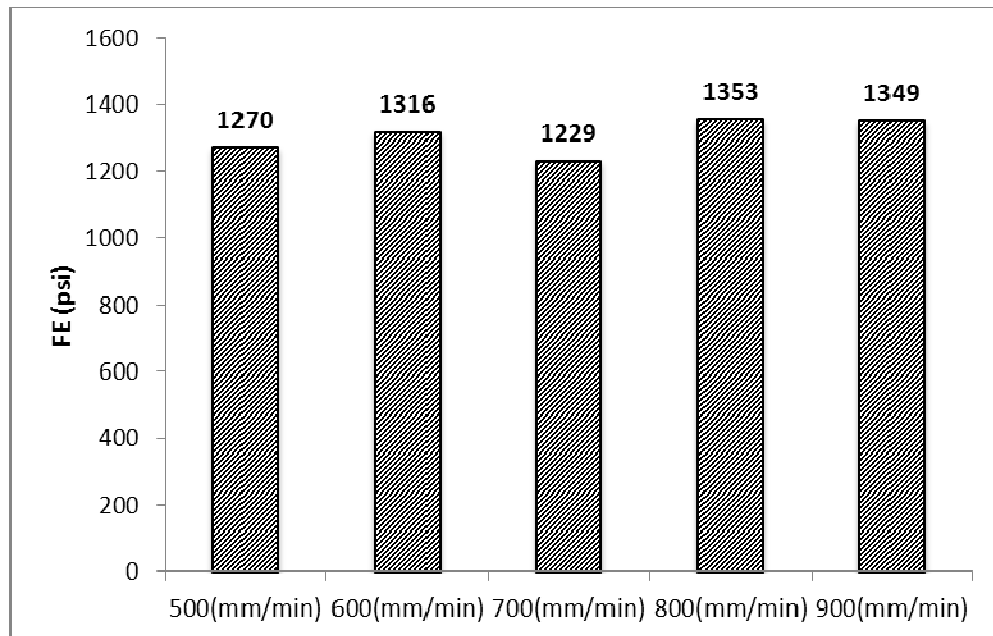
Figure 16 Binder-E, fracture energy vs. loading rates
