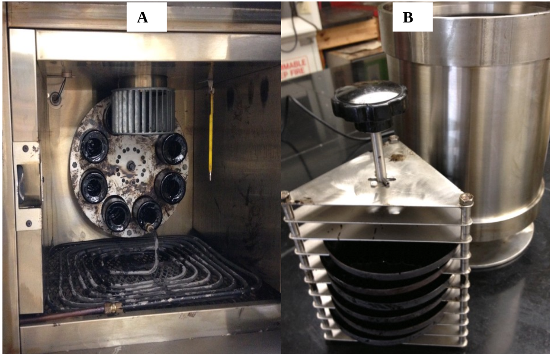
Figure 6 Performing RTFO test (A) and PAV test (B)
