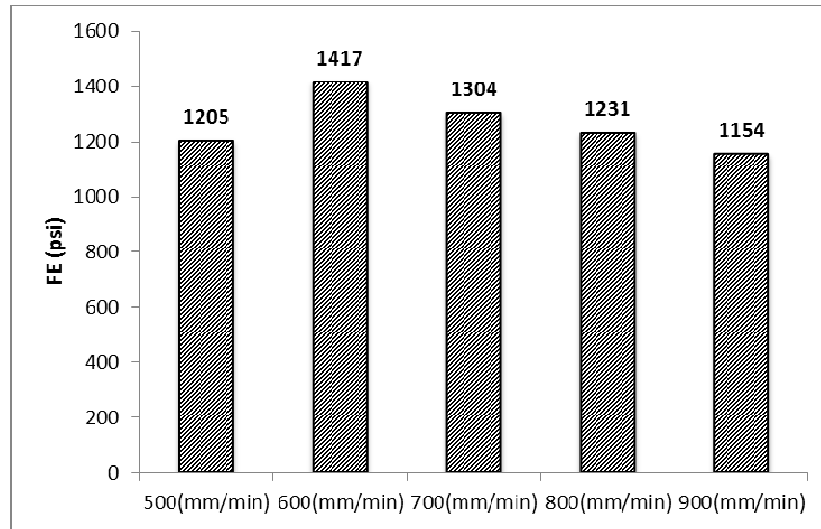
Figure 10 Binder-C, fracture energy vs. loading rates
