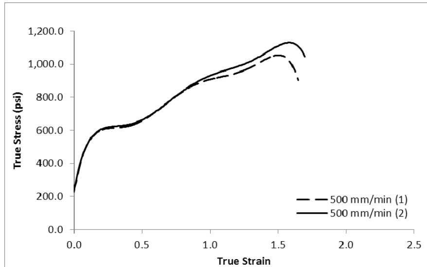
Figure 31 Binder-D, RTFO-plus-PAV, true stress-true strain
