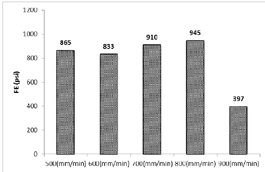
Figure 8 Binder-A, fracture energy vs. loading rates
