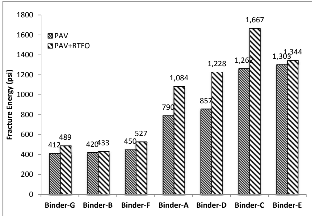
Figure 33 Comparison of fracture energy between PAV residue only and RTFO-plus-PAV specimens
