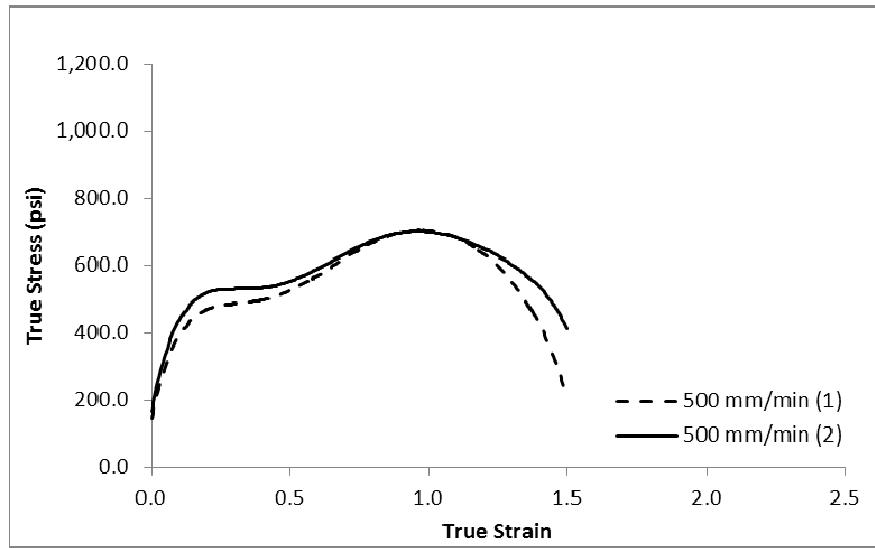
Figure 30 Binder-F, RTFO-plus-PAV, true stress-true strain
