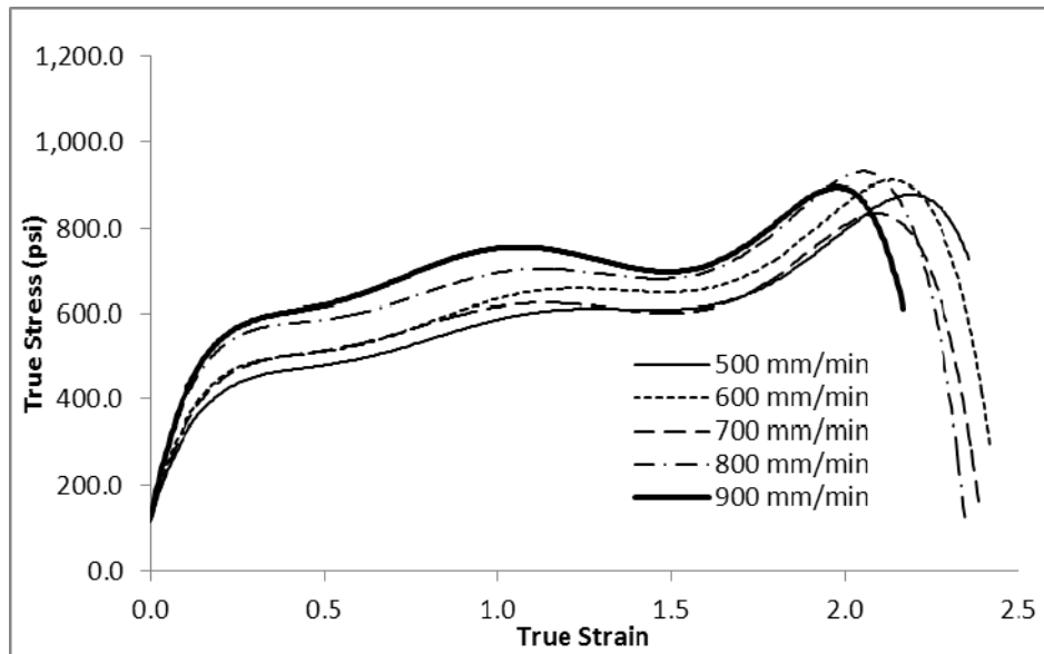
Figure 17 Binder-E, true stress-true strain
