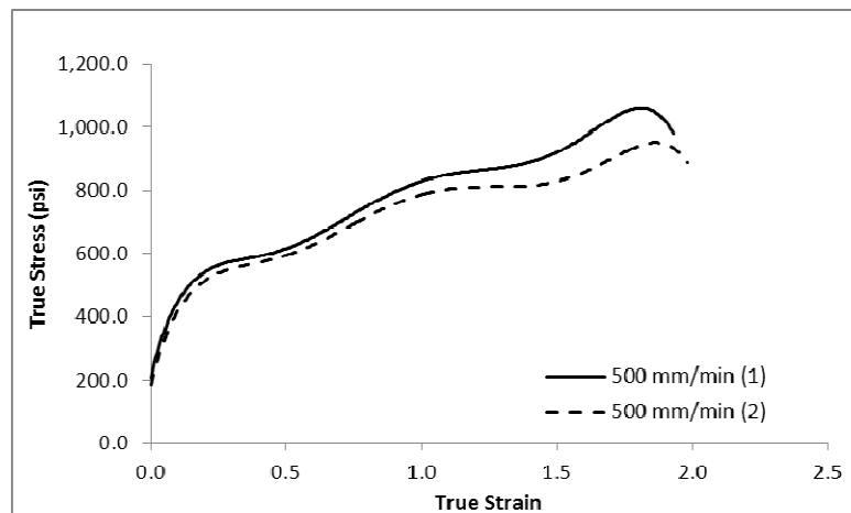
Figure 29 Binder-E, RTFO-plus-PAV, true stress-true strain
