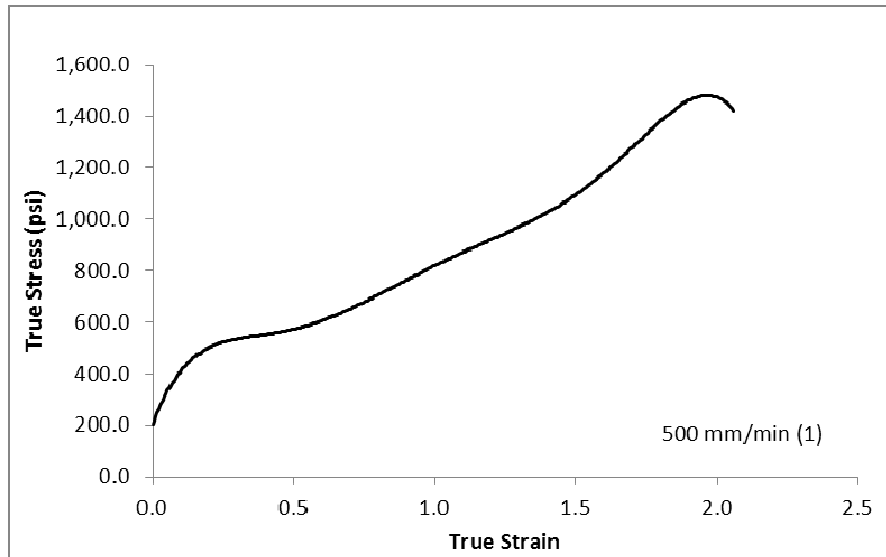
Figure 26 Binder-C, RTFO-plus-PAV, true stress-true strain
