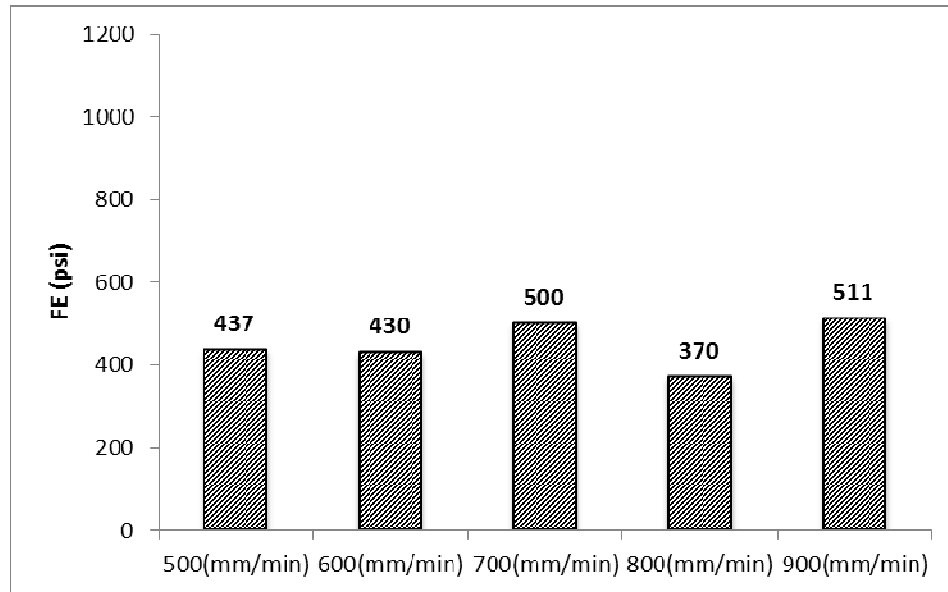
Figure 18 Binder-F, fracture energy vs. loading rates
