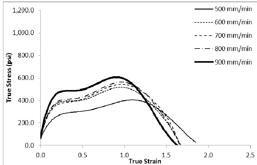
Figure 15 Binder-G, true stress-true strain
