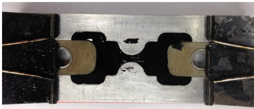
Figure 3 Specimen after trimming surface
