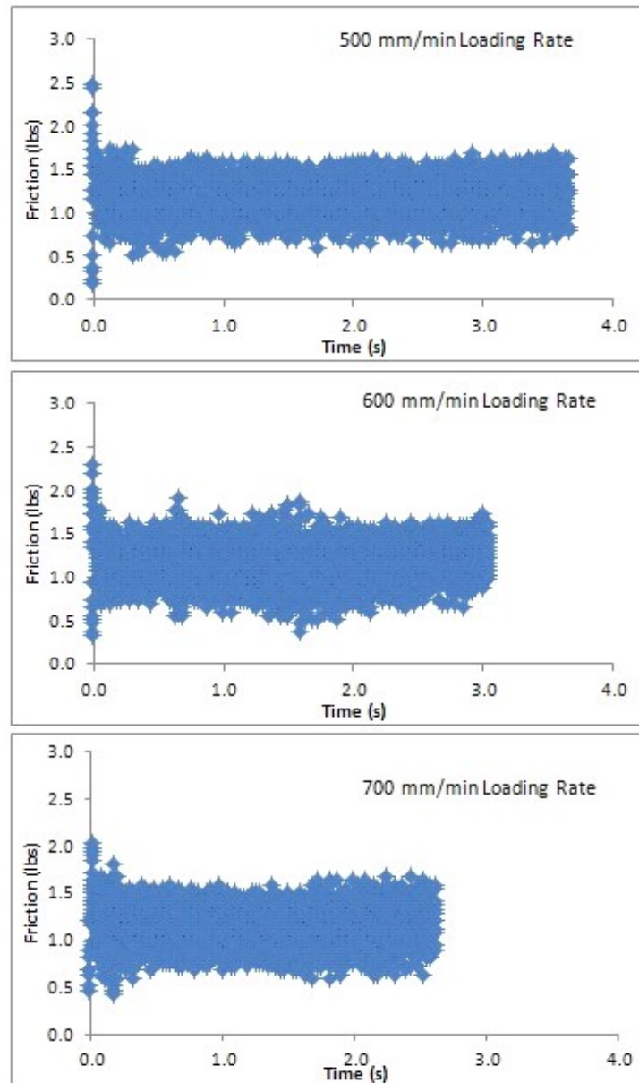
Figure 7 Friction test results at 500, 600, and 700 mm/min loading rates
