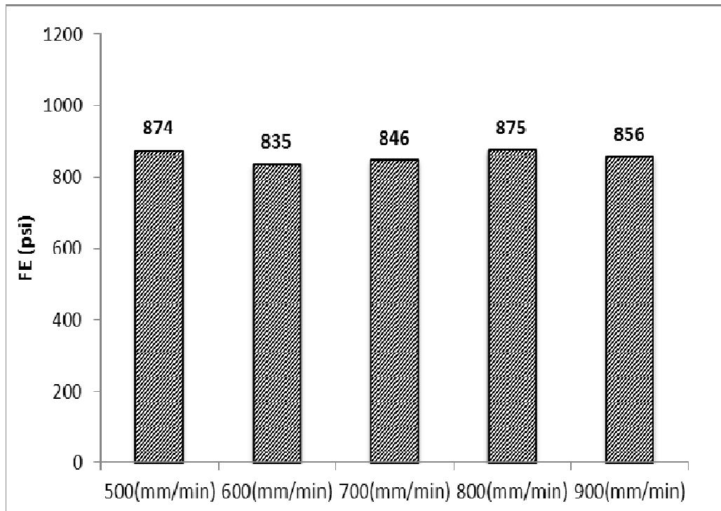
Figure 21 Binder-D, fracture energy vs. loading rates
