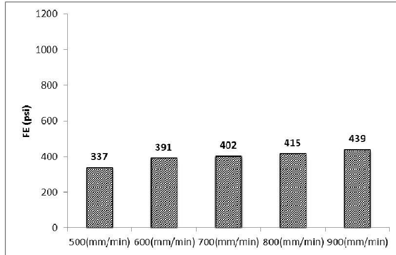
Figure 14 Binder-G, fracture energy vs. loading rates
