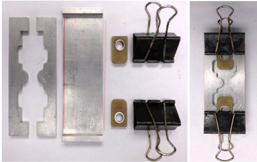
Figure 1 Mold assembly and complete mold set
