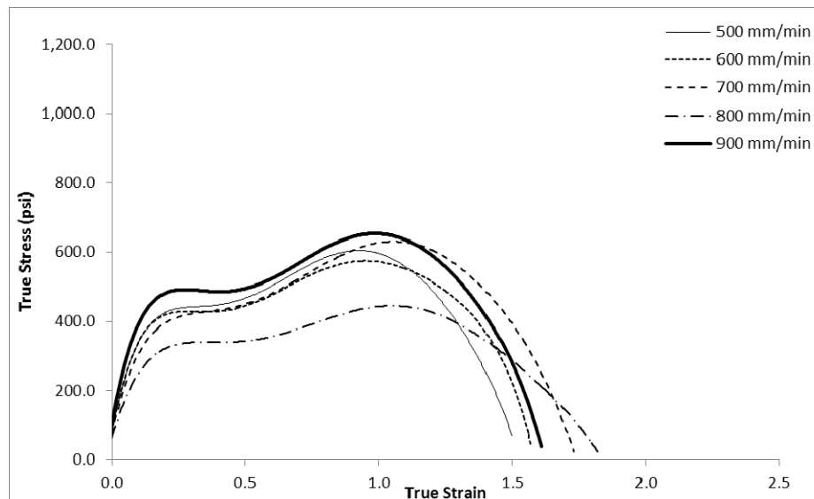
Figure 20 Binder-F, true stress-true strain
