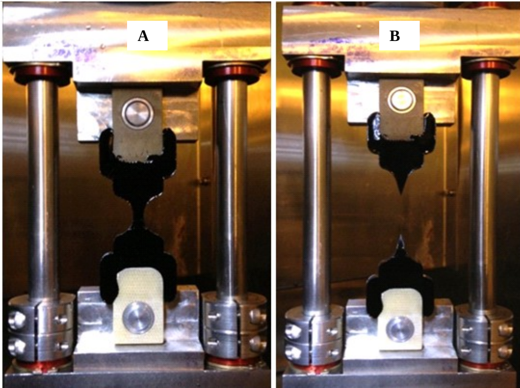
Figure 5 Specimen configurations before (A) and after (B) BFE test
