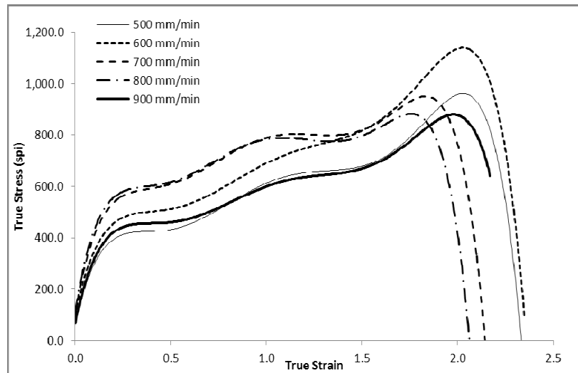
Figure 11 Binder-C, true stress-true strain
