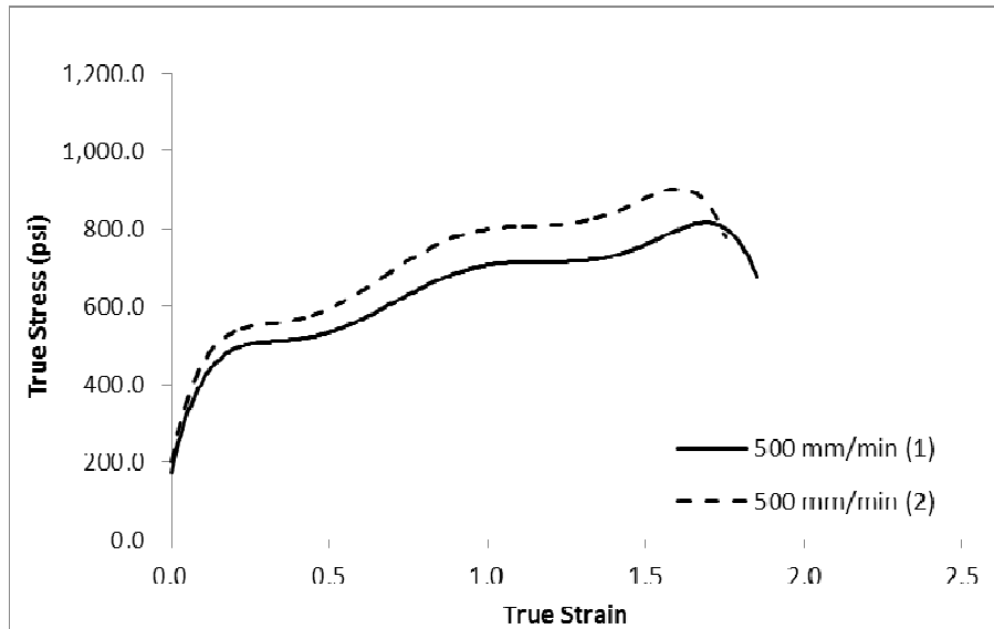
Figure 25 Binder-A, RTFO-plus-PAV, true stress-true strain
