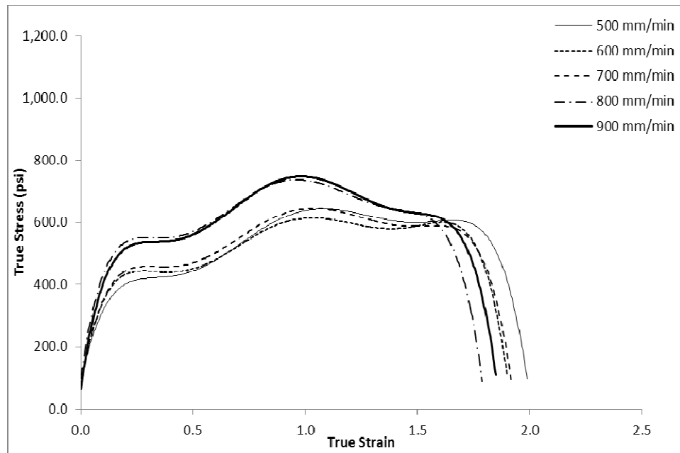
Figure 22 Binder-D, true stress-true strain
