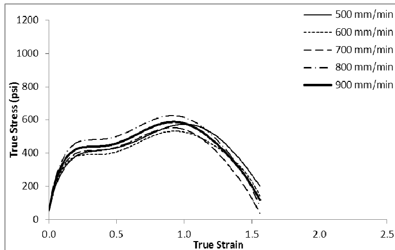
Figure 13 Binder-B, true stress-true strain
