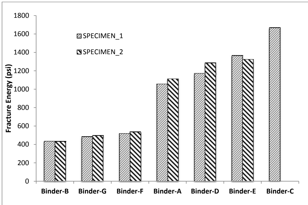
Figure 24 Fracture energy data for all tested specimens at 500 mm/min.
