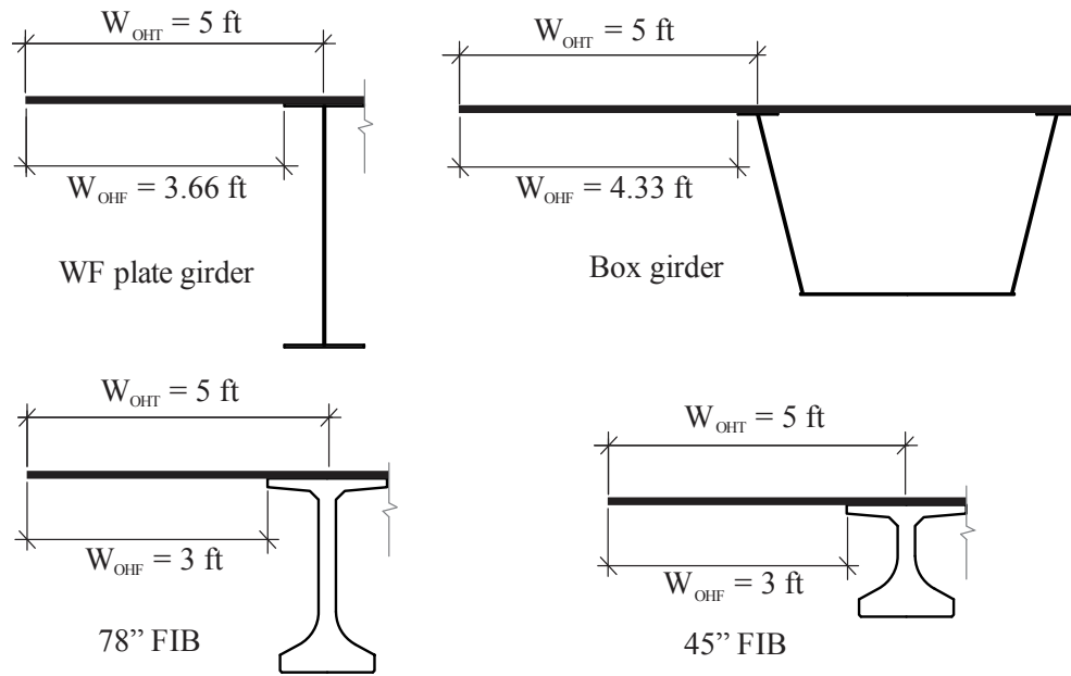
Figure 5.10 Overhang dimensions used in wind tunnel study
