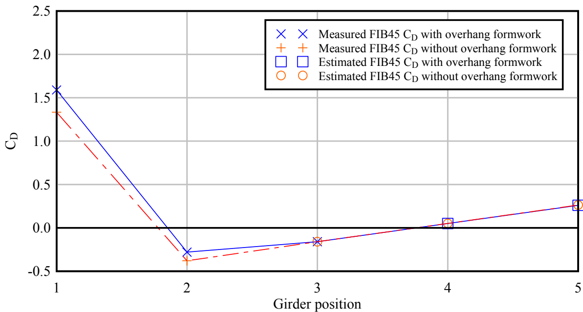
Figure 6.13 Drag coefficients for FIB45 systems (zero degree wind angle)
