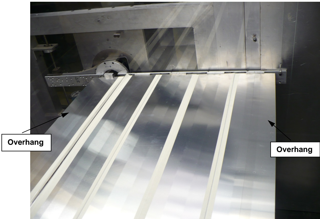
INSTRUMENTED I-BEAM AT 1 st POSITION
