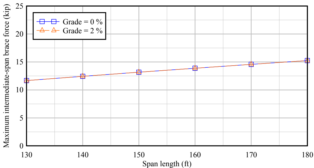
Figure 4.1 Effect of bridge grade on brace forces for an example 78” FIB system
