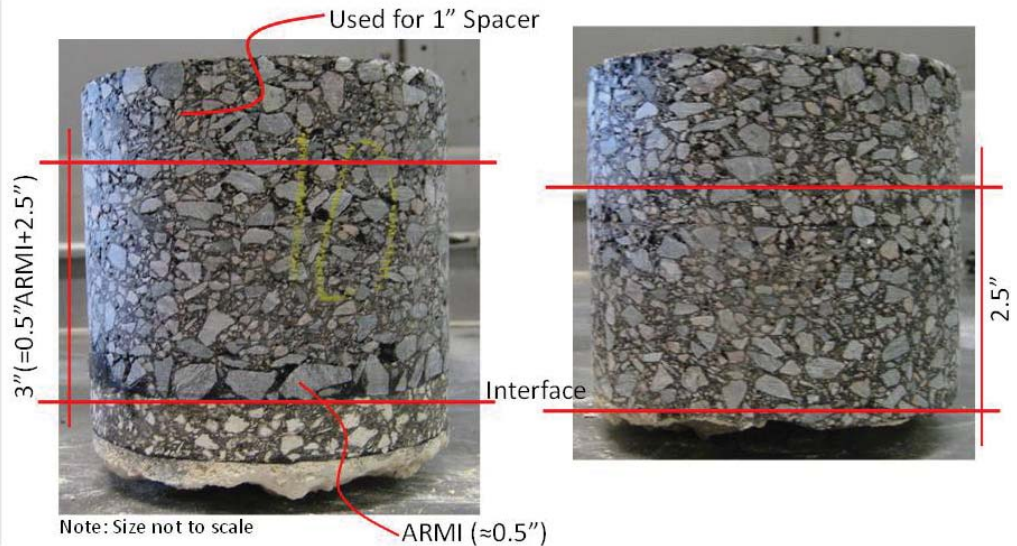
Typical cores from sections with ARMI layer (left) and without ARMI layer (right)
