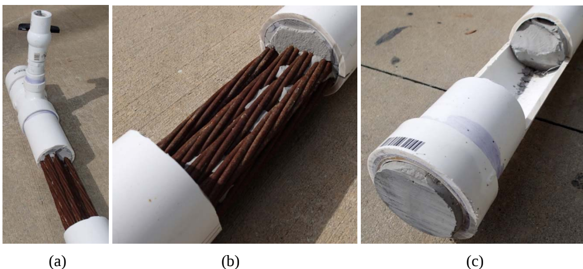
Figure 16—Grout sampling locations (a) at base (b) mid-height and (c) top of inclined tube
