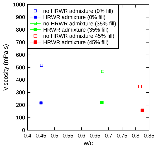
Figure 80—Viscosity for mixes with and without HRWR
