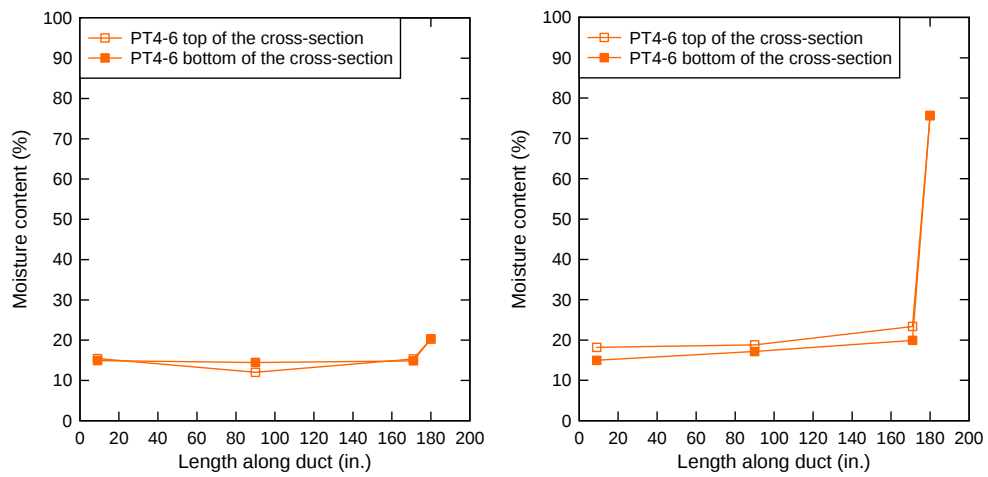
Figure 133—PT4-6 MWD (left), PT4-6 1.15-MWD (right)
