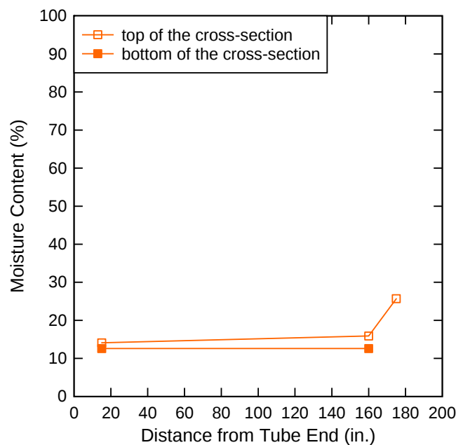
Figure 36—Variation of moisture content with respect to position along tube for material PT4-1 mixed at MWD
