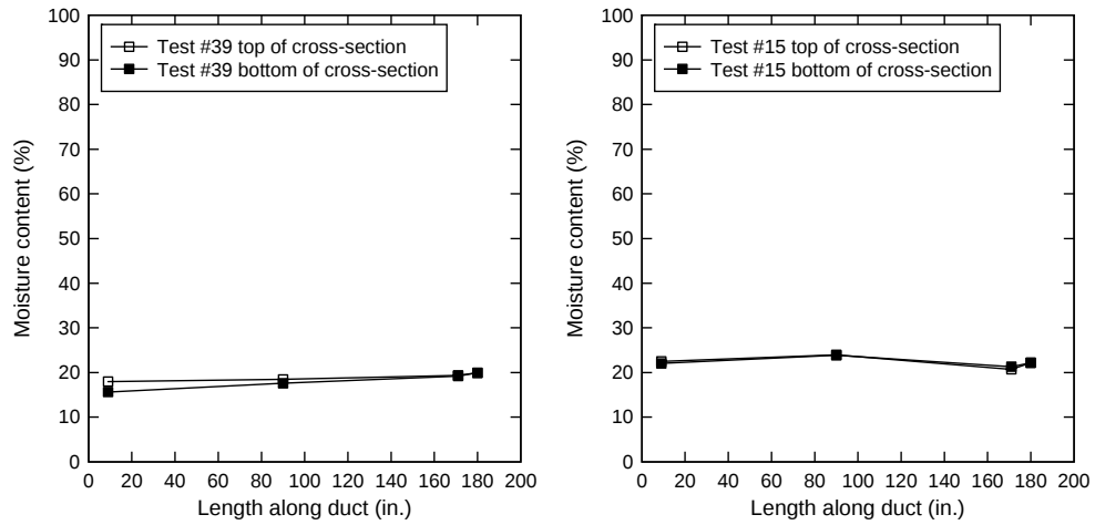
Figure 128—C55-45 (100 mL HRWR) (left), C45-0 (0 mL HRWR) (right)
