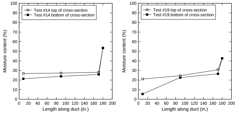
Figure 129—C675-35 (0 mL HRWR) (left), C825-45 (0 mL HRWR) (right)
