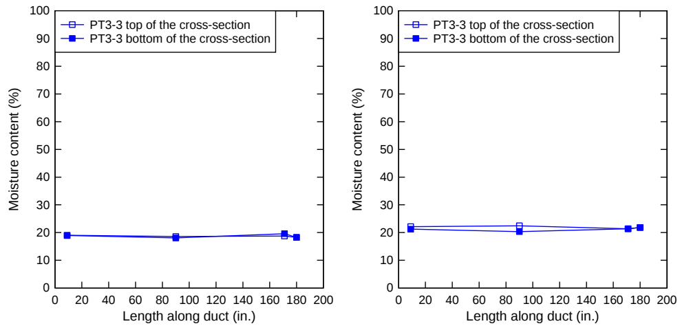
Figure 132—PT3-3 MWD (left), PT3-3 1.15-MWD (right)
