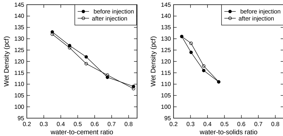
Figure 140—Wet density: 35% filler (left), Wet density: 45% filler (right)
