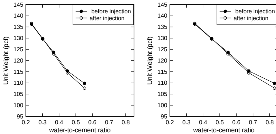
Figure 142—Unit weight: 35% filler (left), Unit weight: 35% filler (right)
