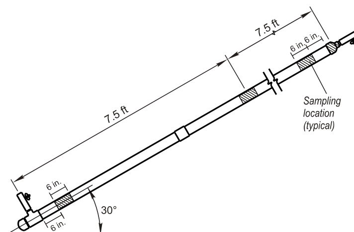
Figure 17—MITT grout sample locations
