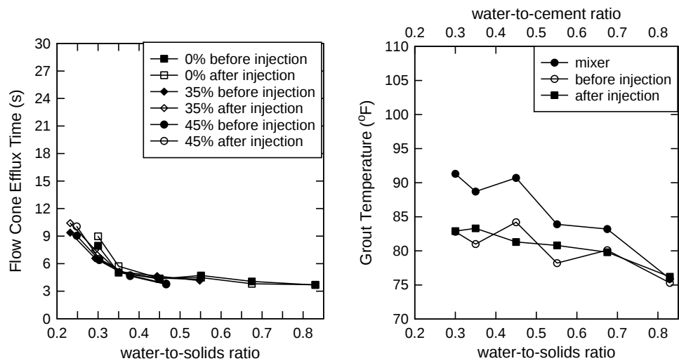
Figure 136—Flow cone efflux time (left), Grout temperature: 0% filler (right)
