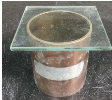
Figure 27—Unit weight used to determine grout density
