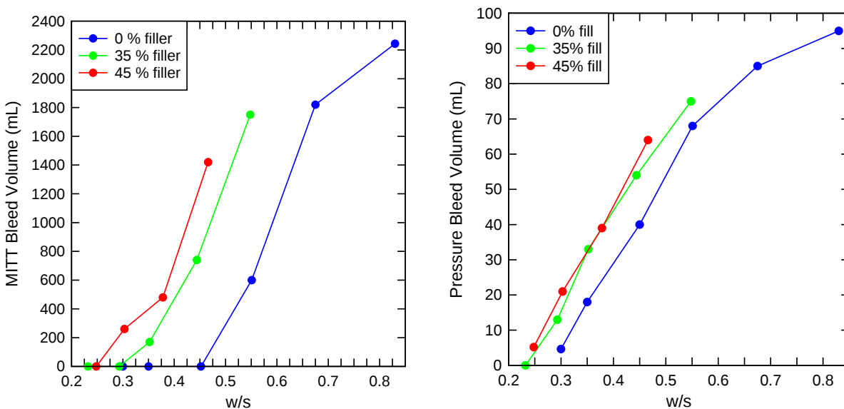
Figure 76—Comparison of modified inclined tube and pressure bleed measurements with respect to w/s
