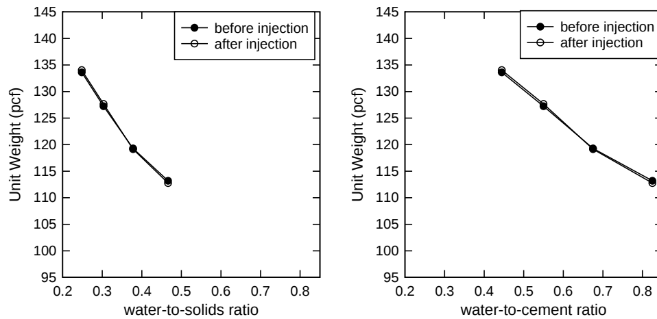
Figure 143—Unit weight: 45% filler (left), Unit weight: 45% filler (right)
