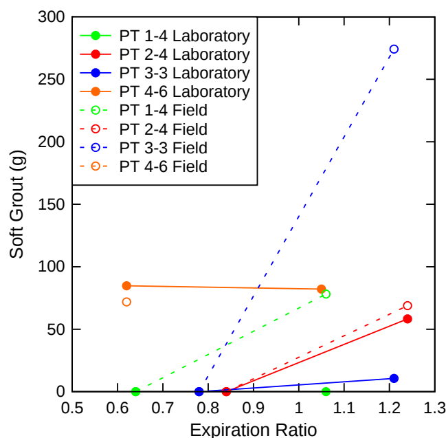
Figure 94—Mass of soft grout collected during MITT for expired and unexpired grout in Laboratory and Field conditions
