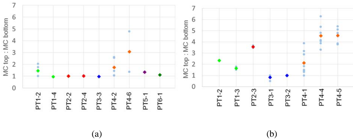
Figure 99—Average ratios of the moisture content at top of the tube to moisture content at the bottom of the tube for all tests using MWD and categorized by lot on (a) unexpired grout and (b) expired grout.
