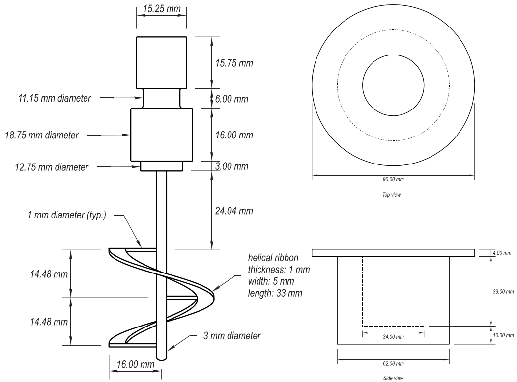
Figure 35—Helical ribbon and cup schematics
