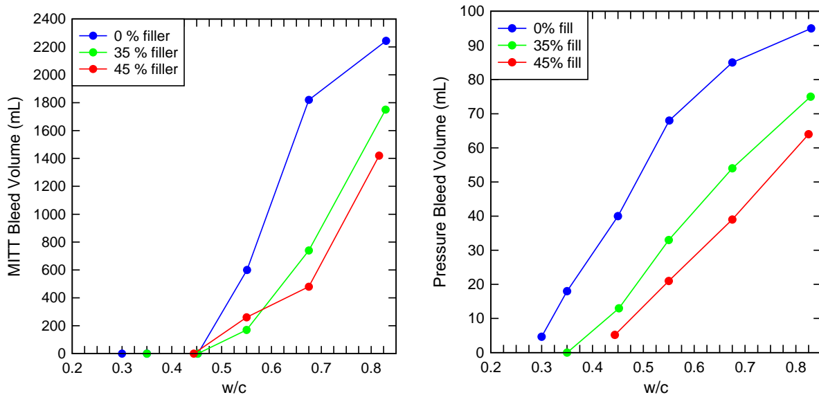
Figure 75—Comparison of modified inclined tube and pressure bleed measurements with respect to w/c
