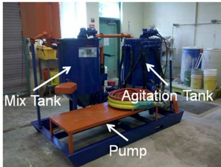
Figure 6—Colloidal grout plant with various parts labeled
