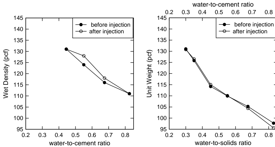
Figure 141—Wet density: 45% filler (left), Unit weight: 0% filler (right)
