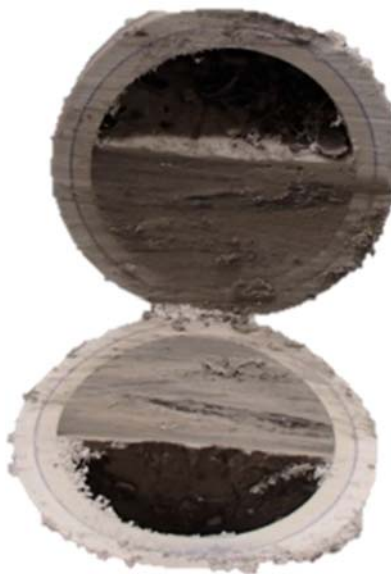
Figure 113—C35-35 hardened grout
