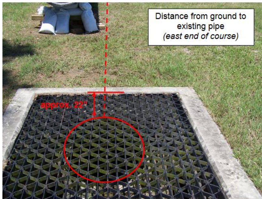
Figure 3-20: Depth to Existing Drainage Pipe (East End)
