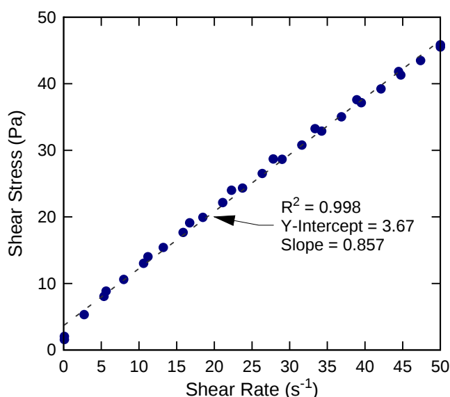
Figure 22—Flow curve results for SRM (prepared with tap water) on the same day as mixing. The uncertainty on the date shown is considered as calculated for the SRM 2492 (see Figure 22)
