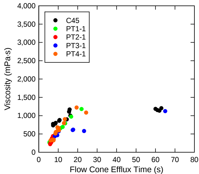
Figure 29—Comparison of DSR viscosity and flow cone efflux time for shear rate of 100 s -1 . The uncertainty is discussed in section 9.2.3 for viscosity and 0.88 s for the flow cone (ASTM C939)
