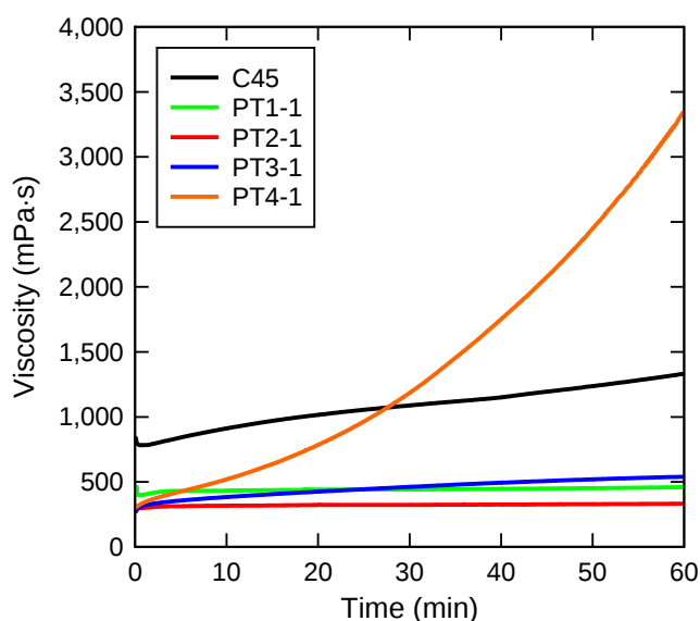
Figure 31—Results of 60 min NSR viscosity test conducted on grouts C45, PT1-1, PT2-1, PT3-1, and PT4-1. The uncertainty is discussed in section 9.2.3
