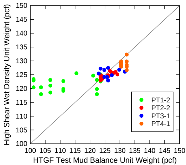
Figure 84—Plot of wet density value measured where high-shear mixer was used for grout conditioning versus mud balance value measured during HTGF test. The uncertainty for this test method in single laboratory tests has not yet been established.
