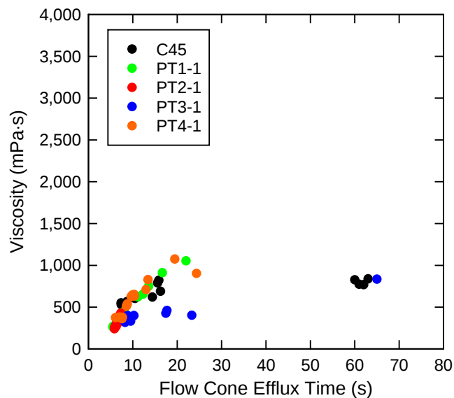
Figure 30—Comparison of DSR viscosity and flow cone efflux time for shear rate of 165 s -1 . The uncertainty is discussed in section 9.2.3 for viscosity and 0.88 s for the flow cone (ASTM C939)
