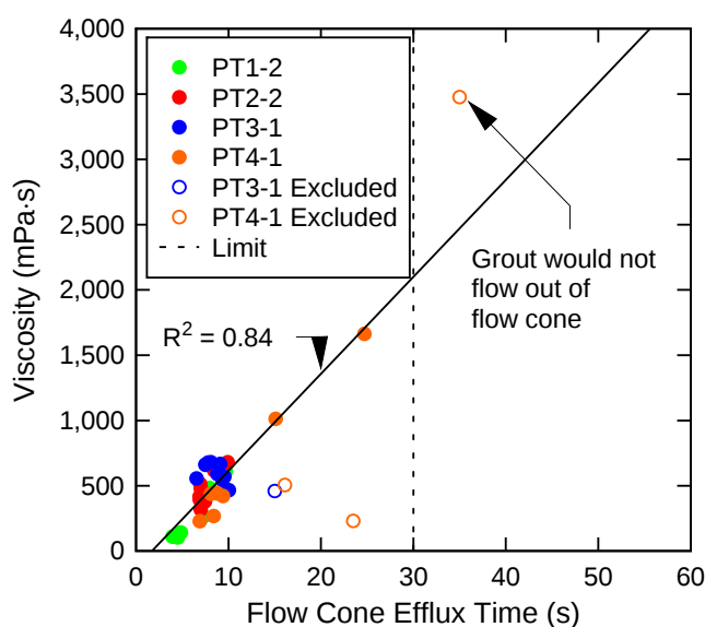
Figure 42—Comparison of NSR viscosity and flow cone efflux time for samples collected during HTGF test. The uncertainty is discussed in section 9.2.3 for the viscosity and 0.88 s for the flow cone (ASTM C939)
