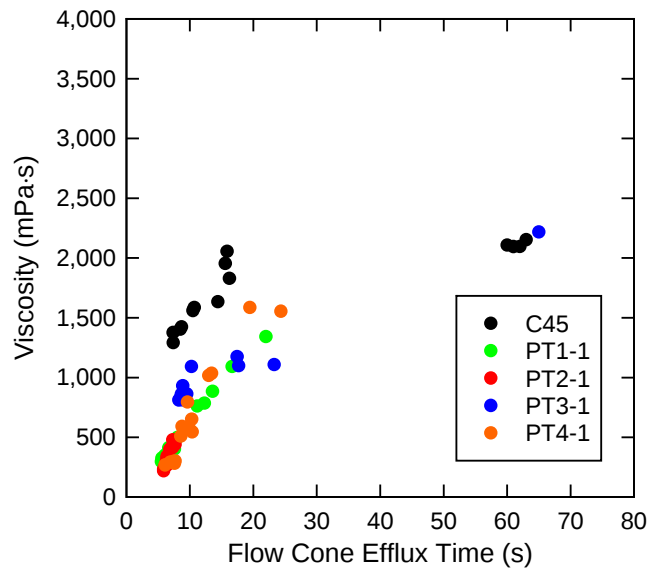
Figure 27—Comparison of DSR viscosity and flow cone efflux time for shear rate of 50 s -1 . The uncertainty is discussed in section 9.2.3 for viscosity and 0.88 s for the flow cone (ASTM C939)
