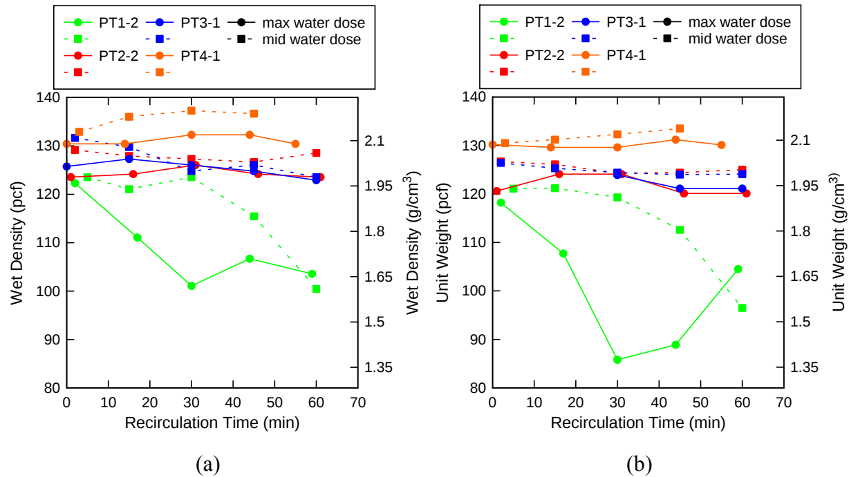
Figure 41—Variation (a) wet density and (b) unit weight during HTGF test. These are single measurements, but the uncertainty could be estimated at 1 pcf (0. 016 g/cm³) from previous measurements not reported here.
