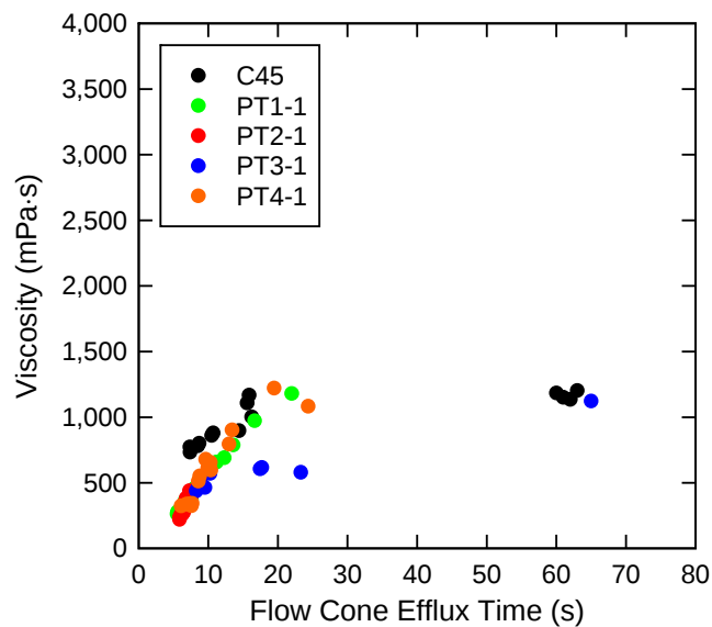
Figure 28—Comparison of DSR viscosity and flow cone efflux time for shear rate of 75 s -1 . The uncertainty is discussed in section 9.2.3 for viscosity and 0.88 s for the flow cone (ASTM C939)
