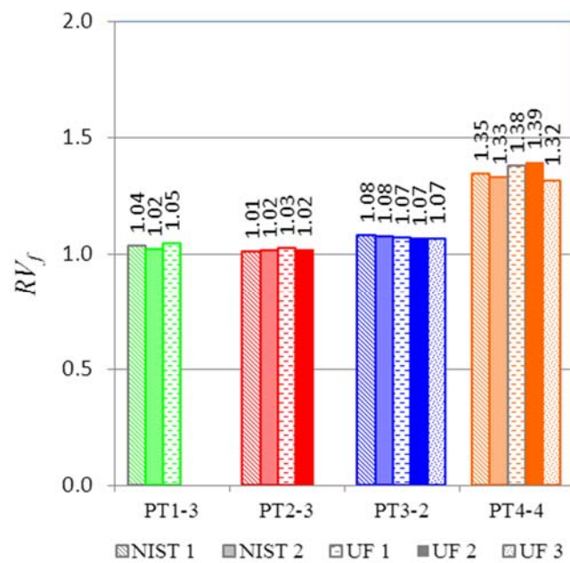
Figure 66—Comparison of RV_f from UF and NIST
