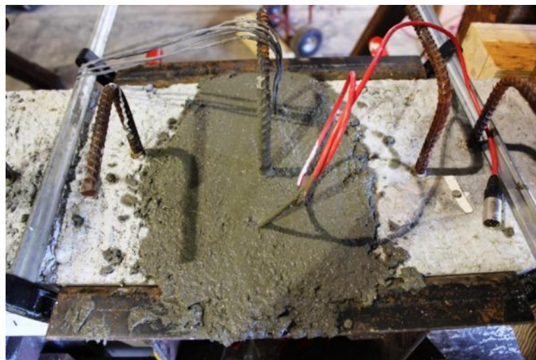
Figure 63—Additional stirrup
