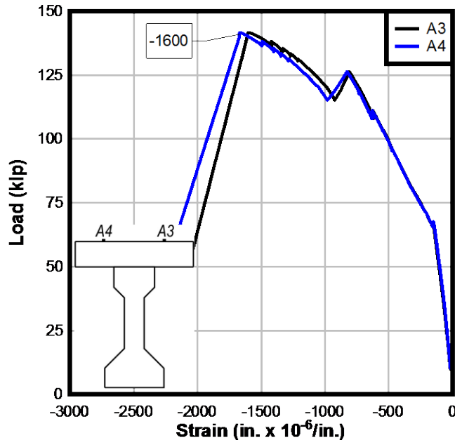
Figure 164-F1: Deck strain
