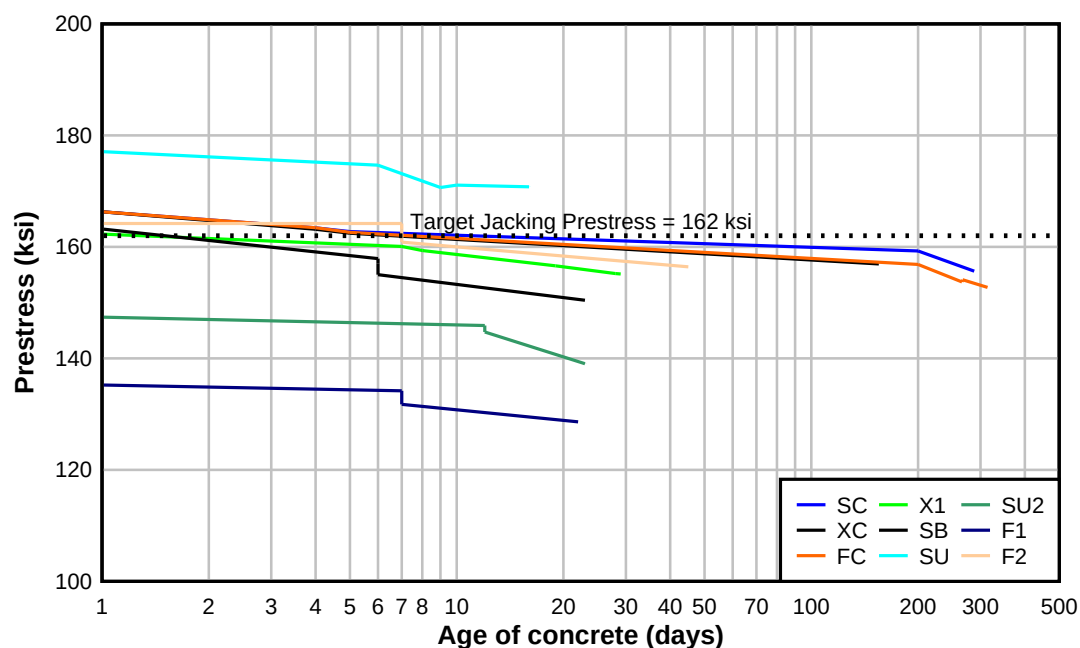
Figure 81—Prestress force
