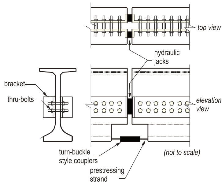
Figure 16—Prototype splice design
