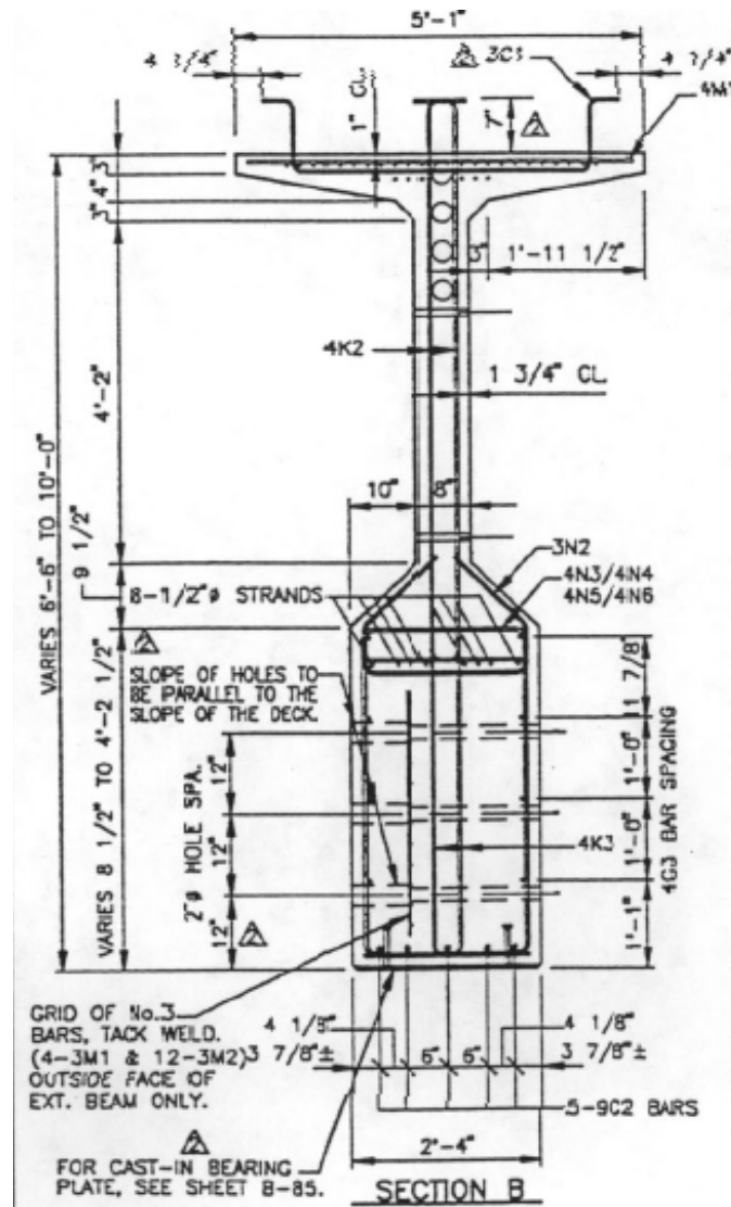
Figure 6–Gandy Bridge splice connection detail (FDOT 1999)
