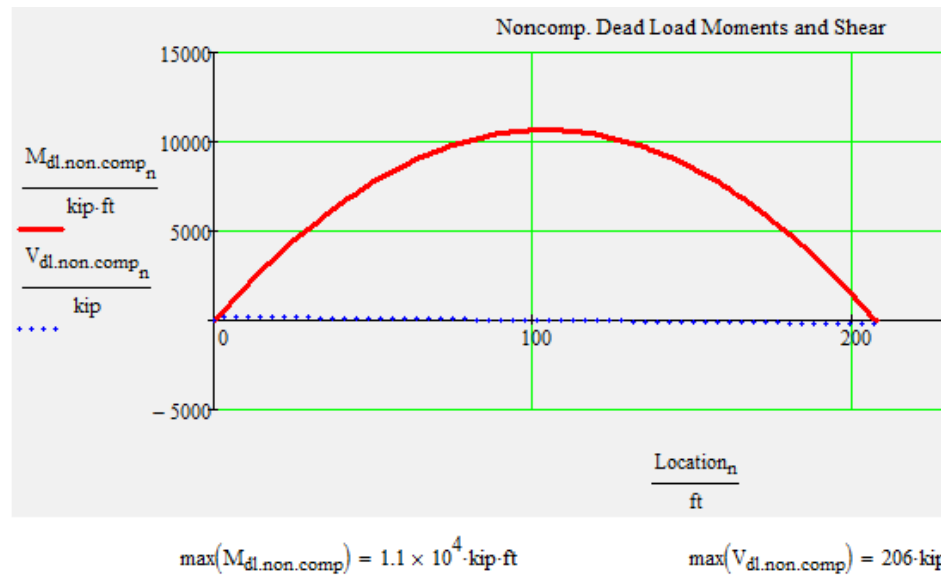
Figure 199–Unfactored Dead Loads on Non-Composite Section–Assembled Length
