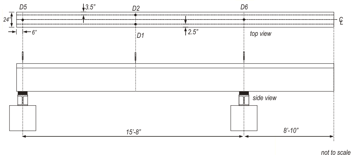
Figure 78—Shear: Vertical displacement gages
