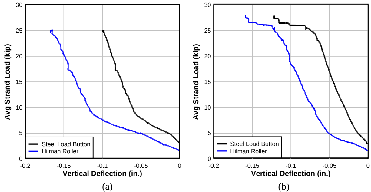
Figure 89–Tie-down deflections: (a) SB and (b) SU
