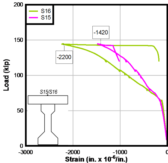
Figure 104-X1: Deck strain
