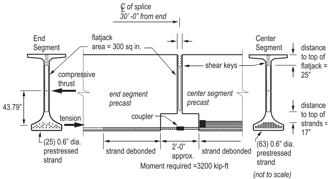
Figure 206—Splice Design C
