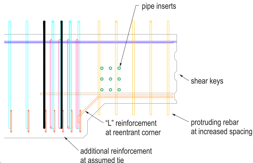
Figure 33–Detailing considerations
