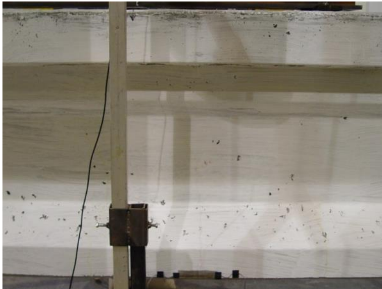
Figure 83—Decompression strain gages
