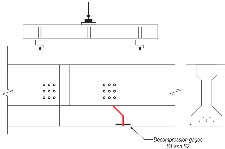
Figure 155 –F1: Joint opening
