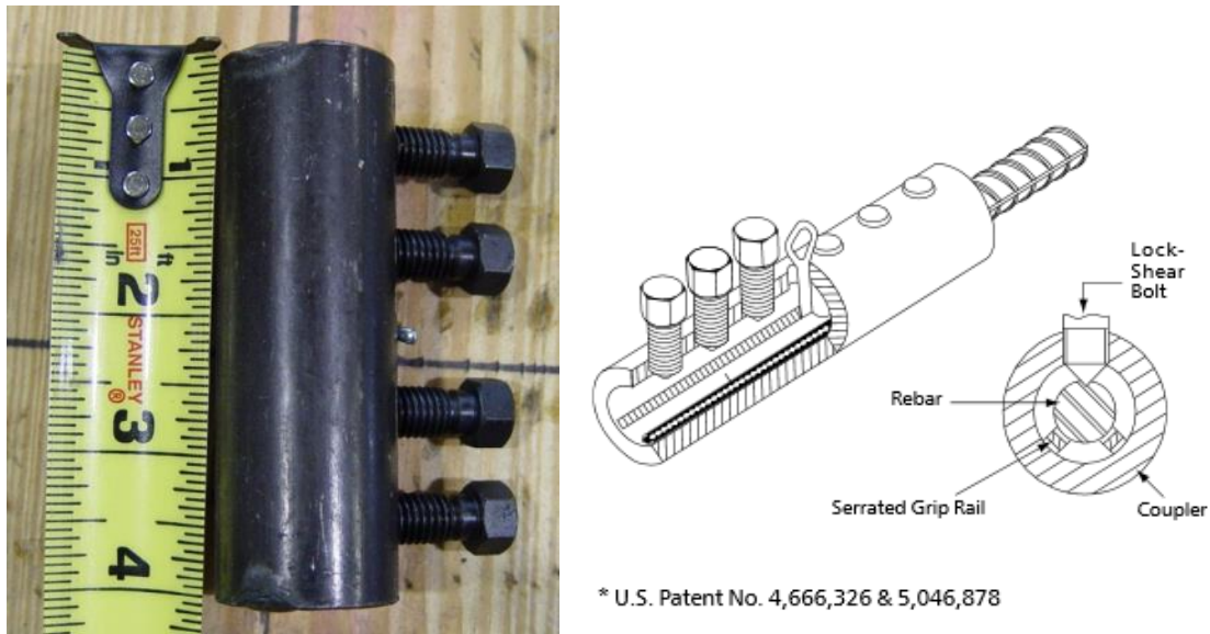
Figure 36–Rebar coupler
