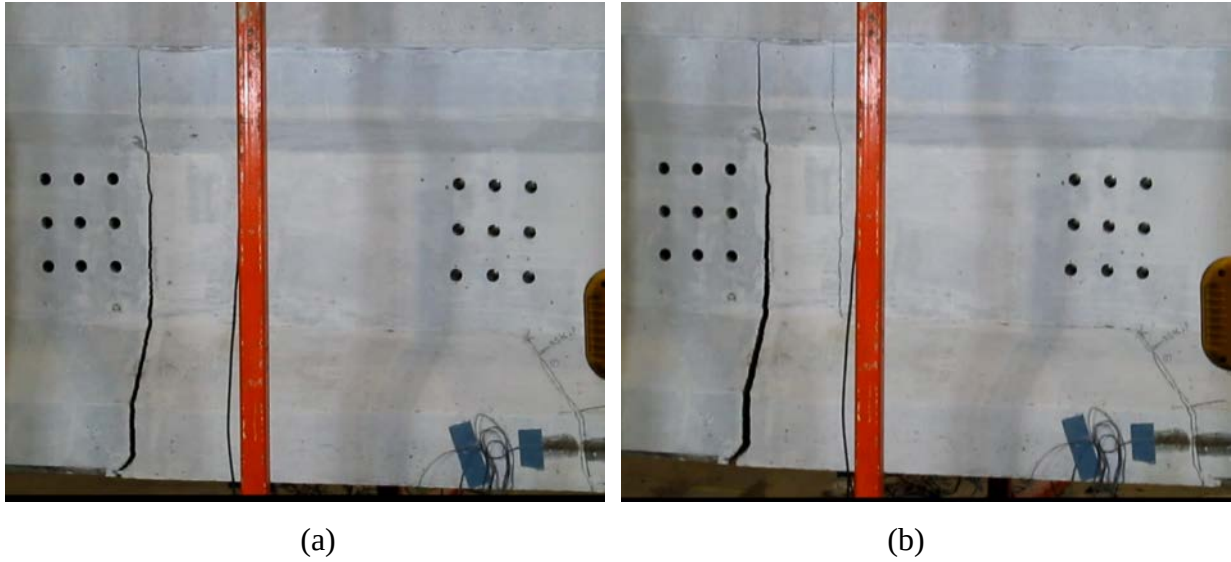
Figure 161–F1: Crack pattern at (a) 125 kip, prior to strand rupture (b) after load drop
