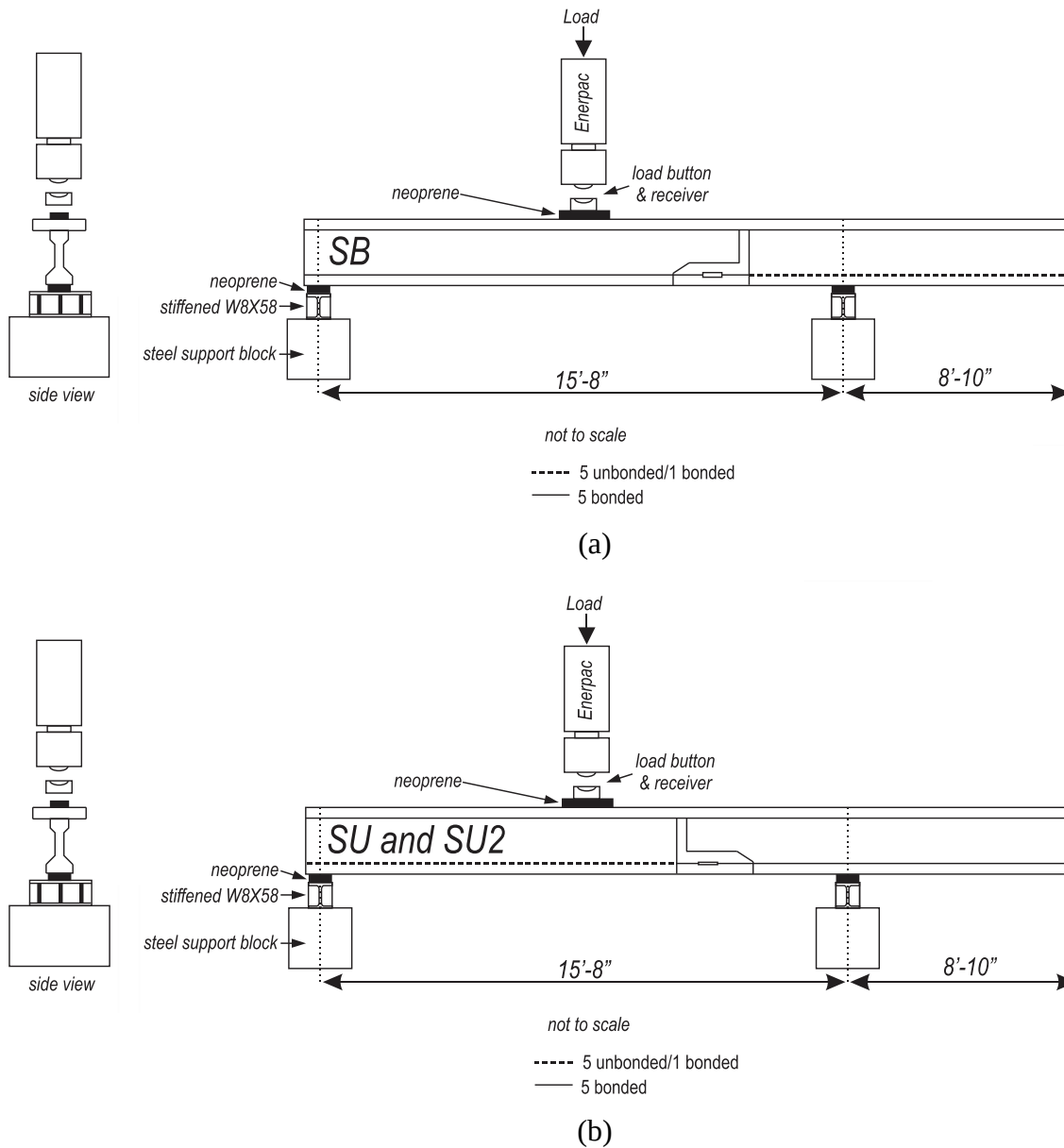
Figure 76–Spliced shear test set-ups for (a) SB and (b) SU and SU2
