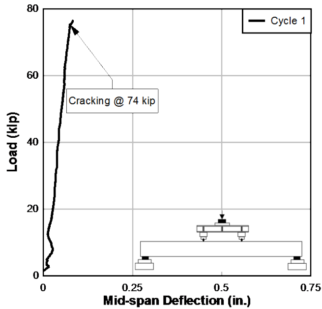
Figure 145-FC: Static conditioning
