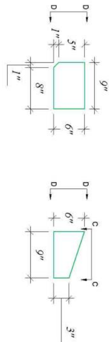
(8) PLATE A - exterior stiffeners Grade 50, t=3/4 in.
