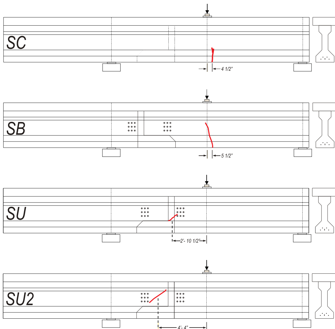
Figure 135–Shear specimens: First crack locations
