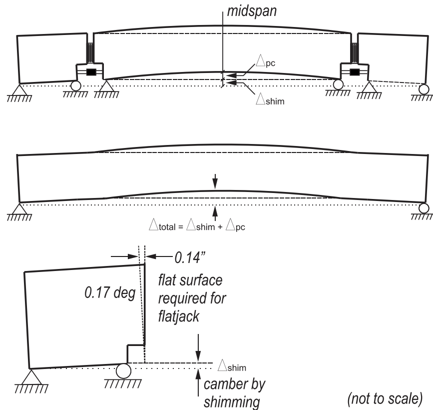
Figure 209–Splice C with canted ends
