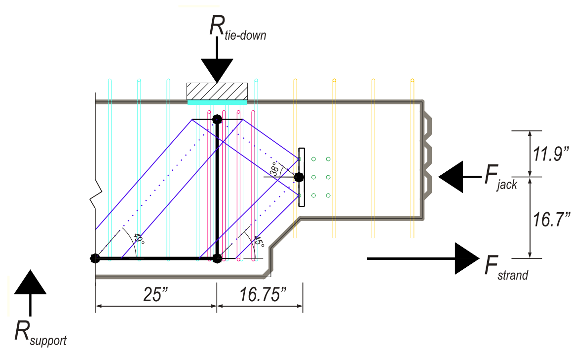
Figure 91–STM: assumed dimensions
