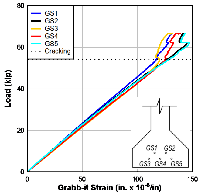
Figure 156–F1: Coupler strain
