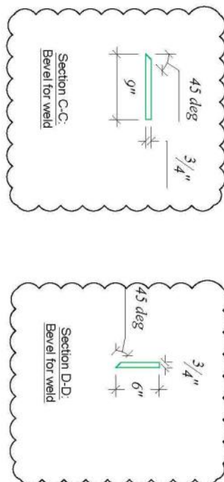
(8) PLATE A - exterior stiffeners Grade 50, t=3/4 in.
