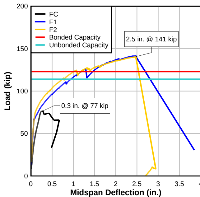
Figure 182 –Post-fatigue Failure: FC, F1 and F2
