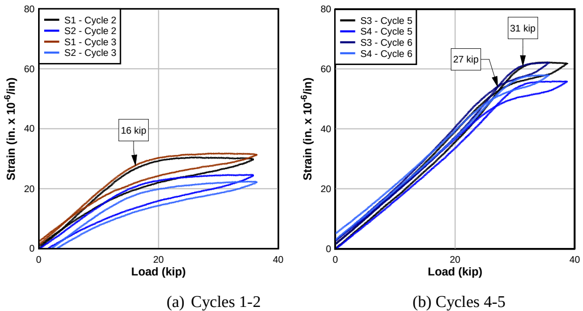
Figure 171-F2: Decompression strain readings
