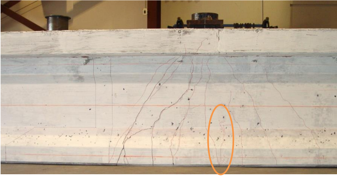
Figure 117-SC: Crack pattern
