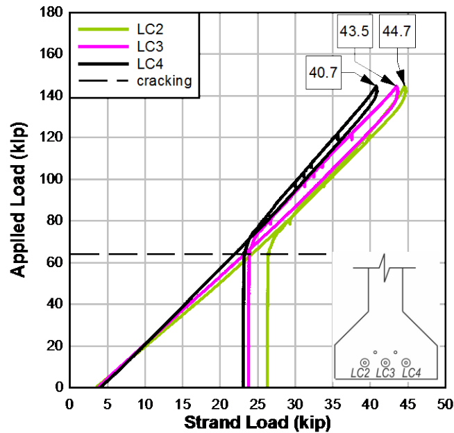
Figure 115-X1: Strand load
