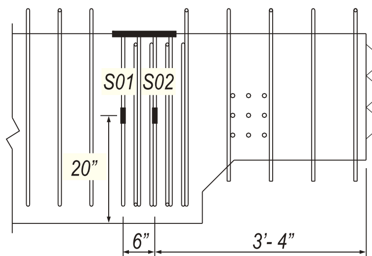
Figure 65—Gaged stirrup locations
