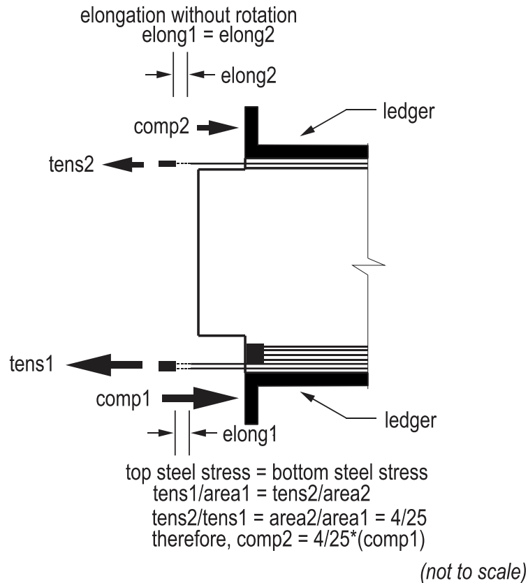
Figure 214—Forces of Splice Design F
