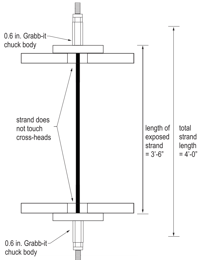
Figure 26—UF tensile test set-up of 0.6 in. dia. coupler
