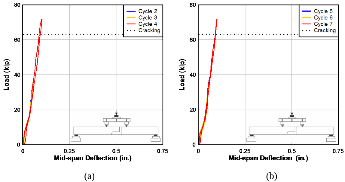
Figure 170-F2: Static load cycles (a) 2-4 and (b) 5-7
