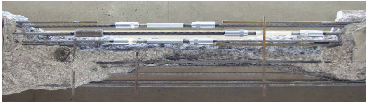
Figure 15–Repair of severed strand using a coupler (Ministry of Transportation of Ontario 2011)
