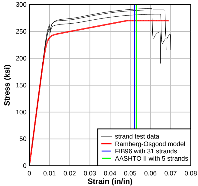
Figure 40—Material properties of 270 ksi lo-lax strand
