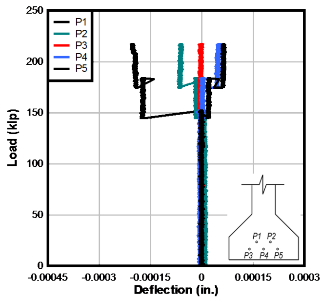
Figure 121–SB: Strand slip
