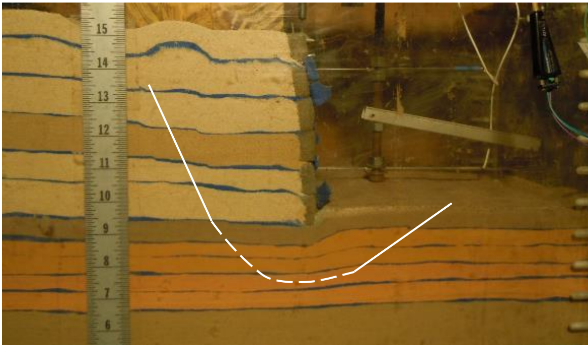
Figure 4-7 Post-test observed rupture surface in Test 15 model ( \delta = 30^\circ and \mu_\phi = 28^\circ ): Dashed line is the estimated surface; Solid line is offset from observed surface
