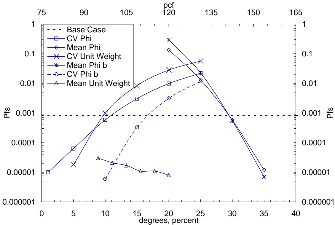
Figure 2-3 Probabilities of failure from sliding stability parametric study
