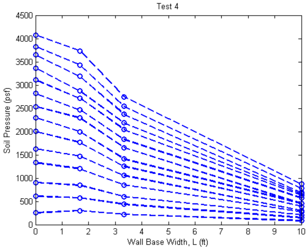
Figure 5-5 Distributions of soil pressure beneath MSE wall in Test 4 for increasing surcharge
