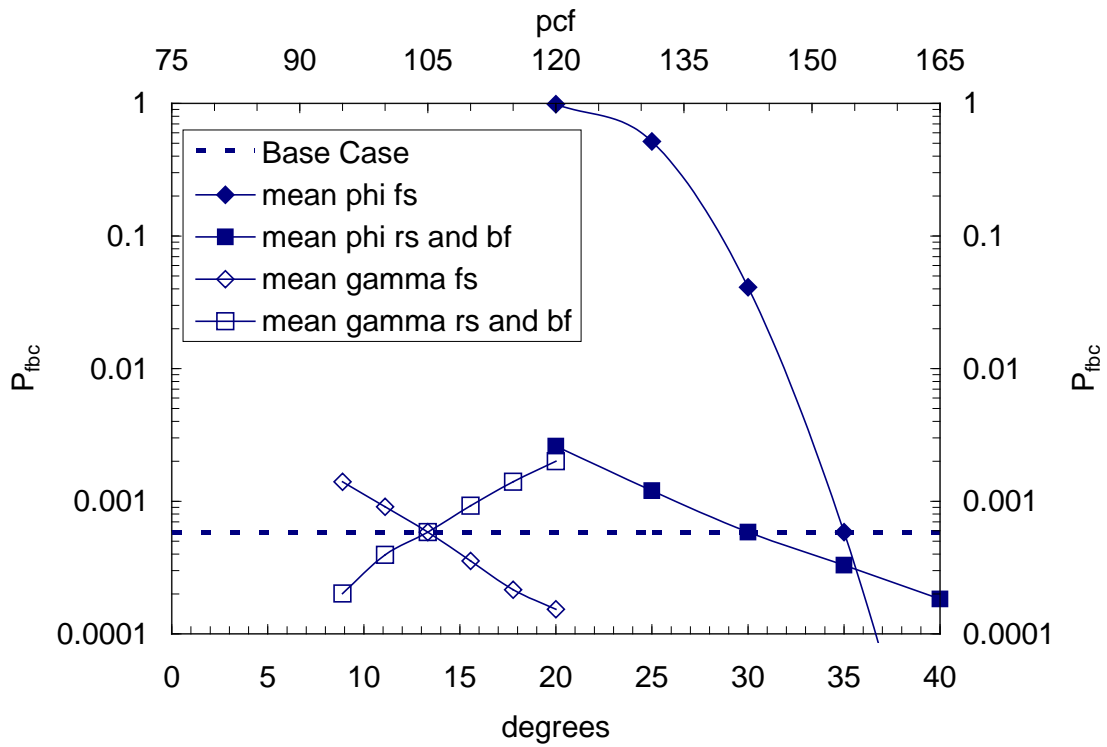
Figure 2-6 P_f from bearing stability parametric study: varied mean values
