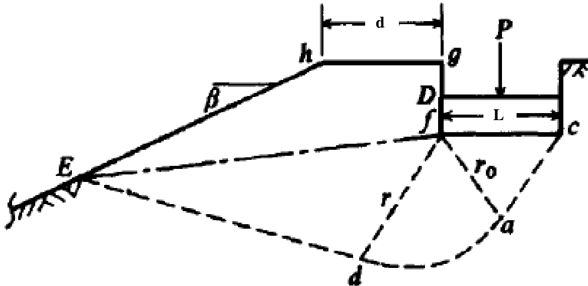
Figure 5-14 Shallow footing with concentric load and near an embankment (Bowles, 1997)
