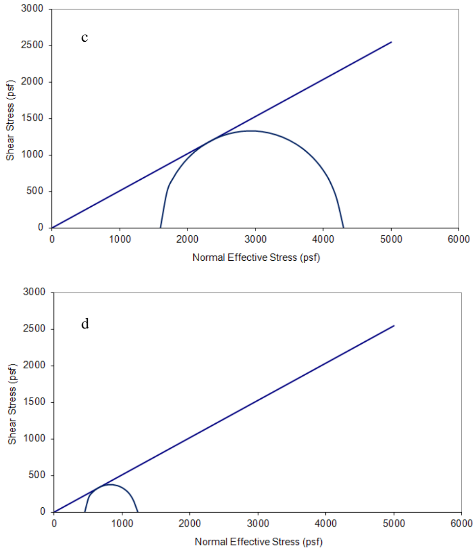
Figure 5-19 Mohr circles for points c and d on the slope rupture surface
