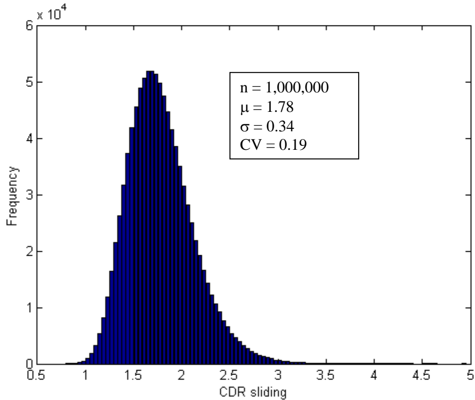
Figure 2-2 Histogram of CDR for MSE wall sliding stability
