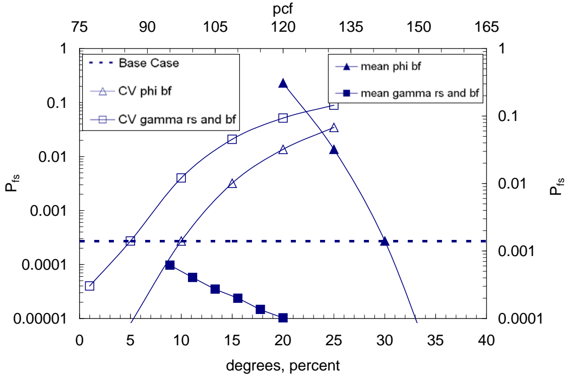
Figure 2-9 Probabilities of failure from sensitivity study on overturning: varied \mu and CV values
