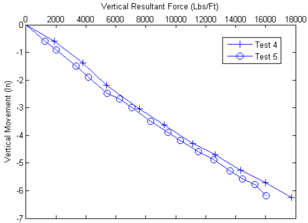
Figure 5-7 Load settlement curves for MSE walls on embankments for Tests 4 and 5
