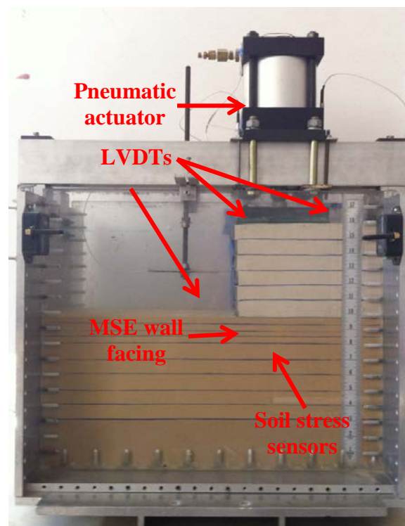
Figure 2-14 Setup of MSE wall model in test container
