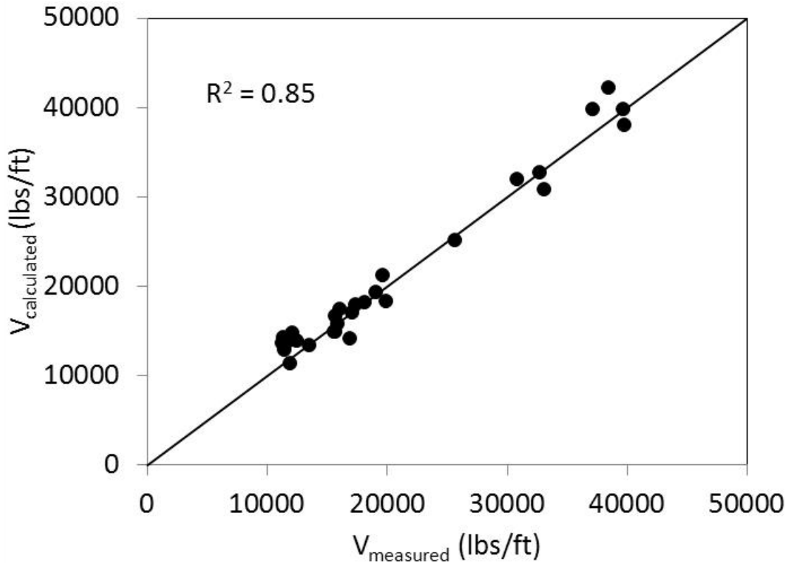
Figure 4-6 V_{\text{calculated}} versus V_{\text{measured}} for all MSE wall tests ( \mu_{\phi_{fs}} = 26^{\circ} - 33^{\circ} )
