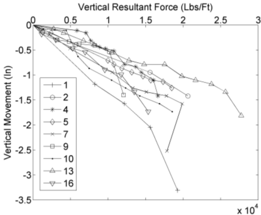
Figure 4-2 Load settlement curves for MSE walls with foundation soil \mu_\phi = 28^\circ - 30^\circ were then grouped into two ranges of mean strength, \mu_\phi of the foundation soil: 26^\circ - 30^\circ and 31^\circ - 33^\circ . Figures 4-3(a) and (b) show the cumulative distributions of the vertical resultant force (i.e., capacity) and fitted lognormal cumulative distribution functions for each range. The lognormal models could not be rejected at a level of significance of 5% as indicated by the Kolmogorov-Smirnov goodness of fit test, ( p = 0.75 and 0.93 , respectively). Further testing on the tails of the cdfs at a level of significance 5% with the Anderson-Darling goodness of fit test indicated the lognormal models could not be rejected ( p = 0.25 and 0.5 , respectively). These two ranges were subsequently used in determining the associated \Phi 's.
