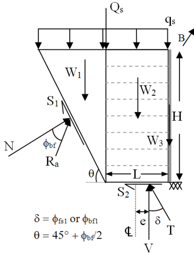
Figure 6-1 Force diagram for MSE wall and soil wedge
