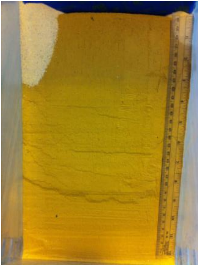
Figure 5-12 Post-test observed rupture on surface of embankment in Test 12 model
