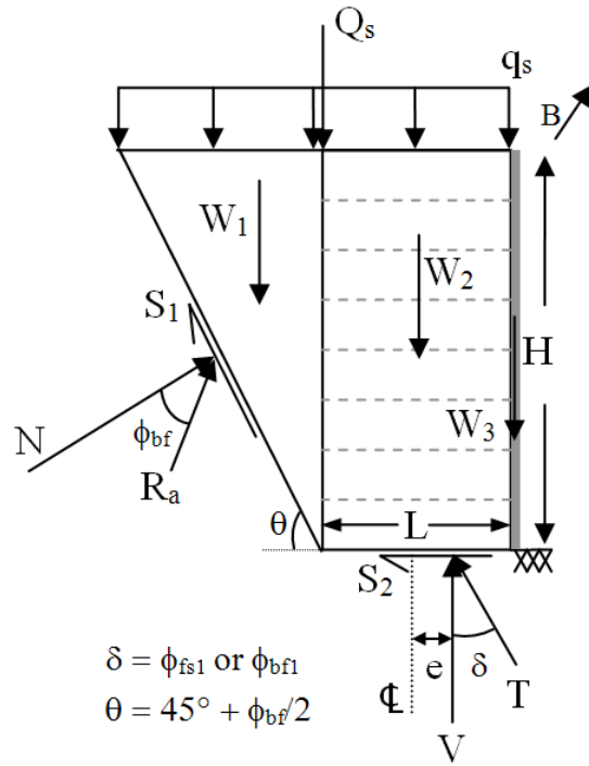
Figure 4-4 Force diagram for MSE wall and soil wedge
