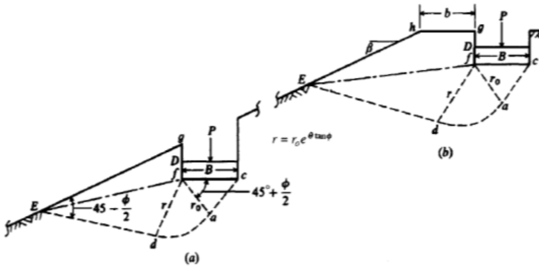
Figure 1-4 Footing (a) on slope and (b) near slope (Bowles, 1997)
