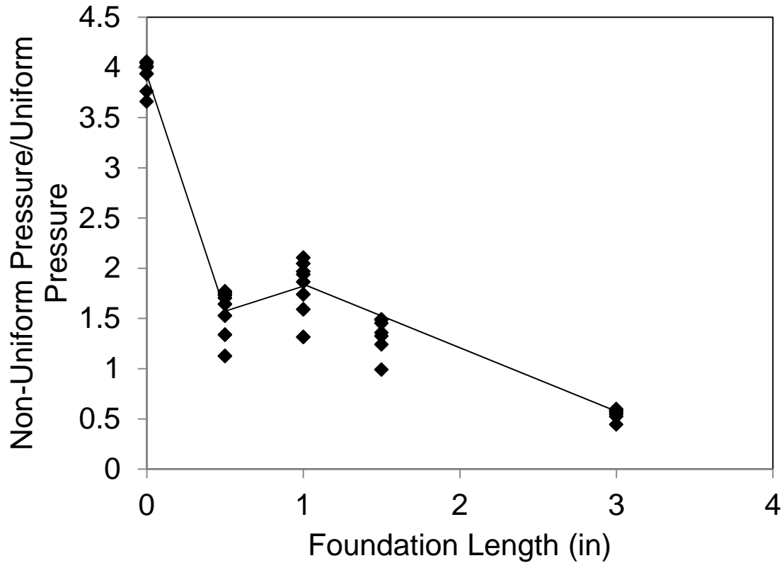
Figure 4-10 Normalized pressure distributions measured from self-weight of MSE wall and piecewise linear approximation
