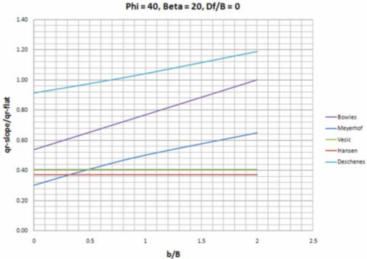
Figure 1-5 Comparison of methods for ratio of bearing capacity to influence of distance to slope, for a beta of 20°
