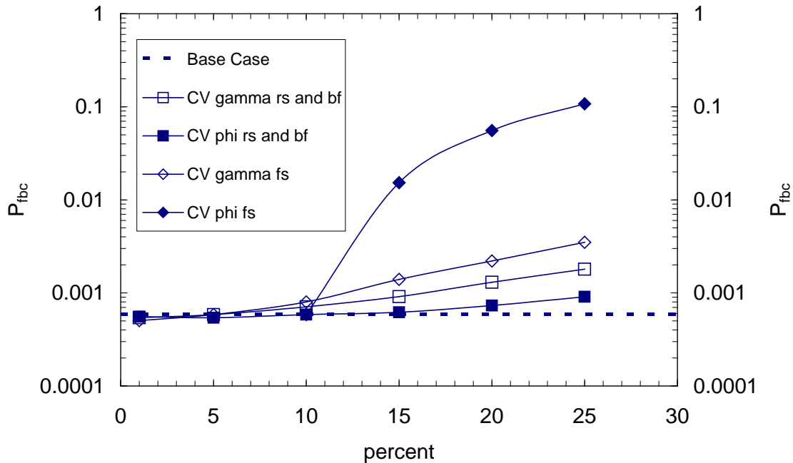
Figure 2-7 P_f from bearing stability parametric study: varied CV values
