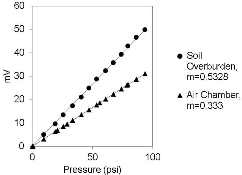
Figure 2-16 Soil stress sensor sensitivities from calibrations (m = slope)
