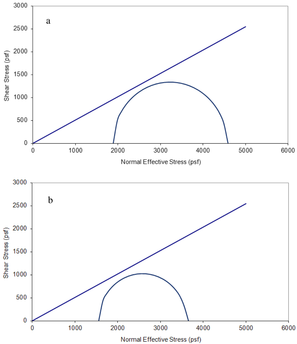
Figure 5-18 Mohr circles for points a and b on the bearing rupture surface
