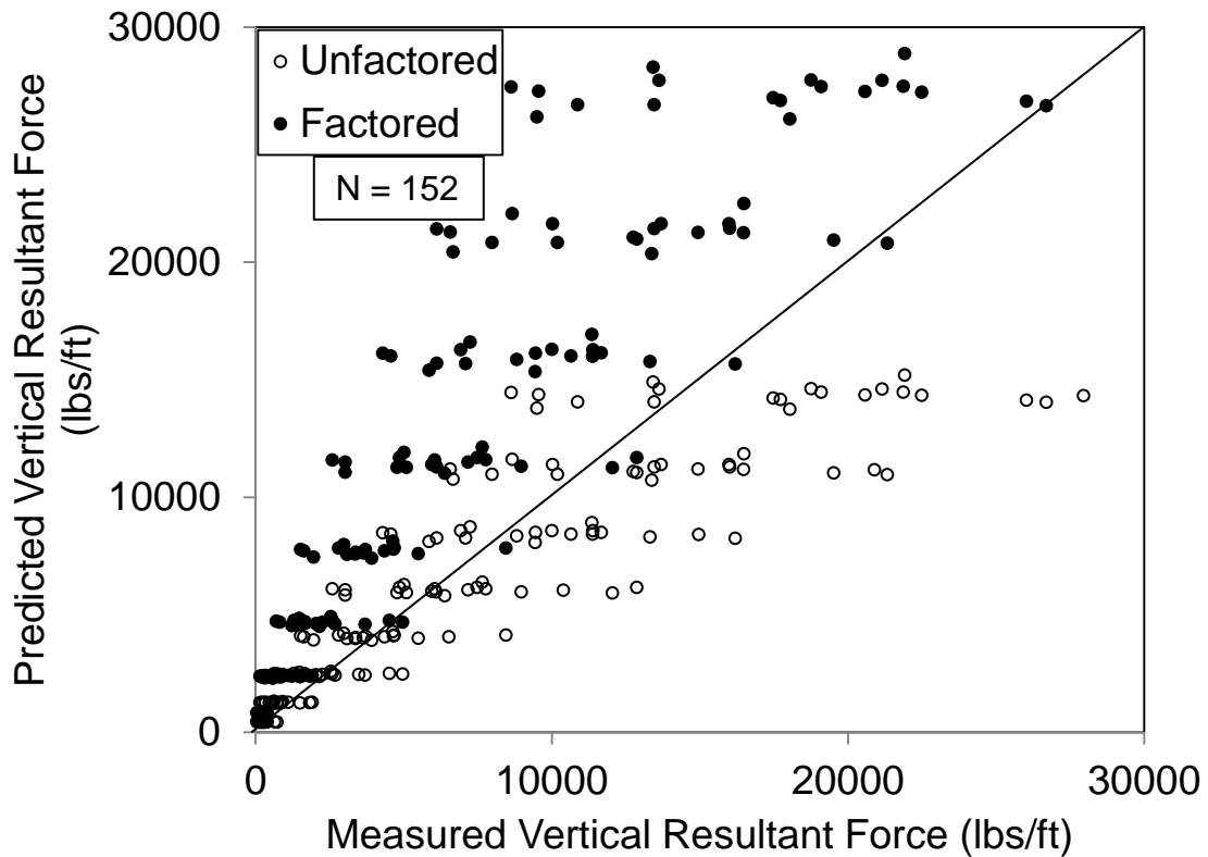
Figure 4-11 Unfactored and factored predicted vertical resultant forces versus measured vertical resultant force
