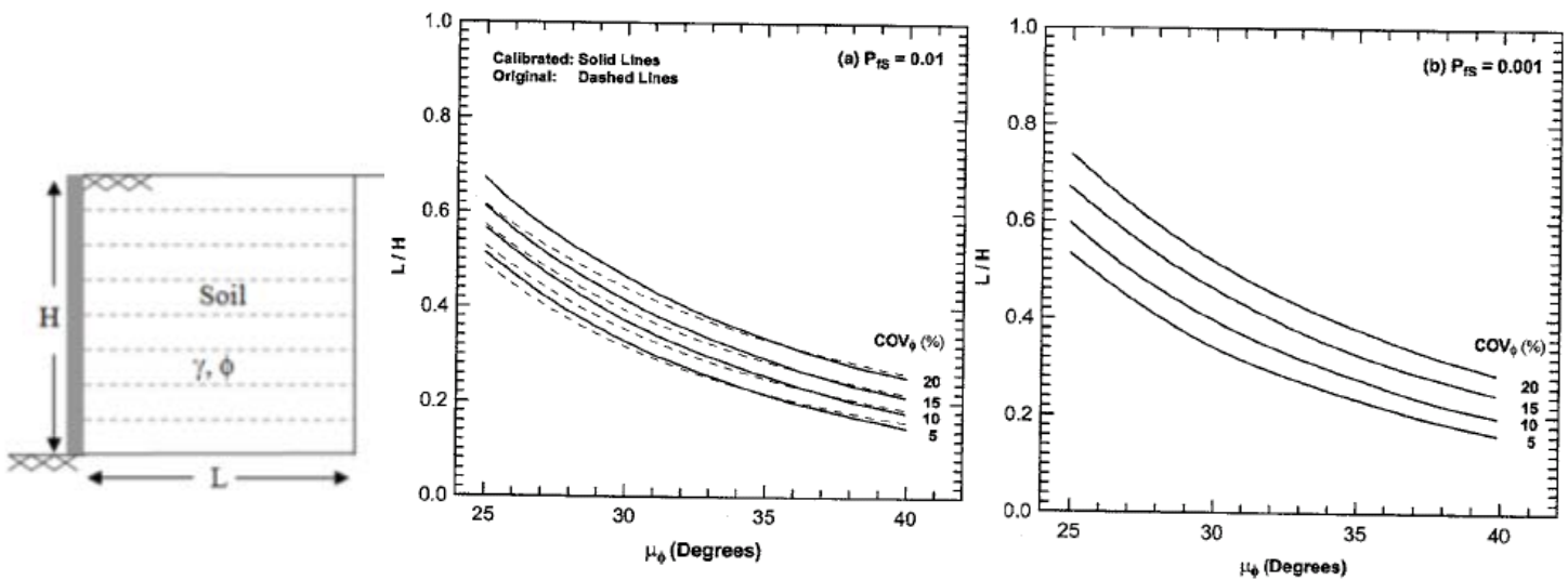
Figure 1-2 Recommended MSE wall L/H as a function of: \mu_\phi and CV_\phi for P_f of 0.01 and 0.001 (Chalermyanont and Benson, 2005)
