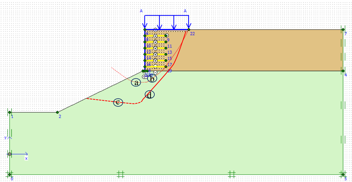
Figure 5-17 Rupture surfaces for bearing failure (points a and b) and slope failure (points c and d) superimposed to Plaxis model
