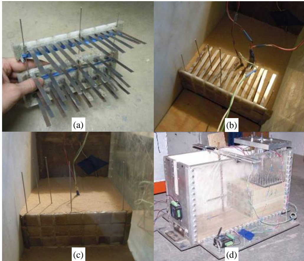
Figure 3-2 Stages of model wall: (a) segmented model wall, (b) segmented model wall during construction, (c) buried segmented model wall and (d) completed segmented model wall ready for test
