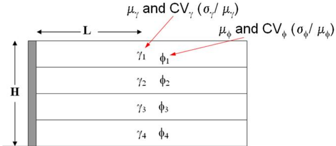
Figure 3-3 Layering process to obtain \mu and CV of backfill properties
