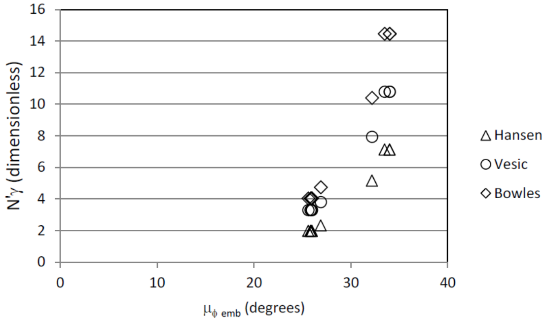
Figure 5-16 N'_\gamma values from Hansen's, Vesic's and Bowles' methods for the model tests
