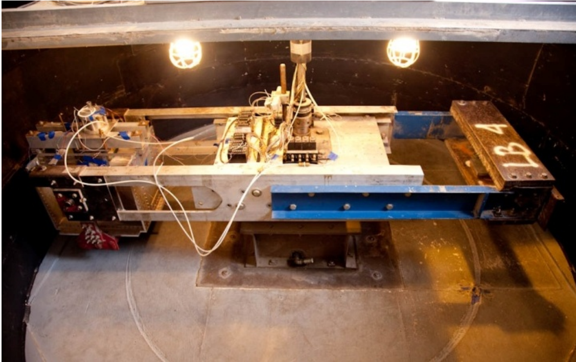
Figure 2-10 University of Florida's large geotechnical centrifuge
