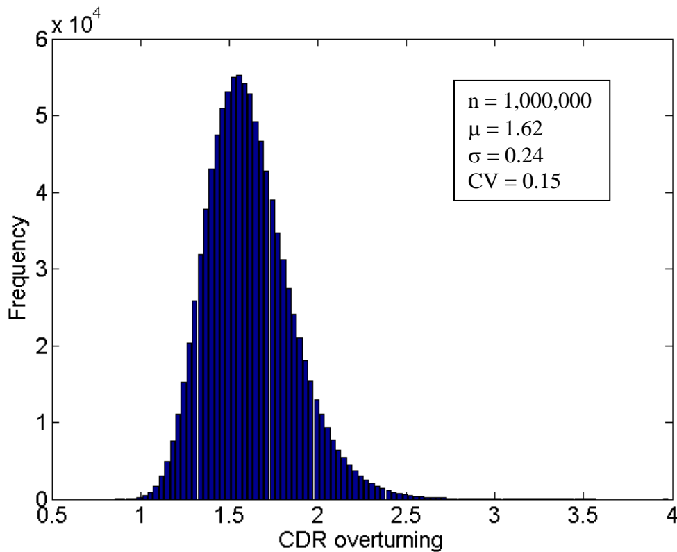
Figure 2-8 Histogram of CDR for MSE overturning
