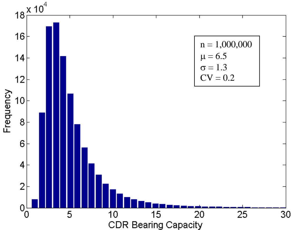
Figure 2-5 Histogram of CDR for MSE bearing capacity
