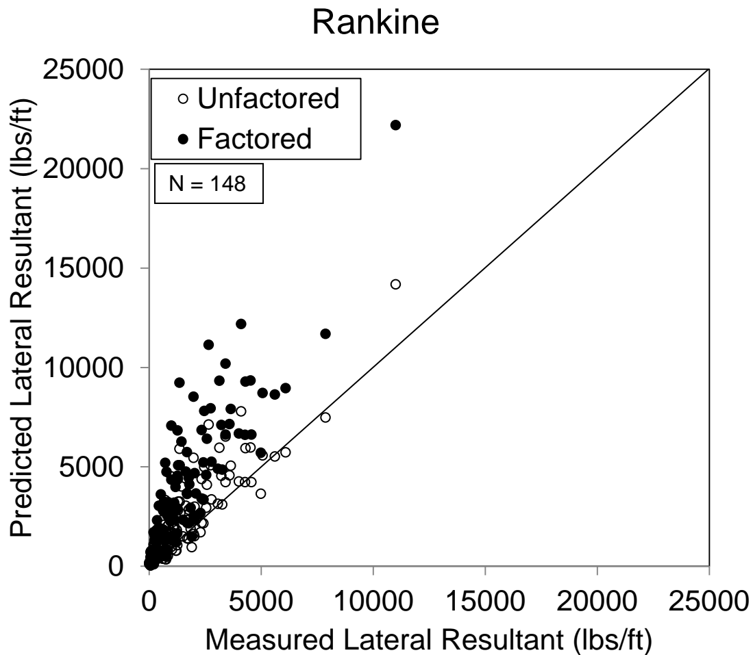
Figure 3-5 Unfactored and factored predicted lateral resultant forces versus measured lateral resultant force based on Rankine analysis
