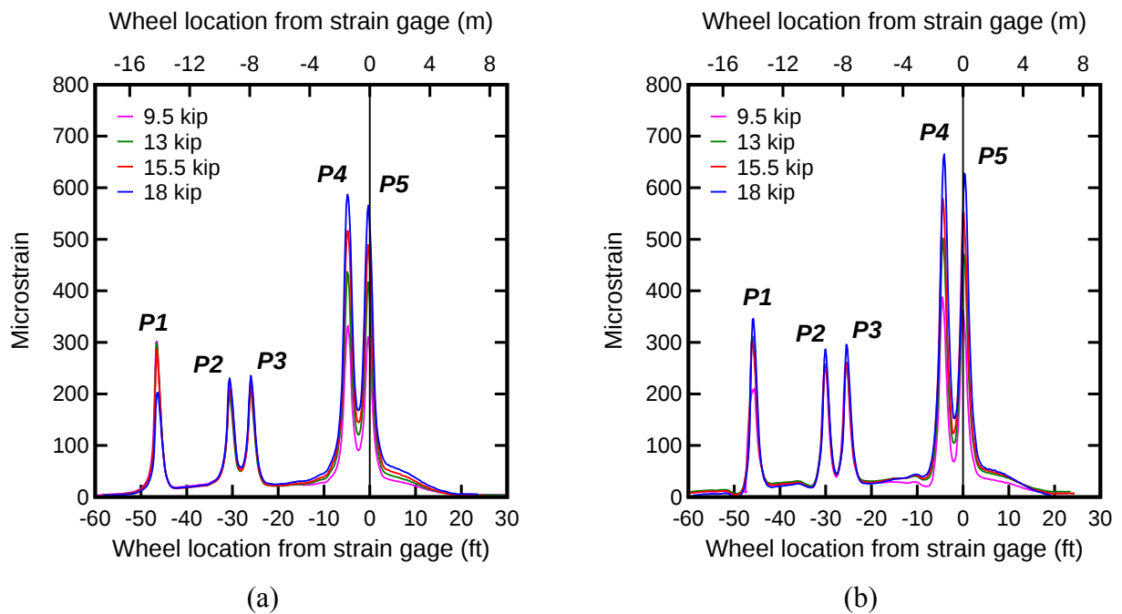
Figure 47 – Influence lines for S2 positive bending (TP1) for (a) 2009 (b) 2010
