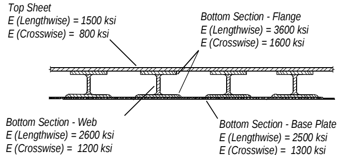
Figure 106 – GFRP deck Modulus map
