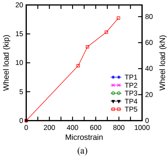
Figure 95 – Gage S3 load-strain calibration curve for (a) 2010
