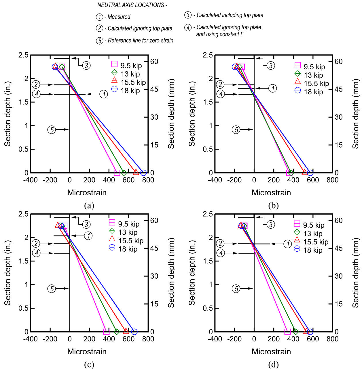
Figure 86 – Composite behavior (2009) demonstrated by (a) Maximum strain in S5 and corresponding strain in R5 (b) Minimum strain in R5 and corresponding strain in S5 (c) Maximum strain in S7 and corresponding strain in R7 (d) Minimum strain in R7 and corresponding strain in S7
