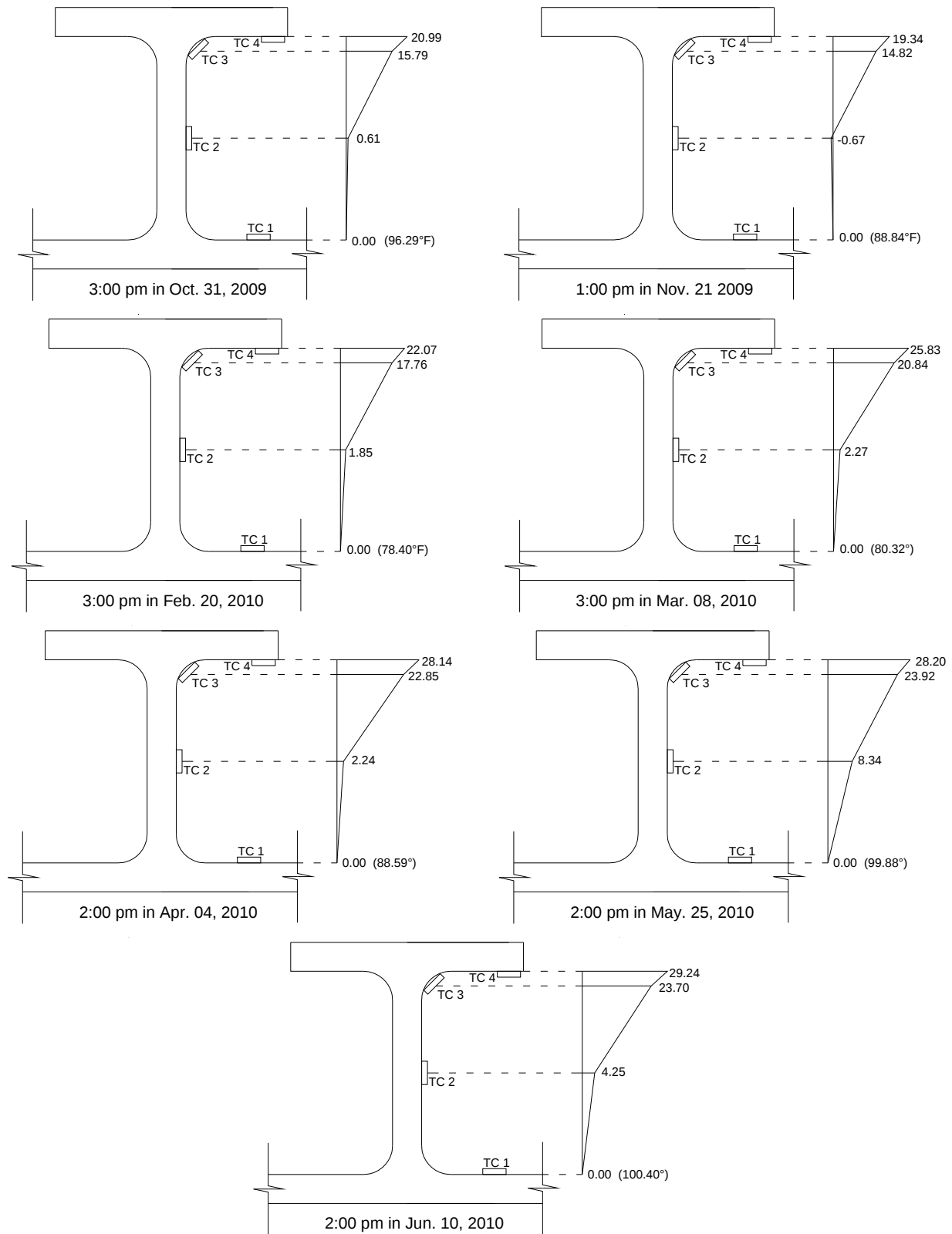
Figure 121 – Maximum thermal gradients throughout the year
