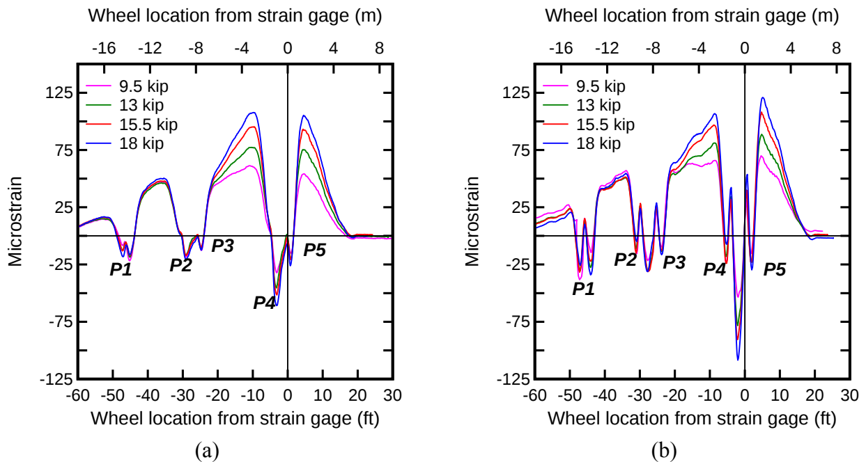
Figure 53 – Influence lines for S6 negative bending (TP1) for (a) 2009 (b) 2010
