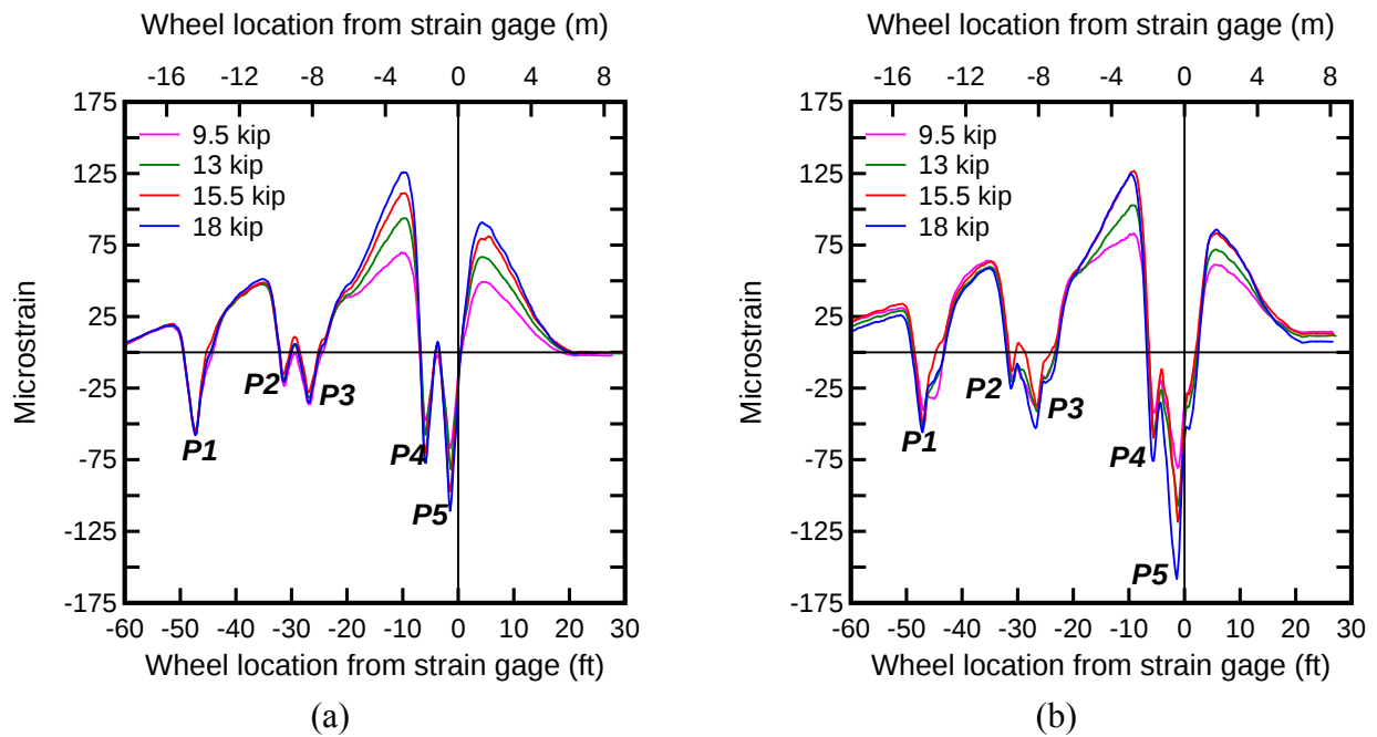
Figure 50 – Influence lines for S4 negative bending (TP5) for (a) 2009 (b) 2010
