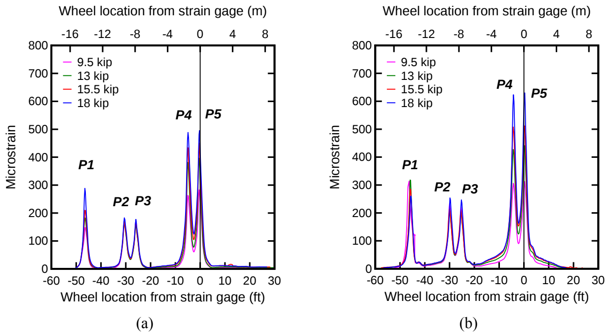
Figure 46 – Influence lines for S1 positive bending (TP1) for (a) 2009 (b) 2010
