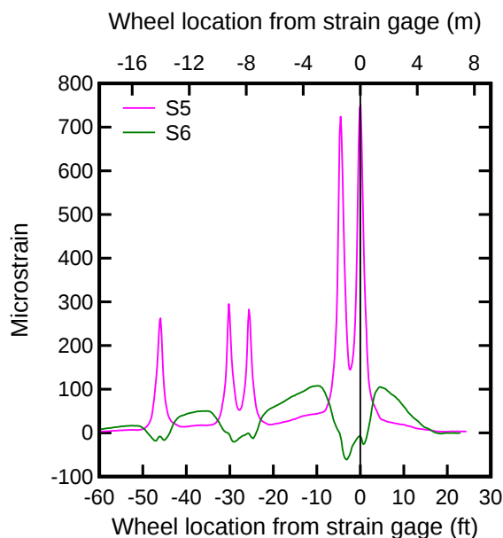
Figure 58 – Influence lines for gage S5 and S6 for TP1 (2009)
