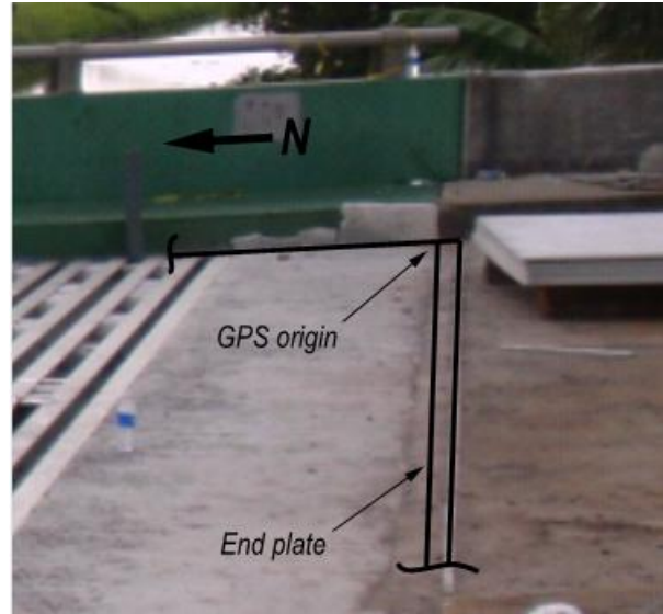
Figure 31 – Coordinate axes used for relative positioning of truck and gages
