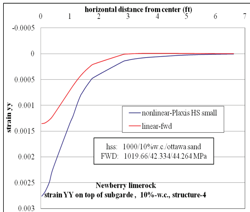
Figure D-33. \epsilon_{yy} at top of subgrade layer comparison for nonlinear and linear cases for Structure-4 with 10% w.c. base layer and nonlinear Ottawa sand subgrade.
