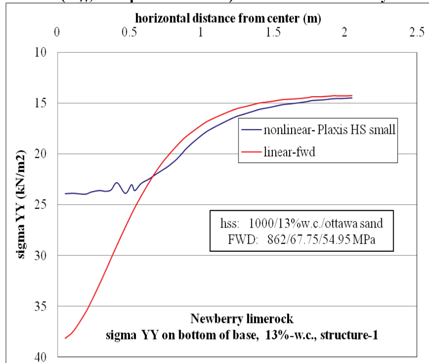
Figure D-22. \sigma_{yy} at bottom of base layer comparison for nonlinear and linear cases, for Structure-1 with 13% w.c. base layer and nonlinear Ottawa sand subgrade.
