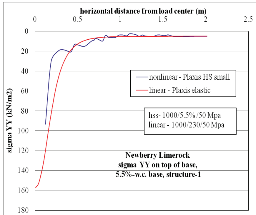
Figure C-44. \sigma_{yy} vertical stress at top of base layer comparison for nonlinear and linear cases, for Structure-1 with 5.5% w.c. base layer.
