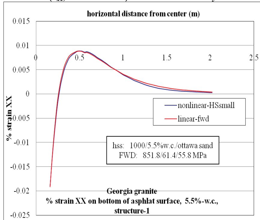
Figure D-42. \epsilon_{xx} at bottom of AC layer comparison for nonlinear and linear cases, for Structure-1 with 5.5% w.c. base layer and nonlinear Ottawa sand subgrade.
