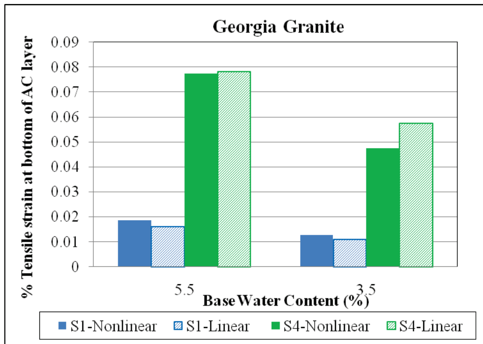
Figure 7-16. Comparison of horizontal tensile strain at bottom of AC layer for Structure 1 and Structure 4 and for different base moisture contents: (a) Newberry limerock and (b) Georgia granite.
