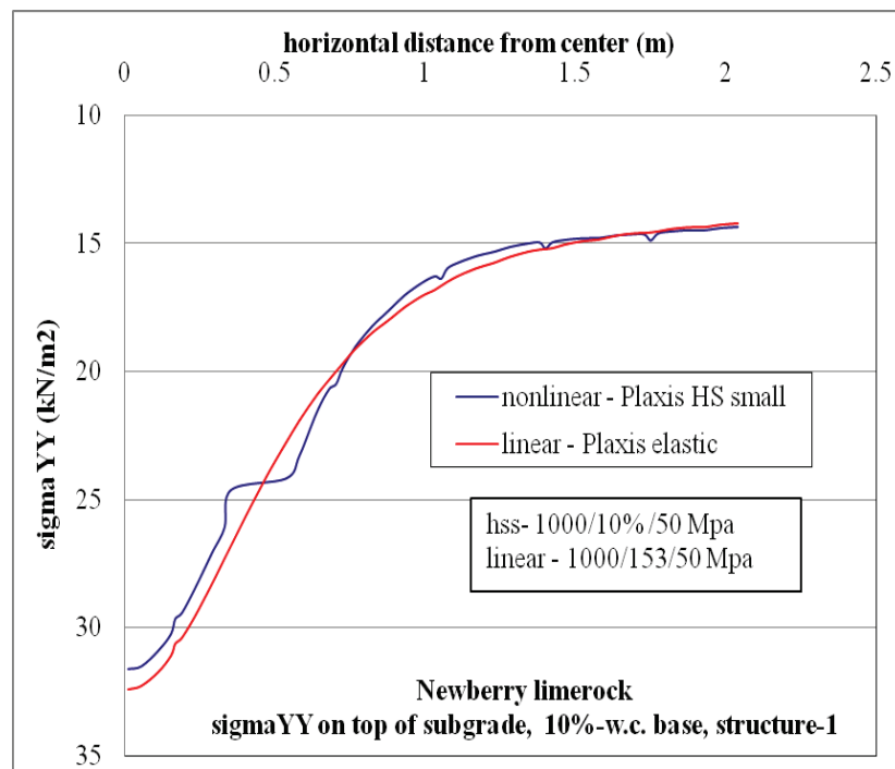
Figure C-74. \sigma_{yy} at top of subgrade comparison for nonlinear and linear cases, for Structure-1 with 10% w.c. base layer.
