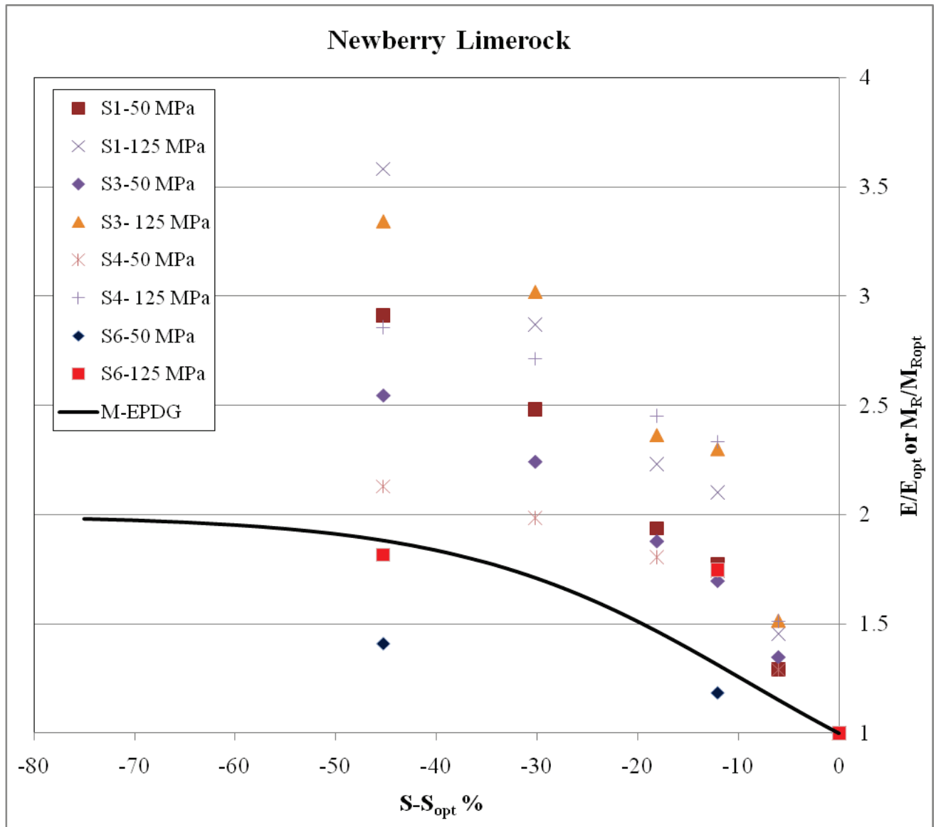
Figure 7-13. Comparison of Newberry limerock effective base moduli with MEPDG model.
