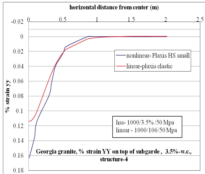
Figure C-132. \epsilon_{yy} at top of subgrade layer comparison for nonlinear and linear cases for Structure-4 with 3.5% w.c. base layer.
