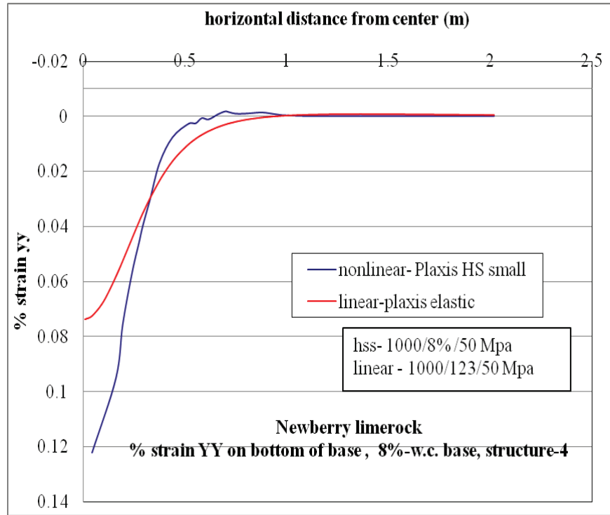
Figure C-71. \epsilon_{yy} at bottom of base layer comparison for nonlinear and linear cases, for Structure-4 with 8% w.c. base layer.
