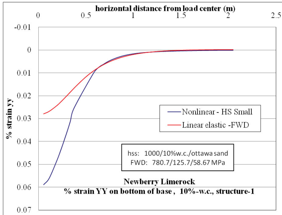
Figure D-26. \epsilon_{yy} at bottom of base layer comparison for nonlinear and linear cases, for Structure-1 with 10% w.c. base layer and nonlinear Ottawa sand subgrade.
