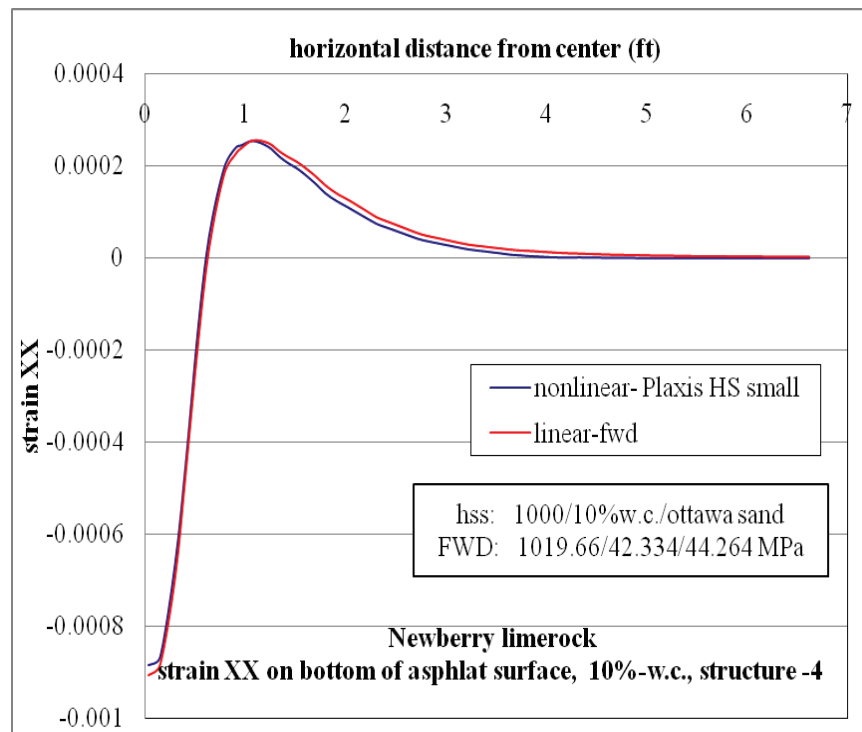
Figure D-15. \epsilon_{xx} at bottom of AC layer comparison for nonlinear and linear cases, for Structure-4 with 10% w.c. base layer and nonlinear Ottawa sand subgrade.
