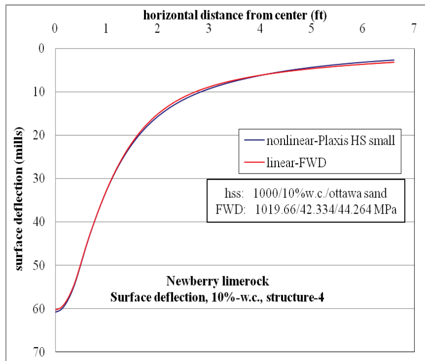
Figure D-3. Surface deflection comparison for nonlinear and linear cases, for Structure-4 with 10% w.c. base layer and nonlinear Ottawa sand subgrade.
