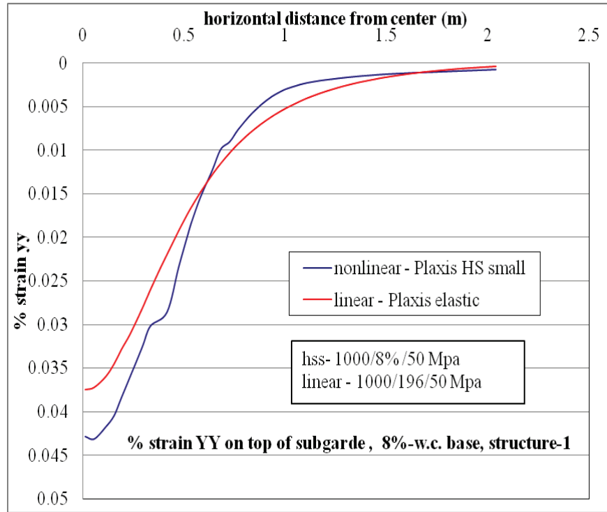
Figure C-83. \epsilon_{yy} at top of subgrade layer comparison for nonlinear and linear cases for Structure-1 with 8% w.c. base layer.
