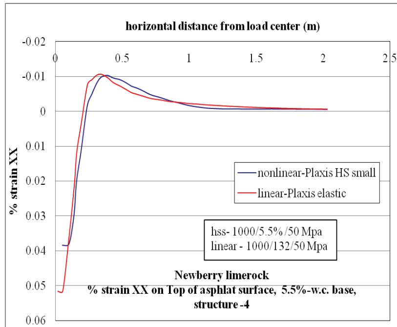
Figure C-24. \epsilon_{xx} at top of AC layer comparison for nonlinear and linear cases, for Structure-4 with 5.5% w.c. base layer.
