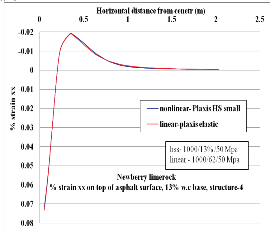
Figure C-21. \epsilon_{xx} at top of AC layer comparison for nonlinear and linear cases, for Structure-4 with 13% w.c. base layer.
