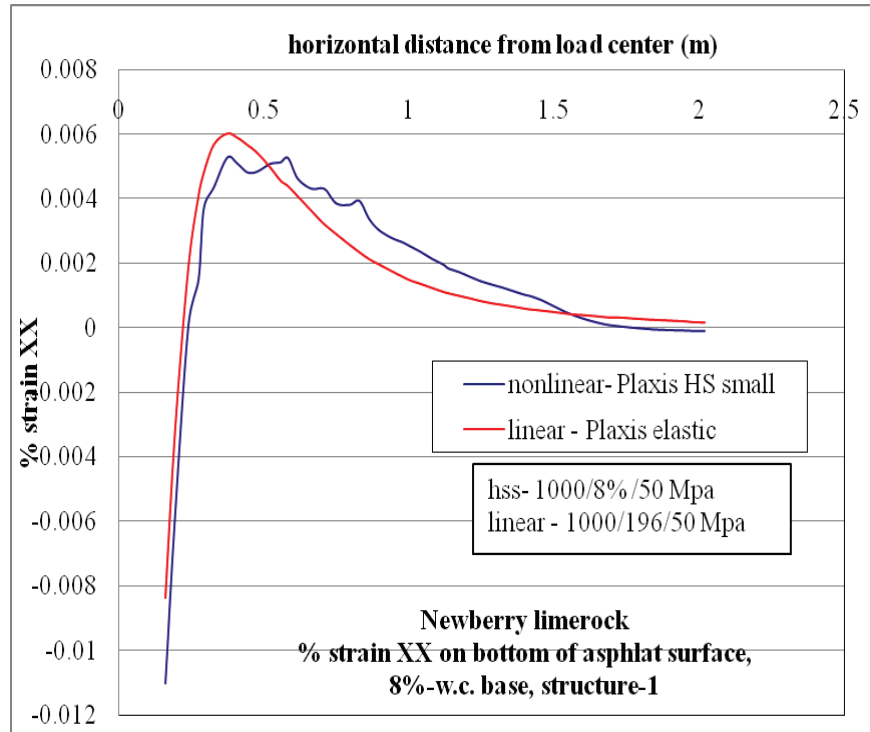
Figure C-35. \epsilon_{xx} at bottom of AC layer comparison for nonlinear and linear cases, for Structure-1 with 8% w.c. base layer.
