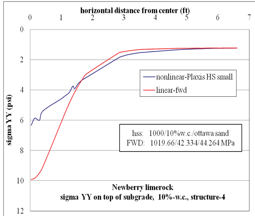
Figure D-30. \sigma_{yy} at top of subgrade comparison for nonlinear and linear cases, for Structure-4 with 10% w.c. base layer and nonlinear Ottawa sand subgrade.
