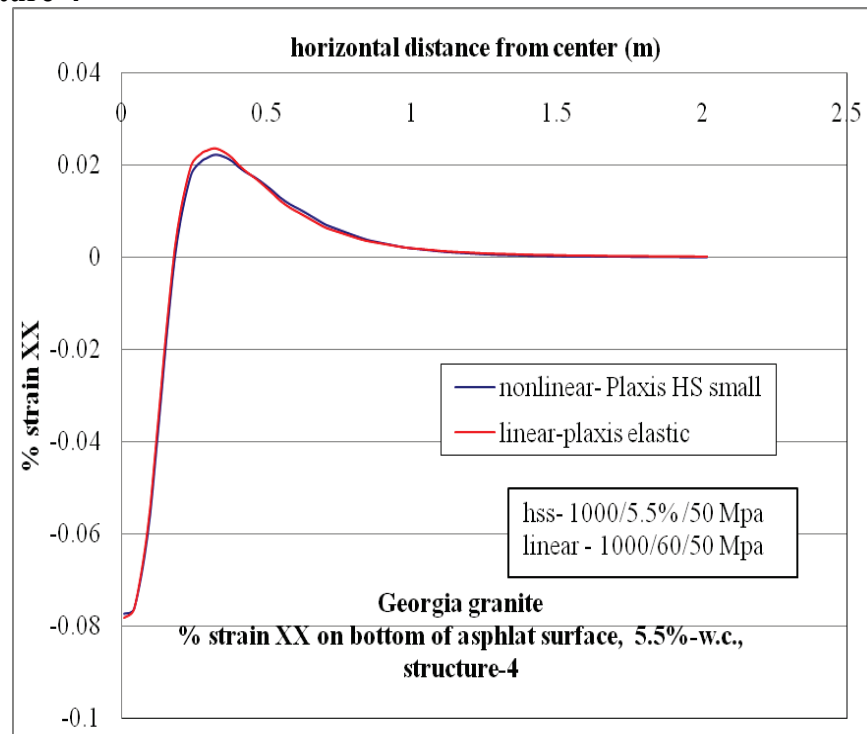
Figure C-107. \epsilon_{xx} at bottom of AC layer comparison for nonlinear and linear cases, for Structure-4 with 5.5% w.c. base layer.
