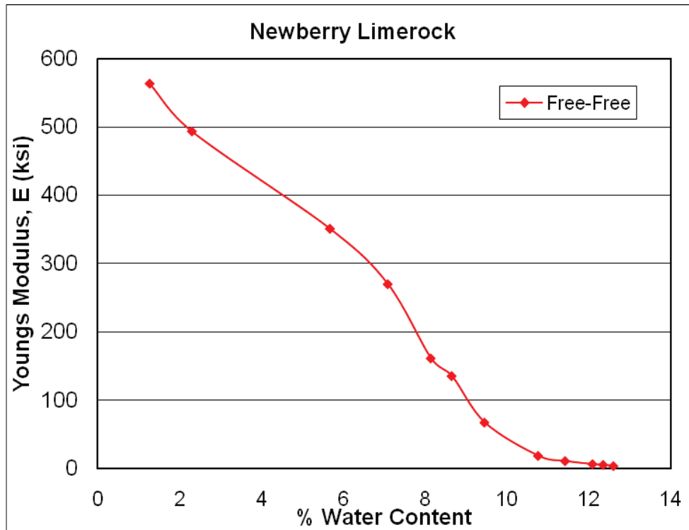
Figure 5-17. Young's modulus versus moisture content results from free-free RC test on Newberry limerock.
