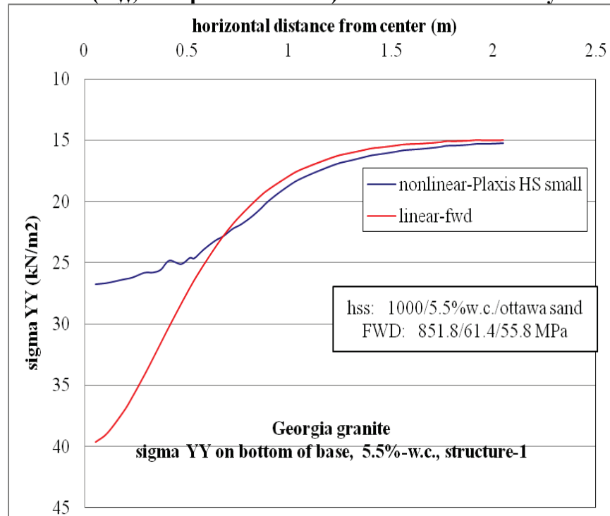
Figure D-48. \sigma_{yy} at bottom of base layer comparison for nonlinear and linear cases, for Structure-1 with 5.5% w.c. base layer and nonlinear Ottawa sand subgrade.
