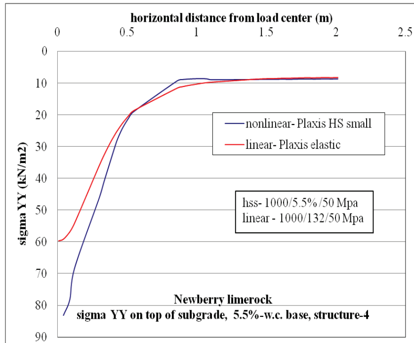
Figure C-80. \sigma_{yy} at top of subgrade comparison for nonlinear and linear cases, for Structure-4 with 5.5% w.c. base layer.
