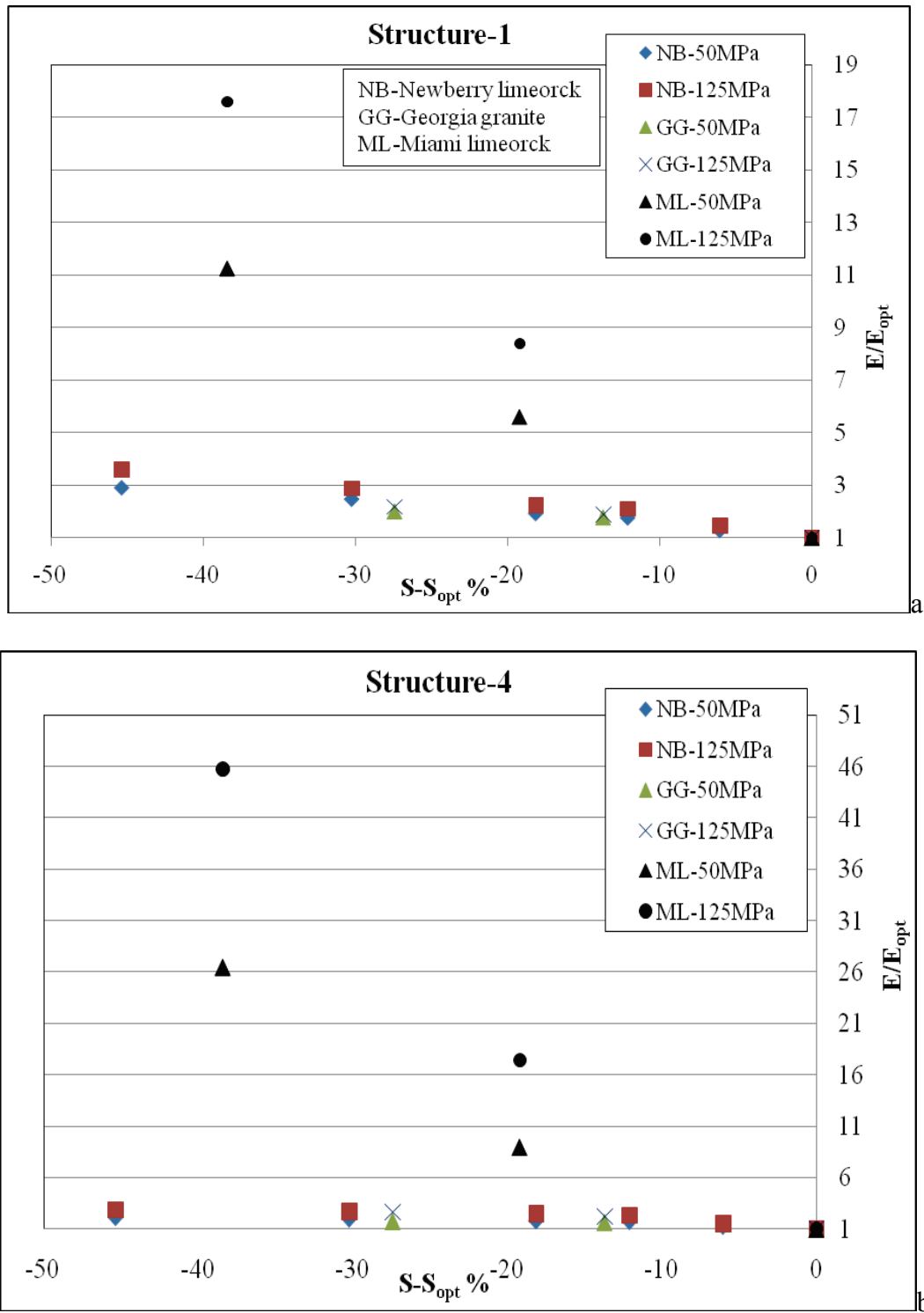
Figure 7-12. Comparison of normalized effective moduli of all three materials with subgrade moduli of 50 MPa and 125 MPa and for: (a) Structure 1 and (b) Structure 4.
