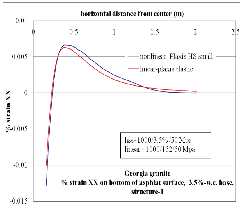
Figure C-106. \epsilon_{xx} at bottom of AC layer comparison for nonlinear and linear cases, for Structure-1 with 3.5% w.c. base layer.
