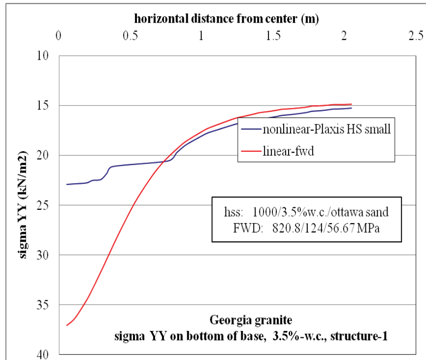
Figure D-49. \sigma_{yy} at bottom of base layer comparison for nonlinear and linear cases, for Structure-1 with 3.5% w.c. base layer and nonlinear Ottawa sand subgrade.
