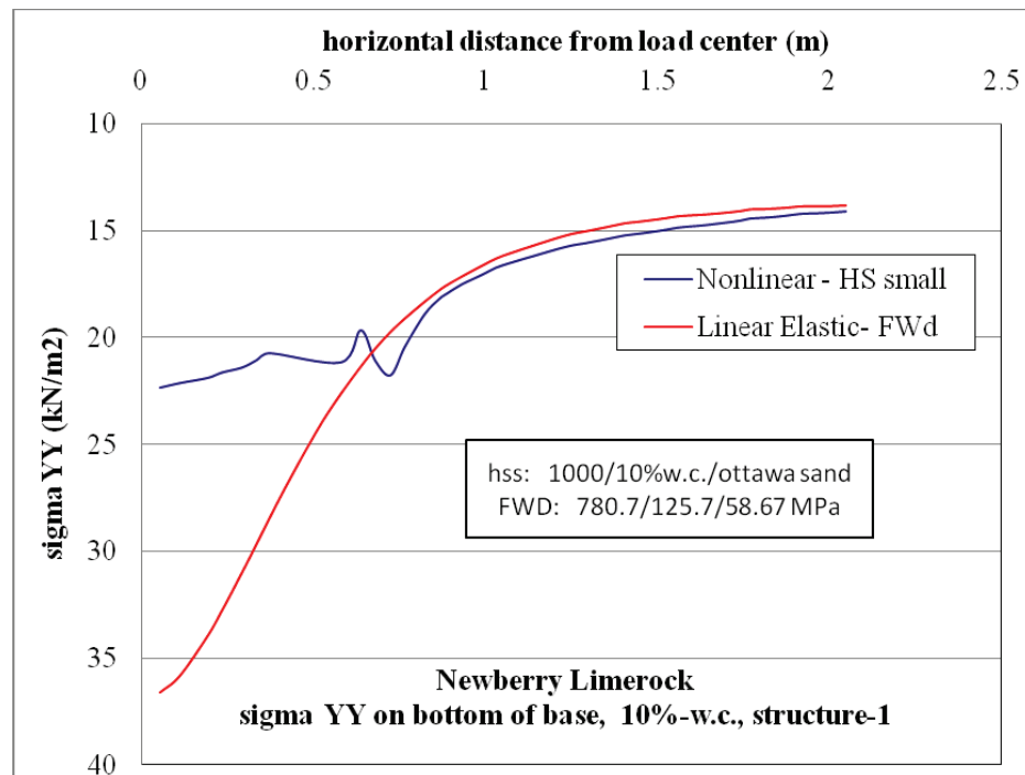
Figure D-23. \sigma_{yy} at bottom of base layer comparison for nonlinear and linear cases, for Structure-1 with 10% w.c. base layer and nonlinear Ottawa sand subgrade.
