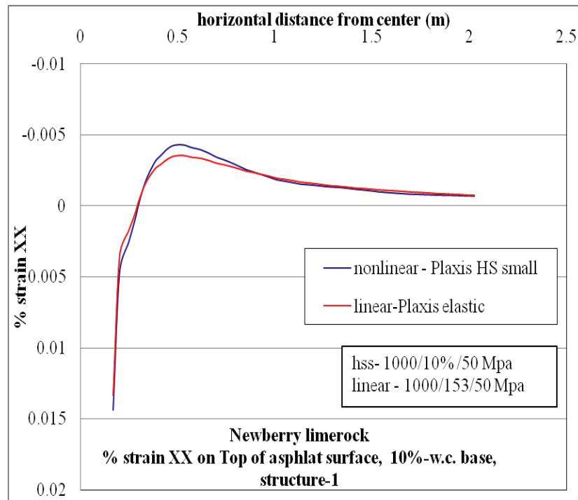
Figure C-18. \epsilon_{xx} at top of AC layer comparison for nonlinear and linear cases, for Structure-1 with 10% w.c. base layer.
