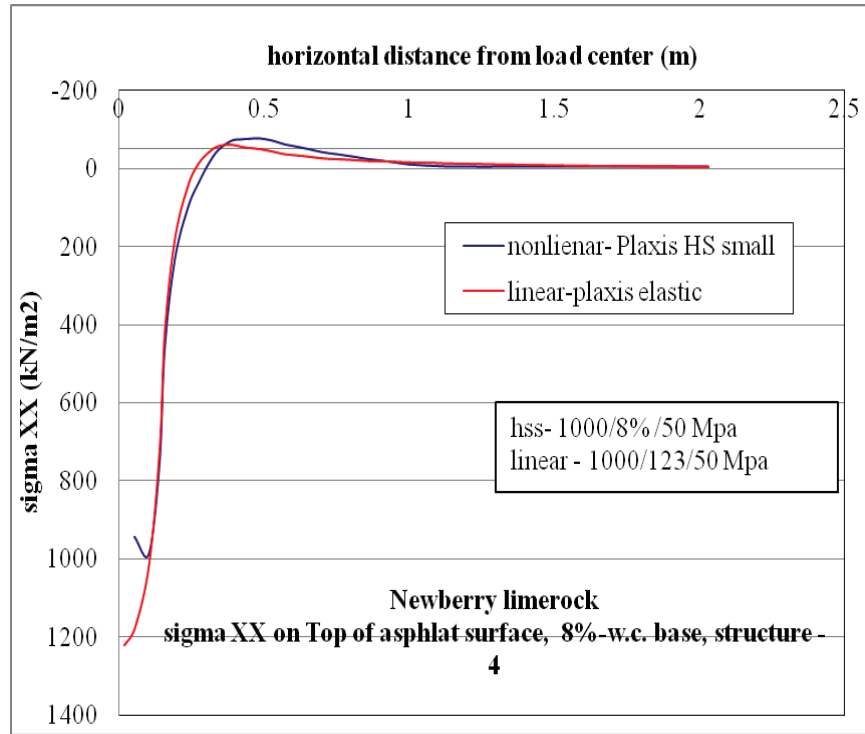
Figure C-15. \sigma_{xx} at top of AC layer comparison for nonlinear and linear cases, for Structure-4 with 8% w.c. base layer.
