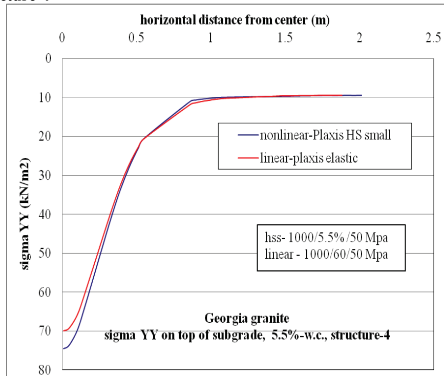
Figure C-127. \sigma_{yy} at top of subgrade layer comparison for nonlinear and linear cases, for Structure-4 with 5.5% w.c. base layer.
