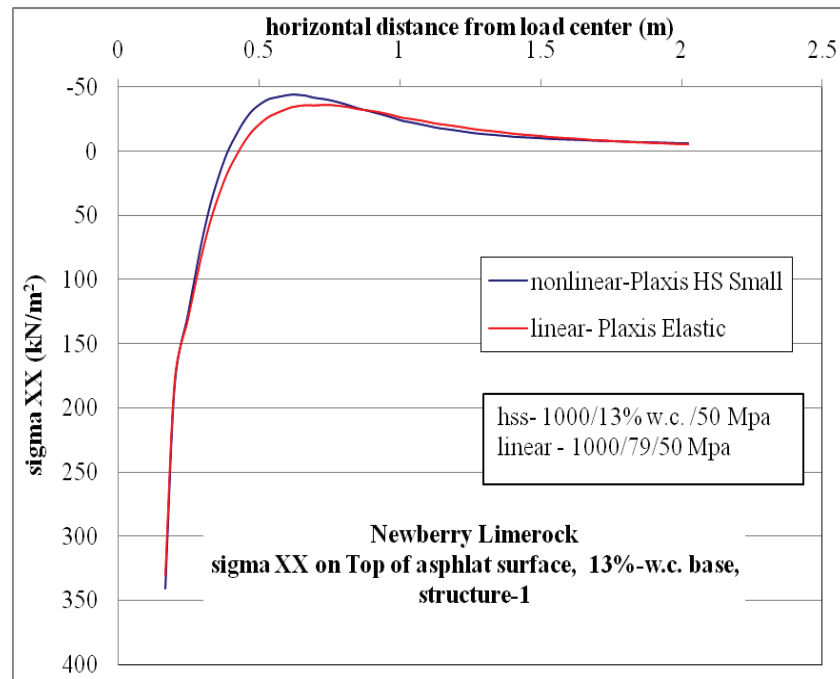
Figure C-9. \sigma_{xx} at top of AC layer comparison for nonlinear and linear cases, for Structure-1 with 13% w.c. base layer.
