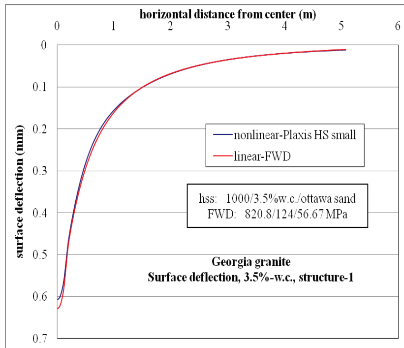
Figure D-35. Surface deflection comparison for nonlinear and linear cases, for Structure-1 with 3.5% w.c. base layer and nonlinear Ottawa sand subgrade.
