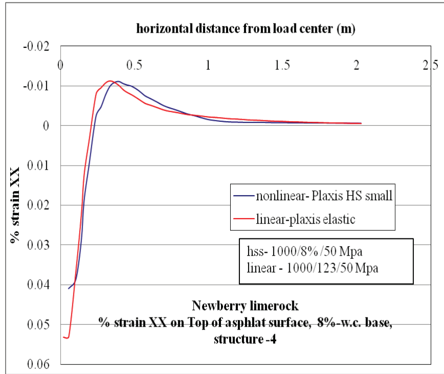
Figure C-23. \epsilon_{xx} at top of AC layer comparison for nonlinear and linear cases, for Structure-4 with 8% w.c. base layer.
