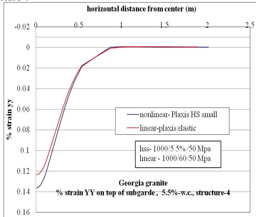
Figure C-131. \epsilon_{yy} at top of subgrade layer comparison for nonlinear and linear cases for Structure-4 with 5.5% w.c. base layer.
