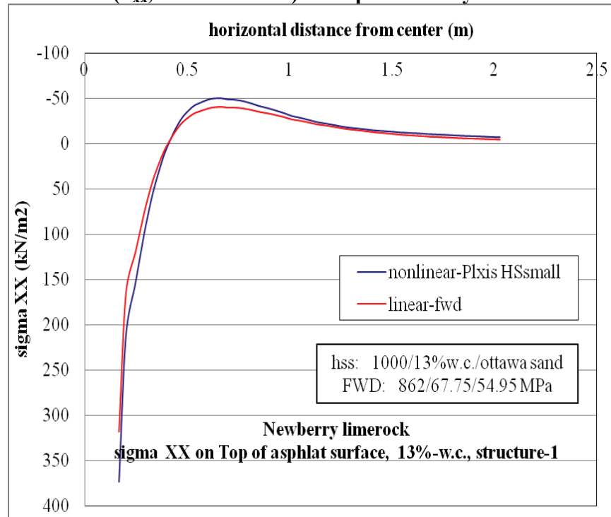
Figure D-4. \sigma_{xx} at top of AC layer comparison for nonlinear and linear cases, for Structure-1 with 13% w.c. base layer and nonlinear Ottawa sand subgrade.
