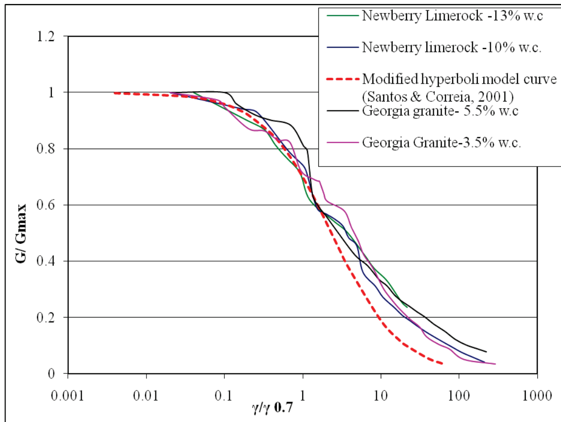
Figure 6-3. Comparison of Newberry limerock and Georgia granite data with Santos and Correia (2001) modified hyperbolic curve.
