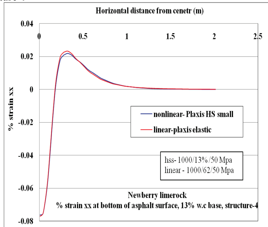
Figure C-37. \epsilon_{xx} at bottom of AC layer comparison for nonlinear and linear cases, for Structure-4 with 13% w.c. base layer.
