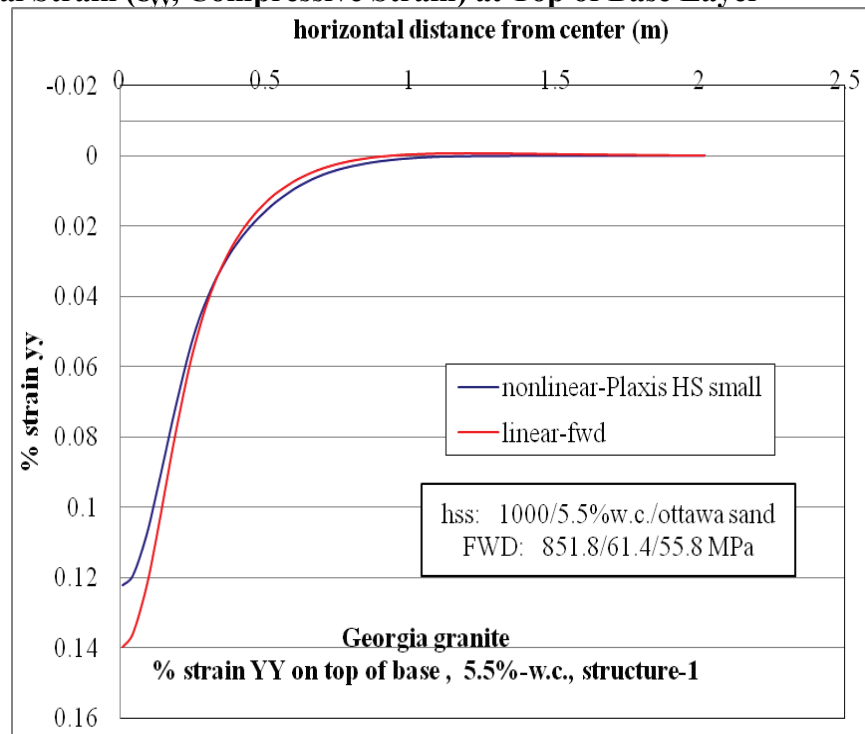
Figure D-46. \epsilon_{yy} at top of base layer comparison for nonlinear and linear cases, for Structure-1 with 5.5% w.c. base layer and nonlinear Ottawa sand subgrade.
