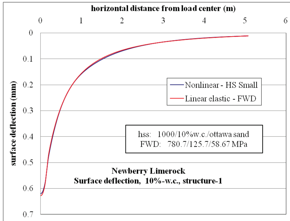
Figure 8-2. Nonlinear and linear surface deflections for Structure 1 with 10% moisture base and Ottawa sand subgrade.
