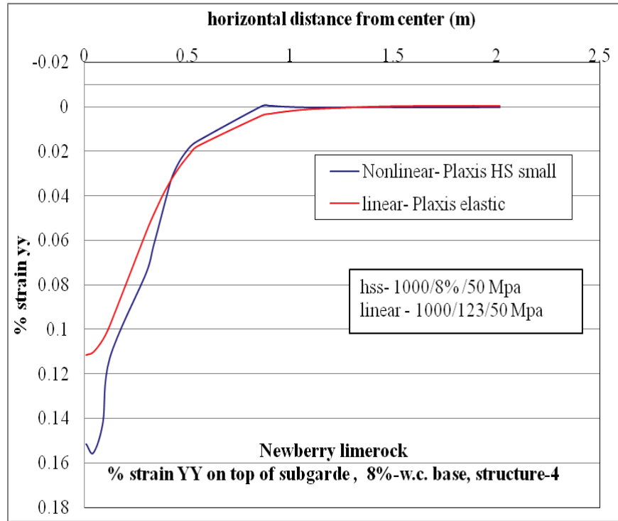
Figure C-87. \epsilon_{yy} at top of subgrade layer comparison for nonlinear and linear cases for Structure-4 with 8% w.c. base layer.
