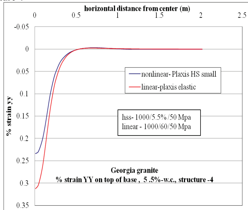
Figure C-115. \epsilon_{yy} at top of base layer comparison for nonlinear and linear cases, for Structure-4 with 5.5% w.c. base layer.
