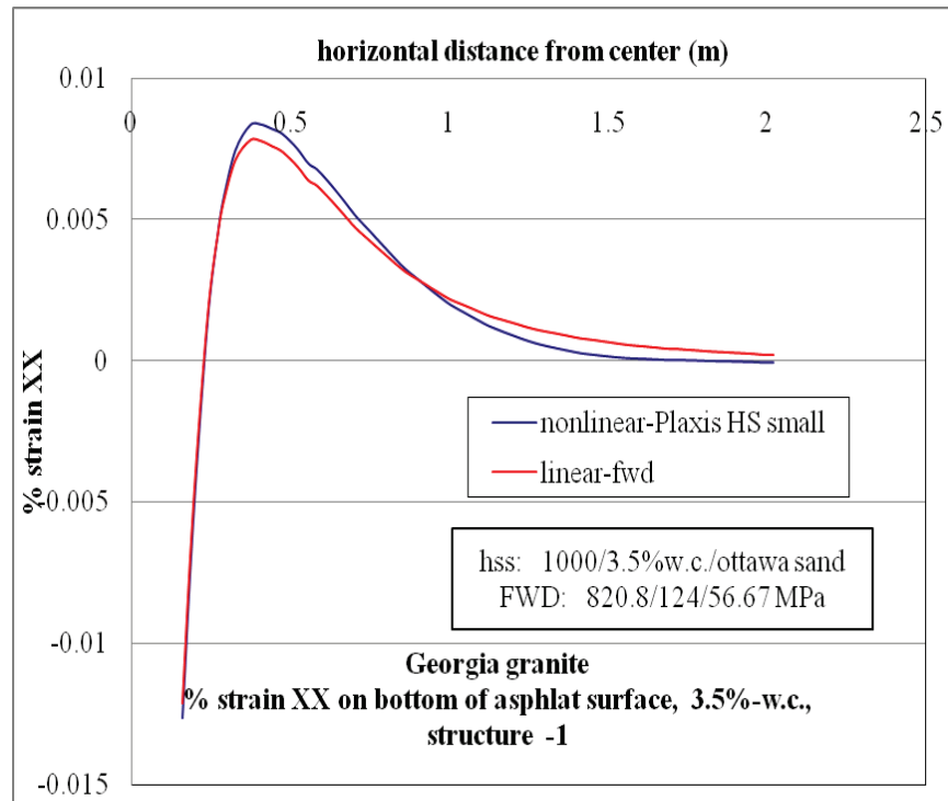
Figure D-43. \epsilon_{xx} at bottom of AC layer comparison for nonlinear and linear cases, for Structure-1 with 3.5% w.c. base layer and nonlinear Ottawa sand subgrade.
