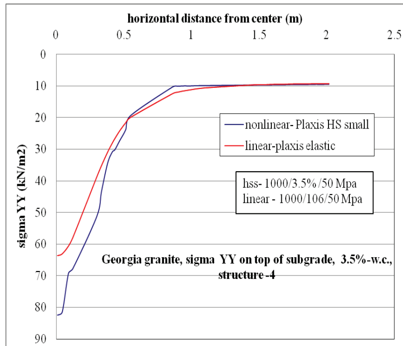
Figure C-128. \sigma_{yy} at top of subgrade layer comparison for nonlinear and linear cases for Structure-4 with 3.5% w.c. base layer.
