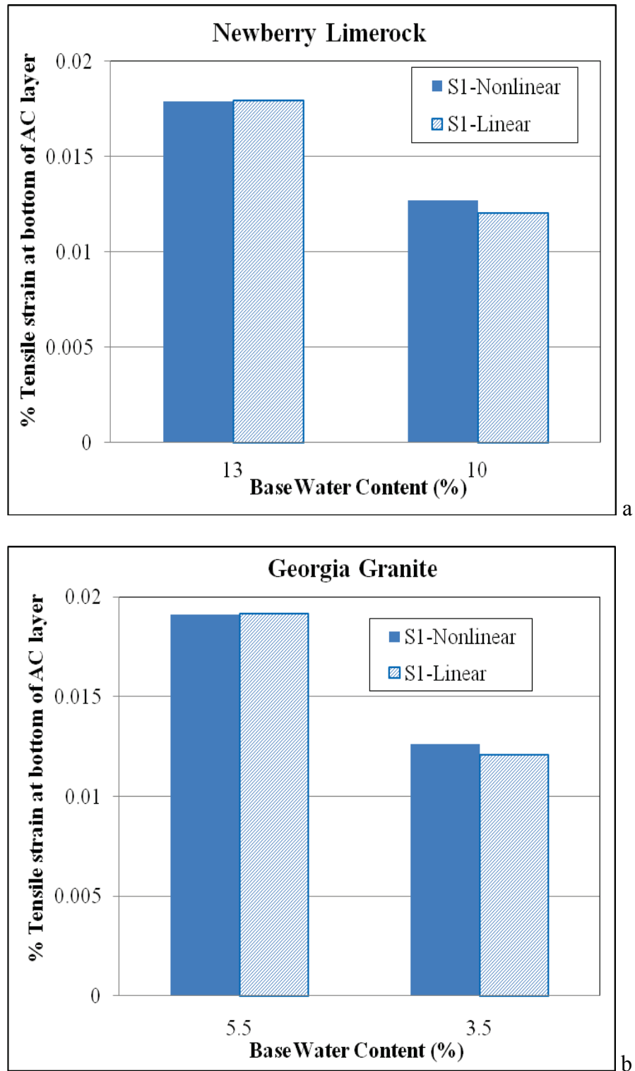
Figure 8-3. Horizontal tensile strain at bottom of AC layer of Structure 1 with Ottawa sand subgrade and two base moisture contents for: (a) Newberry limerock and (b) Georgia granite.
