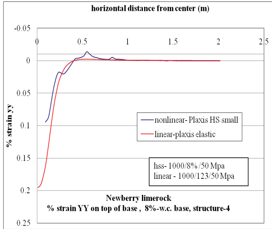
Figure C-55. \epsilon_{yy} at top of base layer comparison for nonlinear and linear cases, for Structure-4 with 8% w.c. base layer.
