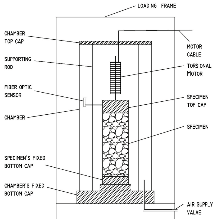
Figure 3-3. Fixed-free RC equipment.
