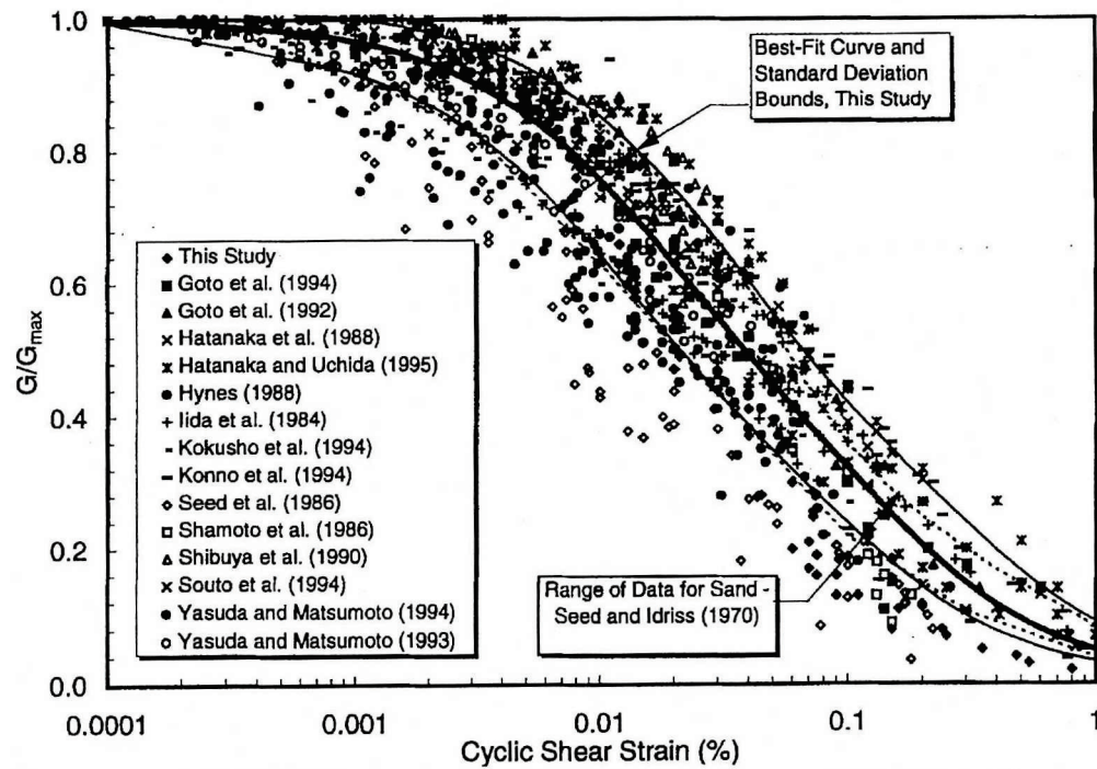
Figure 2-10. Data points defining G/G_{max} versus \gamma relationship for gravelly soils based on testing by all 15 investigators along with best-fit curve and \pm one standard deviation bounds for entire data set (from Rollins et al., 1998).
