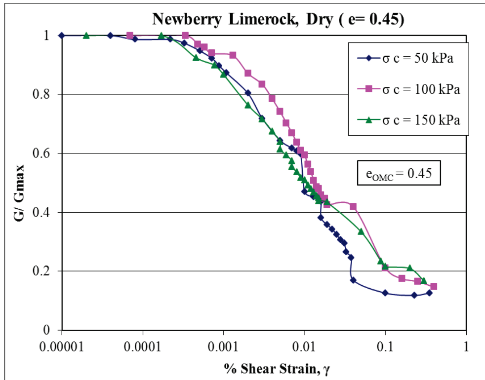
Figure 5-3. G/G_{max} versus shear strain ( \gamma ) curves at e = e_{OMC} for Newberry limerock.
