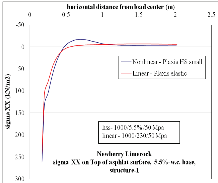
Figure C-12. \sigma_{xx} at top of AC layer comparison for nonlinear and linear cases, for Structure-1 with 5.5% w.c. base layer.
