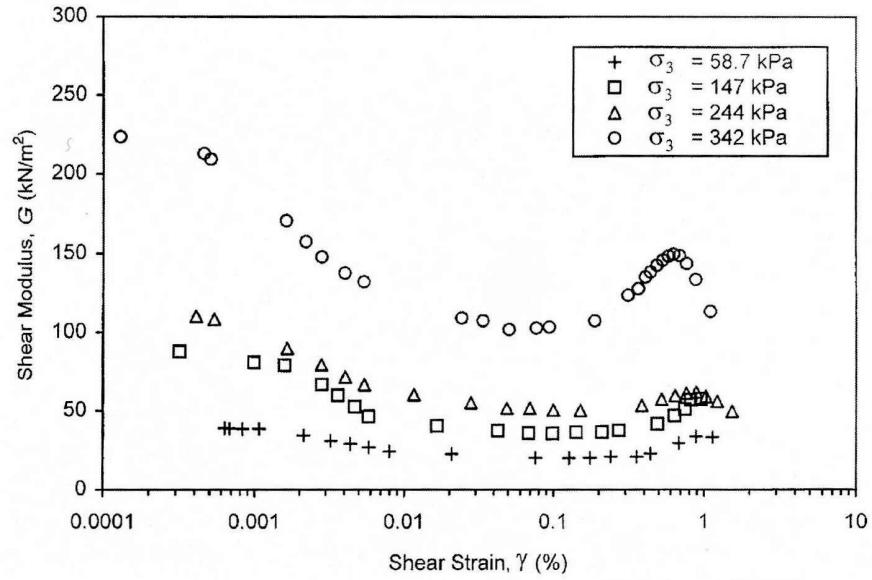
Figure 2-4. Effect of \sigma_3 on the G - \gamma relationship ( d_{\max} = 1.27 cm) (from Lin et al., 2000).
