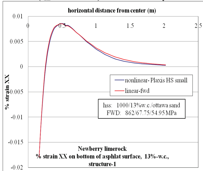
Figure D-13. \epsilon_{xx} at bottom of AC layer comparison for nonlinear and linear cases, for Structure-1 with 13% w.c. base layer and nonlinear Ottawa sand subgrade.
