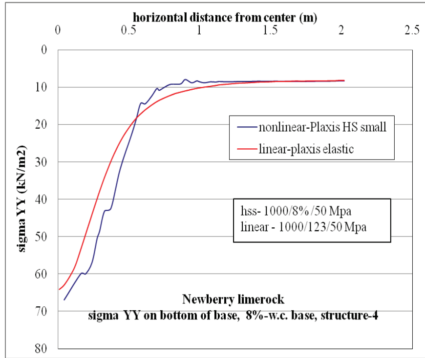
Figure C-63. \sigma_{yy} at bottom of base layer comparison for nonlinear and linear cases, for Structure-4 with 8% w.c. base layer.
