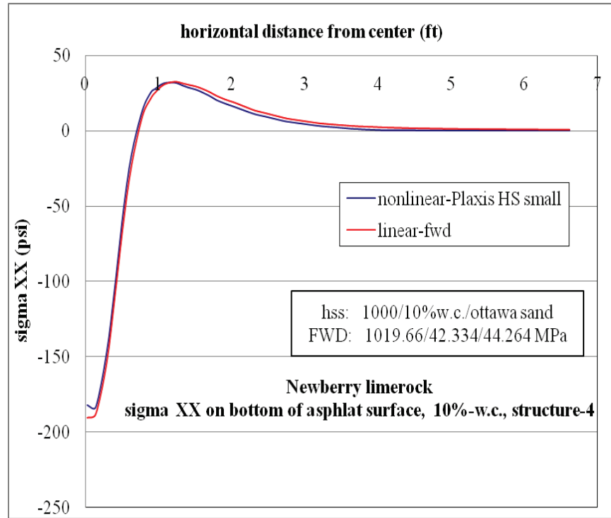
Figure D-12. \sigma_{xx} at bottom of AC layer comparison for nonlinear and linear cases, for Structure-4 with 10% w.c. base layer and nonlinear Ottawa sand subgrade.
