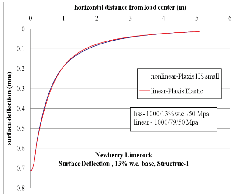
Figure C-1. Surface deflection comparison for nonlinear and linear cases, for Structure-1 with 13% w.c. base layer.
