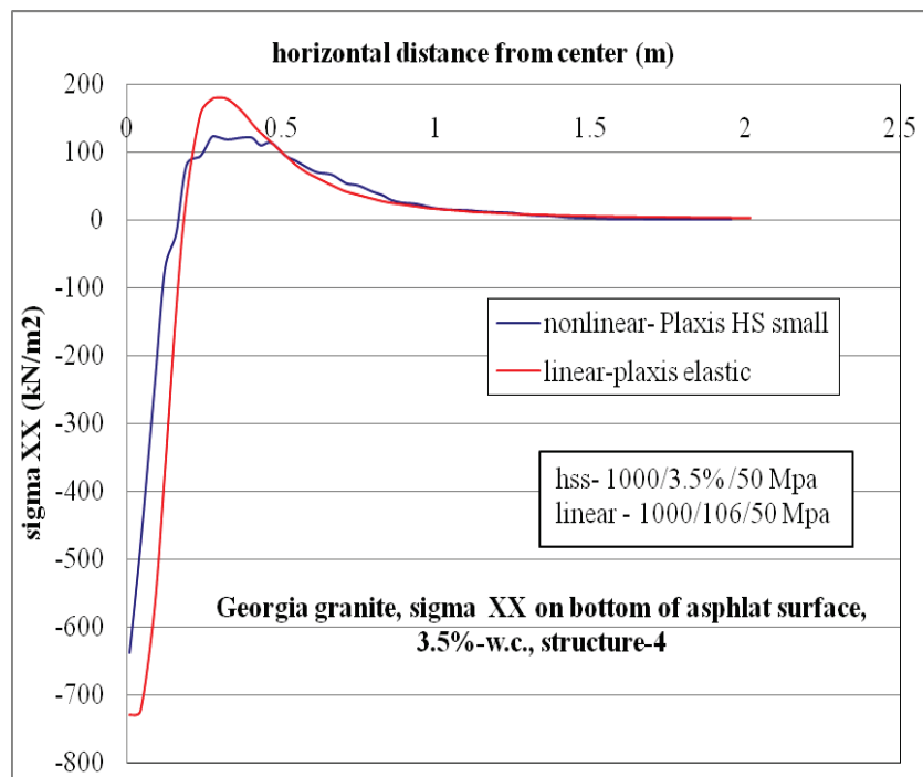
Figure C-104. \sigma_{xx} at bottom of AC layer comparison for nonlinear and linear cases, for Structure-4 with 3.5% w.c. base layer.
