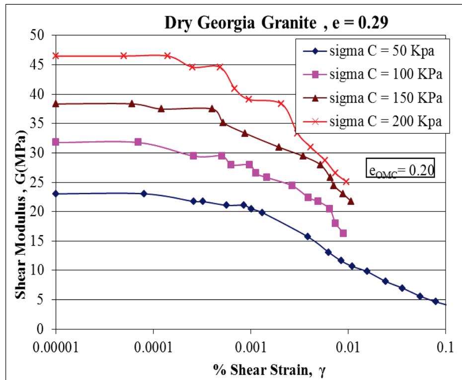
Figure A-6. Shear Modulus (G) versus % Shear strain ( \gamma ) curves for dry Georgia granite at e=0.29 .
