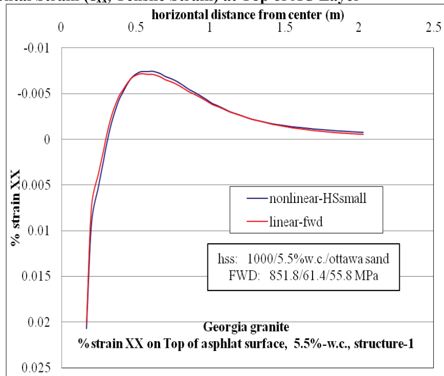
Figure D-38. \epsilon_{xx} at top of AC layer comparison for nonlinear and linear cases, for Structure-1 with 5.5% w.c. base layer and nonlinear Ottawa sand subgrade.
