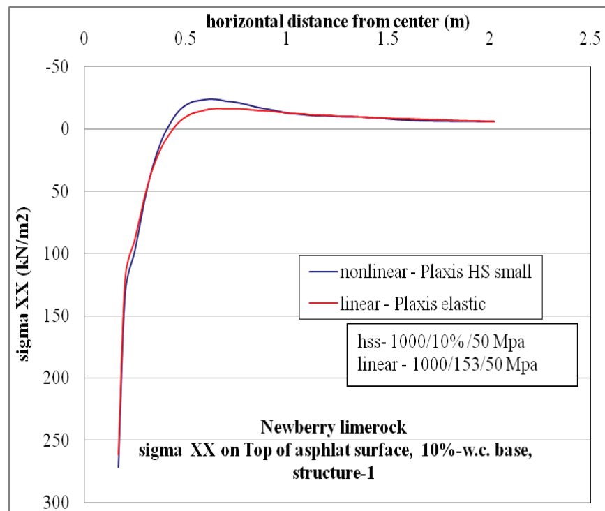
Figure C-10. \sigma_{xx} at top of AC layer comparison for nonlinear and linear cases, for Structure-1 with 10% w.c. base layer.
