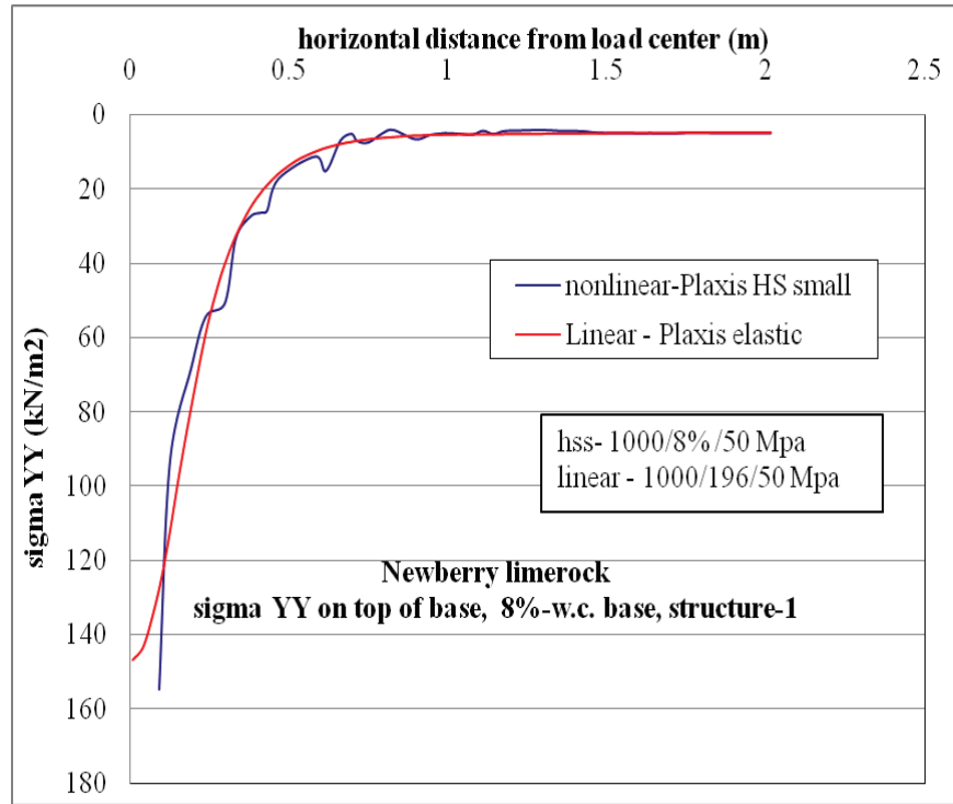
Figure C-43. \sigma_{yy} vertical stress at top of base layer comparison for nonlinear and linear cases, for Structure-1 with 8% w.c. base layer.
