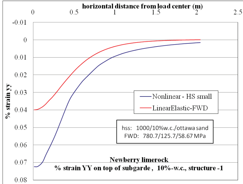
Figure D-32. \epsilon_{yy} at top of subgrade layer comparison for nonlinear and linear cases for Structure-1 with 10% w.c. base layer and nonlinear Ottawa sand subgrade.
