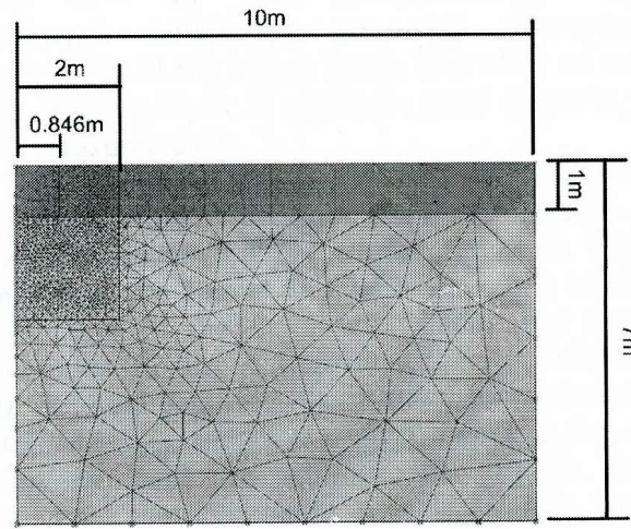
Figure 6-6. Finite element mesh used for model recalibration analysis (footing 1 from Lehane et al., 2008).
