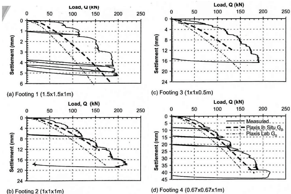
Figure 2-20. Comparison of measured foundation load settlement response at Shenton Park to prediction using Plaxis-HSsmall model (from Lehane et al., 2008).
