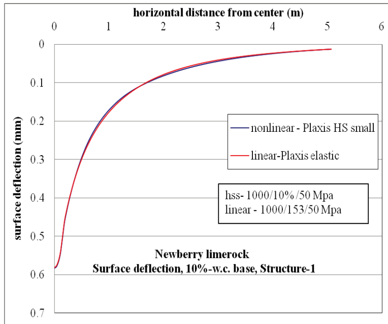
Figure C-2 Surface deflection comparison for nonlinear and linear cases, for Structure-1 with 10% w.c. base layer.
