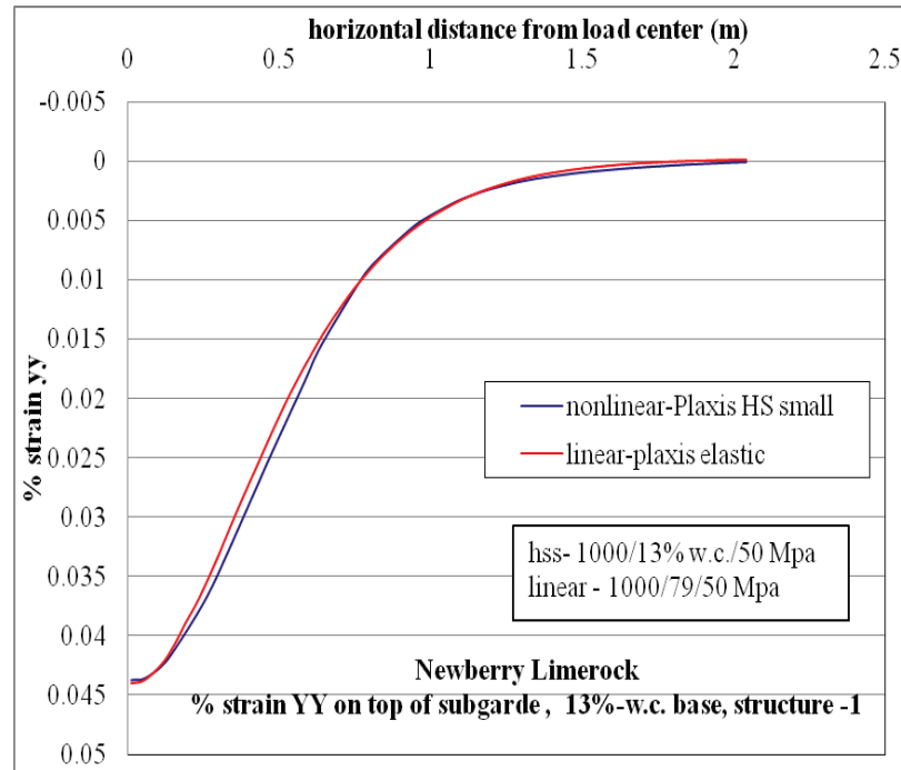
Figure C-81. \epsilon_{yy} at top of subgrade layer comparison for nonlinear and linear cases for Structure-1 with 13% w.c. base layer.
