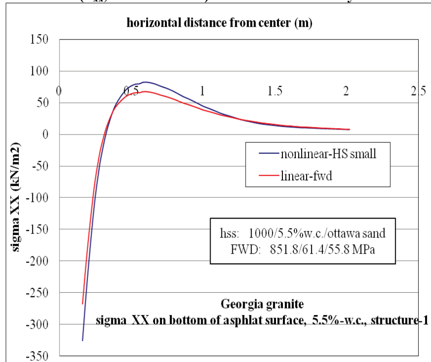
Figure D-40. \sigma_{xx} at bottom of AC layer comparison for nonlinear and linear cases, for Structure-1 with 5.5% w.c. base layer and nonlinear Ottawa sand subgrade.
