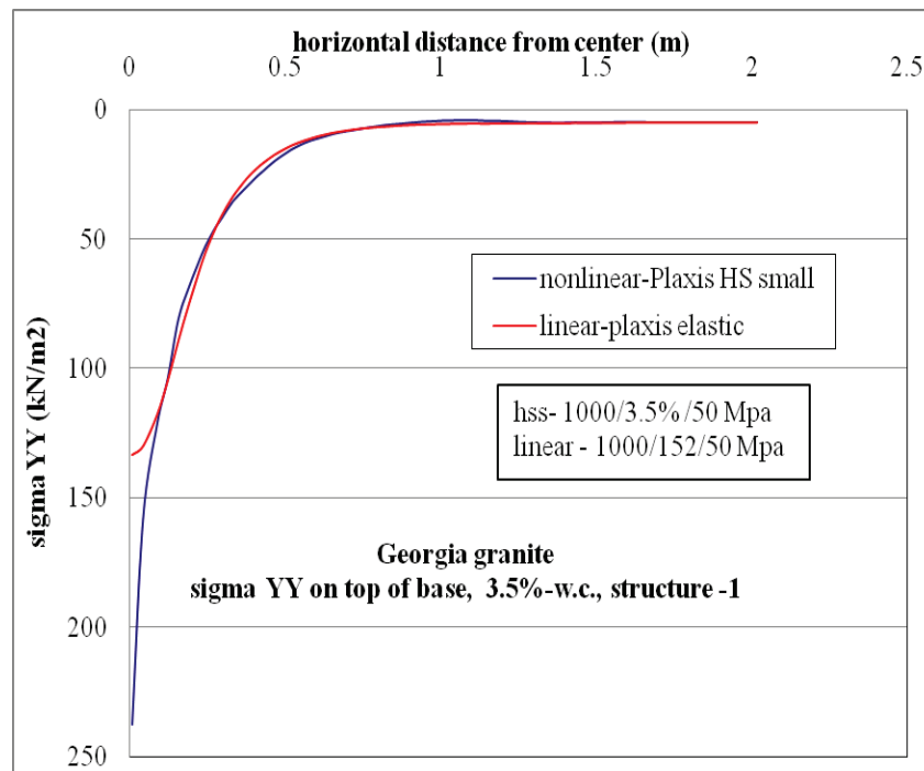
Figure C-110. \sigma_{yy} vertical stress at top of base layer comparison for nonlinear and linear cases, for Structure-1 with 3.5% w.c. base layer.
