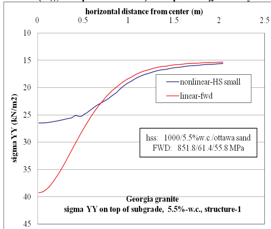
Figure D-52. \sigma_{yy} at top of subgrade comparison for nonlinear and linear cases, for Structure-1 with 5.5% w.c. base layer and nonlinear Ottawa sand subgrade.
