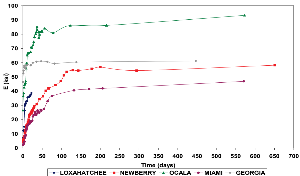
Figure 2-15. FFRC test results of specimen exposed to constant moisture (from Toros, 2008).
