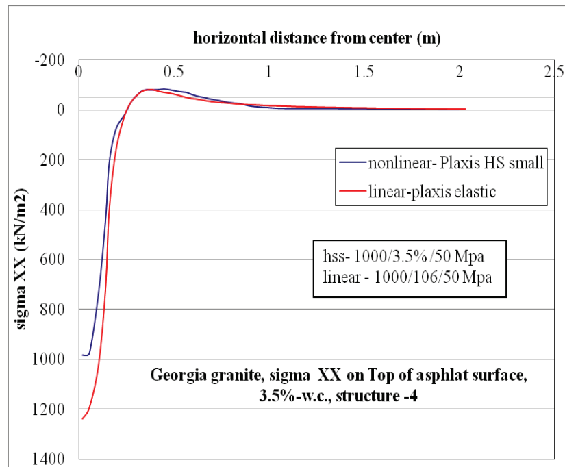
Figure C-96. \sigma_{XX} at top of AC layer comparison for nonlinear and linear cases, for Structure-4 with 3.5% w.c. base layer.
