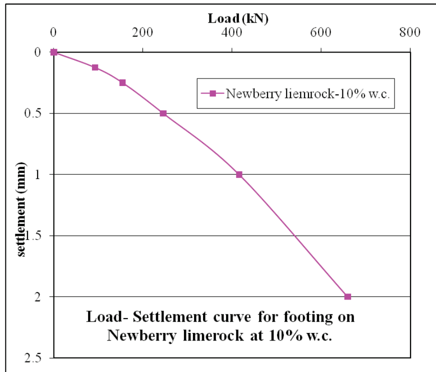
Figure 6-9. Load versus settlement curve to demonstrate material input parameters nonlinearity.
