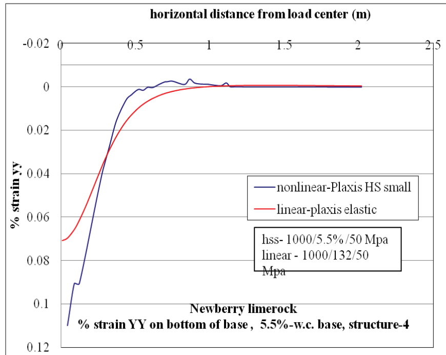
Figure C-72. \epsilon_{yy} at bottom of base layer comparison for nonlinear and linear cases, for Structure-4 with 5.5% w.c. base layer.
