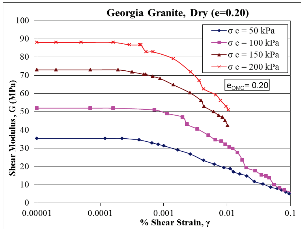
Figure 5-2. Shear modulus ( G ) versus shear strain ( \gamma ) curves for dry Georgia granite at e_{OMC} (i.e., e=0.20 ).
