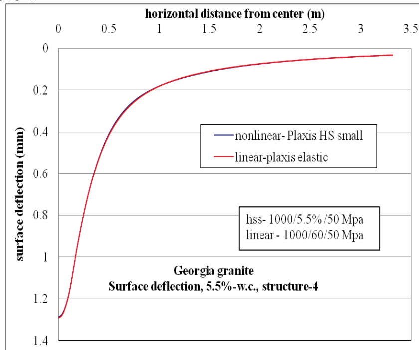
Figure C-91. Surface deflection comparison for nonlinear and linear cases, for Structure-4 with 5.5% w.c. base layer.
