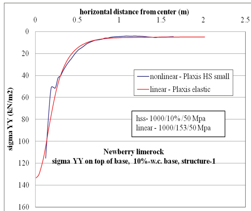
Figure C-42. \sigma_{yy} vertical stress at top of base layer comparison for nonlinear and linear cases, for Structure-1 with 10% w.c. base layer.
