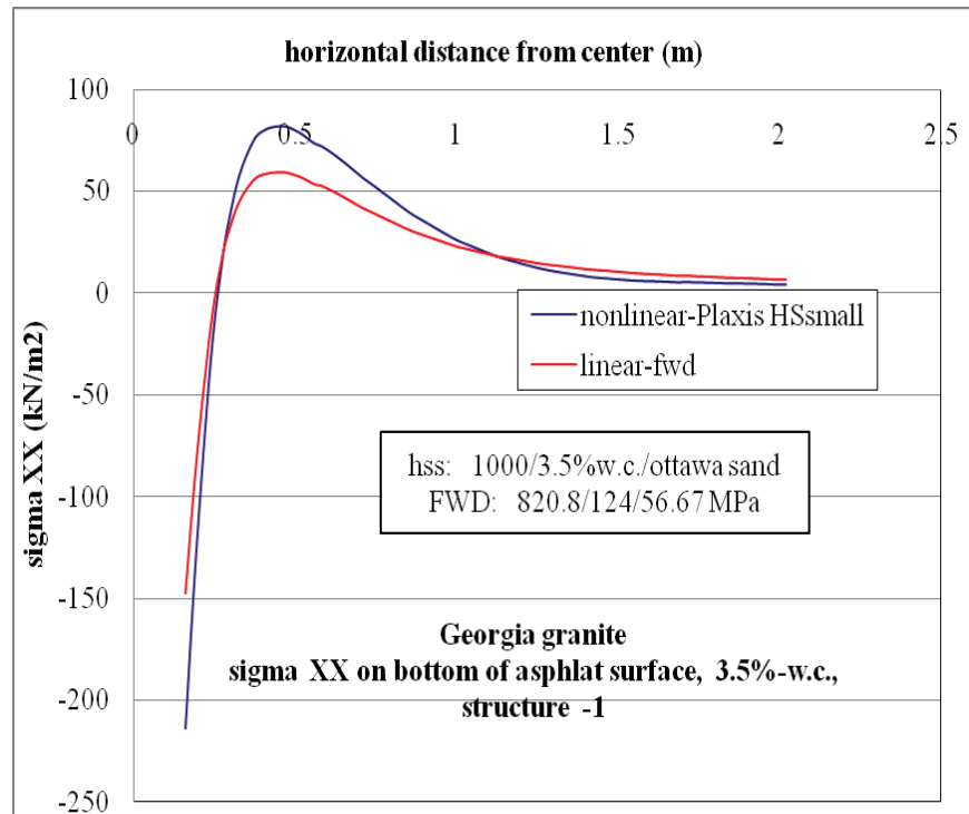
Figure D-41. \sigma_{xx} at bottom of AC layer comparison for nonlinear and linear cases, for Structure-1 with 3.5% w.c. base layer and nonlinear Ottawa sand subgrade.
