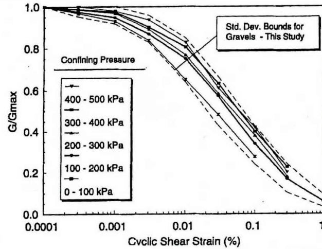
Figure 2-12. Mean curves defining G/G_{max} versus \gamma relationships for gravelly soils at various confining pressures along with standard deviation boundaries for reduced data set (from Rollins et al., 1998).
