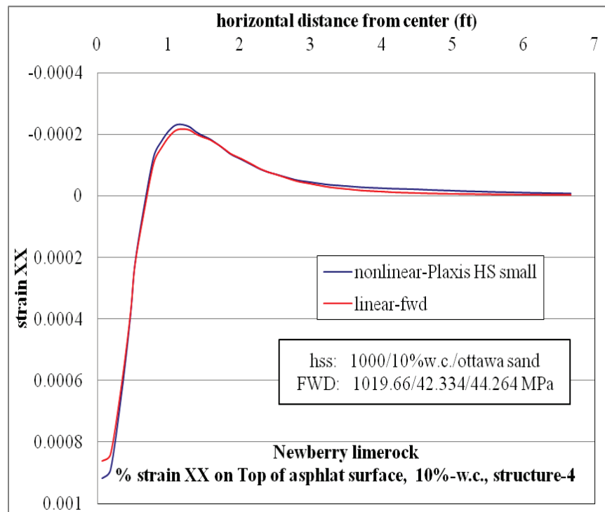
Figure D-9. \epsilon_{xx} at top of AC layer comparison for nonlinear and linear cases, for Structure-4 with 10% w.c. base layer and nonlinear Ottawa sand subgrade.
