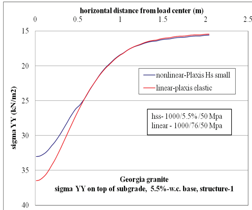
Figure C-125. \sigma_{yy} at top of subgrade comparison for nonlinear and linear cases, for Structure-1 with 5.5% w.c. base layer.
