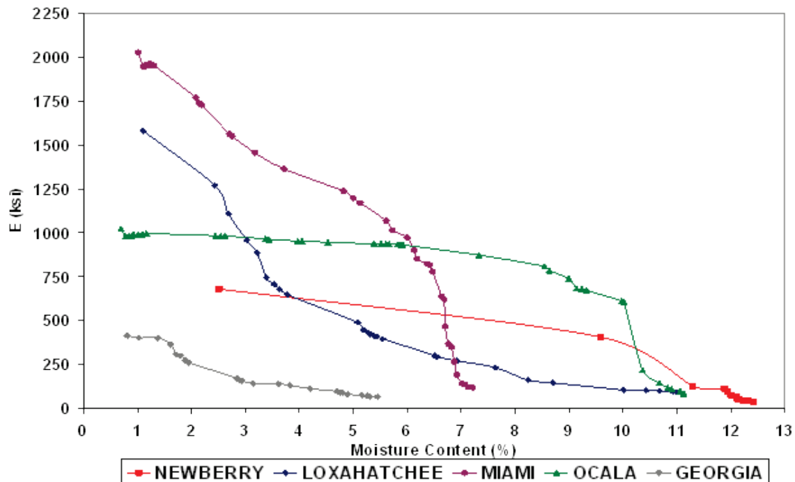
Figure 2-18. FFRC test results of each material during first cycle of wetting (from Toros, 2008).
