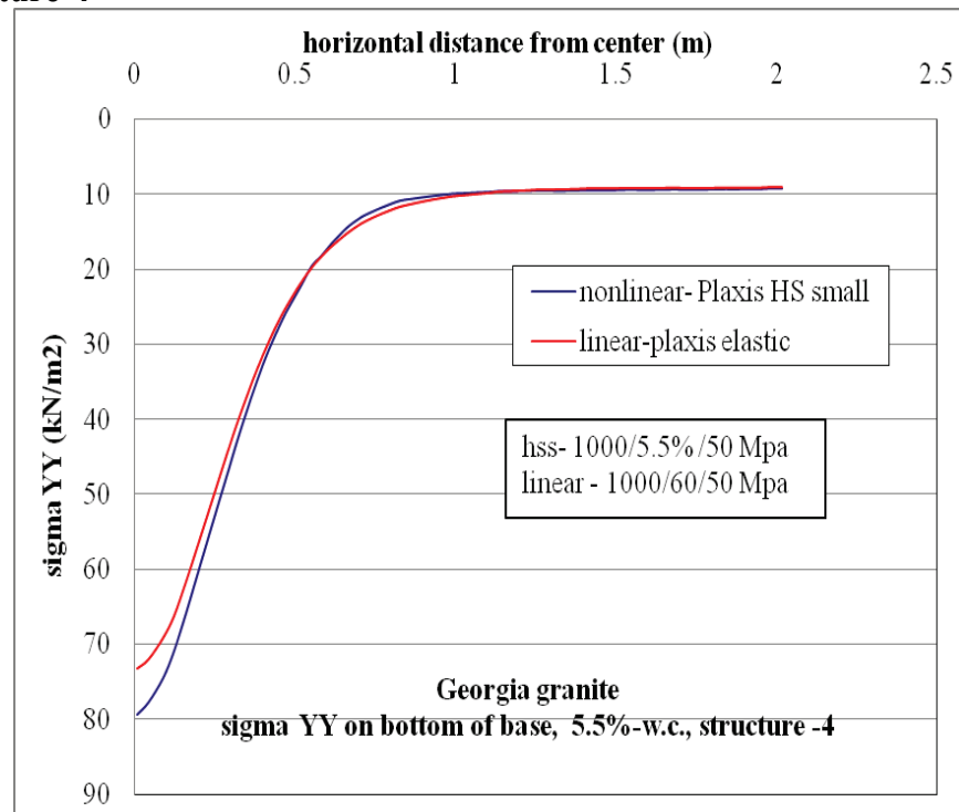
Figure C-119. \sigma_{yy} at bottom of base layer comparison for nonlinear and linear cases, for Structure-4 with 5.5% w.c. base layer.
