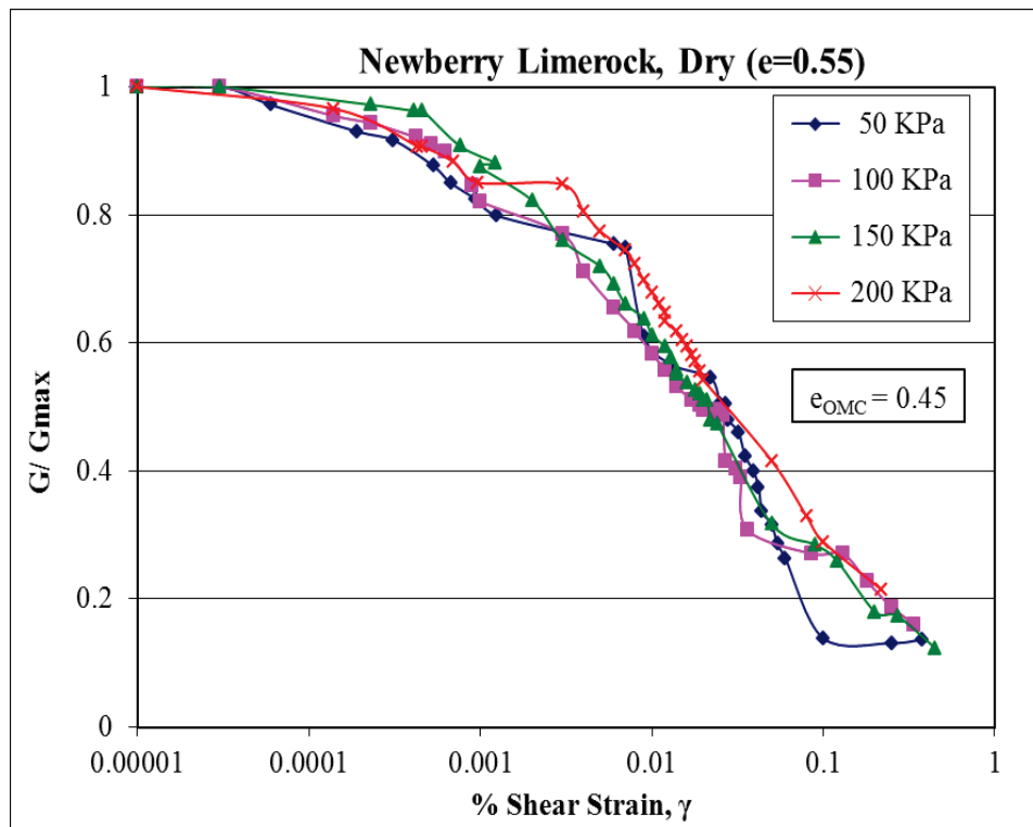
Figure A-4. G/G_{max} versus % shear strain ( \gamma ) curves at e=0.55 for Newberry limerock.
