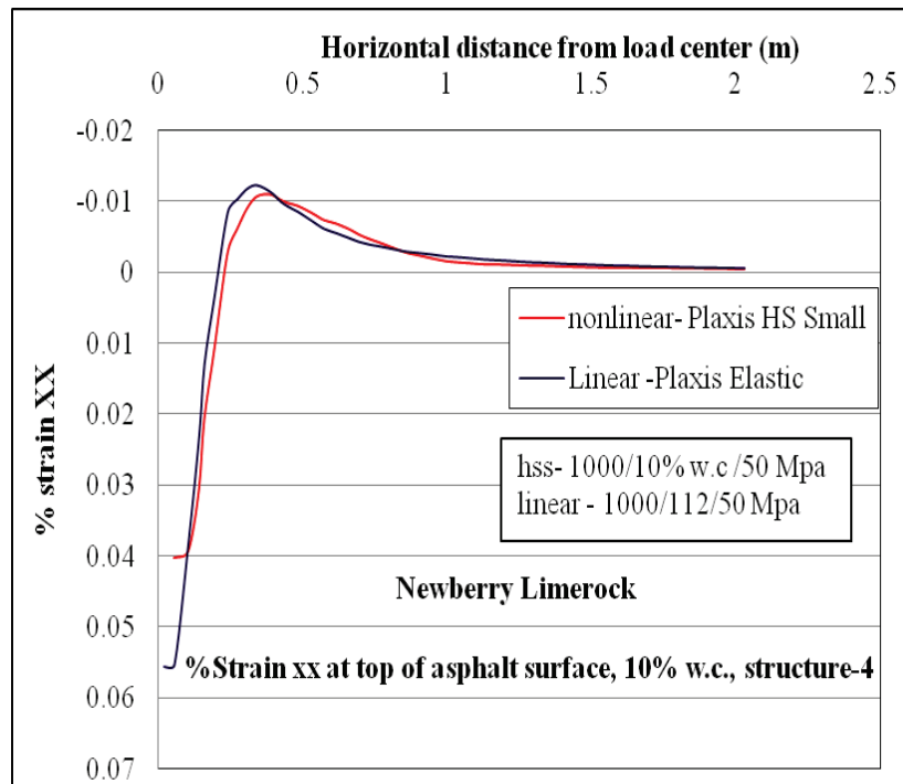
Figure C-22. \epsilon_{xx} at top of AC layer comparison for nonlinear and linear cases, for Structure-4 with 10% w.c. base layer.
