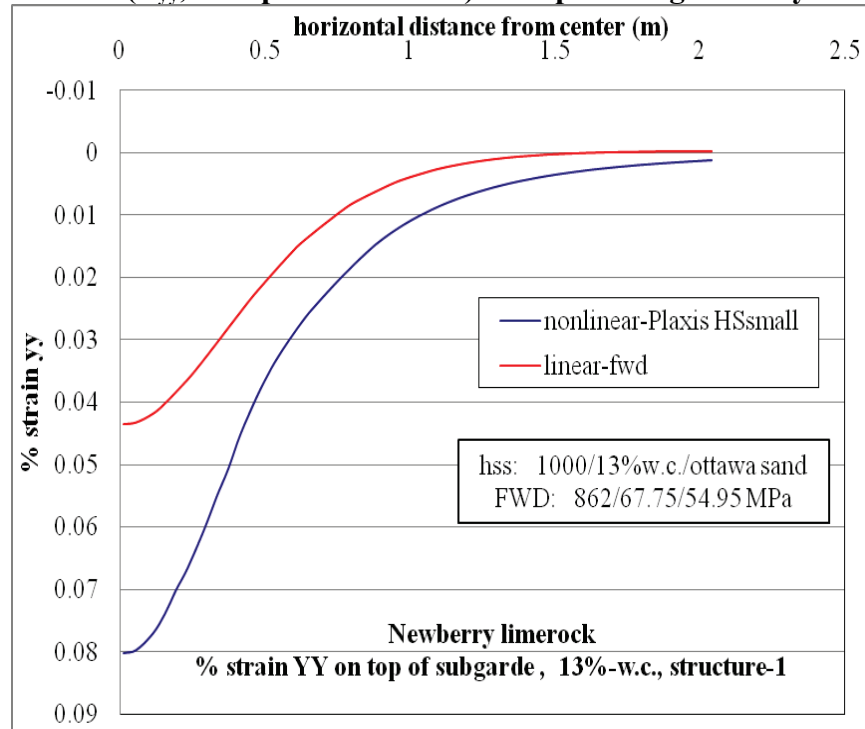
Figure D-31. \epsilon_{yy} at top of subgrade layer comparison for nonlinear and linear cases for Structure-1 with 13% w.c. base layer and nonlinear Ottawa sand subgrade.
