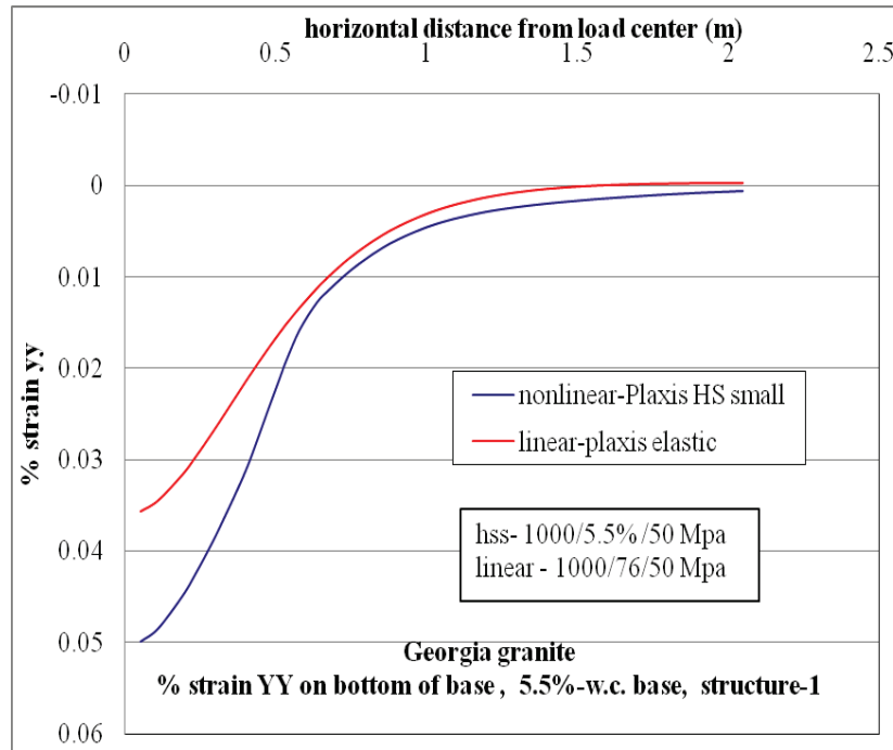
Figure C-121. \epsilon_{yy} at bottom of base layer comparison for nonlinear and linear cases, for Structure-1 with 5.5% w.c. base layer.
