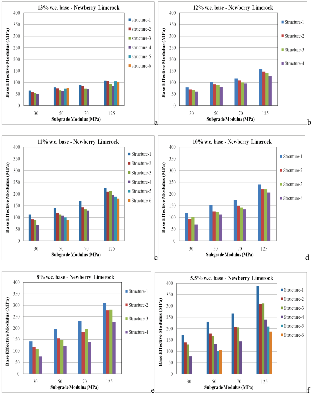
Figure 7-8. Newberry limerock effective base modulus versus subgrade modulus for different structures and at constant moisture contents of: (a) 13%, (b) 12%, (c) 11%, (d) 10%, (e) 8%, and (f) 5.5%.
