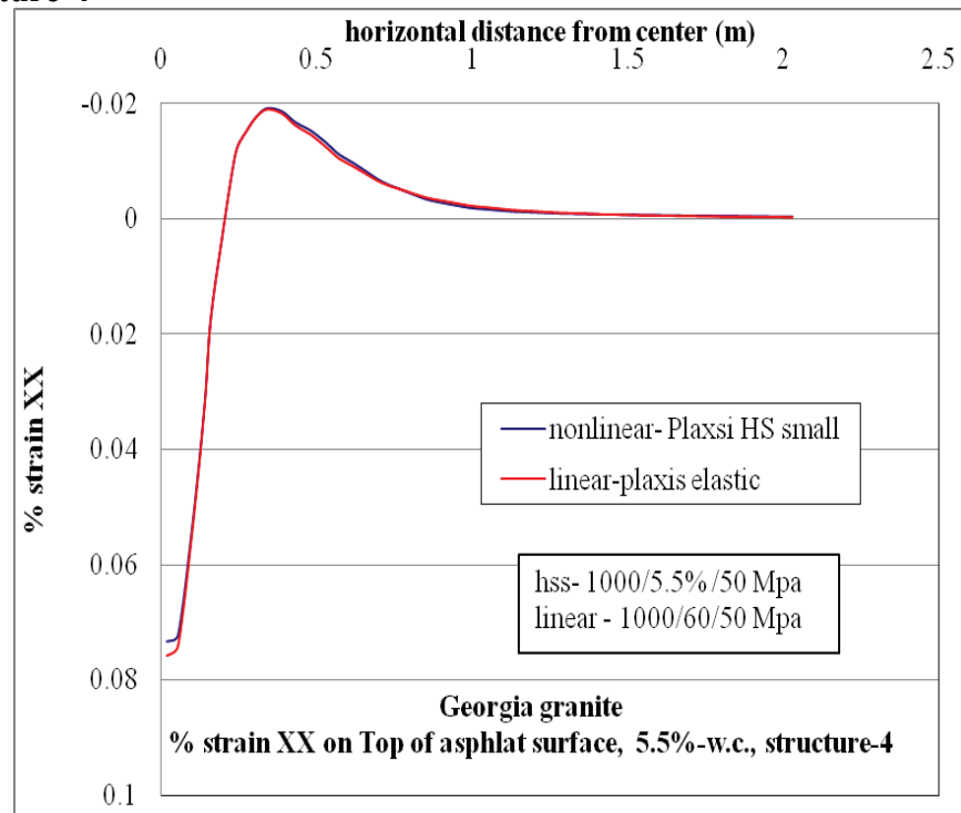
Figure C-99. \epsilon_{xx} at top of AC layer comparison for nonlinear and linear cases, for Structure-4 with 5.5% w.c. base layer.
