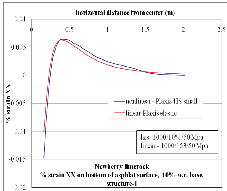
Figure C-34. \epsilon_{xx} at bottom of AC layer comparison for nonlinear and linear cases, for Structure-1 with 10% w.c. base layer.
