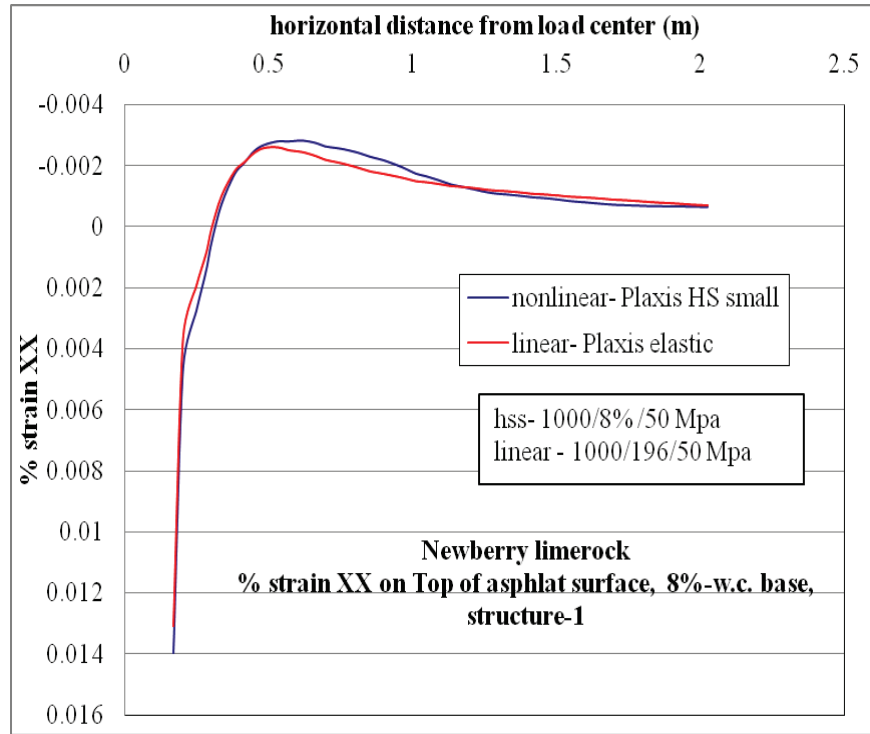
Figure C-19. \epsilon_{xx} at top of AC layer comparison for nonlinear and linear cases, for Structure-1 with 8% w.c. base layer.
