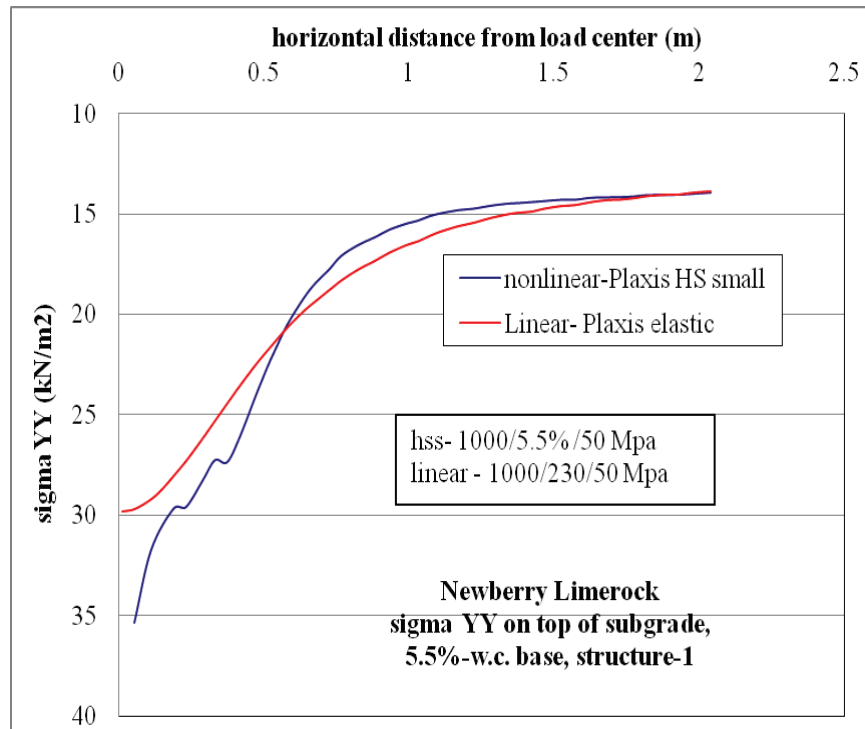
Figure C-76. \sigma_{yy} at top of subgrade comparison for nonlinear and linear cases, for Structure-1 with 5.5% w.c. base layer.
