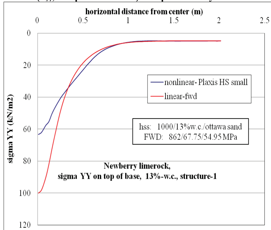
Figure D-16. \sigma_{yy} vertical stress at top of base layer comparison for nonlinear and linear cases, for Structure-1 with 13% w.c. base layer and nonlinear Ottawa sand subgrade.
