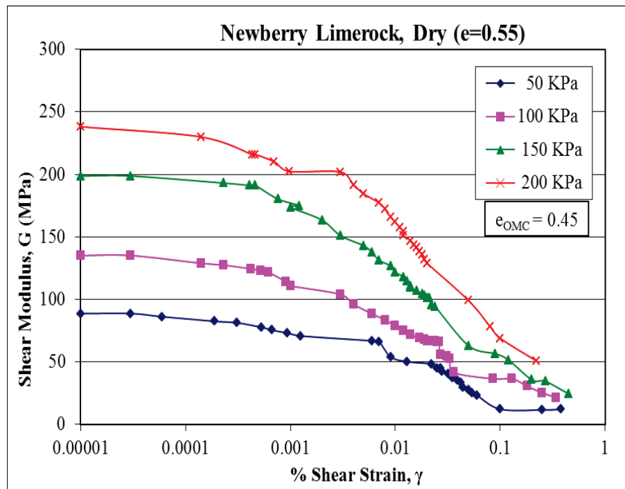
Figure A-2. Shear Modulus (G) versus % Shear strain ( \gamma ) curves for dry Newberry limerock at e=0.55 .
