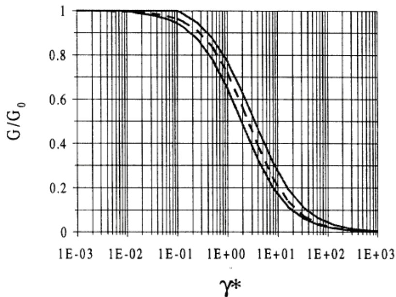
Figure 2-13. Shear modulus degradation curve proposed by Santos and Correia (2001).
