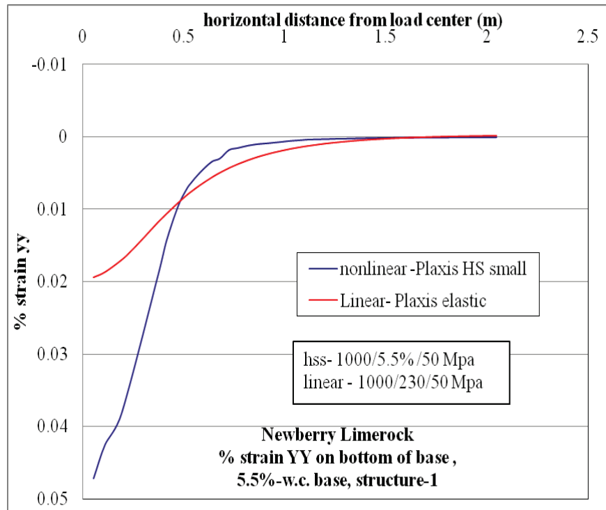
Figure C-68. \epsilon_{yy} at bottom of base layer comparison for nonlinear and linear cases, for Structure-1 with 5.5% w.c. base layer.
