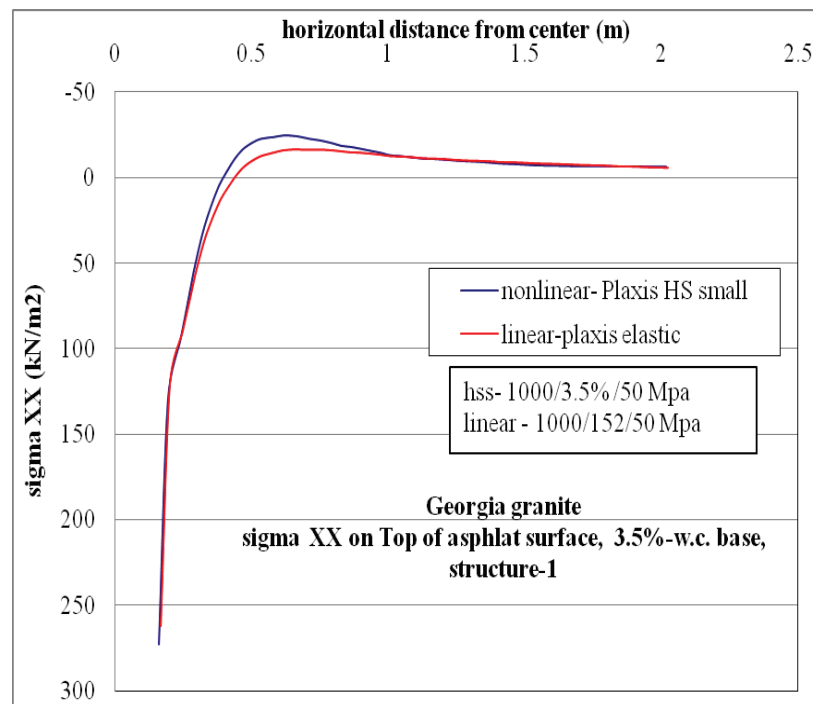
Figure C-94. \sigma_{xx} at top of AC layer comparison for nonlinear and linear cases, for Structure-1 with 3.5% w.c. base layer.
