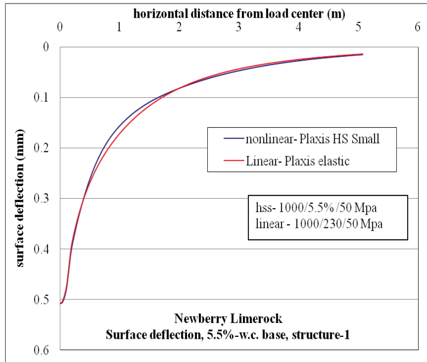
Figure C-4. Surface deflection comparison for nonlinear and linear cases, for Structure-1 with 5.5% w.c. base layer.
