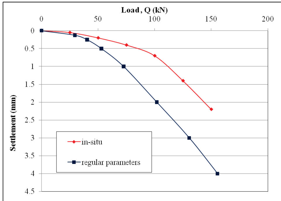
Figure 6-7a. Comparison of actual settlements with settlements predicted using suggested parameters and Plaxis-HSsmall footing model.
