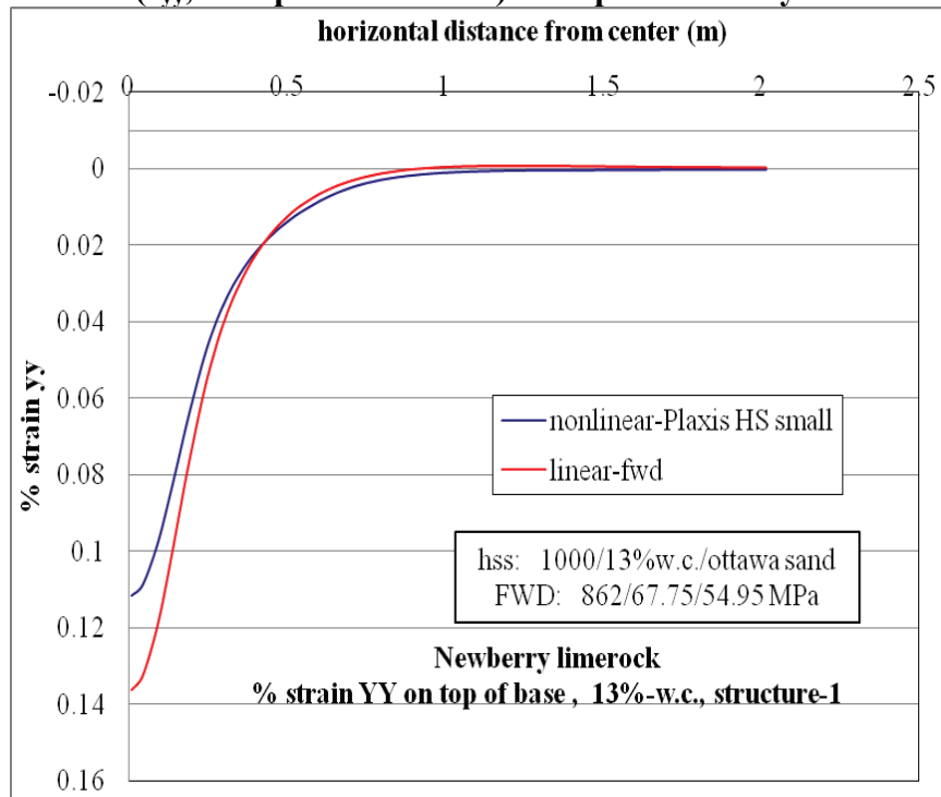
Figure D-19. \epsilon_{yy} at top of base layer comparison for nonlinear and linear cases, for Structure-1 with 13% w.c. base layer and nonlinear Ottawa sand subgrade.
