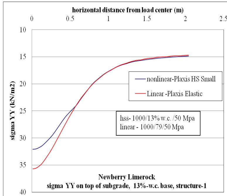
Figure C-73. \sigma_{yy} at top of subgrade comparison for nonlinear and linear cases, for Structure-1 with 13% w.c. base layer.
