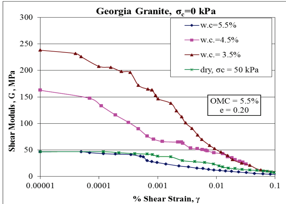
Figure 5-10. Shear modulus (G) versus shear strain ( \gamma ) curves for Georgia granite at different moisture contents.
