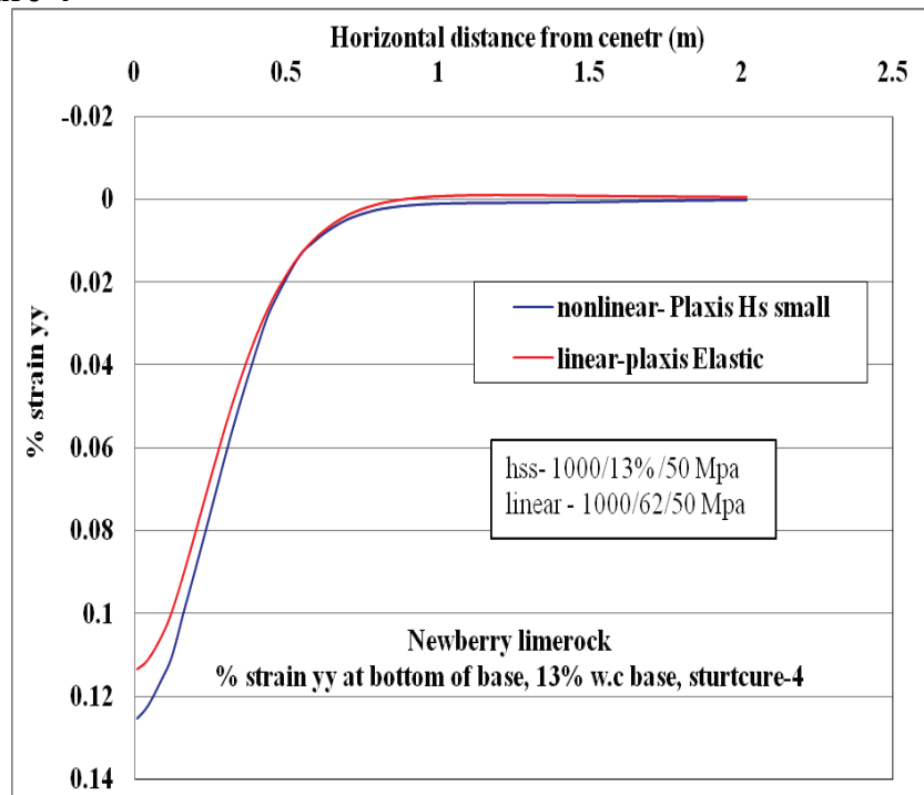
Figure C-69. \epsilon_{yy} at bottom of base layer comparison for nonlinear and linear cases, for Structure-4 with 13% w.c. base layer.
