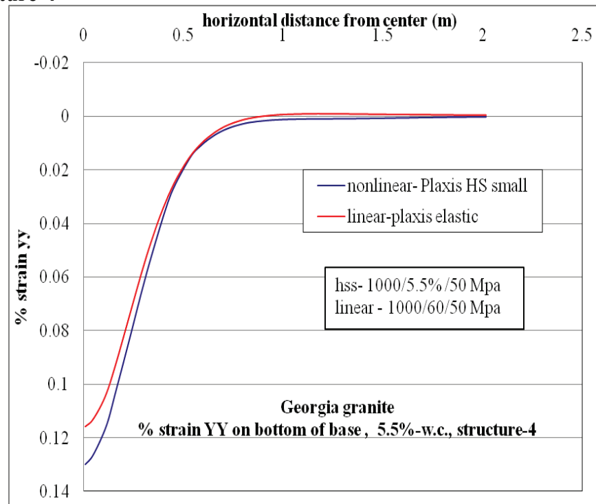
Figure C-123. \epsilon_{yy} at bottom of base layer comparison for nonlinear and linear cases, for Structure-4 with 5.5% w.c. base layer.
