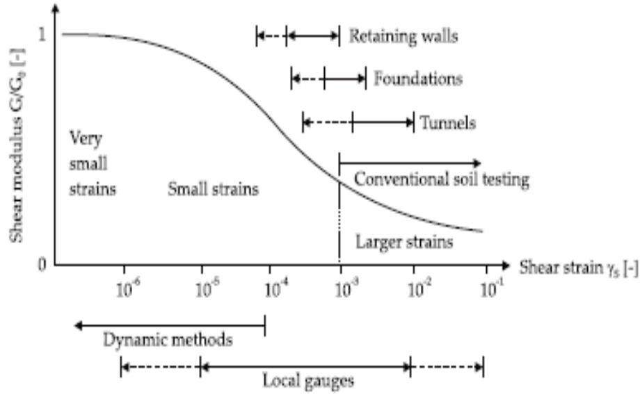
Figure 2-1. Characteristic modulus-strain behavior of soils with typical strain ranges for laboratory tests and structures (from Atkinson and Sallfors, 1991).
