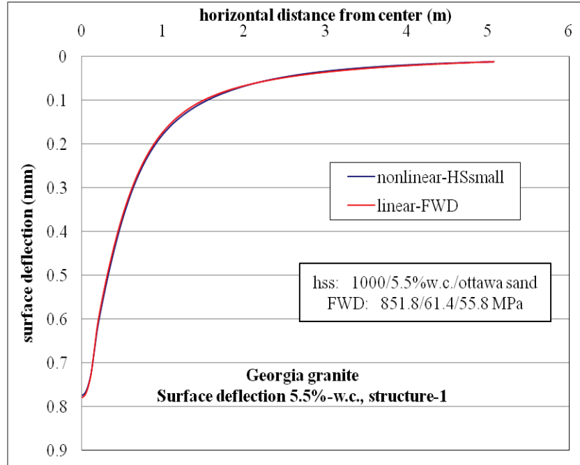
Figure D-34. Surface deflection comparison for nonlinear and linear cases, for Structure-1 with 5.5% w.c. base layer and nonlinear Ottawa sand subgrade.
