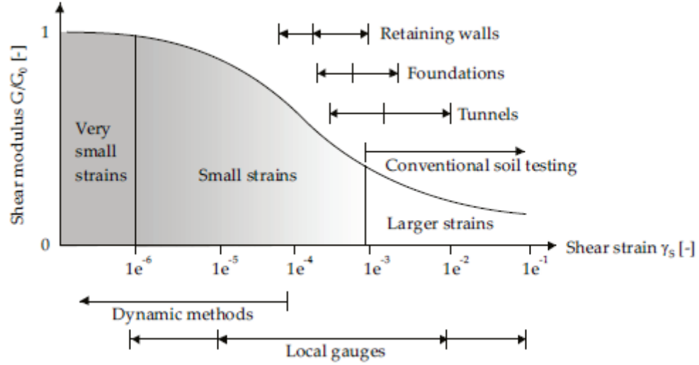
Figure 6-1. Characteristic modulus versus strain behavior of soil with typical strain ranges for laboratory tests and structures (from Atkinson and Sallfors, 1991).
