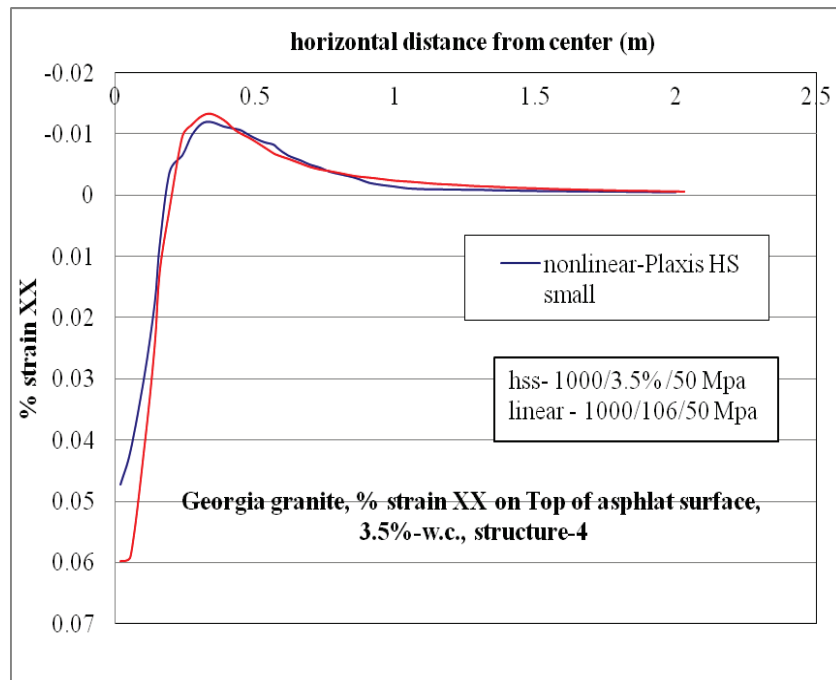
Figure C-100. \epsilon_{xx} at top of AC layer comparison for nonlinear and linear cases, for Structure-4 with 3.5% w.c. base layer.
