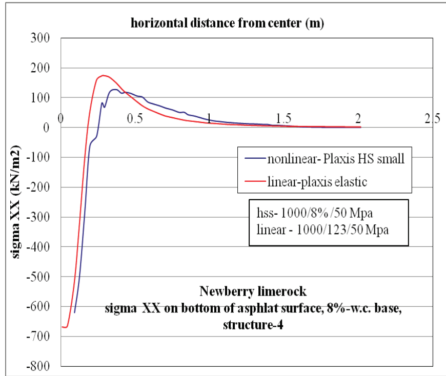
Figure C-31. \sigma_{xx} at bottom of AC layer comparison for nonlinear and linear cases, for Structure-4 with 8% w.c. base layer.
