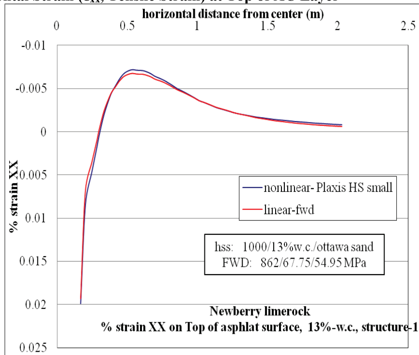
Figure D-7. \epsilon_{xx} at top of AC layer comparison for nonlinear and linear cases, for Structure-1 with 13% w.c. base layer and nonlinear Ottawa sand subgrade.
