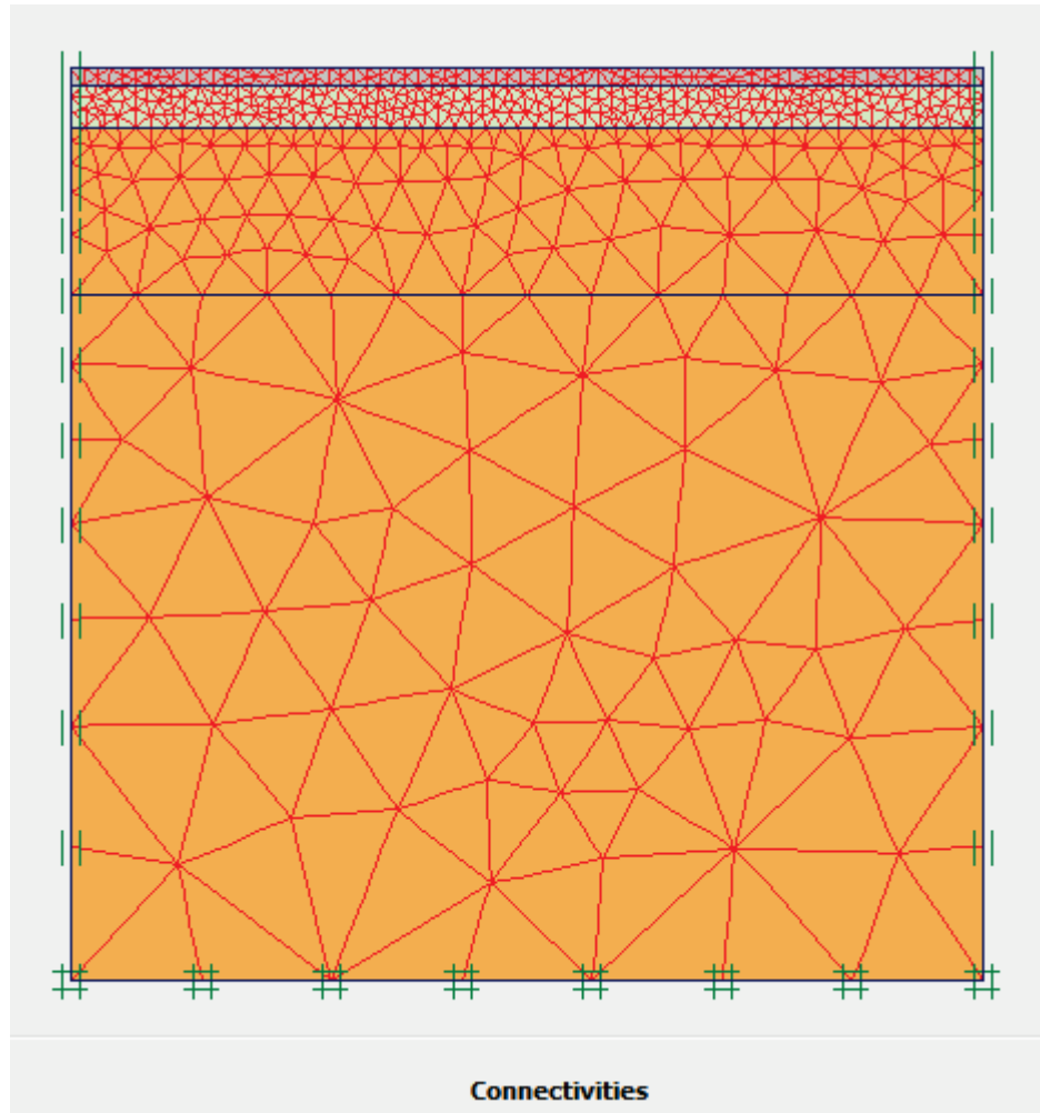
Figure 6-4b. Typical HSsmall model finite element mesh of a pavement cross-section.
