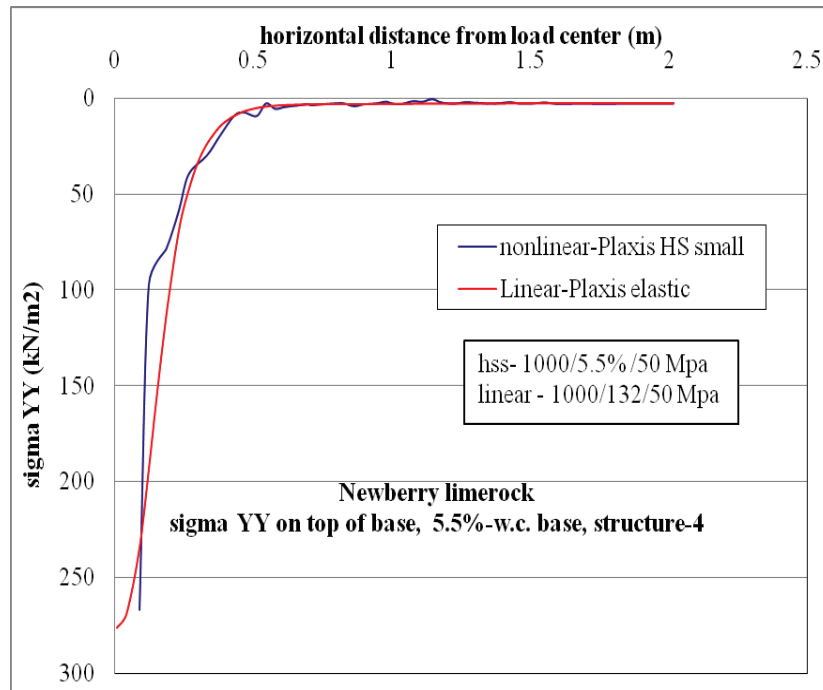
Figure C-48. \sigma_{yy} vertical stress at top of base layer comparison for nonlinear and linear cases, for Structure-4 with 5.5% w.c. base layer.
