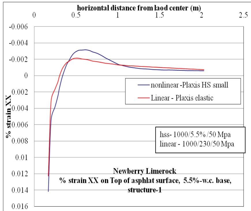
Figure C-20. \epsilon_{xx} at top of AC layer comparison for nonlinear and linear cases, for Structure-1 with 5.5% w.c. base layer.
