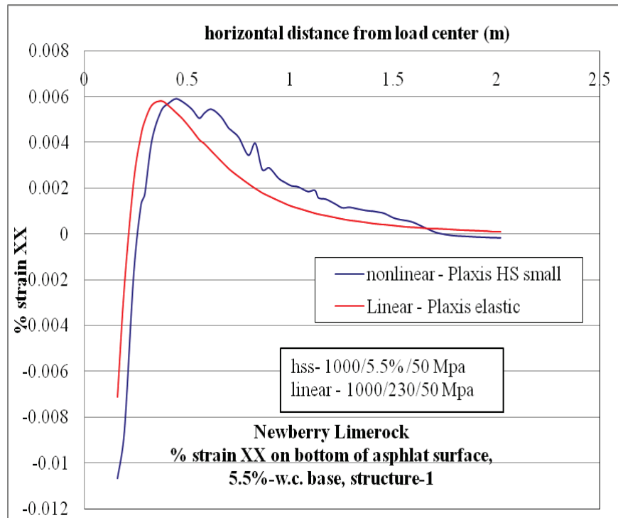
Figure C-36. \epsilon_{xx} at bottom of AC layer comparison for nonlinear and linear cases, for Structure-1 with 5.5% w.c. base layer.
