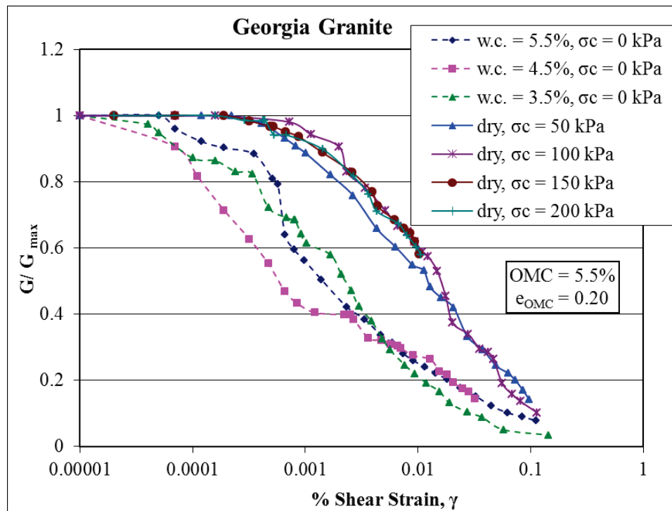
Figure 5-12. G/G_{max} versus shear strain curves for Georgia granite for both dry and wet specimens.
