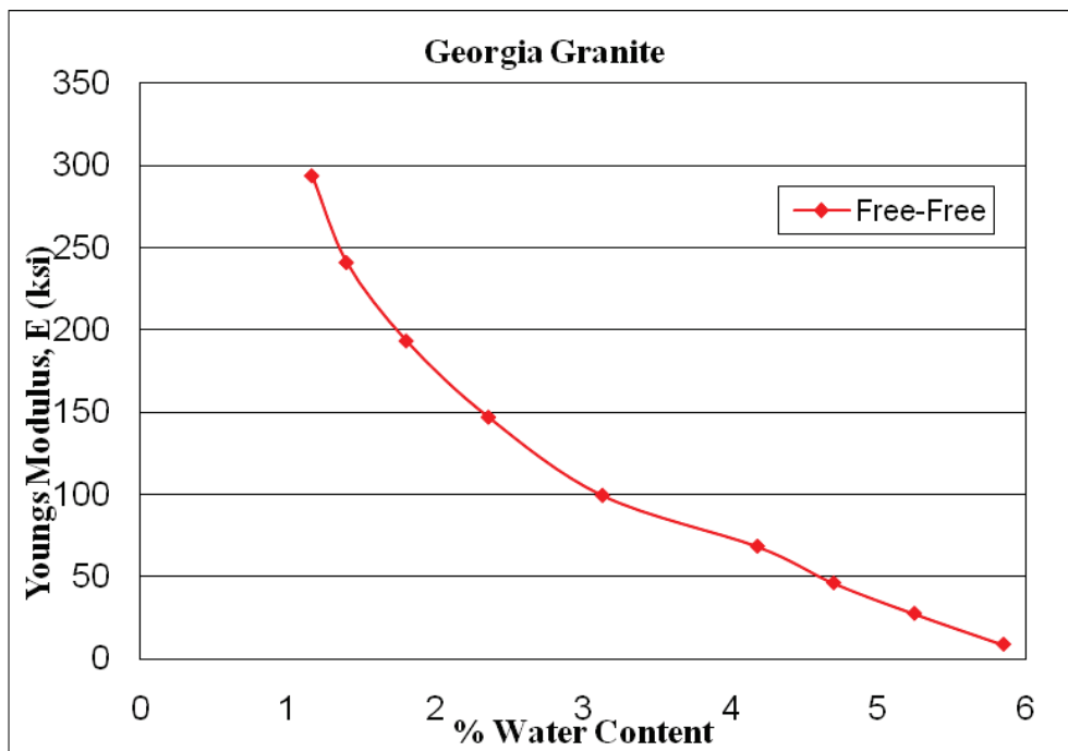
Figure 5-18. Young's modulus versus moisture content results from free-free RC test on Georgia granite.
