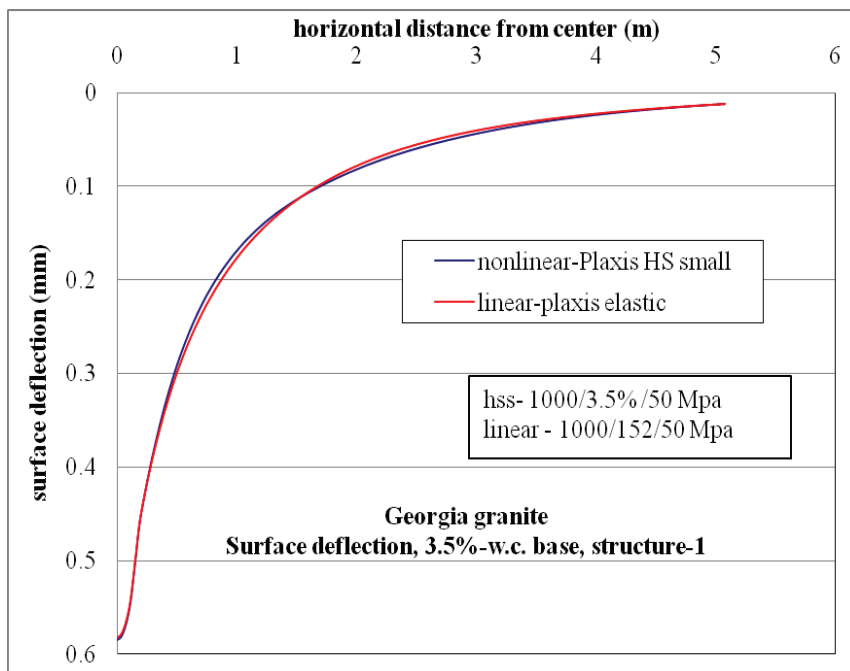
Figure C-90. Surface deflection comparison for nonlinear and linear cases, for Structure-1 with 3.5% w.c. base layer.
