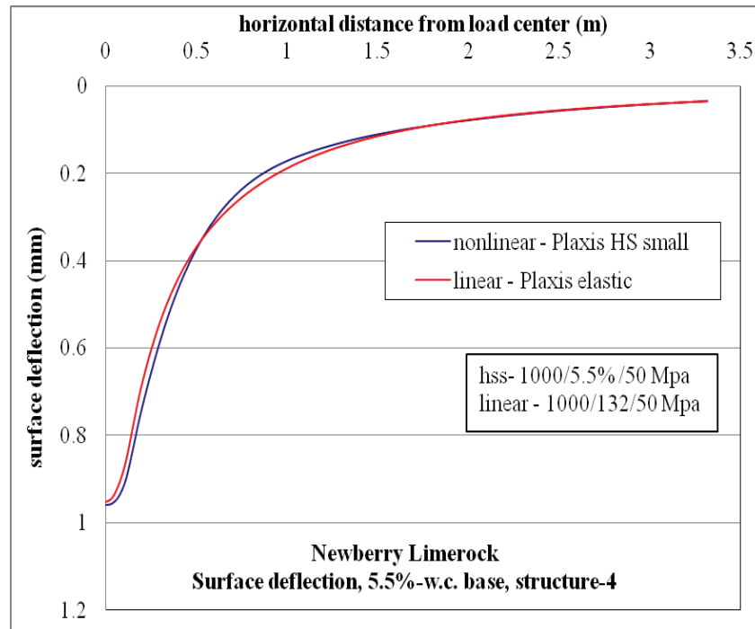
Figure C-8. Surface deflection comparison for nonlinear and linear cases, for Structure-4 with 5.5% w.c. base layer.
