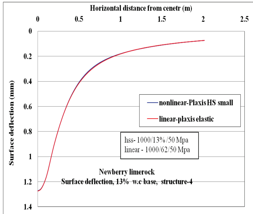
Figure C-5. Surface deflection comparison for nonlinear and linear cases, for Structure-4 with 13% w.c. base layer.
