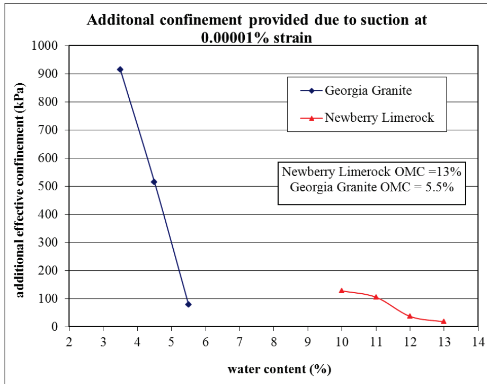
Figure 5-15. Additional confinement provided due to suction at 10^{-5}\% strain at different moisture contents.
