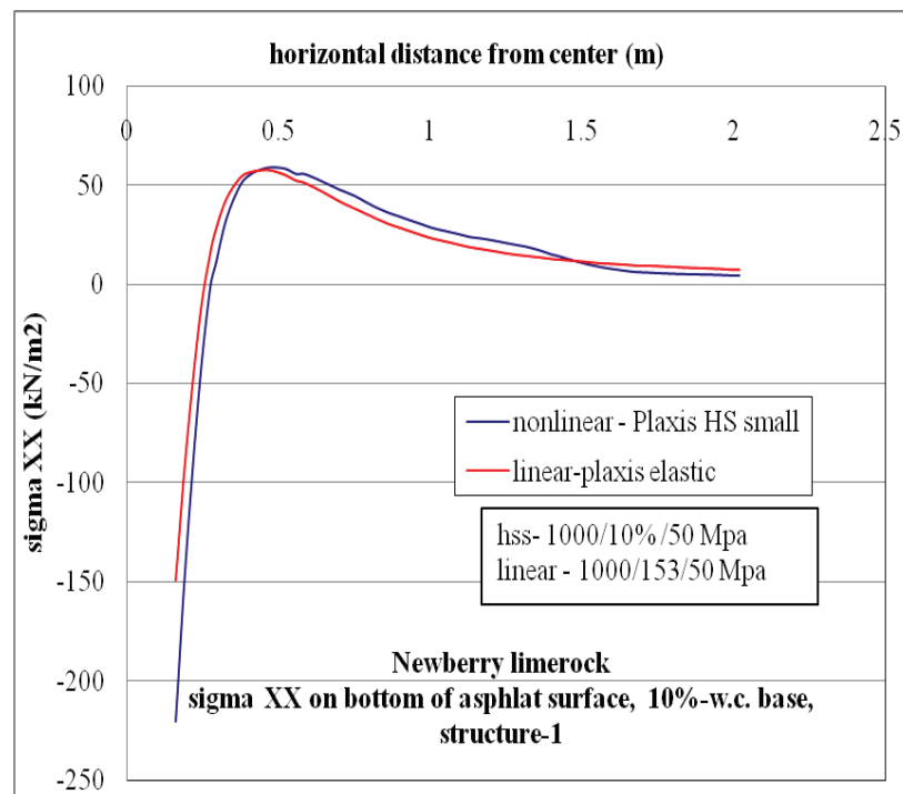
Figure C-26. \sigma_{xx} at bottom of AC layer comparison for nonlinear and linear cases, for Structure-1 with 10% w.c. base layer.
