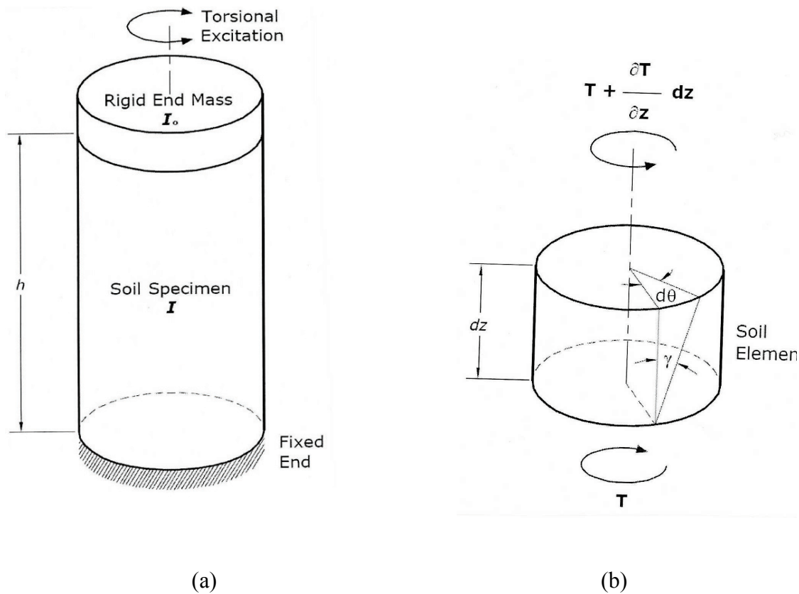
Figure 3-1. Fixed-free RC: (a) idealized testing specimen and (b) differential soil element.
