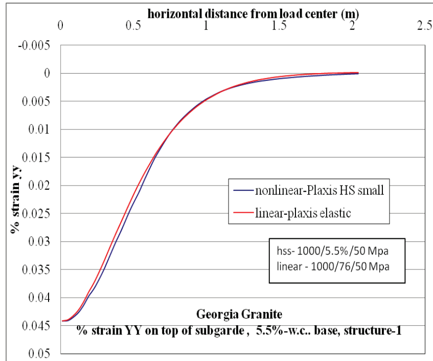
Figure C-129. \epsilon_{yy} at top of subgrade layer comparison for nonlinear and linear cases for Structure-1 with 5.5% w.c. base layer.
