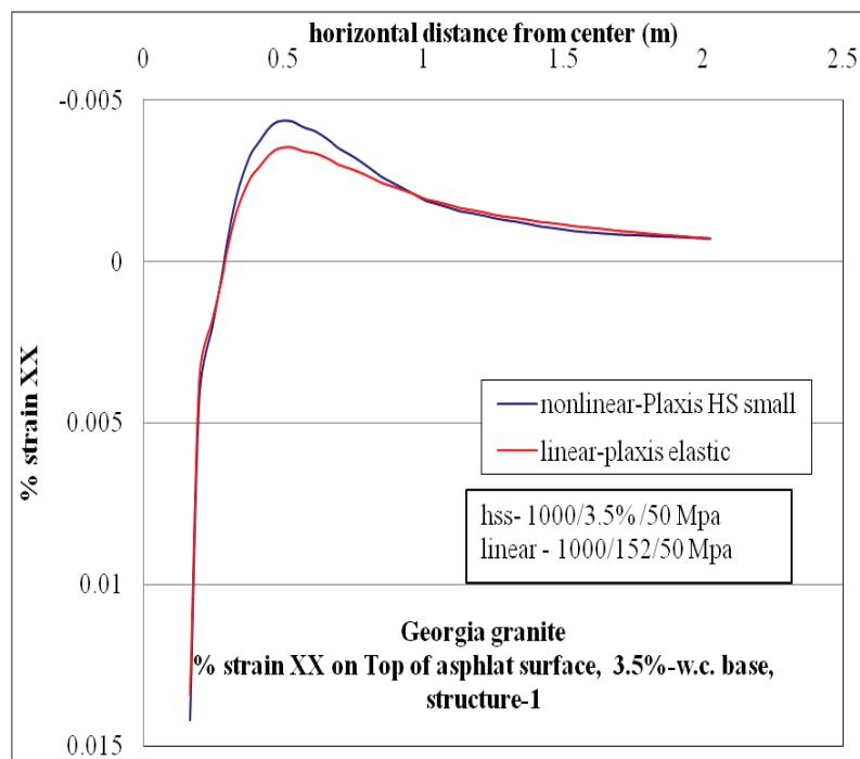
Figure C-98. \epsilon_{xx} at top of AC layer comparison for nonlinear and linear cases, for Structure-1 with 3.5% w.c. base layer.
