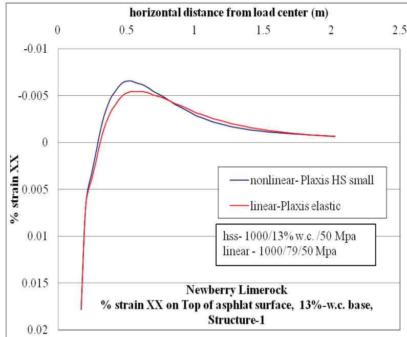
Figure C-17. \epsilon_{xx} at top of AC layer comparison for nonlinear and linear cases, for Structure-1 with 13% w.c. base layer.
