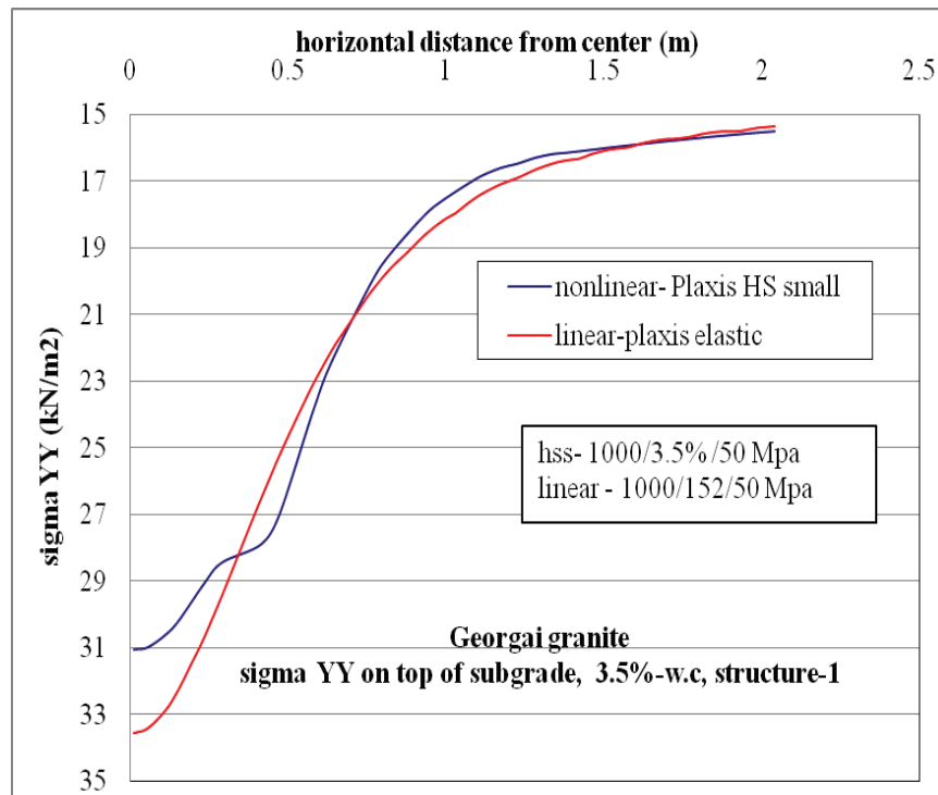
Figure C-126. \sigma_{yy} at top of subgrade layer comparison for nonlinear and linear cases for Structure-1 with 3.5% w.c. base layer.
