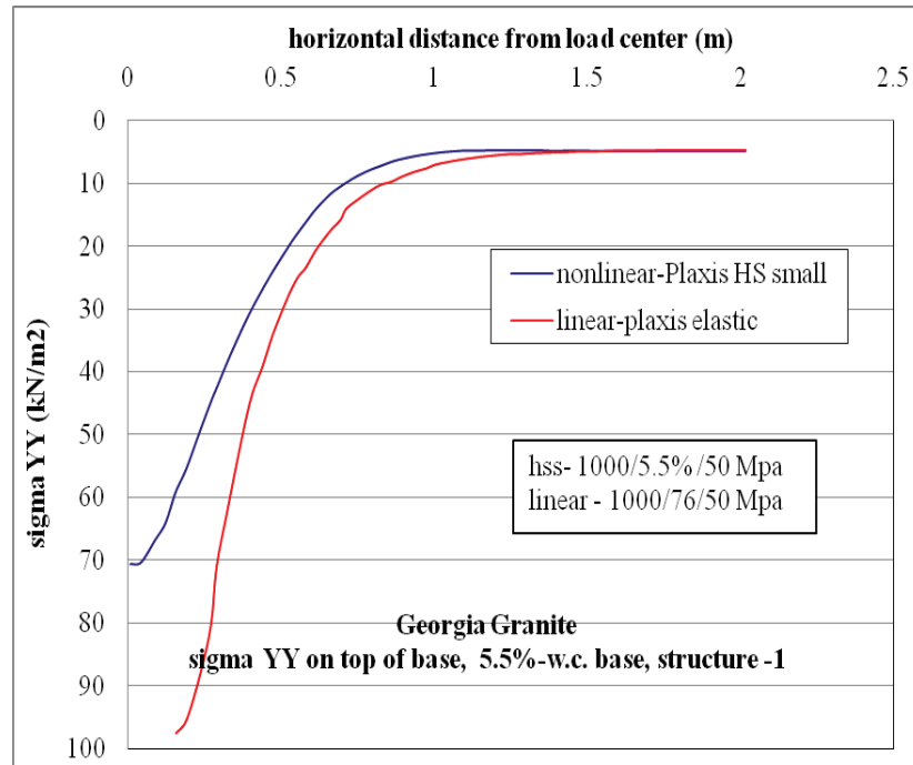
Figure C-109. \sigma_{yy} vertical stress at top of base layer comparison for nonlinear and linear cases, for Structure-1 with 5.5% w.c. base layer.
