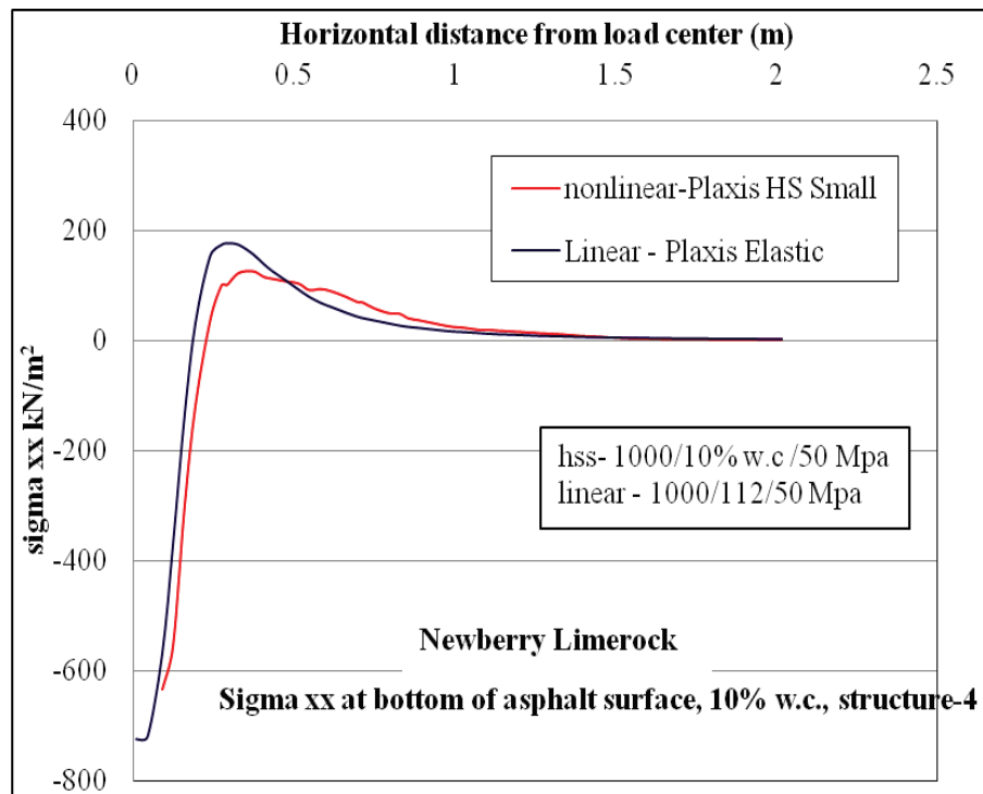
Figure C-30. \sigma_{xx} at bottom of AC layer comparison for nonlinear and linear cases, for Structure-4 with 10% w.c. base layer.
