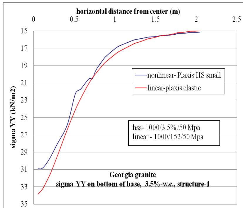
Figure C-118. \sigma_{yy} at bottom of base layer comparison for nonlinear and linear cases, for Structure-1 with 3.5% w.c. base layer.
