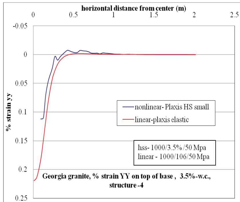
Figure C-116. \epsilon_{yy} at top of base layer comparison for nonlinear and linear cases, for Structure-4 with 3.5% w.c. base layer.
