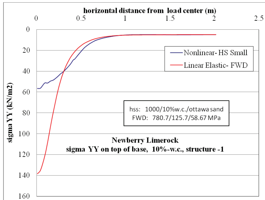
Figure D-17. \sigma_{yy} vertical stress at top of base layer comparison for nonlinear and linear cases, for Structure-1 with 10% w.c. base layer and nonlinear Ottawa sand subgrade.
