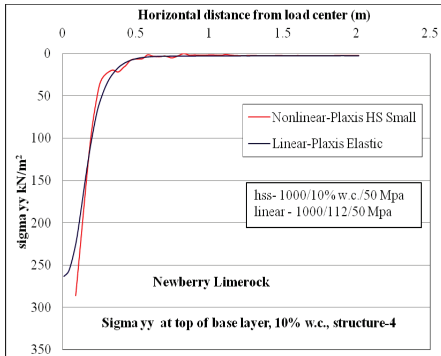
Figure C-46. \sigma_{yy} vertical stress at top of base layer comparison for nonlinear and linear cases, for Structure-4 with 10% w.c. base layer.
