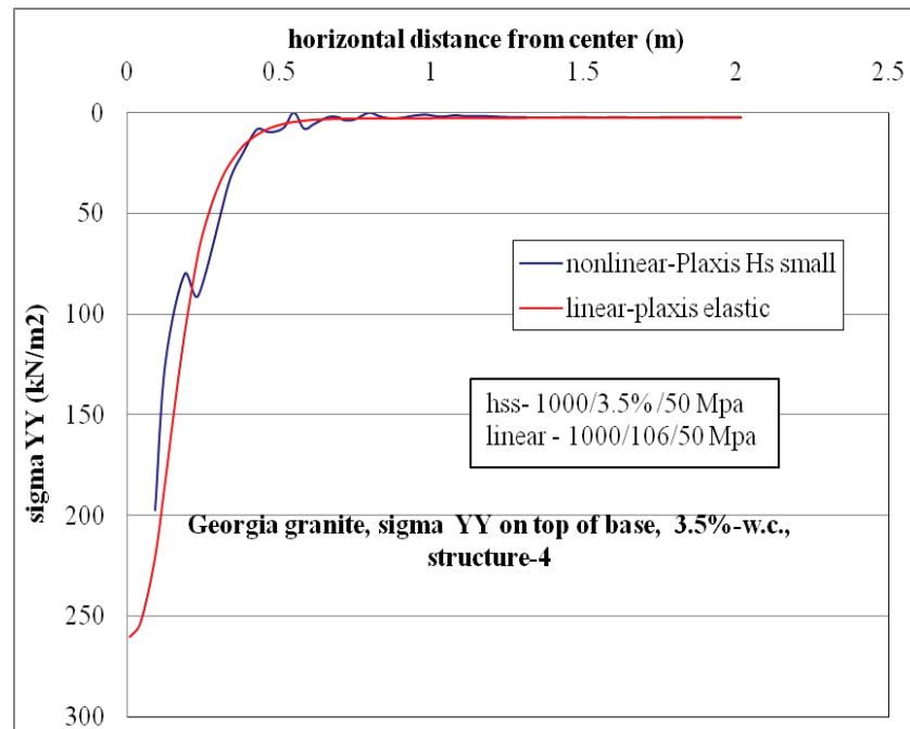
Figure C-112. \sigma_{yy} vertical stress at top of base layer comparison for nonlinear and linear cases, for Structure-4 with 3.5% w.c. base layer.
