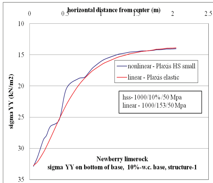
Figure C-58. \sigma_{yy} at bottom of base layer comparison for nonlinear and linear cases, for Structure-1 with 10% w.c. base layer.
