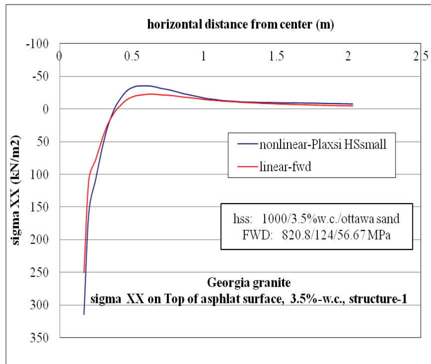
Figure D-37. \sigma_{xx} at top of AC layer comparison for nonlinear and linear cases, for Structure-1 with 3.5% w.c. base layer and nonlinear Ottawa sand subgrade.
