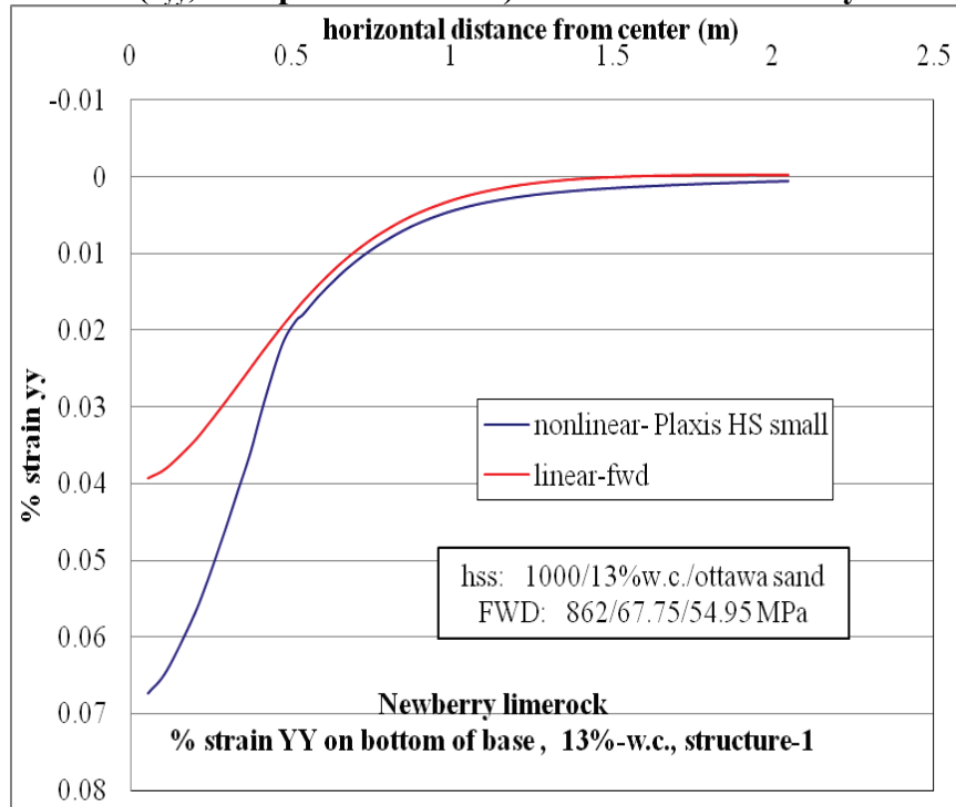
Figure D-25. \epsilon_{yy} at bottom of base layer comparison for nonlinear and linear cases, for Structure-1 with 13% w.c. base layer and nonlinear Ottawa sand subgrade.
