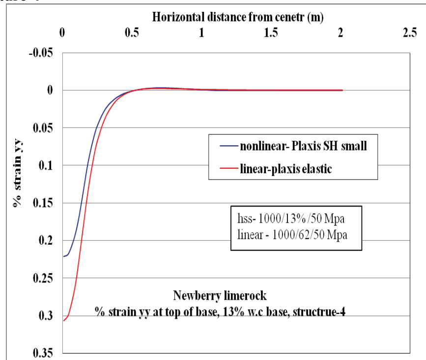
Figure C-53. \epsilon_{yy} at top of base layer comparison for nonlinear and linear cases, for Structure-4 with 13% w.c. base layer.
