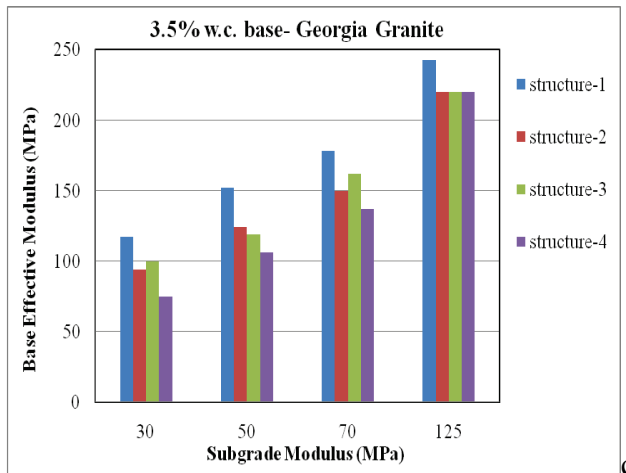
Figure 7-9. Georgia granite effective base modulus versus subgrade modulus for different structures and at constant moisture contents of: (a) 5.5%, (b) 4.5%, and (c) 3.5%.
