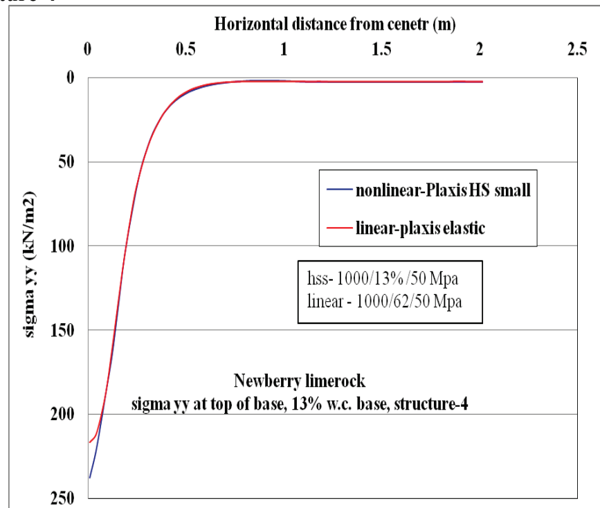
Figure C-45. \sigma_{yy} at top of base layer comparison for nonlinear and linear cases, for Structure-4 with 13% w.c. base layer.
