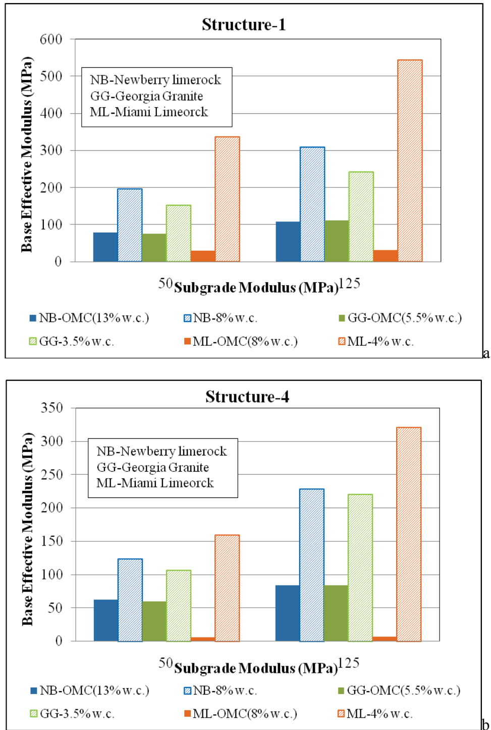
Figure 7-11. Comparison of effective moduli of all three materials at different base moisture contents and two subgrade moduli for: (a) Structure 1 and (b) Structure 4.
