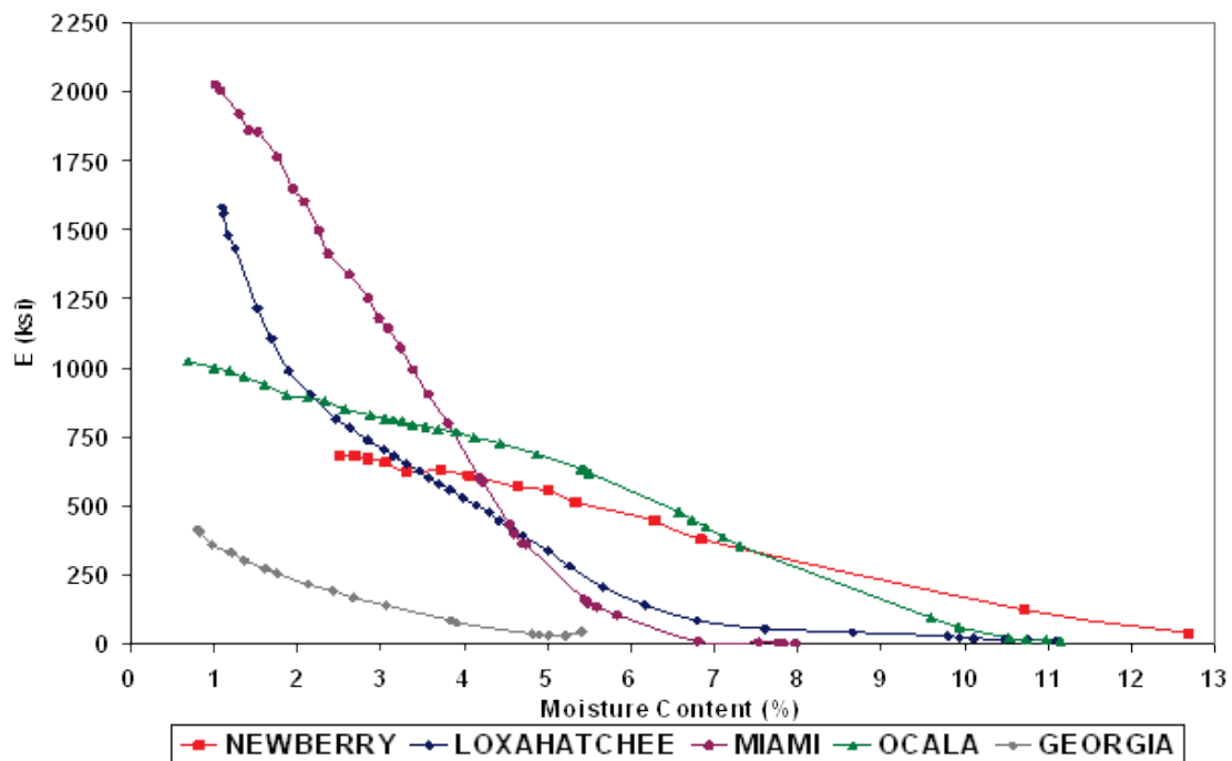
Figure 2-16. FFRC test results of specimens exposed to laboratory ambient (from Toros, 2008).
