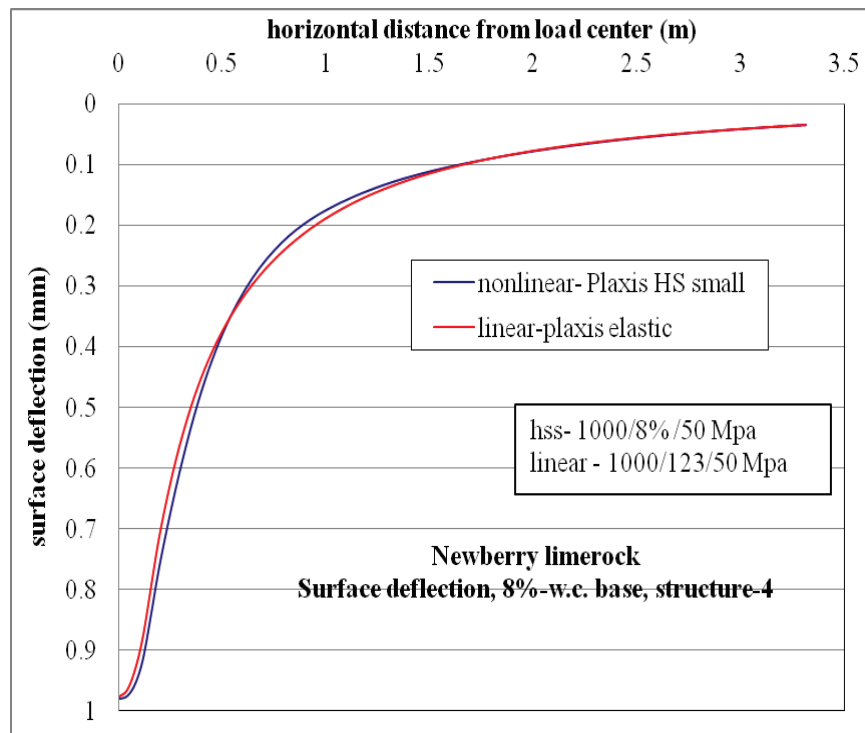
Figure C-7. Surface deflection comparison for nonlinear and linear cases, for Structure-4 with 8% w.c. base layer.
