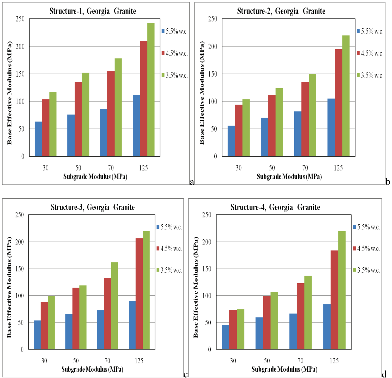
Figure 7-6. Georgia granite effective base modulus versus subgrade modulus for different moisture contents and structures: (a) Structure 1, (b) Structure 2, (c) Structure 3, and (d) Structure 4.
