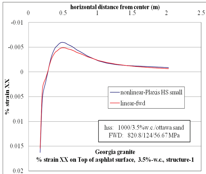
Figure D-39. \epsilon_{xx} at top of AC layer comparison for nonlinear and linear cases, for Structure-1 with 3.5% w.c. base layer and nonlinear Ottawa sand subgrade.
