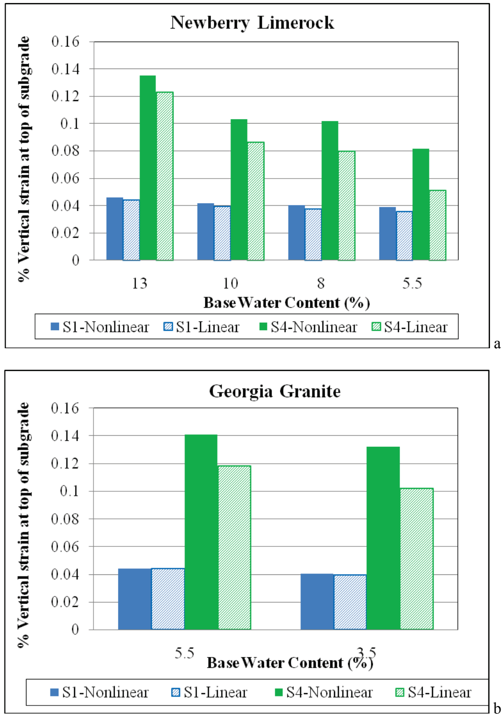
Figure 7-17. Comparison of vertical compressive strain at top of subgrade for Structure 1 and Structure 4 and for different base moisture contents: (a) Newberry limerock and (b) Georgia granite.
