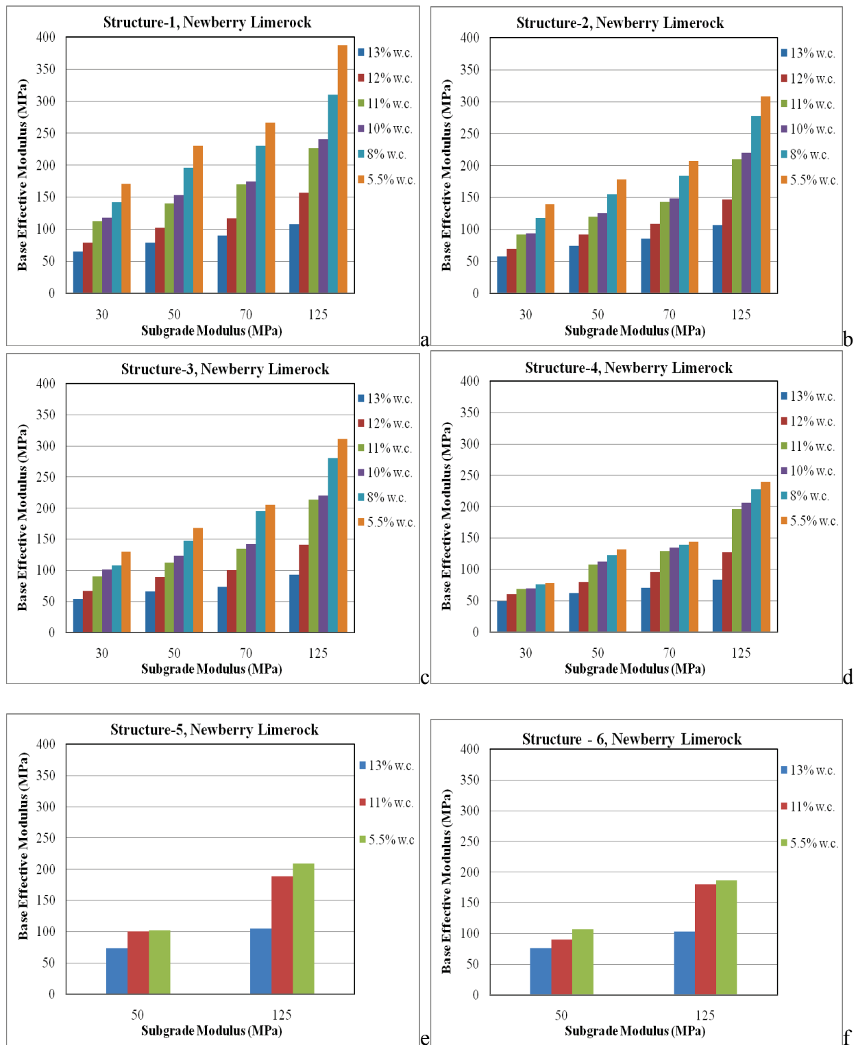
Figure 7-5. Newberry limerock effective base modulus versus subgrade modulus relationship for different moisture contents and structures: (a) Structure 1, (b) Structure 2, (c) Structure 3, (d) Structure 4, (e) Structure 5, and (f) Structure 6.
