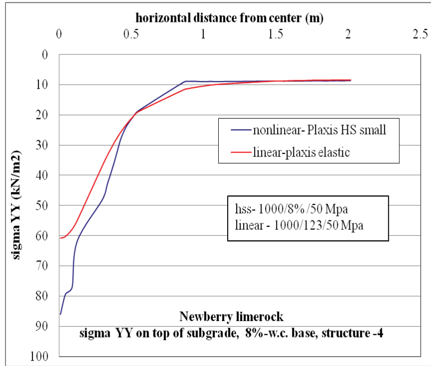
Figure C-79. \sigma_{yy} at top of subgrade comparison for nonlinear and linear cases, for Structure-4 with 8% w.c. base layer.
