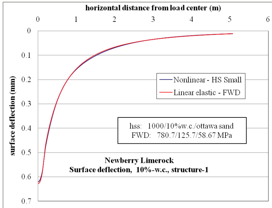
Figure D-2. Surface deflection comparison for nonlinear and linear cases, for Structure-1 with 10% w.c. base layer and nonlinear Ottawa sand subgrade.
