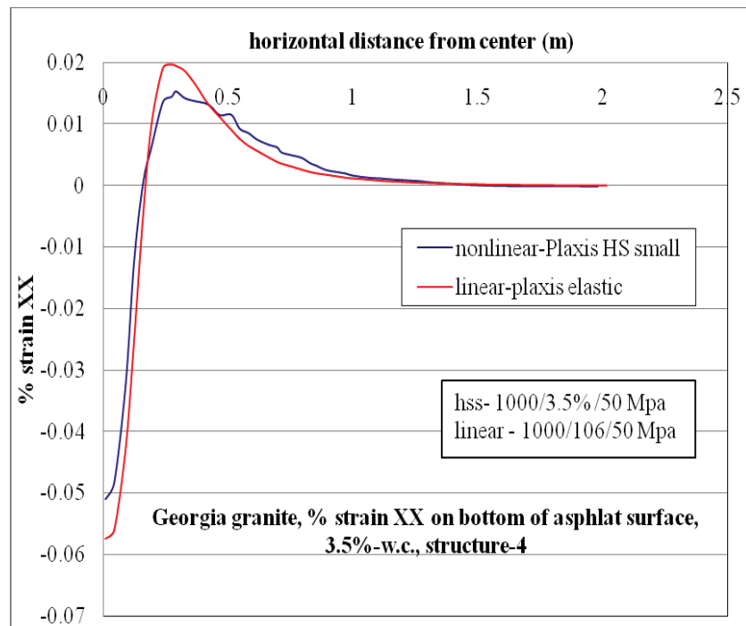
Figure C-108. \epsilon_{xx} at bottom of AC layer comparison for nonlinear and linear cases, for Structure-4 with 3.5% w.c. base layer.
