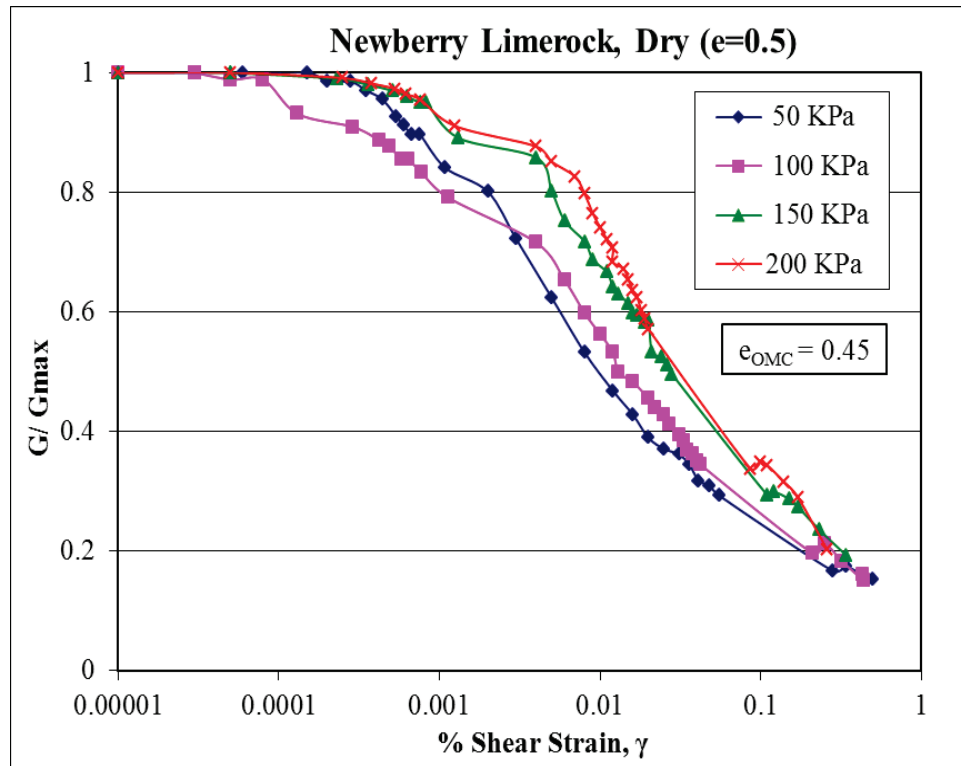
Figure A-3. G/G_{max} versus % shear strain( \gamma ) curves at e=0.5 for Newberry limerock.
