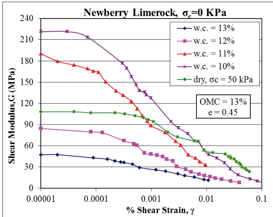
Figure 5-9. Shear modulus (G) versus shear strain ( \gamma ) curves for Newberry limerock at different moisture contents.
