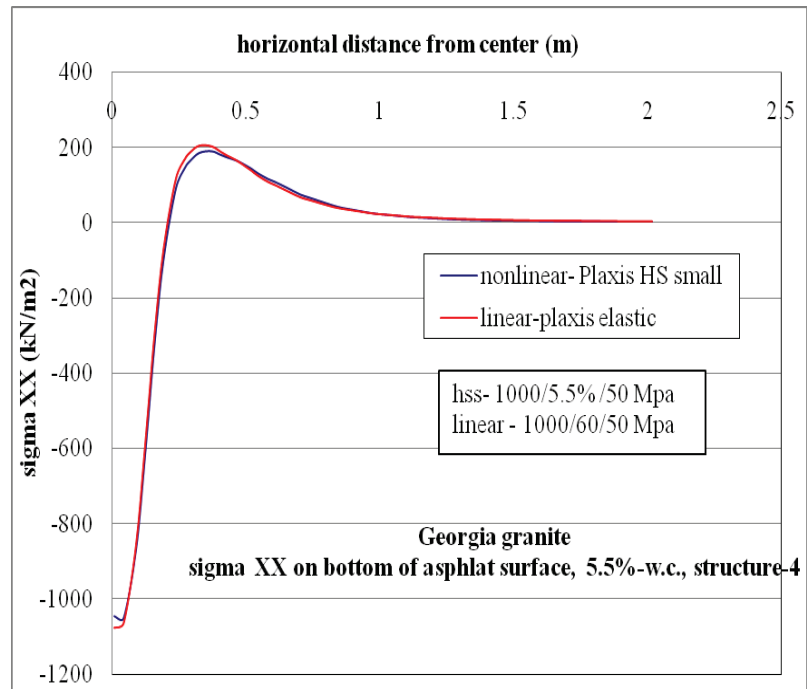
Figure C-103. \sigma_{xx} at bottom of AC layer comparison for nonlinear and linear cases, for Structure-4 with 5.5% w.c. base layer.
