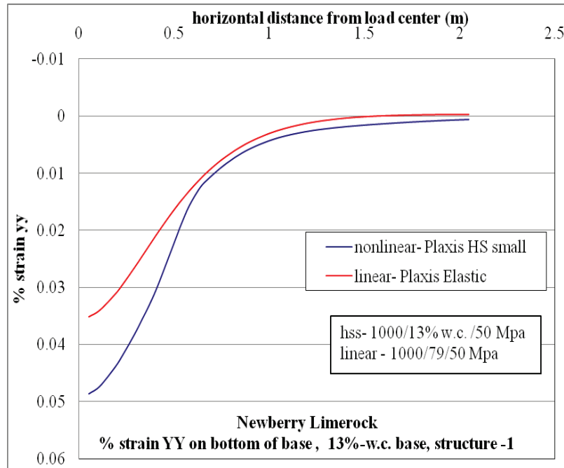
Figure C-65. \epsilon_{yy} at bottom of base layer comparison for nonlinear and linear cases, for Structure-1 with 13% w.c. base layer.
