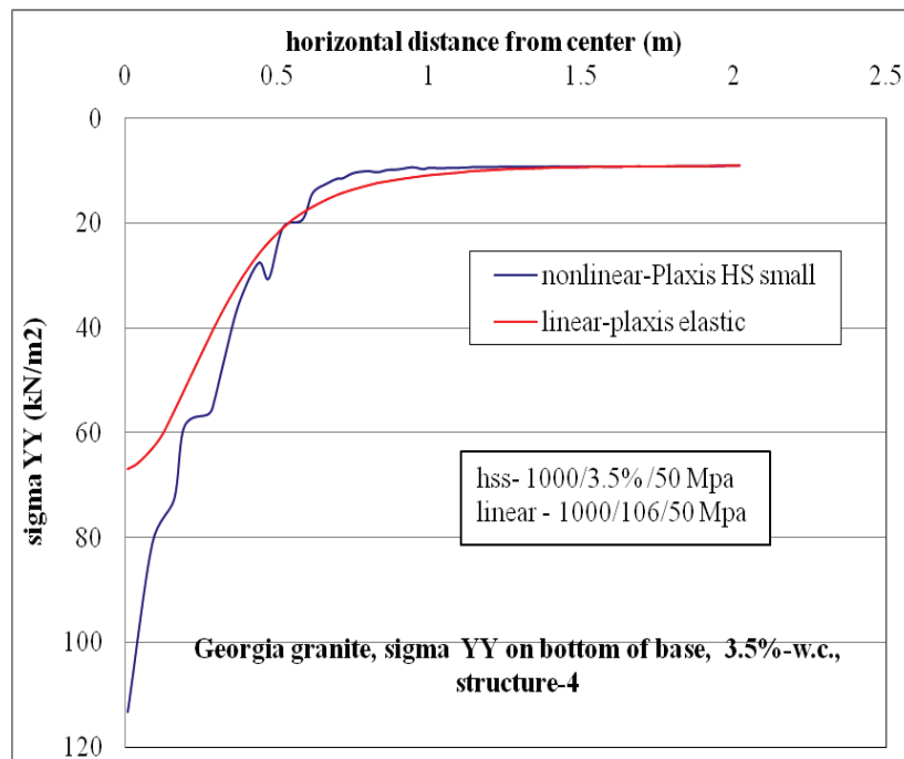
Figure C-120. \sigma_{yy} at bottom of base layer comparison for nonlinear and linear cases, for Structure-4 with 3.5% w.c. base layer.
