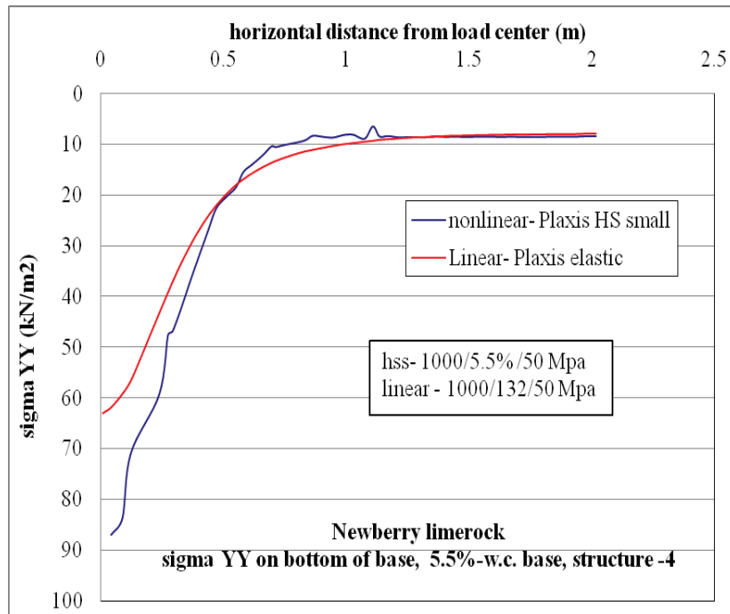
Figure C-64. \sigma_{yy} at bottom of base layer comparison for nonlinear and linear cases, for Structure-4 with 5.5% w.c. base layer.
