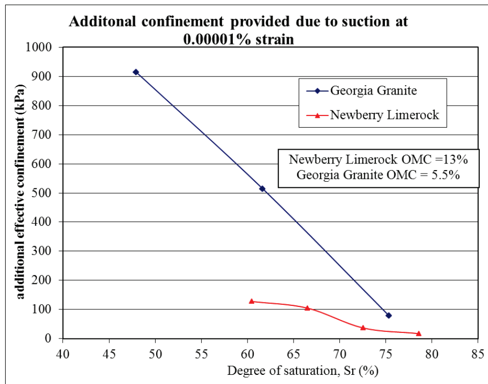
Figure 5-16. Additional confinement provided due to suction at 10^{-5}\% strain at different degrees of saturation.
