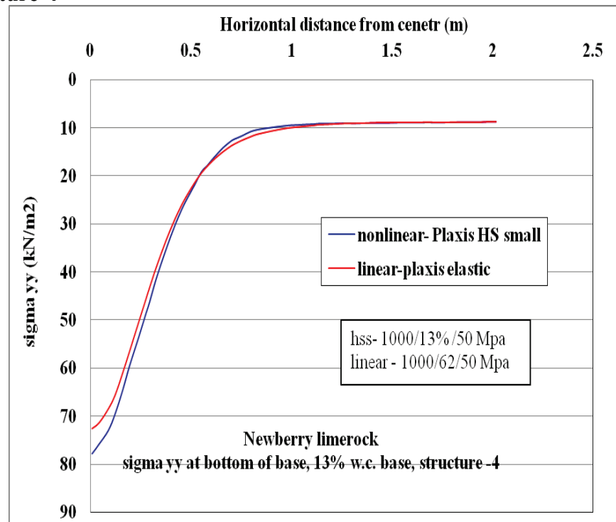
Figure C-61. \sigma_{yy} at bottom of base layer comparison for nonlinear and linear cases, for Structure-4 with 13% w.c. base layer.
