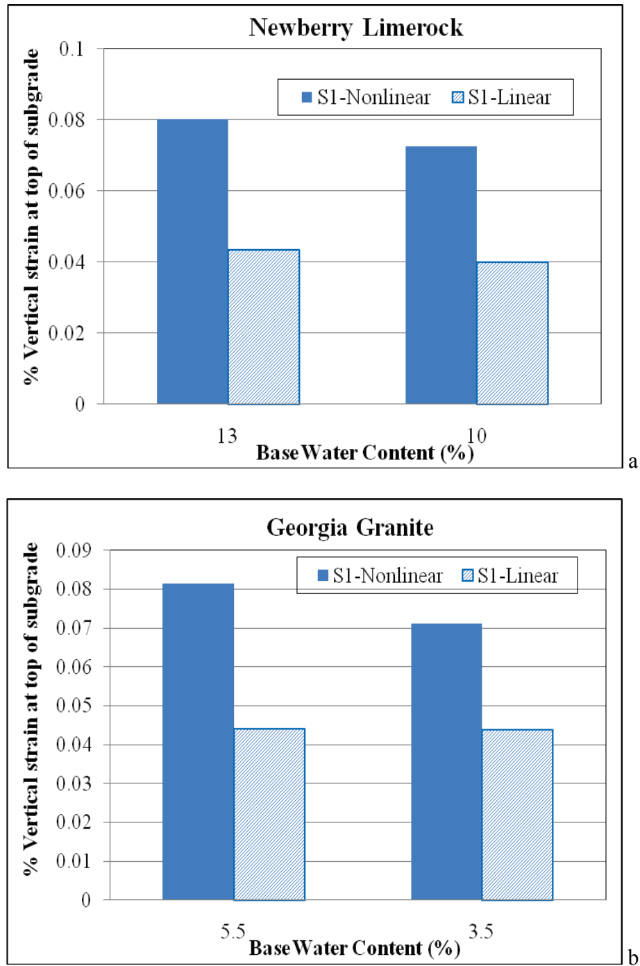
Figure 8-4. Vertical compressive strain at top of subgrade for Structure 1 with Ottawa sand subgrade and two base moisture contents for: (a) Newberry limerock and (b) Georgia granite.
