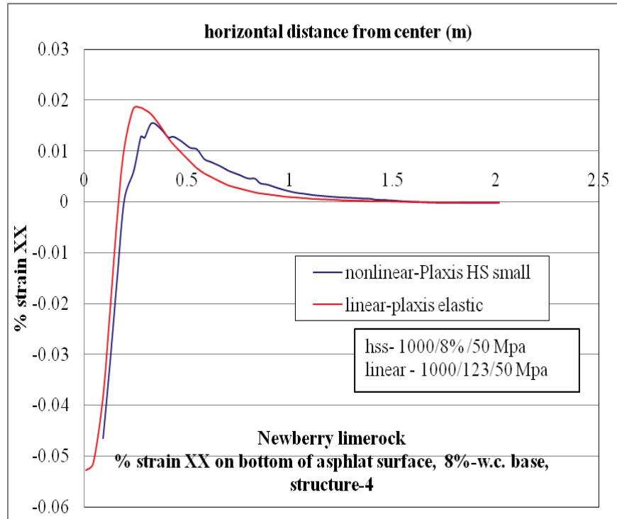
Figure C-39. \epsilon_{xx} at bottom of AC layer comparison for nonlinear and linear cases, for Structure-4 with 8% w.c. base layer.
