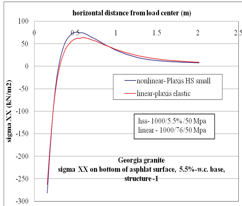
Figure C-101. \sigma_{xx} at bottom of AC layer comparison for nonlinear and linear cases, for Structure-1 with 5.5% w.c. base layer.
