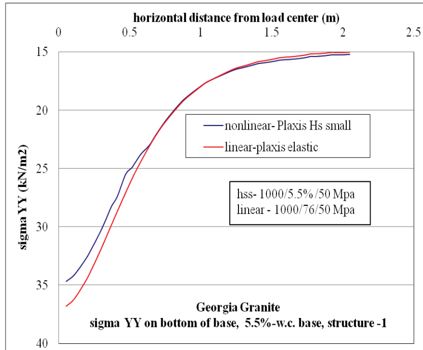
Figure C-117. \sigma_{yy} at bottom of base layer comparison for nonlinear and linear cases, for Structure-1 with 5.5% w.c. base layer.
