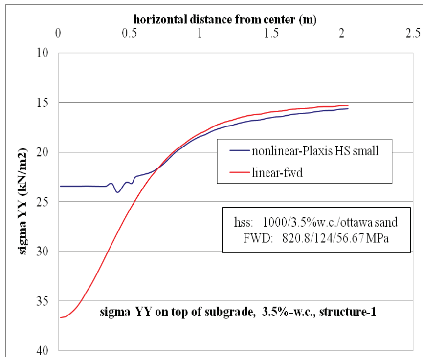
Figure D-53. \sigma_{yy} at top of subgrade comparison for nonlinear and linear cases, for Structure-1 with 3.5% w.c. base layer and nonlinear Ottawa sand subgrade.
