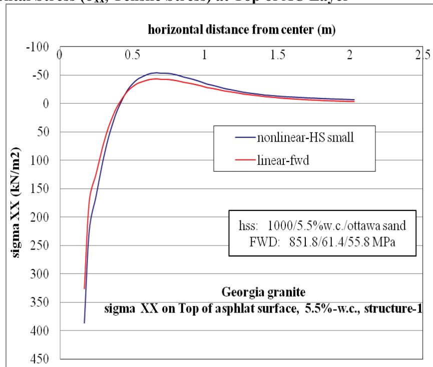
Figure D-36. \sigma_{xx} at top of AC layer comparison for nonlinear and linear cases, for Structure-1 with 5.5% w.c. base layer and nonlinear Ottawa sand subgrade.
