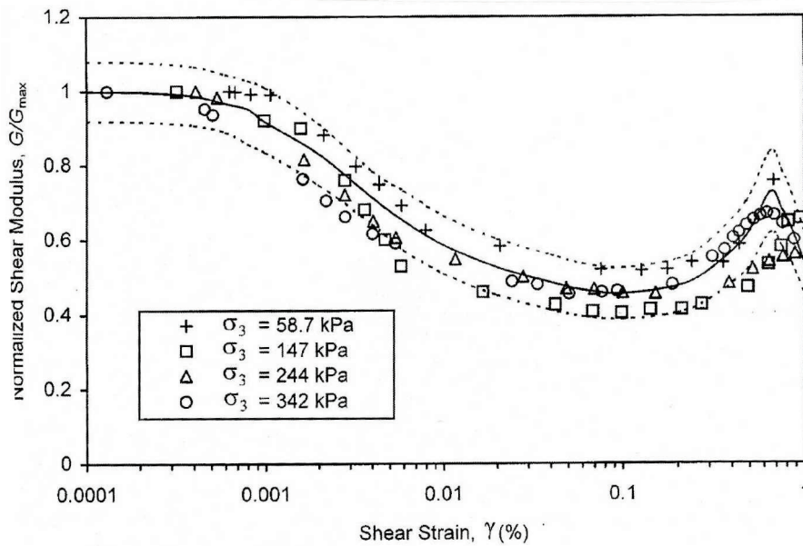
Figure 2-5. Variation of normalized shear modulus with shear strain ( d_{\max} = 1.27 cm) (from Lin et al., 2000).
