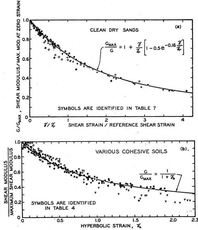
Figure 2-9. Comparison of calculated and measured values of normalized shear modulus (from Hardin and Drnevich, 1972).
