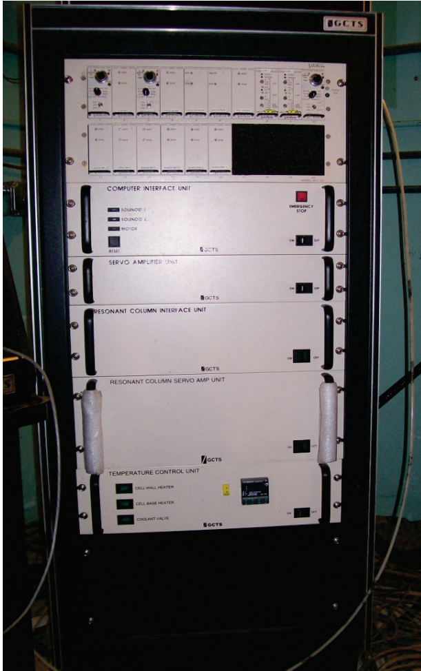
Figure 3-5. Controlling units of fixed-free RC equipment: (a) resonant column interface unit and servo amplifier unit, (b) pressure control panel, and (c) fiber optic sensor placed facing the target attached to specimen.
