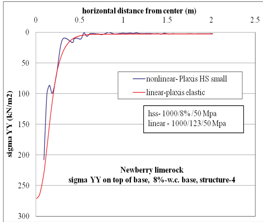
Figure C-47. \sigma_{yy} vertical stress at top of base layer comparison for nonlinear and linear cases, for Structure-4 with 8% w.c. base layer.
