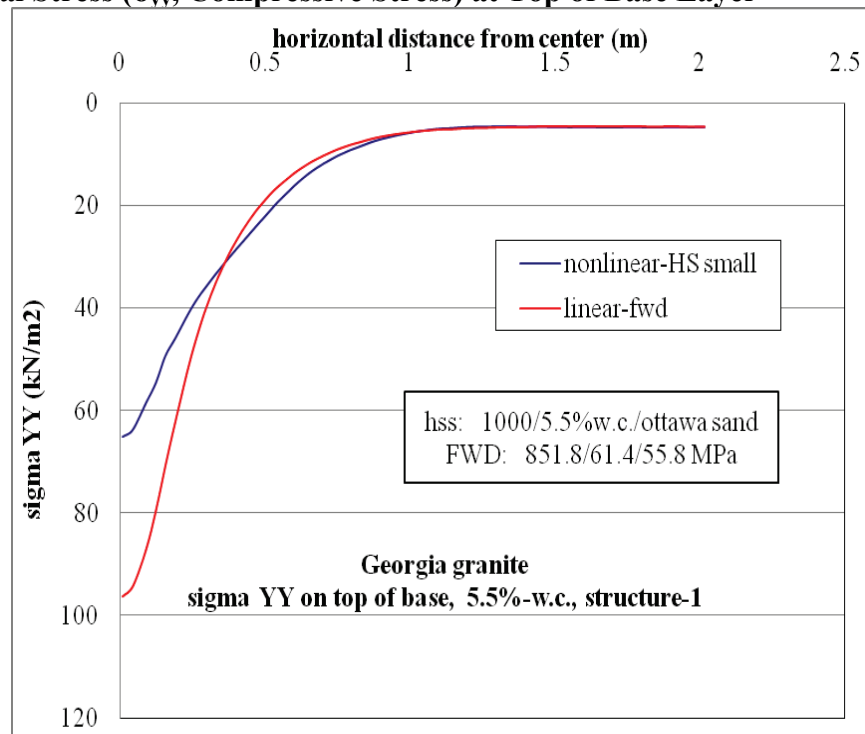
Figure D-44. \sigma_{yy} vertical stress at top of base layer comparison for nonlinear and linear cases, for Structure-1 with 5.5% w.c. base layer and nonlinear Ottawa sand subgrade.
