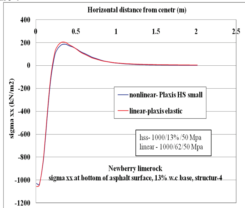
Figure C-29. \sigma_{xx} at bottom of AC layer comparison for nonlinear and linear cases, for Structure-4 with 13% w.c. base layer.
