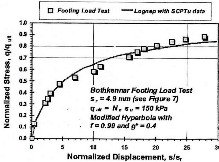
Figure 2-19. Load-displacement curves at Bothkennar footing test fitted using the proposed model (from Elhakim and Mayne, 2008).
