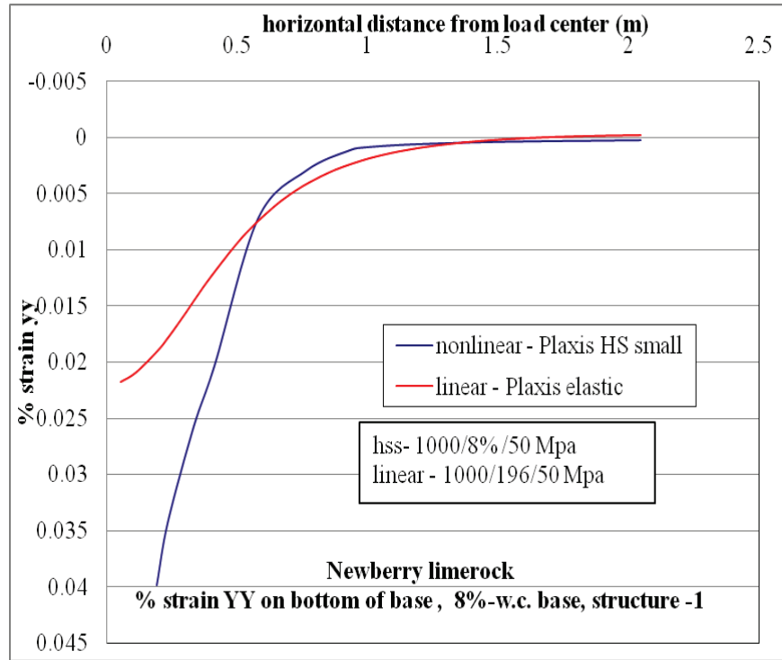
Figure C-67. \epsilon_{yy} at bottom of base layer comparison for nonlinear and linear cases, for Structure-1 with 8% w.c. base layer.
