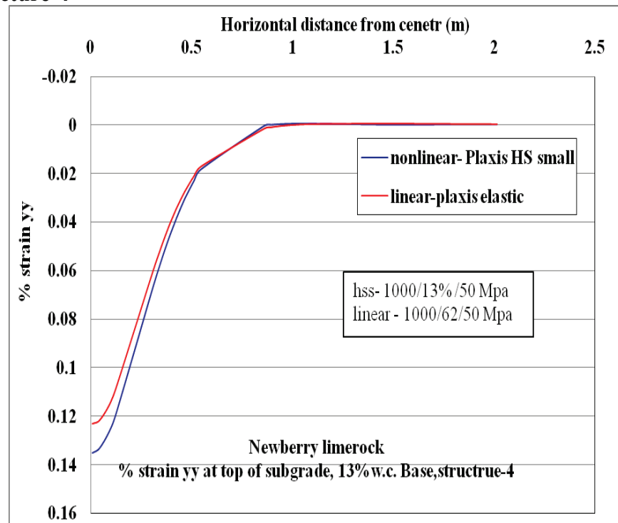
Figure C-85. \epsilon_{yy} at top of subgrade layer comparison for nonlinear and linear cases for Structure-4 with 13% w.c. base layer.
