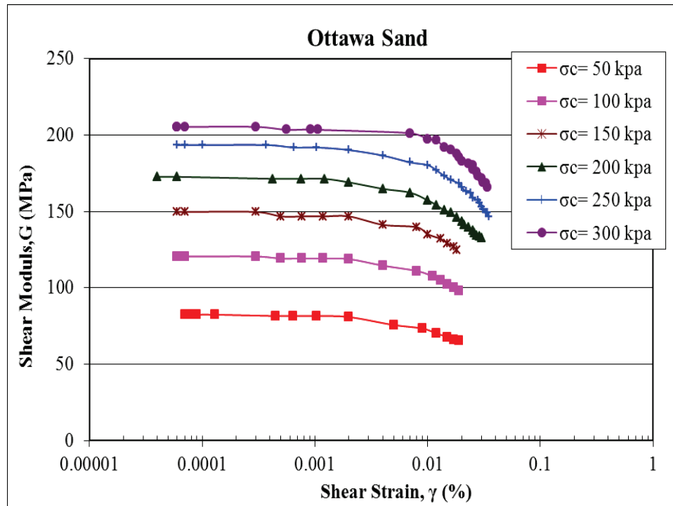
Figure 3-8. Shear modulus versus shear strain curves at different confining pressures for Ottawa sand.
