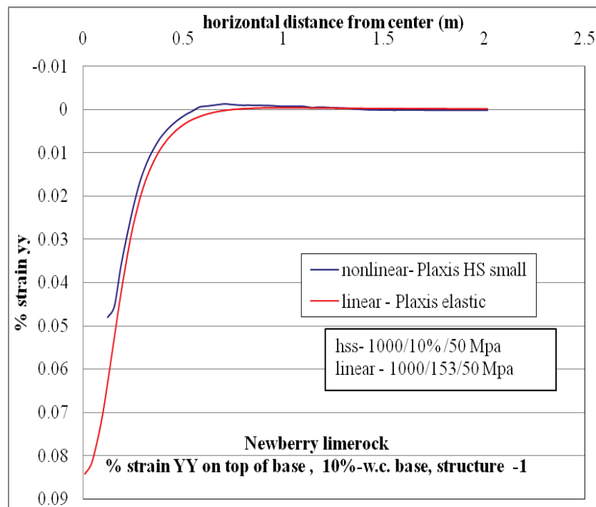
Figure C-50. \epsilon_{yy} at top of base layer comparison for nonlinear and linear cases, for Structure-1 with 10% w.c. base layer.
