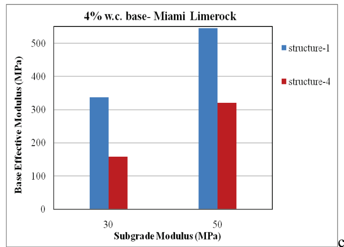
Figure 7-10. Miami limerock effective base modulus versus subgrade modulus for different structures and at constant moisture contents of: (a) 8%, (b) 6%, and (c) 4%.
