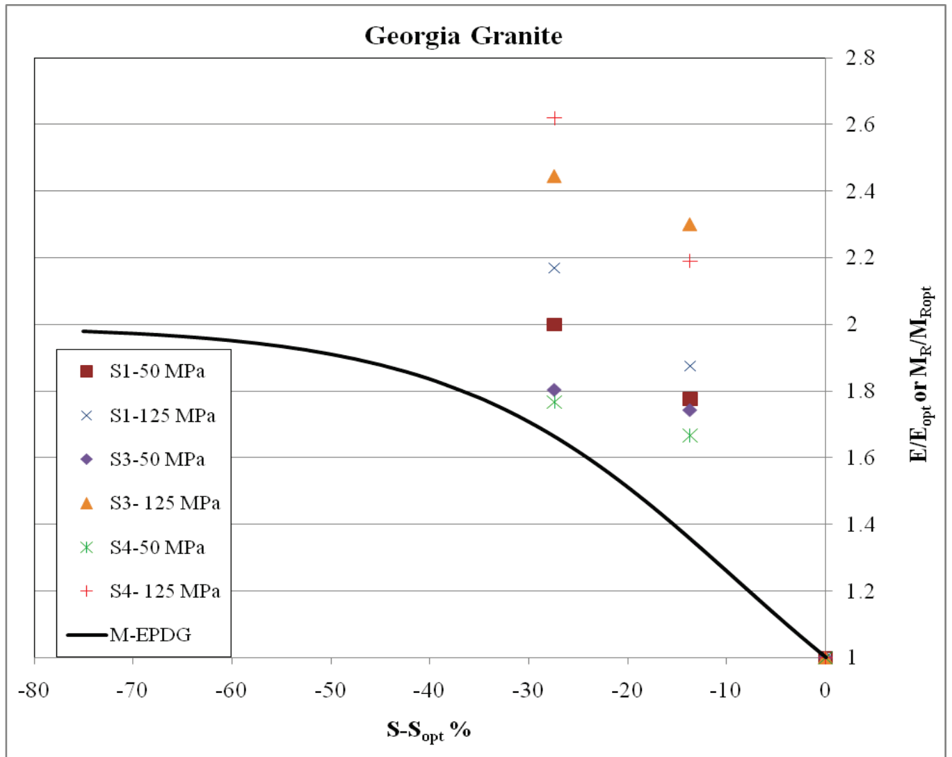
Figure 7-14. Comparison of Georgia granite effective base moduli with MEPDG model.
