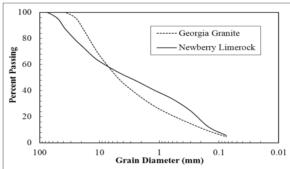
Figure 4-2. Grain size distribution.
