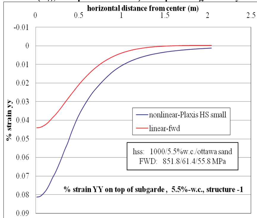
Figure D-54. \epsilon_{yy} at top of subgrade layer comparison for nonlinear and linear cases for Structure-1 with 5.5% w.c. base layer and nonlinear Ottawa sand subgrade.
