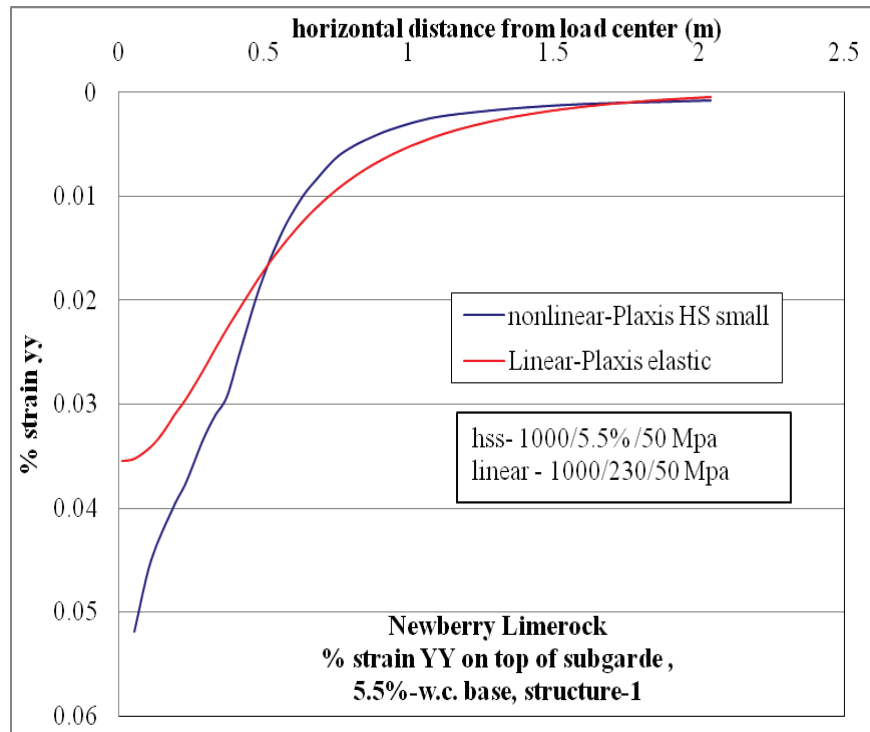
Figure C-84. \epsilon_{yy} at top of subgrade layer comparison for nonlinear and linear cases for Structure-1 with 5.5% w.c. base layer.
