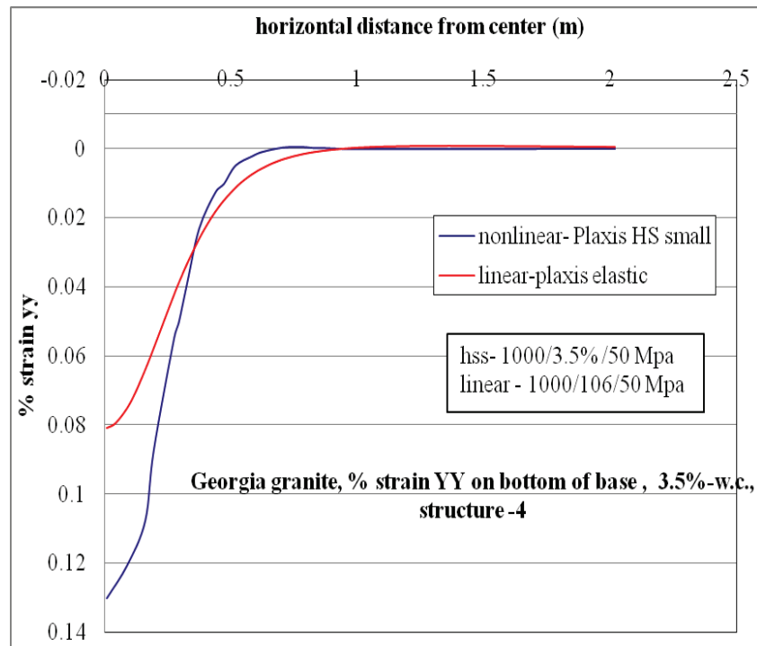
Figure C-124. \epsilon_{yy} at bottom of base layer comparison for nonlinear and linear cases, for Structure-4 with 3.5% w.c. base layer.
