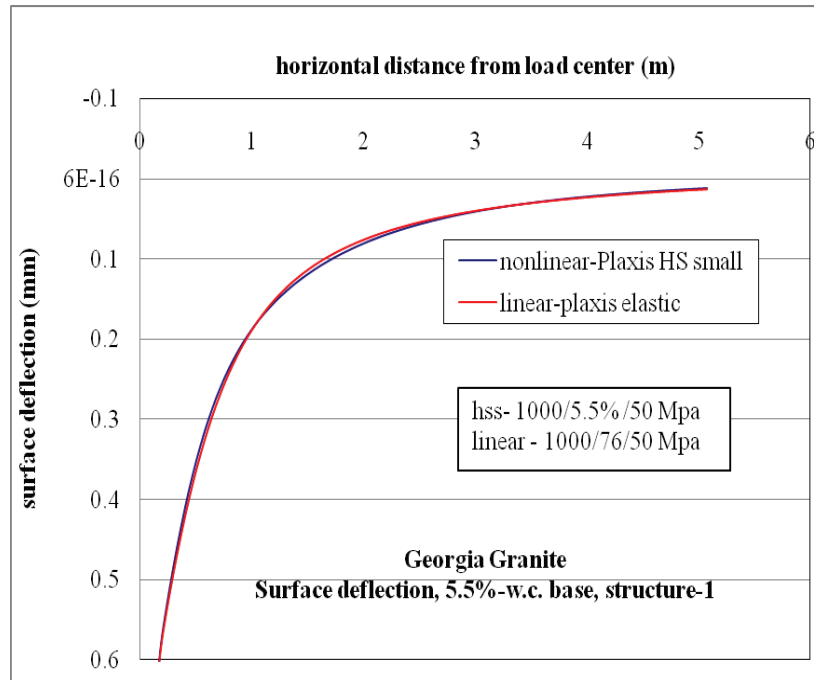
Figure C-89. Surface deflection comparison for nonlinear and linear cases, for Structure-1 with 5.5% w.c. base layer.
