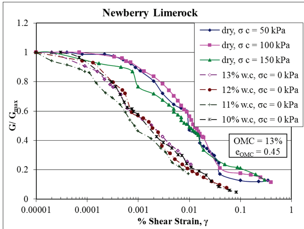
Figure 5-11. G/G_{max} versus shear strain curves for Newberry limerock for both dry and wet specimens.
