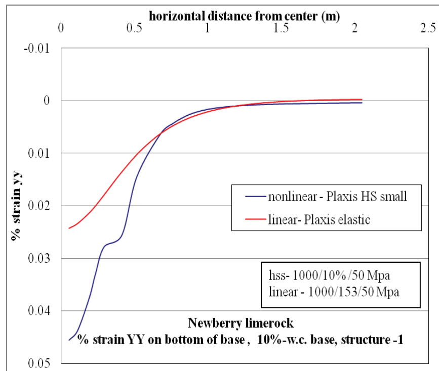
Figure C-66. \epsilon_{yy} at bottom of base layer comparison for nonlinear and linear cases, for Structure-1 with 10% w.c. base layer.
