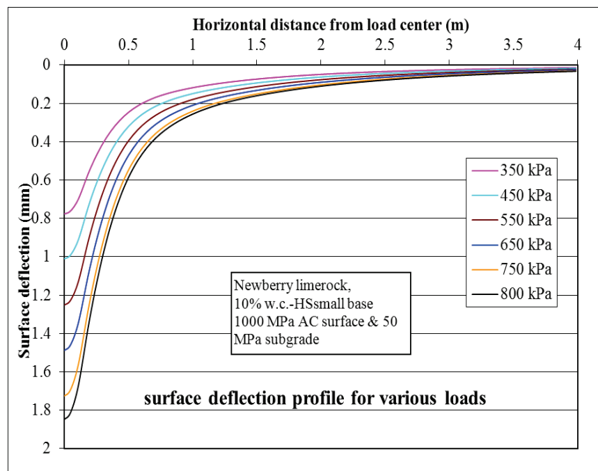
Figure 6-10. Pavement surface deflection basins for different loads demonstrating pavement model nonlinearity.
