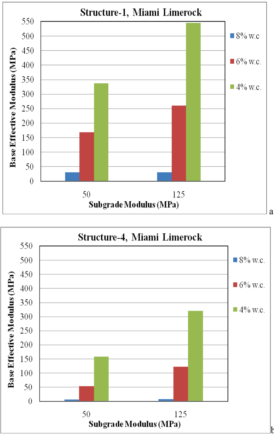
Figure 7-7. Miami limerock effective base modulus versus subgrade modulus for different moisture contents and structures: (a) Structure 1 and (b) Structure 4.
