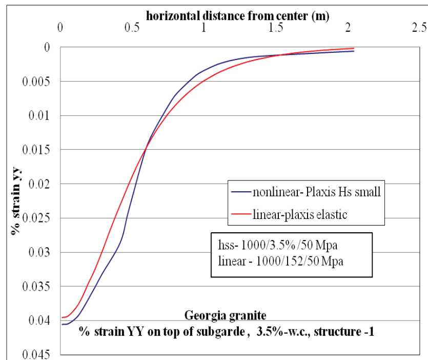
Figure C-130. \epsilon_{yy} at top of subgrade layer comparison for nonlinear and linear cases for Structure-1 with 3.5% w.c. base layer.
