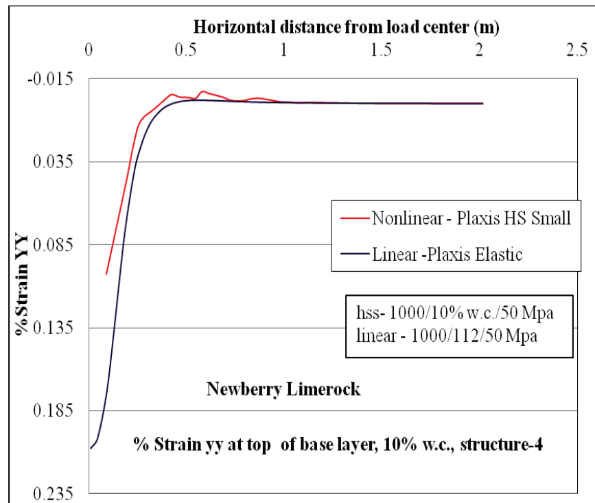
Figure C-54. \epsilon_{yy} at top of base layer comparison for nonlinear and linear cases, for Structure-4 with 10% w.c. base layer.
