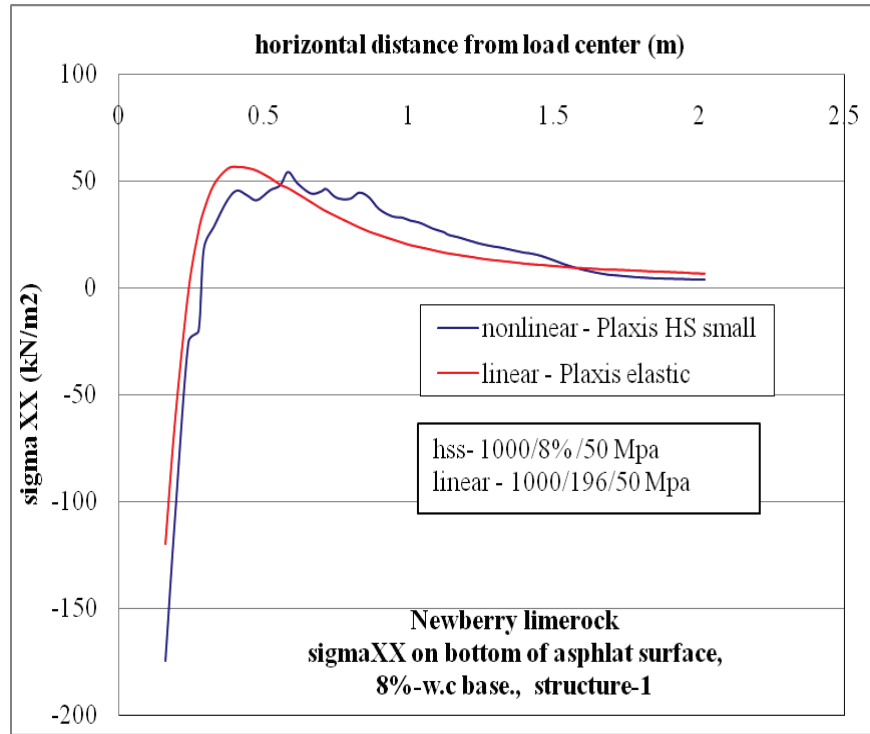
Figure C-27. \sigma_{xx} at bottom of AC layer comparison for nonlinear and linear cases, for Structure-1 with 8% w.c. base layer.
