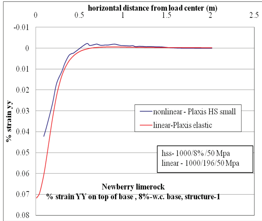
Figure C-51. \epsilon_{yy} at top of base layer comparison for nonlinear and linear cases, for Structure-1 with 8% w.c. base layer.
