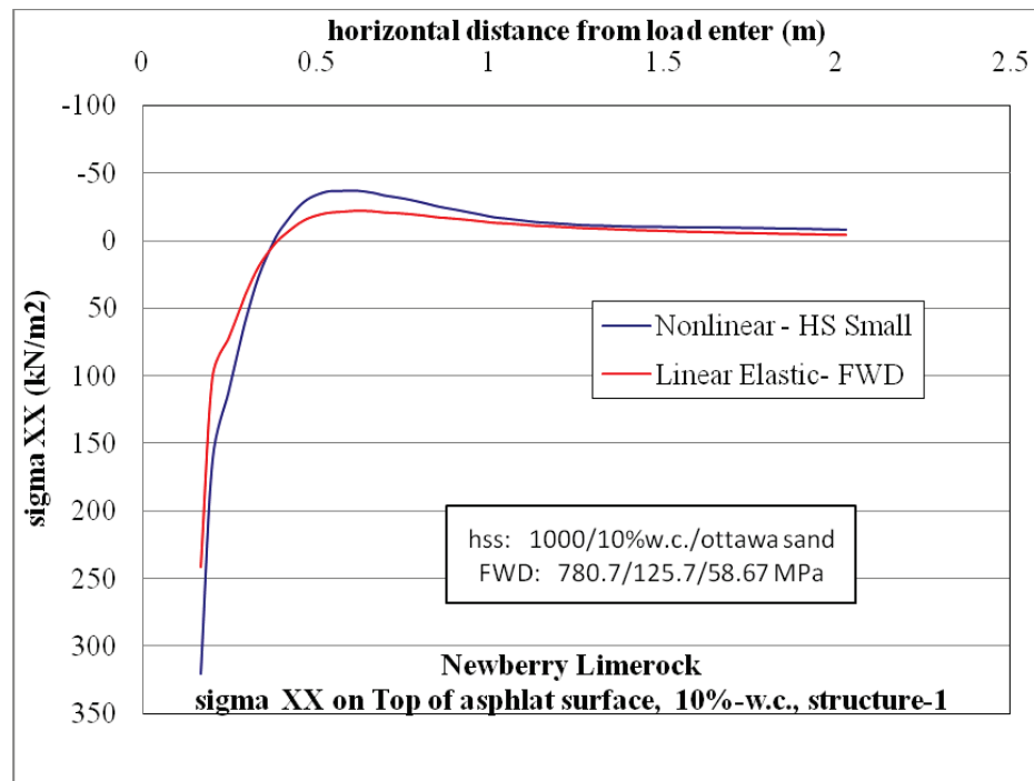
Figure D-5. \sigma_{xx} at top of AC layer comparison for nonlinear and linear cases, for Structure-1 with 10% w.c. base layer and nonlinear Ottawa sand subgrade.
