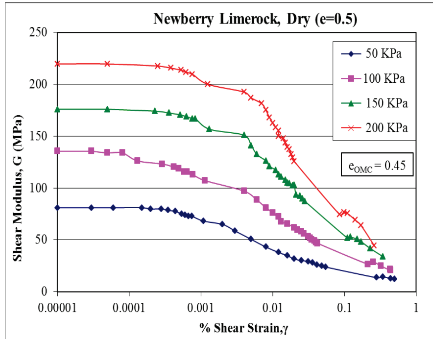
Figure A-1. Shear Modulus (G) versus % Shear strain ( \gamma ) curves for dry Newberry limerock at e=0.5 .
