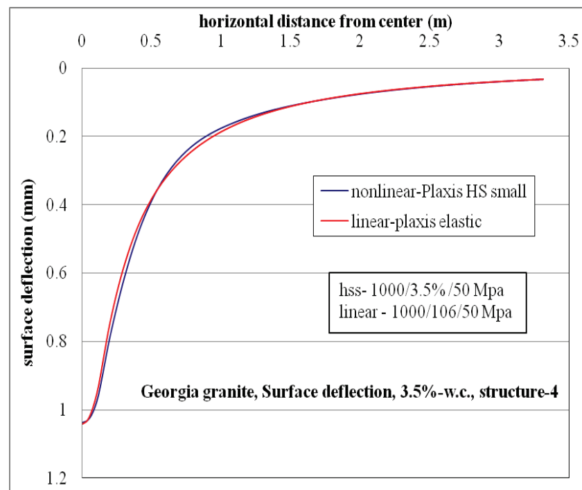
Figure C-92. Surface deflection comparison for nonlinear and linear cases, for Structure-4 with 3.5% w.c. base layer.
