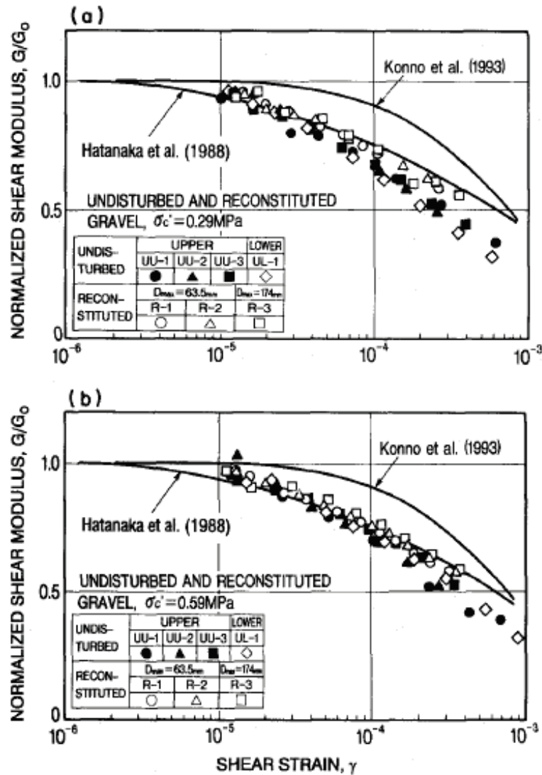
Figure 2-3. G/G_{\max} versus \log \gamma curves of undisturbed and reconstituted riverbed gravel for: (a) \sigma'_c = 0.29 \text{ MPa} and (b) \sigma'_c = 0.59 \text{ MPa} (from Yasuda et al., 1996).
