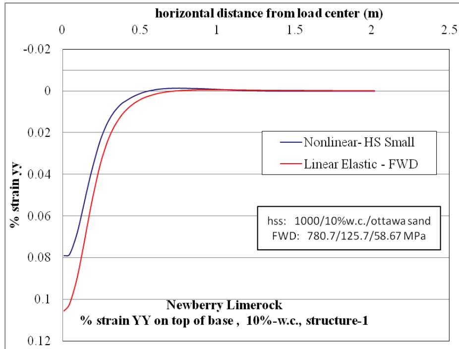
Figure D-20. \epsilon_{yy} at top of base layer comparison for nonlinear and linear cases, for Structure-1 with 10% w.c. base layer and nonlinear Ottawa sand subgrade.
