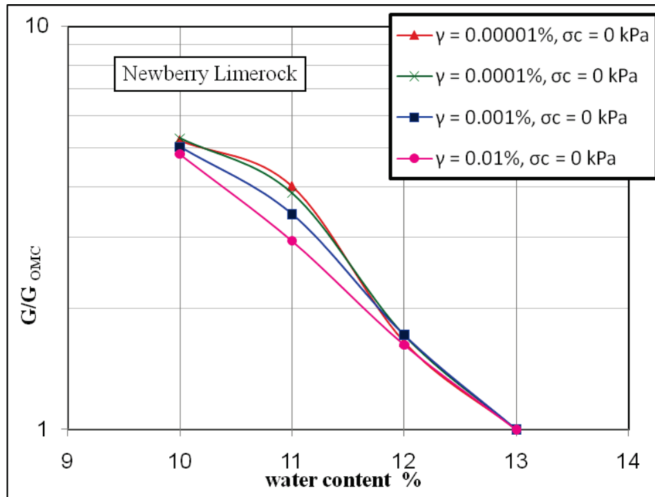
Figure 5-13. G/G_{OMC} versus moisture content at different strain levels for Newberry limerock.
