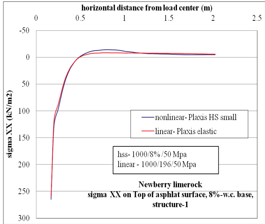
Figure C-11. \sigma_{xx} at top of AC layer comparison for nonlinear and linear cases, for Structure-1 with 8% w.c. base layer.
