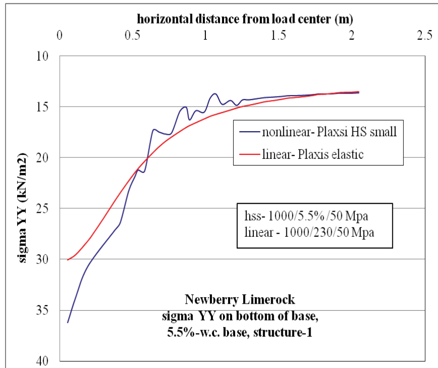
Figure C-60. \sigma_{yy} at bottom of base layer comparison for nonlinear and linear cases, for Structure-1 with 5.5% w.c. base layer.
