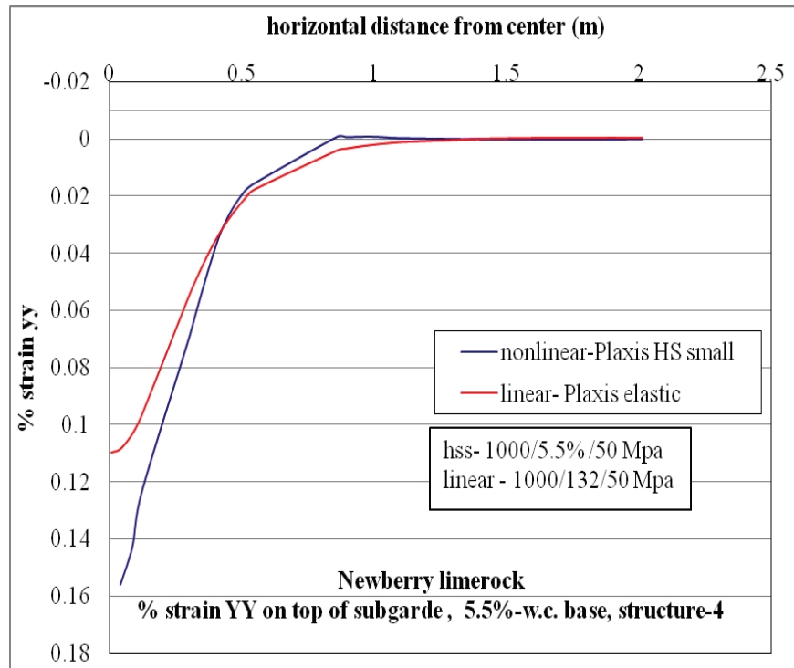
Figure C-88. \epsilon_{yy} at top of subgrade layer comparison for nonlinear and linear cases for Structure-4 with 5.5% w.c. base layer.
