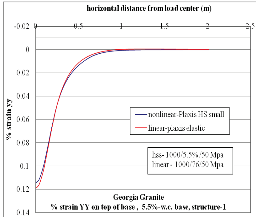
Figure C-113. \epsilon_{yy} at top of base layer comparison for nonlinear and linear cases, for Structure-1 with 5.5% w.c. base layer.
