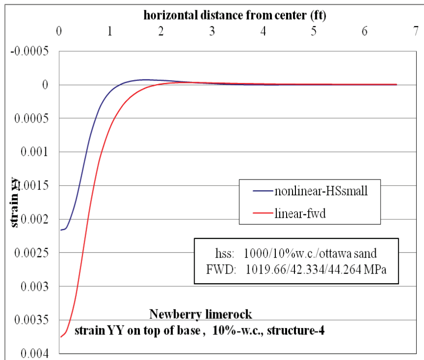
Figure D-21. \epsilon_{yy} at top of base layer comparison for nonlinear and linear cases, for Structure-4 with 10% w.c. base layer and nonlinear Ottawa sand subgrade.
