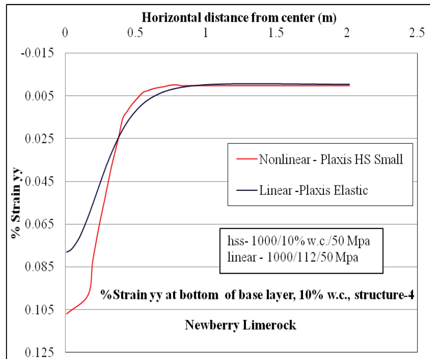
Figure C-70. \epsilon_{yy} at bottom of base layer comparison for nonlinear and linear cases, for Structure-4 with 10% w.c. base layer.
