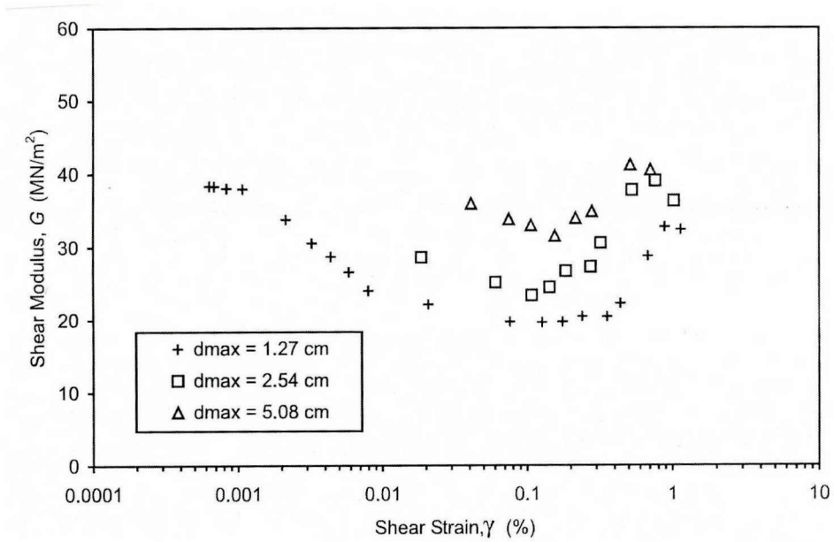
Figure 2-6. G - \gamma relationship ( \sigma_3 = 58.7 kN/m 2 ) (from Lin et al., 2000).
