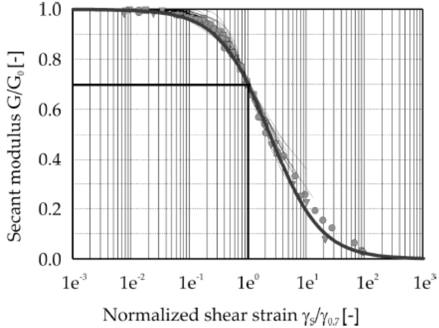
Figure 6-2. Results from modified Hardin-Drnevich relationship compared to test data by Santos and Correia (2001).
