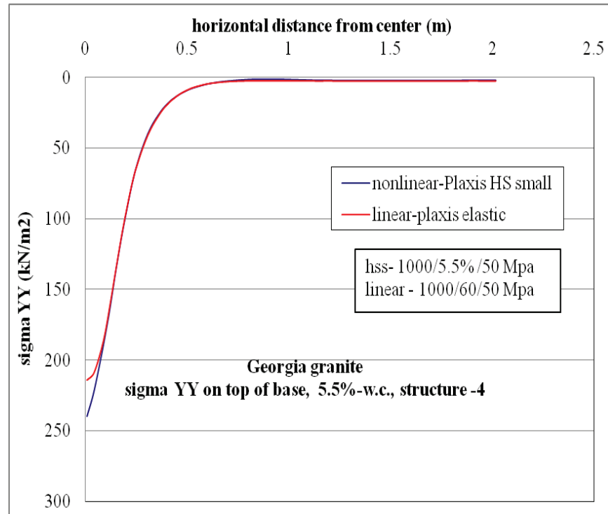
Figure C-111. \sigma_{yy} vertical stress at top of base layer comparison for nonlinear and linear cases, for Structure-4 with 5.5% w.c. base layer.
