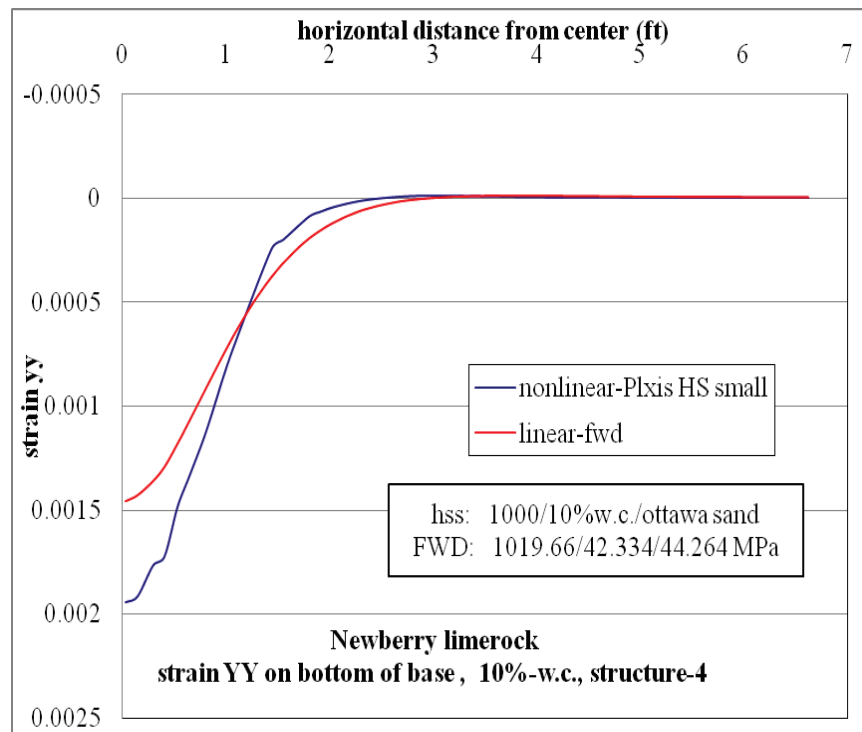
Figure D-27. \epsilon_{yy} at bottom of base layer comparison for nonlinear and linear cases, for Structure-4 with 10% w.c. base layer and nonlinear Ottawa sand subgrade.
