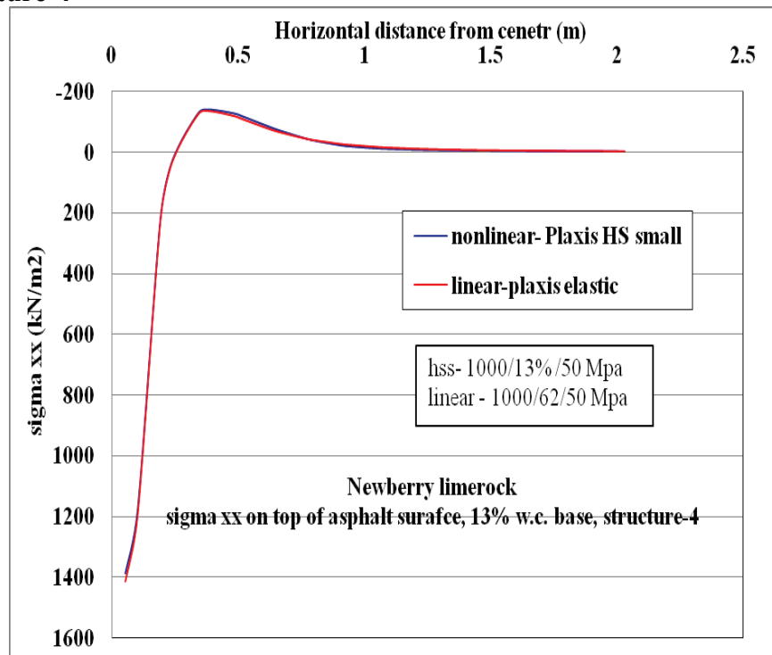
Figure C-13. \sigma_{xx} at top of AC layer comparison for nonlinear and linear cases, for Structure-4 with 13% w.c. base layer.
