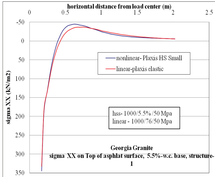
Figure C-93. \sigma_{xx} at top of AC layer comparison for nonlinear and linear cases, for Structure-1 with 5.5% w.c. base layer.
