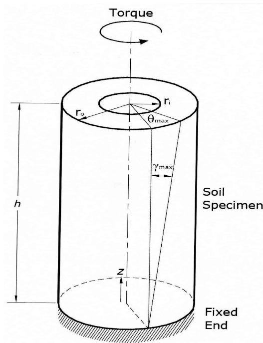
Figure 3-2. Shear strain in soil specimen.
