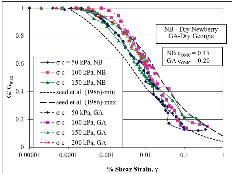
Figure 5-5. Comparison of G/G_{\max} versus shear strain ( \gamma ) data of Newberry limerock and Georgia granite with Seed and Idriss (1986) maximum and minimum limits.
