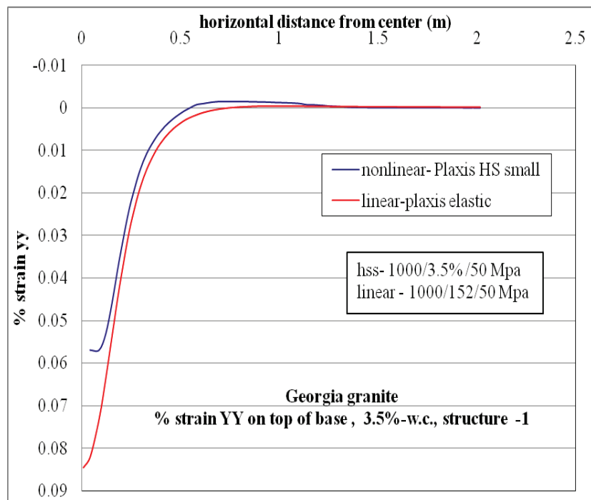
Figure C-114. \epsilon_{yy} at top of base layer comparison for nonlinear and linear cases, for Structure-1 with 3.5% w.c. base layer.
