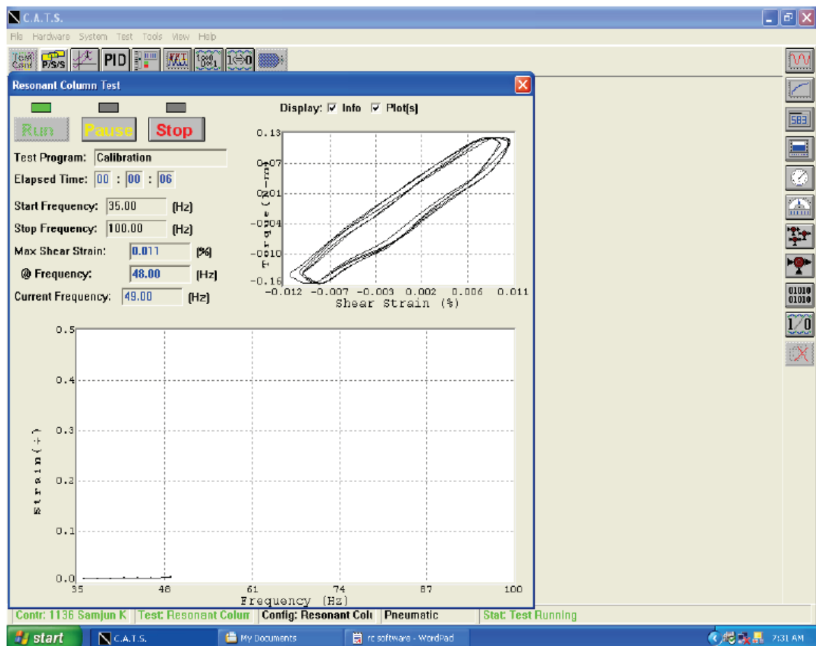
Figure 3-6. Real-time test execution window showing resonant frequency and loading loop.
