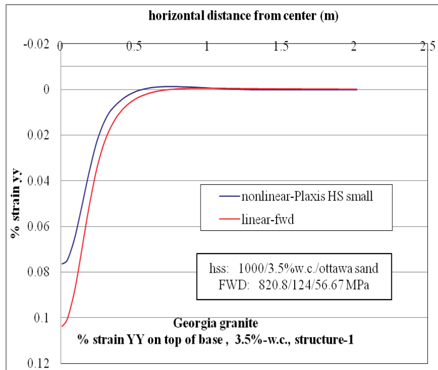
Figure D-47. \epsilon_{yy} at top of base layer comparison for nonlinear and linear cases, for Structure-1 with 3.5% w.c. base layer and nonlinear Ottawa sand subgrade.
