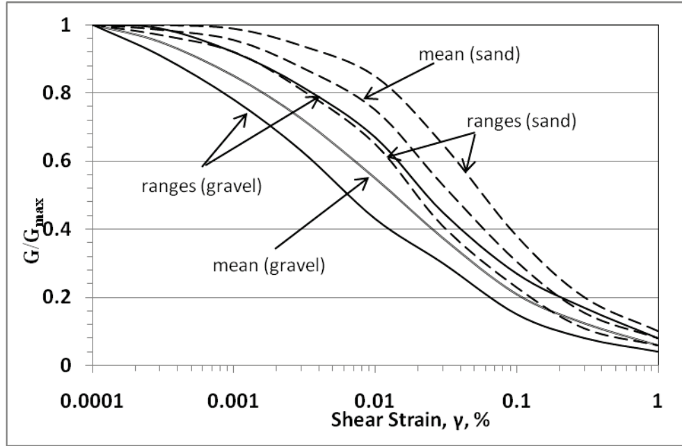
Figure 2-2. G/G_{max} versus \log \gamma curves of gravelly sandy soils reported by Seed et al. (1986).
