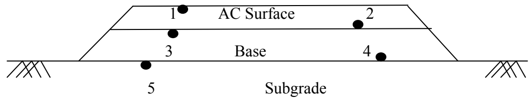
Figure 7-1. Critical locations for pavement response analysis (1=top of AC surface layer, 2=bottom of AC surface layer, 3=top of base layer, 4=bottom of base layer, and 5=top of subgrade layer).
