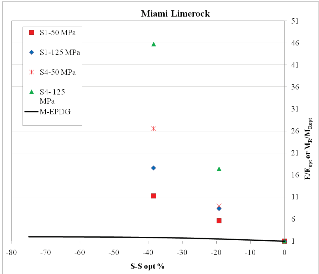
Figure 7-15. Comparison of Miami limerock effective base moduli with MEPDG model.
