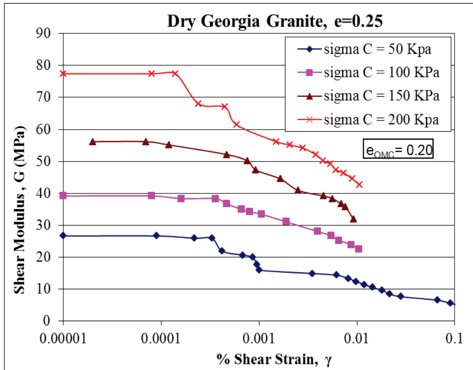
Figure A-5. Shear Modulus (G) versus % Shear strain ( \gamma ) curves for dry Georgia granite at e=0.25 .
