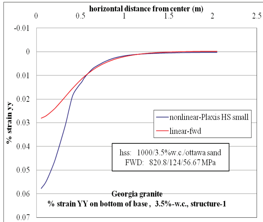
Figure D-51. \epsilon_{yy} at bottom of base layer comparison for nonlinear and linear cases, for Structure-1 with 3.5% w.c. base layer and nonlinear Ottawa sand subgrade.
