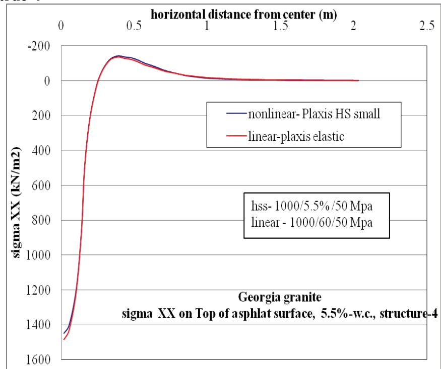
Figure C-95. \sigma_{XX} at top of AC layer comparison for nonlinear and linear cases, for Structure-4 with 5.5% w.c. base layer.
