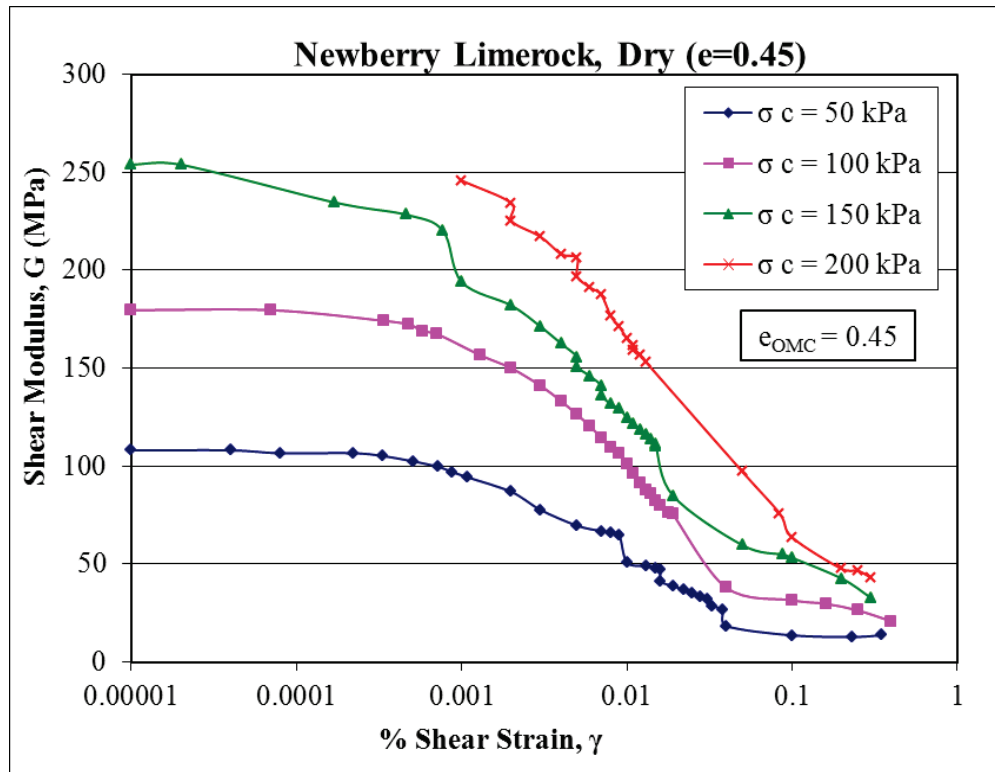
Figure 5-1. Shear modulus ( G ) versus shear strain ( \gamma ) curves for dry Newberry limerock at e_{OMC} (i.e., e = 0.45 ).
