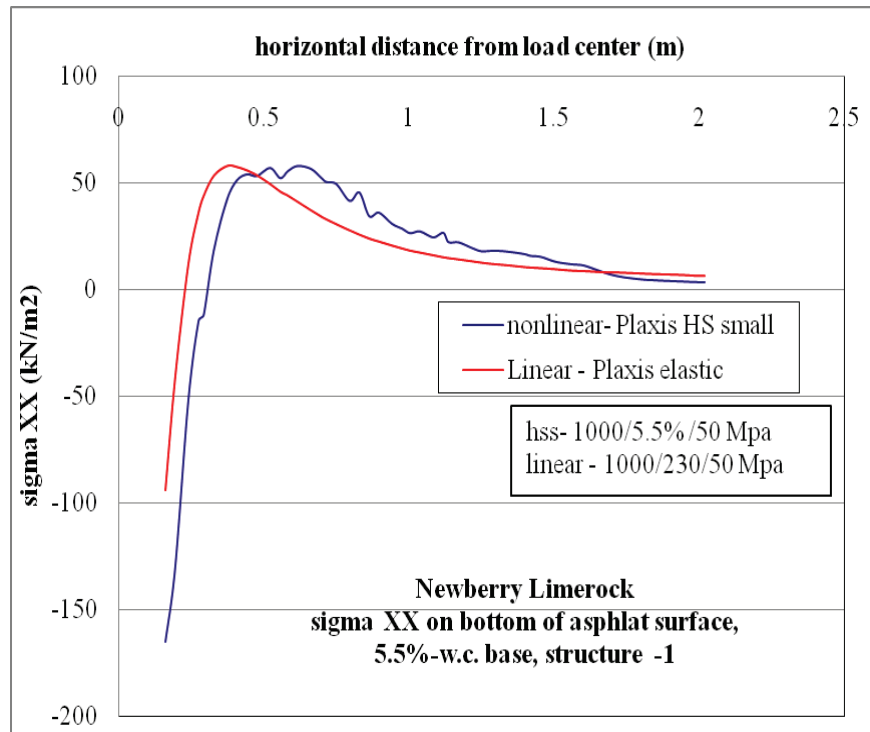
Figure C-28. \sigma_{xx} at bottom of AC layer comparison for nonlinear and linear cases, for Structure-1 with 5.5% w.c. base layer.
