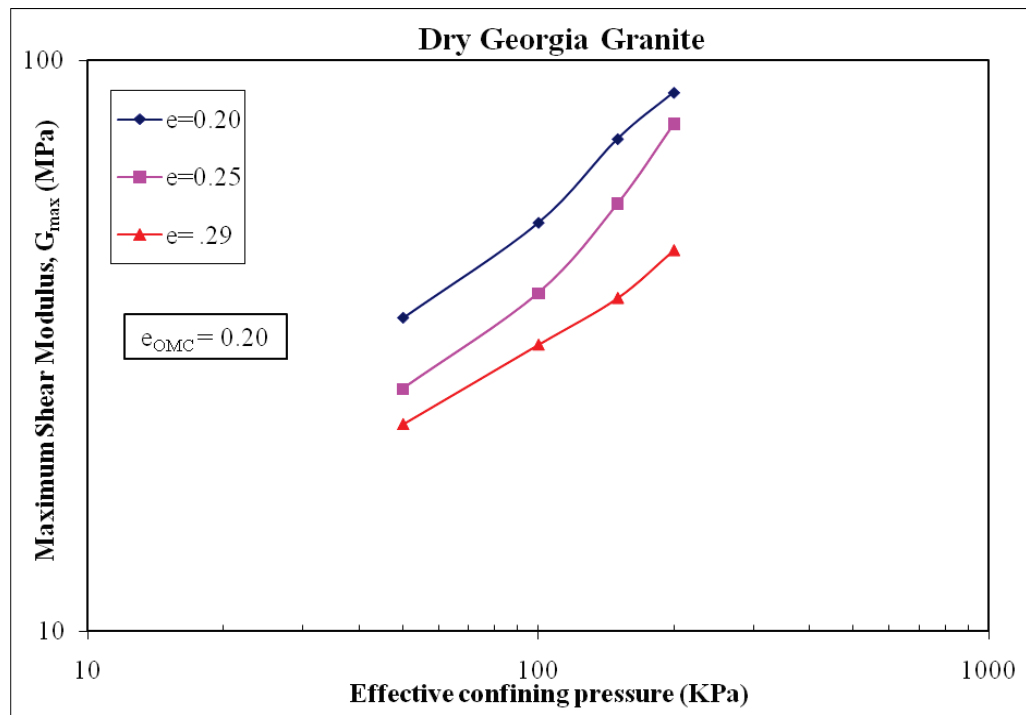
Figure 5-7. G_{\max} versus confining pressure for Georgia granite at different void ratios.
