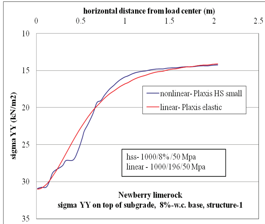
Figure C-75. \sigma_{yy} at top of subgrade comparison for nonlinear and linear cases, for Structure-1 with 8% w.c. base layer.
