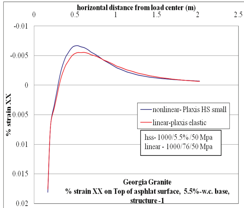
Figure C-97. \epsilon_{xx} at top of AC layer comparison for nonlinear and linear cases, for Structure-1 with 5.5% w.c. base layer.
