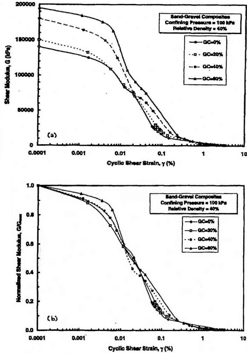
Figure 2-11. (a) G versus \gamma curves and (b) G/G_{\max} versus \gamma curves determined for test specimens containing 0, 20, 40 and 60% gravel size particles (from Rollins et al., 1998).
