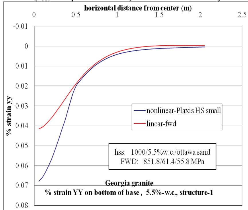
Figure D-50. \epsilon_{yy} at bottom of base layer comparison for nonlinear and linear cases, for Structure-1 with 5.5% w.c. base layer and nonlinear Ottawa sand subgrade.
