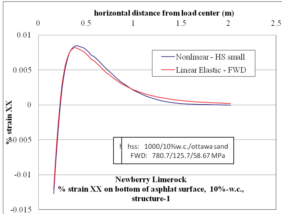
Figure D-14. \epsilon_{xx} at bottom of AC layer comparison for nonlinear and linear cases, for Structure-1 with 10% w.c. base layer and nonlinear Ottawa sand subgrade.
