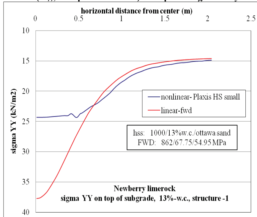
Figure D-28. \sigma_{yy} at top of subgrade comparison for nonlinear and linear cases, for Structure-1 with 13% w.c. base layer and nonlinear Ottawa sand subgrade.
