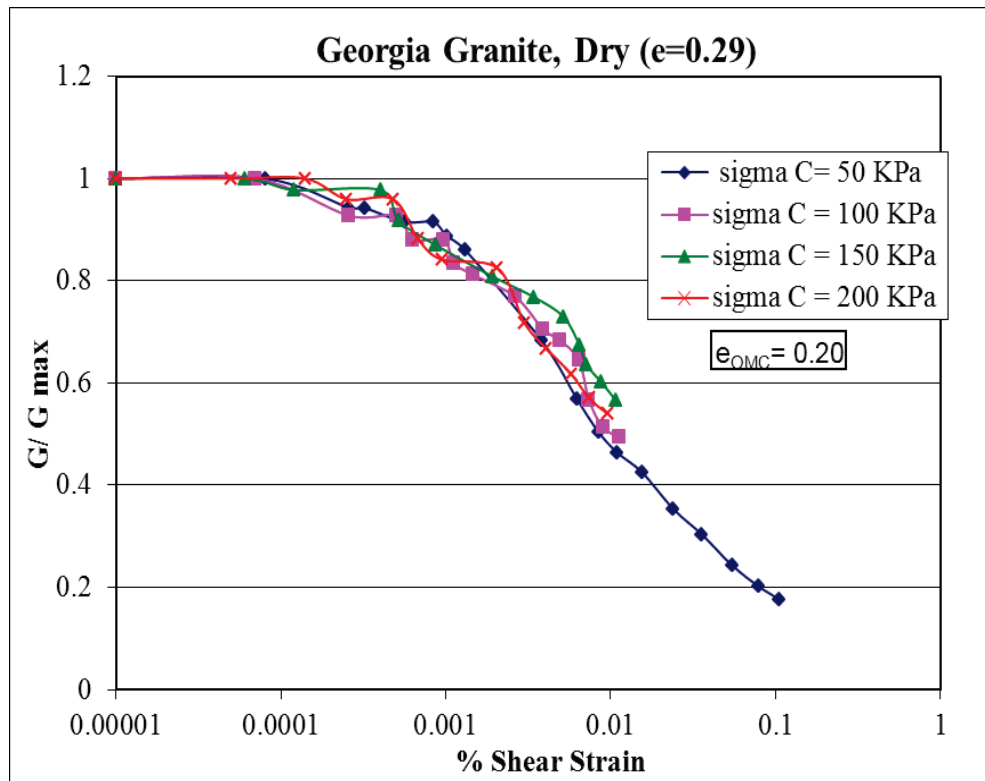
Figure A-8. G/G_{\max} versus % shear strain( \gamma ) curves at e=0.29 for Georgia granite.
