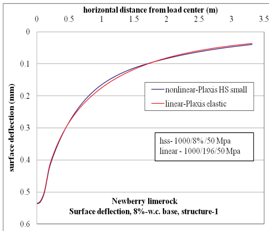
Figure C-3. Surface deflection comparison for nonlinear and linear cases, for Structure-1 with 8% w.c. base layer.
