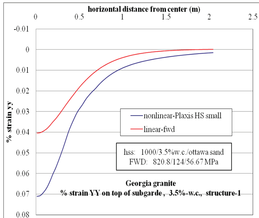
Figure D-55. \epsilon_{yy} at top of subgrade layer comparison for nonlinear and linear cases for Structure-1 with 3.5% w.c. base layer and nonlinear Ottawa sand subgrade.
