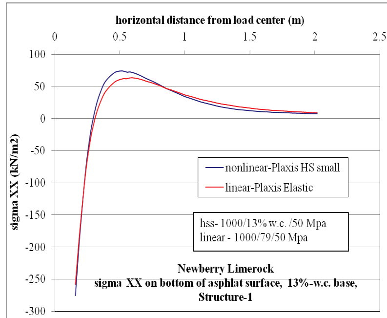
Figure C-25. \sigma_{xx} at bottom of AC layer comparison for nonlinear and linear cases, for Structure-1 with 13% w.c. base layer.
