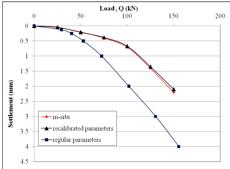
Figure 6-7b. Comparison of actual settlements with settlements predicted using recalibrated parameters and Plaxis-HSsmall footing model.
