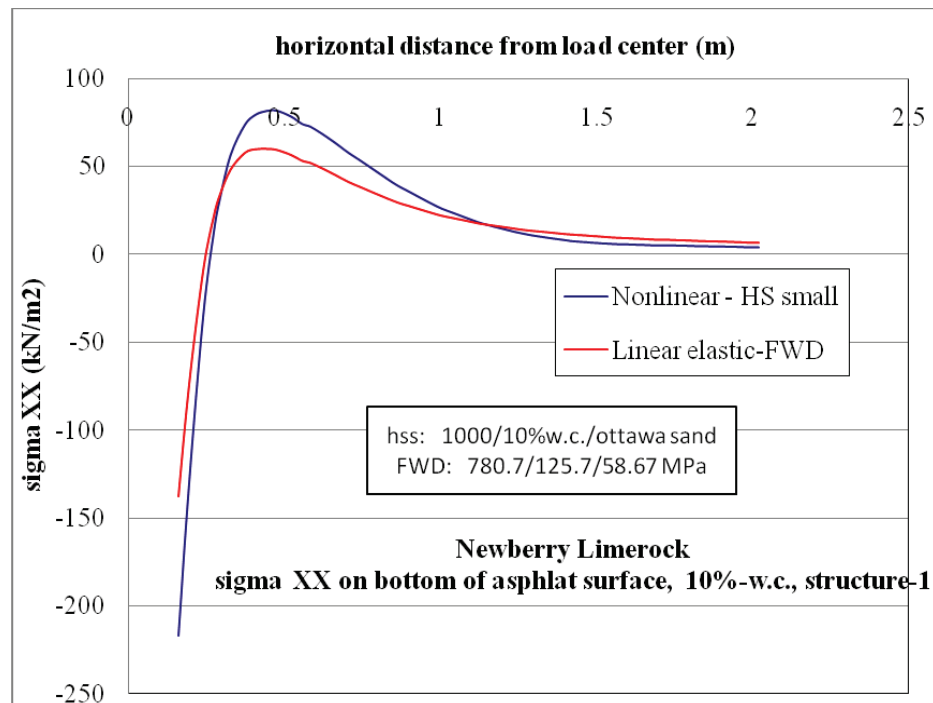
Figure D-11. \sigma_{xx} at bottom of AC layer comparison for nonlinear and linear cases, for Structure-1 with 10% w.c. base layer and nonlinear Ottawa sand subgrade.
