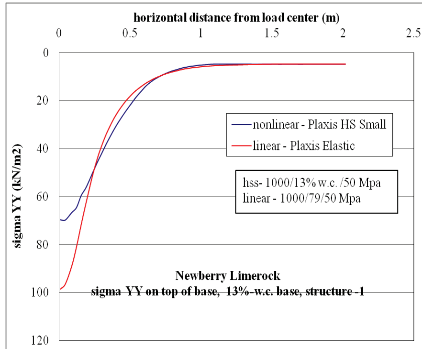
Figure C-41. \sigma_{yy} vertical stress at top of base layer comparison for nonlinear and linear cases, for Structure-1 with 13% w.c. base layer.
