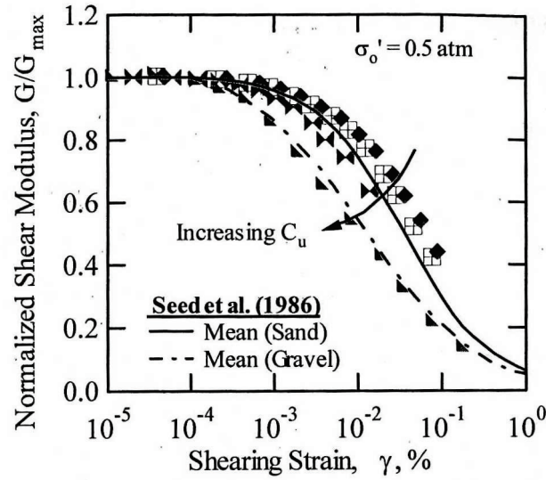
Figure 2-8. G/G_{max} - \log \gamma relationship for gravelly soils (from Menq, 2003).
