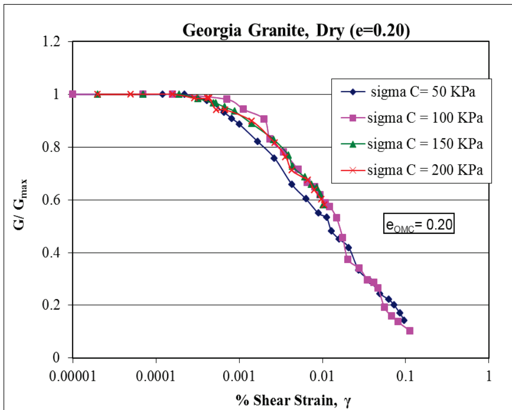
Figure 5-4. G/G_{max} versus shear strain ( \gamma ) curves at e = e_{OMC} for Georgia granite.
