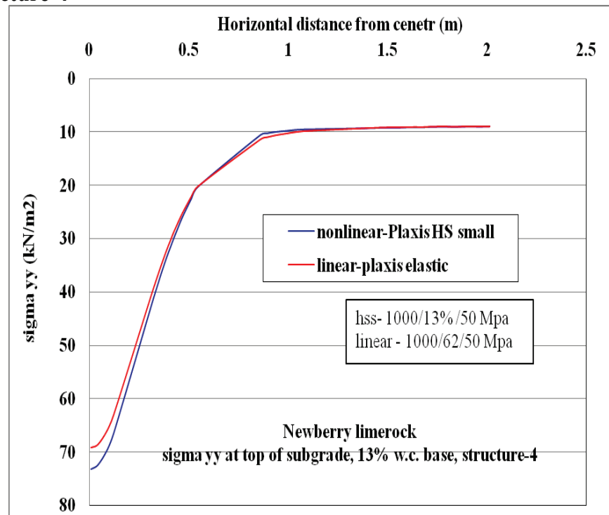
Figure C-77. \sigma_{yy} at top of subgrade comparison for nonlinear and linear cases, for Structure-4 with 13% w.c. base layer.
