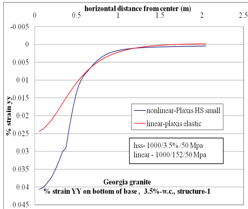
Figure C-122. \epsilon_{yy} at bottom of base layer comparison for nonlinear and linear cases, for Structure-1 with 3.5% w.c. base layer.
