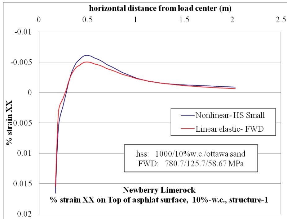
Figure D-8. \epsilon_{xx} at top of AC layer comparison for nonlinear and linear cases, for Structure-1 with 10% w.c. base layer and nonlinear Ottawa sand subgrade.
