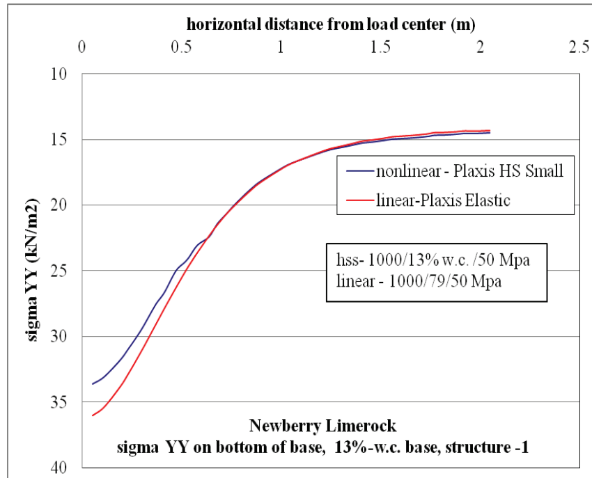
Figure C-57. \sigma_{yy} at bottom of base layer comparison for nonlinear and linear cases, for Structure-1 with 13% w.c. base layer.
