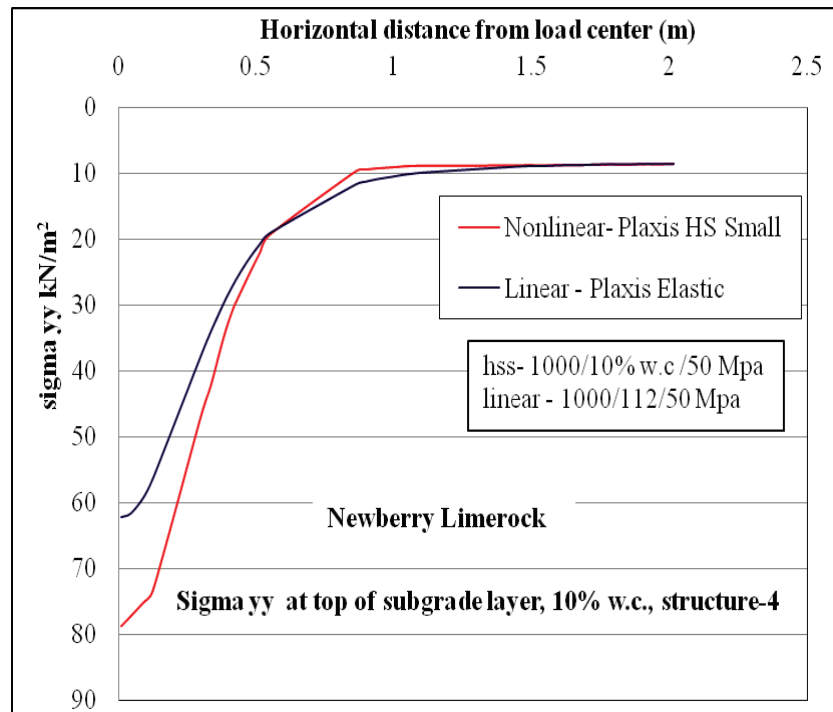
Figure C-78. \sigma_{yy} at top of subgrade comparison for nonlinear and linear cases, for Structure-4 with 10% w.c. base layer.
