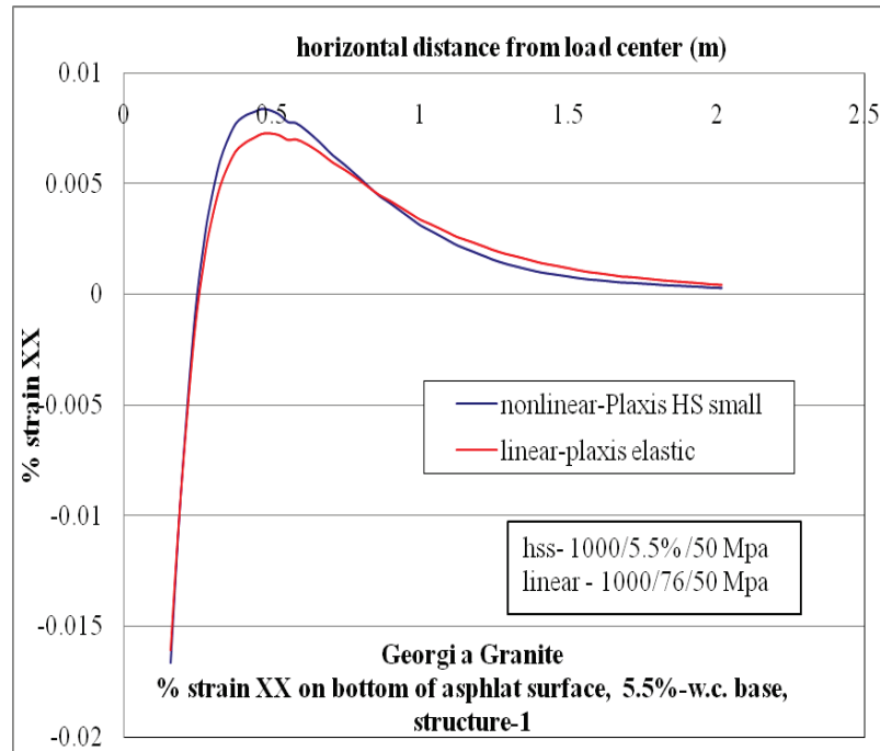
Figure C-105. \epsilon_{xx} at bottom of AC layer comparison for nonlinear and linear cases, for Structure-1 with 5.5% w.c. base layer.
