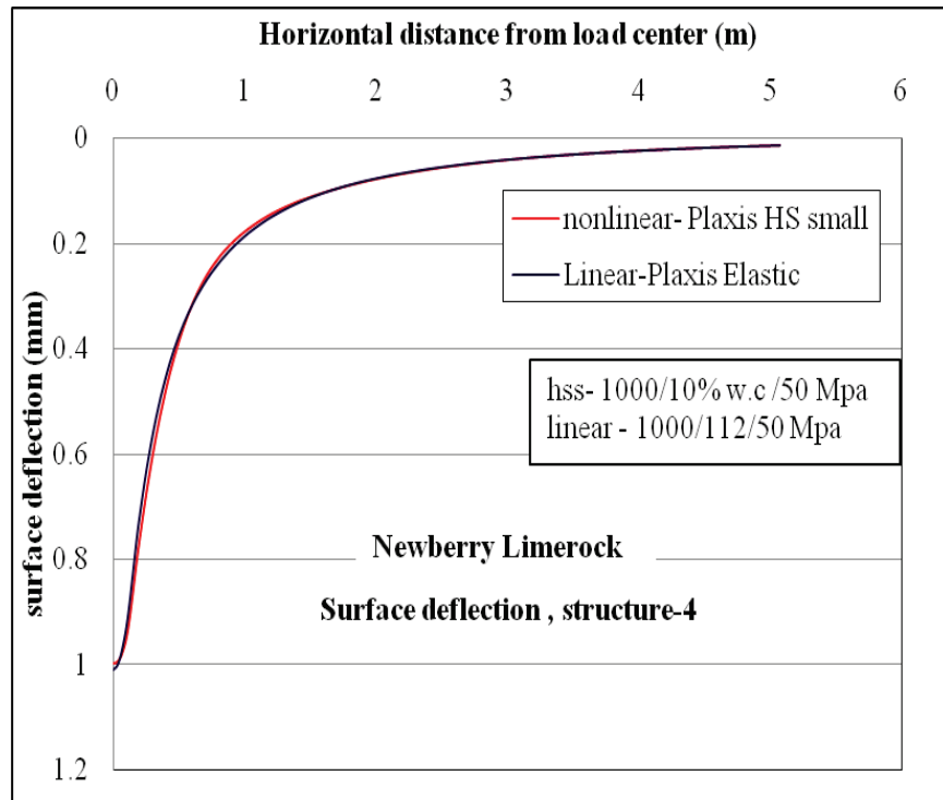
Figure C-6. Surface deflection comparison for nonlinear and linear cases, for Structure-4 with 10% w.c. base layer.
