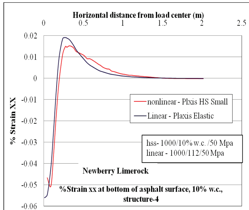
Figure C-38. \epsilon_{xx} at bottom of AC layer comparison for nonlinear and linear cases, for Structure-4 with 10% w.c. base layer.
