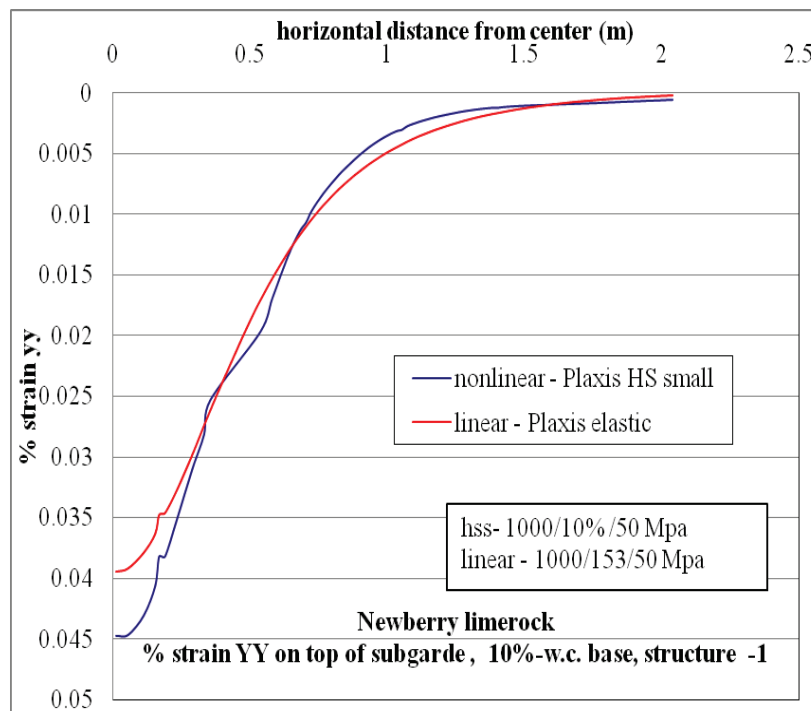
Figure C-82. \epsilon_{yy} at top of subgrade layer comparison for nonlinear and linear cases for Structure-1 with 10% w.c. base layer.
