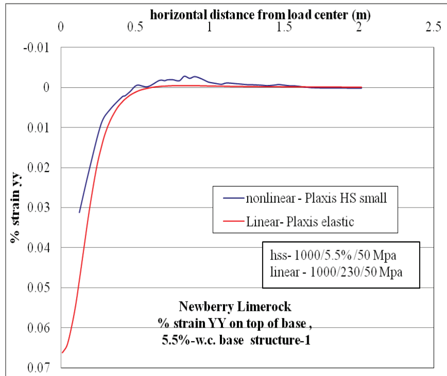
Figure C-52. \epsilon_{yy} at top of base layer comparison for nonlinear and linear cases, for Structure-1 with 5.5% w.c. base layer.
