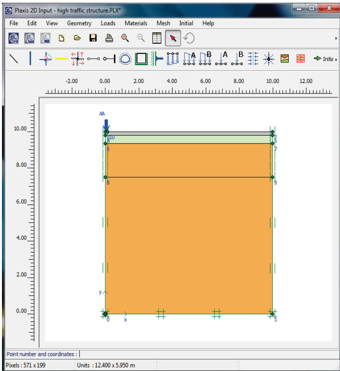
Figure 6-4a. Typical Plaxis-HSsmall model cross-section used for nonlinear analysis.
