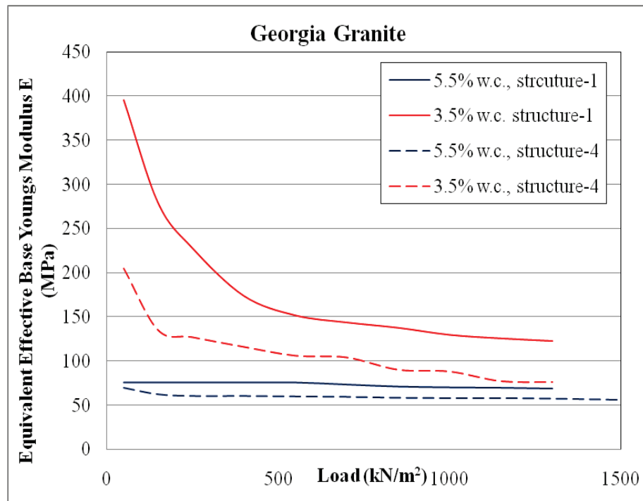
Figure 7-4. Nonlinear variation of effective modulus with increase in load for Georgia granite base at 5.5% and 3.5% moisture contents.
