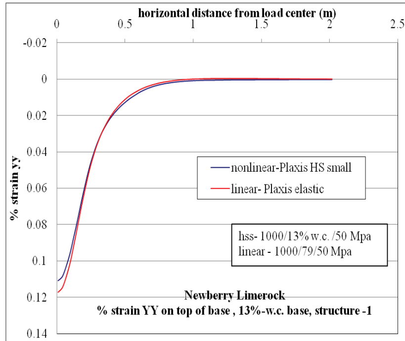
Figure C-49. \epsilon_{yy} at top of base layer comparison for nonlinear and linear cases, for Structure-1 with 13% w.c. base layer.
