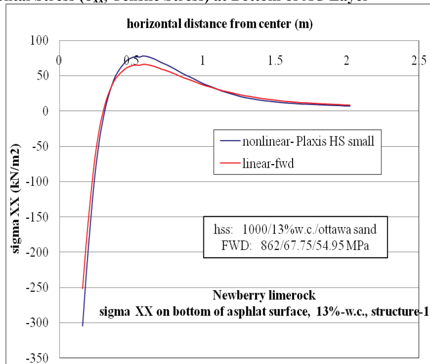
Figure D-10. \sigma_{xx} at bottom of AC layer comparison for nonlinear and linear cases, for Structure-1 with 13% w.c. base layer and nonlinear Ottawa sand subgrade.
