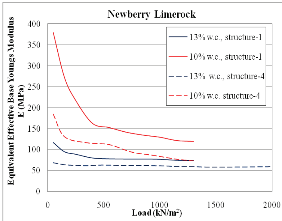
Figure 7-3. Nonlinear variation of effective modulus with increase in load for Newberry limerock base at 13% and 10% moisture contents.
