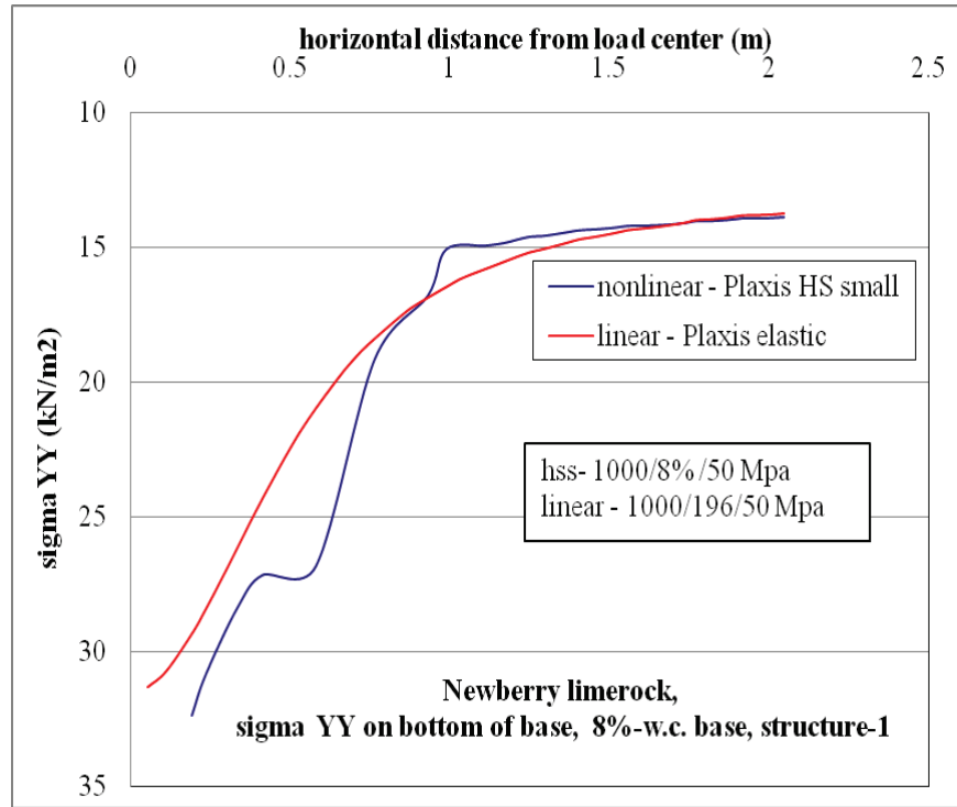
Figure C-59. \sigma_{yy} at bottom of base layer comparison for nonlinear and linear cases, for Structure-1 with 8% w.c. base layer.
