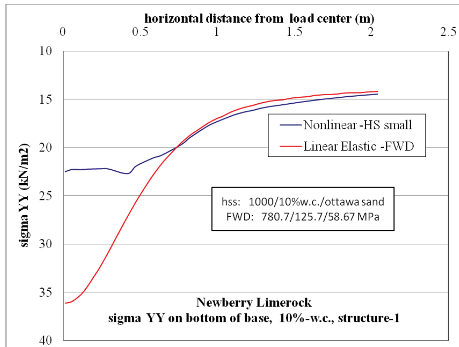
Figure D-29. \sigma_{yy} at top of subgrade comparison for nonlinear and linear cases, for Structure-1 with 10% w.c. base layer and nonlinear Ottawa sand subgrade.
