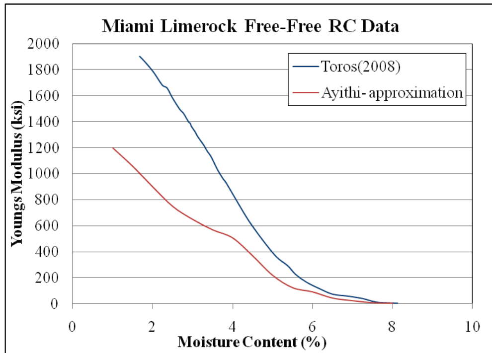
Figure 6-8. G_{\max} versus moisture content for Miami limerock.
