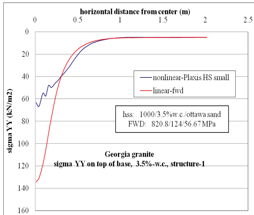
Figure D-45. \sigma_{yy} vertical stress at top of base layer comparison for nonlinear and linear cases, for Structure-1 with 3.5% w.c. base layer and nonlinear Ottawa sand subgrade.
