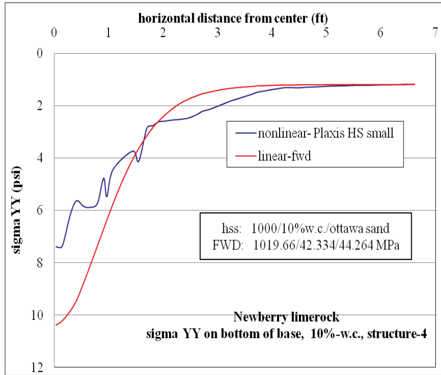
Figure D-24. \sigma_{yy} at bottom of base layer comparison for nonlinear and linear cases, for Structure-4 with 10% w.c. base layer and nonlinear Ottawa sand subgrade.
