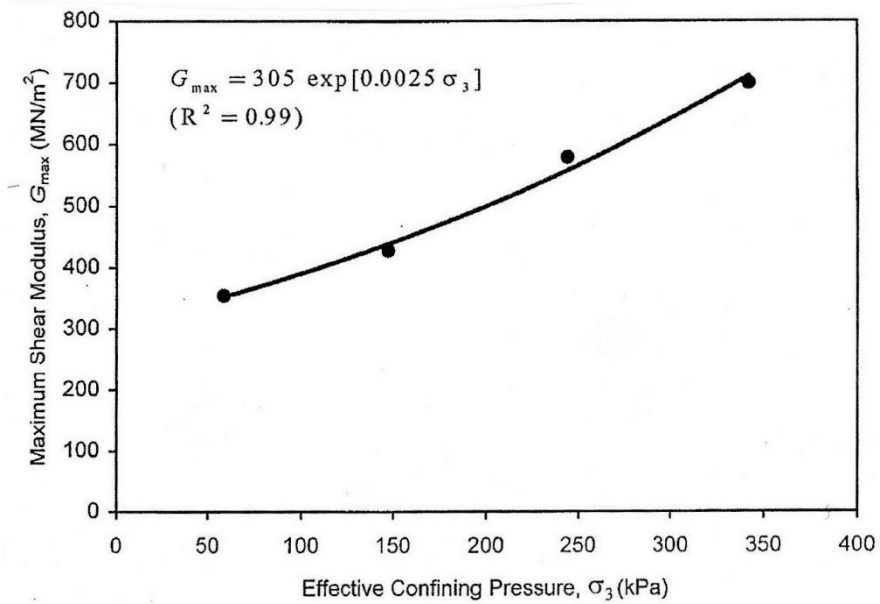
Figure 2-7. Variation of G_{max} of the field deposit with \sigma_3 (from Lin et al., 2000).
