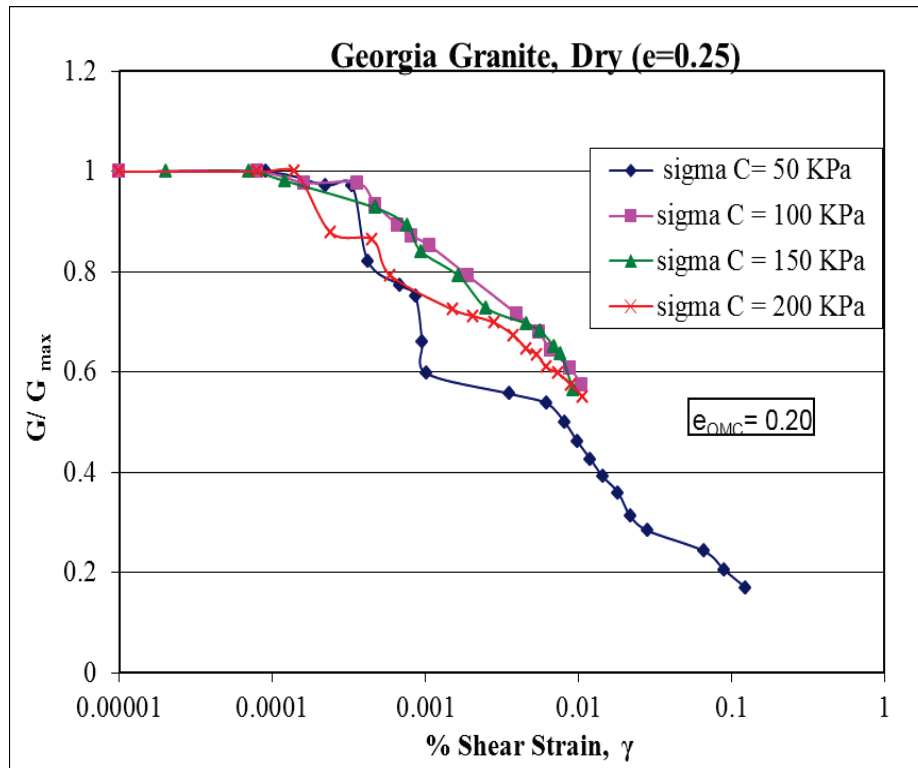
Figure A-7. G/G_{\max} versus % shear strain( \gamma ) curves at e=0.25 for Georgia granite.
