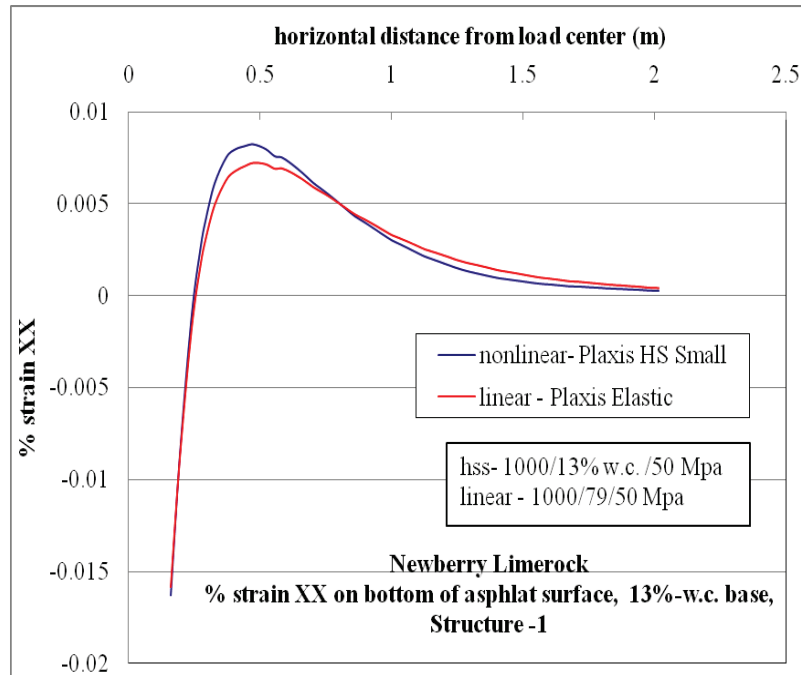
Figure C-33. \epsilon_{xx} at bottom of AC layer comparison for nonlinear and linear cases, for Structure-1 with 13% w.c. base layer.
