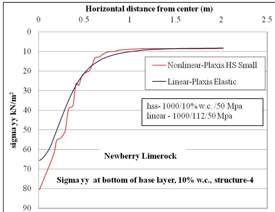
Figure C-62. \sigma_{yy} at bottom of base layer comparison for nonlinear and linear cases, for Structure-4 with 10% w.c. base layer.
