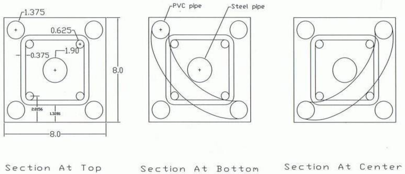
Figure 4-1 Cross-sectional views of jet-grouted pile group.
