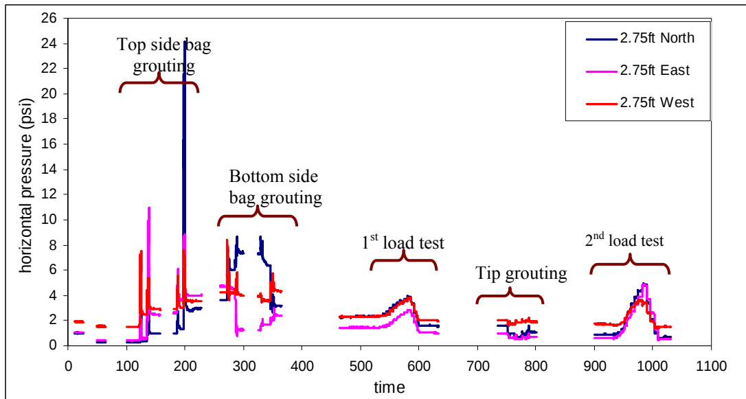
Figure 4-68 Variation of horizontal stress at 2.75-ft. depth close to pile.
