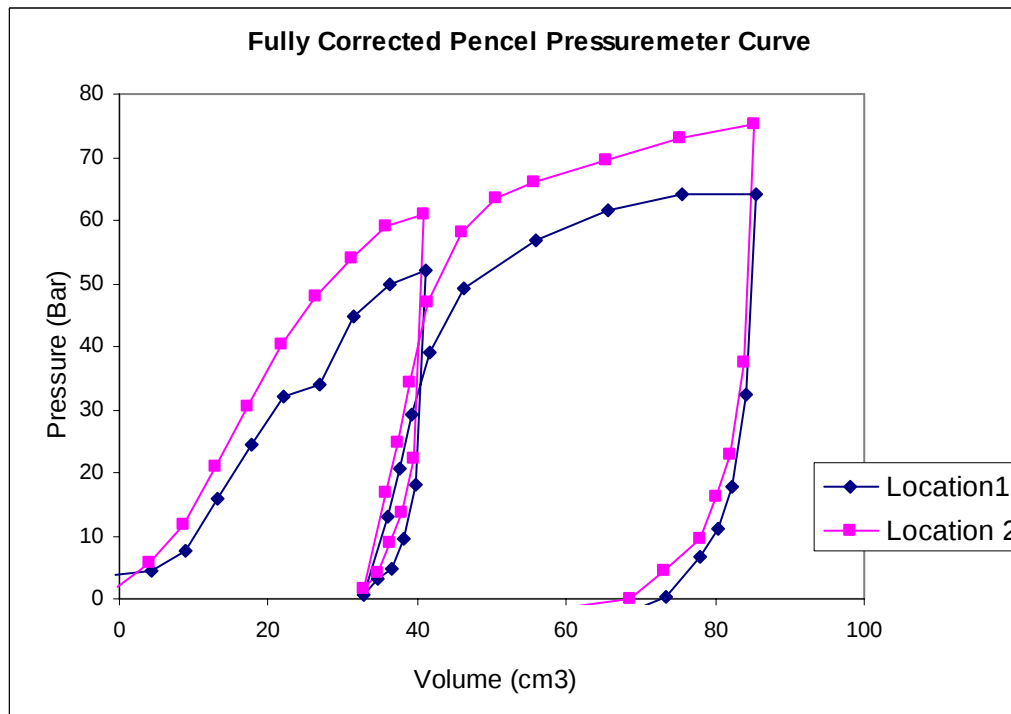
Figure 3-7 PMT results at 6-ft. depth.
