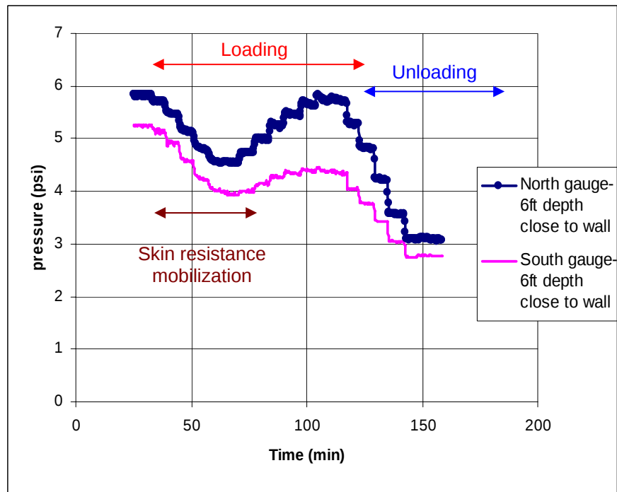
Figure 4-50 Variation of lateral stress during load test at 6-ft. depth, 6 inches off from the boundary.
