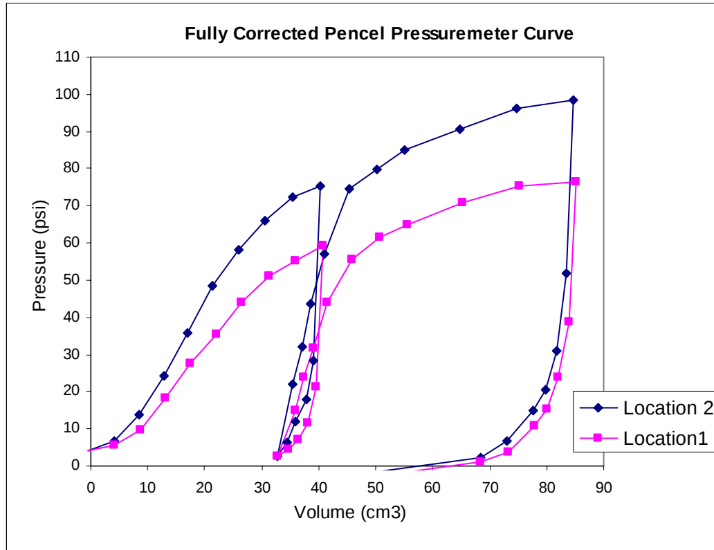
Figure 3-8 PMT results at 11-ft. depth.
