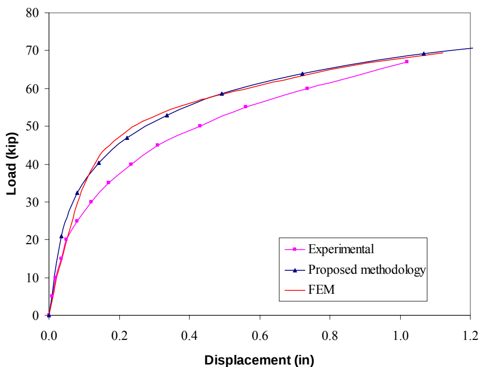
Figure 6-7 Comparison of load-displacement curves for 6-inch square \times 8-ft. long (15-inch diameter bulb) jet-grouted pile.
