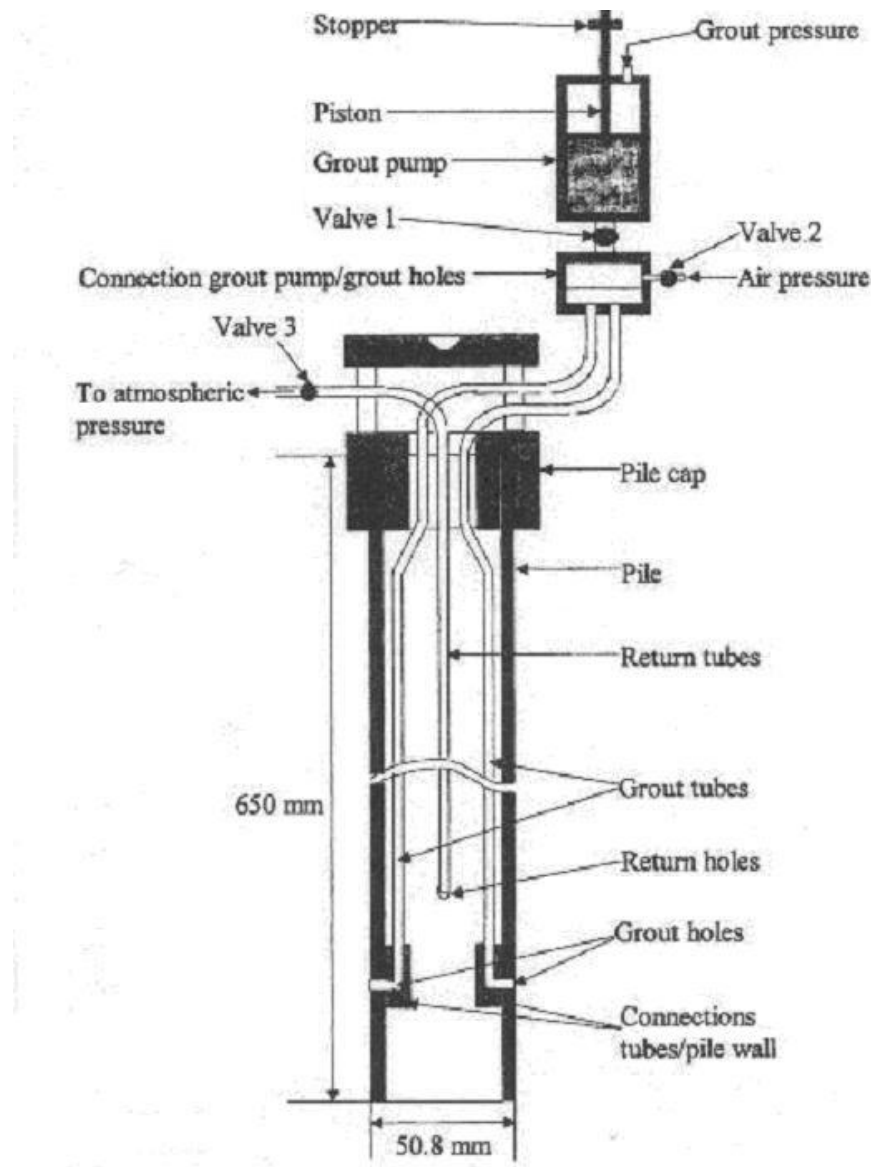
Figure 2-7 Side grouting system for precast pile (Joer et al. 1998).
