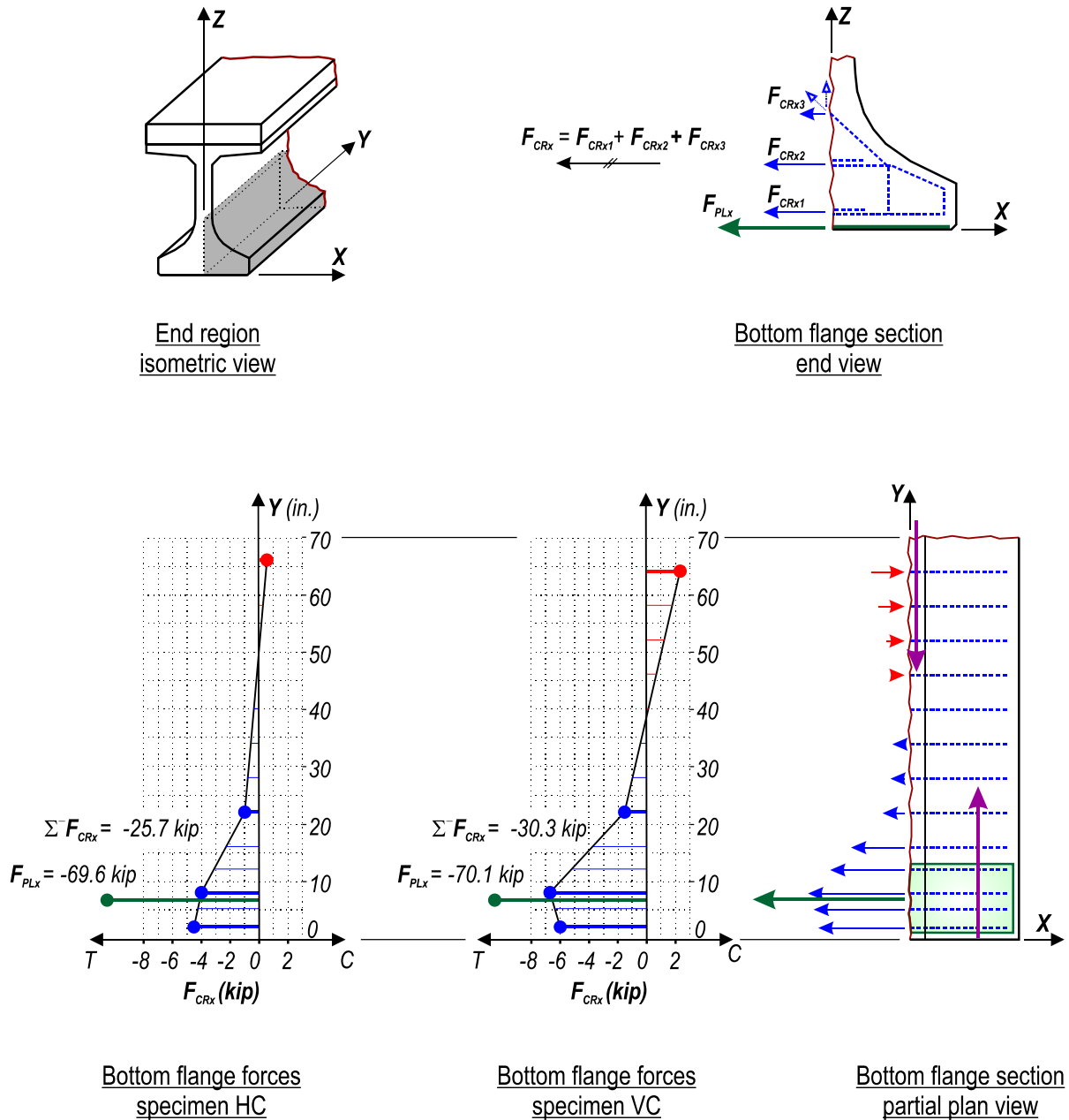
Figure 31–Transverse forces in confinement reinforcement and bearing plates
