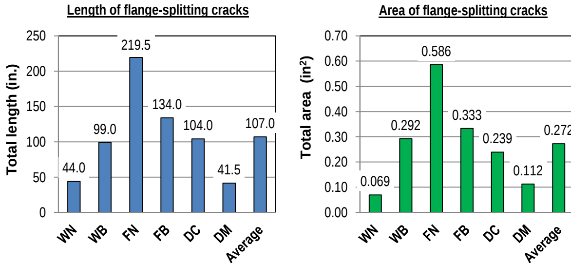
Figure 25—Flange splitting cracks girders W, F, and D
