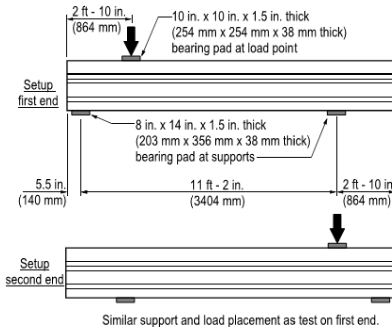
Figure 7–Test setup
