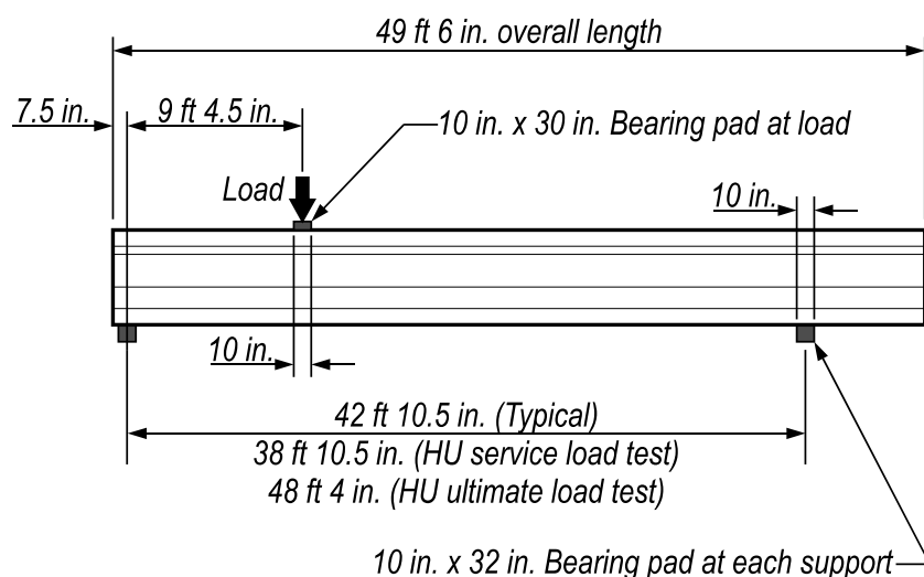
Figure 20–FIB-54 test setup
