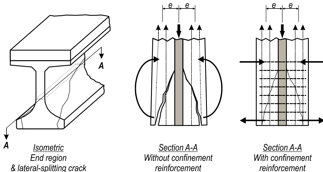
Figure 28–Lateral-splitting failure mechanics
