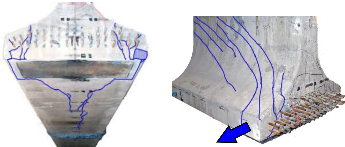
Figure 3–Lateral-splitting failure
