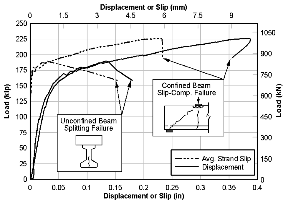
Figure 8—Load vs. displacement and strand slip
