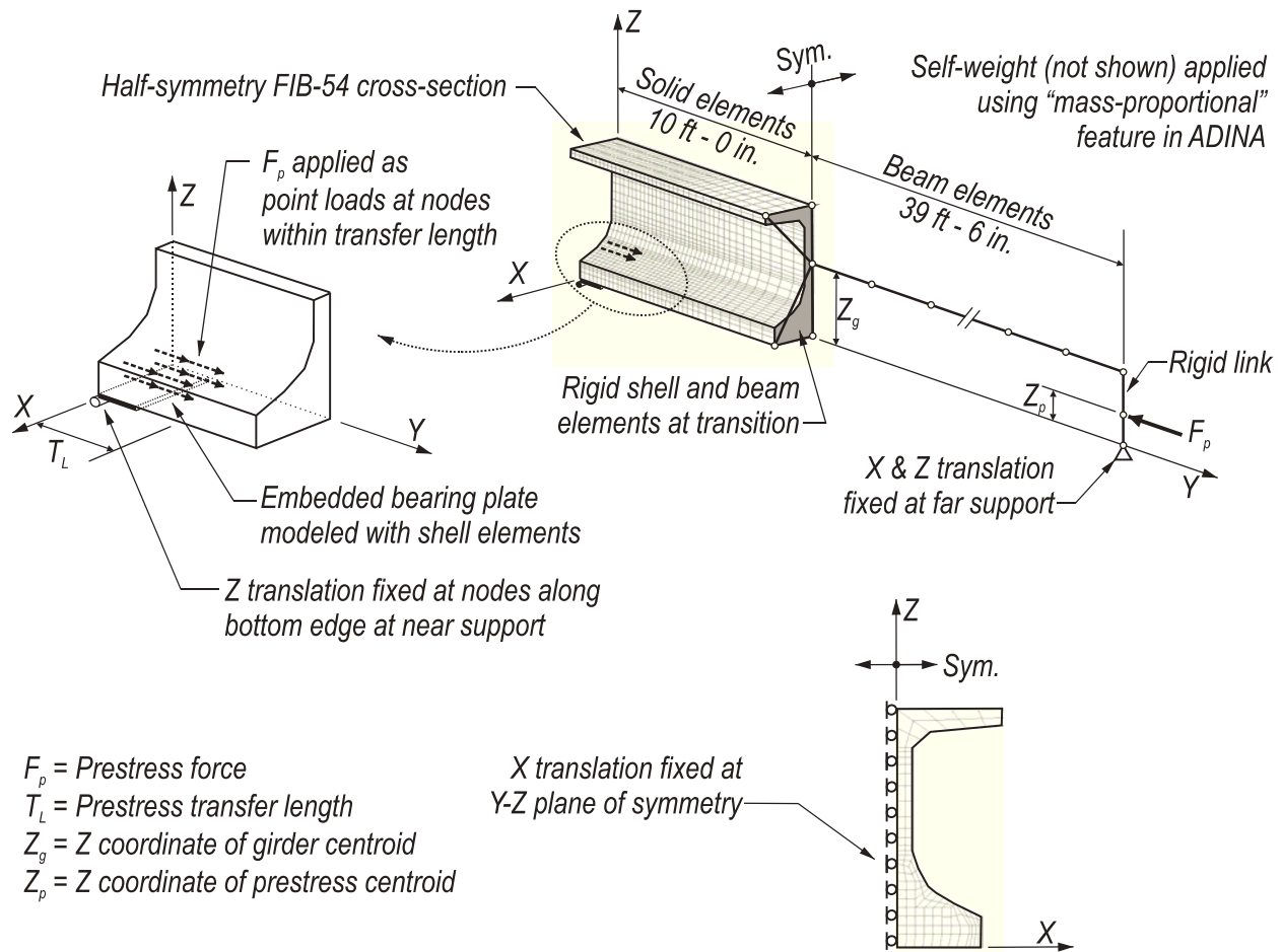
Figure 42—FE model details
