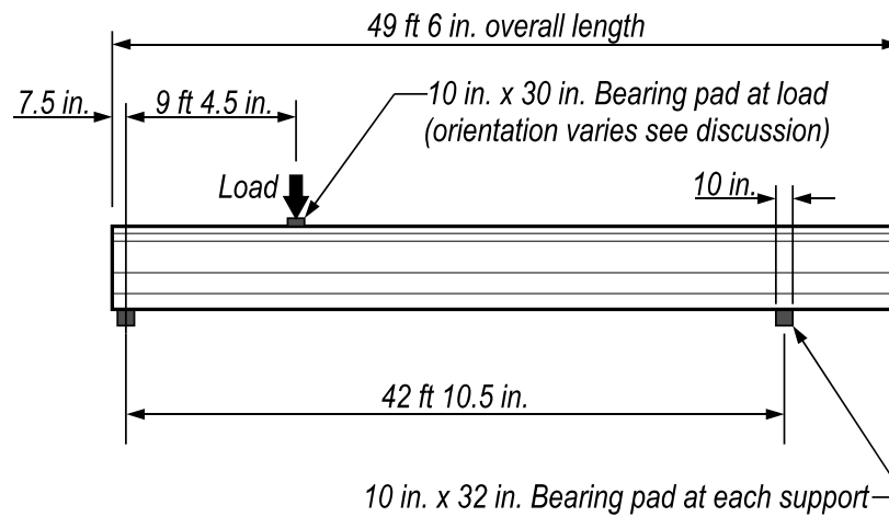
Figure 34—FIB-63 test setup
