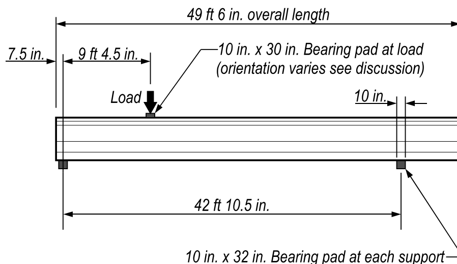
Figure 28–Test setup
