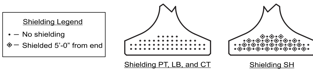
Figure 7–Strand bond and shielding patterns
