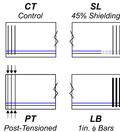
Figure 3–Test specimen labels
