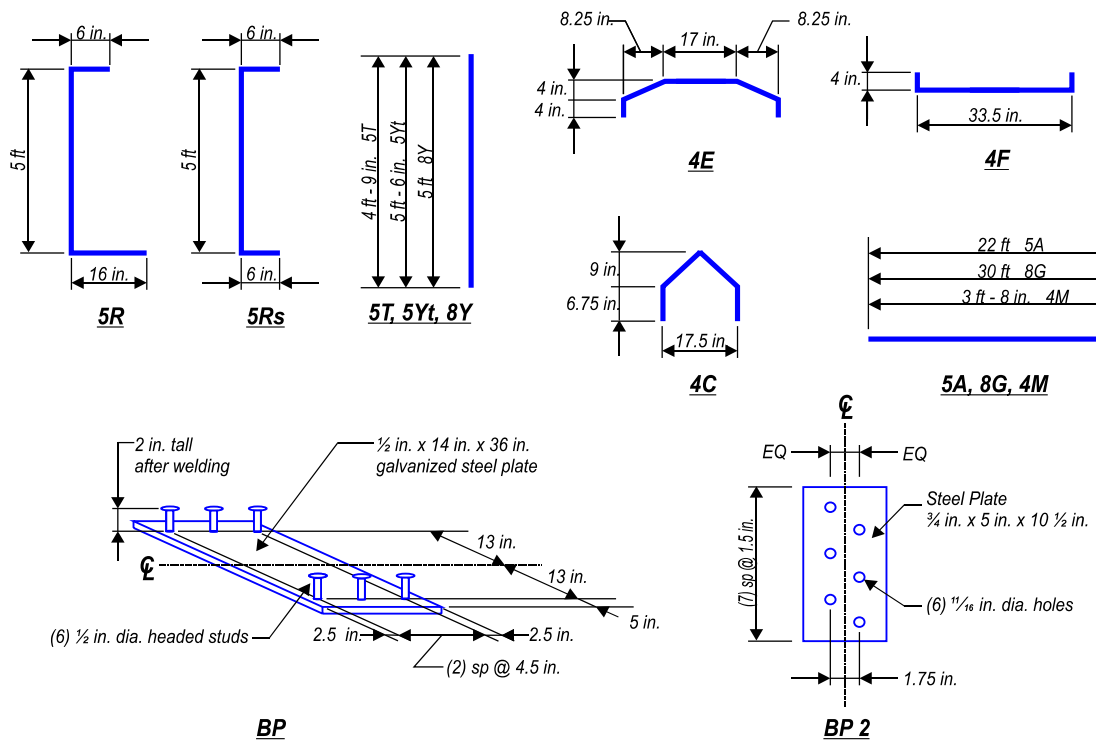
Figure 11–Reinforcement and bearing plate details
