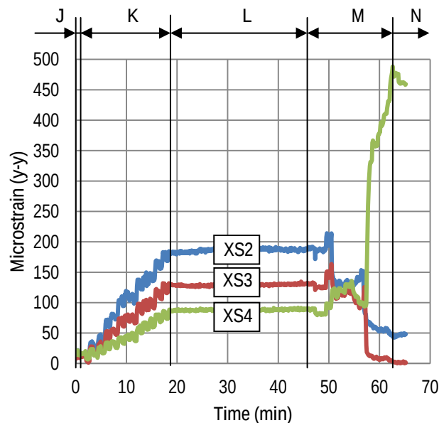
Figure 50—Concrete strain in specimen CT during prestress transfer
