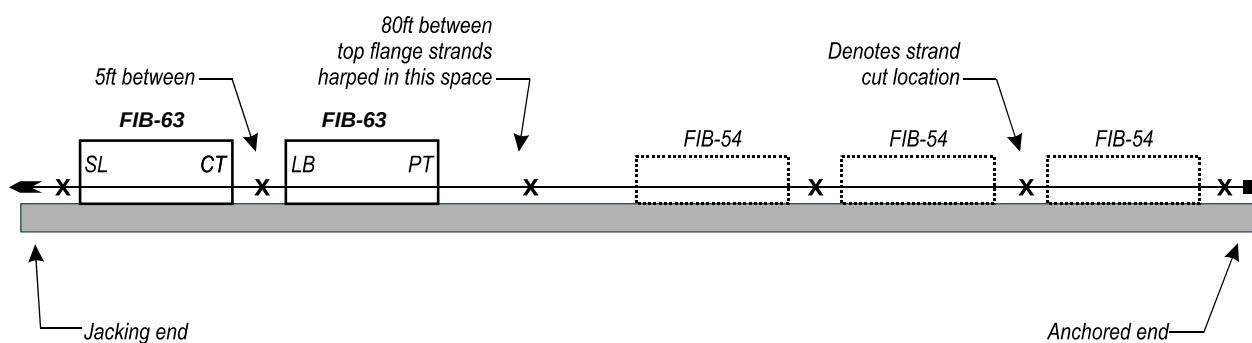
Figure 4–Specimen orientation in stressing bed
