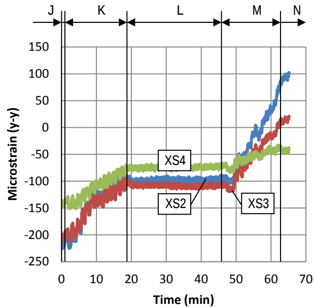
Figure 52—Concrete strain in specimen PT during prestress transfer
