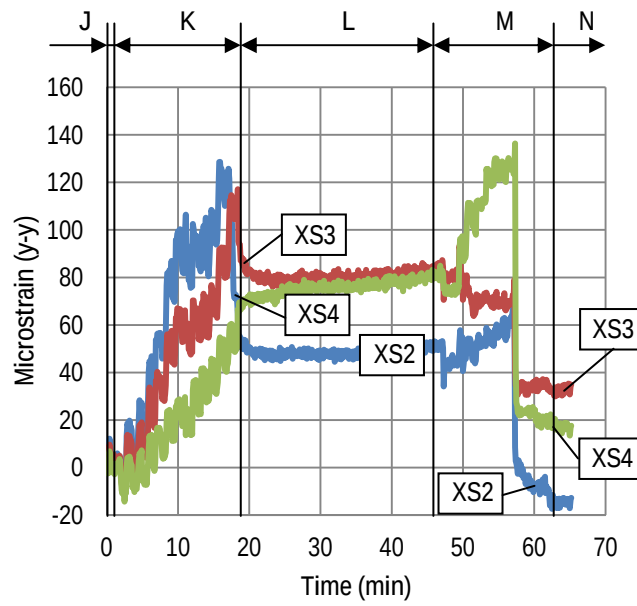
Figure 53—Concrete strain in specimen LB during prestress transfer
