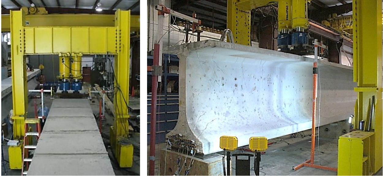
Figure 32—View of test specimen and load frame from above (left) and side view of specimen (right)
