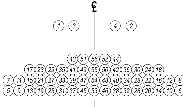
Figure 25–Strand cutting pattern
