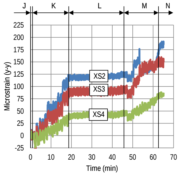
Figure 51—Concrete strain in specimen SL during prestress transfer
