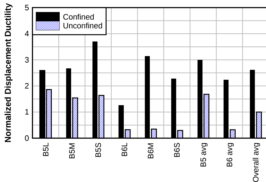
Figure 39–Normalized displacement ductility
