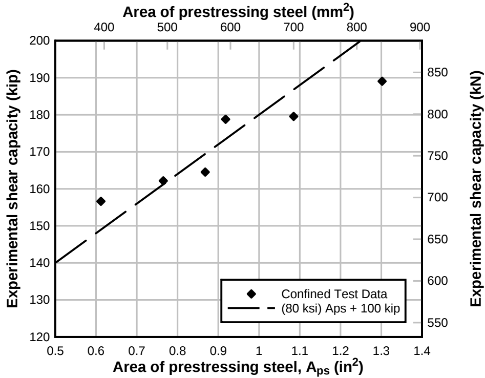
Figure 42–Experimental shear capacity vs. area of prestressing steel
