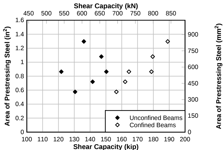
Figure 38—Effect of area of prestressing on shear capacity
