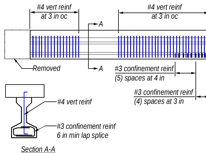
Figure 3—Vertical and confinement reinforcement
