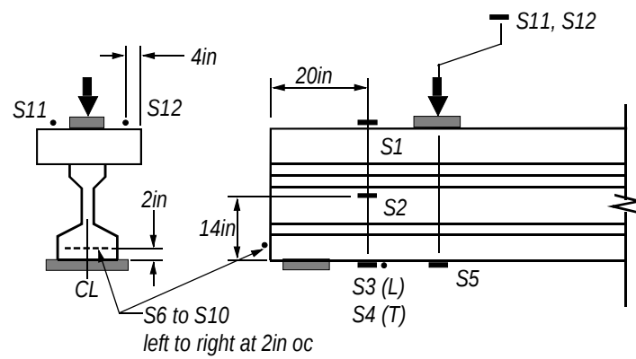
Figure 15–Strain gage placement
