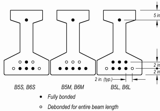
Figure 6—Strand layouts for beams containing 0.5-in. and 0.6-in. strand
