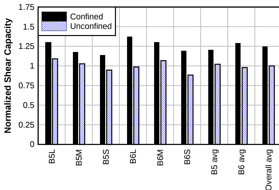
Figure 37–Normalized shear capacity
