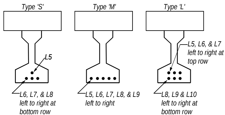
Figure 13–LVDTs at strands
