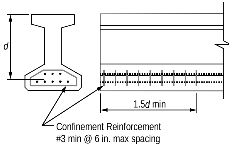
Figure 1—Confinement reinforcement
