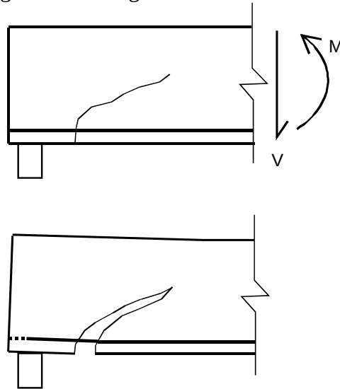
Figure 8—End region strut-and-tie behavior
