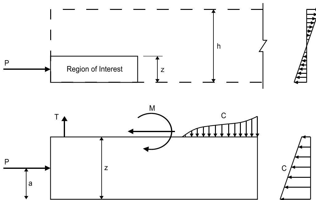
Figure 19–Free-body diagram based on Gergely-Sozen model (after Gergely et al. 1963)
