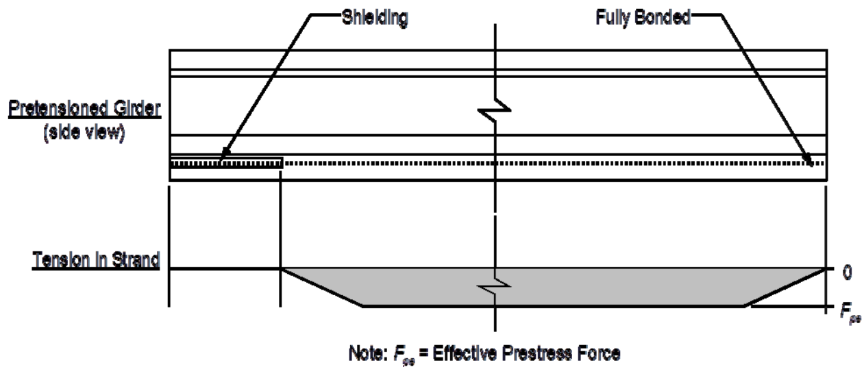
Figure 7—Strand debonding (shielding)
