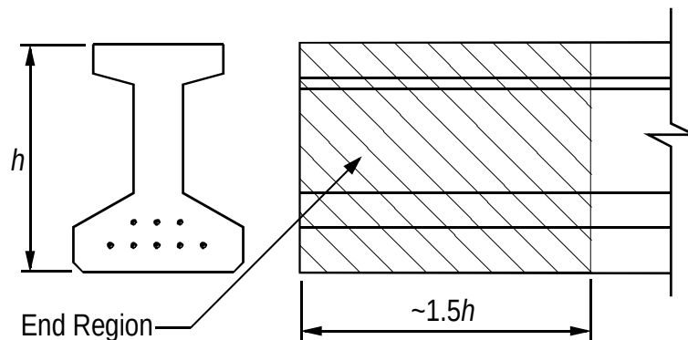
Figure 2—End region
