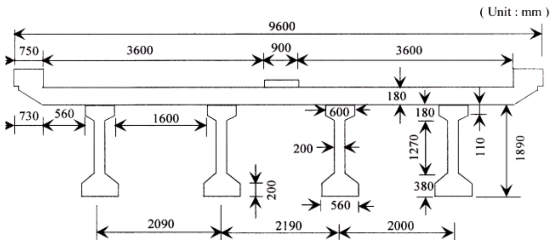
Figure 26—Cross section of test bridge (Oh et al. 2002)
