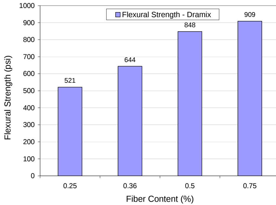
Figure 3-14: Flexural Strength of Dramix SFRC.
