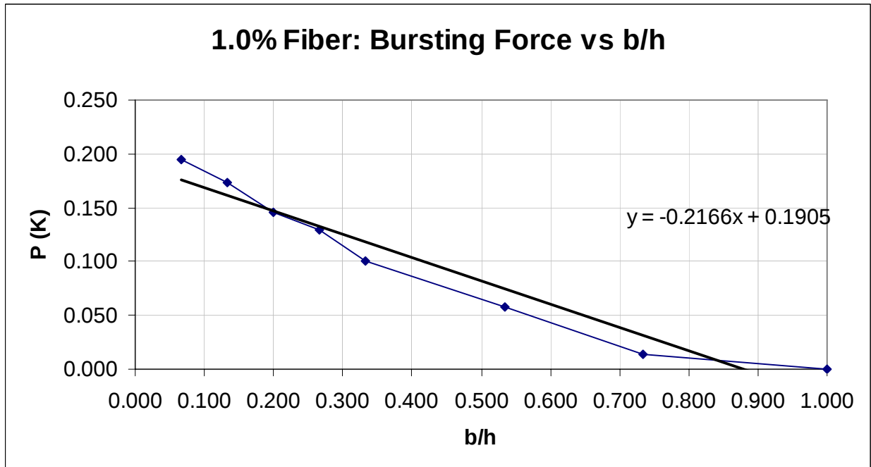
Figure 6-13: 1.0% Fiber Bursting Forces Versus b/h
