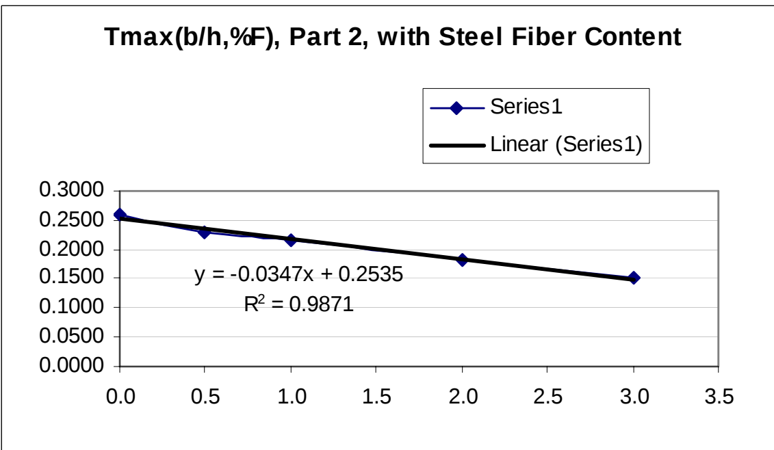
Figure 6-17: T_{\max} (P, b/h), Part 2, vs. % Fiber
