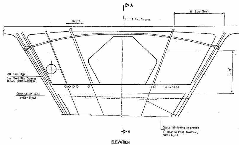
Figure 6-23: Cross-Section of Roosevelt Bridge Pier Segment
