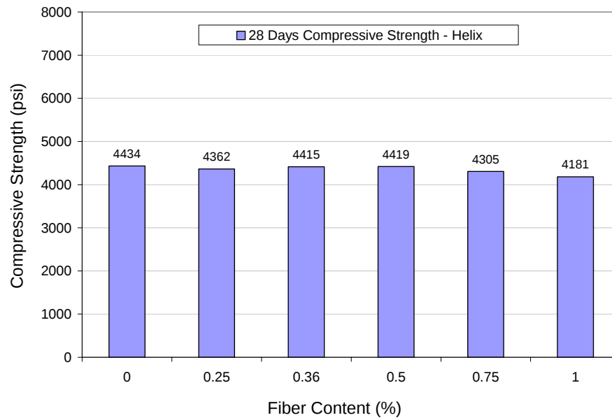
Figure 3-9: Compressive Strength of Helix SFRC.
