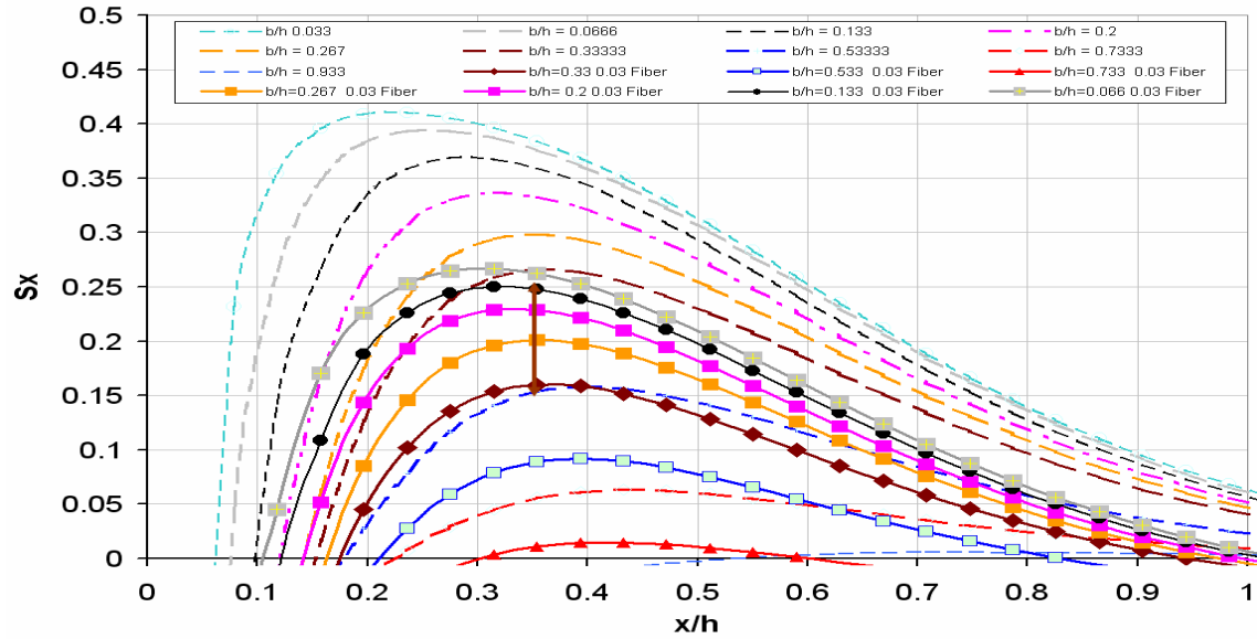
Figure 6-10: Maximum Tensile Stress, S_x , Versus x/h For 3.0% Fiber
