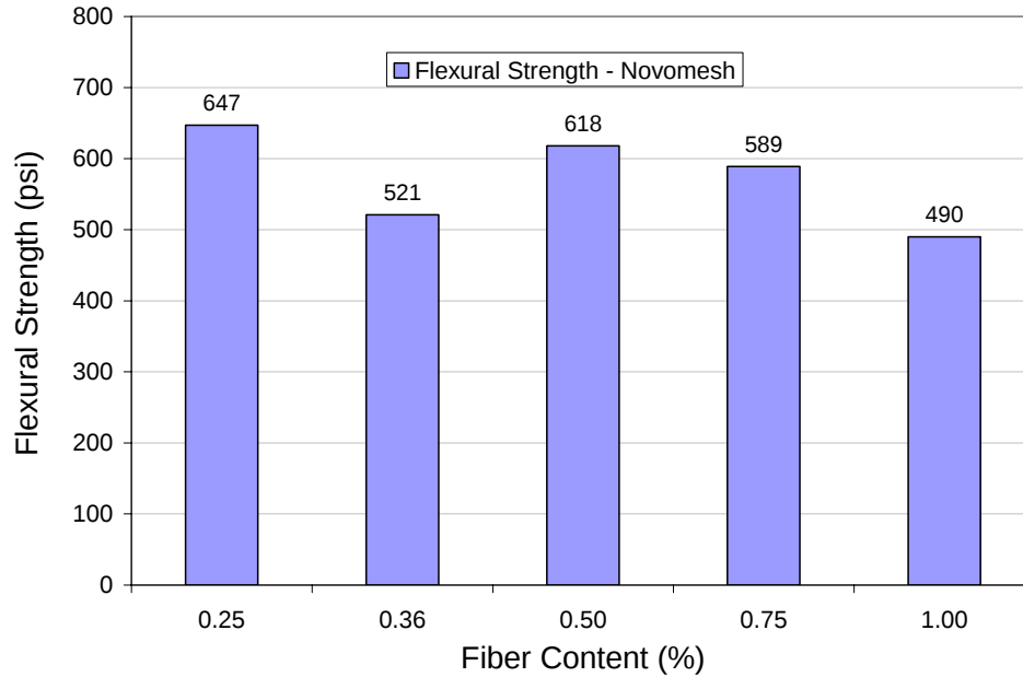
Figure 3-16: Flexural Strength of Novomesh SFRC.
