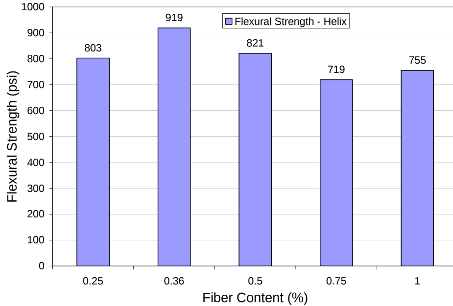
Figure 3-15: Flexural Strength of Helix SFRC.
