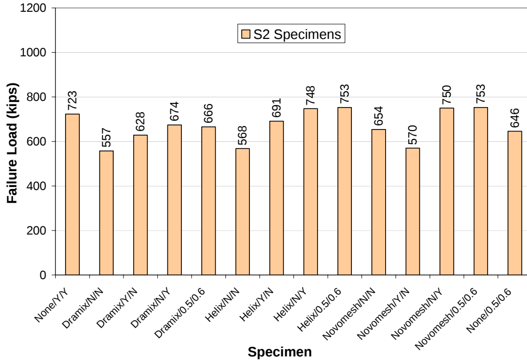
Figure 5-72: Load Capacity for S2 Specimens
