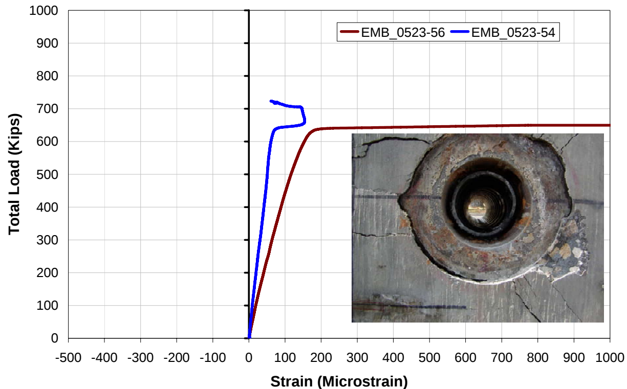
Figure 5-44: Load vs. Strain Relationship for Embedded Gauges of S2-1
