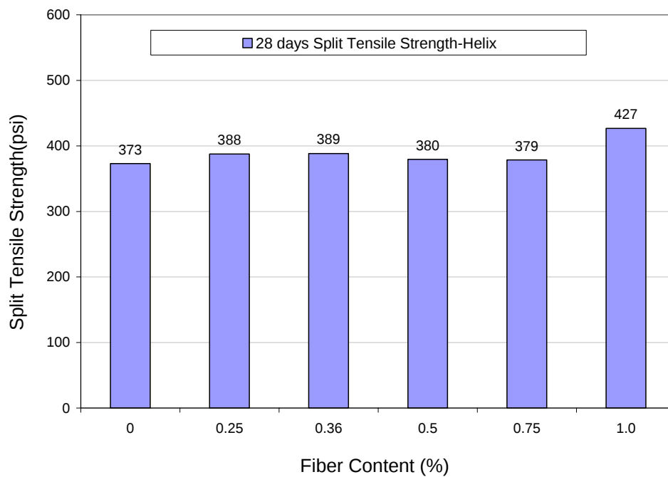
Figure 3-12: Split Tensile Strength of Helix SFRC.
