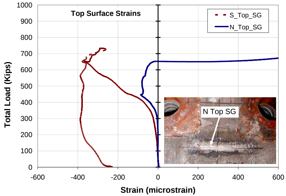
Figure 5-13: Load vs. Strain Relationship for Embedded Gauges in S1-13.
