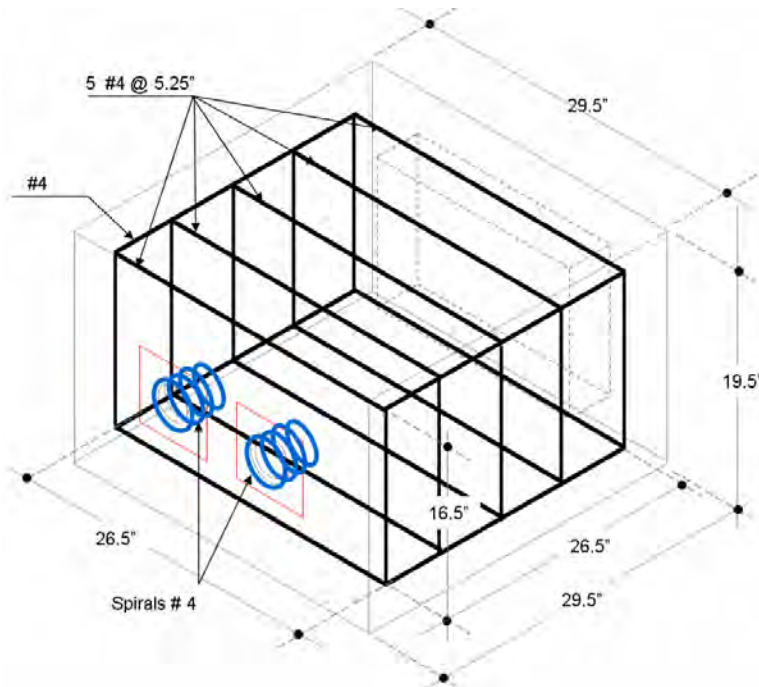
Figure 5-4: Anchorage Test Specimen Steel Tie Reinforcement.
