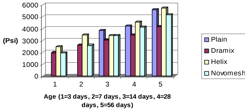
Figure 3-4: S2 Specimens Compressive Strength Results
