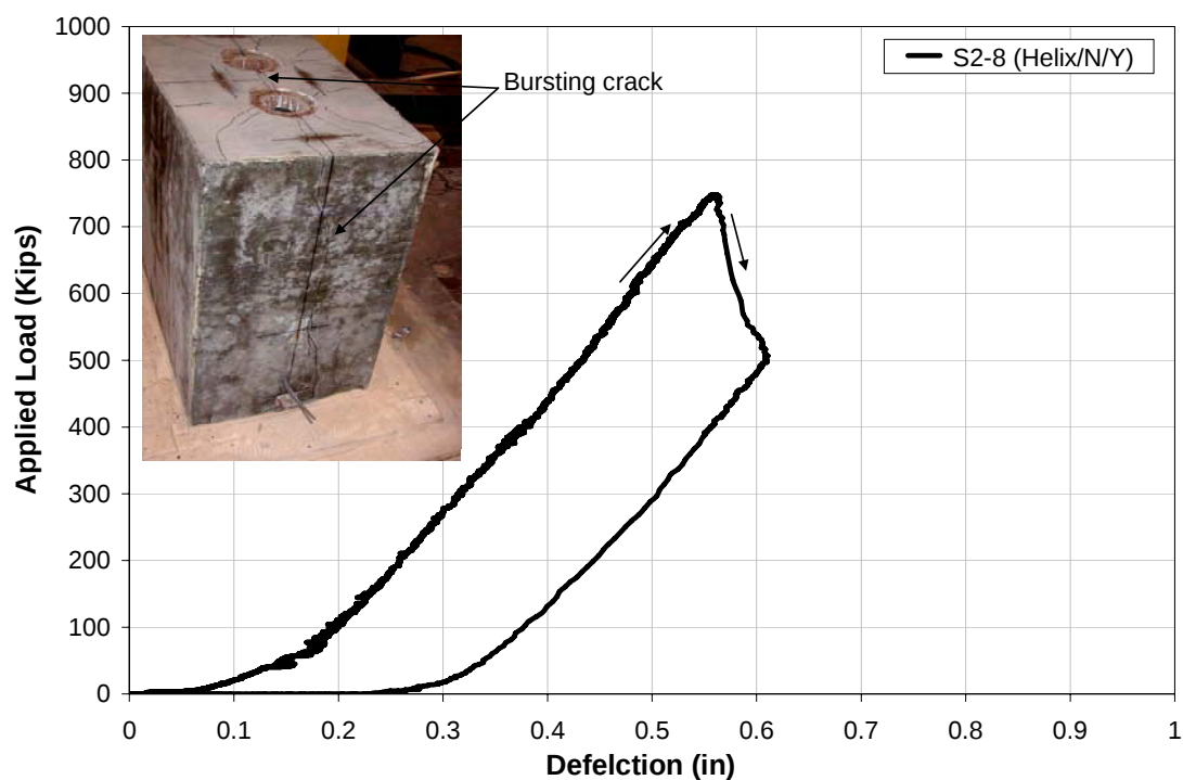
Figure 5-59: Load vs. Deflection of S2-8
