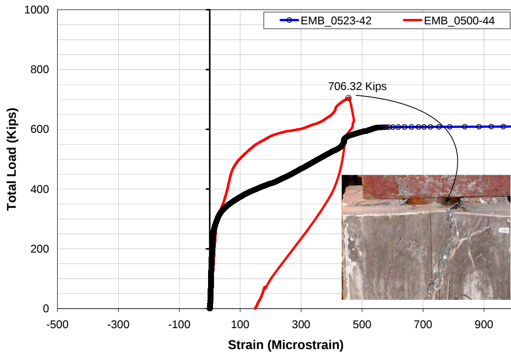
Figure 5-40: Load vs. Strain Relationship for Embedded Gauges of S1-11
