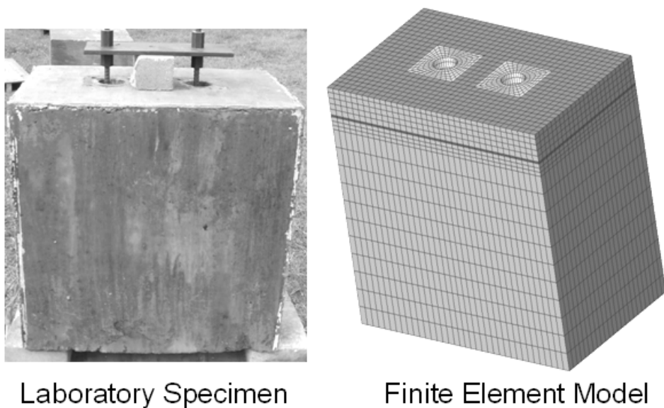
Figure 6-1: Anchor Specimen and Finite Element Model
