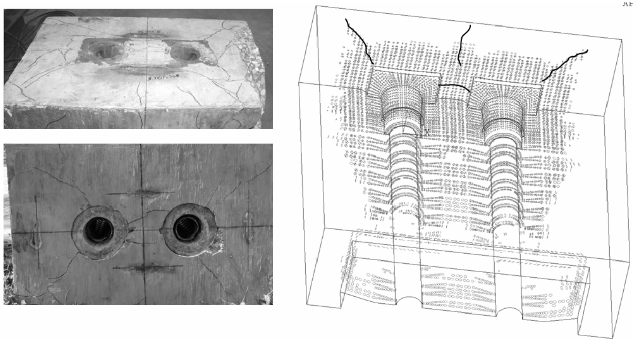
Figure 6-2: Cracking From Lab Testing and Finite Element Analysis
