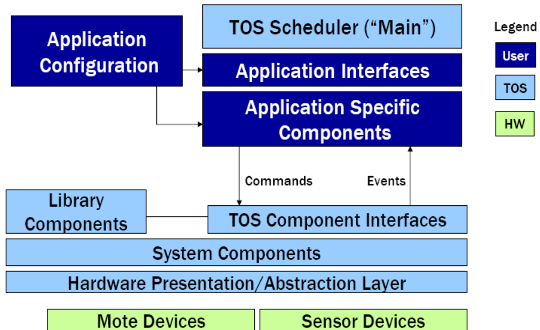
Figure 10 – TinyOS Architecture
