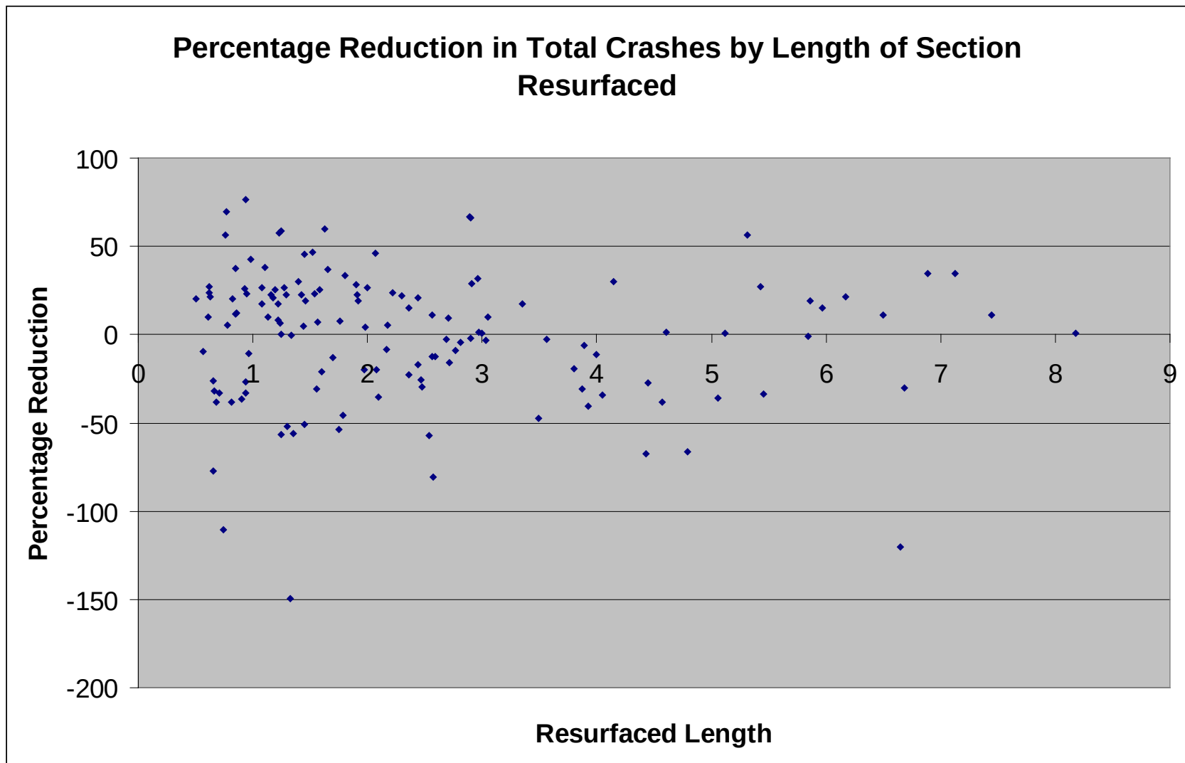
Figure 6-1: Percentage Reduction in Total Crashes by Length of the Section Resurfaced
