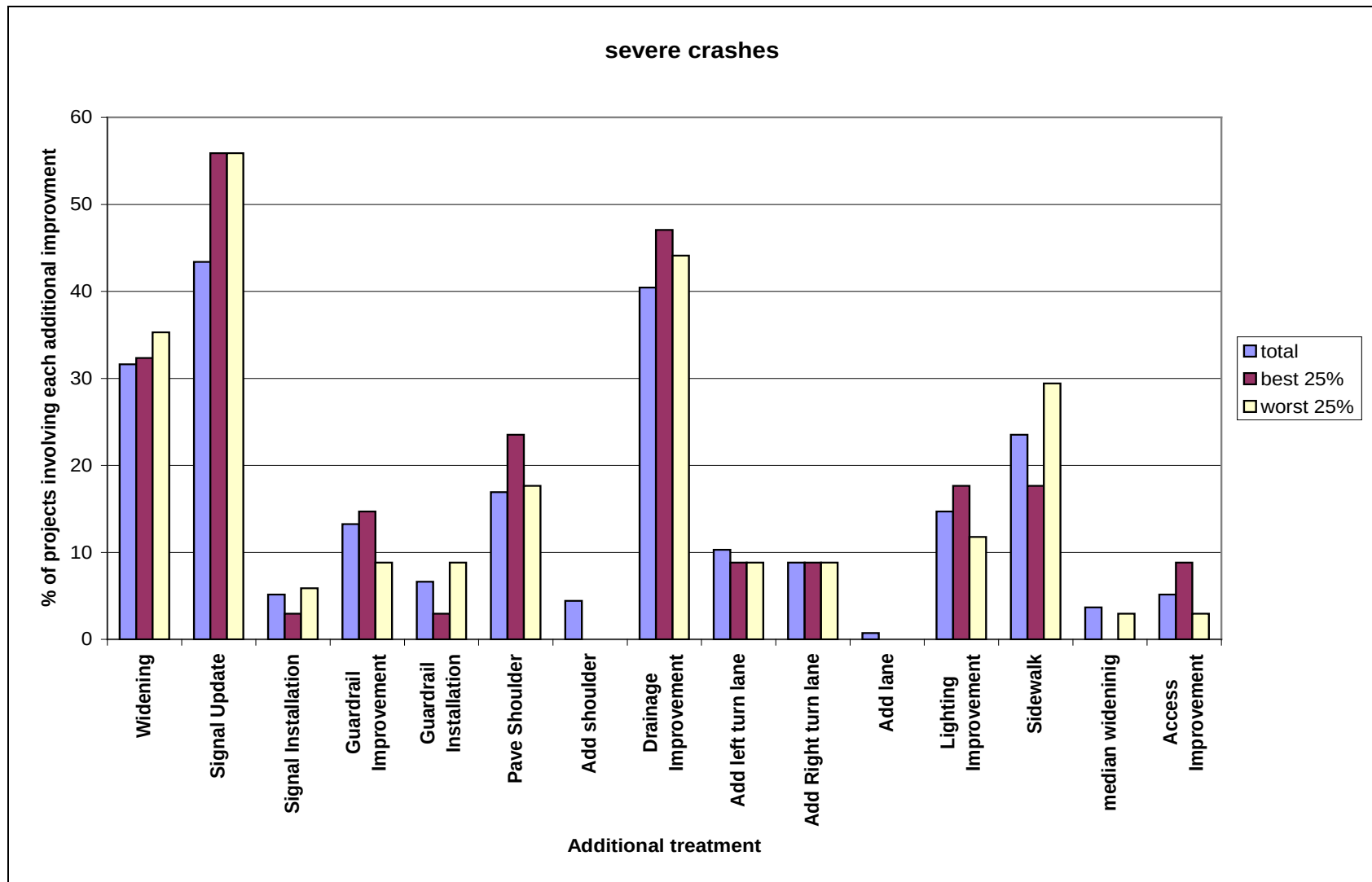
Figure 6-3: Comparison of Proportions (of project with each additional improvement) in Best 25%, Worst 25%, and Overall (100%; 136) Projects in Terms of Changes in Severe Crashes
