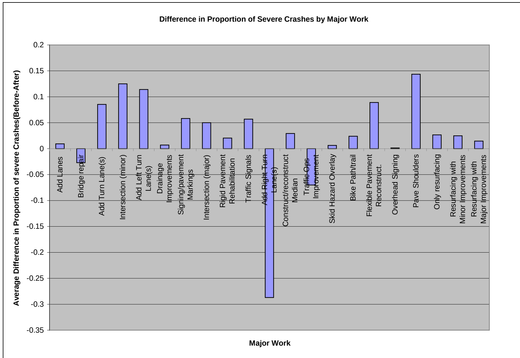
Figure 3-12: Bar Chart Showing Average Difference in the Proportion of Severe Crashes for Each Project Type (positive value indicates that the proportion of severe crashes in the before period is more than the after period's)
