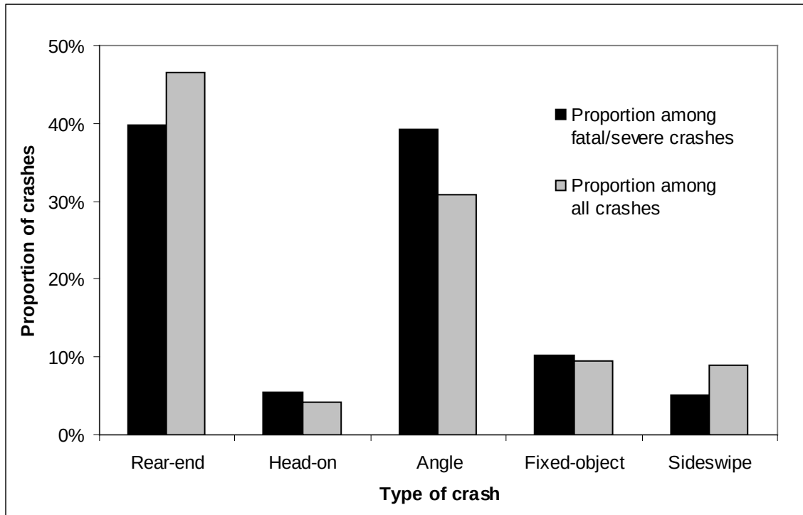
Figure 5-2: Distribution of Crashes on Multi-lane Arterials by Severity and Type Characterized by First Harmful Event
