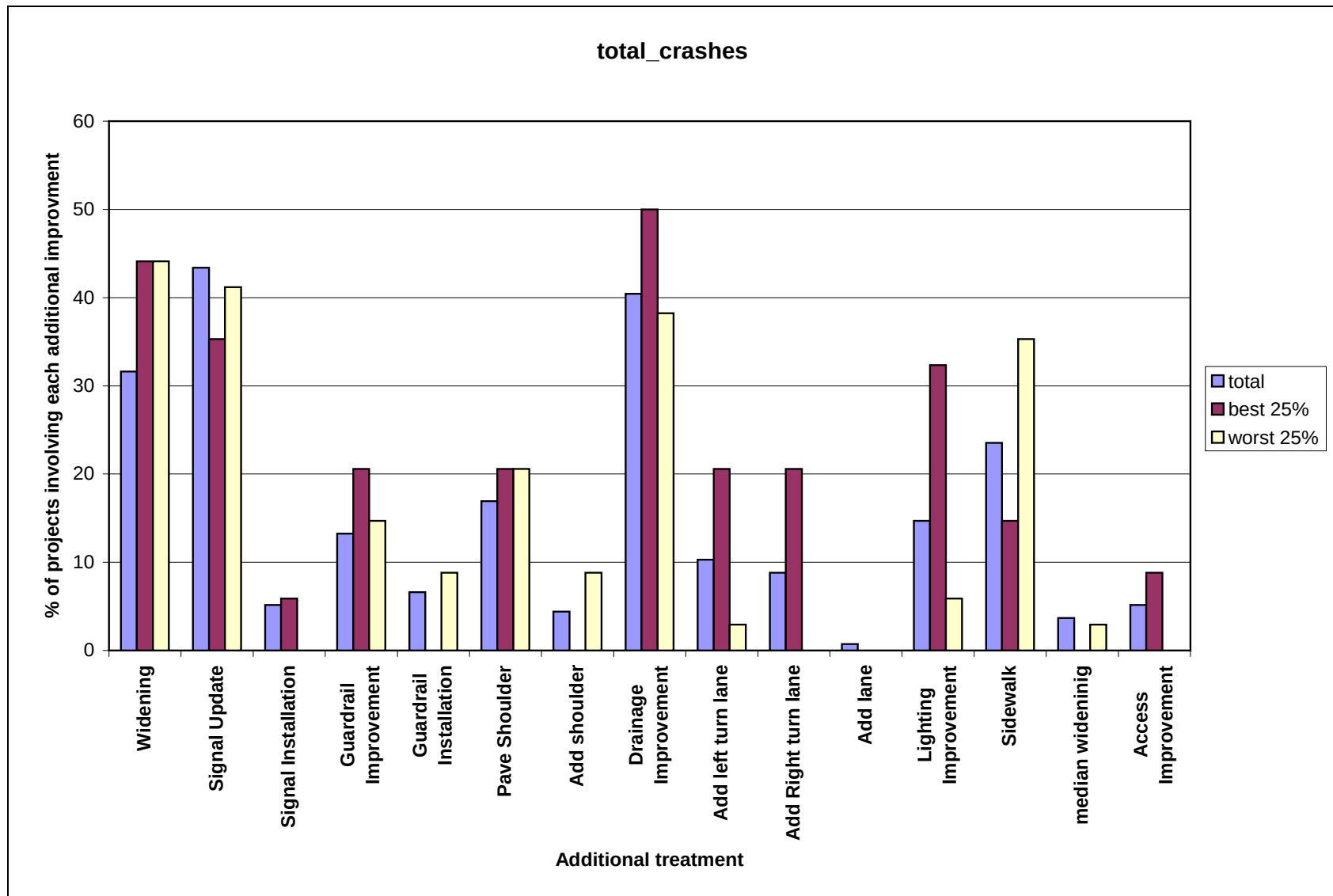
Figure 6-2: Comparison of Proportions (of project with each additional improvement) in Best 25%, Worst 25%, and All (100%; 136) Projects in Terms of Changes in Total Crashes
