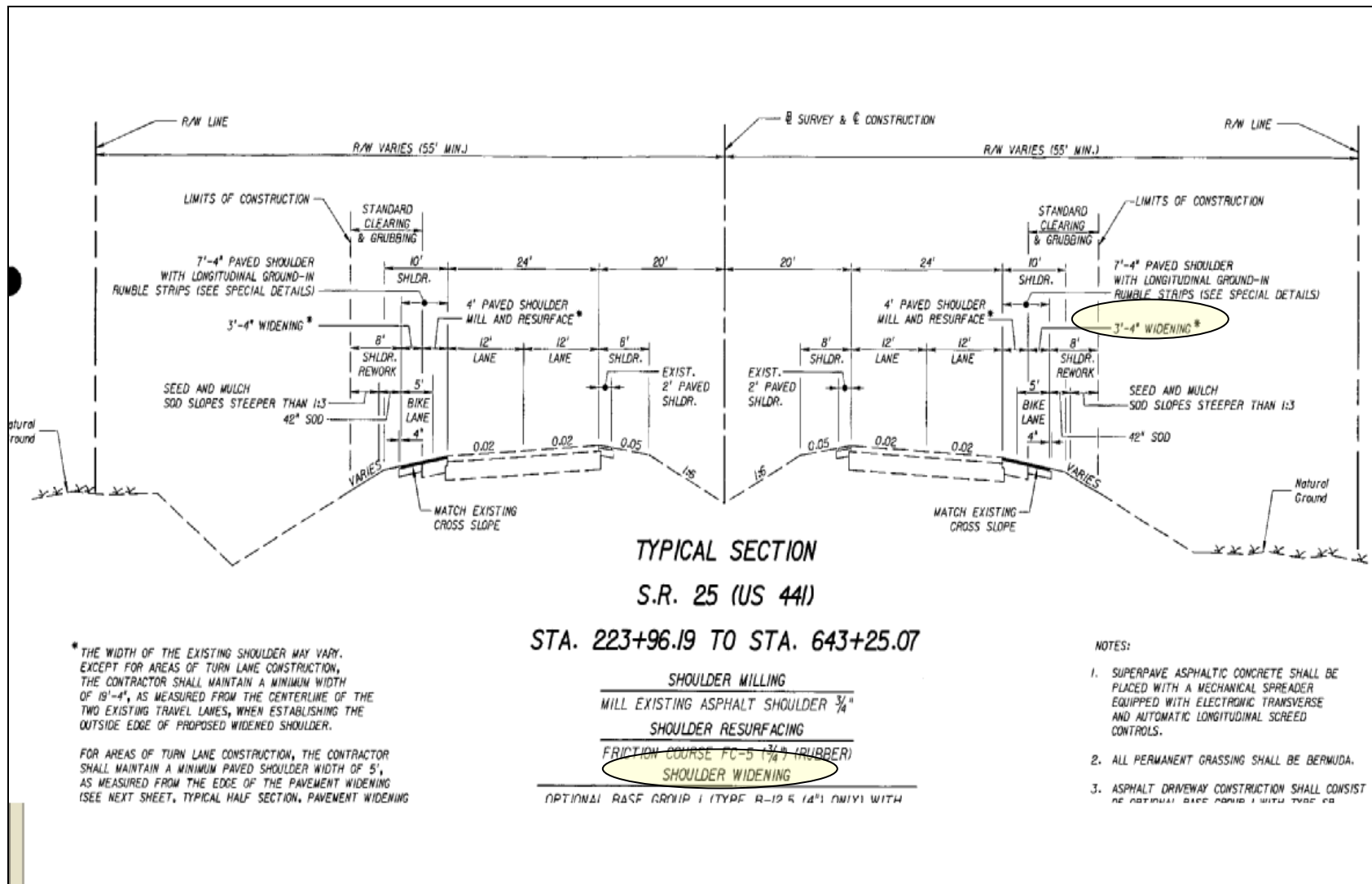
Figure 3-5: Project Plan Showing Shoulder Widening
