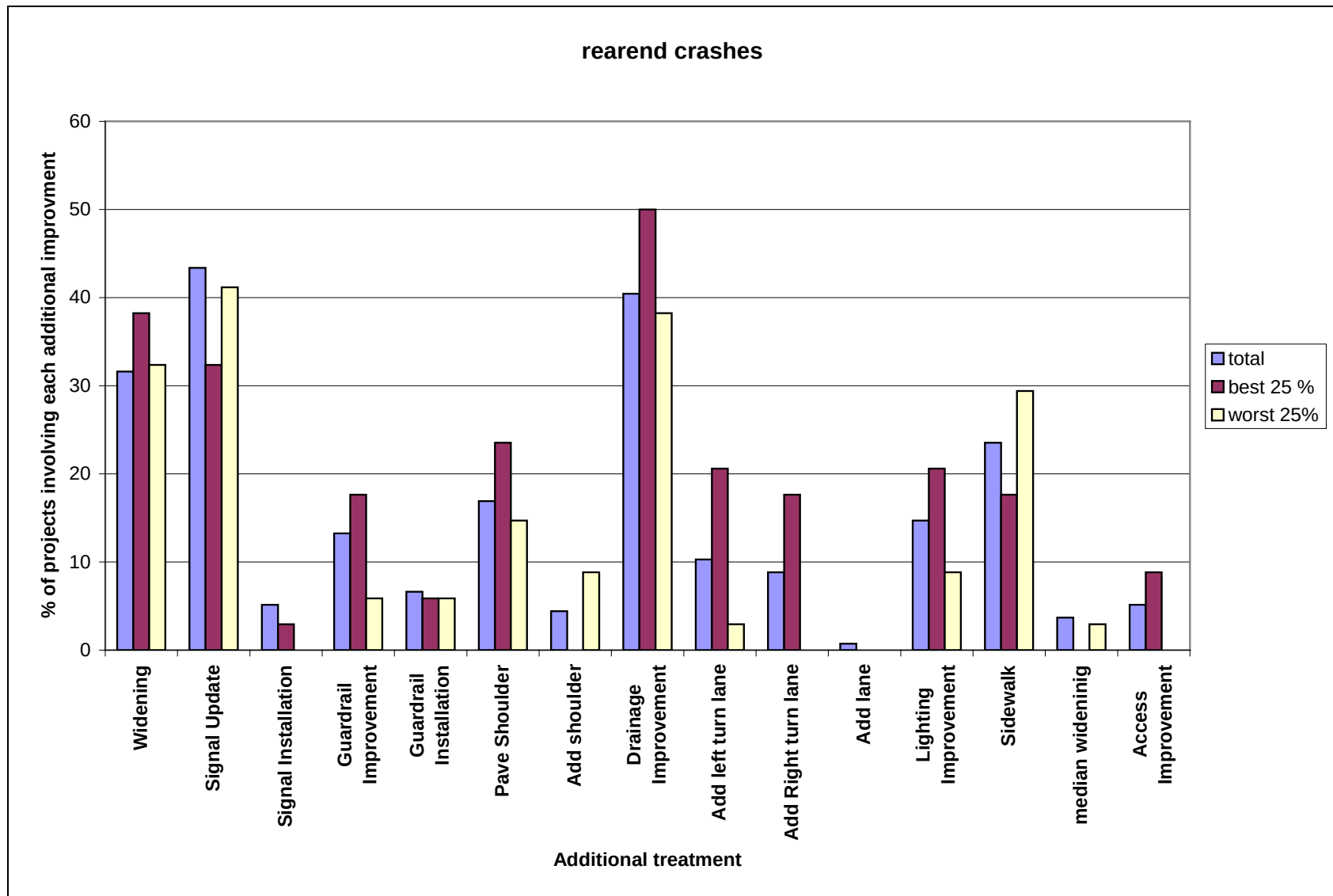
Figure 6-4: Comparison of Proportions (of project with each additional improvement) in Best 25%, Worst 25%, and Overall (100%; 136) Projects in Terms of Changes in Rear-end Crashes
