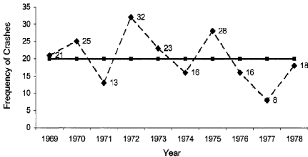
Figure 2-1: Example Demonstrating Regression-to-the-mean Phenomenon (Council et al. (1980)).
