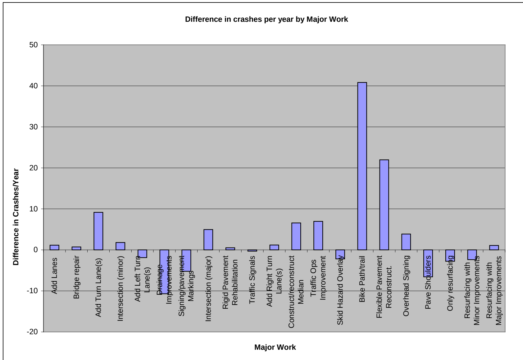
Figure 3-9: Histogram Showing Average Difference in Crash per Year (positive value indicates that crash per year in the before period is greater than that in the after period's.)
