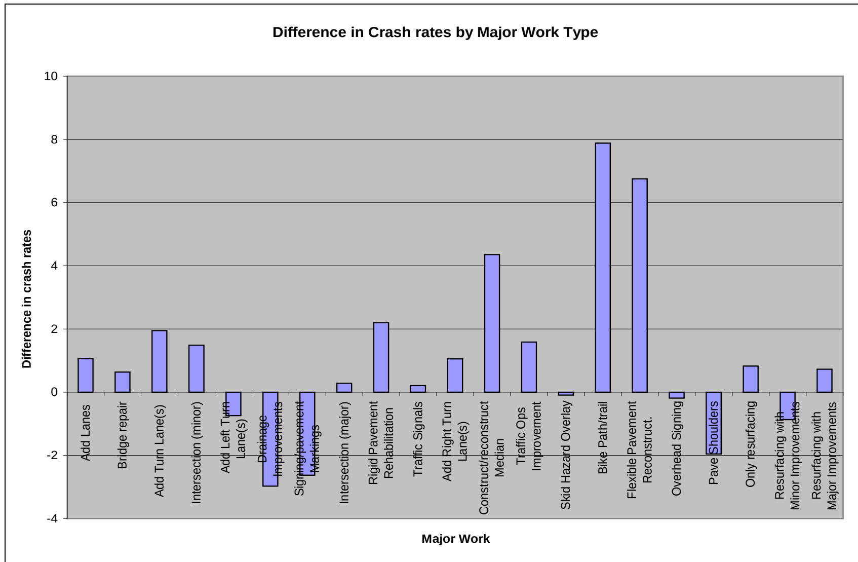
Figure 3-10: Histogram Showing Average Difference in Crash Rates (positive value indicates that crash rate in the before period is greater than the after period's.)
