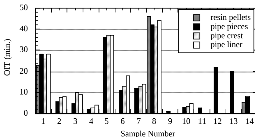
Fig. 2.18 - OIT data of fourteen commercially new pipe samples [B1]
