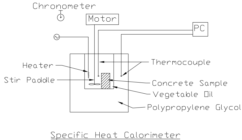
Figure 6-7. Schematic of the specific heat capacity calorimeter.
