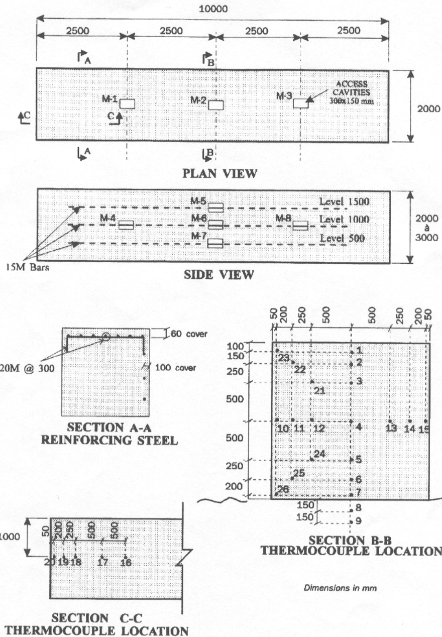
Figure 2-4. Thermocouple and strain gage locations in the James Bay concrete monolith (Ayotte et al. 1997).
