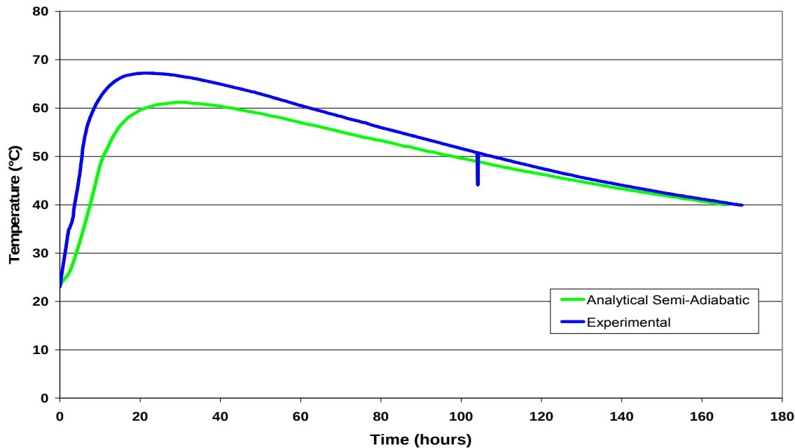
Figure 7-8. Semi-adiabatic and experimentally measured temperature-time histories at the center of the block, 21 in. below the exposed top surface of Mixture 1.
