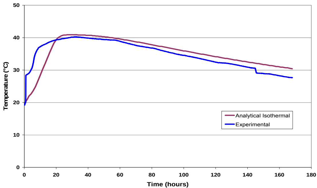
Figure 7-28. Isothermal and experimentally measured temperature-time histories at the center of the block, 4 in. below the exposed top surface of Mixture 4.
