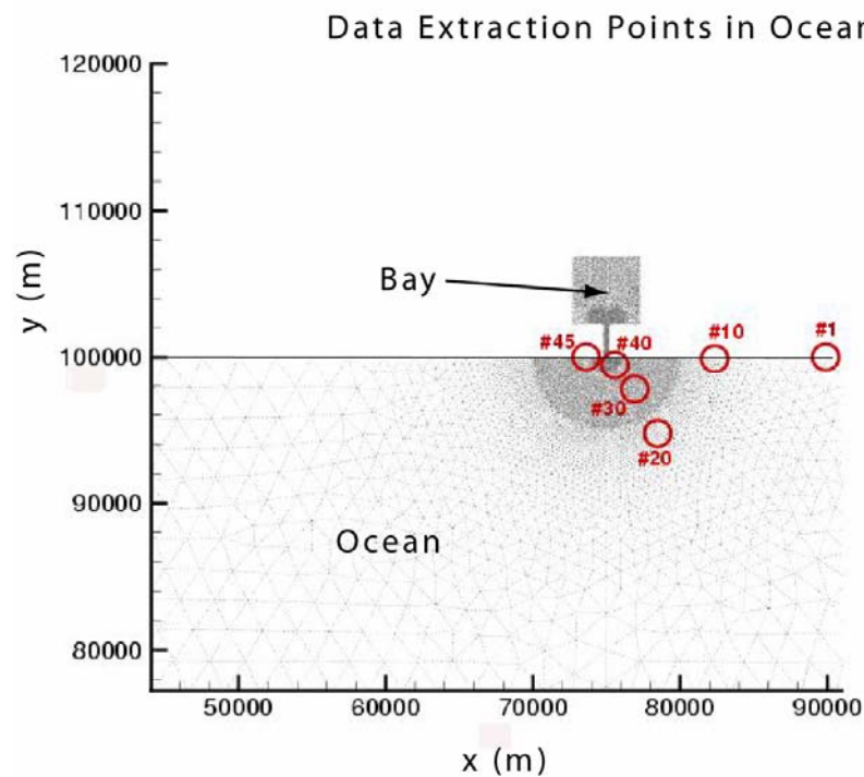
Figure 9 Definition drawing showing locations where data was extracted.
