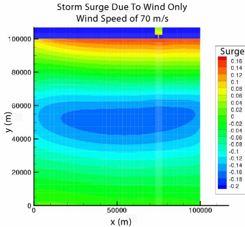
Figure 27 Storm Surge due to 70 m/s Wind Only (No Wave Input).
