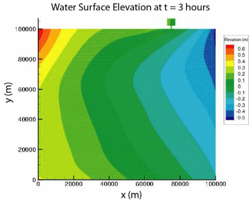
Figure 42 Water Surface Elevation at Time = 3 hours.
