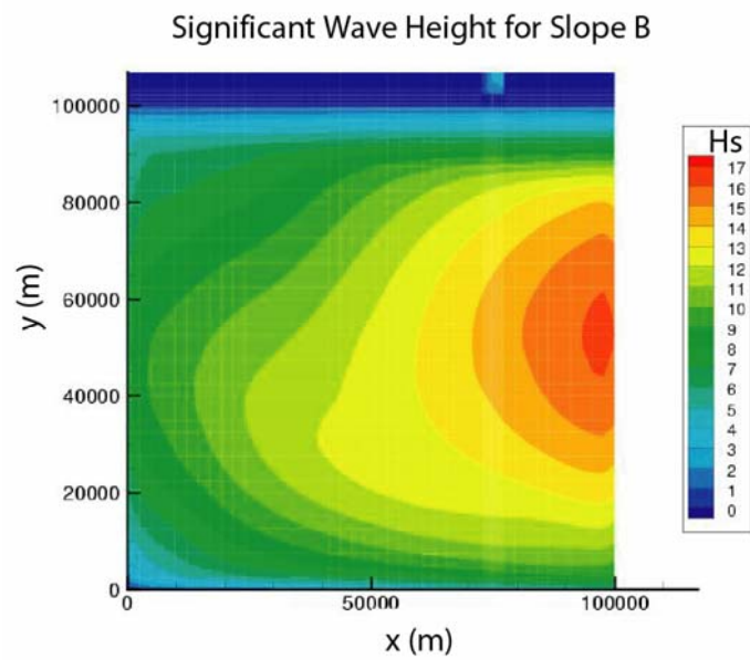
Figure 51 Significant Wave Height Contours for Slope B (same time as Figure 50).
