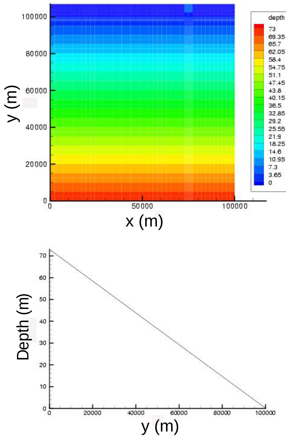
Figure 2 Elevation and plan views of the idealized model geometry for one of the bed slopes.
