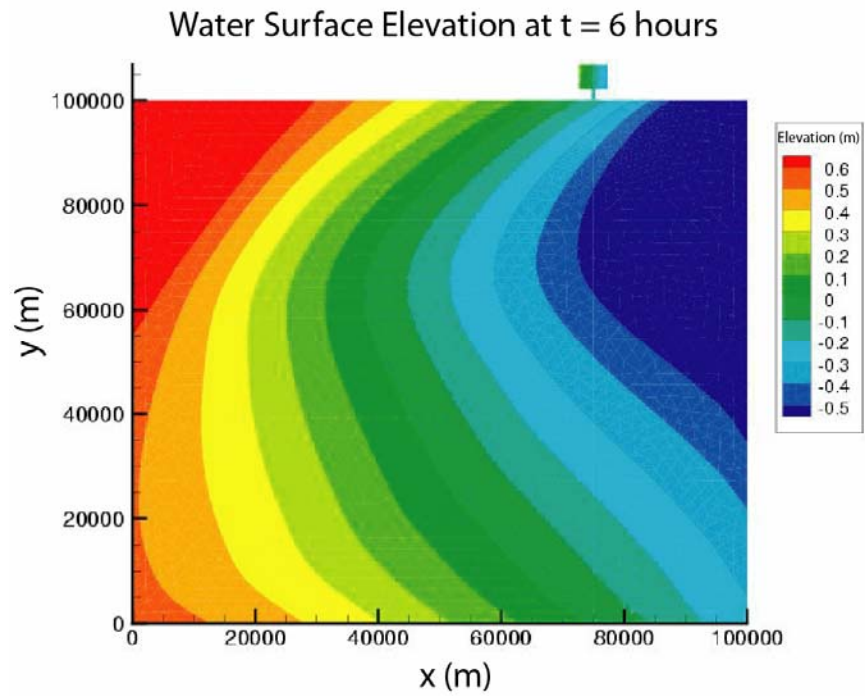
Figure 43 Water Surface Elevation at Time = 6 hours.
