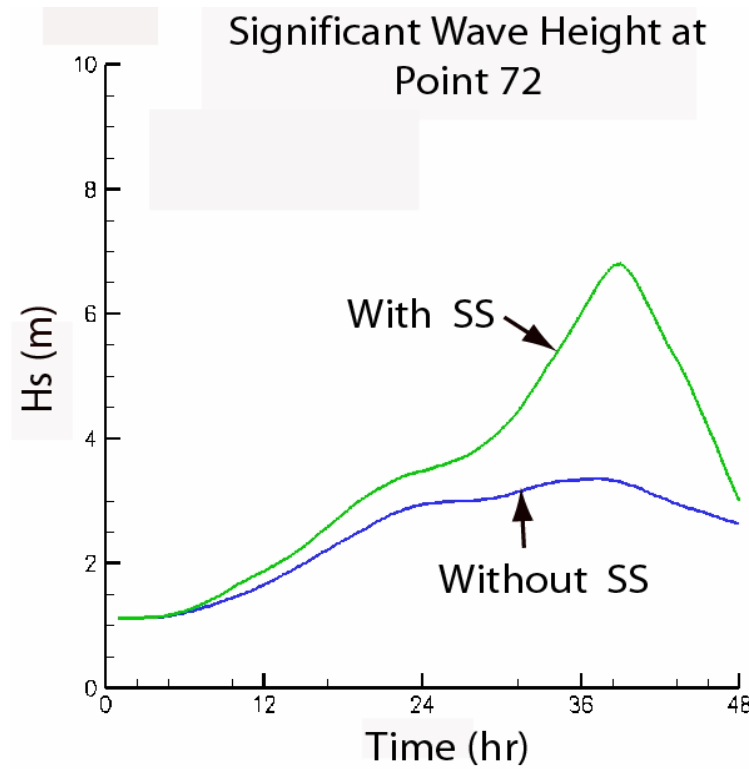
Figure 63 Significant Wave Height at Point 72 (see Figure 60) Without and With Storm Surge (SS) Input.
