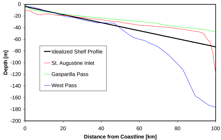
Figure P2- 10 Comparison of Idealized Shelf Profile with Actual Florida Shelf Profiles for the West/Northeast Florida a Domain.
