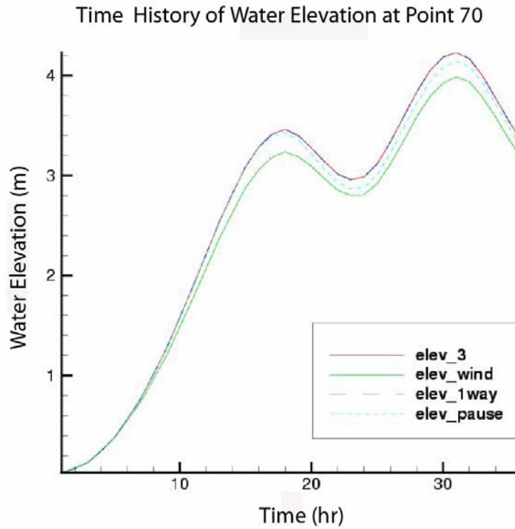
Figure 24 Time history of water elevation at Point 70 near the inlet (see Figure 10), Wind Speed = 50 m/s.
