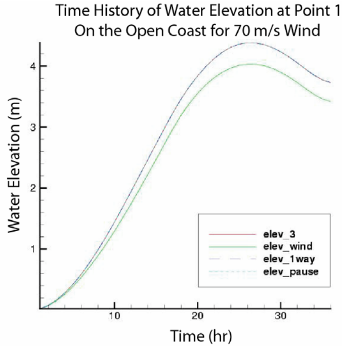
Figure 28 Time history of water elevation at Point 1 on the open coast (see Figure 9), Wind Speed = 70 m/s.
