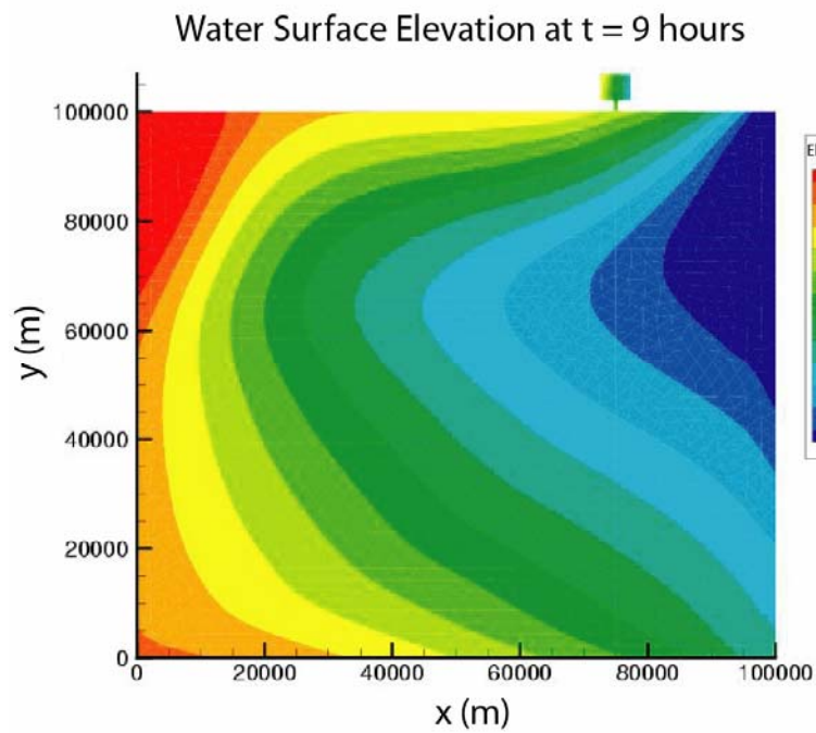
Figure 44 Water Surface Elevation at Time = 9 hours.
