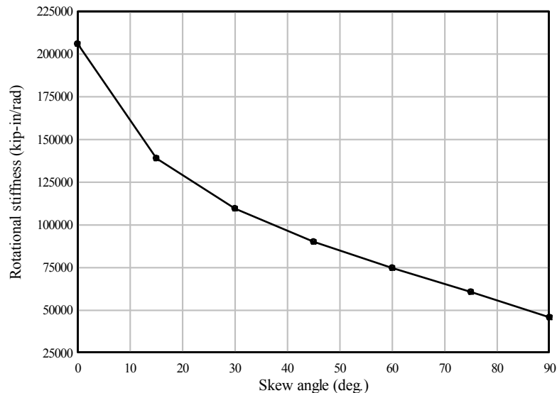
Figure 5.10 Rotational stiffness vs. skew angle
