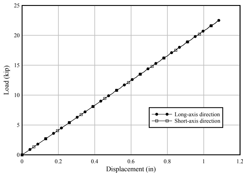
Figure 5.6 Shear stiffness results
