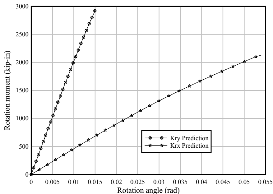
Figure 5.8 Rotational stiffness results
