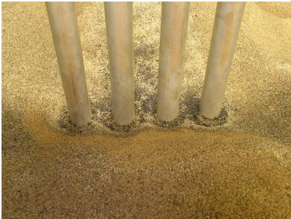
Figure 35 Post Scour Test 3 Photograph Taken From Upstream.
