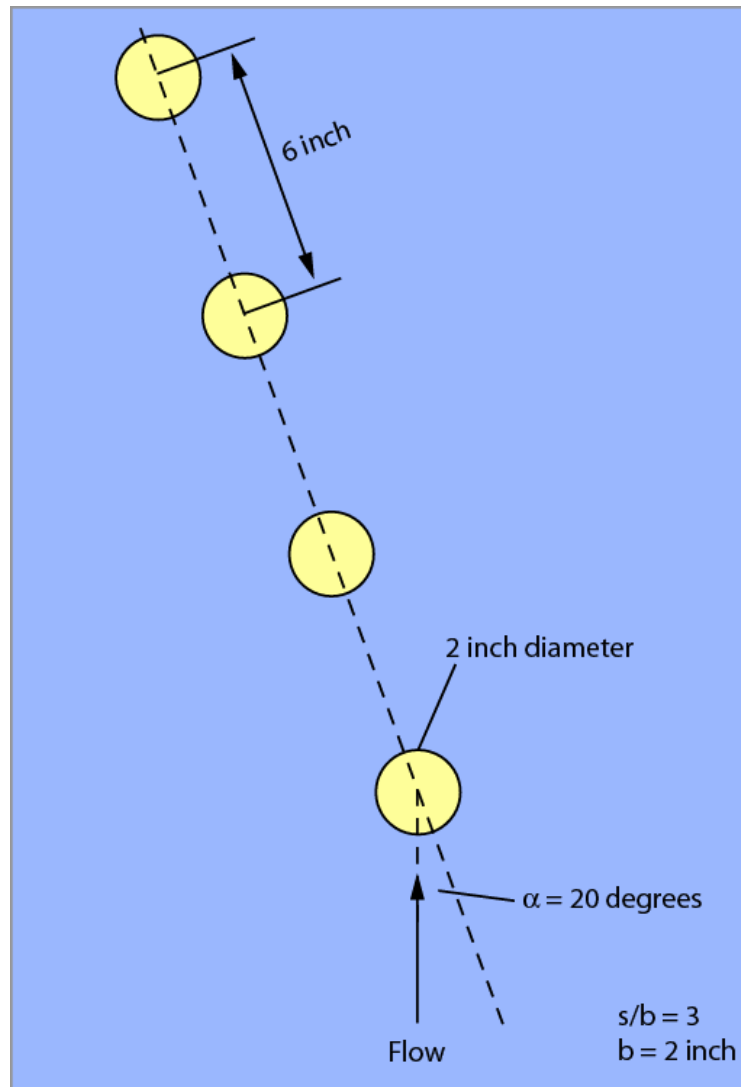
Figure 13 Plan View of Test 4 Set-Up (Pier 3).
