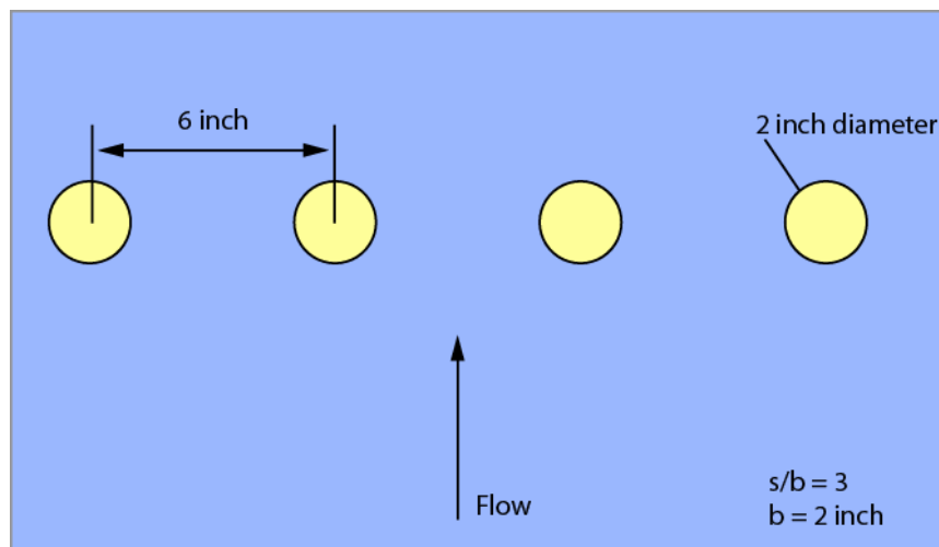
Figure 14 Plan View of Test 5 Set-Up (Pier 3).
