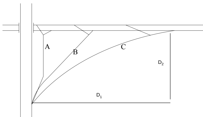
Figure 10.4 Exit Ramp Configurations
