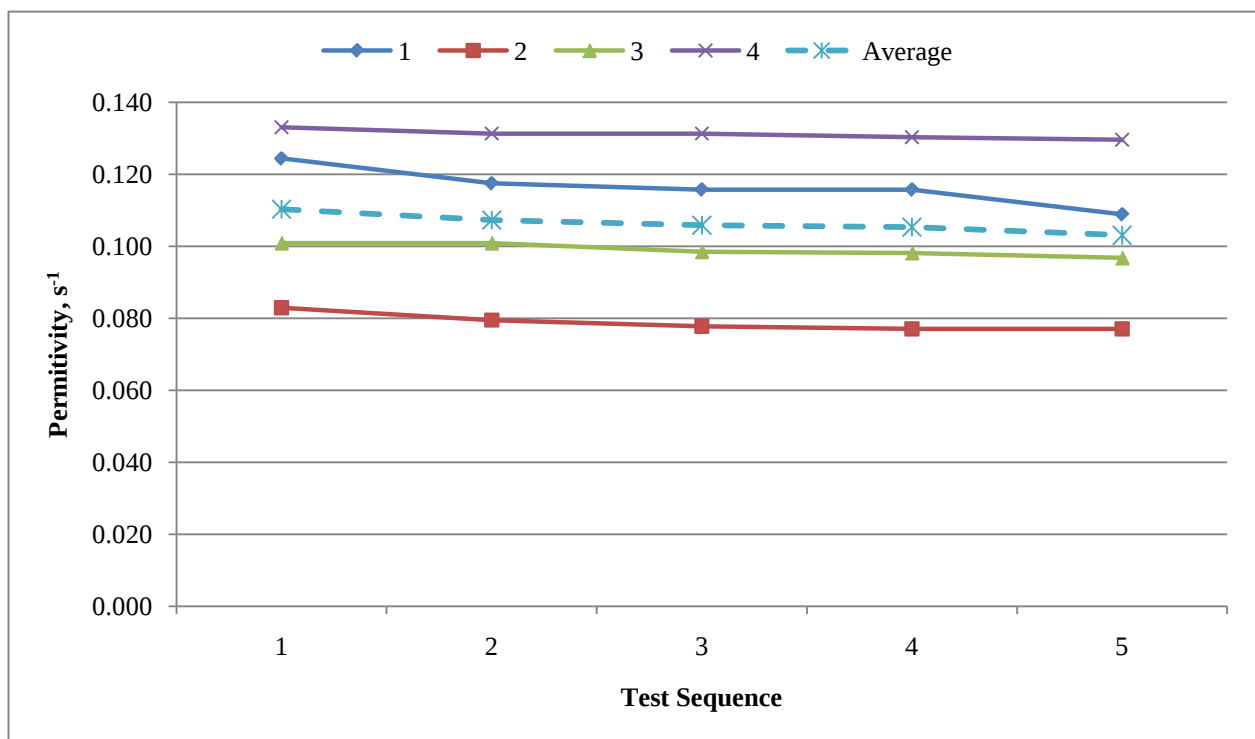
Figure 48 Plot of permittivity versus test sequence for Type III silt fence material
