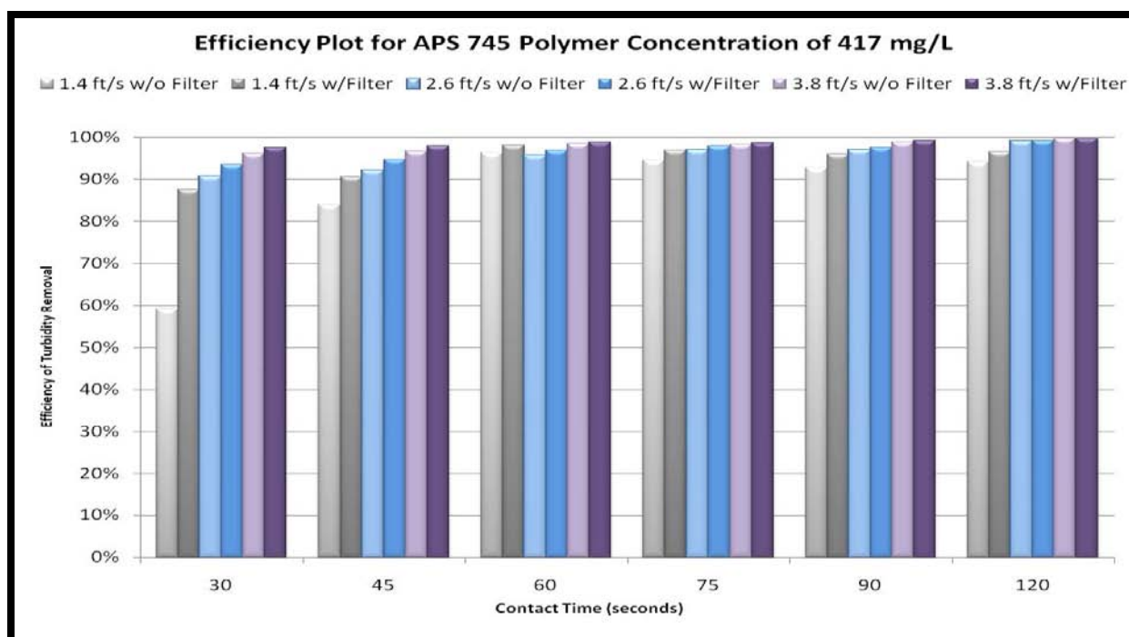
Figure 53 Plot of efficiencies for polymer APS 745 at a concentration of 417 mg/L
