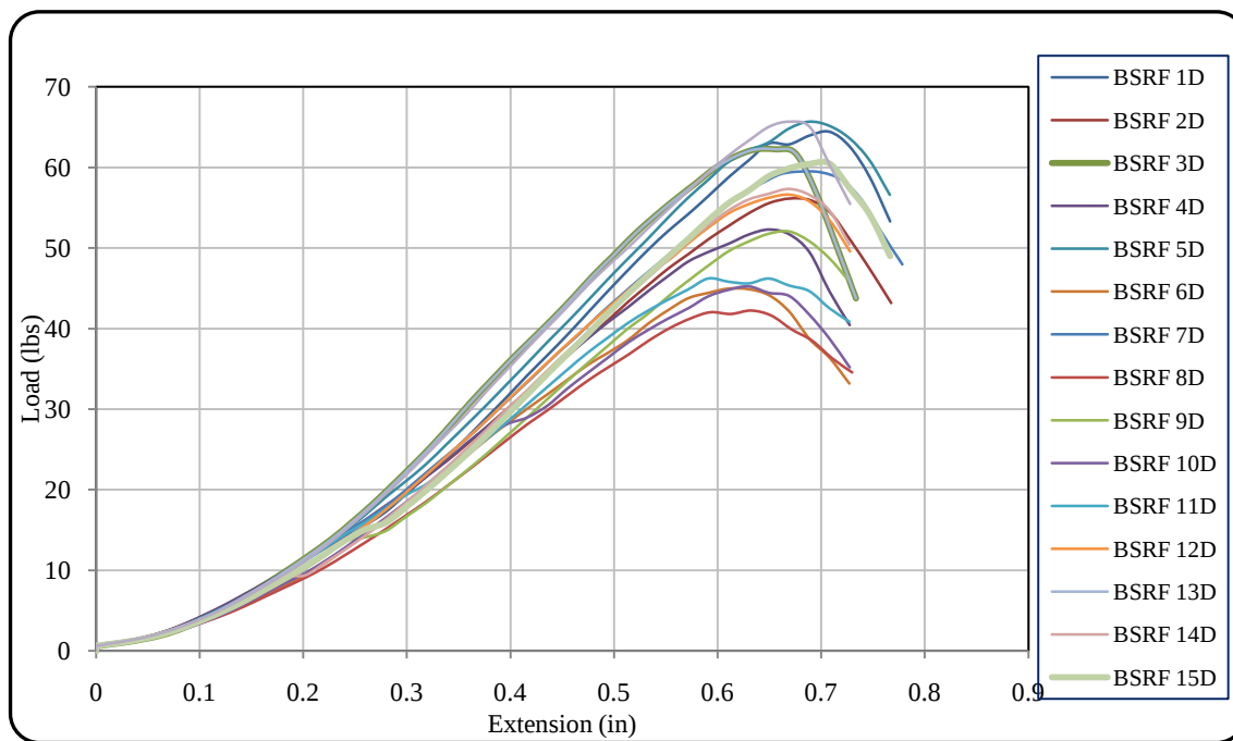
Figure 37 Puncture resistance plot for BSRF in dry condition
