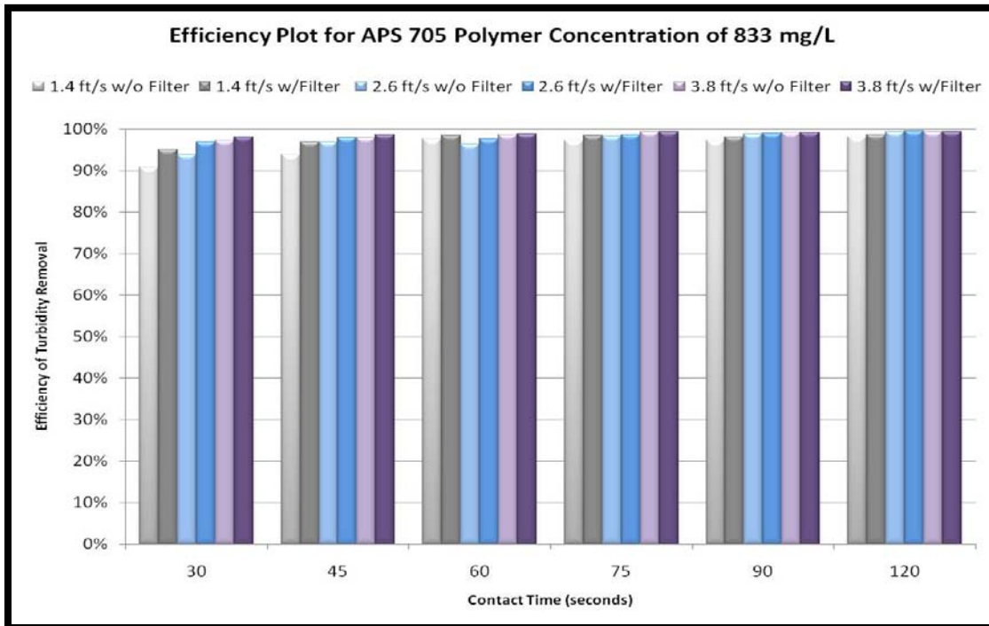
Figure 61 Plot of efficiencies for 833 mg/L concentration of APS 705 PAM product
