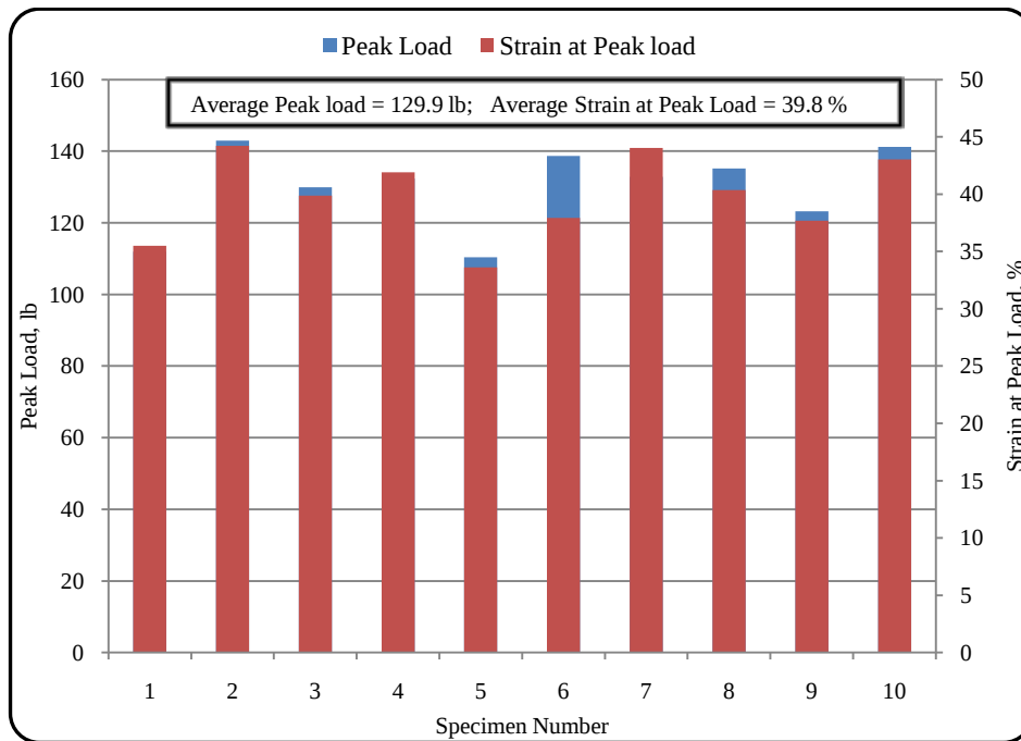
Figure 17 Peak Loads and corresponding strains for dry, machine direction (DMD) on BSRF
