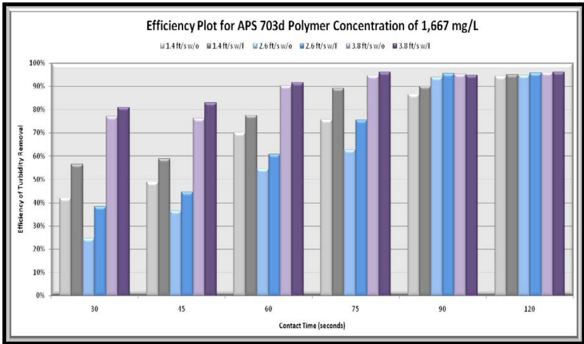
Figure 58 Plot of efficiencies for 1667 mg/L concentration of APS 703d PAM product
