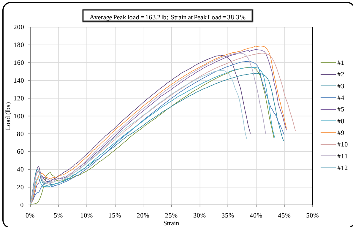
Figure 14 Load versus strain plot for dry, cross-machine direction (DCMD) on BSRF
