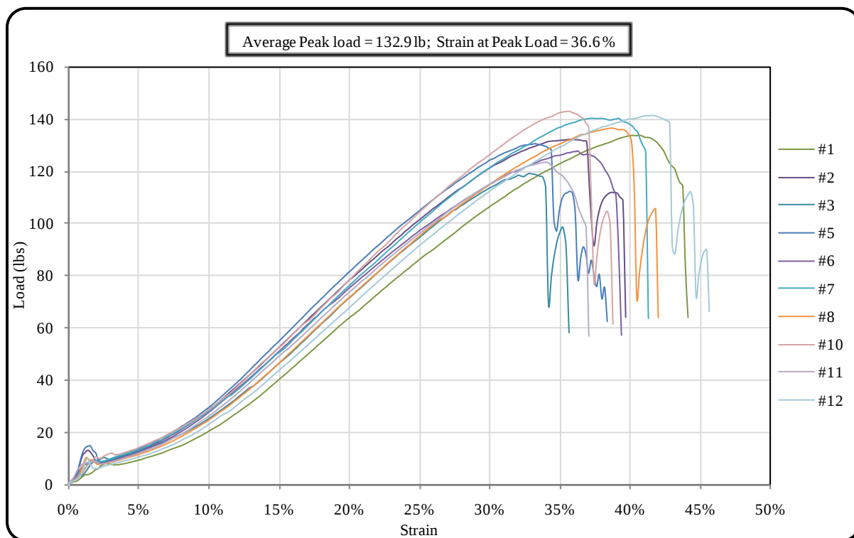
Figure 20 Load versus strain plot for wet, machine direction (WMD) on BSRF
