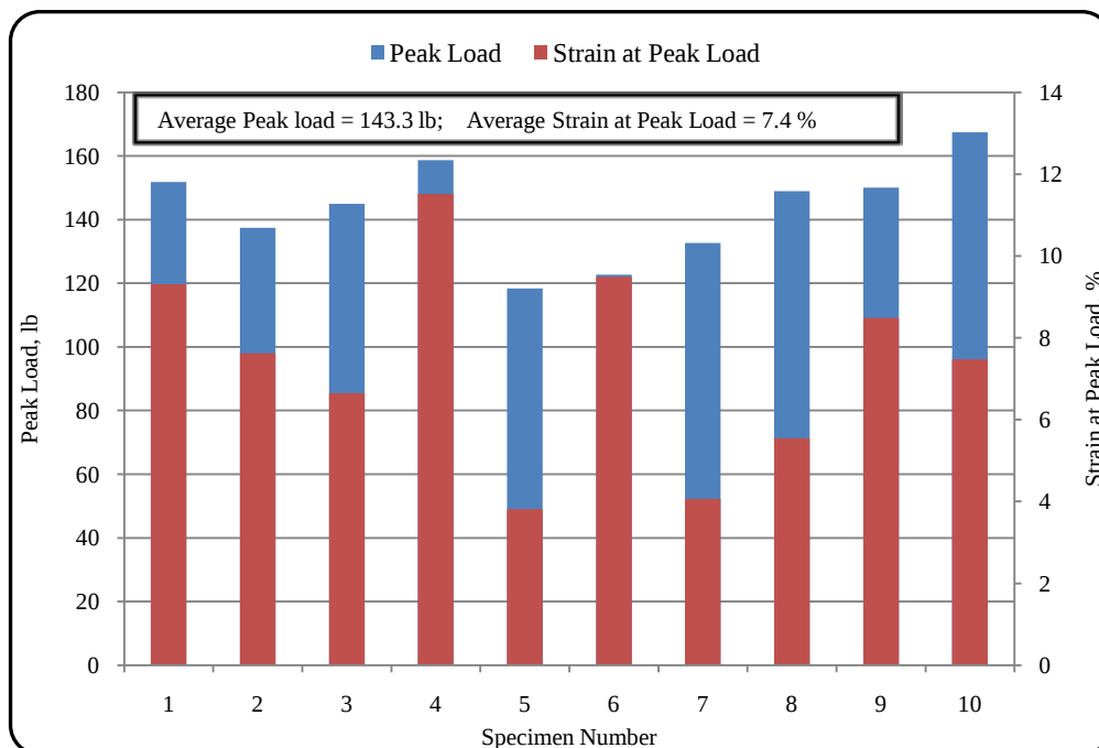
Figure 23 Peak loads and corresponding strains for DCMD on Type III silt fence
