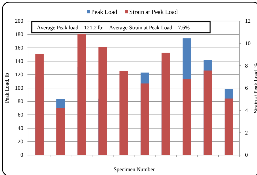
Figure 29 Peak loads and corresponding strains for WMD on Type III silt fence
