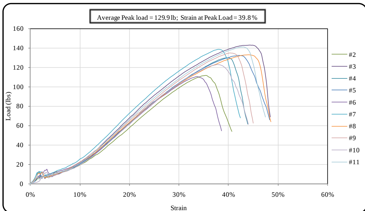
Figure 16 Load versus strain plot for dry, machine direction (DMD) on BSRF
