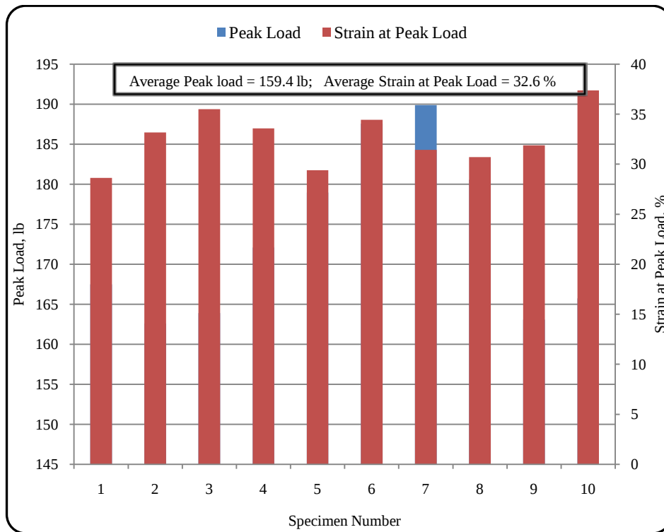
Figure 19 Peak Loads and corresponding strains for wet, cross-machine direction (WCMD) on BSRF
