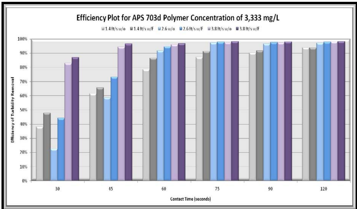
Figure 59 Plot of efficiencies for 3334 mg/L concentration of APS 703d PAM product
