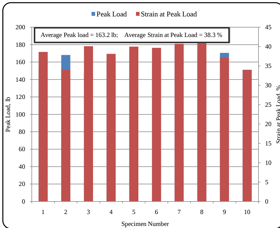
Figure 15 Peak Loads and corresponding strains for dry, cross-machine direction (DCMD) on BSRF
