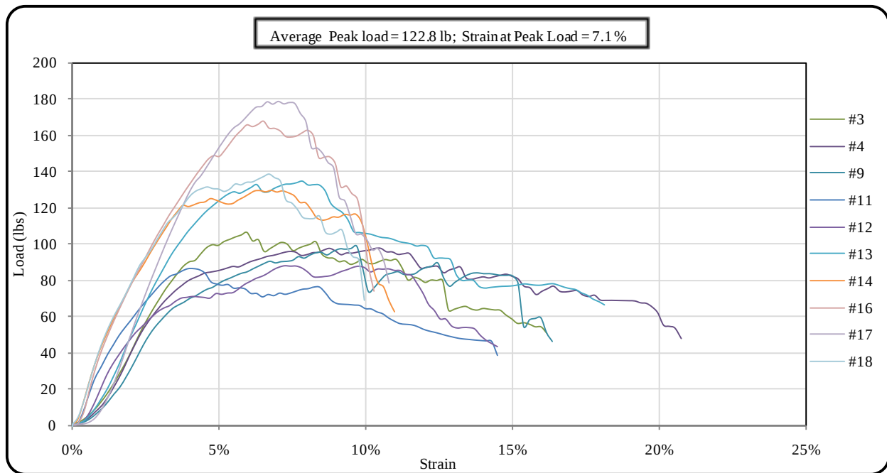
Figure 26 Load versus strain plot for WCMD on Type III silt fence
