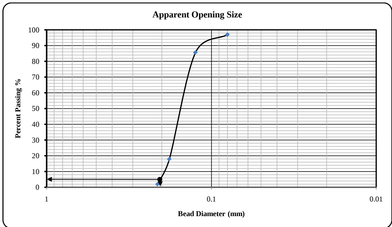
Figure 43 Plot of apparent opening size for BSRF silt fence material
