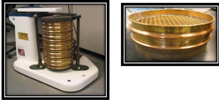
Figure 3 Apparatus for apparent opening size test on geotextiles (rotary sieve shaker and sieve set) – ASTM D4751
