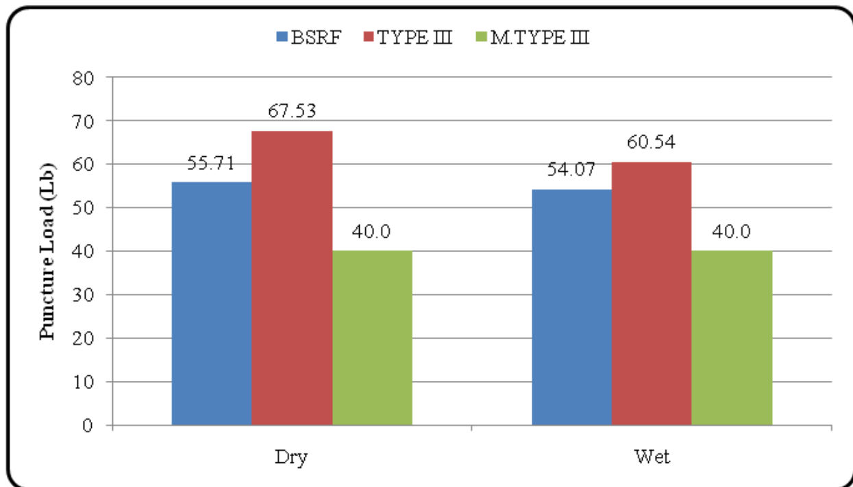
Figure 41 Comparison of average puncture resistance between BSRF* and Type III silt fence barriers
