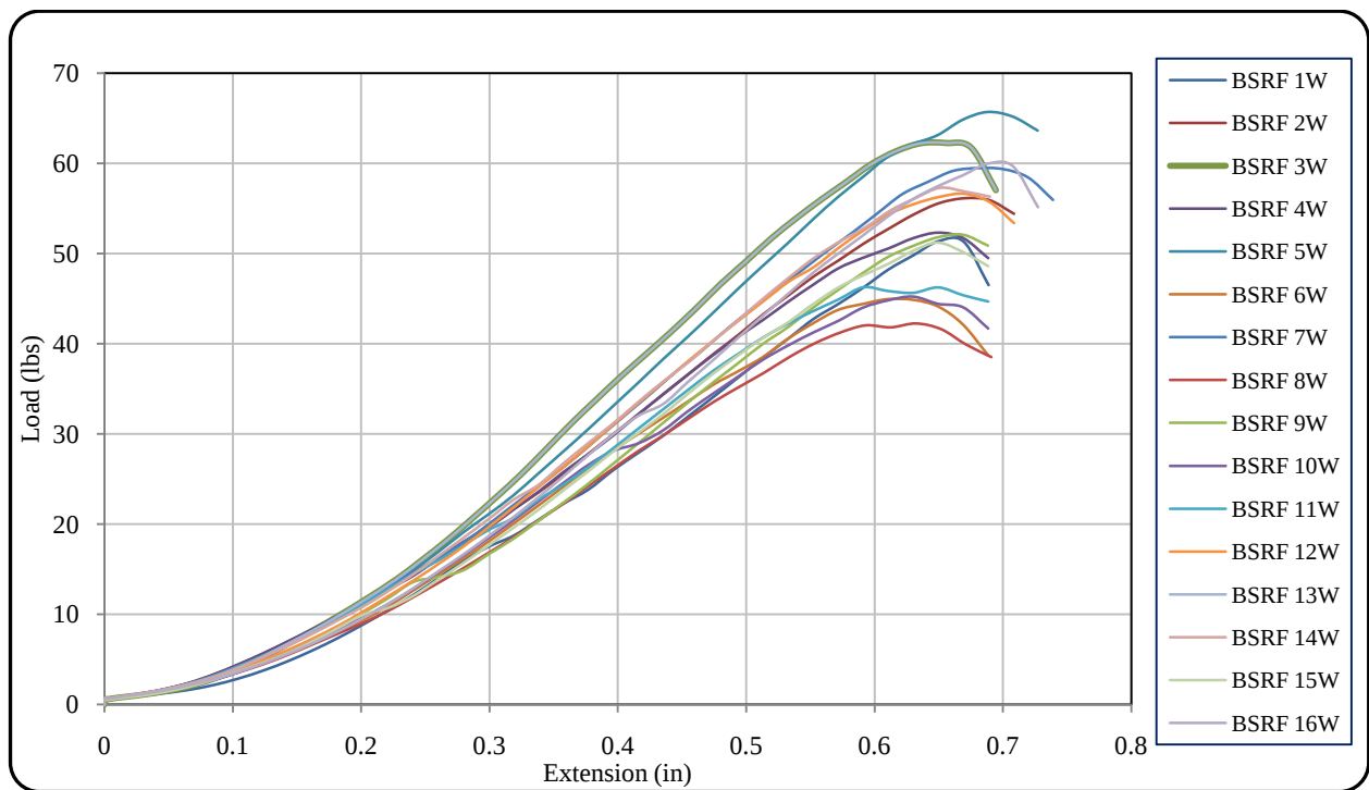
Figure 38 Puncture resistance plot for BSRF in wet condition
