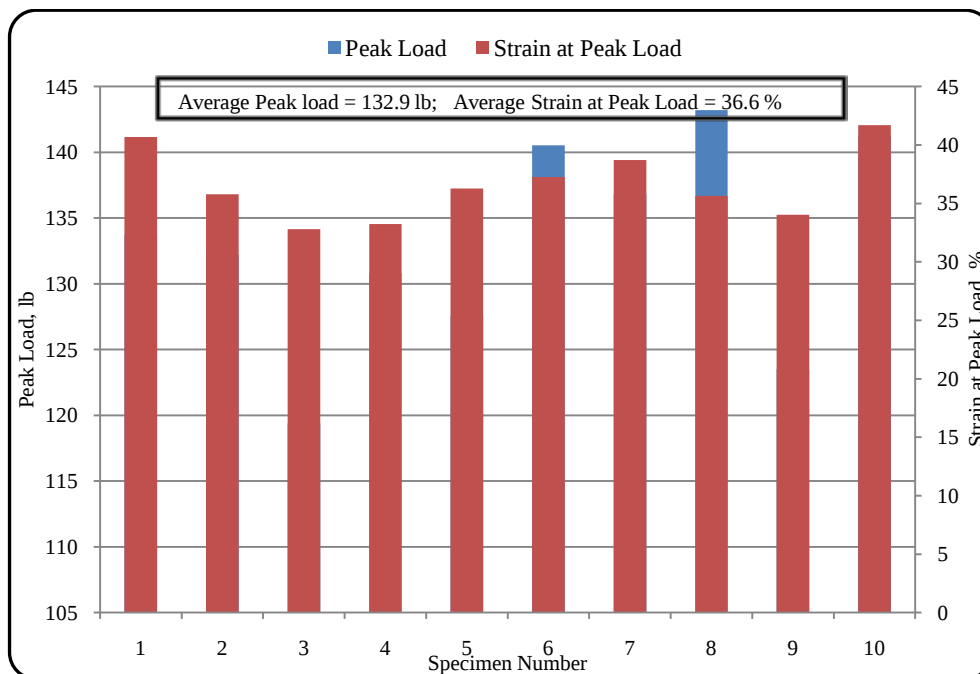
Figure 21 Peak Loads and corresponding strains for wet, machine direction (WMD) on BSRF
