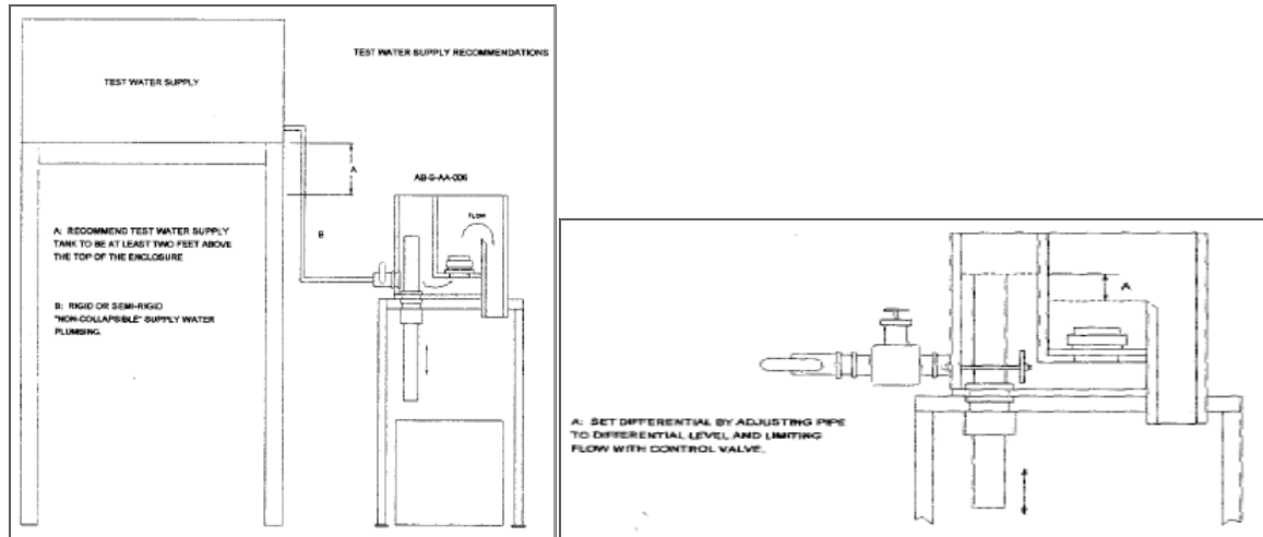
Figure 46 Constant head test setup of the permittivity device
