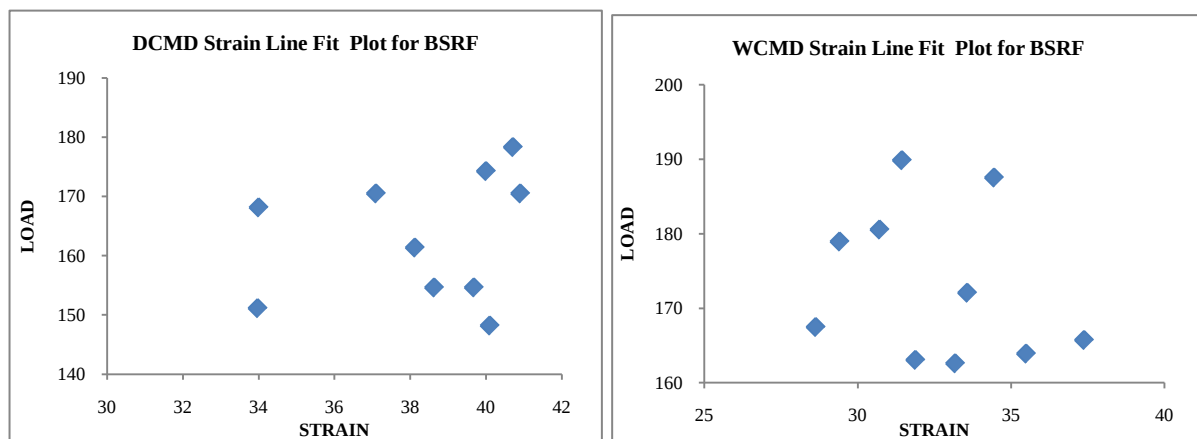
Figure 31 Correlation plot between grab strength and strain at peak load for DCMD and WCMD tests on BSRF
