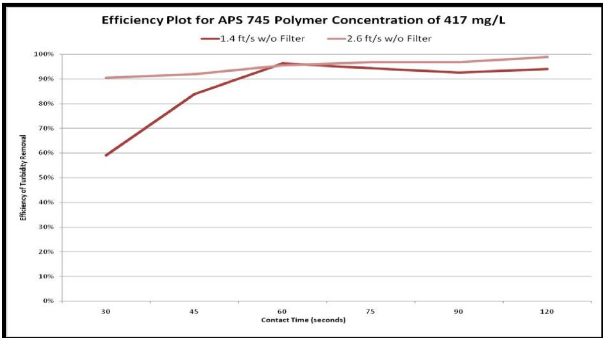
Figure 54 Line graph for APS 745 Polymer at concentration of 417 mg/L
