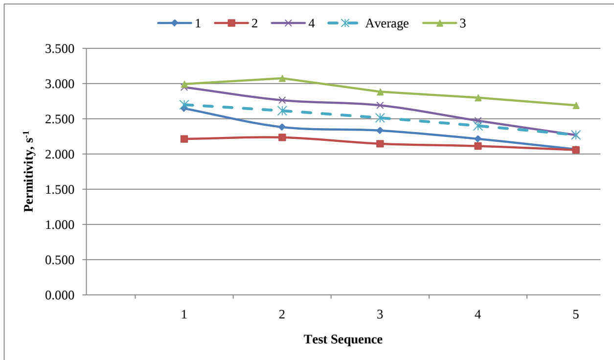
Figure 47 Plot of permittivity versus test sequence for BSRF silt fence material
