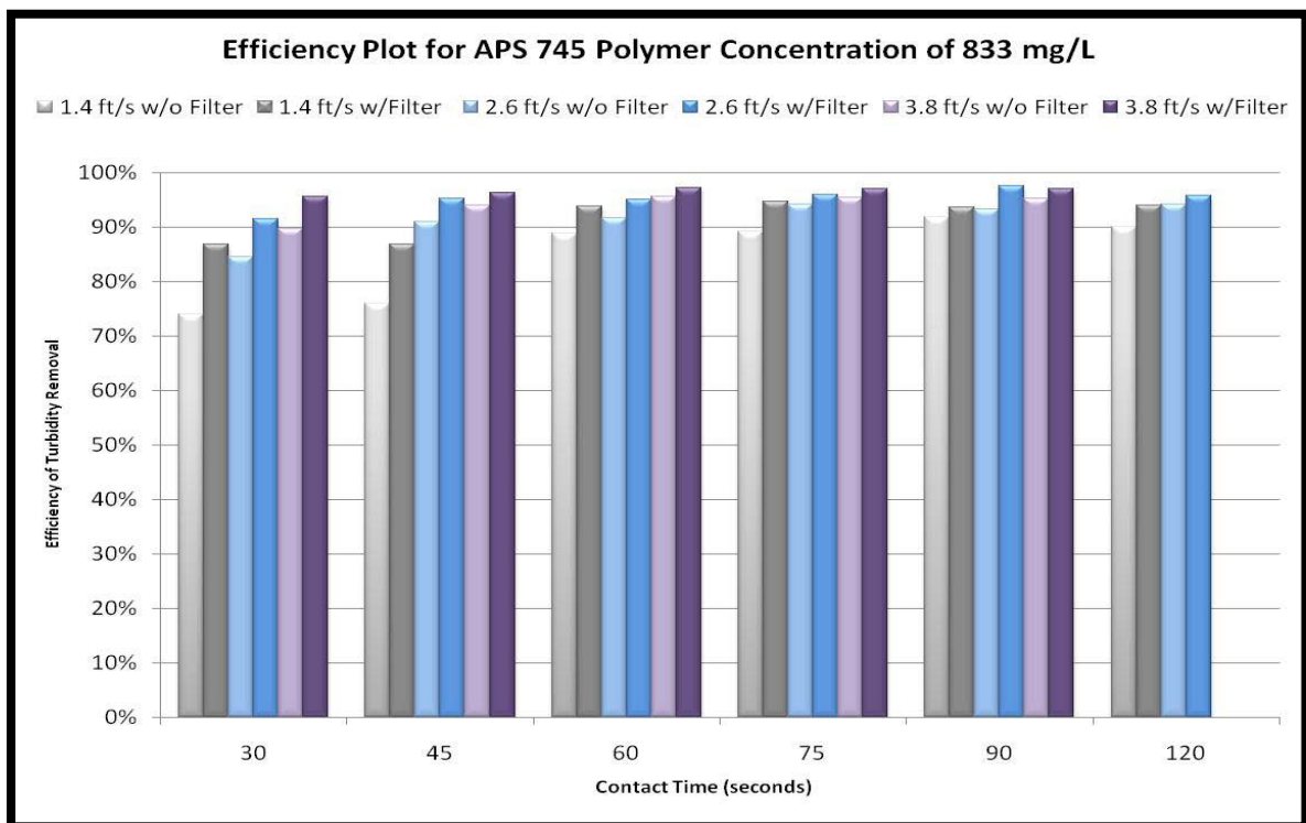
Figure 55 Plot of efficiencies for polymer APS 745 at a concentration of 833 mg/L
