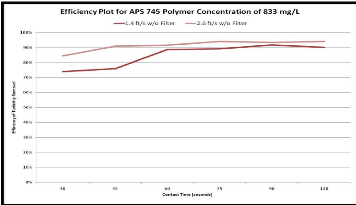
Figure 56 Line graph for APS 745 Polymer at concentration of 833 mg/L
