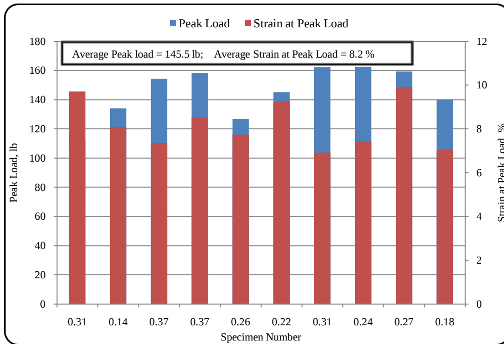
Figure 25 Peak loads and corresponding strains for DMD on Type III silt fence
