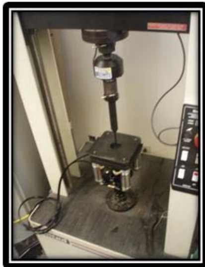
Figure 4 Apparatus for puncture test (Tensile/compression testing machine, clamp attachment and solid steel rod) – ASTM D4833
