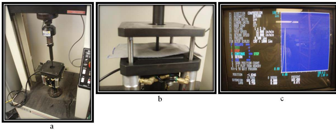
Figure 36 Index puncture resistance test set-up and fixtures
