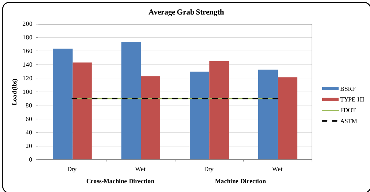
Figure 34 Comparisons of average grab strength results with specifications
