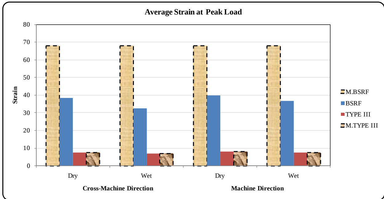
Figure 35 Comparisons of actual average strains at peak loads with manufacturers' specifications
