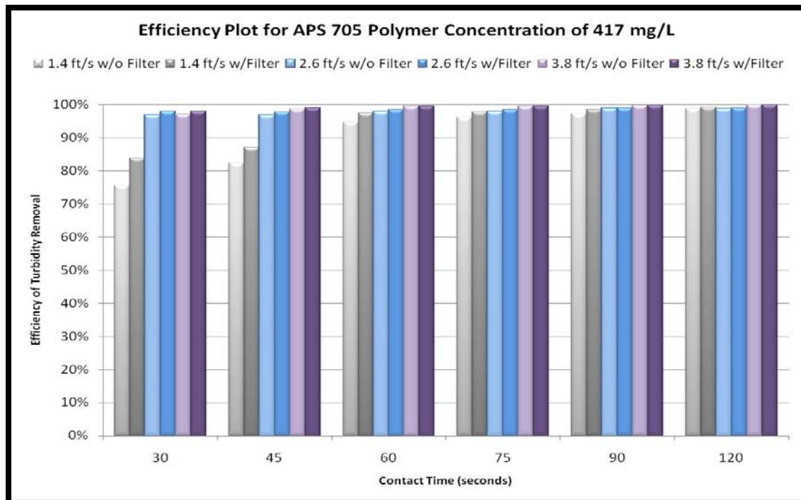
Figure 60 Plot of efficiencies for 417 mg/L concentration of APS 705 PAM product
