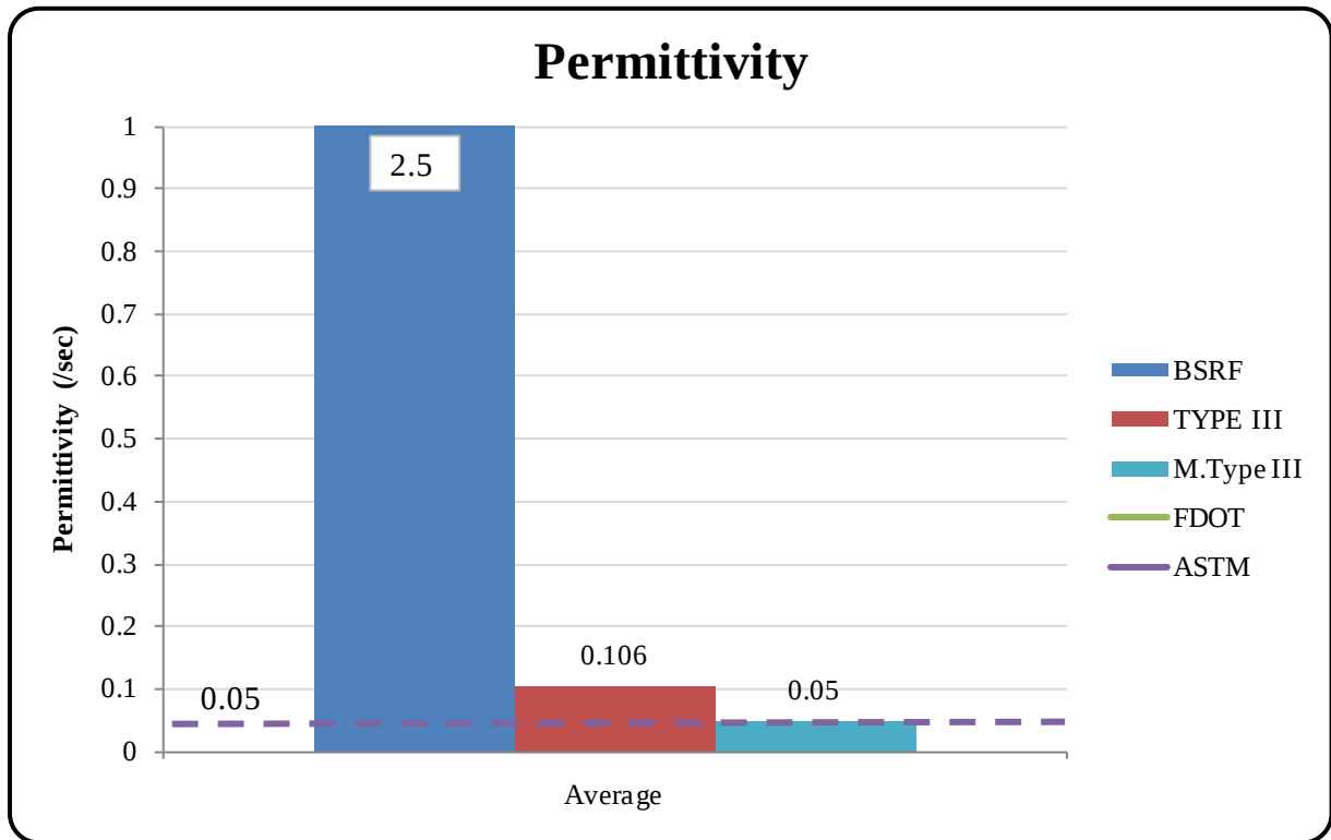
Figure 51 Comparison of permittivity values of silt fence materials
