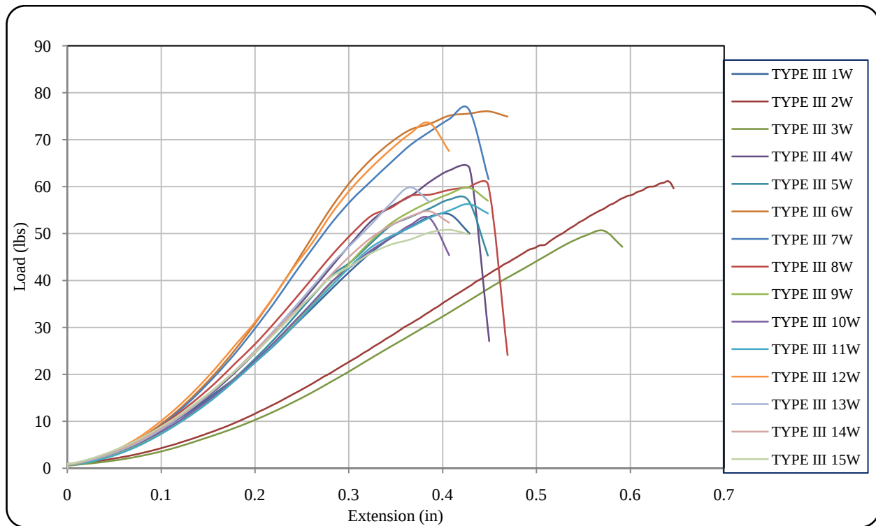
Figure 40 Puncture resistance plot for Type III in wet condition
