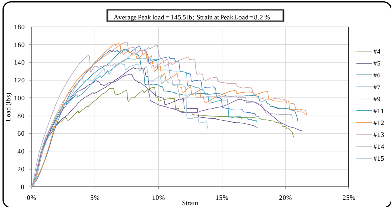
Figure 24 Load versus strain plot for DMD on Type III silt fence
