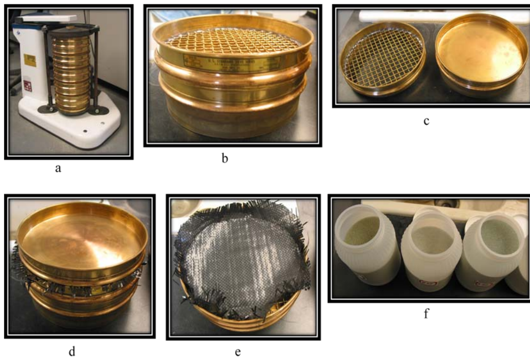
Figure 42 AOS Sieve shaker, sieve frame, glass beads and silt fence material
