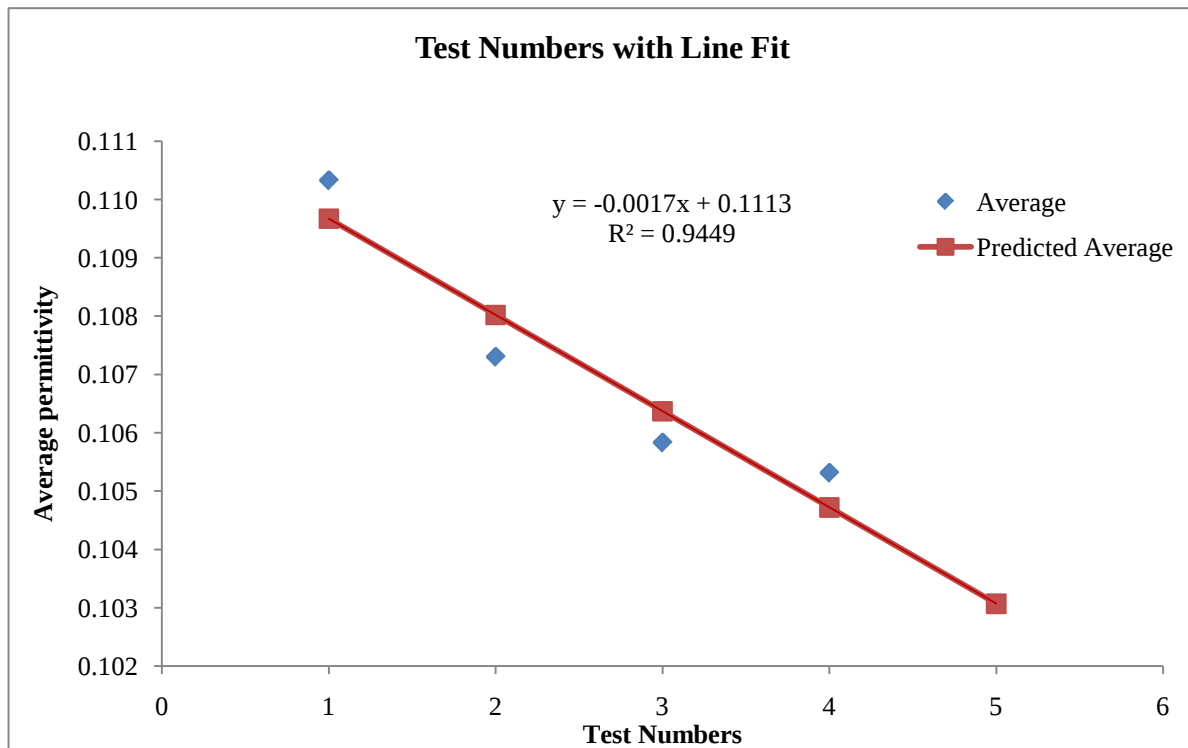
Figure 50 Permittivity regression plots for Type III silt fence
