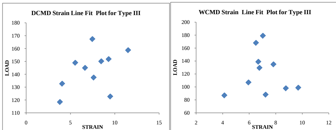
Figure 33 Correlation plot between grab strength and strain at peak load for DCMD and WCMD tests on Type III silt fence
