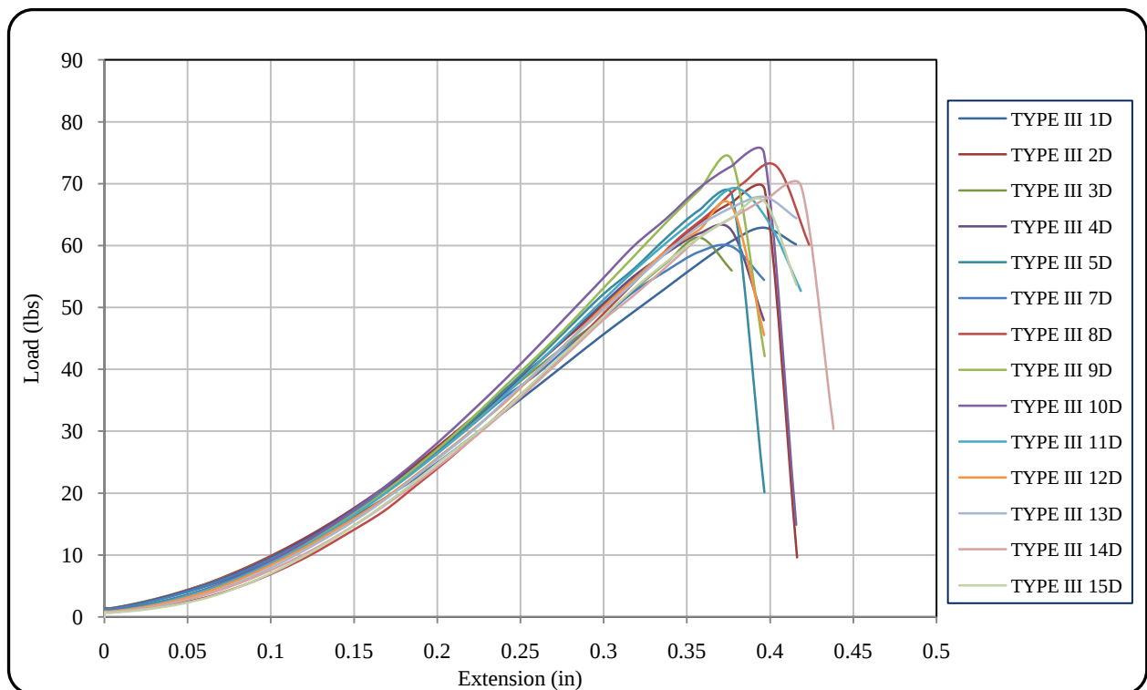
Figure 39 Puncture resistance plot for Type III in dry condition
