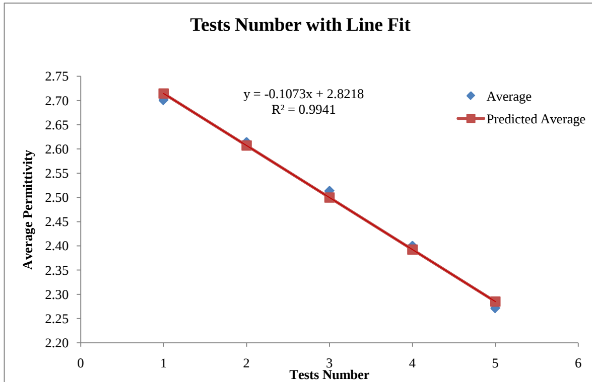
Figure 49 Permittivity regression plots for BSRF silt fence
