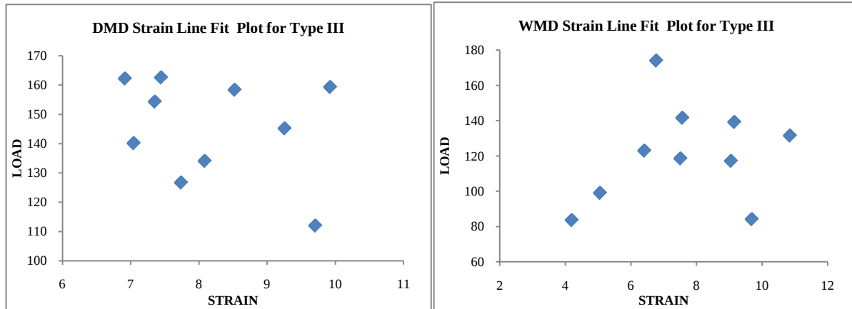
Figure 32 Correlation plot between grab strength and strain at peak load for DMD and WMD tests on Type III silt fence
