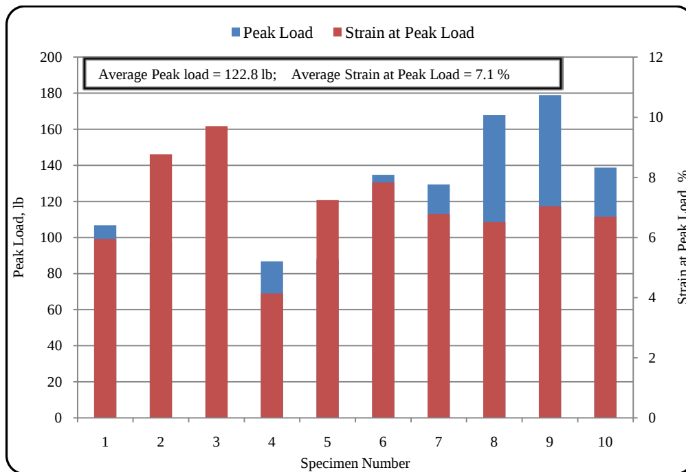
Figure 27 Peak loads and corresponding strains for WCMD on Type III silt fence
