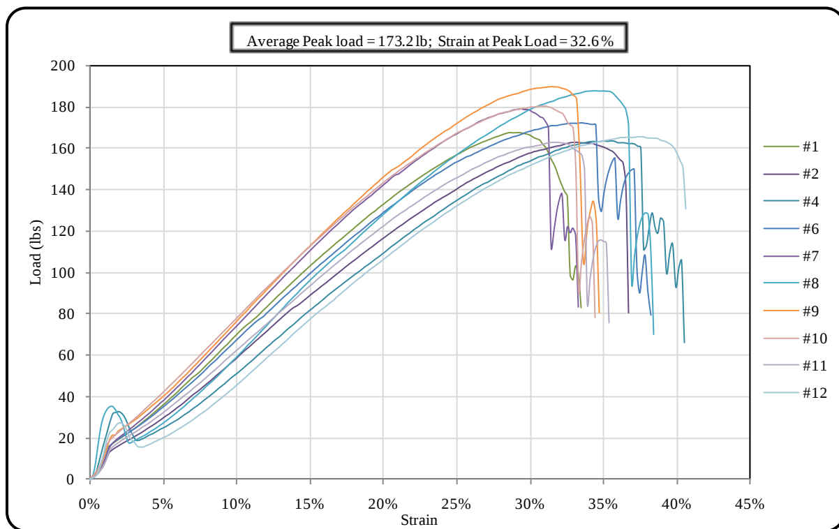
Figure 18 Load versus strain plot for wet, cross-machine direction (WCMD) on BSRF
