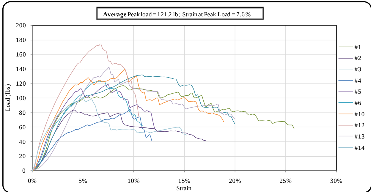
Figure 28 Load versus strain plot for WMD on Type III silt fence
