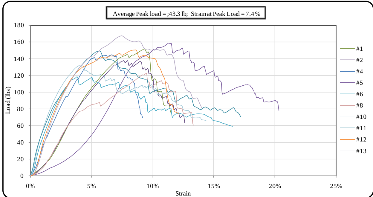
Figure 22 Load vs. strain plot for DCMD on Type III silt fence
