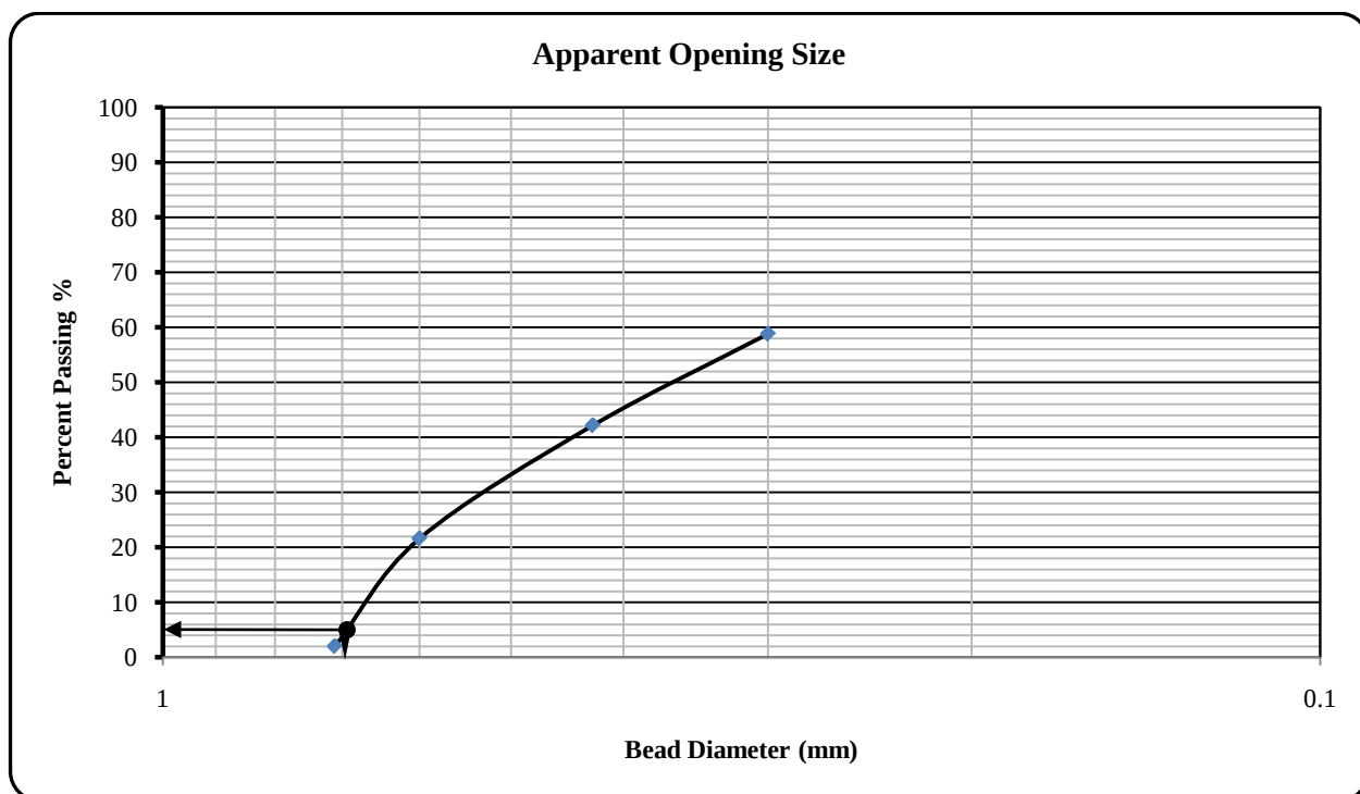
Figure 44 Plot of apparent opening size for Type III silt fence material
