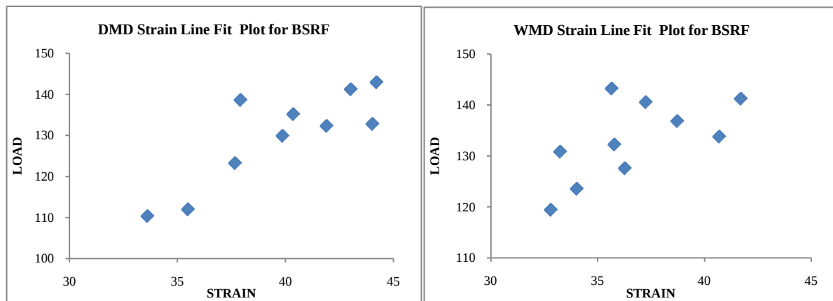
Figure 30 Correlation plot between grab strength and strain at peak load for DMD and WMD tests on BSRF
