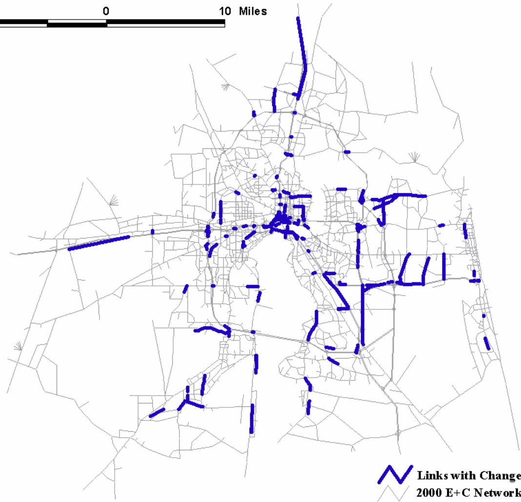
Figure 7.4 Links with Changed Number of Lanes in the 2000 E+C Network
