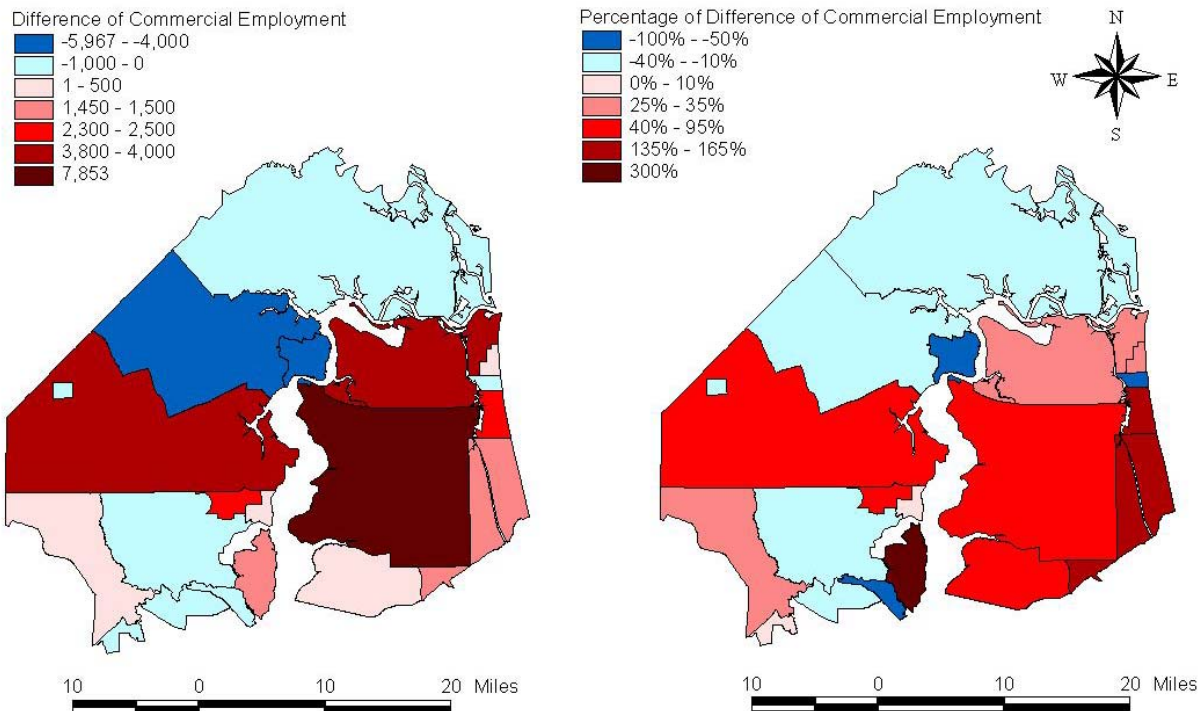
Figure 6.16 Differences in Commercial Employment Estimations for E+C and 2000 Base Year Models
