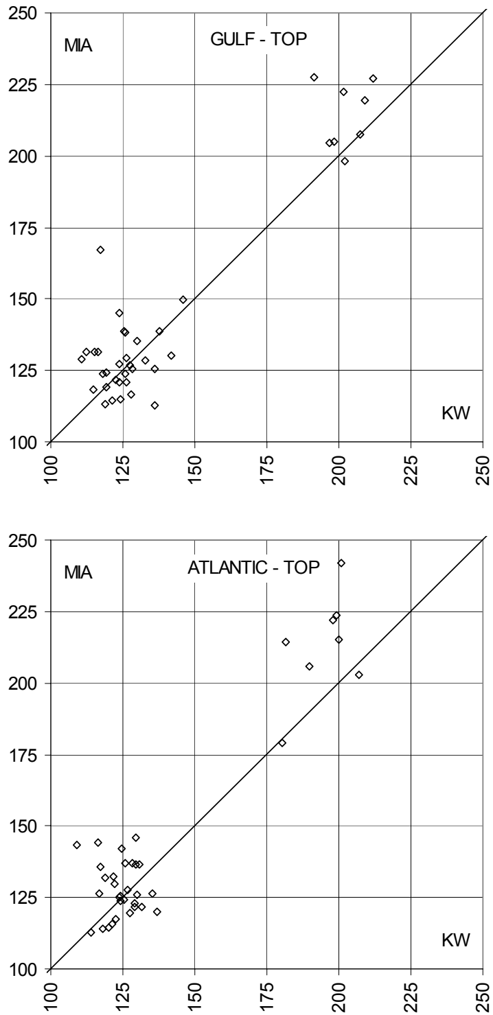
Figure 10. Calculated stiffness (kN-m 2 ) at the Miami end (MIA), as function of the stiffness as the Key West end (KW), of each Top tendon in the bridge. An ideal 1:1 diagonal line is shown for reference. The upper and lower graphs are for Top tendons on the Gulf and Atlantic sides of the bridge respectively. The group of 8 symbols with higher stiffness values corresponds to the 27-strand tendons. The results shown are obtained using only the low frequency component of the double peaks.
