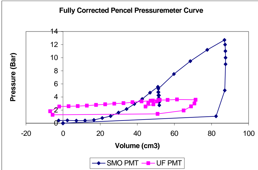
Figure 16. Comparison Graph of Data Interpretation from UF and SMO Pressuremeter at Depth 35 Feet
