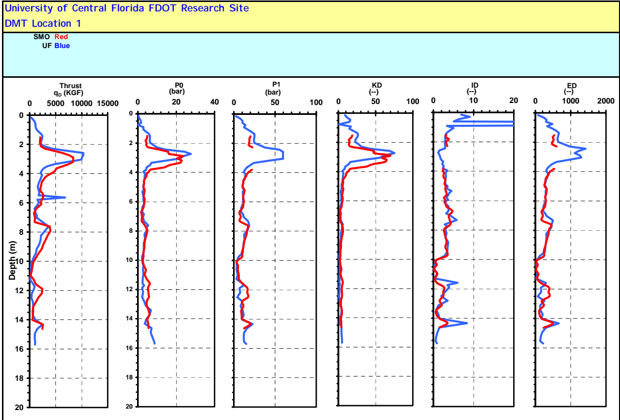
Figure 8. DMT Results for UF DMT 1 and SMO Located at East Group of SPT Tests
