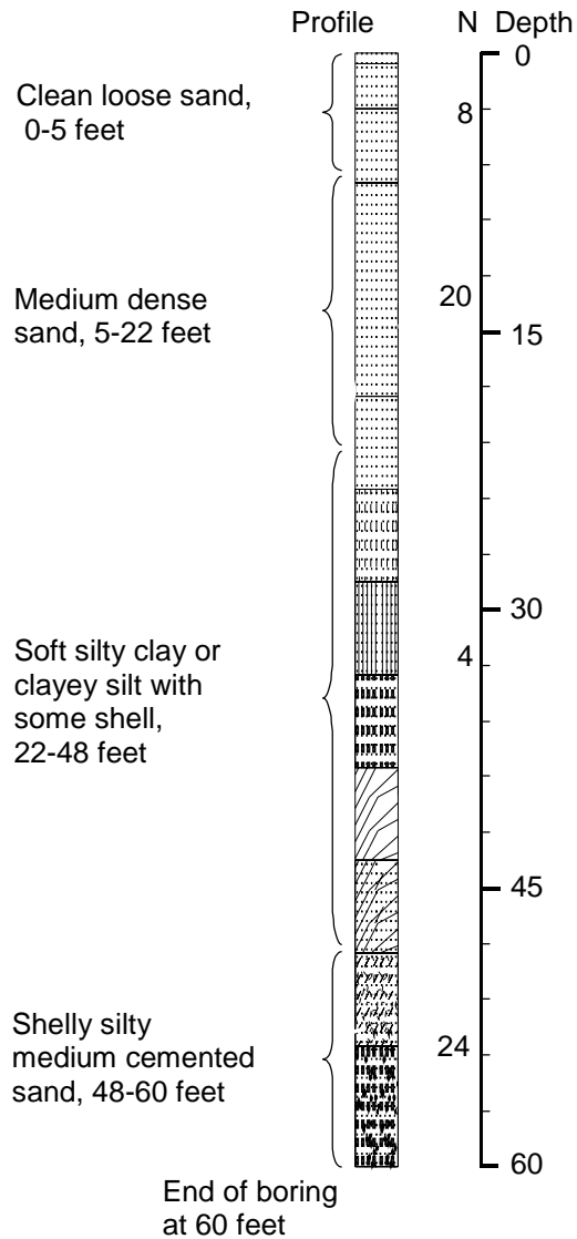
Figure 7. Generalized Site Stratigraphy from 5 SPT Tests
