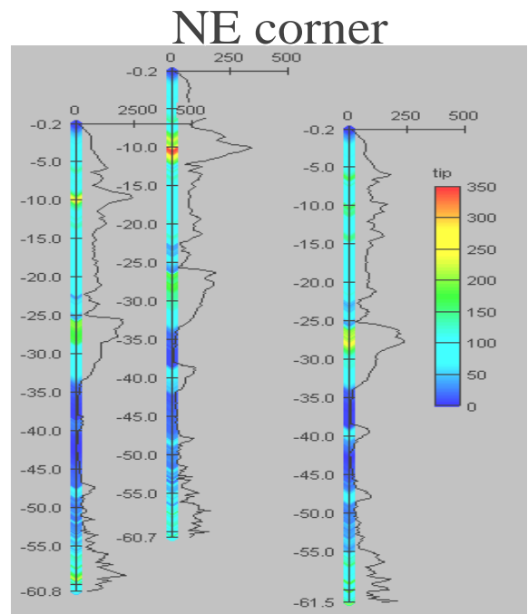
Figure 33. A Closer Look at the Change on Tip Resistance Between the “Hard” NE Corner and “Soft” SW Corner
