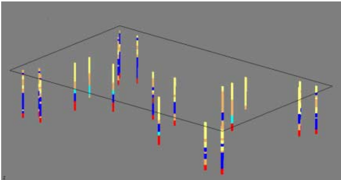
Figure 26. Relative Location of the CPT, SPT and DMT Borings Performed at the Site
