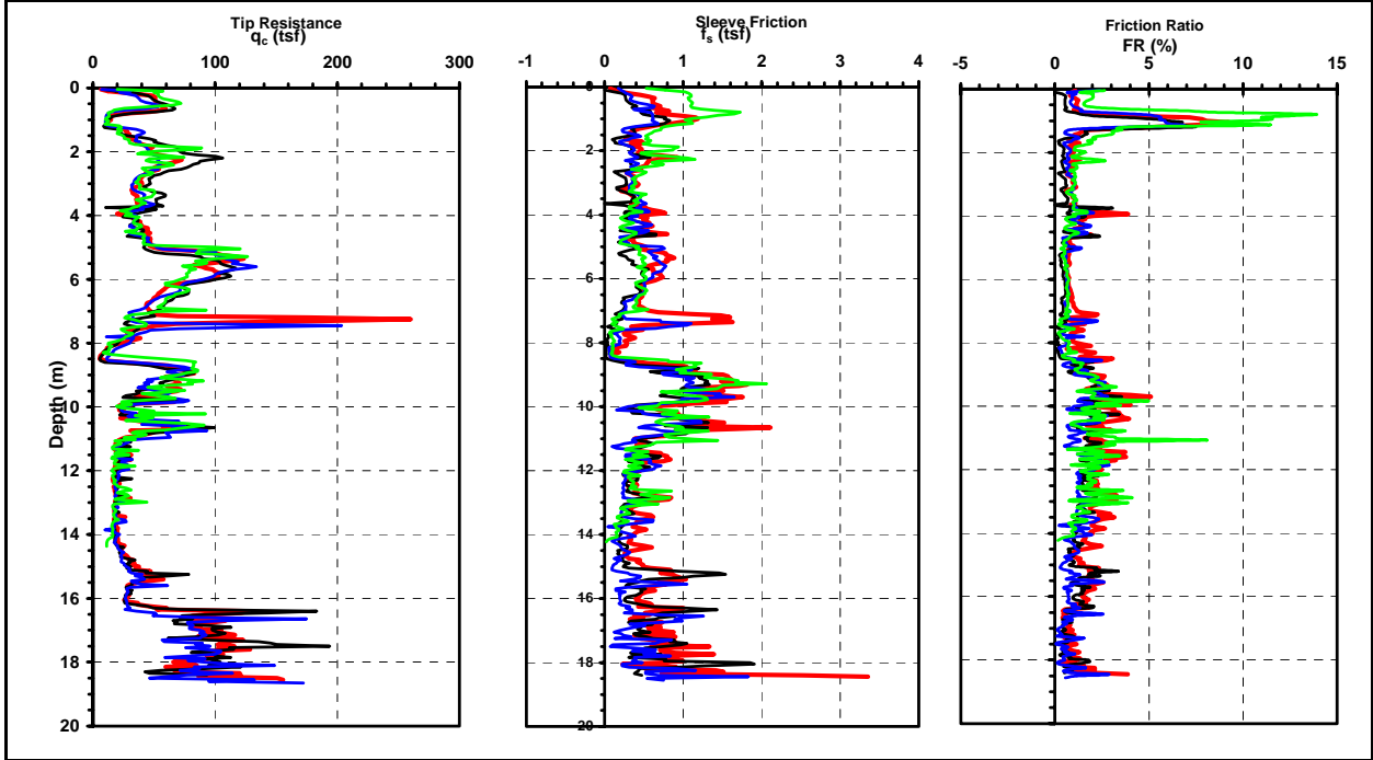
Figure 18. CPT Soundings at NW Corner Location 2
