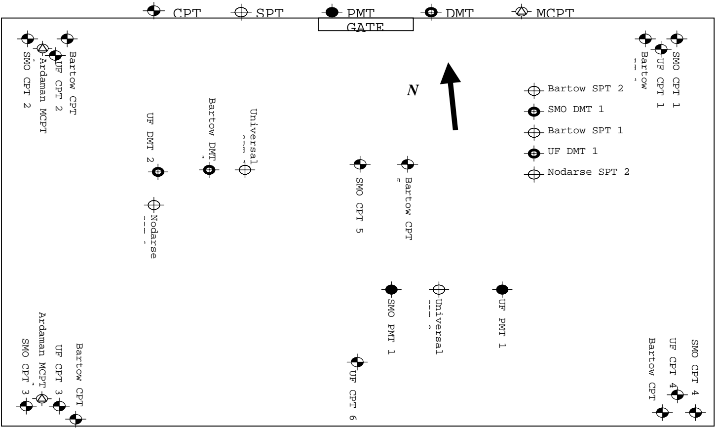
Figure 2. Boring and Sounding Plan
