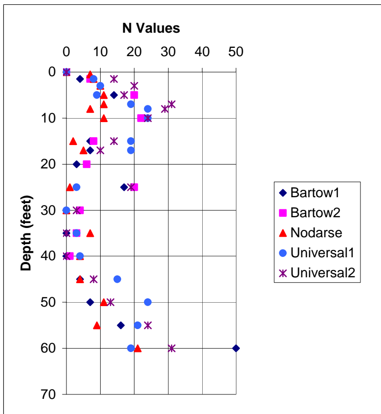
Figure 6. Summary of 5 SPT Borings at UCF Test Site
