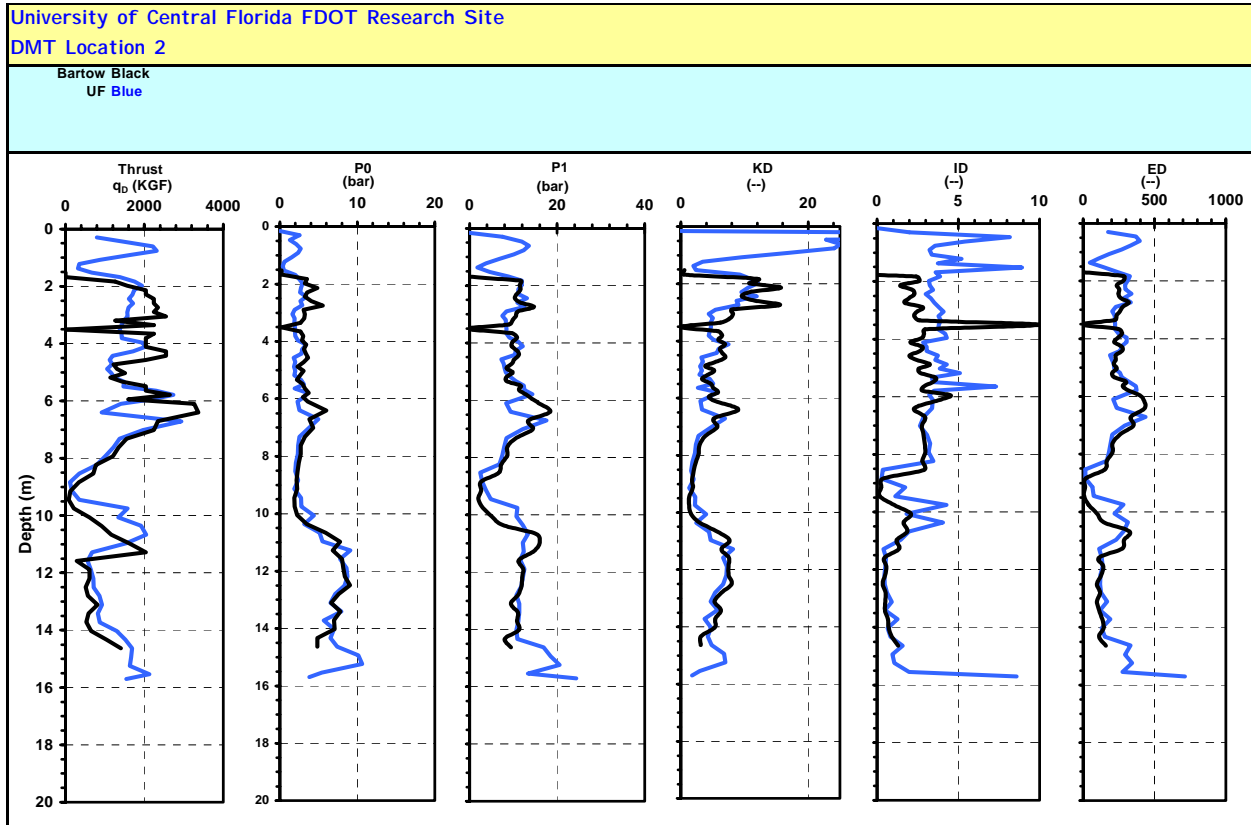
Figure 9. DMT Results for UF DMT 2 and FDOT District 1 Located at West Group of SPT Tests
