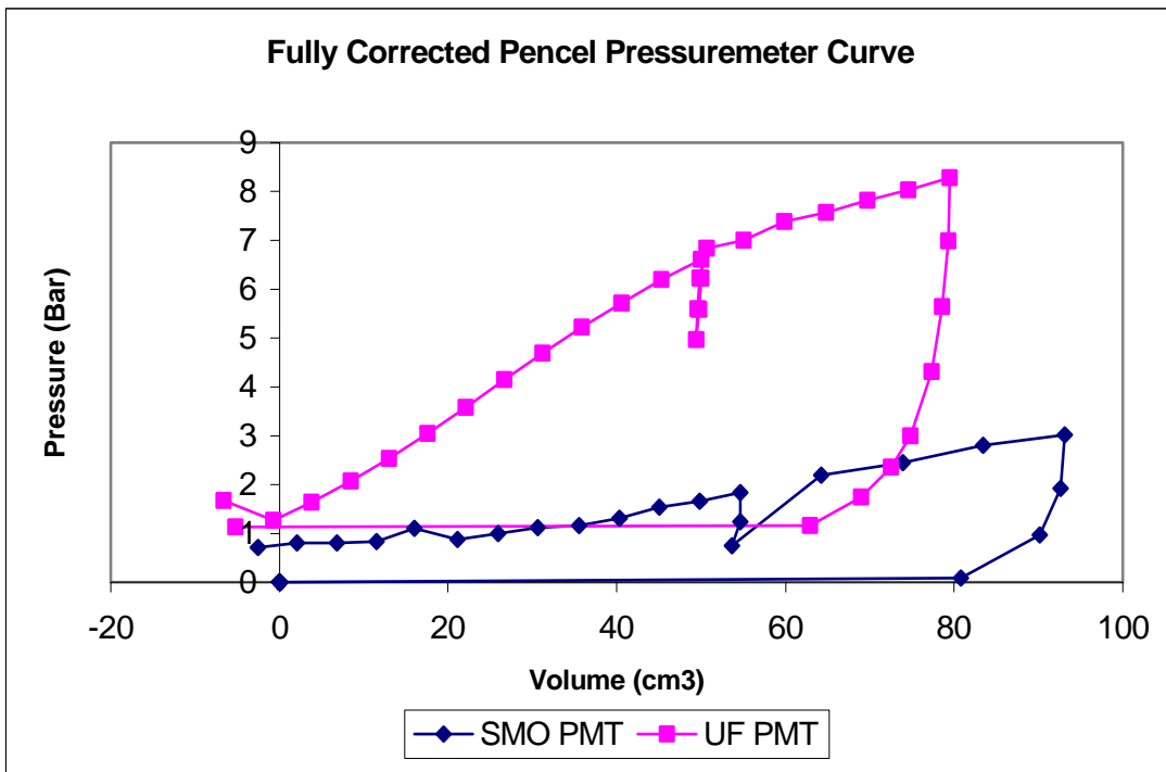
Figure 15. Comparison Graph of Data Interpretation from UF and SMO Pressuremeter at Depth 30 Feet
