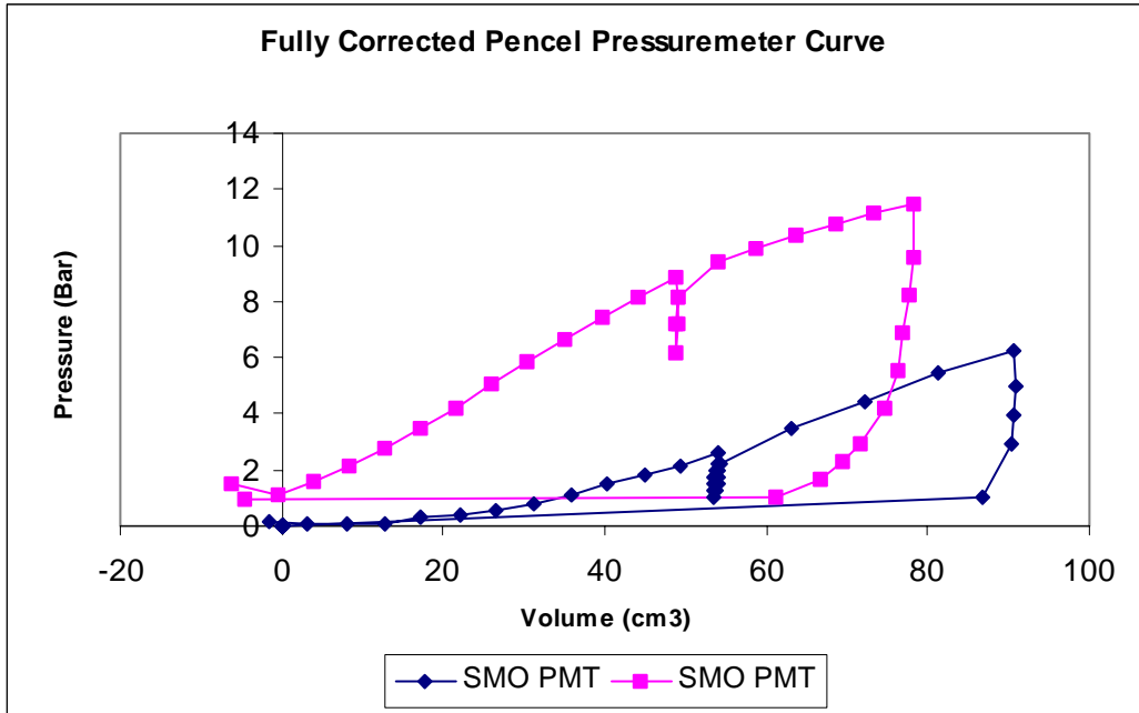
Figure 14. Comparison Graph of Data Interpretation from UF and SMO Pressuremeter at Depth 25 Feet
