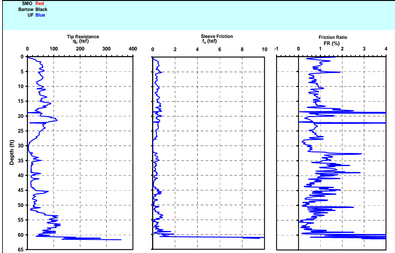
Figure 22. CPT Soundings at South Location 6 (South Center)
