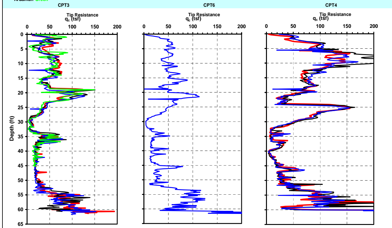
Figure 23. CPT Soundings Cross Section Show Increasing Tip Resistance Along SW to SE Portion of the Site
