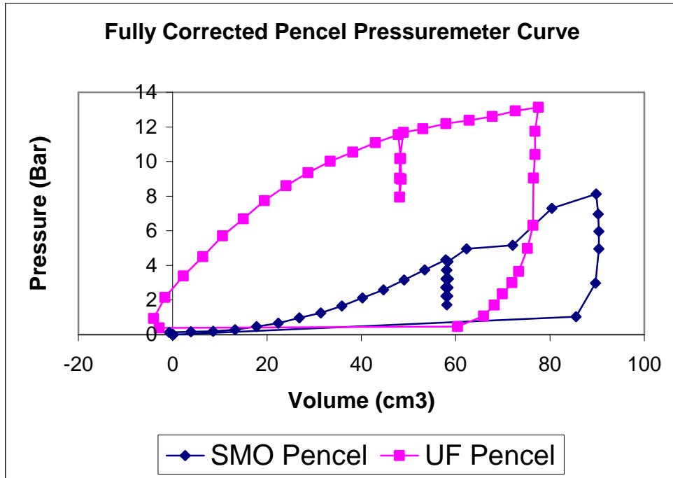
Figure 10. Comparison Graph of Data Interpretation from UF and SMO Pressuremeter at Depth 5 Feet
