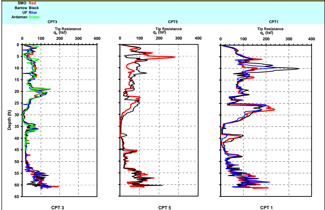
Figure 25. CPT Soundings Show Increasing Tip Resistance Along SW to NE Cross Section of the Site
