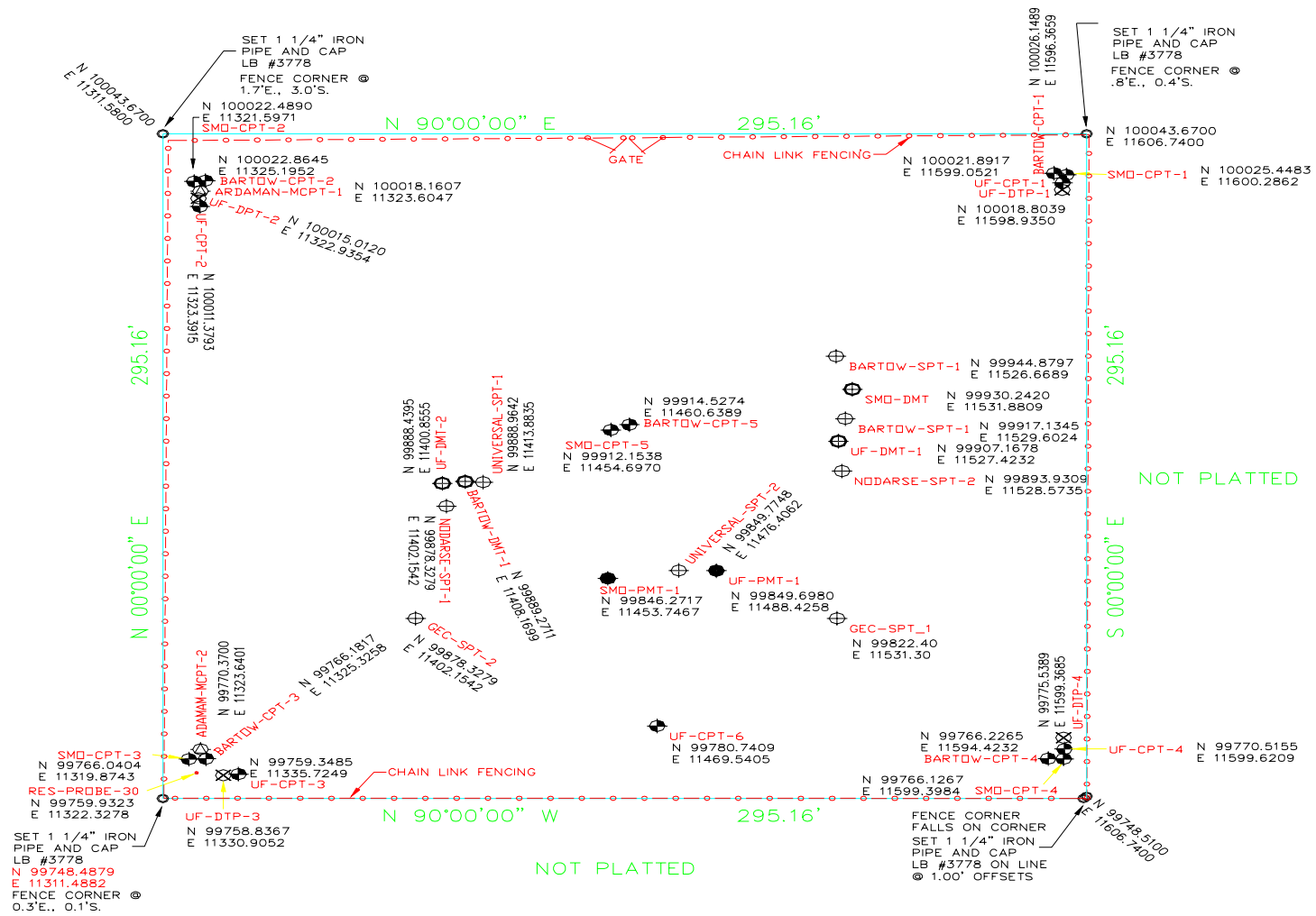
Figure 3. Plan View of the Site with the Exact Location of the Tests Performed
