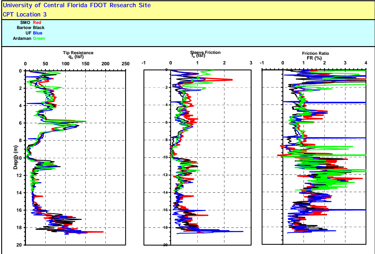
Figure 19. CPT Soundings at SW Corner Location 3
