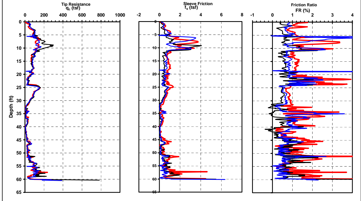
Figure 20. CPT Soundings at SW Corner Location 4
