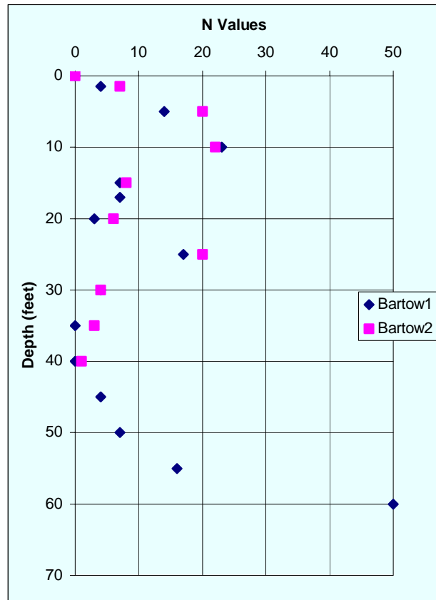
Figure 4. Energy Analysis SPT Group East
