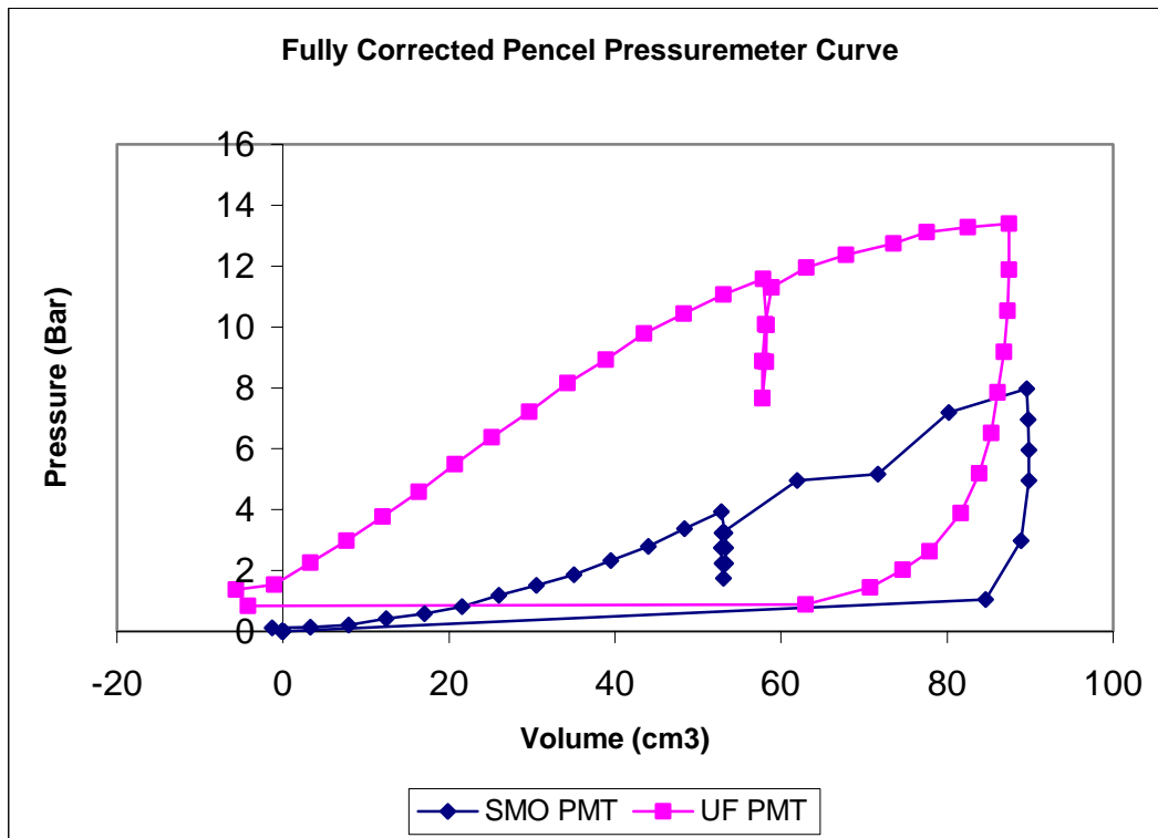
Figure 13. Comparison Graph of Data Interpretation from UF and SMO Pressuremeter at Depth 20 Feet
