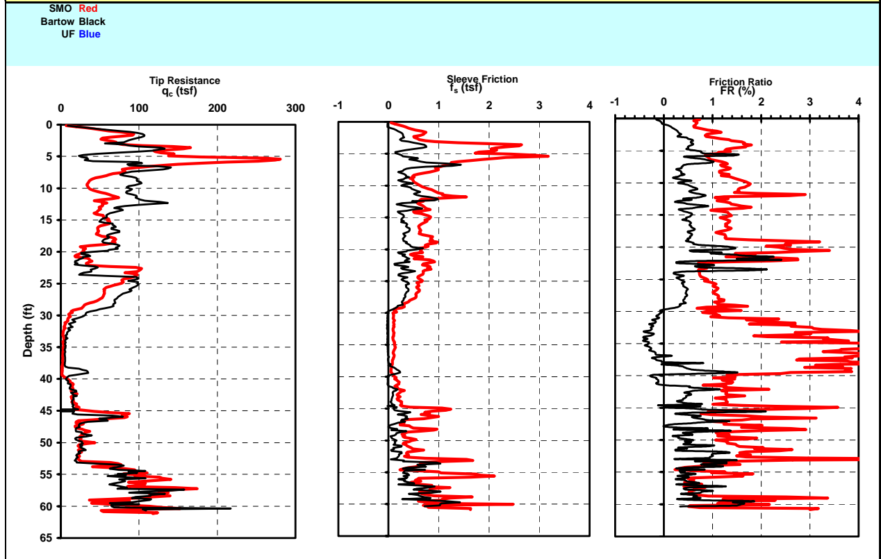
Figure 21. CPT Soundings at Center Location 5
