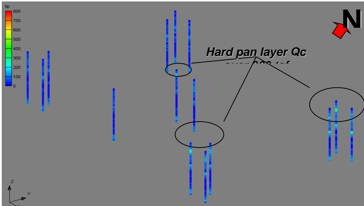
Figure 32. General Tip Resistance Characterization of the Site
