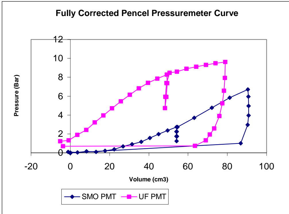
Figure 12. Comparison Graph of Data Interpretation from UF and SMO Pressuremeter at Depth 15 Feet
