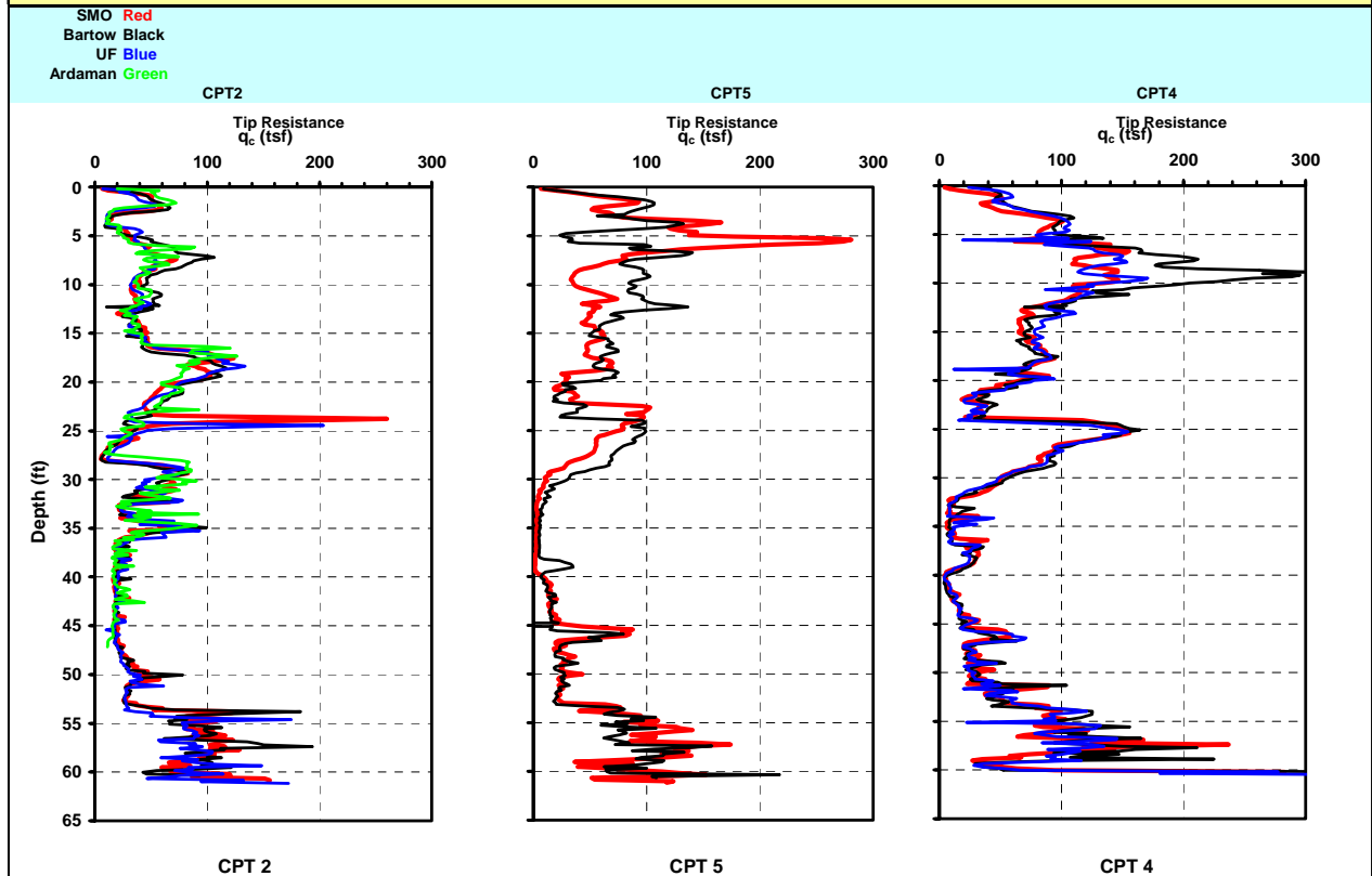
Figure 24. CPT Soundings Show Increasing Tip Resistance Along NW to SE Cross Section of the Site
