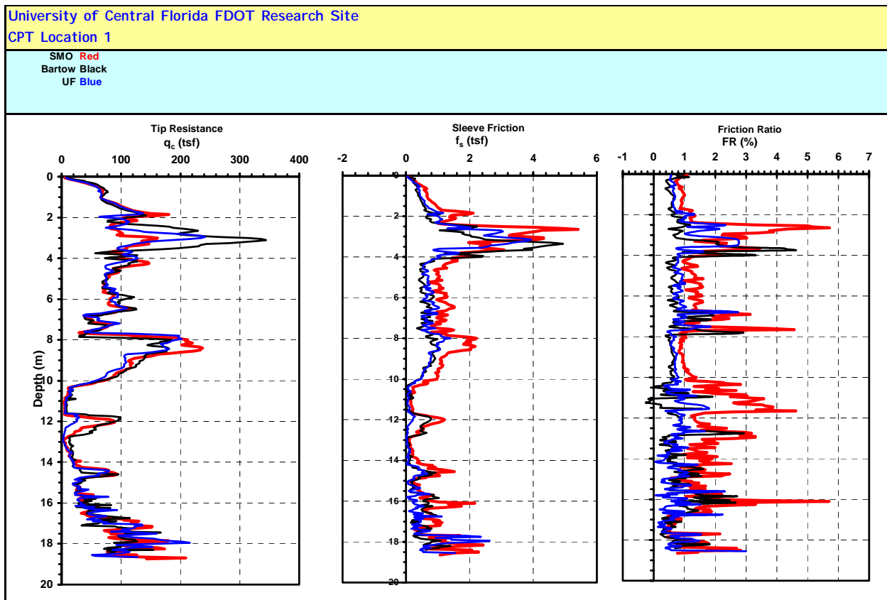
Figure 17. CPT Soundings at NE Corner Location 1
