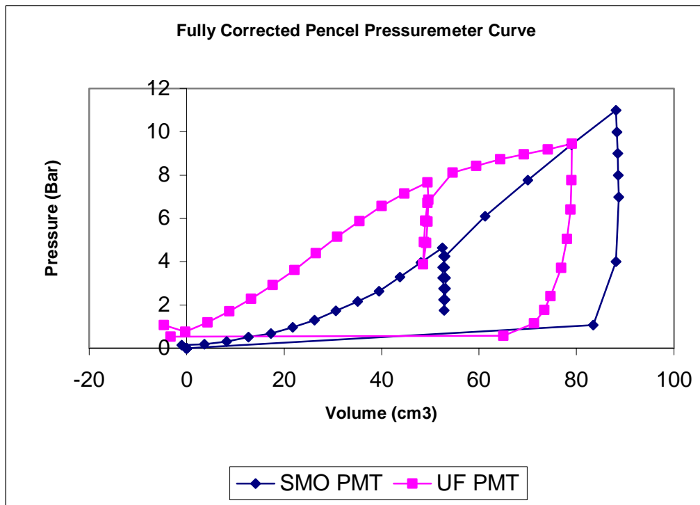
Figure 11. Comparison Graph of Data Interpretation from UF and SMO Pressuremeter at Depth 10 Feet
