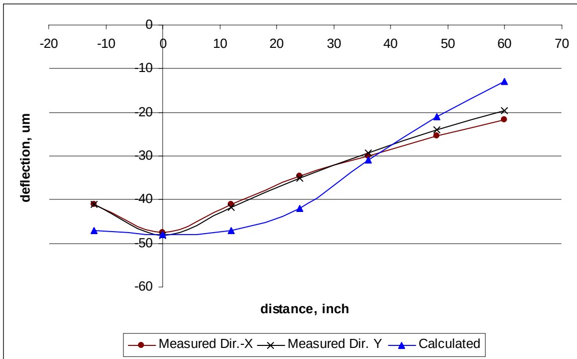
Figure 58. Measured and computed deflection basins caused by a 9-kip FWD load at slab center for Slab 2C
