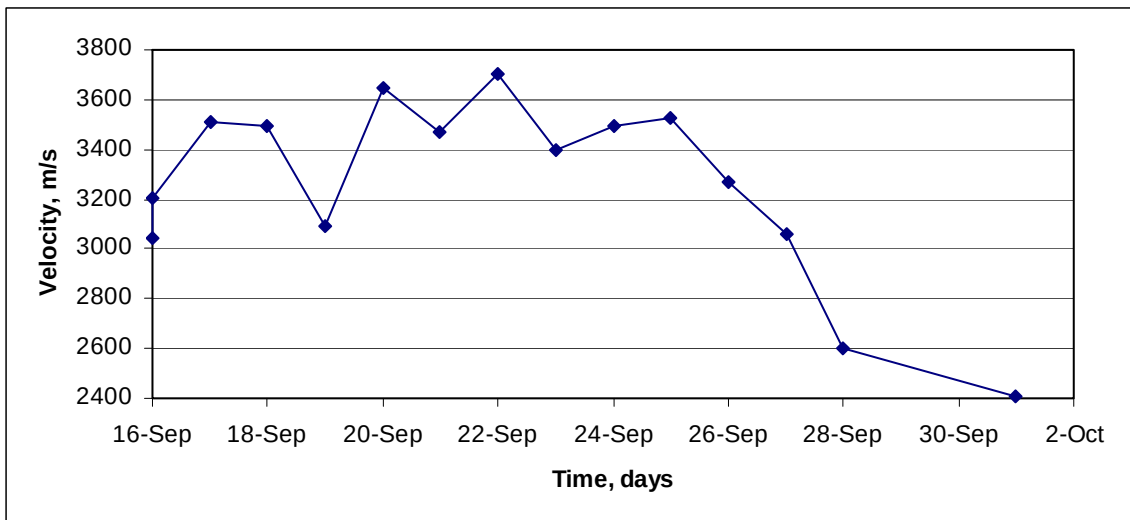
Figure 75. Measured P-wave speed along line 4 at corner of Slab 1G
