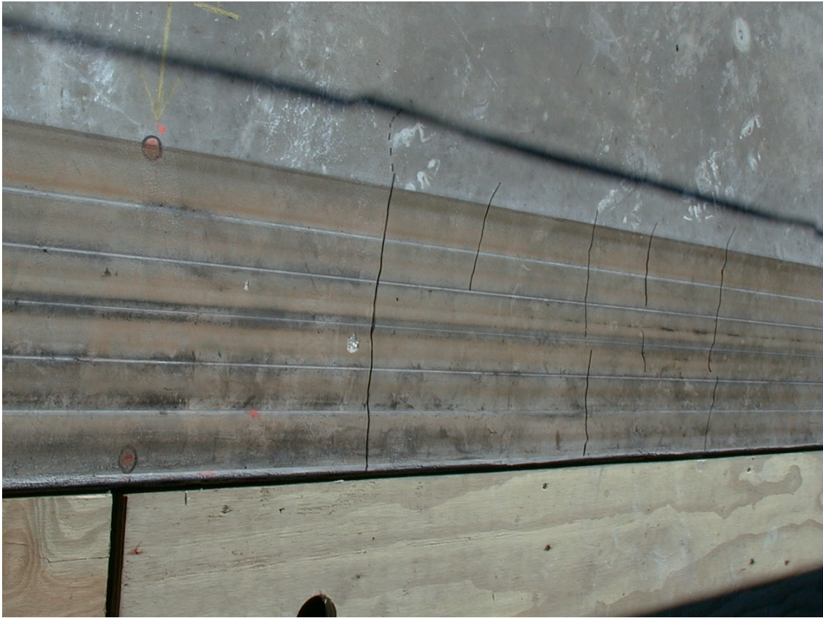
Figure 51. Cracks on Slab 2C at the end of HVS testing
