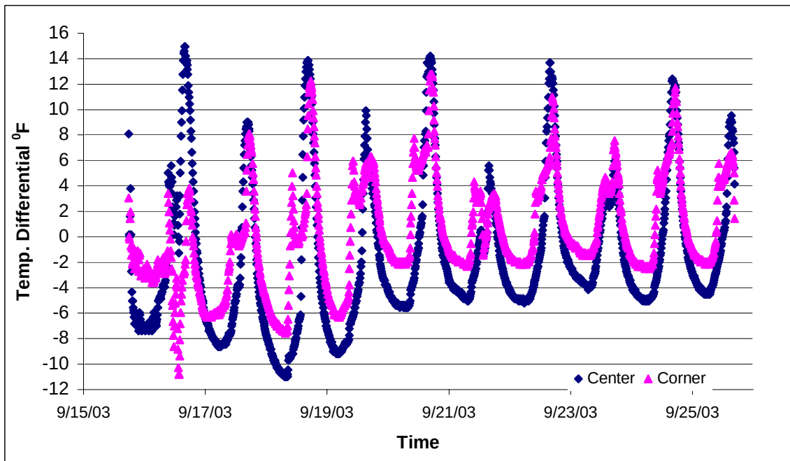
Figure 34. Temperature differentials at Slab 1G
