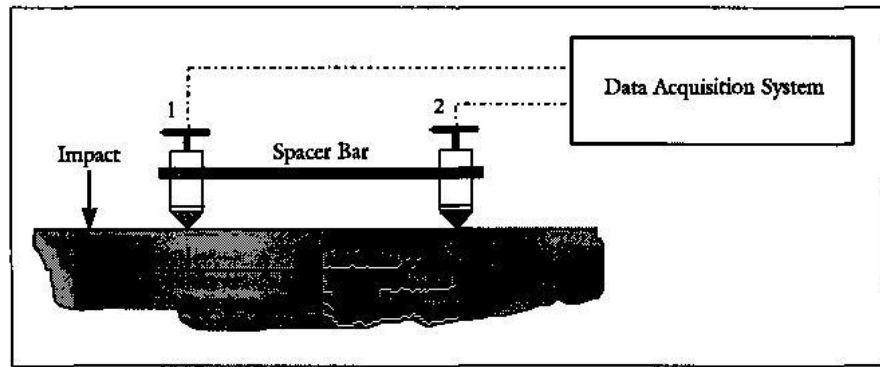
Figure 38. Schematic representation of test set-up for wave speed measurement
