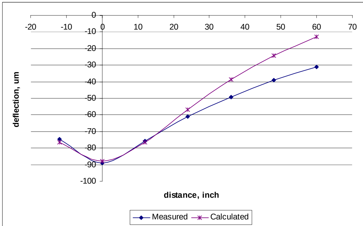
Figure 59. Measured and computed deflection basin caused by a 9-kip FWD load at slab joint for Slab 1G
