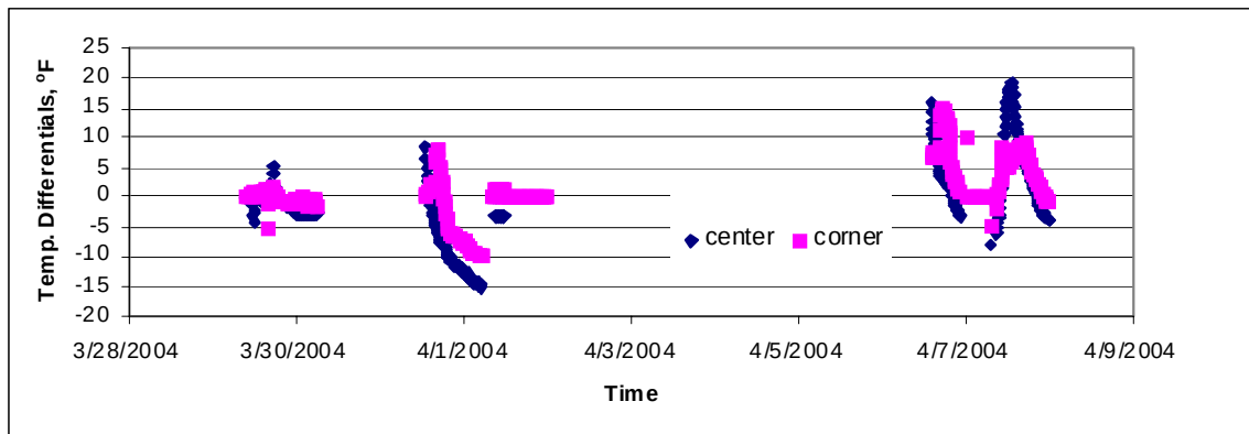
Figure 37. Temperature differentials at Slab 2G
