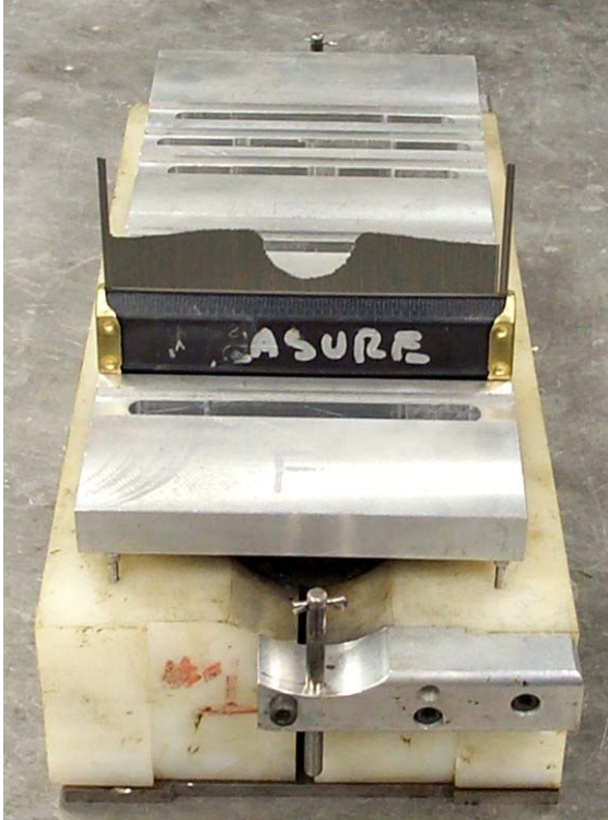
Figure 3-8 Measuring plate and contour gage for modified measuring technique
