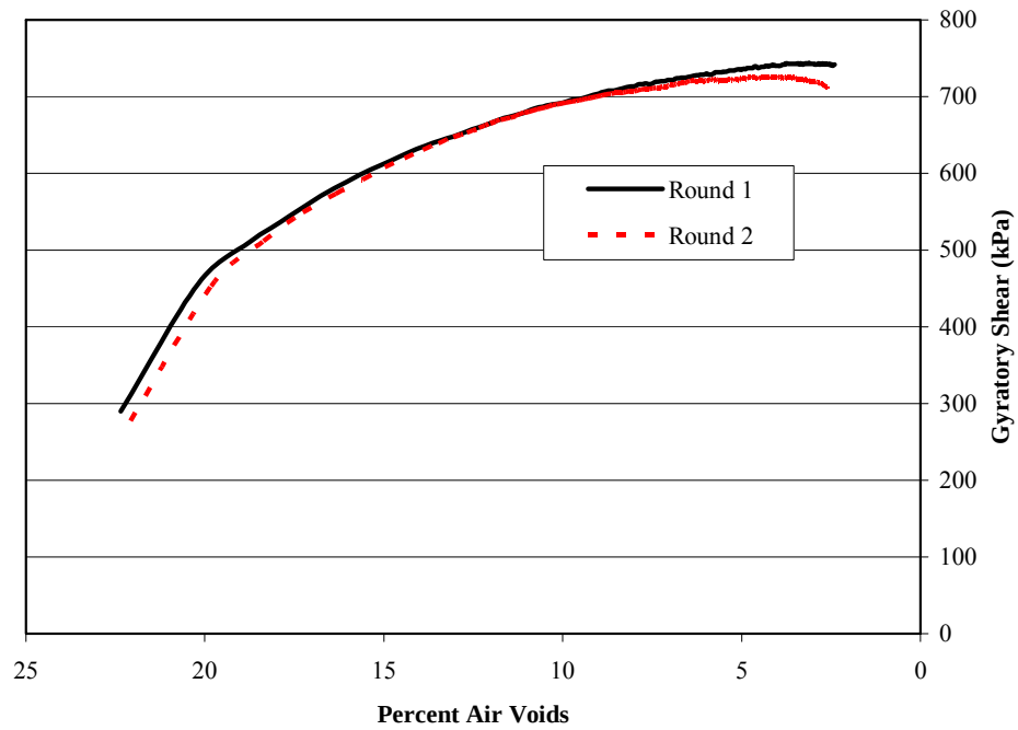
Figure 4-18 Gyratory shear versus percent air voids for Alabama limestone mixtures
