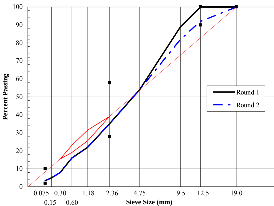
Figure 3-1 Gradation plots for Alabama limestone mixtures
