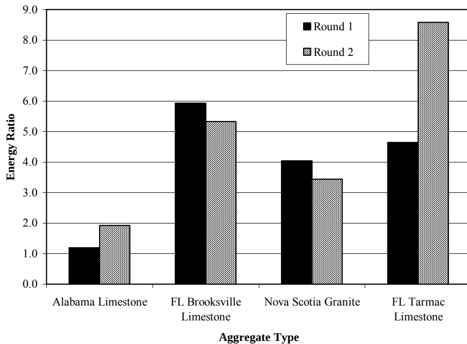
Figure 4-24 Energy ratios for long-term oven aged specimens
