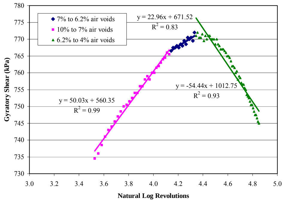
Figure 4-14 Gyratory shear slope for Florida Brooksville limestone round one mixture
