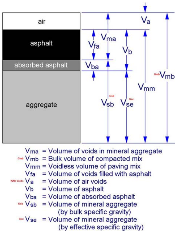
Figure 2-1. Volumetric diagram
