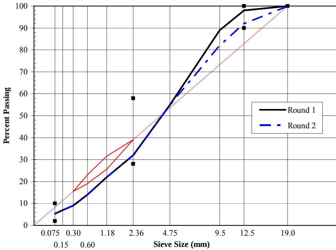
Figure 3-2 Gradation plots for Brooksville limestone mixtures
