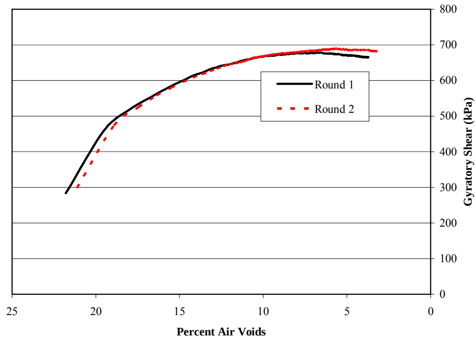
Figure 4-20 Gyratory shear versus percent air voids for Nova Scotia granite mixtures
