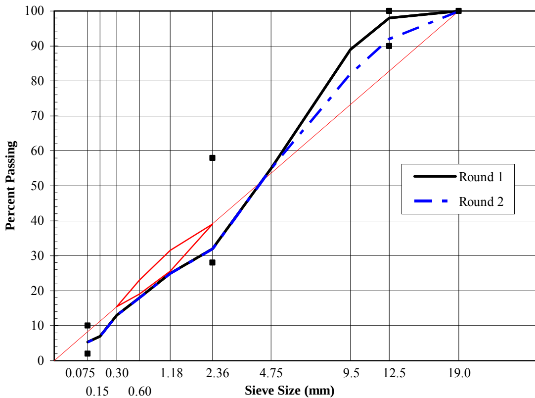
Figure 3-4 Gradation plots for Tarmac limestone mixtures
