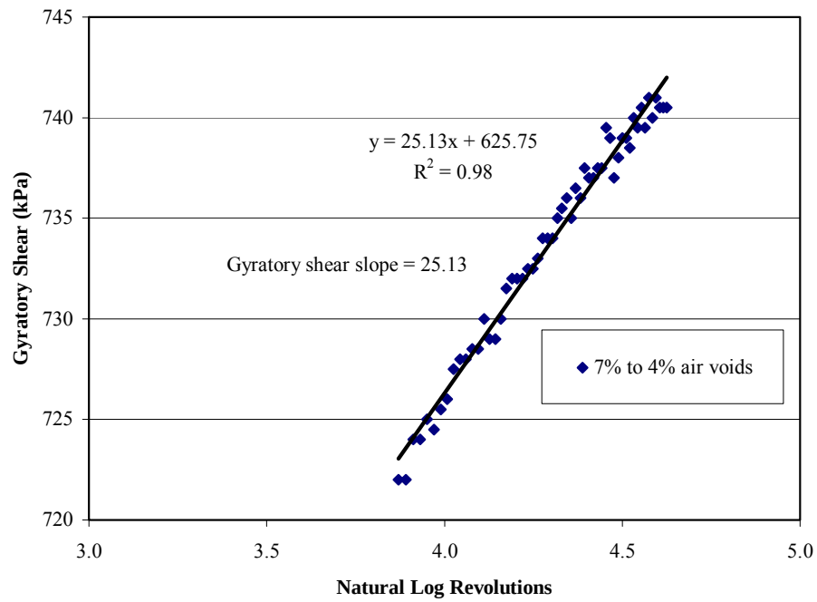
Figure 4-13 Gyratory shear slope for Alabama limestone round one mixture
