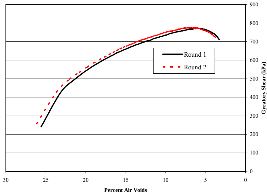
Figure 4-19 Gyratory shear versus percent air voids for Florida Brooksville limestone mixtures
