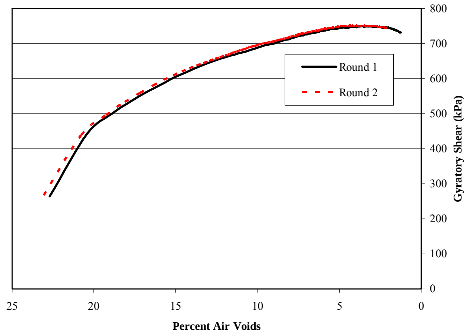
Figure 4-21 Gyratory shear versus percent air voids for Florida Tarmac limestone mixtures
