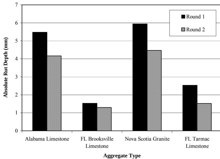
Figure 4-6 APA absolute rut depth using conventional measuring device for 7% air voids, 75 mm tall specimens
